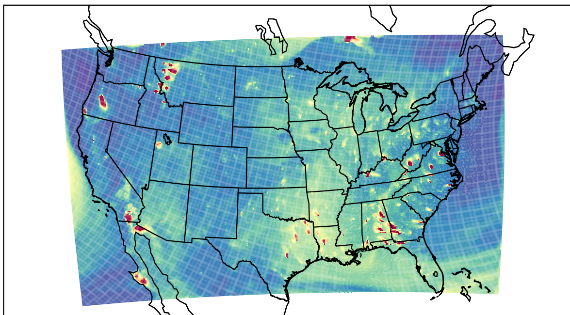
WRF 2023-08-03_02:00:00
