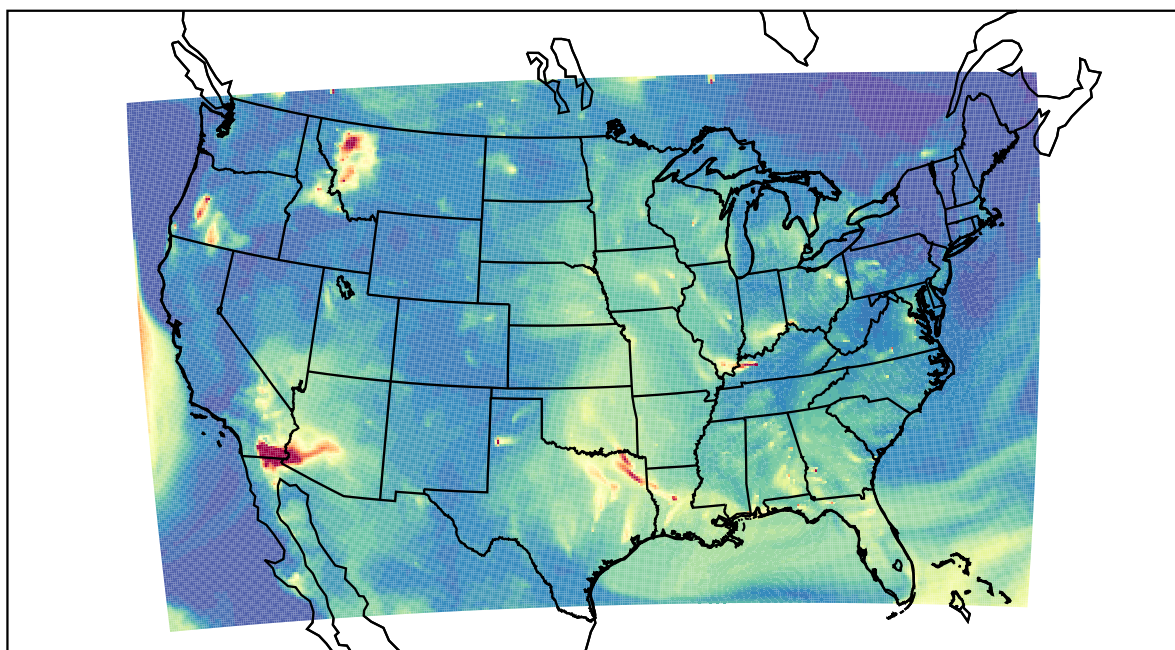
WRF 2023-08-02_08:00:00
