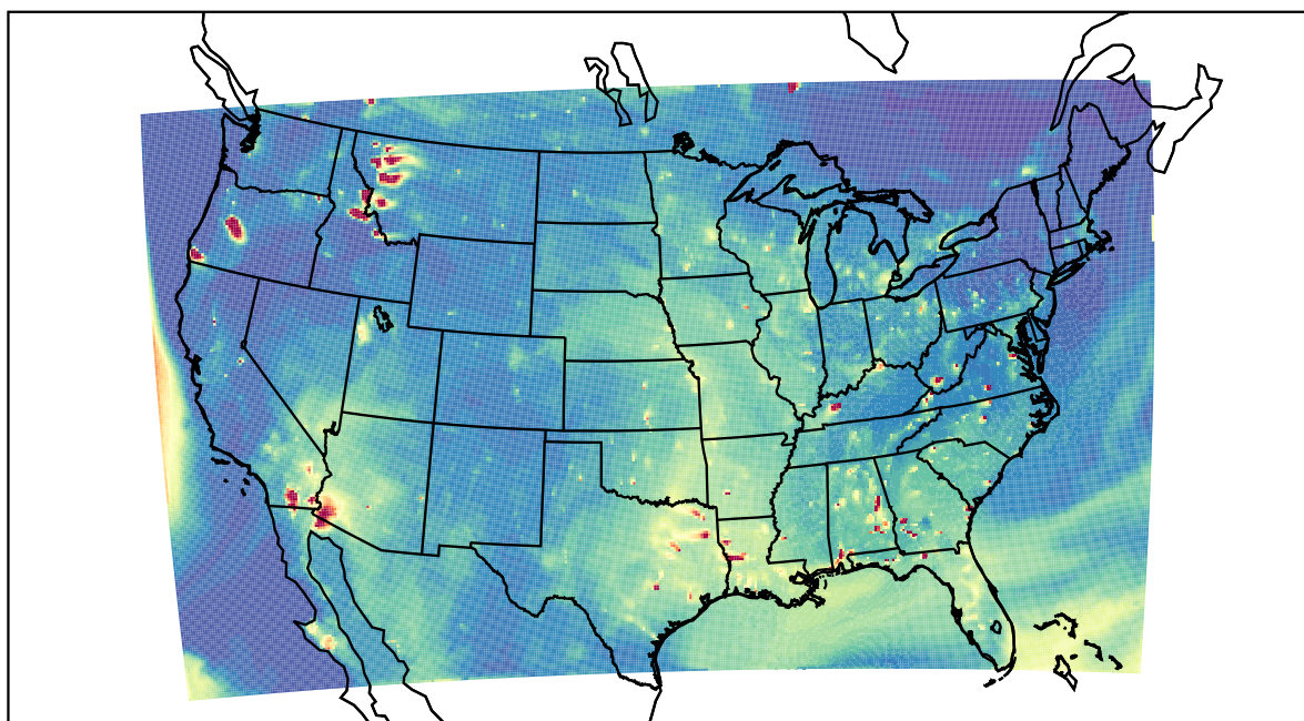
WRF 2023-08-02_02:00:00
