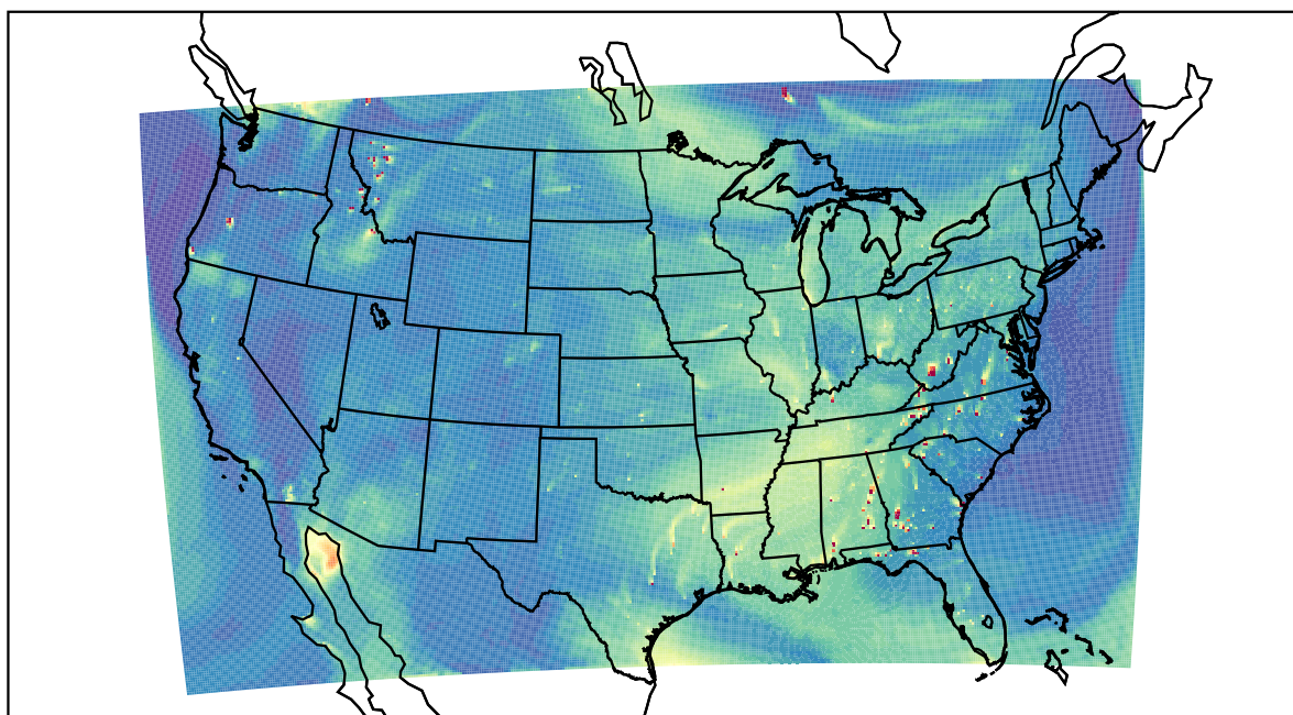
WRF 2023-08-03_21:00:00
