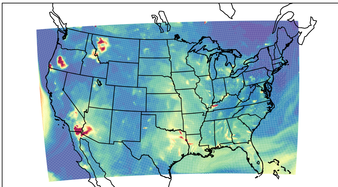
WRF 2023-08-02_05:00:00
