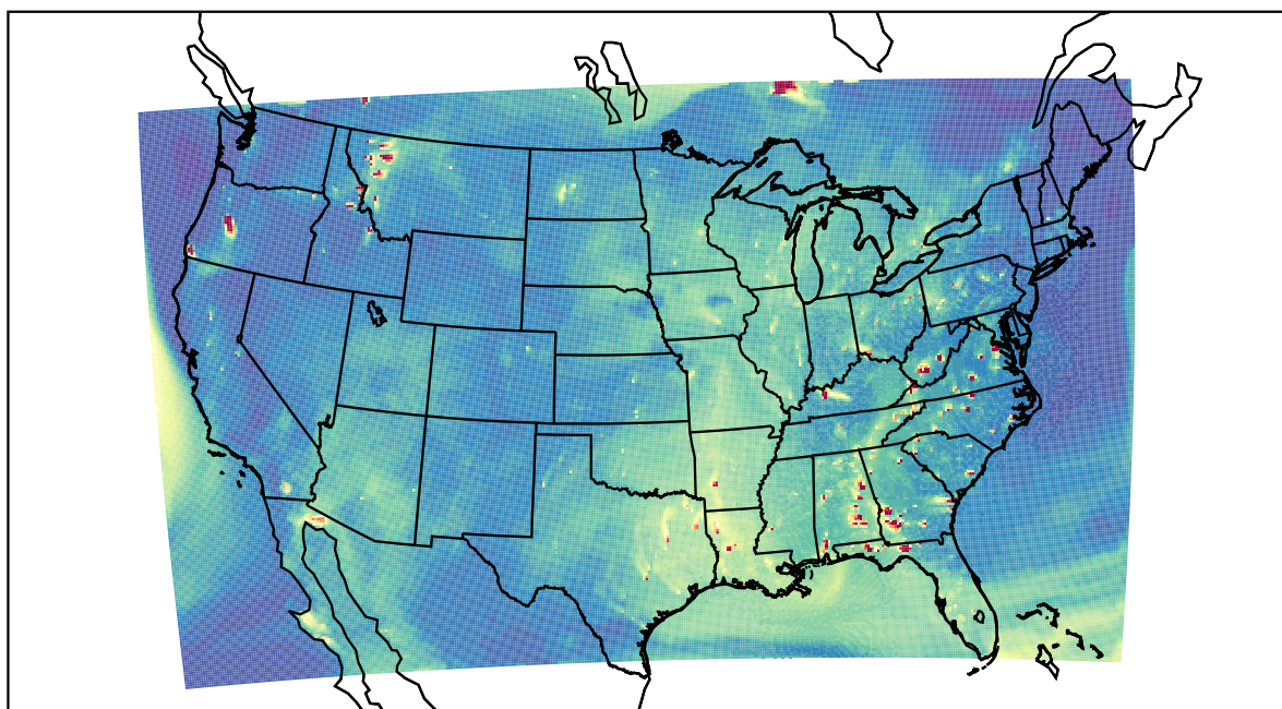
WRF 2023-08-03_00:00:00
