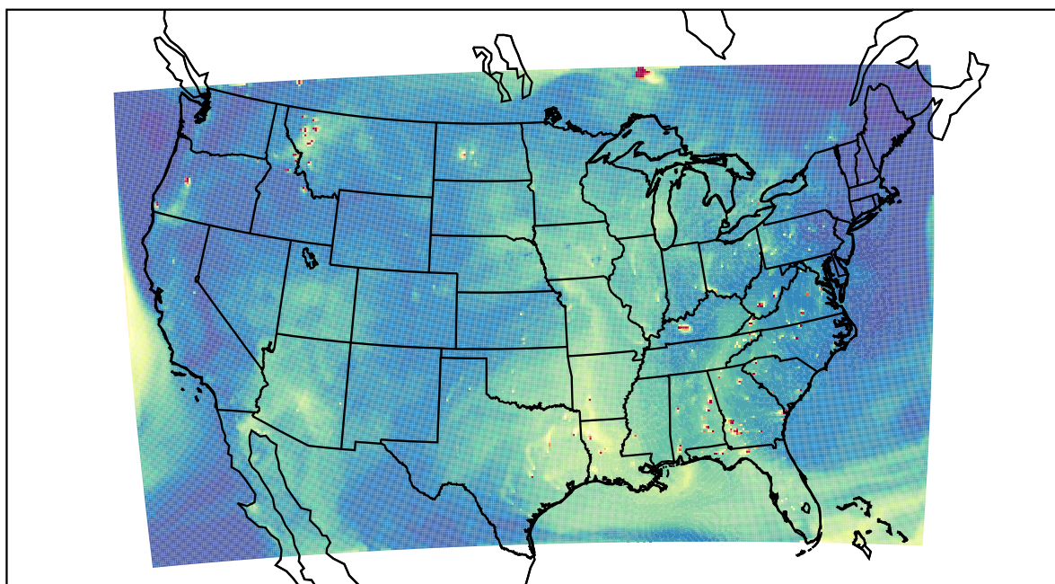
WRF 2023-08-02_21:00:00
