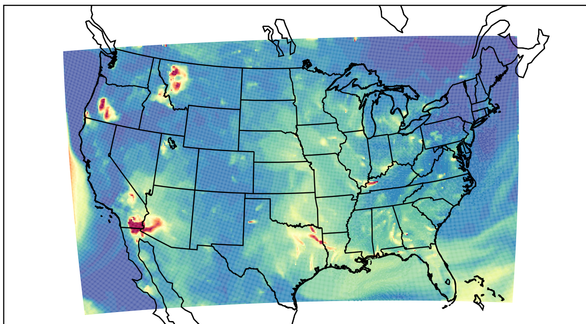
WRF 2023-08-02_06:00:00
