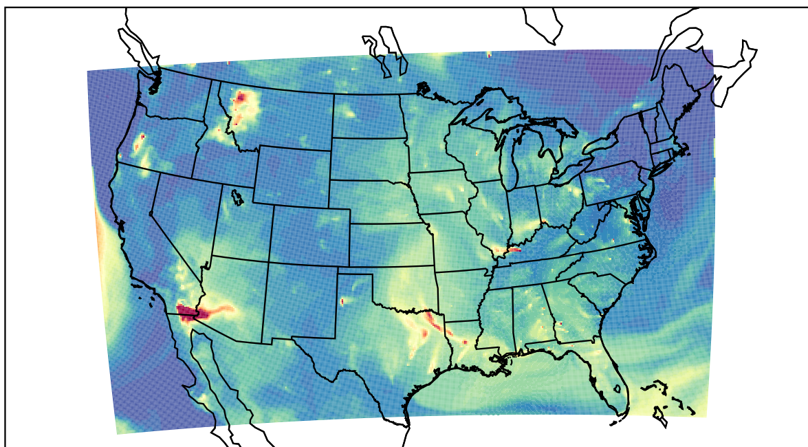
WRF 2023-08-02_09:00:00
