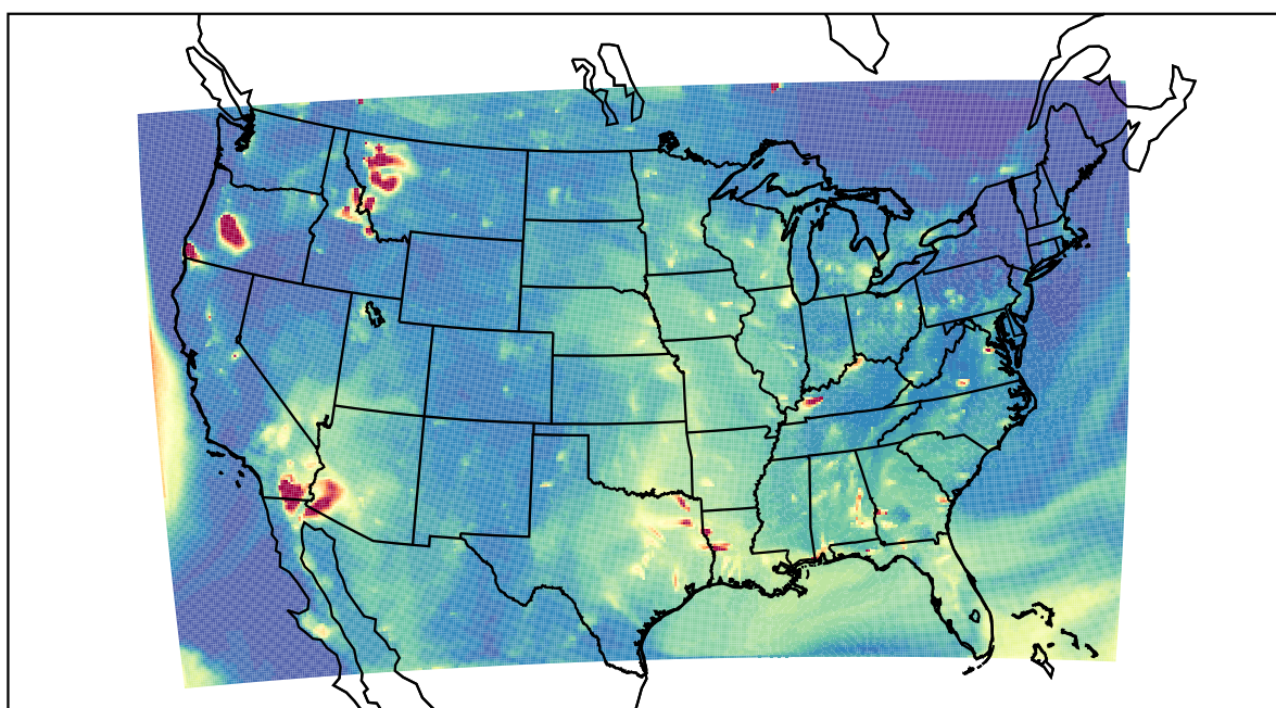
WRF 2023-08-02_04:00:00
