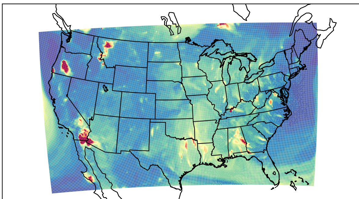
WRF 2023-08-03_05:00:00
