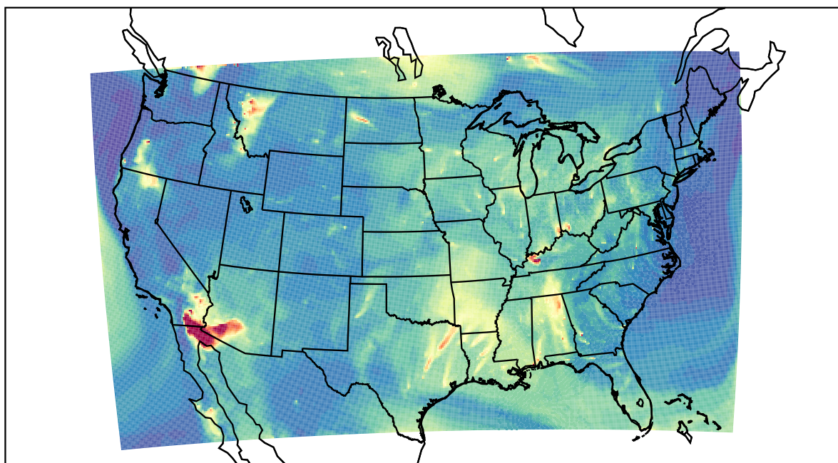
WRF 2023-08-03_11:00:00
