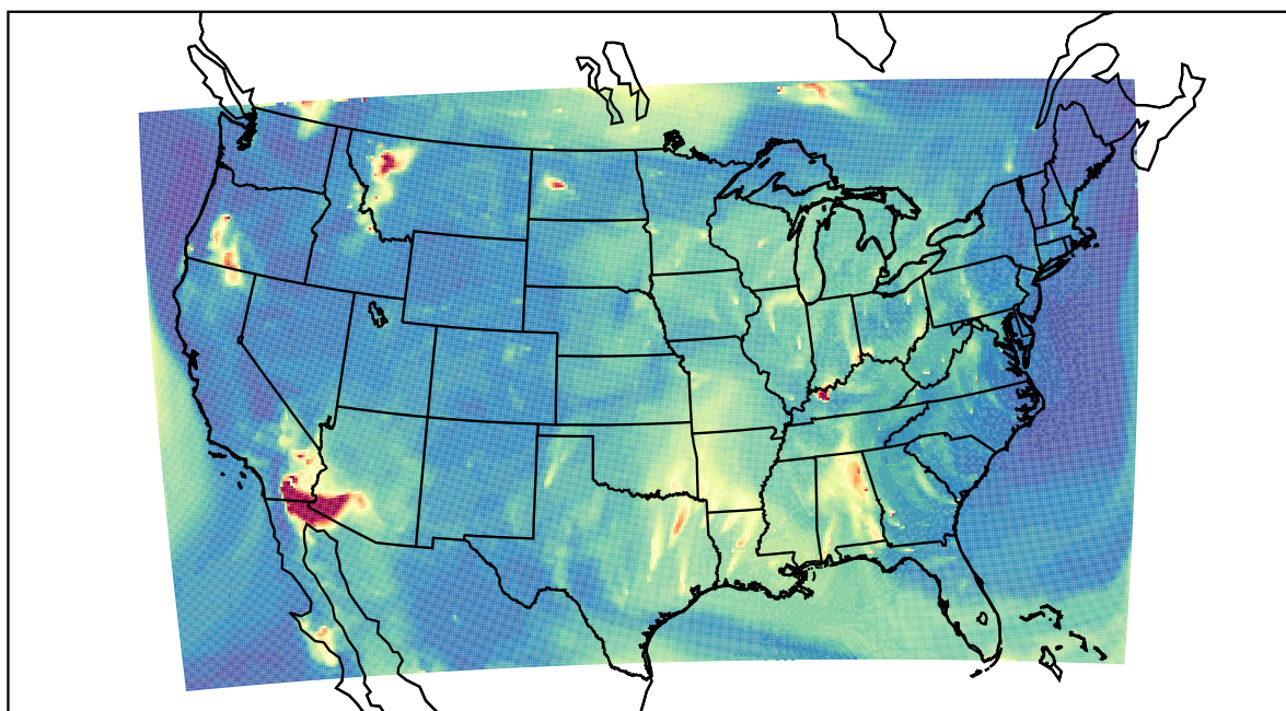
WRF 2023-08-03_09:00:00
