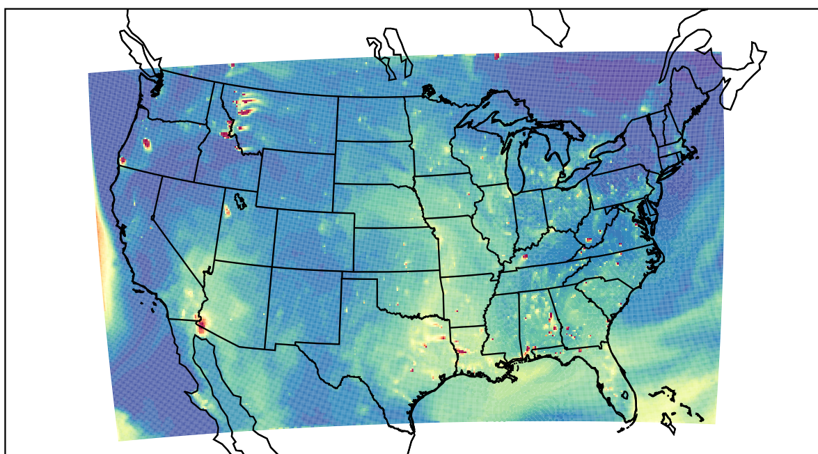
WRF 2023-08-02_01:00:00
