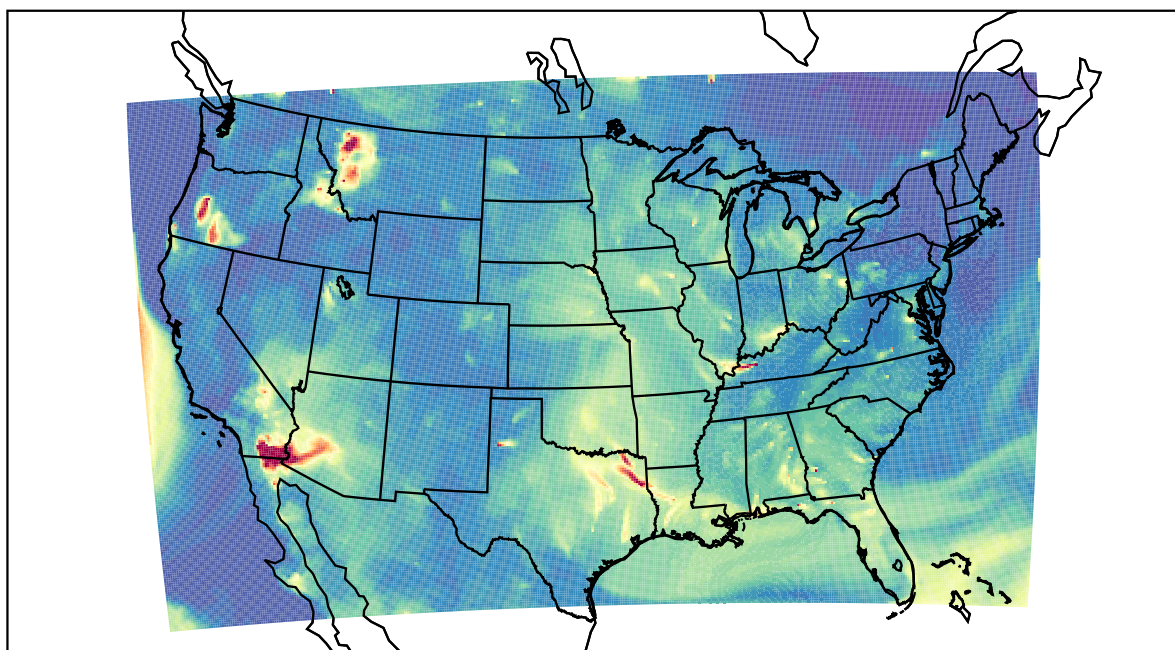
WRF 2023-08-02_07:00:00
