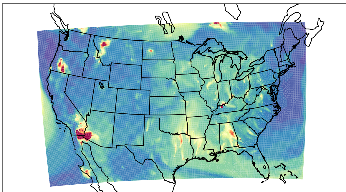
WRF 2023-08-03_07:00:00
