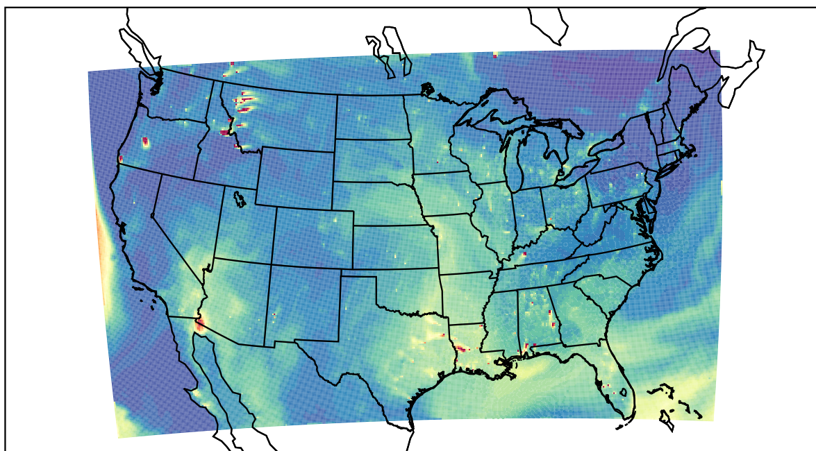
WRF 2023-08-02_00:00:00
