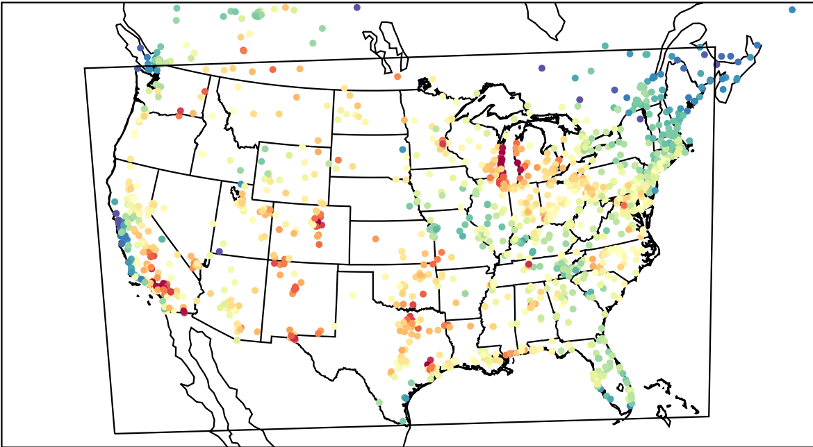
AirNOW (2023-08-02_21:00:00)
