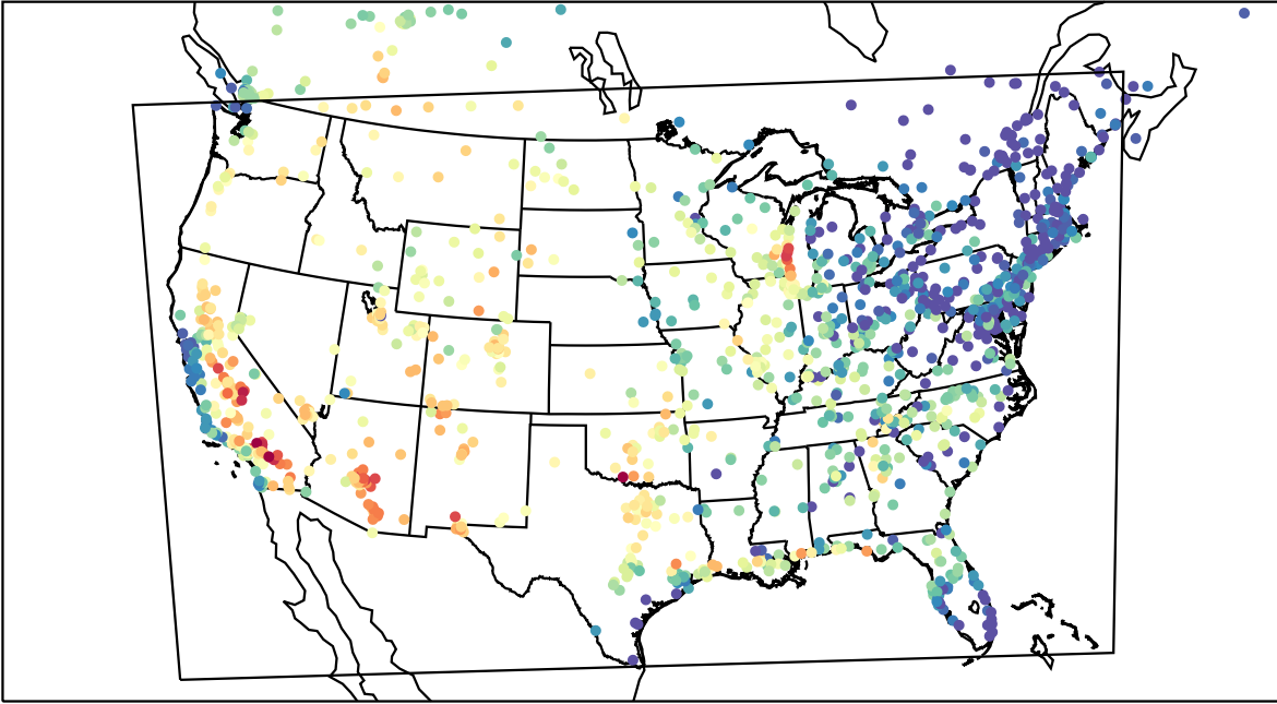
AirNOW (2023-08-02_01:00:00)
