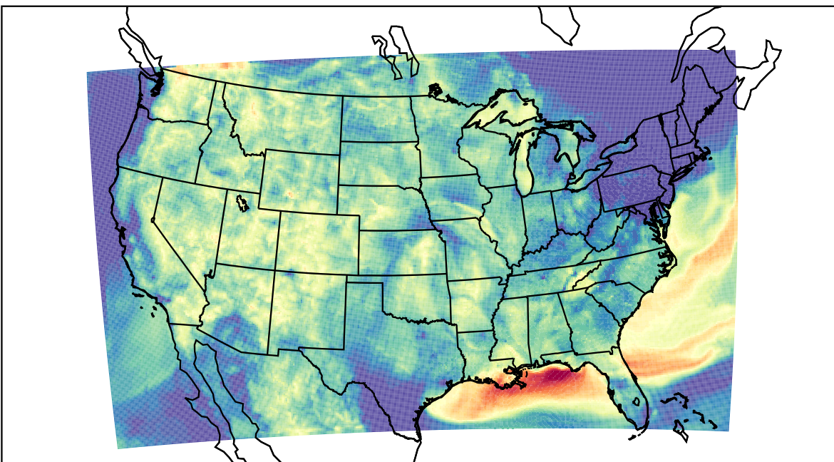
WRF (2023-08-02_11:00:00)
