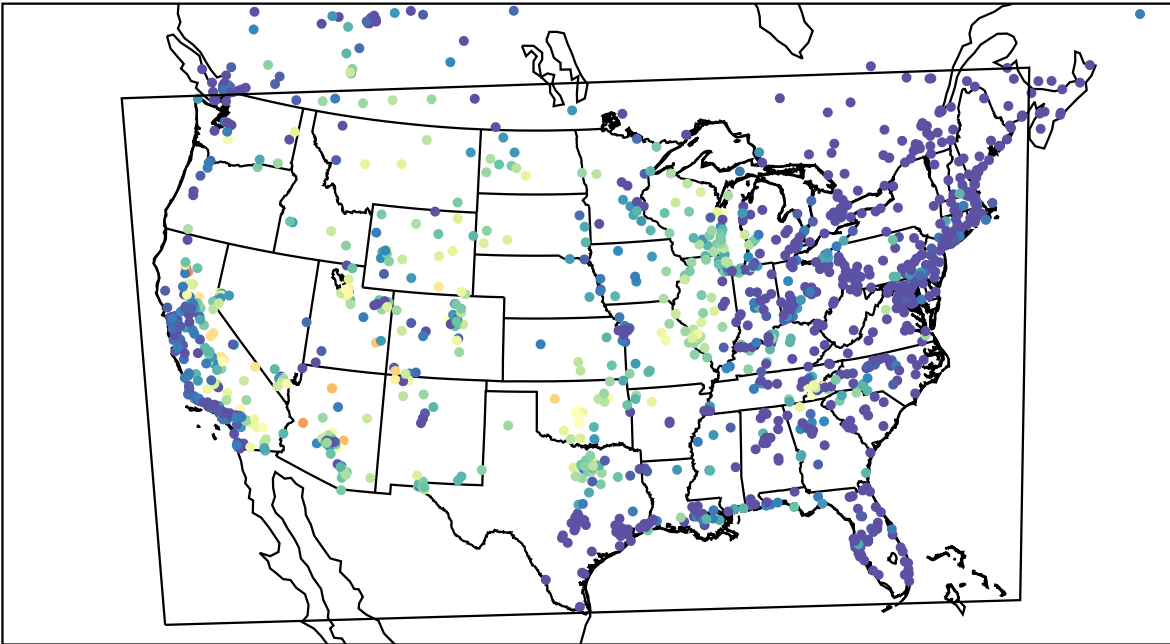
AirNOW (2023-08-02_07:00:00)
