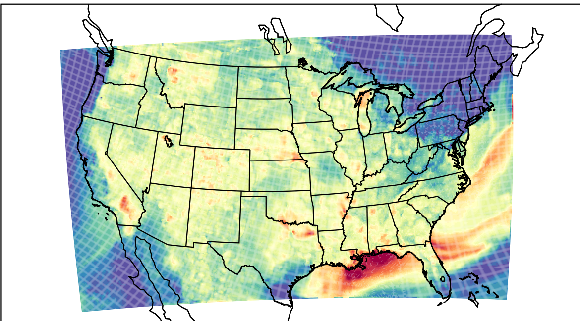
WRF (2023-08-02_03:00:00)
