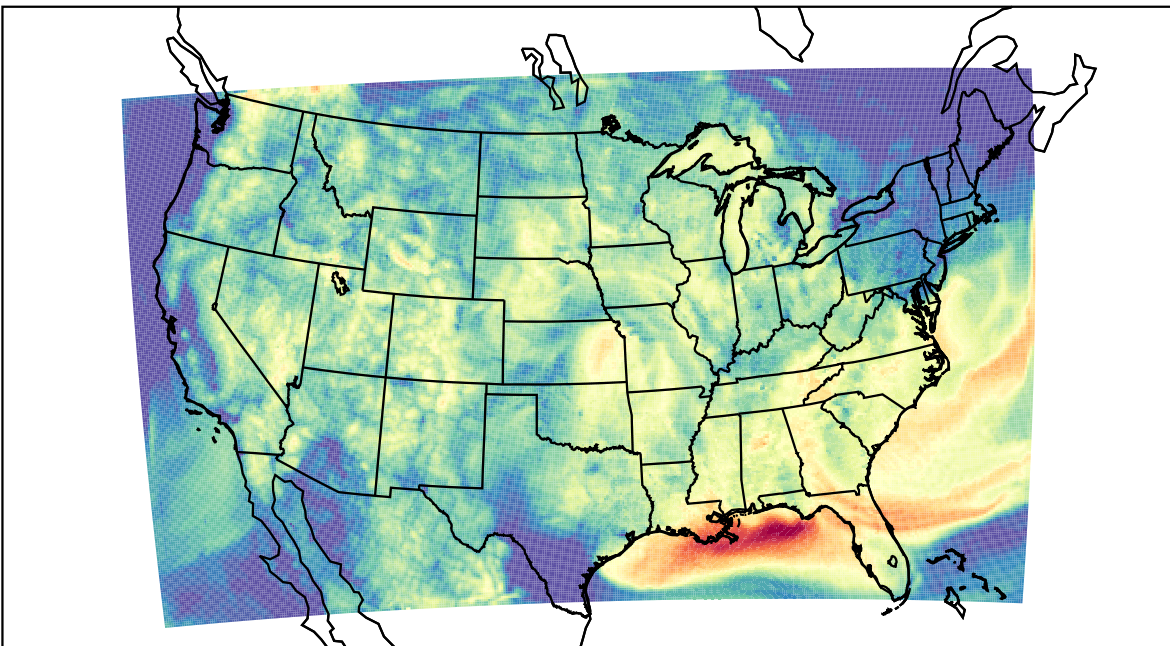
WRF (2023-08-02_14:00:00)
