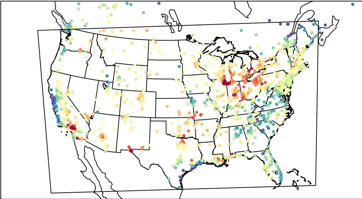
AirNOW (2023-08-03_21:00:00)
