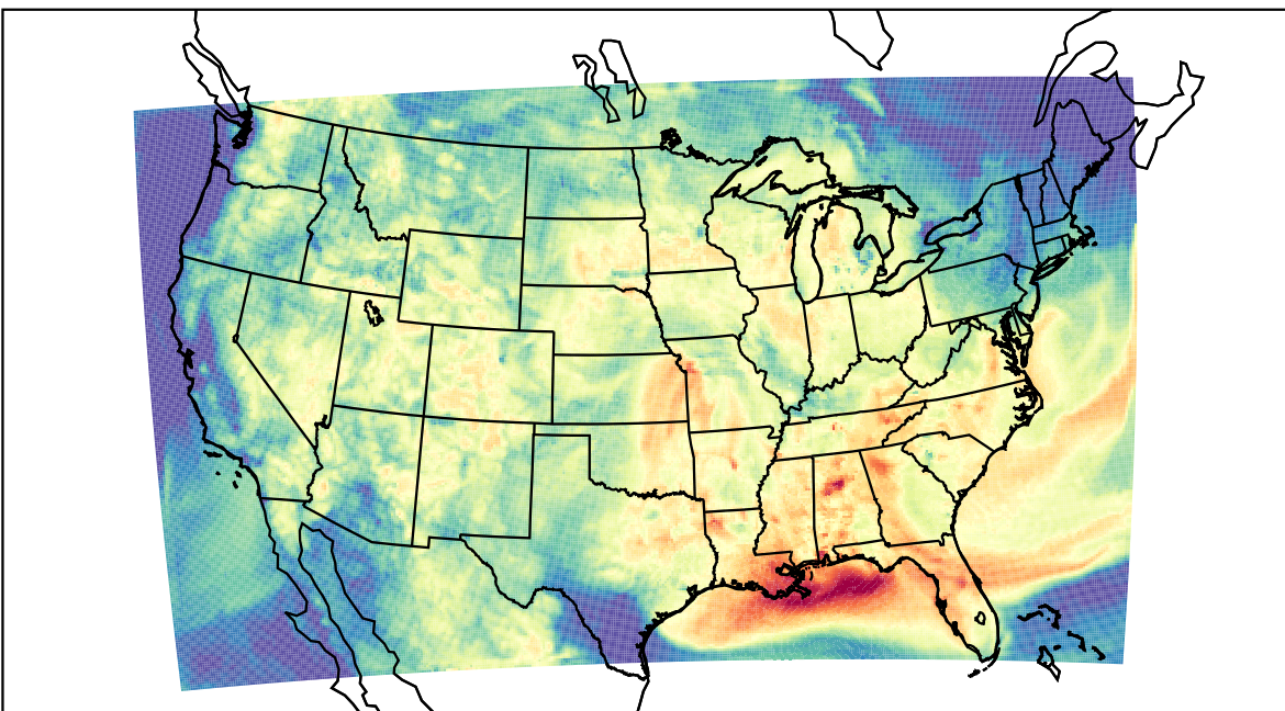
WRF (2023-08-02_15:00:00)
