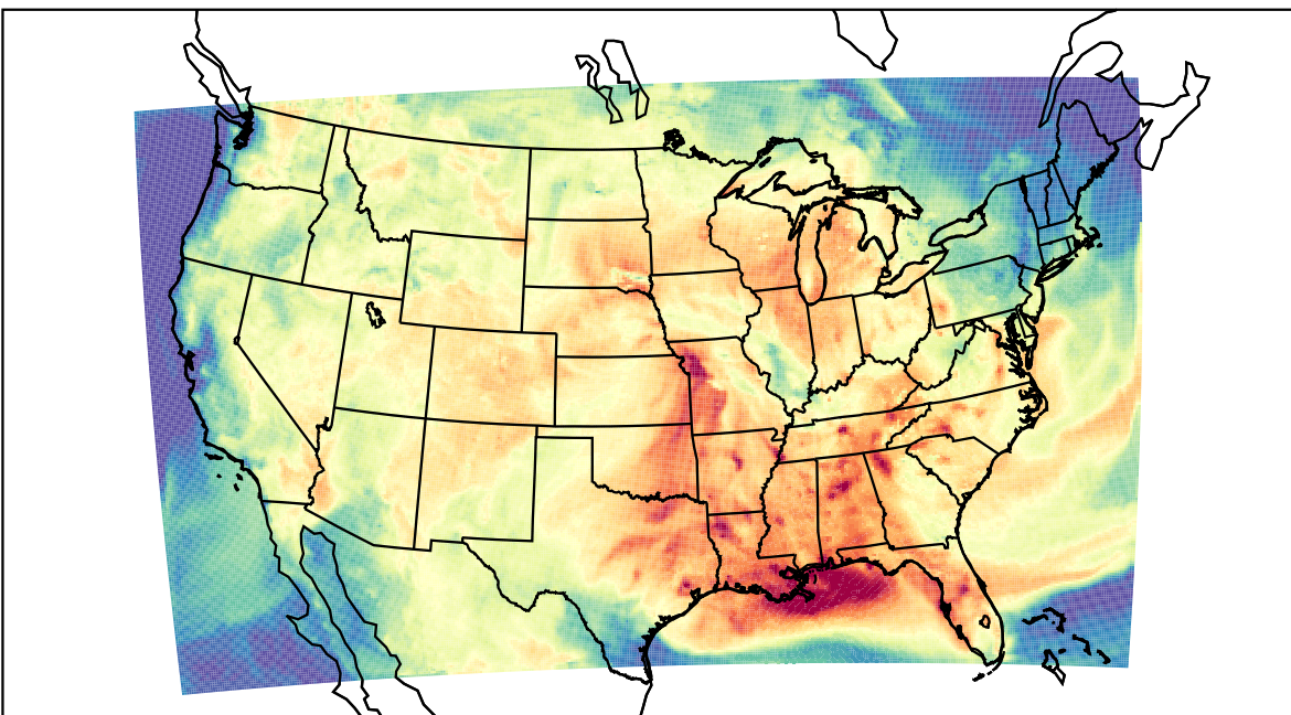
WRF (2023-08-02_17:00:00)
