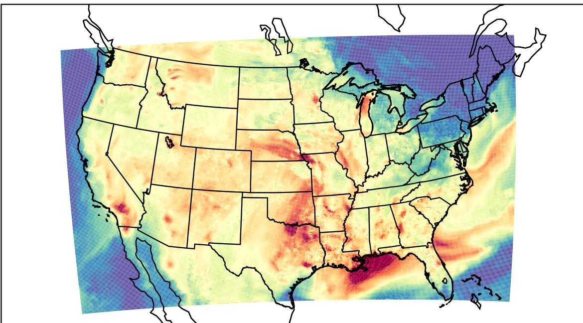
WRF (2023-08-02_00:00:00)
