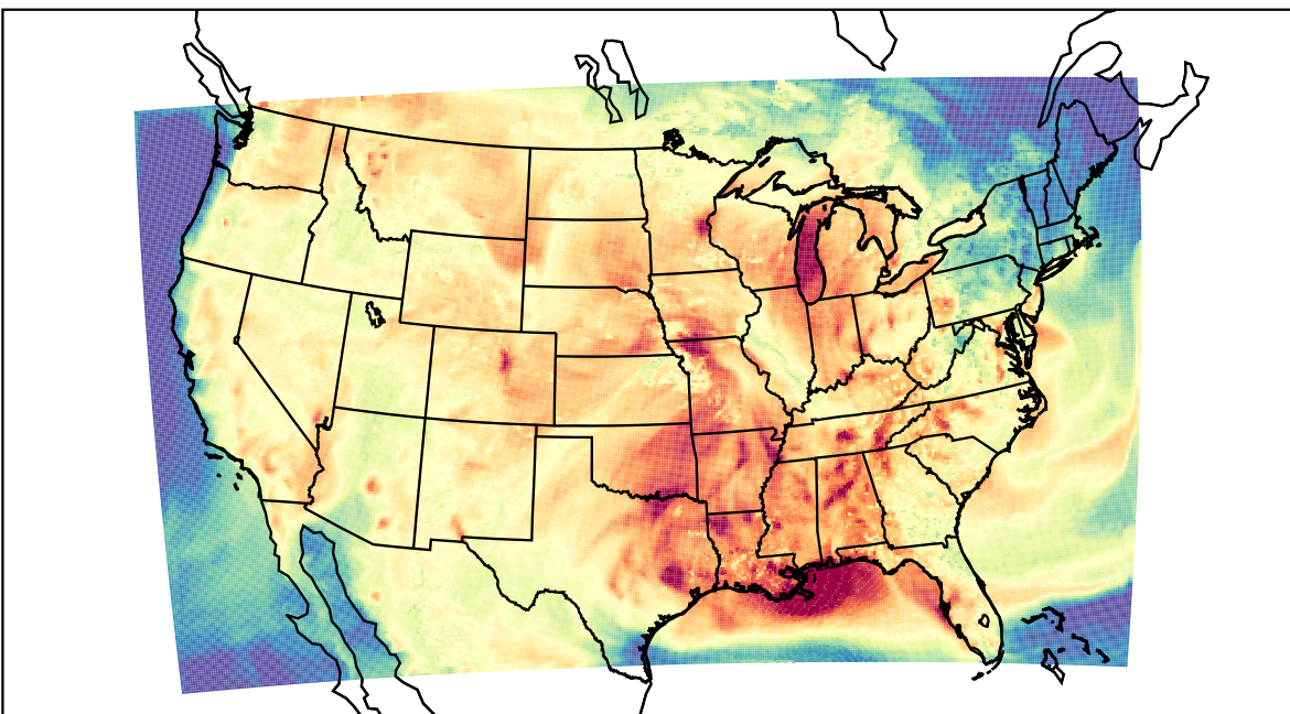
WRF (2023-08-02_22:00:00)
