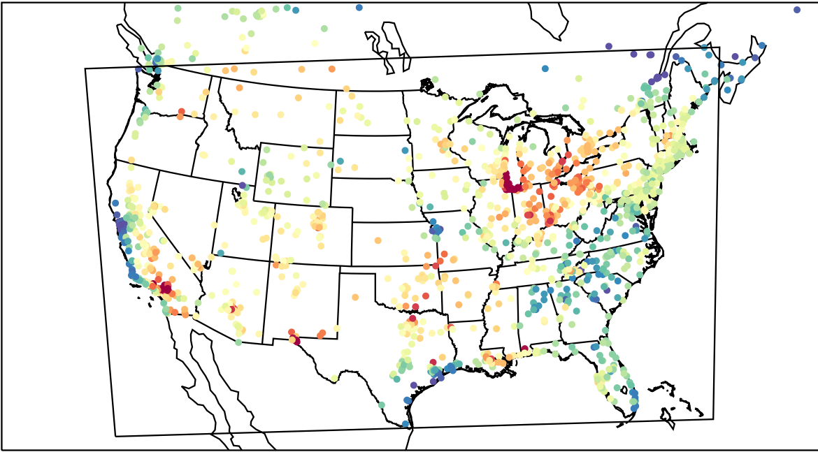
AirNOW (2023-08-03_22:00:00)
