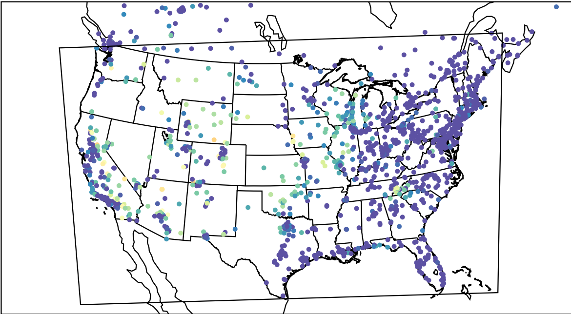
AirNOW (2023-08-02_11:00:00)
