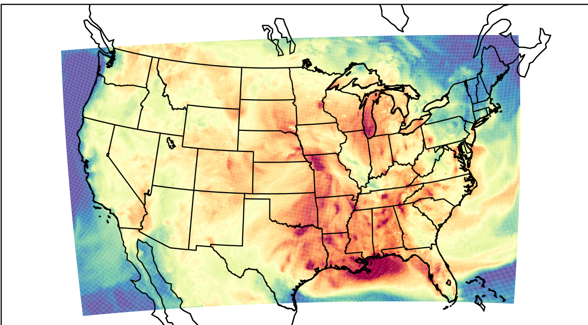
WRF (2023-08-02_19:00:00)
