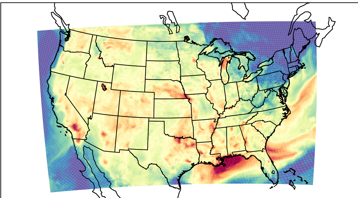
WRF (2023-08-02_01:00:00)
