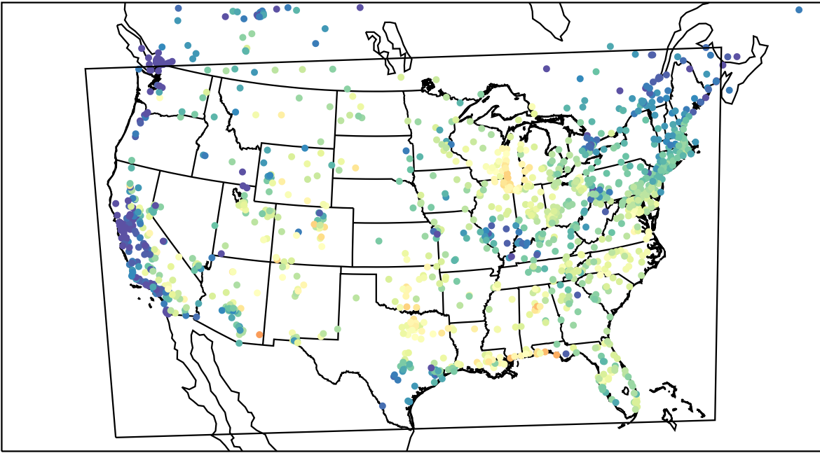
AirNOW (2023-08-02_15:00:00)
