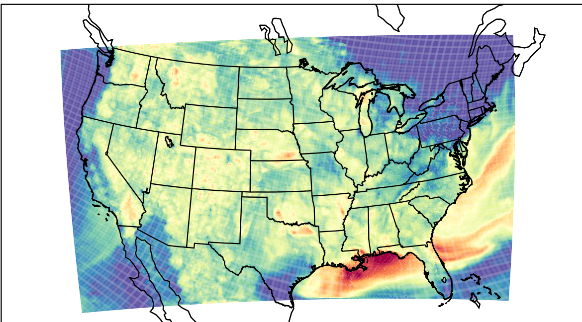
WRF (2023-08-02_05:00:00)
