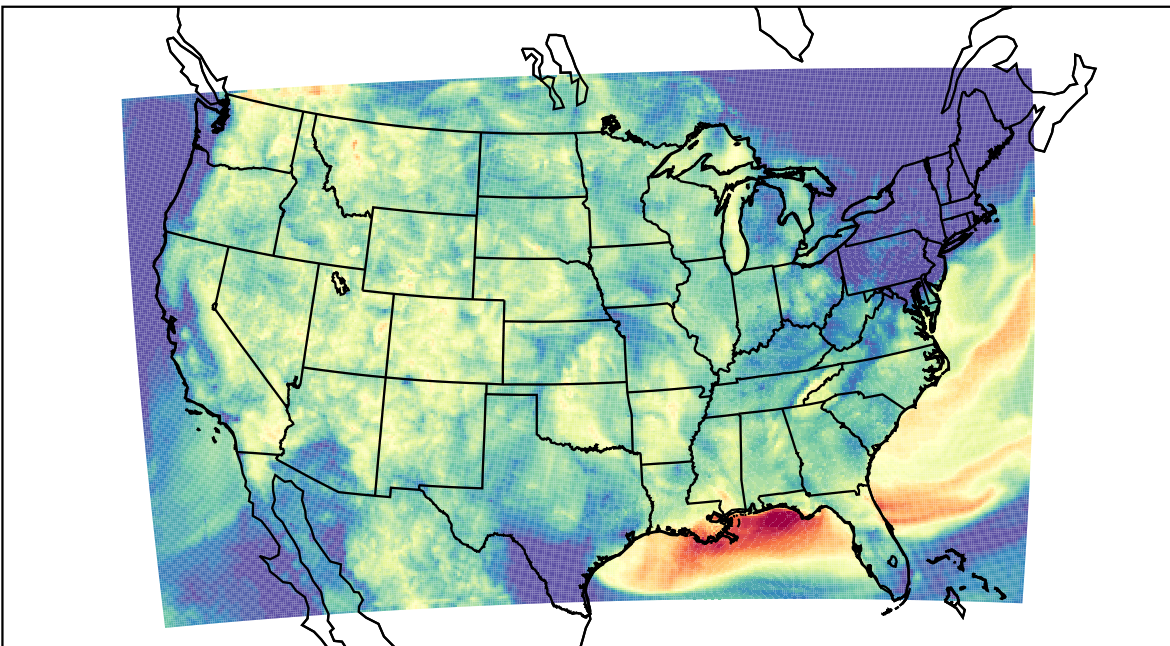
WRF (2023-08-02_09:00:00)
