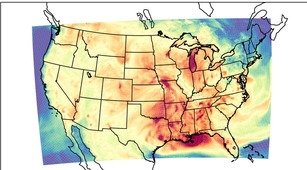
WRF (2023-08-02_21:00:00)
