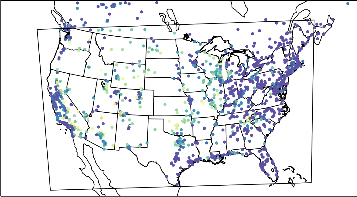
AirNOW (2023-08-02_09:00:00)
