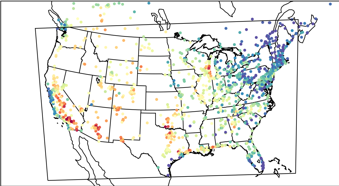
AirNOW (2023-08-02_00:00:00)
