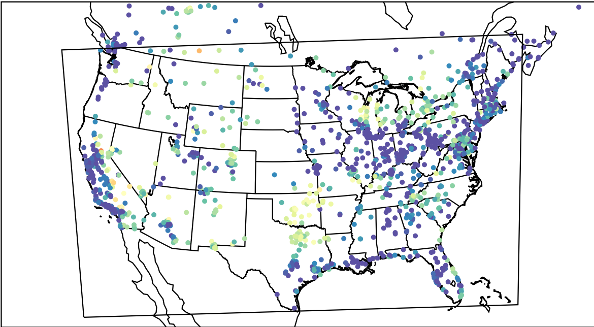
AirNOW (2023-08-03_08:00:00)
