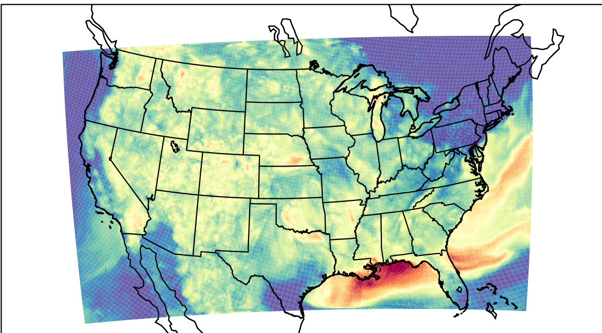
WRF (2023-08-02_06:00:00)
