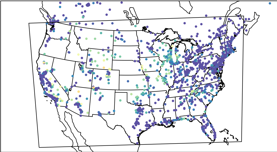
AirNOW (2023-08-02_12:00:00)
