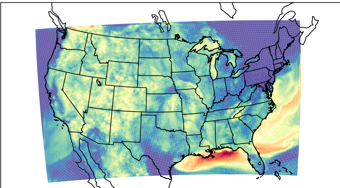
WRF (2023-08-02_12:00:00)
