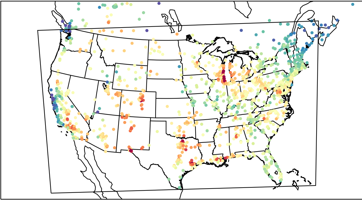
AirNOW (2023-08-02_19:00:00)
