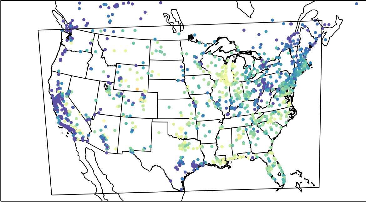
AirNOW (2023-08-02_14:00:00)
