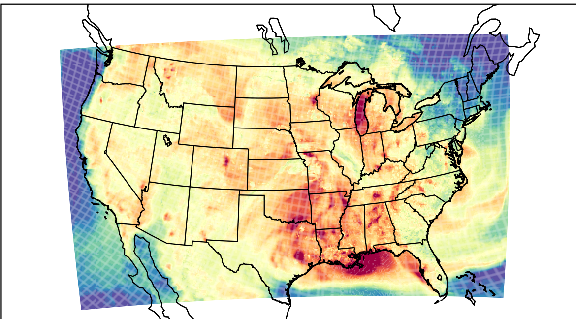
WRF (2023-08-02_23:00:00)
