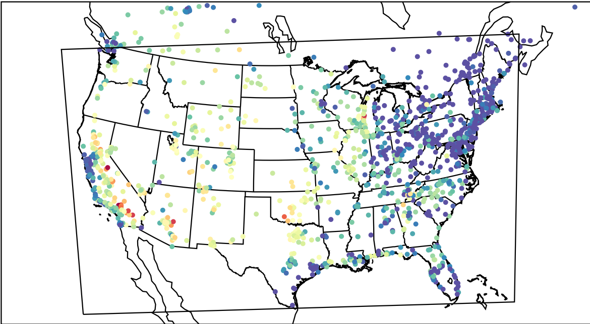
AirNOW (2023-08-02_03:00:00)
