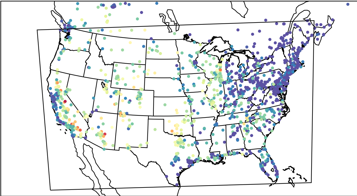
AirNOW (2023-08-02_04:00:00)
