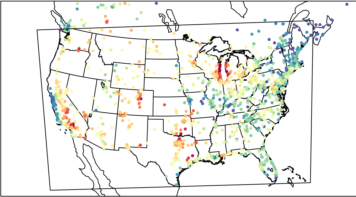
AirNOW (2023-08-02_23:00:00)
