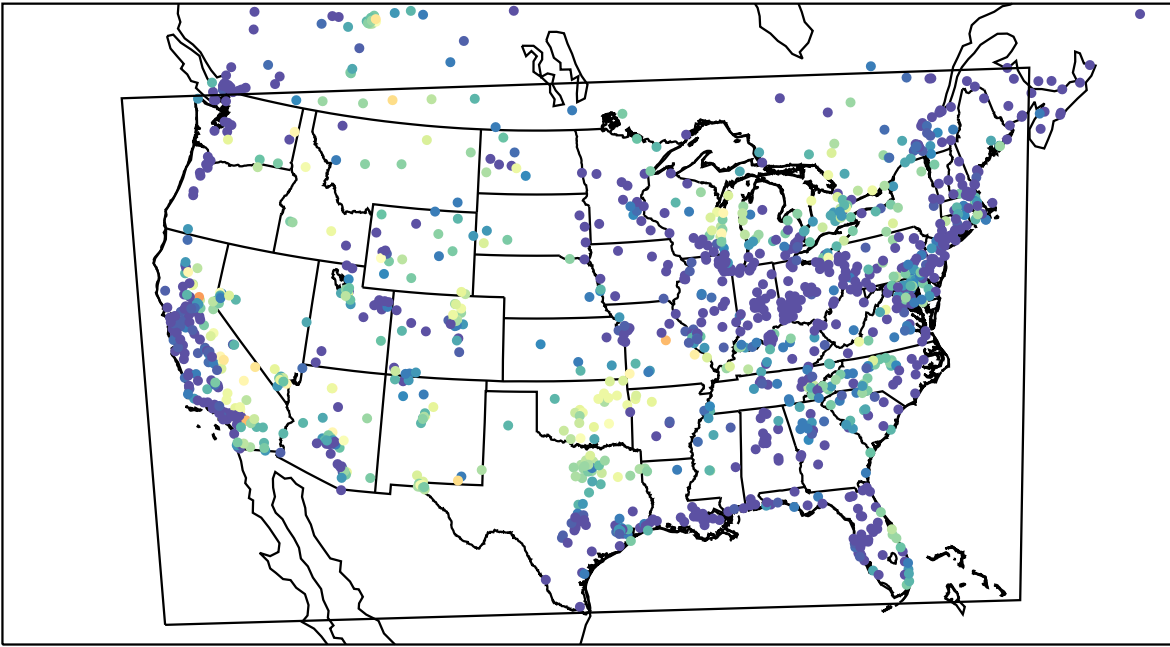
AirNOW (2023-08-03_09:00:00)
