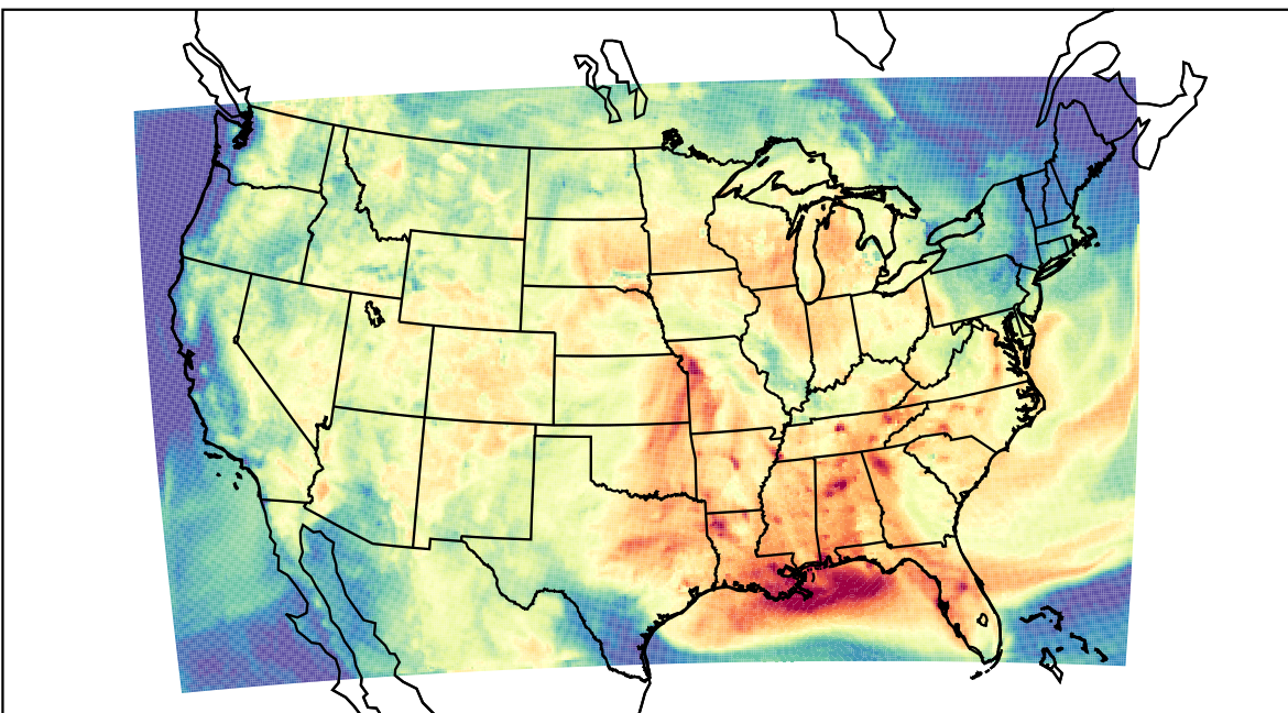
WRF (2023-08-02_16:00:00)
