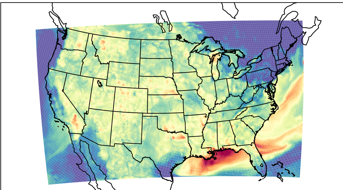
WRF (2023-08-02_04:00:00)
