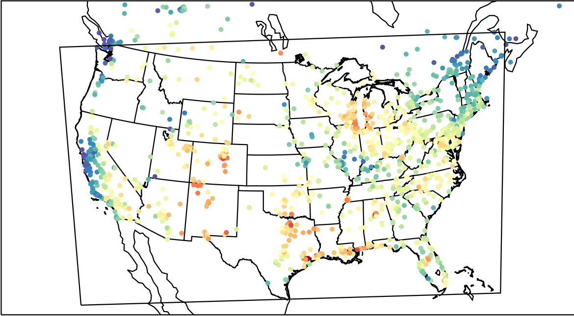
AirNOW (2023-08-02_17:00:00)
