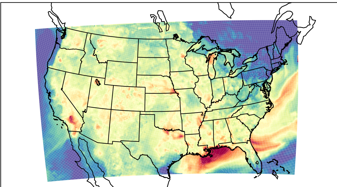
WRF (2023-08-02_02:00:00)
