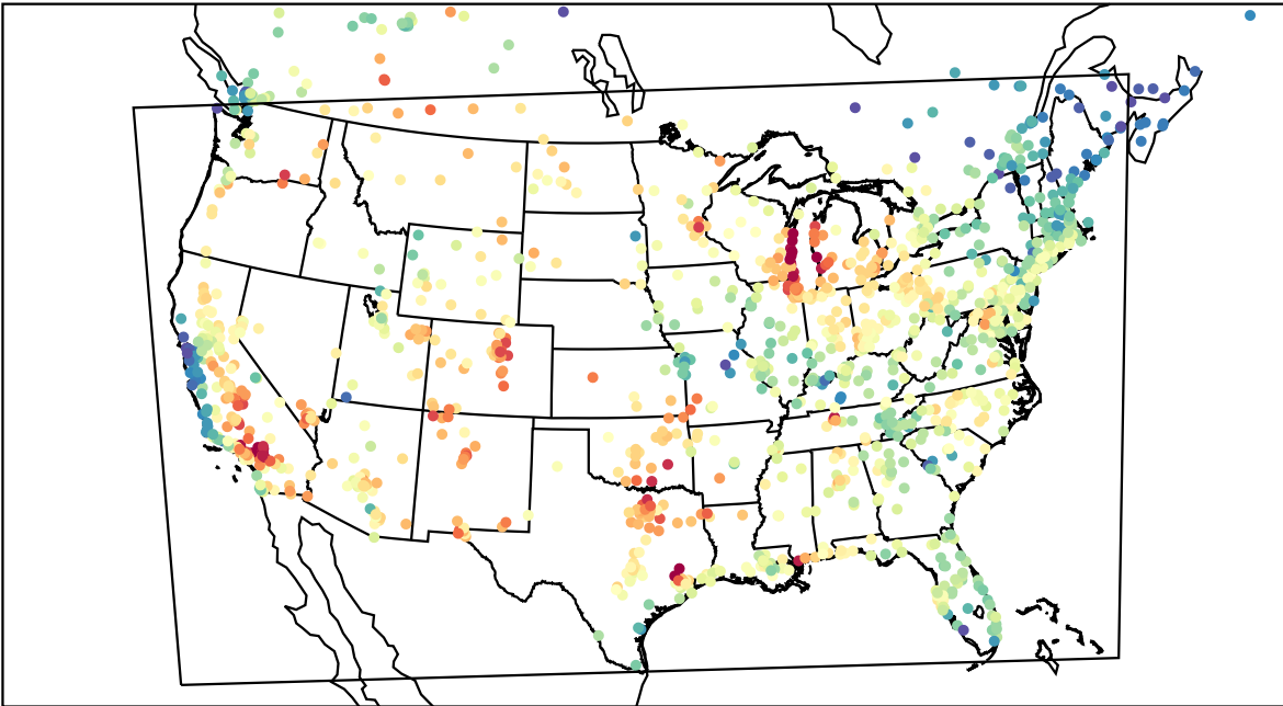
AirNOW (2023-08-02_22:00:00)
