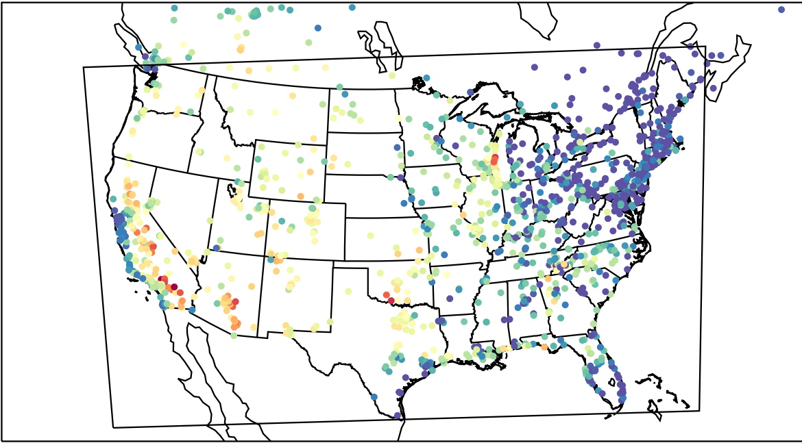
AirNOW (2023-08-02_02:00:00)
