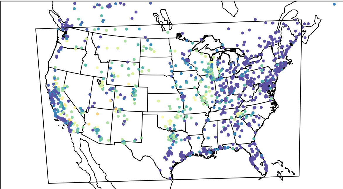
AirNOW (2023-08-02_08:00:00)
