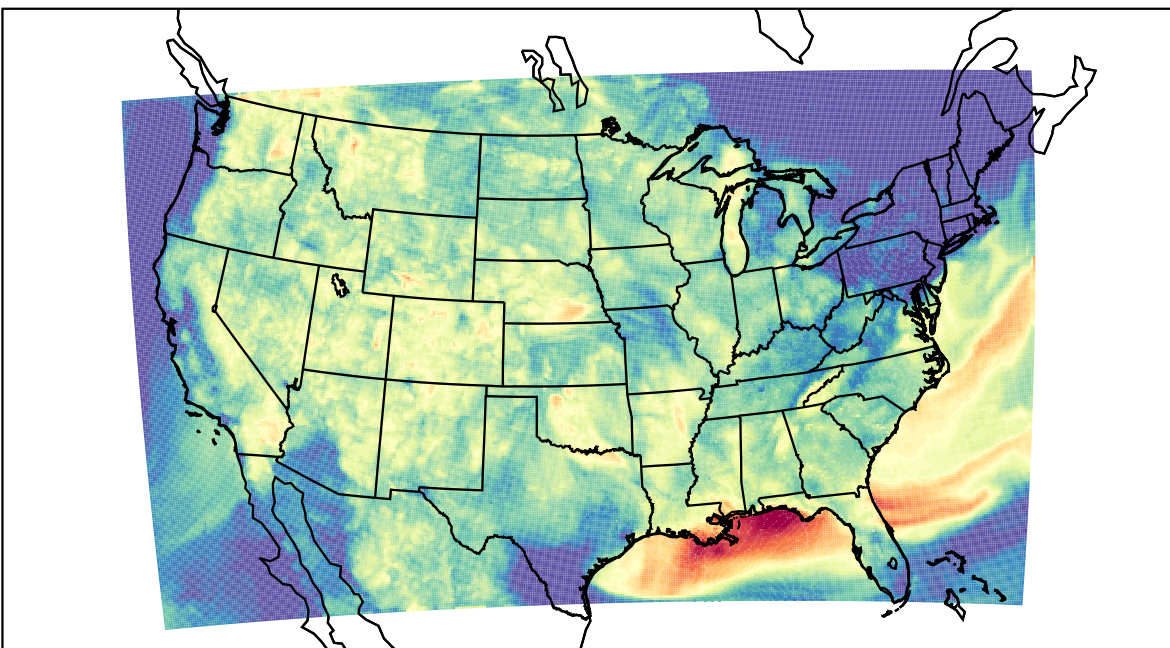
WRF (2023-08-02_07:00:00)
