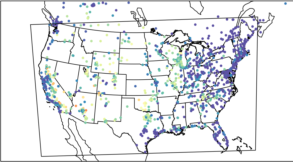
AirNOW (2023-08-02_06:00:00)
