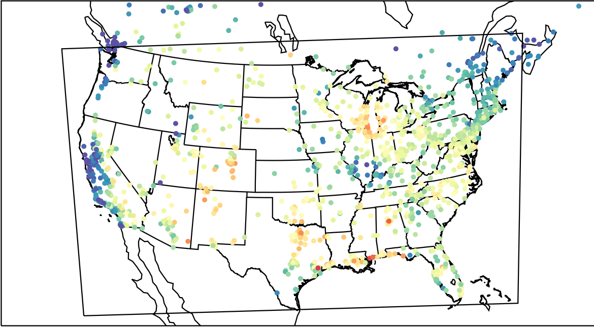
AirNOW (2023-08-02_16:00:00)
