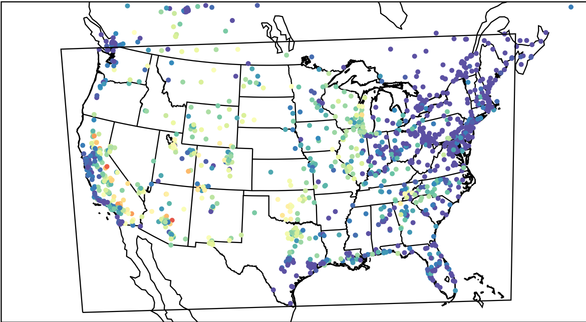
AirNOW (2023-08-02_05:00:00)
