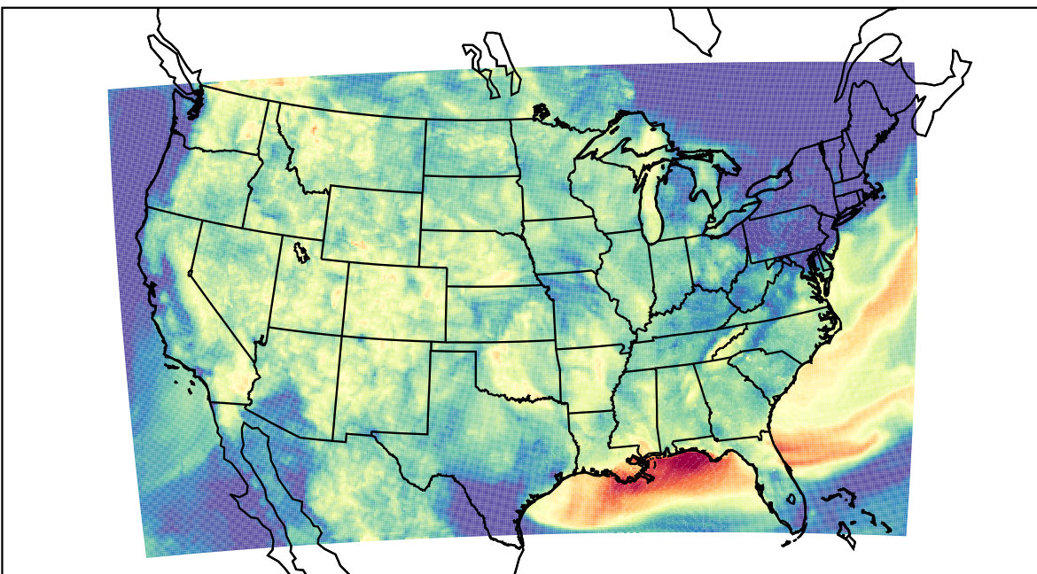
WRF (2023-08-02_08:00:00)
