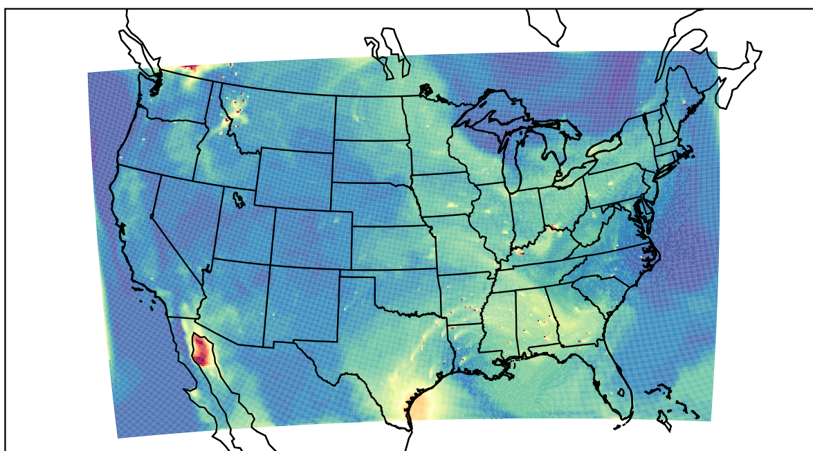
WRF 2023-08-04_19:00:00
