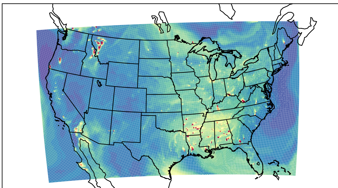
WRF 2023-08-04_00:00:00
