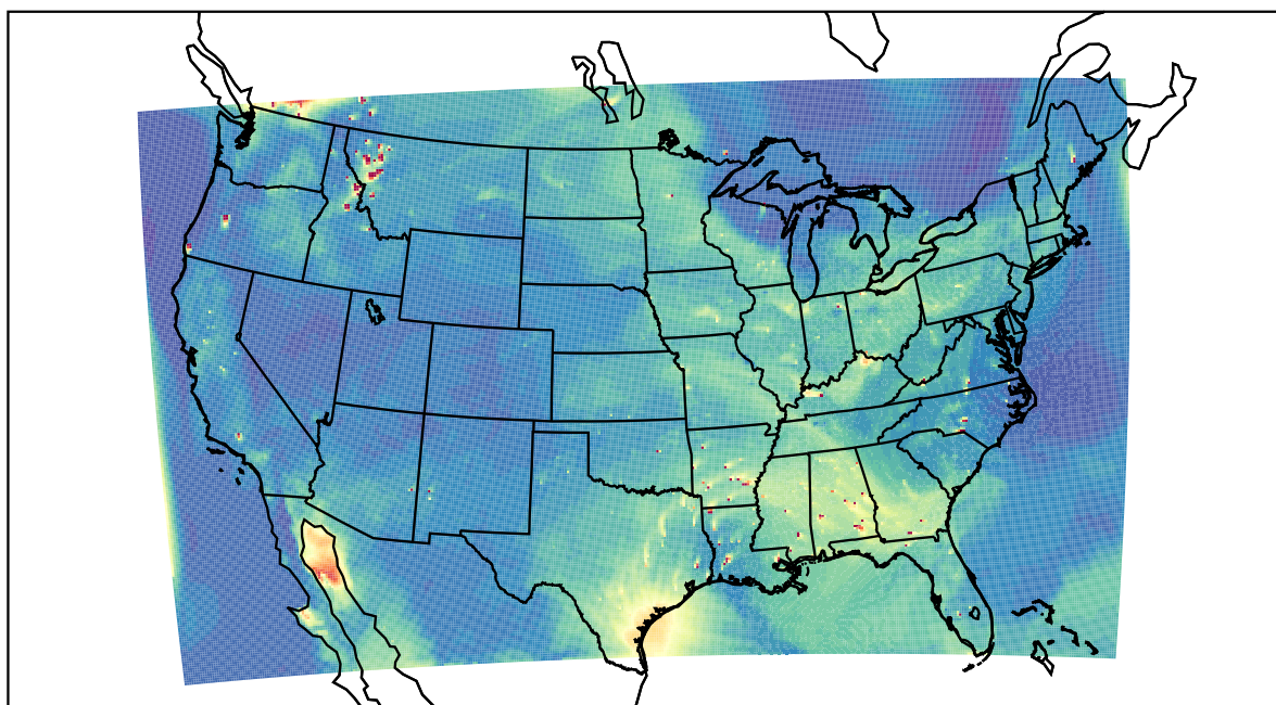
WRF 2023-08-04_22:00:00
