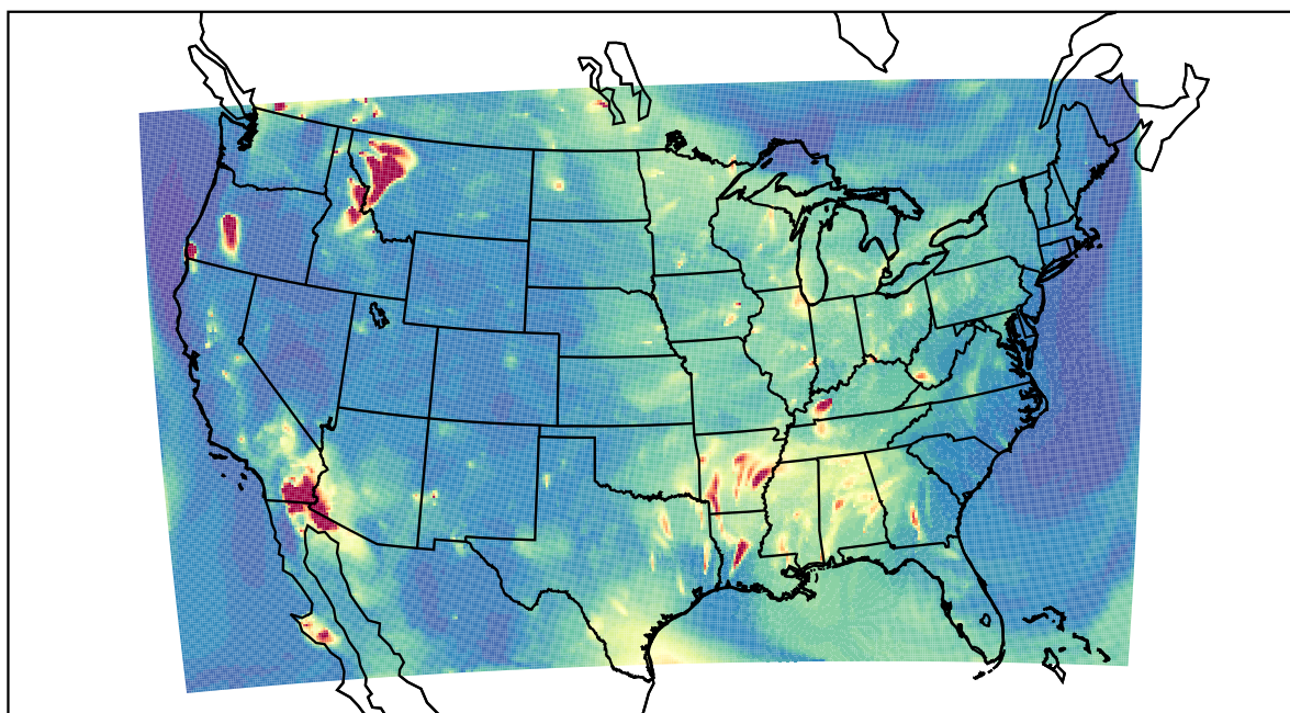
WRF 2023-08-04_04:00:00
