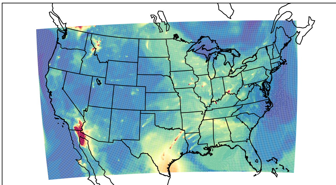
WRF 2023-08-04_14:00:00
