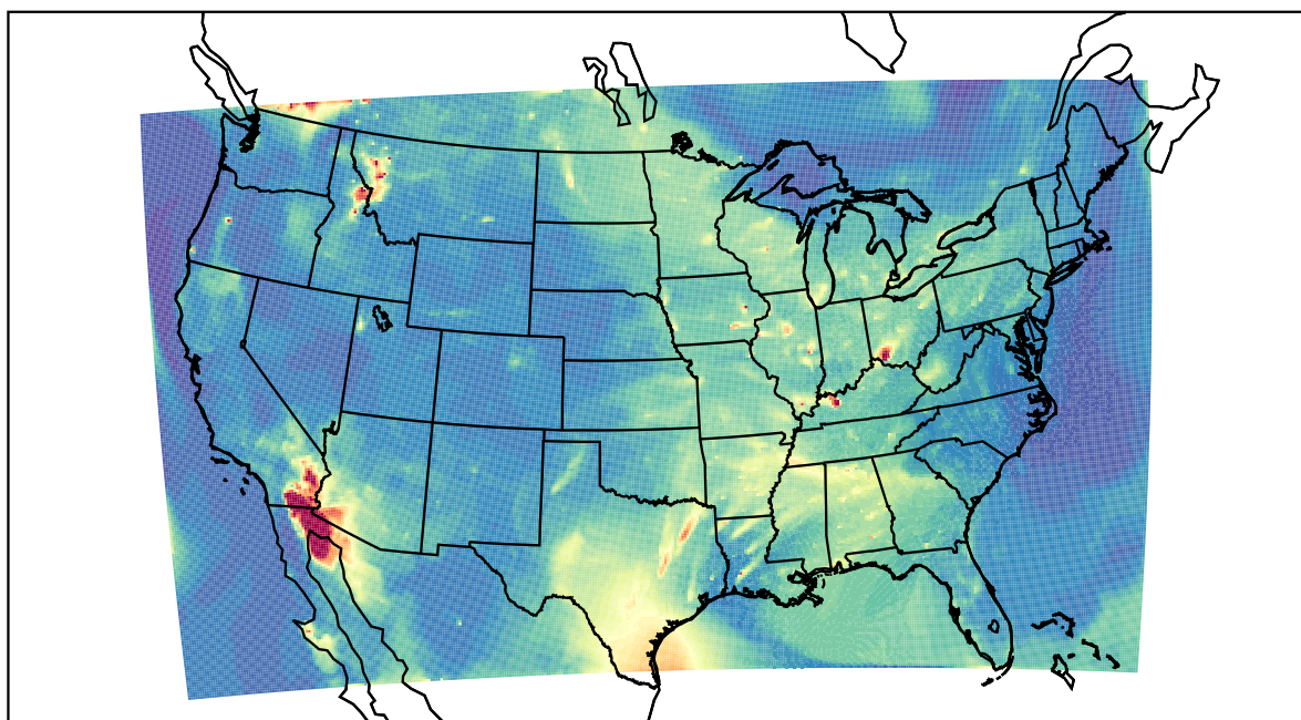
WRF 2023-08-04_12:00:00
