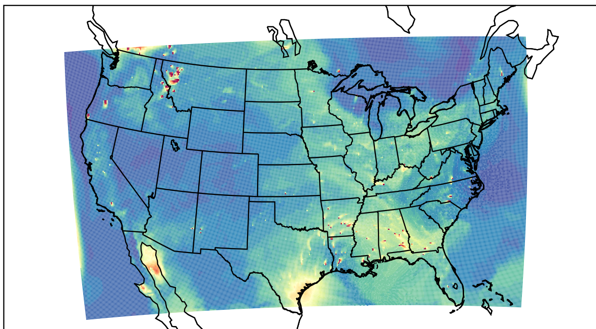
WRF 2023-08-04_23:00:00
