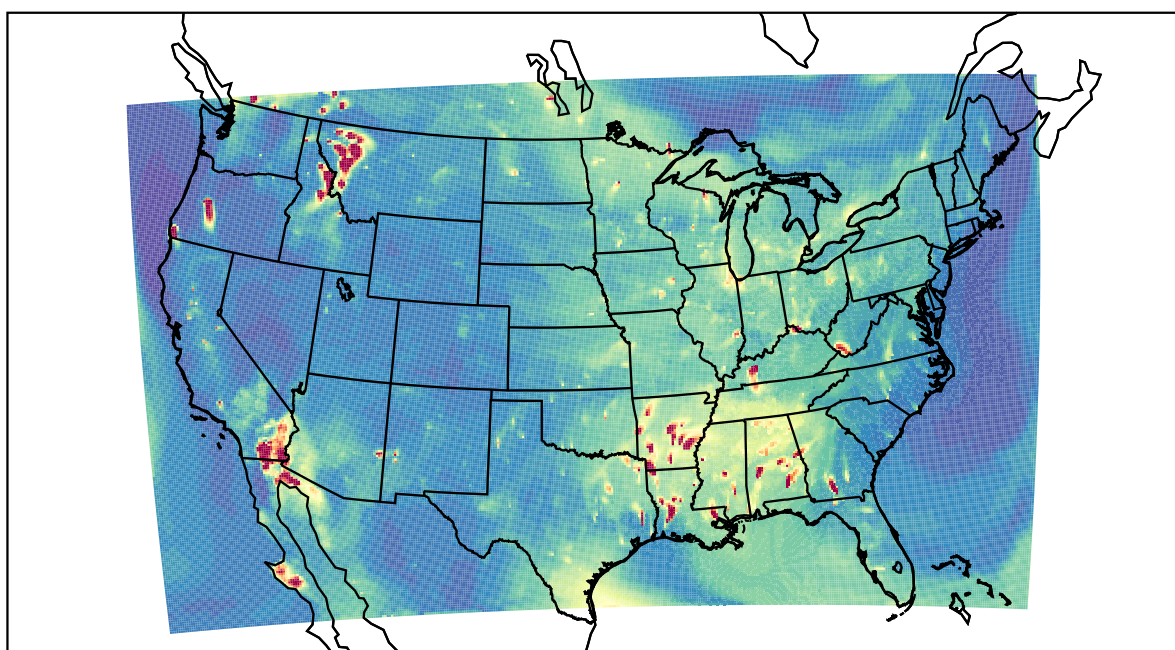
WRF 2023-08-04_02:00:00
