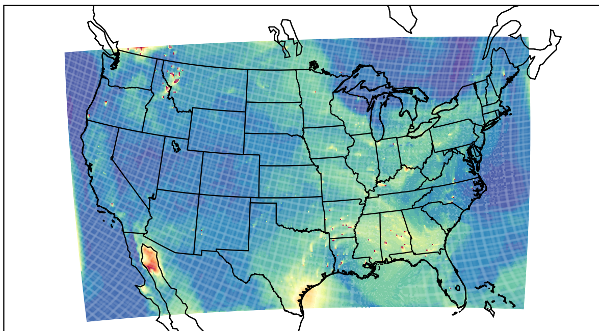
WRF 2023-08-04_21:00:00
