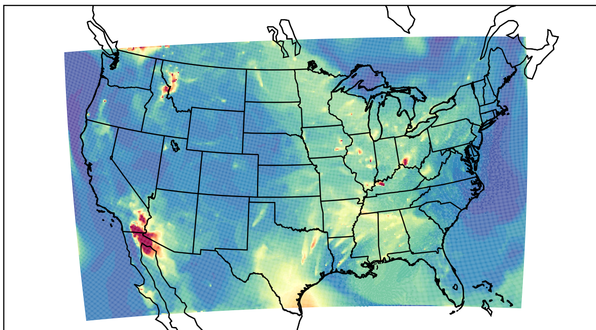
WRF 2023-08-04_11:00:00
