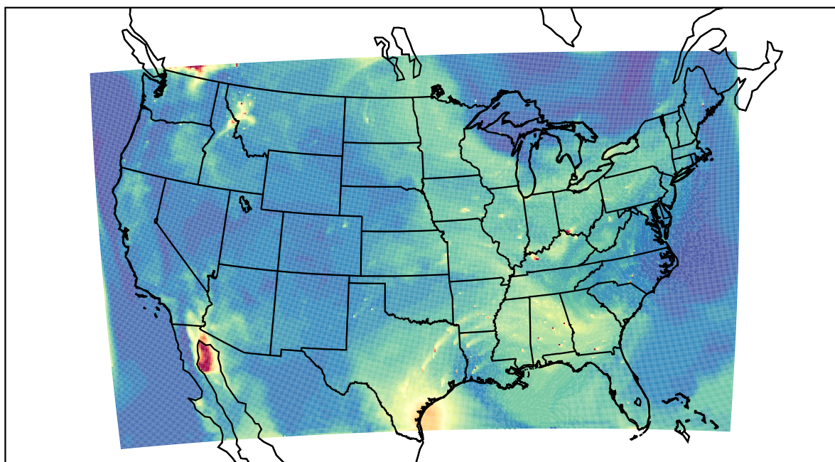
WRF 2023-08-04_18:00:00
