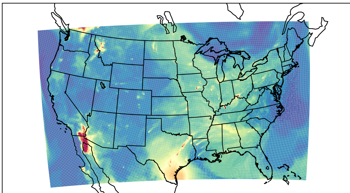
WRF 2023-08-04_15:00:00
