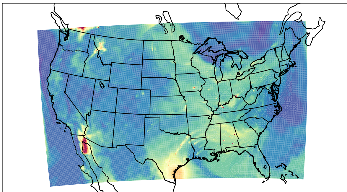
WRF 2023-08-04_17:00:00
