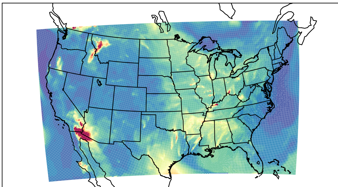
WRF 2023-08-04_08:00:00
