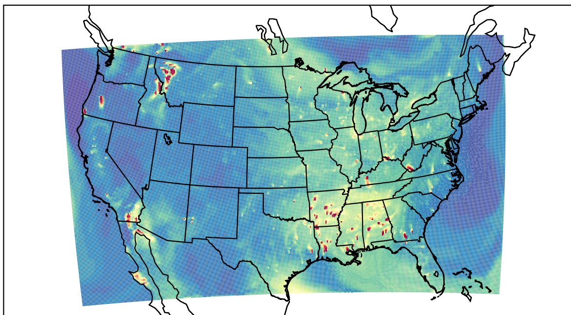
WRF 2023-08-04_01:00:00
