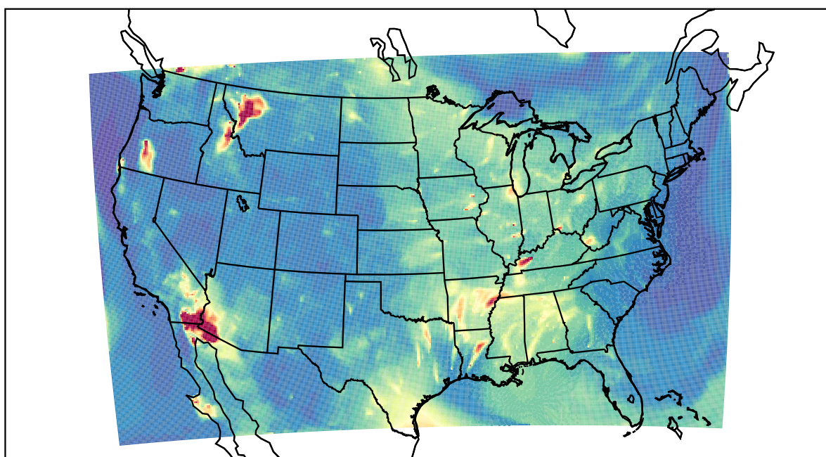
WRF 2023-08-04_06:00:00
