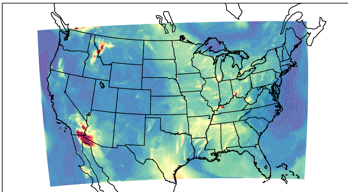
WRF 2023-08-04_09:00:00
