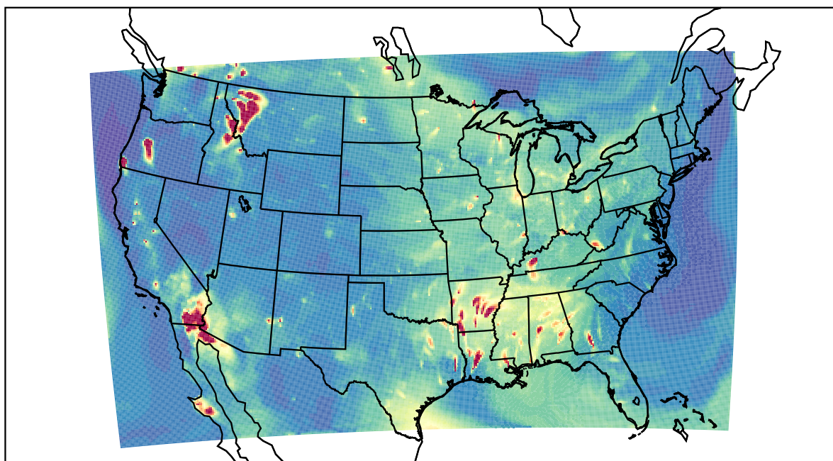
WRF 2023-08-04_03:00:00
