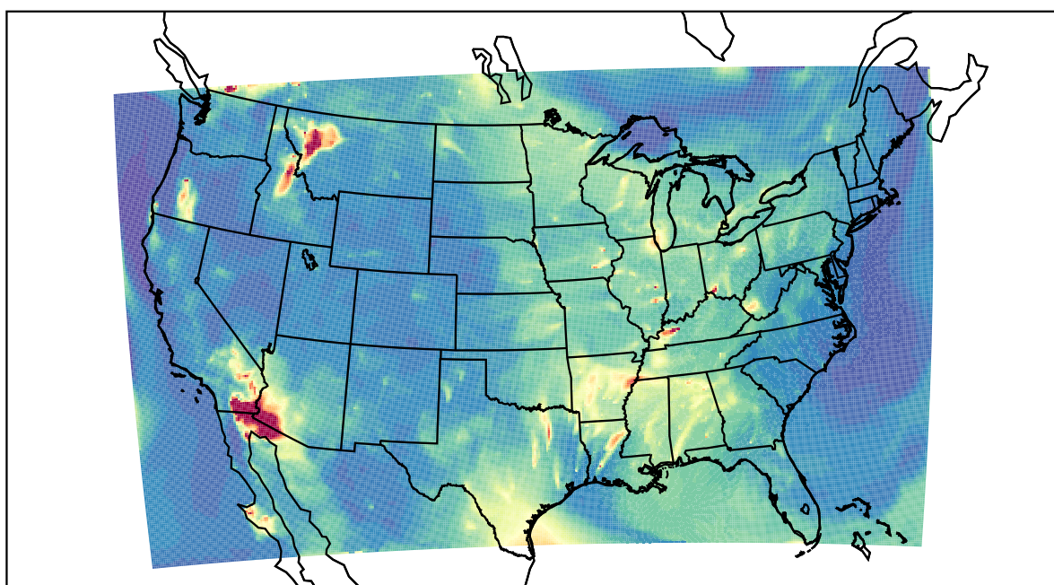
WRF 2023-08-04_07:00:00
