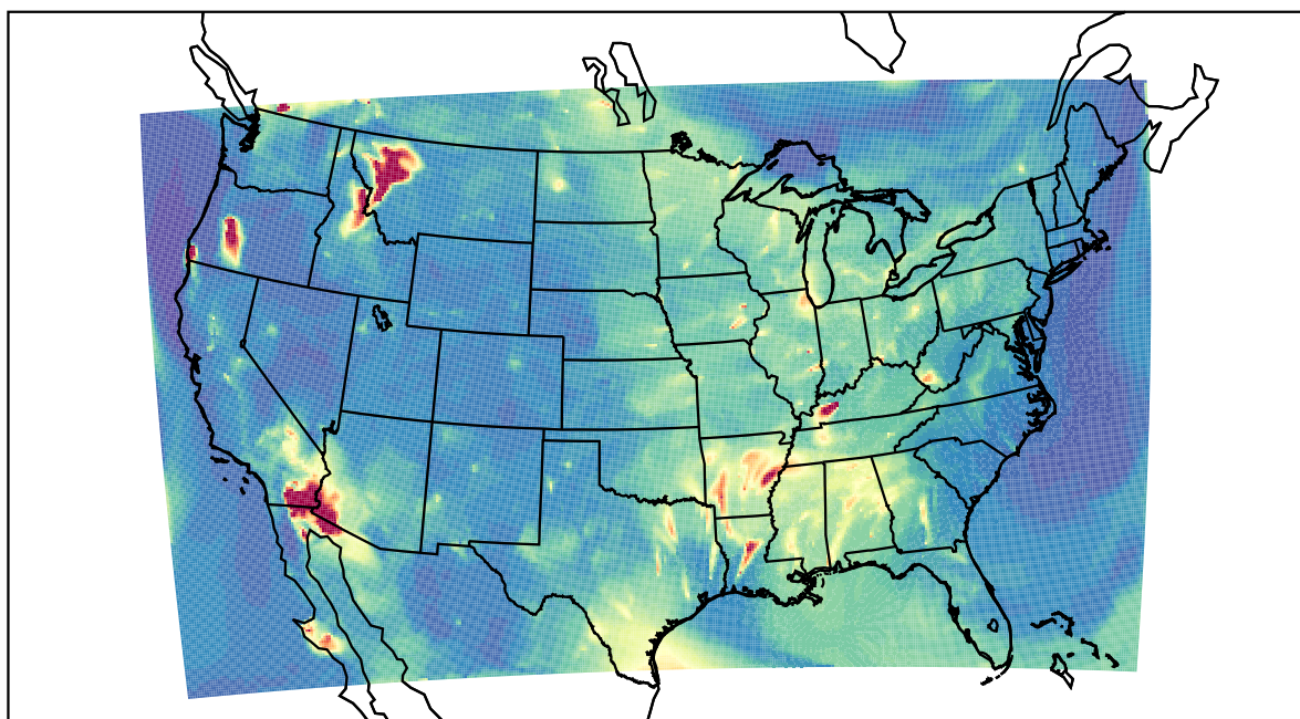
WRF 2023-08-04_05:00:00
