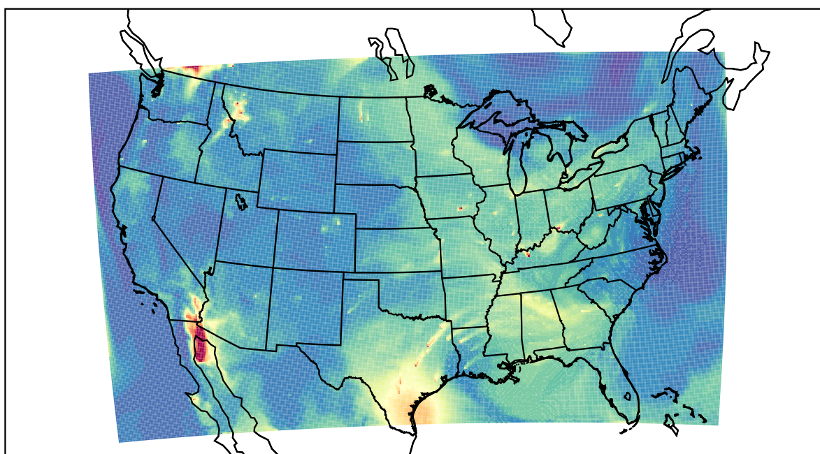
WRF 2023-08-04_16:00:00
