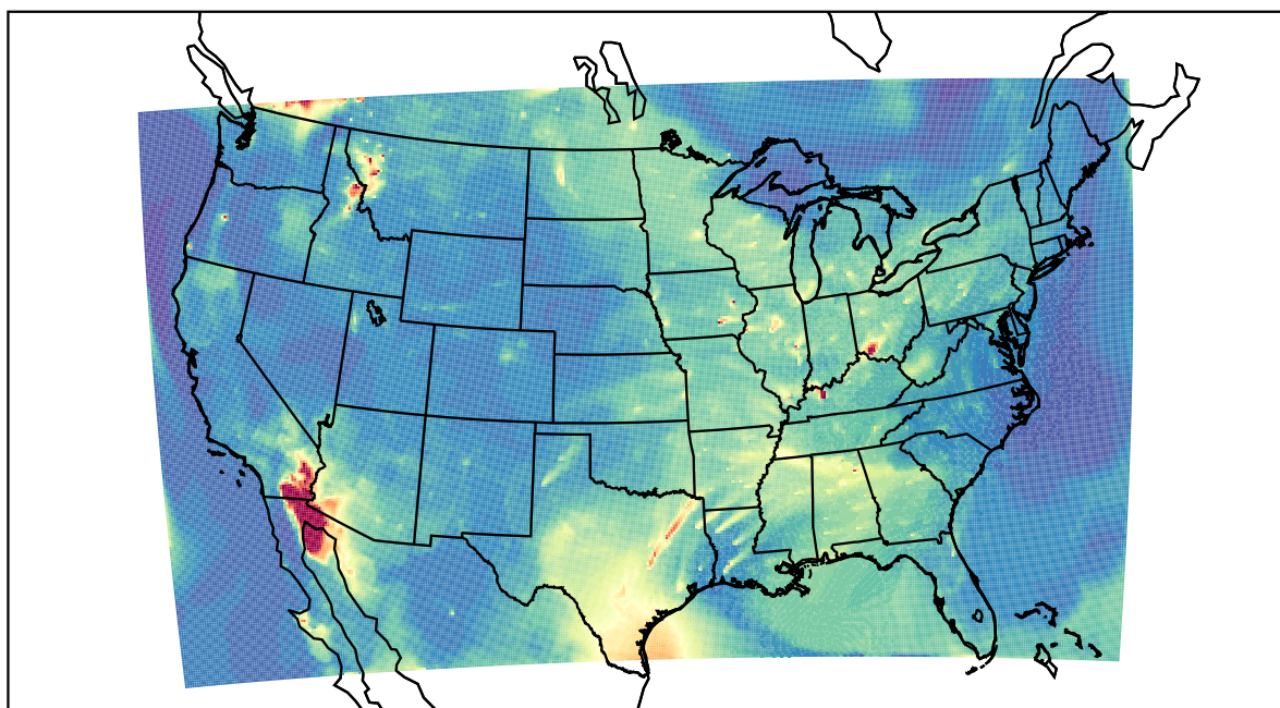
WRF 2023-08-04_13:00:00
