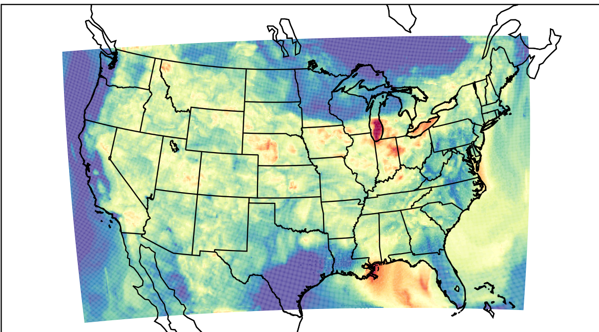
WRF (2023-08-04_06:00:00)
