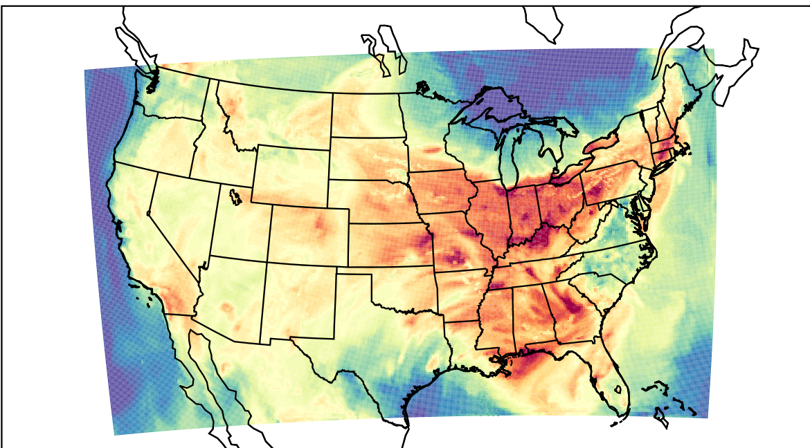
WRF (2023-08-04_19:00:00)
