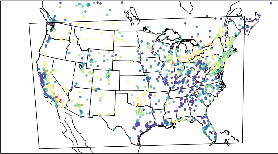
AirNOW (2023-08-04_03:00:00)
