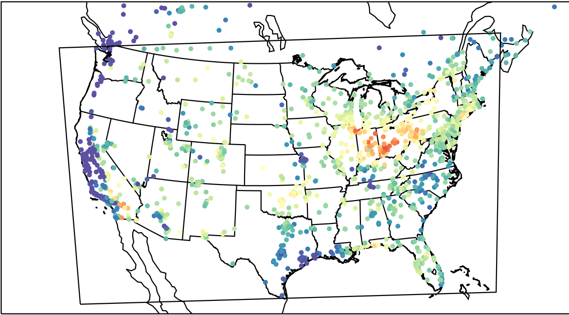
AirNOW (2023-08-04_15:00:00)
