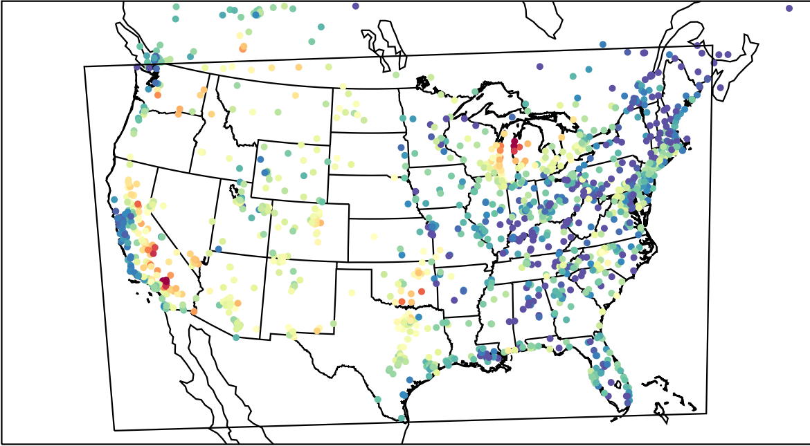
AirNOW (2023-08-03_02:00:00)
