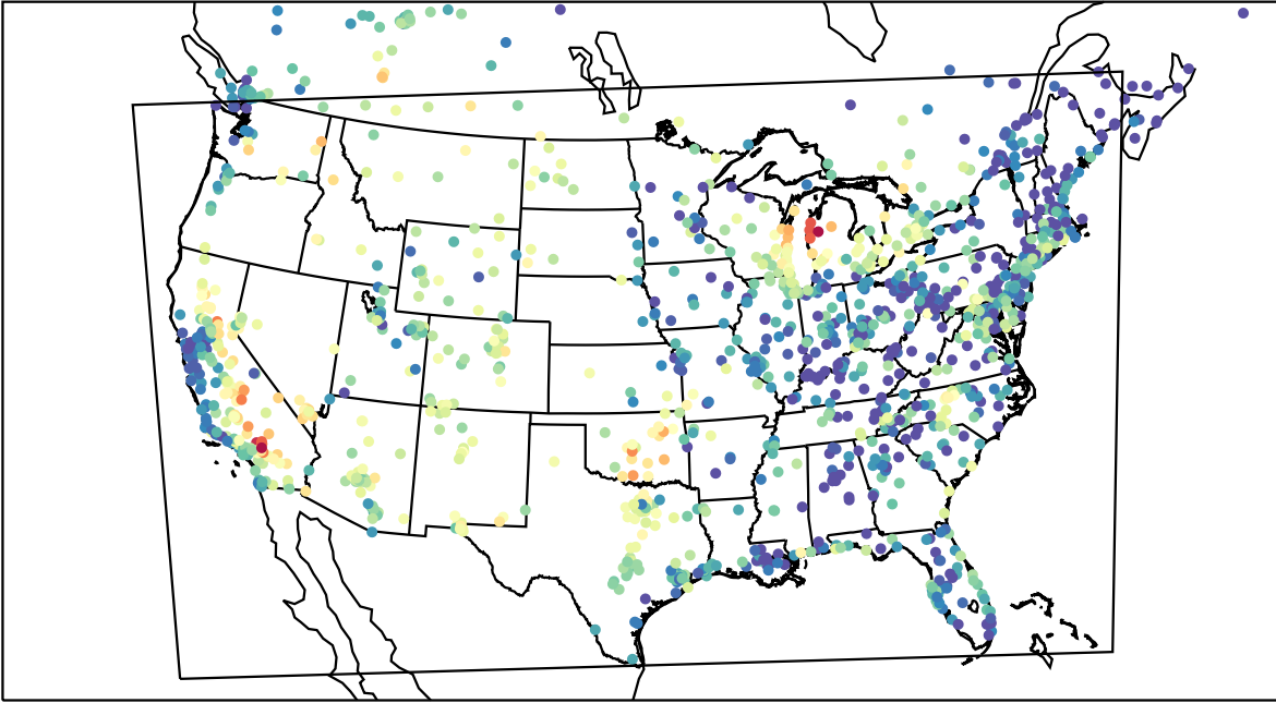
AirNOW (2023-08-03_03:00:00)
