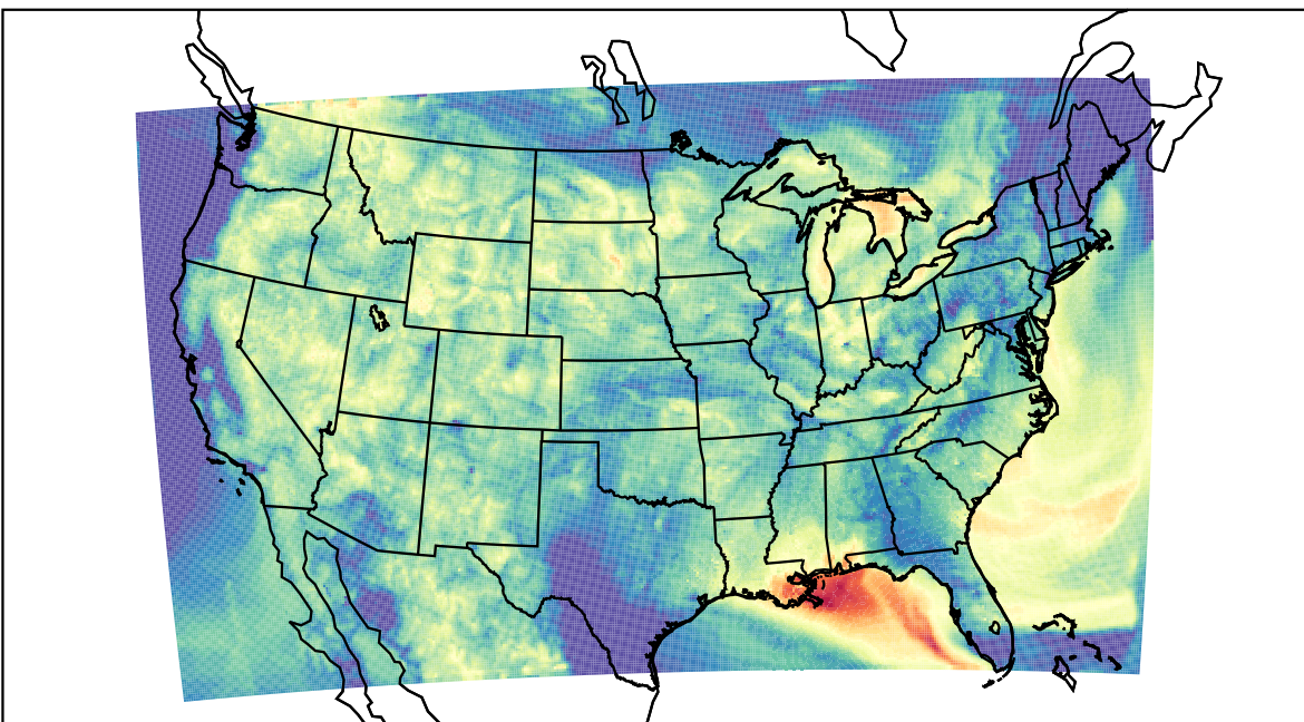
WRF (2023-08-03_11:00:00)
