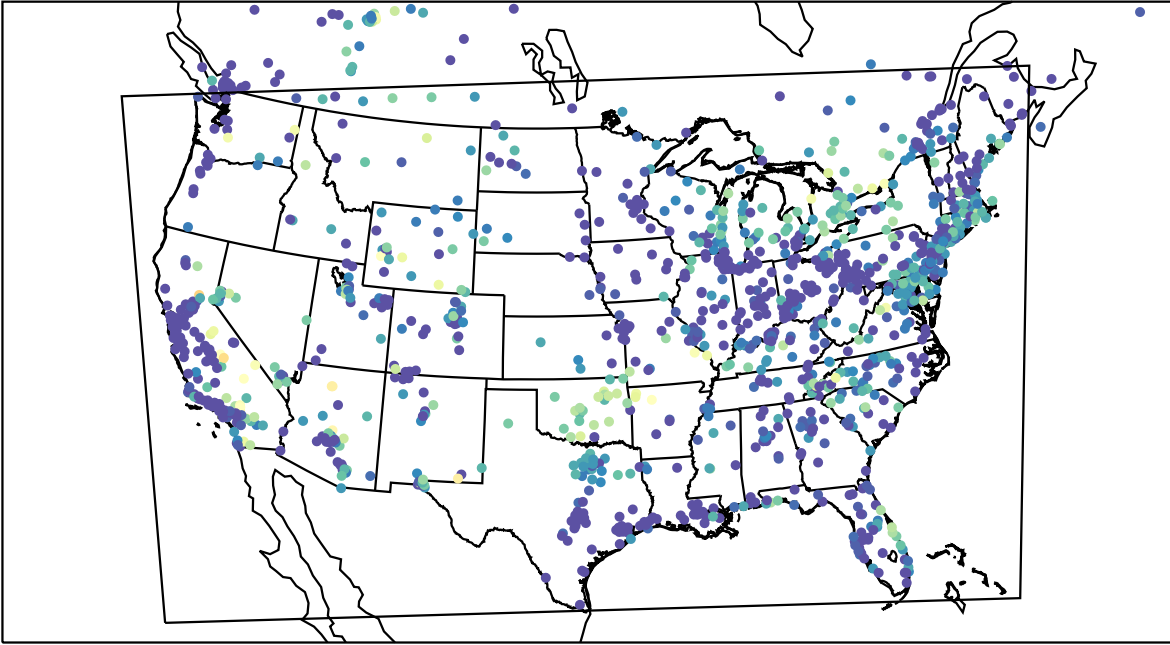
AirNOW (2023-08-03_12:00:00)
