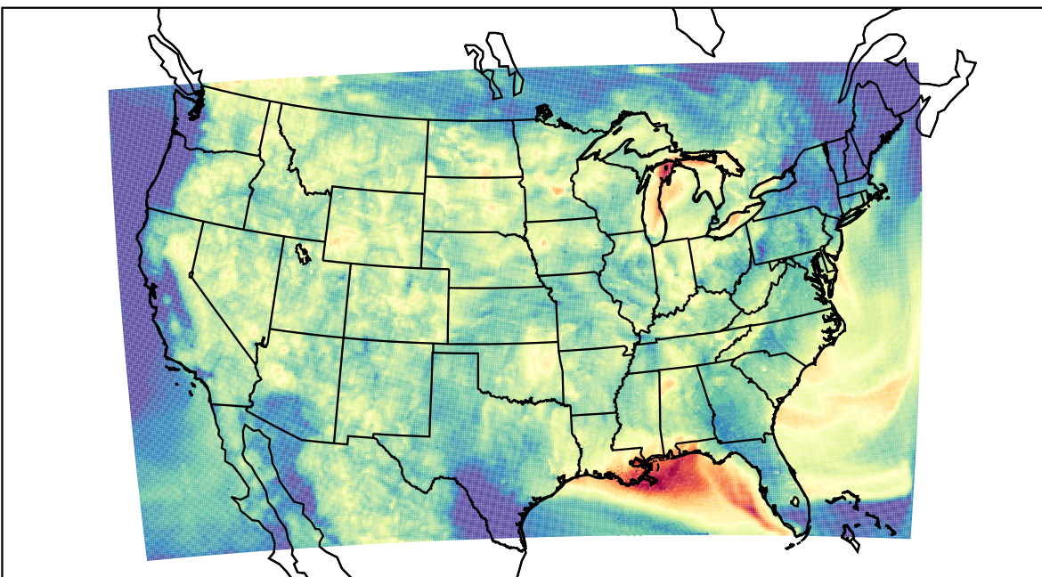
WRF (2023-08-03_07:00:00)
