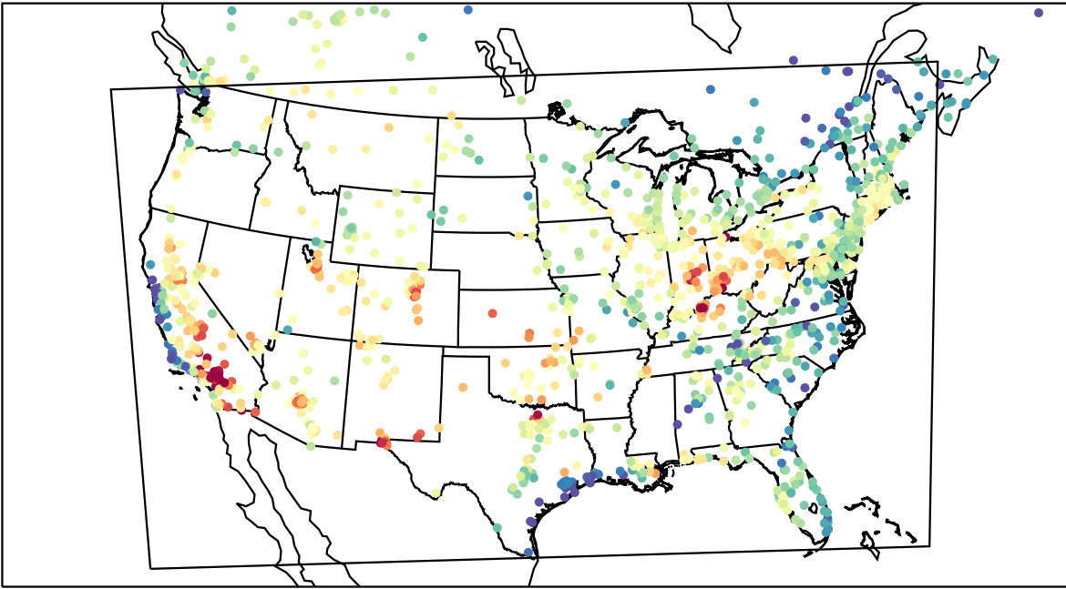
AirNOW (2023-08-04_23:00:00)
