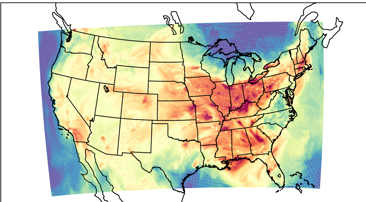
WRF (2023-08-04_20:00:00)
