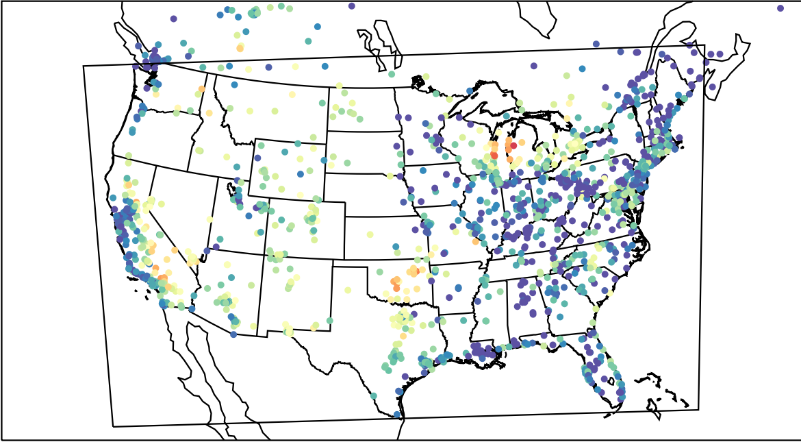
AirNOW (2023-08-03_04:00:00)
