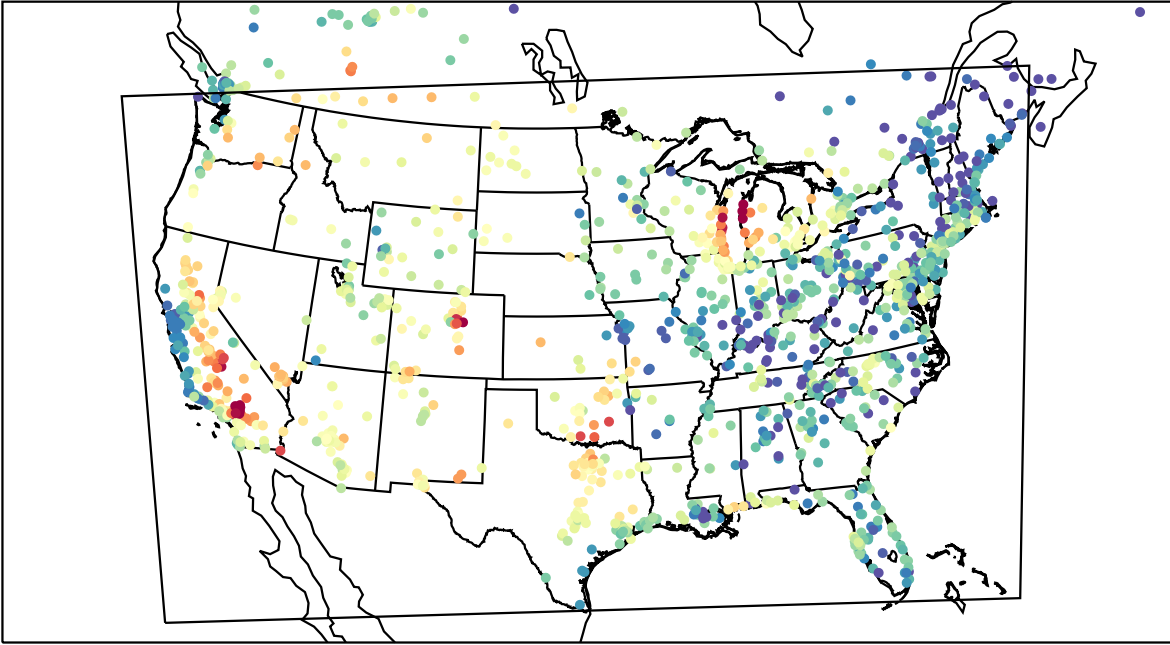
AirNOW (2023-08-03_01:00:00)
