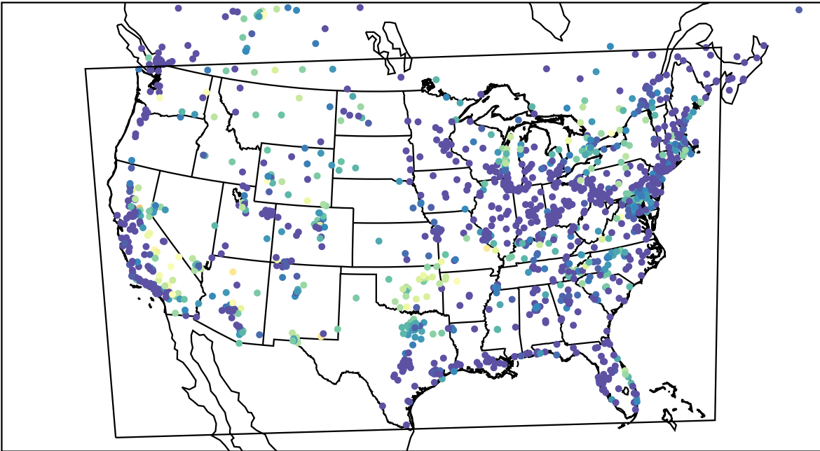
AirNOW (2023-08-03_11:00:00)
