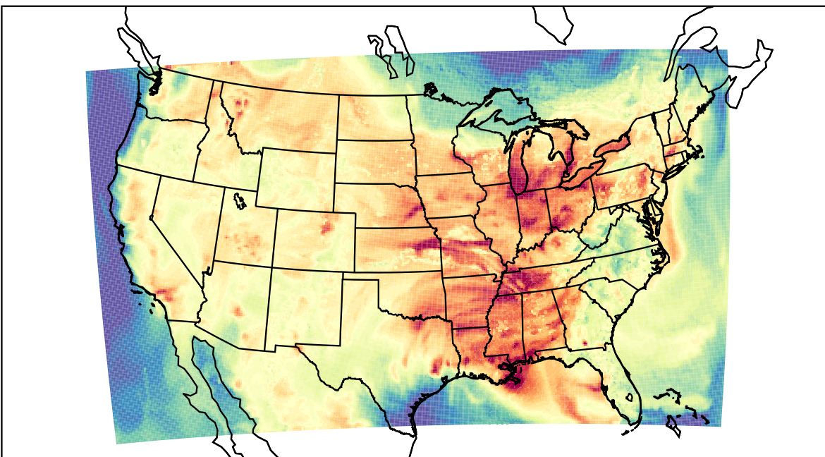
WRF (2023-08-03_22:00:00)
