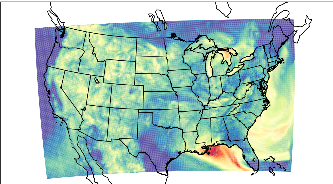
WRF (2023-08-03_12:00:00)
