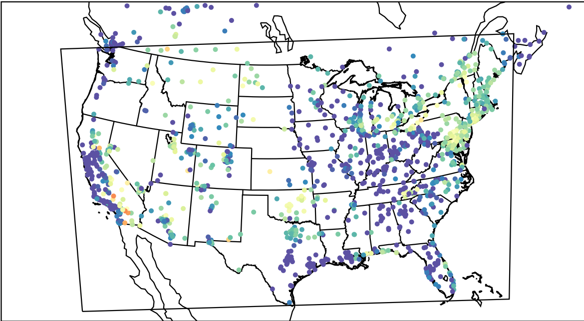
AirNOW (2023-08-04_07:00:00)
