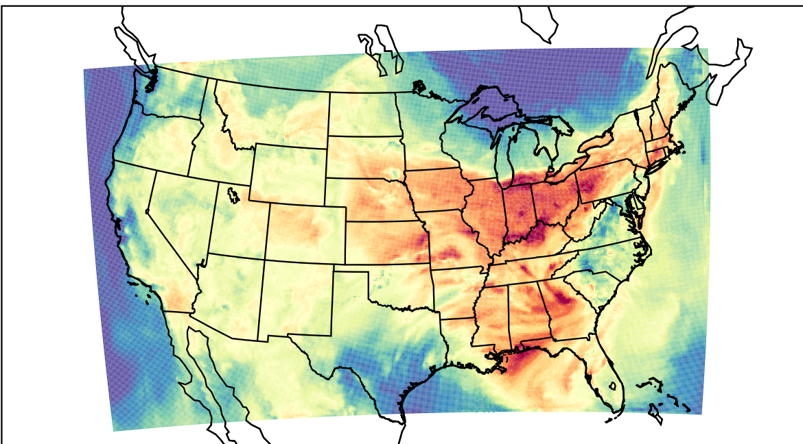
WRF (2023-08-04_17:00:00)
