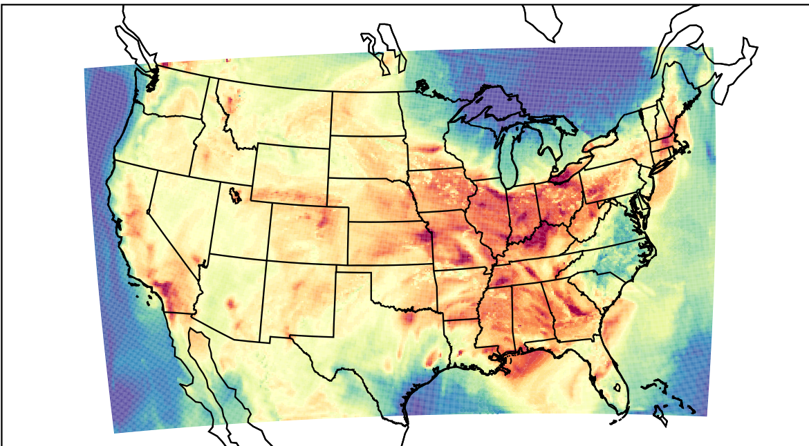
WRF (2023-08-04_22:00:00)
