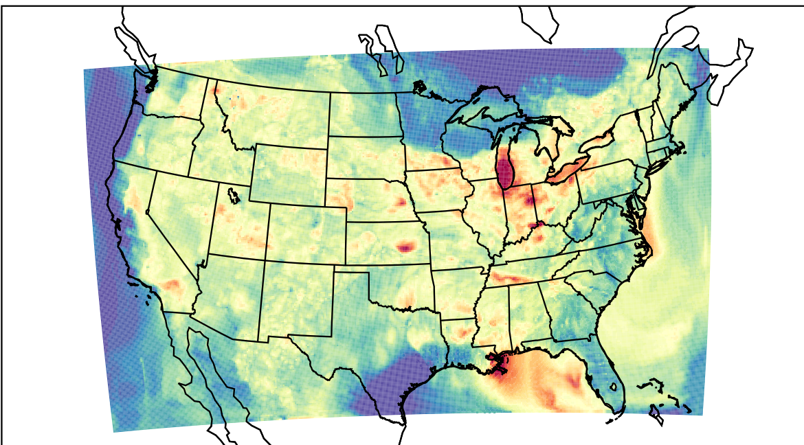
WRF (2023-08-04_03:00:00)
