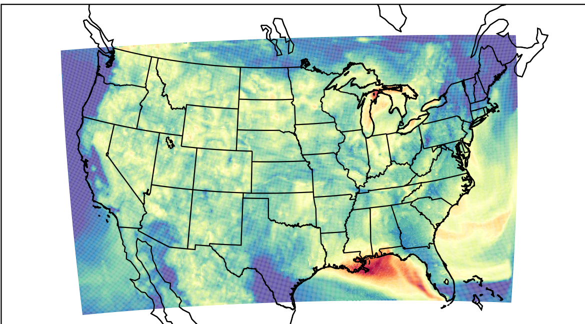
WRF (2023-08-03_08:00:00)
