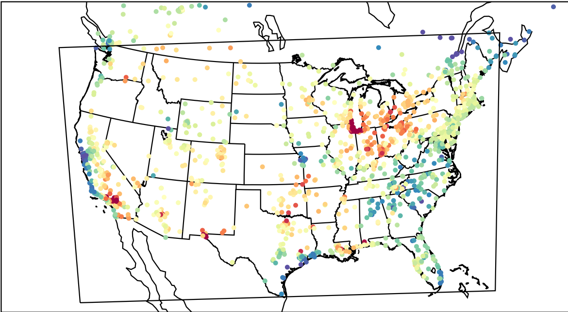
AirNOW (2023-08-03_22:00:00)
