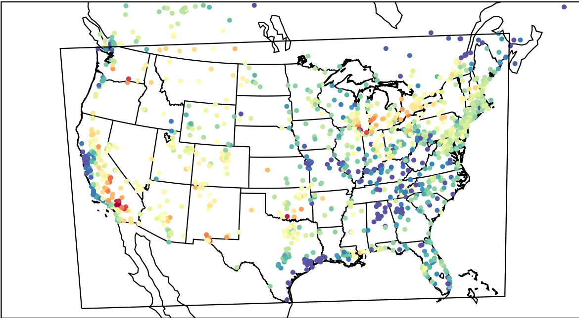
AirNOW (2023-08-04_01:00:00)
