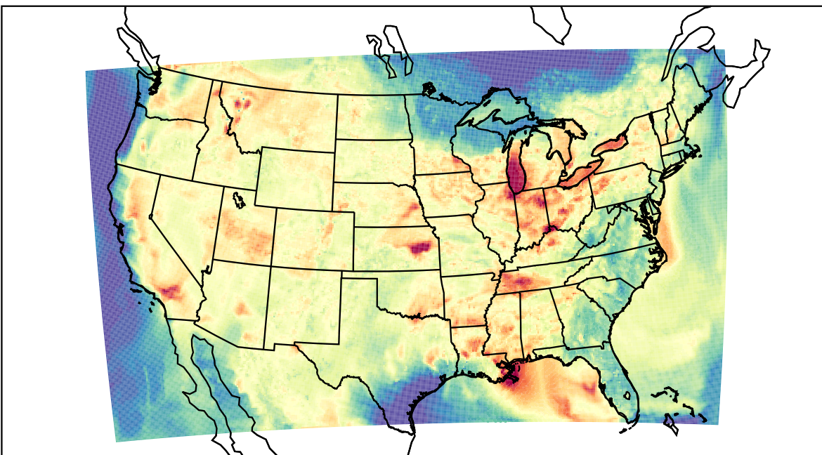
WRF (2023-08-04_01:00:00)
