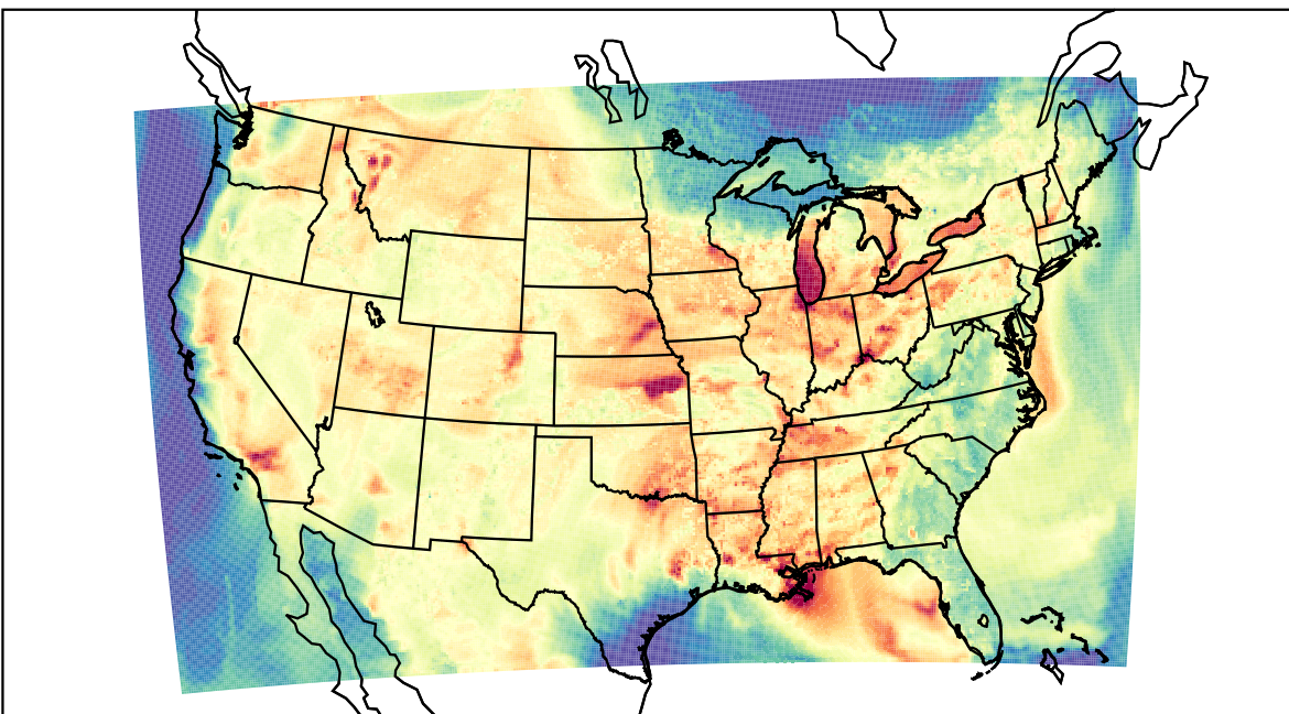
WRF (2023-08-04_00:00:00)
