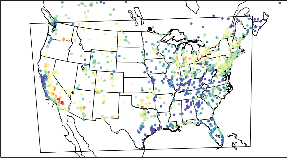
AirNOW (2023-08-04_02:00:00)
