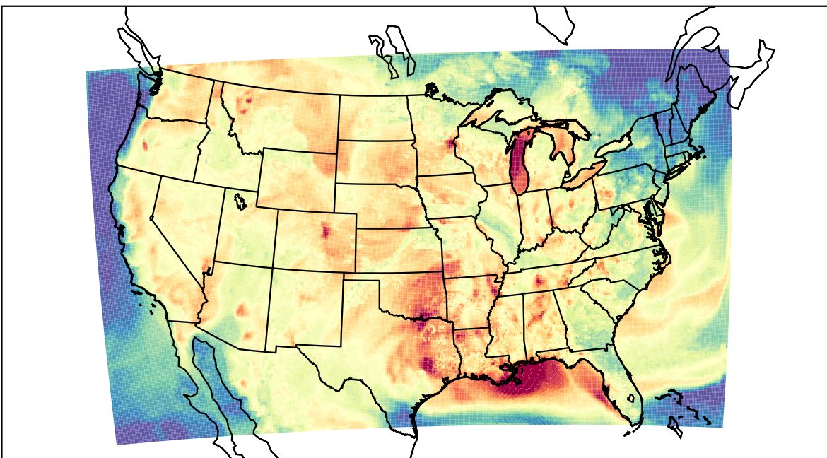
WRF (2023-08-03_00:00:00)
