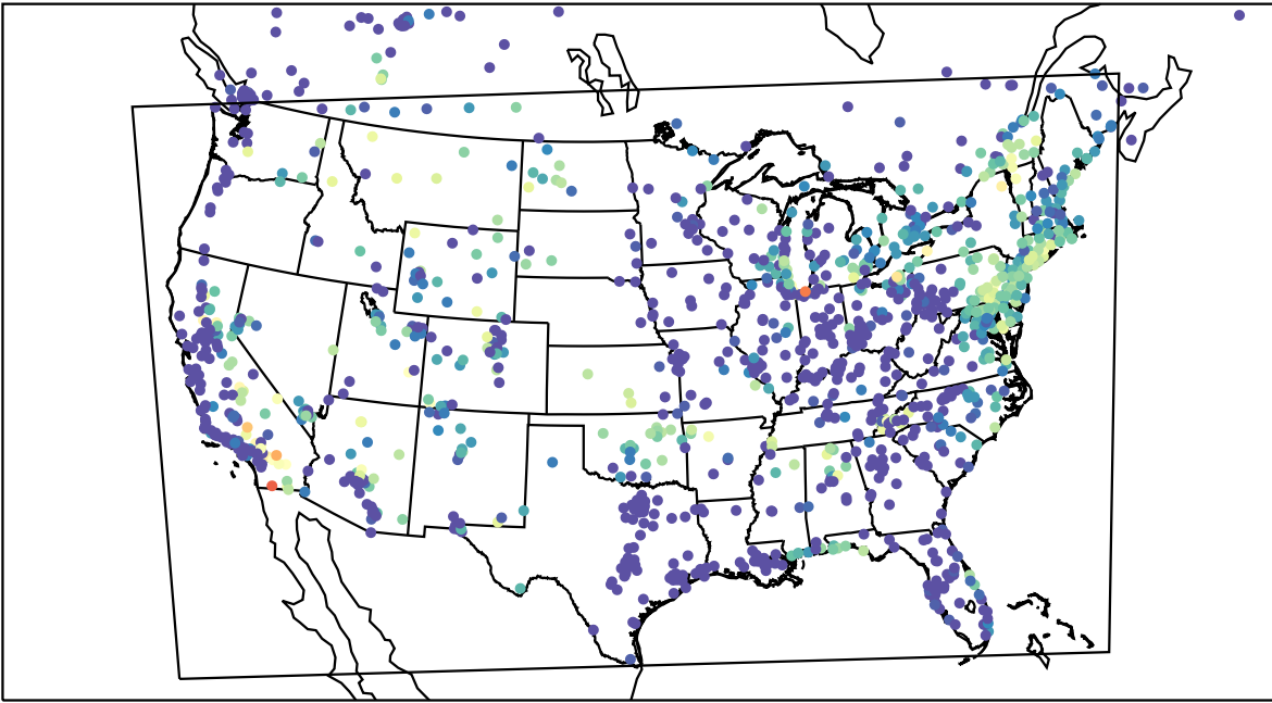
AirNOW (2023-08-04_11:00:00)
