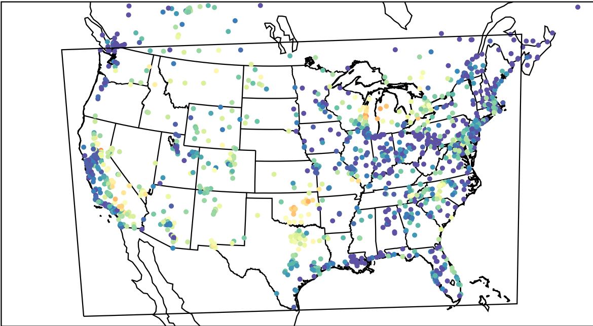
AirNOW (2023-08-03_05:00:00)
