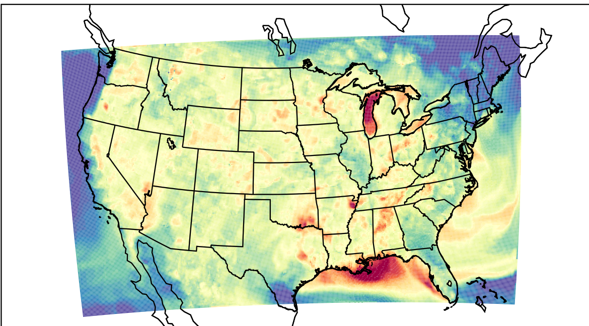
WRF (2023-08-03_02:00:00)
