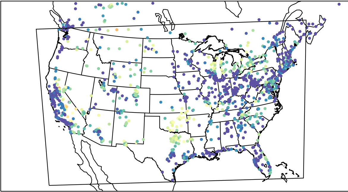
AirNOW (2023-08-03_08:00:00)
