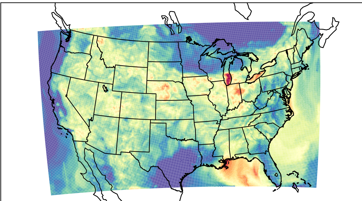
WRF (2023-08-04_07:00:00)
