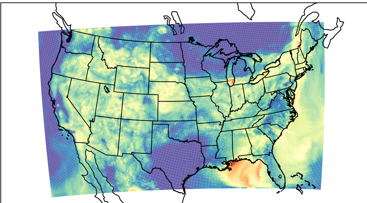
WRF (2023-08-04_13:00:00)
