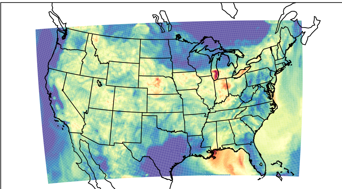
WRF (2023-08-04_08:00:00)
