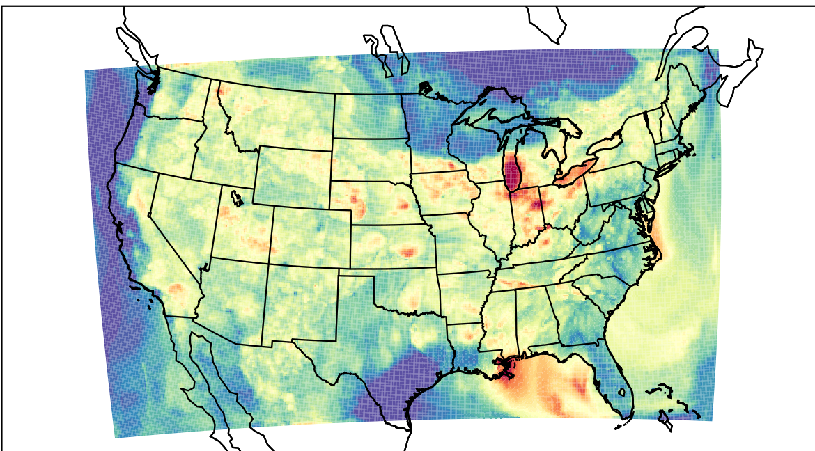
WRF (2023-08-04_04:00:00)
