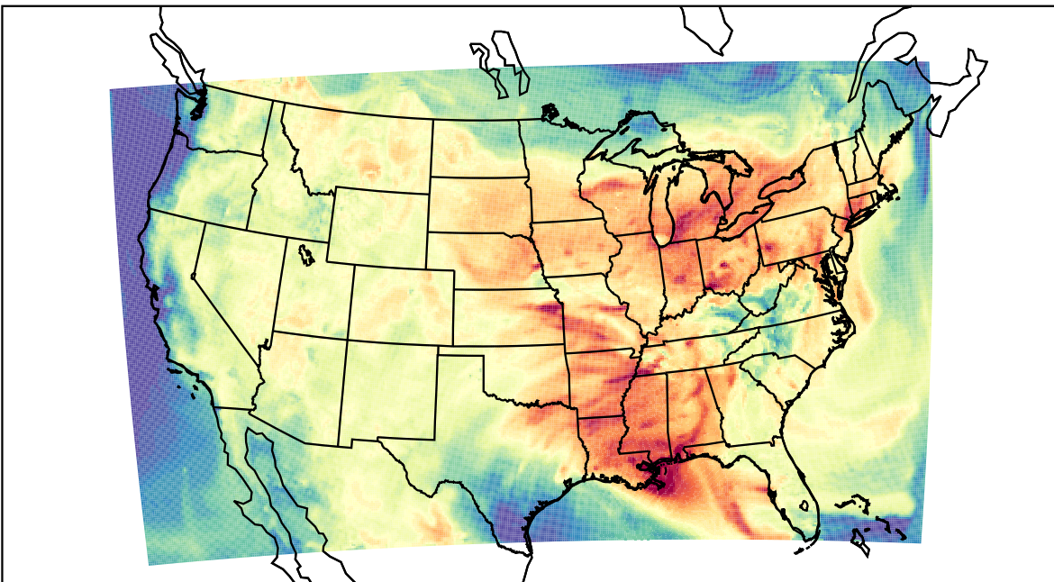
WRF (2023-08-03_17:00:00)
