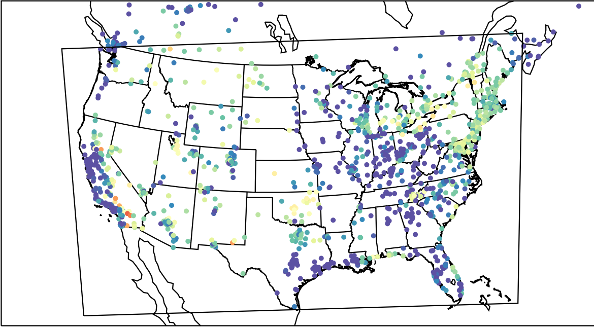
AirNOW (2023-08-04_06:00:00)
