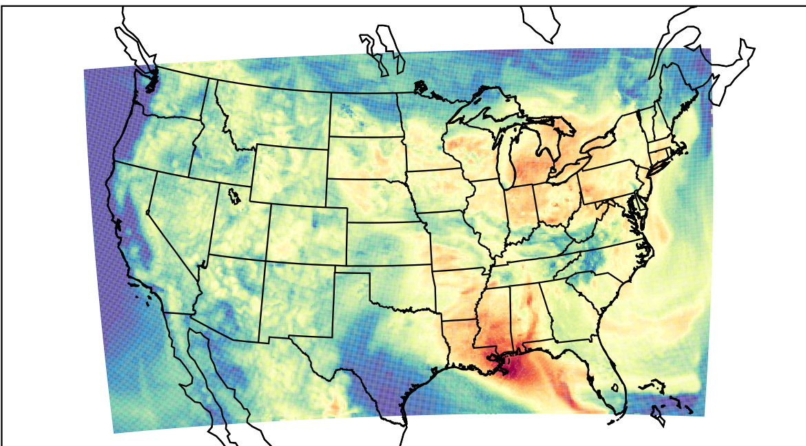
WRF (2023-08-03_15:00:00)
