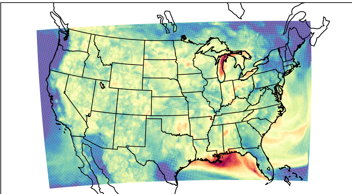
WRF (2023-08-03_05:00:00)
