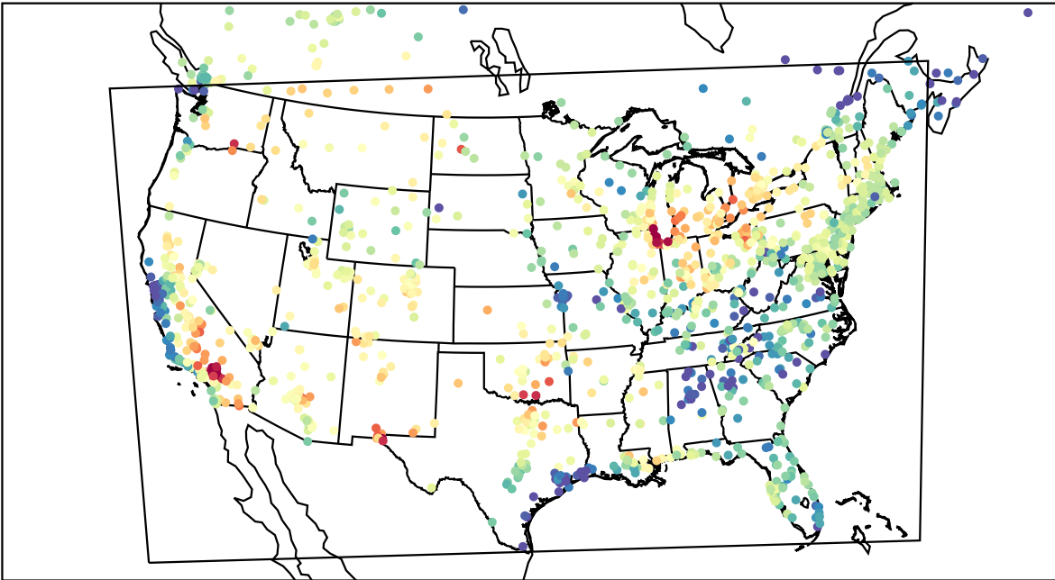
AirNOW (2023-08-04_00:00:00)
