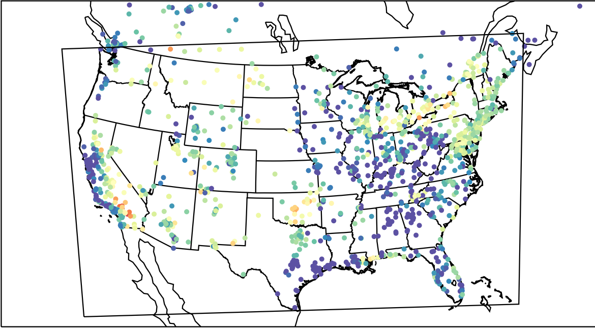
AirNOW (2023-08-04_04:00:00)
