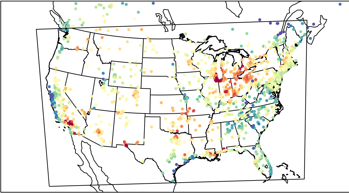
AirNOW (2023-08-03_21:00:00)
