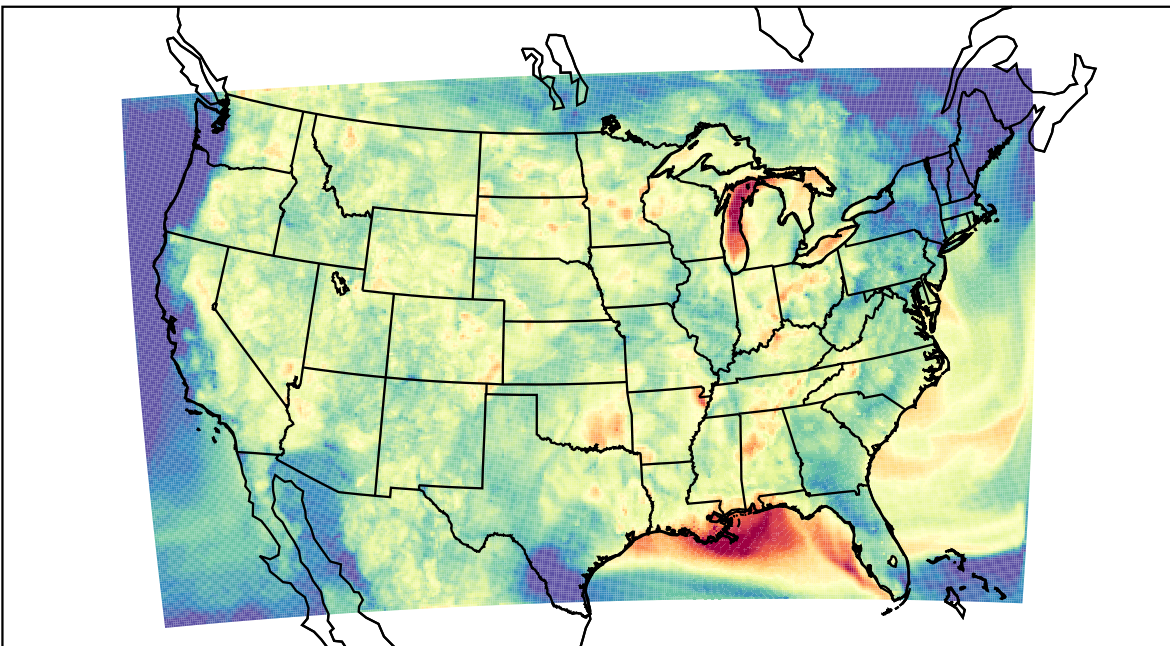
WRF (2023-08-03_04:00:00)
