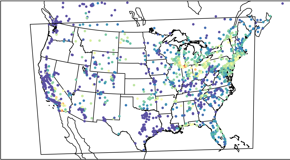
AirNOW (2023-08-04_13:00:00)
