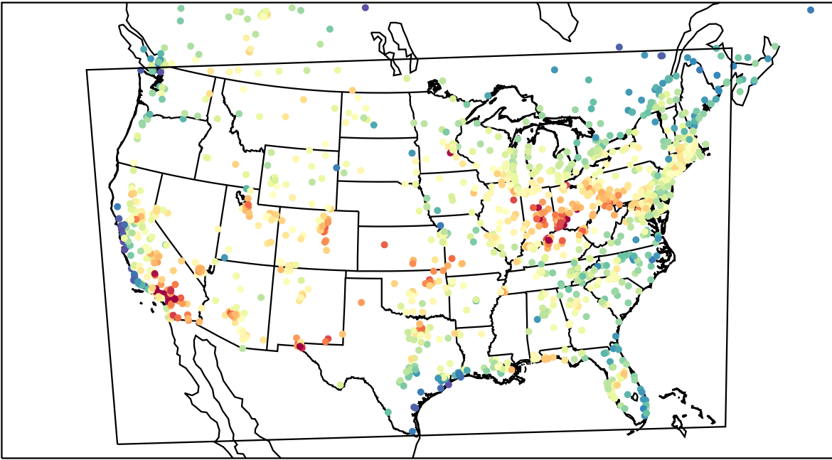
AirNOW (2023-08-04_20:00:00)
