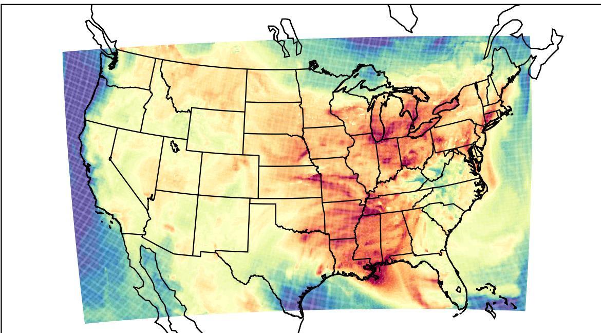
WRF (2023-08-03_19:00:00)
