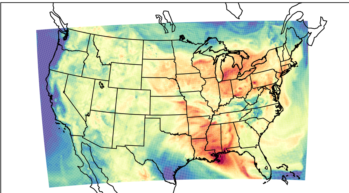
WRF (2023-08-03_16:00:00)
