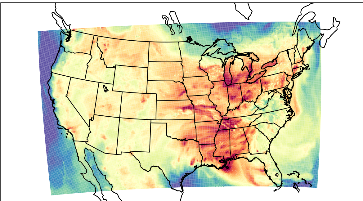
WRF (2023-08-03_21:00:00)
