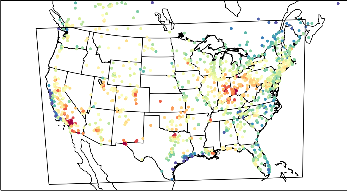
AirNOW (2023-08-04_22:00:00)
