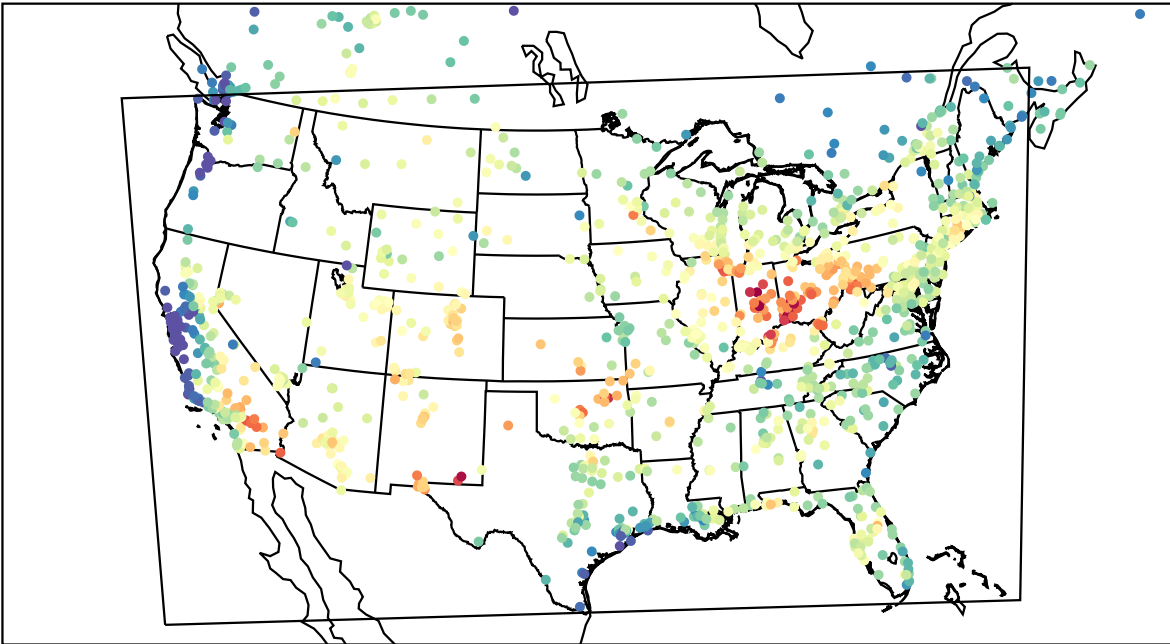
AirNOW (2023-08-04_17:00:00)
