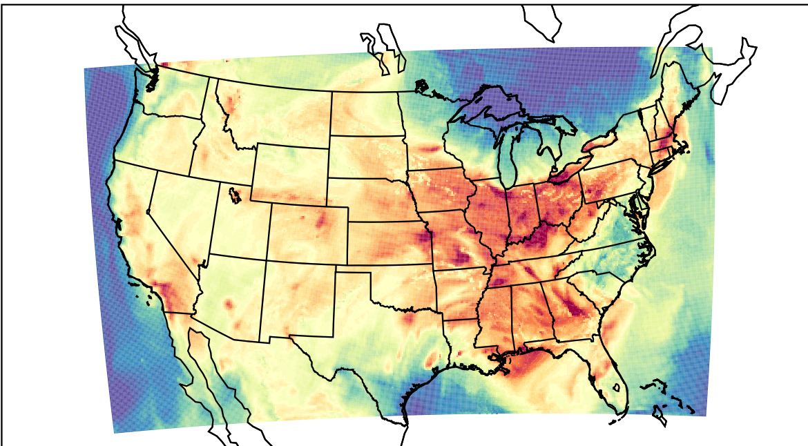
WRF (2023-08-04_21:00:00)
