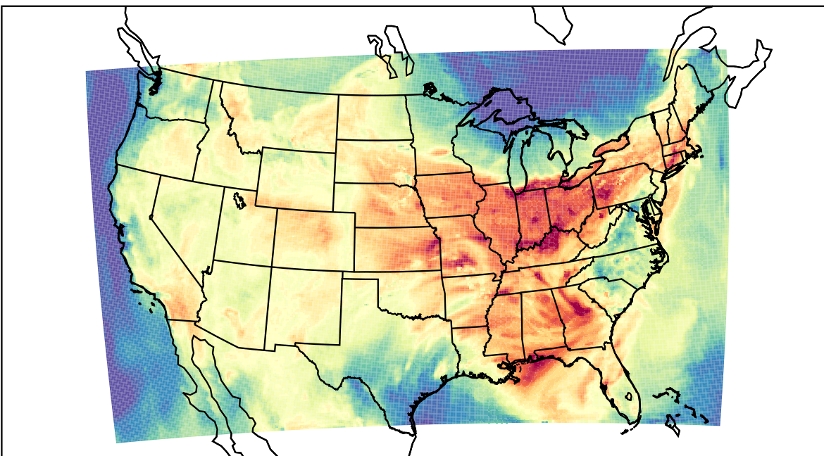
WRF (2023-08-04_18:00:00)
