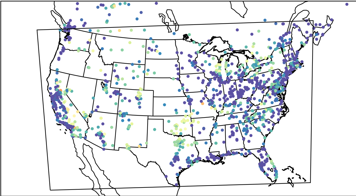
AirNOW (2023-08-03_09:00:00)
