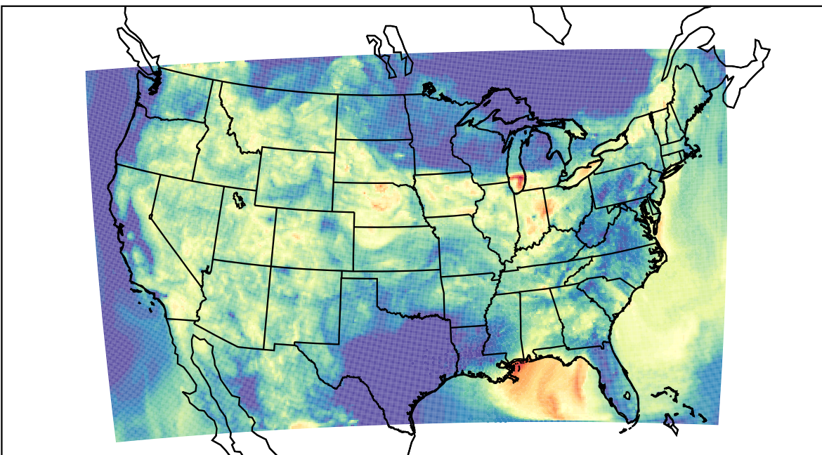
WRF (2023-08-04_11:00:00)
