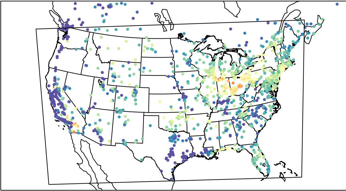
AirNOW (2023-08-04_14:00:00)
