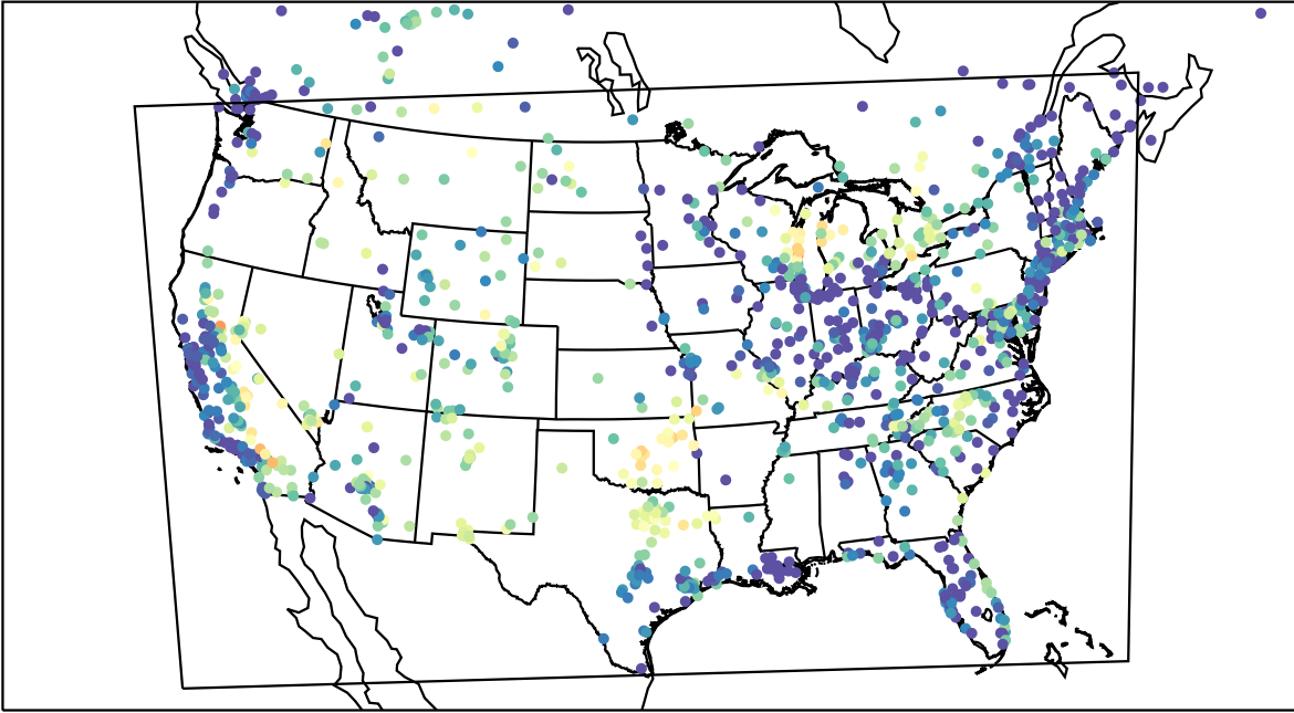
AirNOW (2023-08-03_06:00:00)
