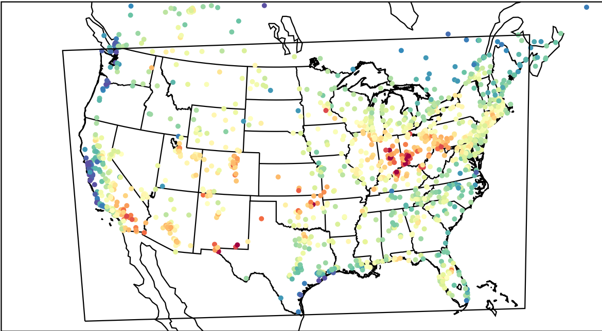
AirNOW (2023-08-04_18:00:00)
