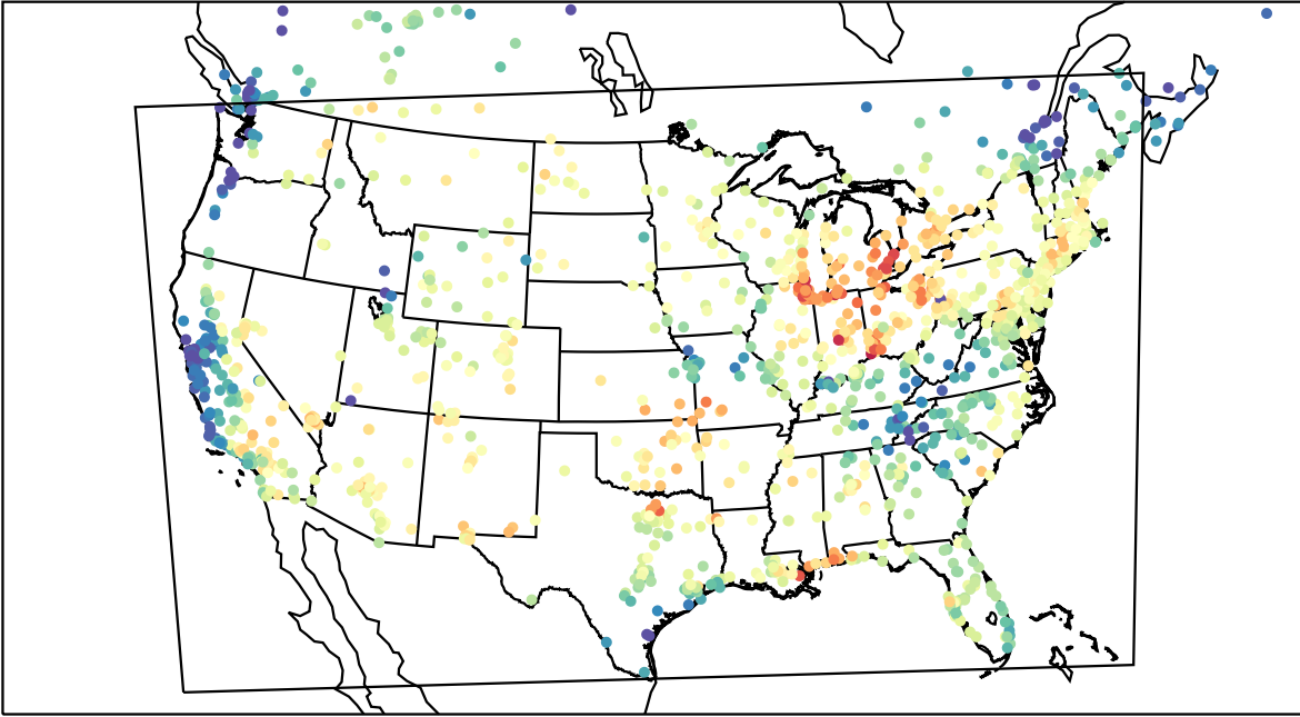
AirNOW (2023-08-03_17:00:00)
