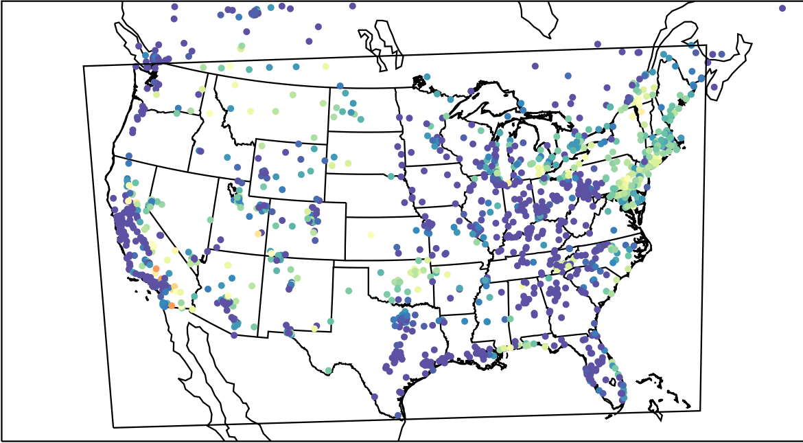
AirNOW (2023-08-04_09:00:00)
