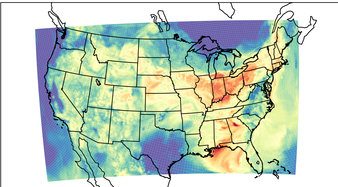
WRF (2023-08-04_15:00:00)
