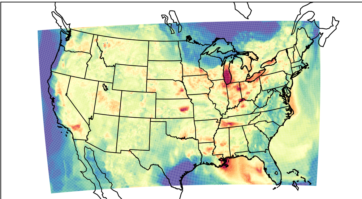
WRF (2023-08-04_02:00:00)
