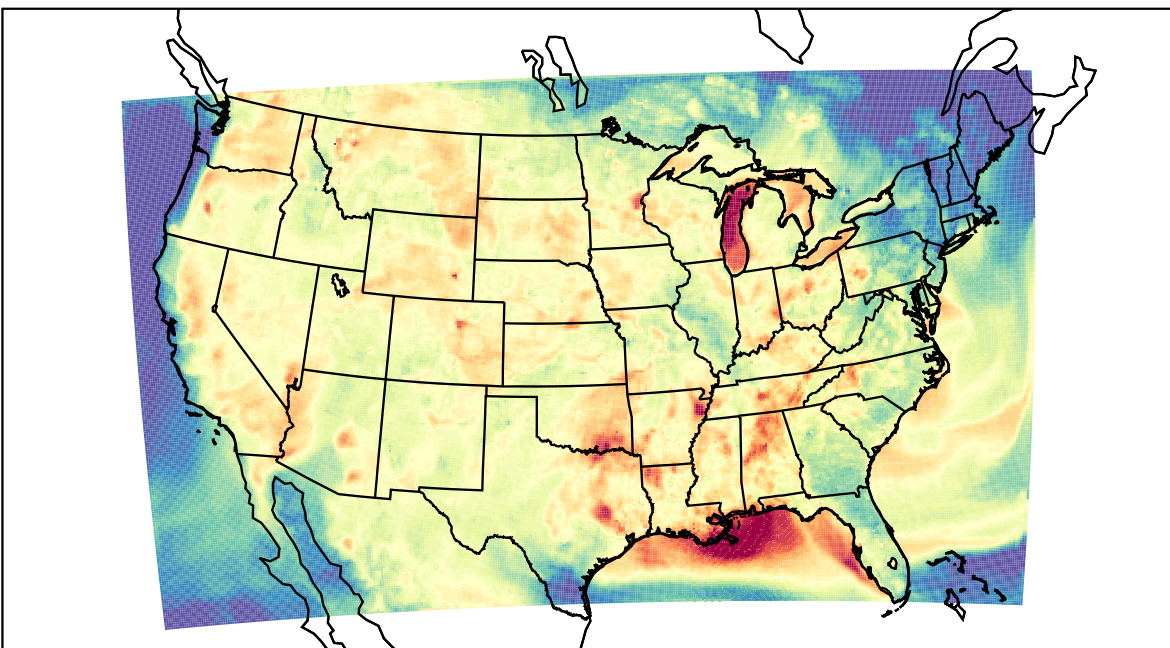
WRF (2023-08-03_01:00:00)
