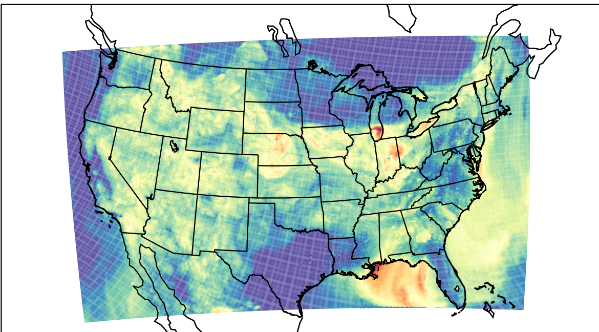
WRF (2023-08-04_10:00:00)
