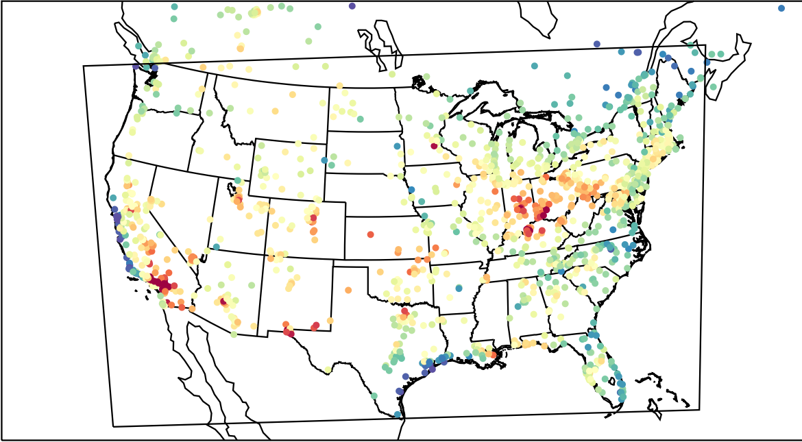
AirNOW (2023-08-04_21:00:00)
