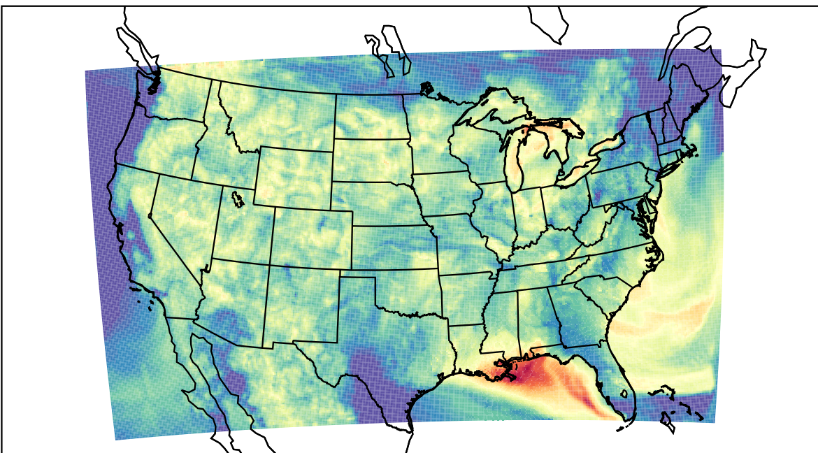
WRF (2023-08-03_09:00:00)
