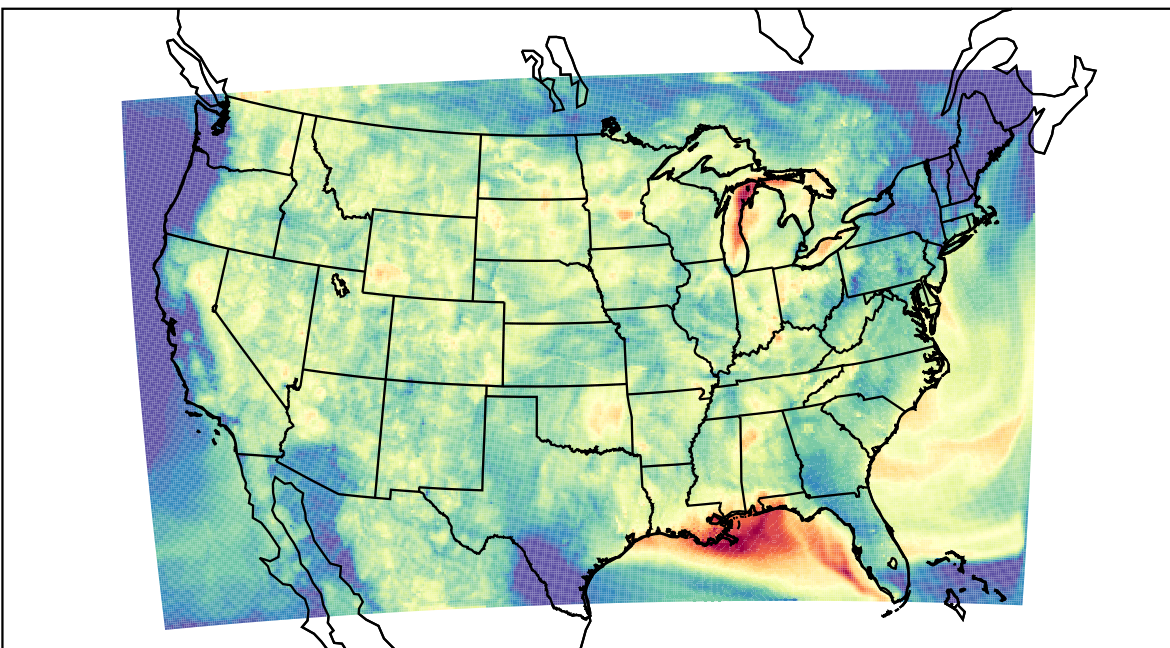
WRF (2023-08-03_06:00:00)
