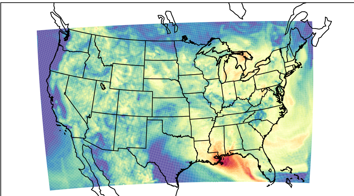
WRF (2023-08-03_14:00:00)
