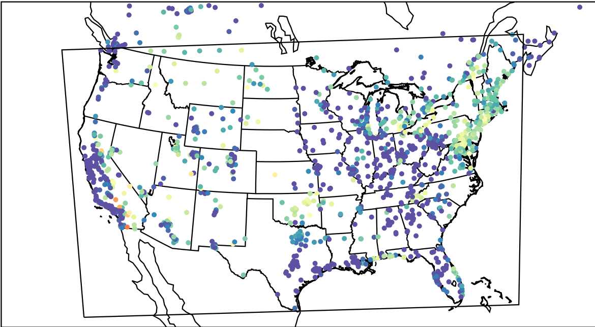
AirNOW (2023-08-04_08:00:00)
