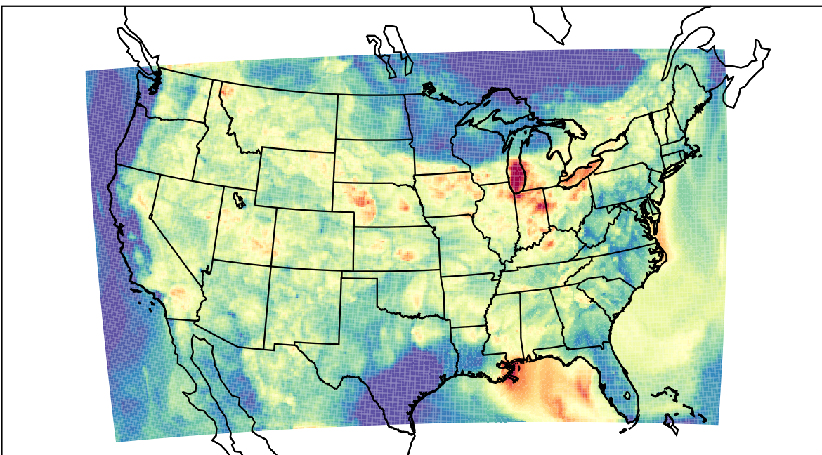
WRF (2023-08-04_05:00:00)
