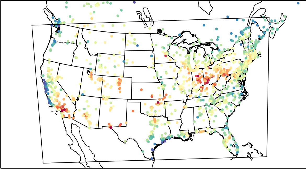
AirNOW (2023-08-04_19:00:00)
