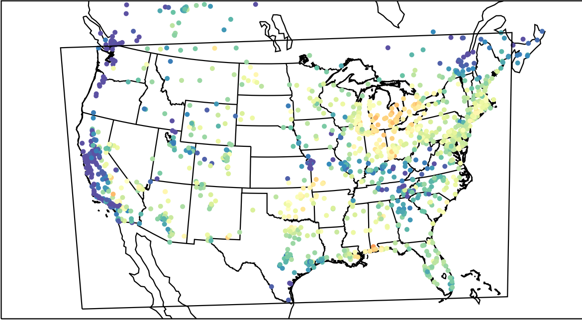
AirNOW (2023-08-03_15:00:00)
