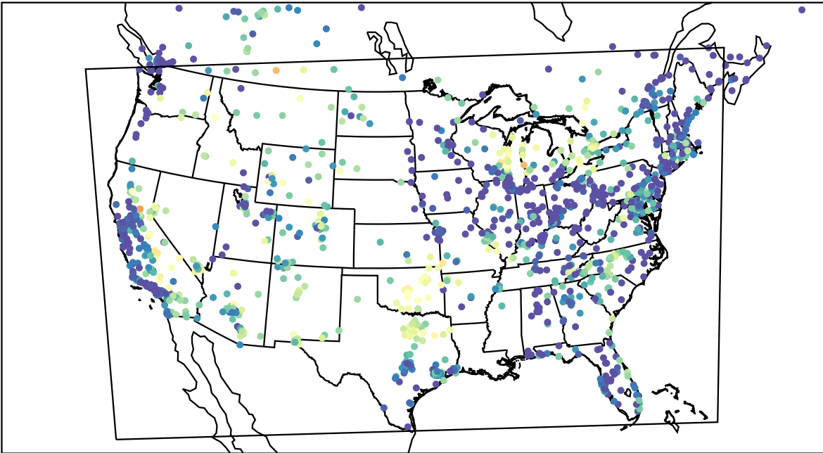
AirNOW (2023-08-03_07:00:00)
