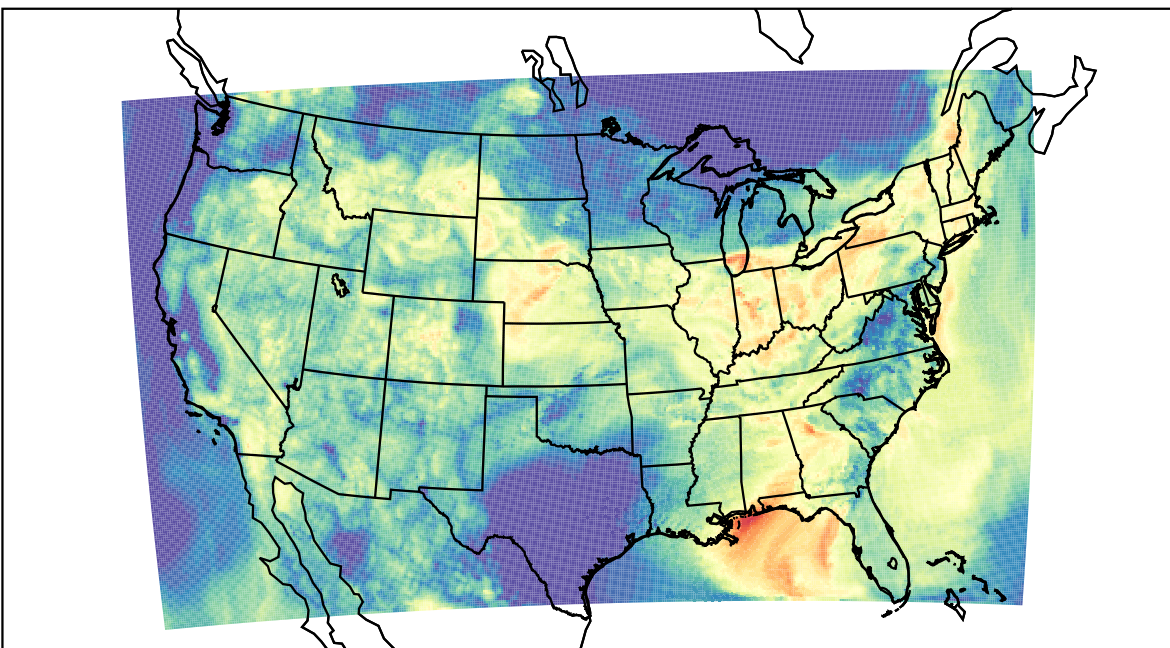
WRF (2023-08-04_14:00:00)
