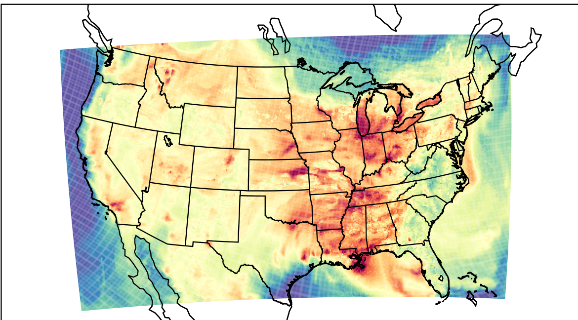
WRF (2023-08-03_23:00:00)
