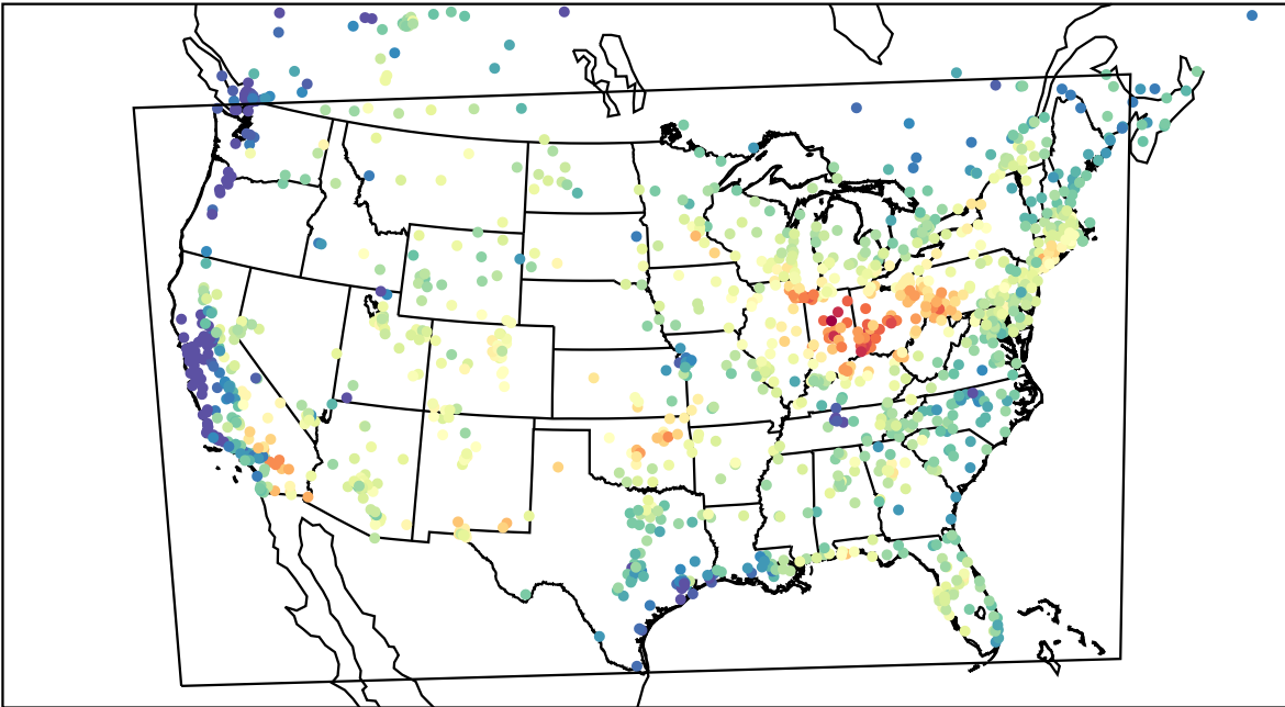
AirNOW (2023-08-04_16:00:00)
