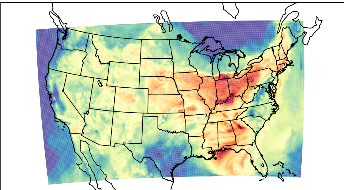
WRF (2023-08-04_16:00:00)
