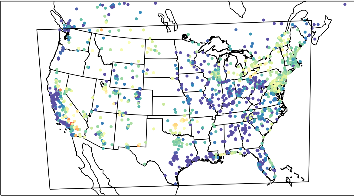
AirNOW (2023-08-04_05:00:00)
