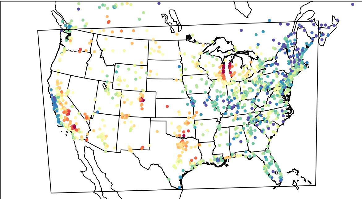
AirNOW (2023-08-03_00:00:00)
