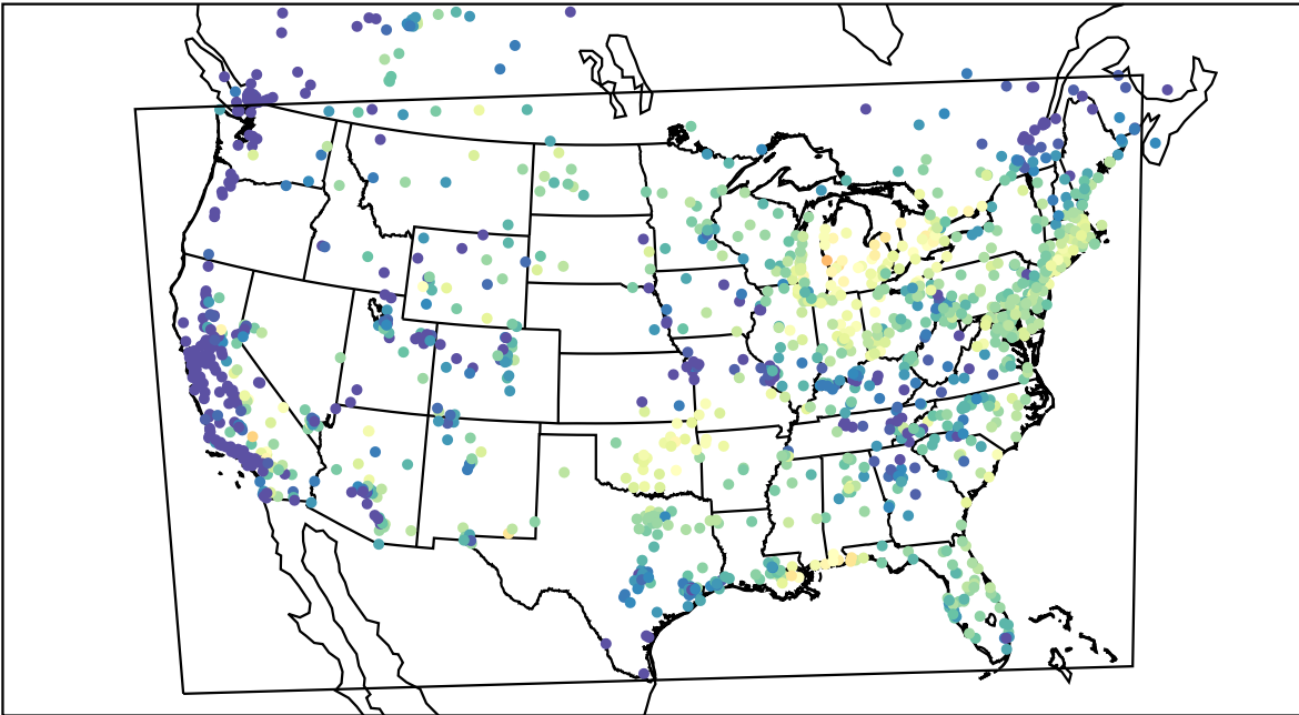
AirNOW (2023-08-03_14:00:00)
