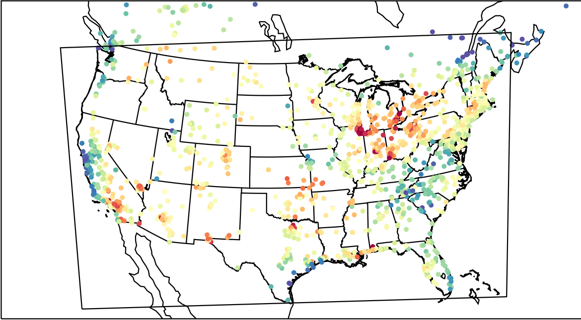
AirNOW (2023-08-03_19:00:00)
