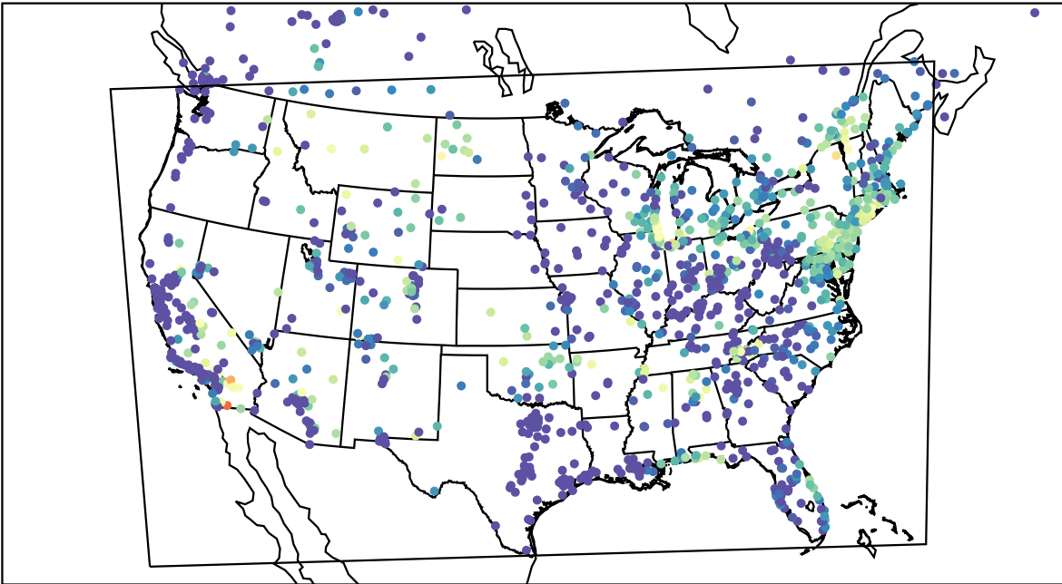
AirNOW (2023-08-04_12:00:00)
