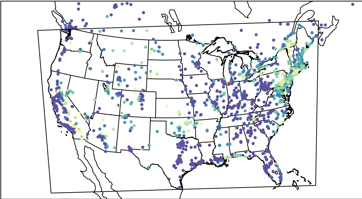
AirNOW (2023-08-04_10:00:00)
