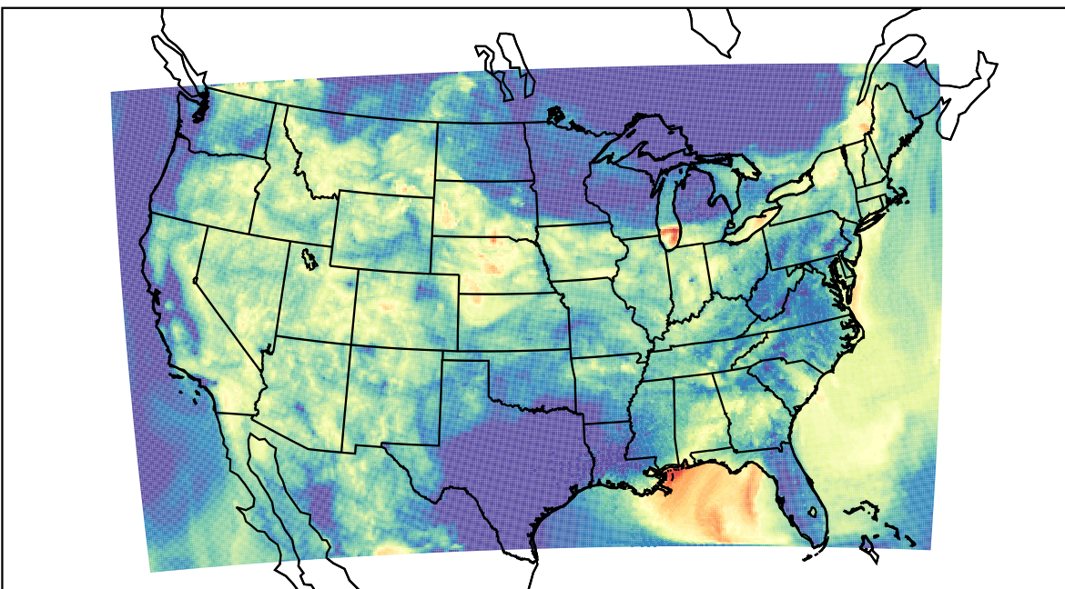
WRF (2023-08-04_12:00:00)
