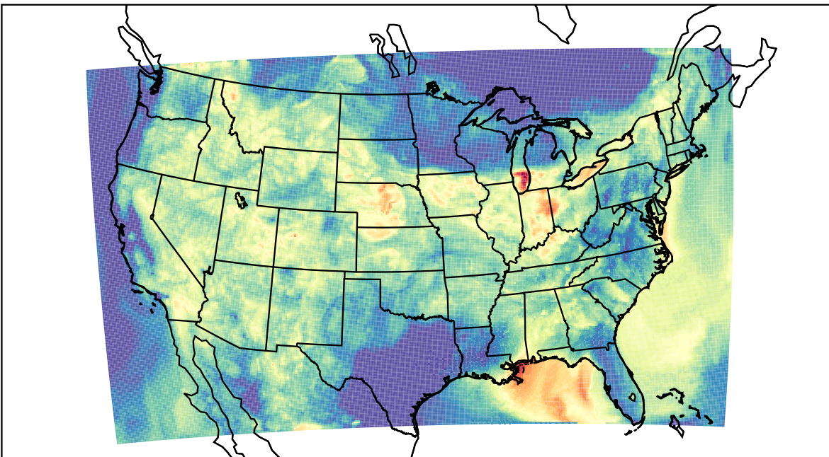
WRF (2023-08-04_09:00:00)
