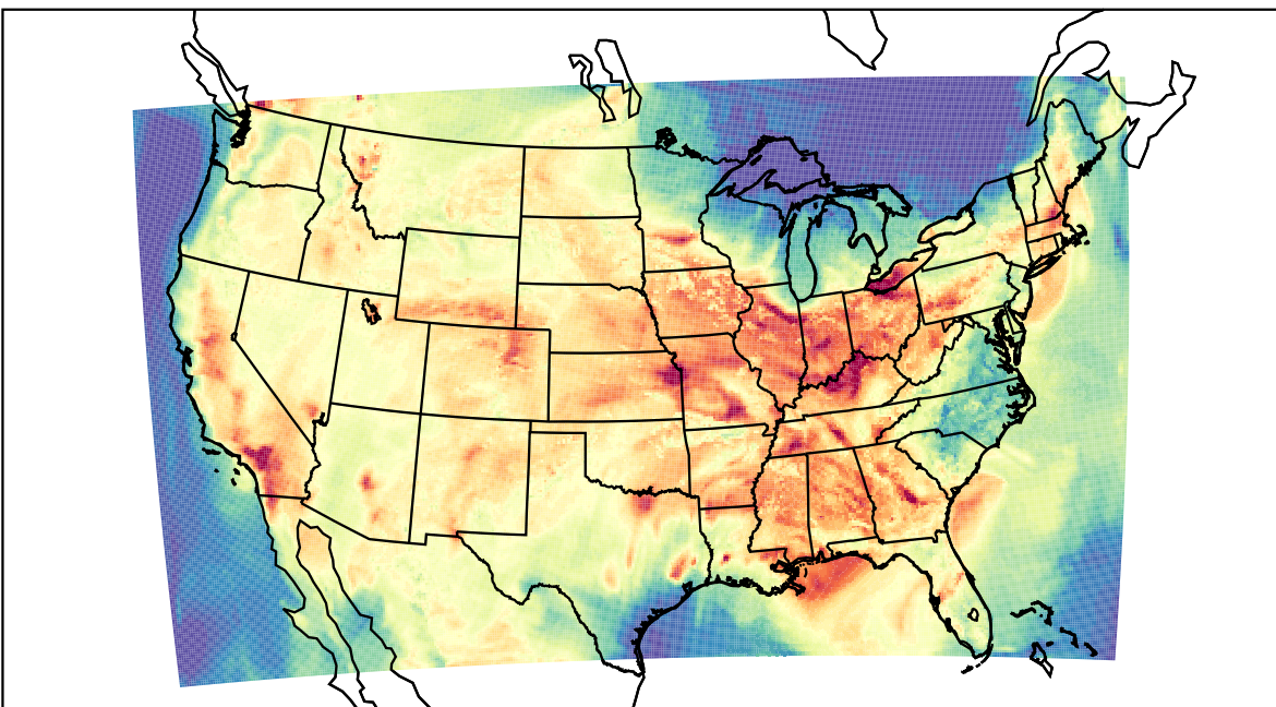
WRF (2023-08-04_23:00:00)
