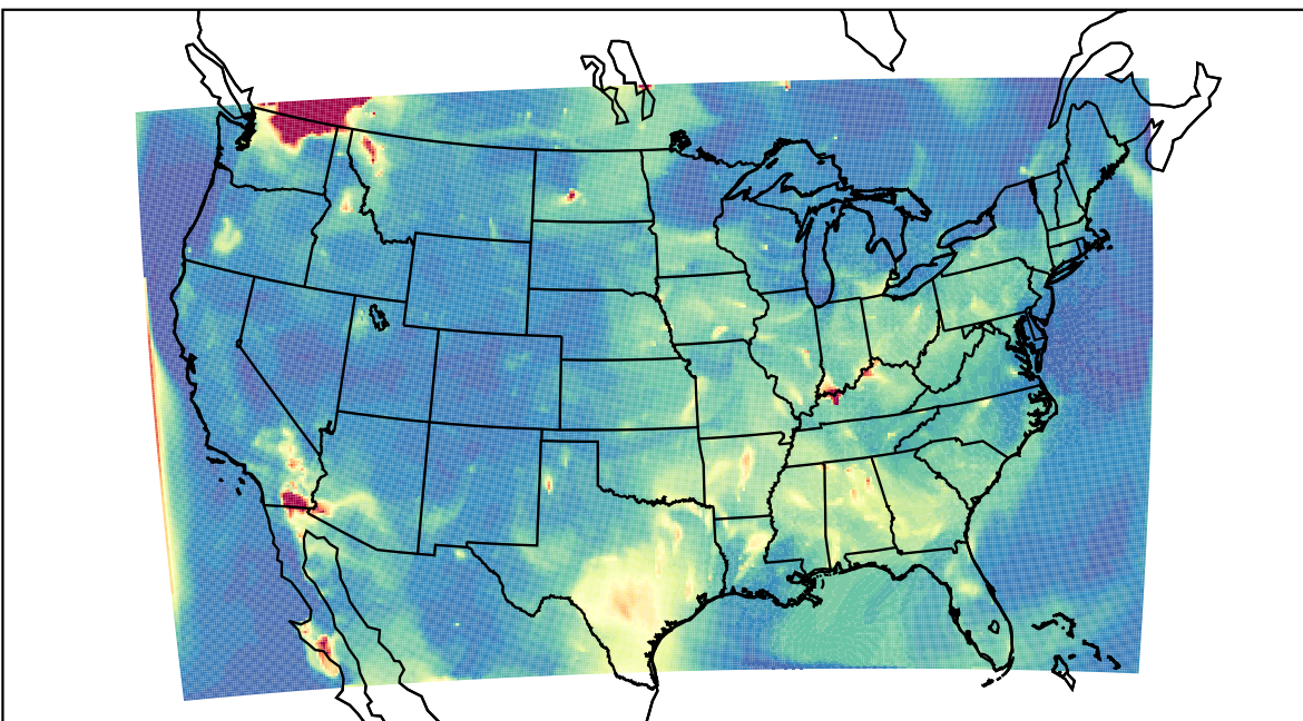
WRF 2023-08-05_07:00:00
