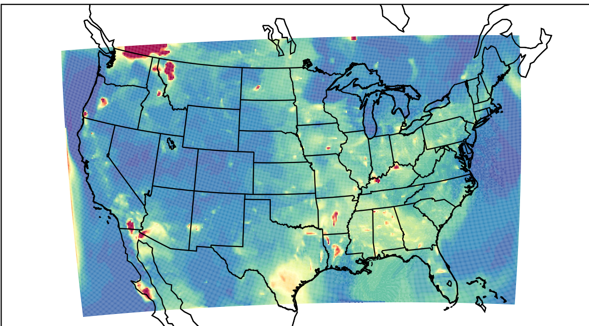
WRF 2023-08-05_04:00:00
