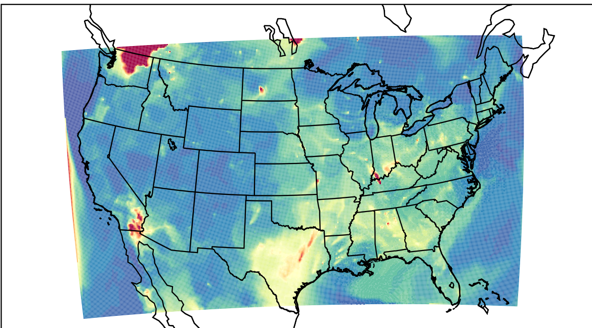
WRF 2023-08-05_11:00:00
