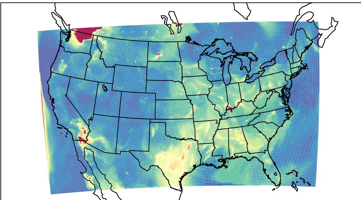
WRF 2023-08-05_09:00:00
