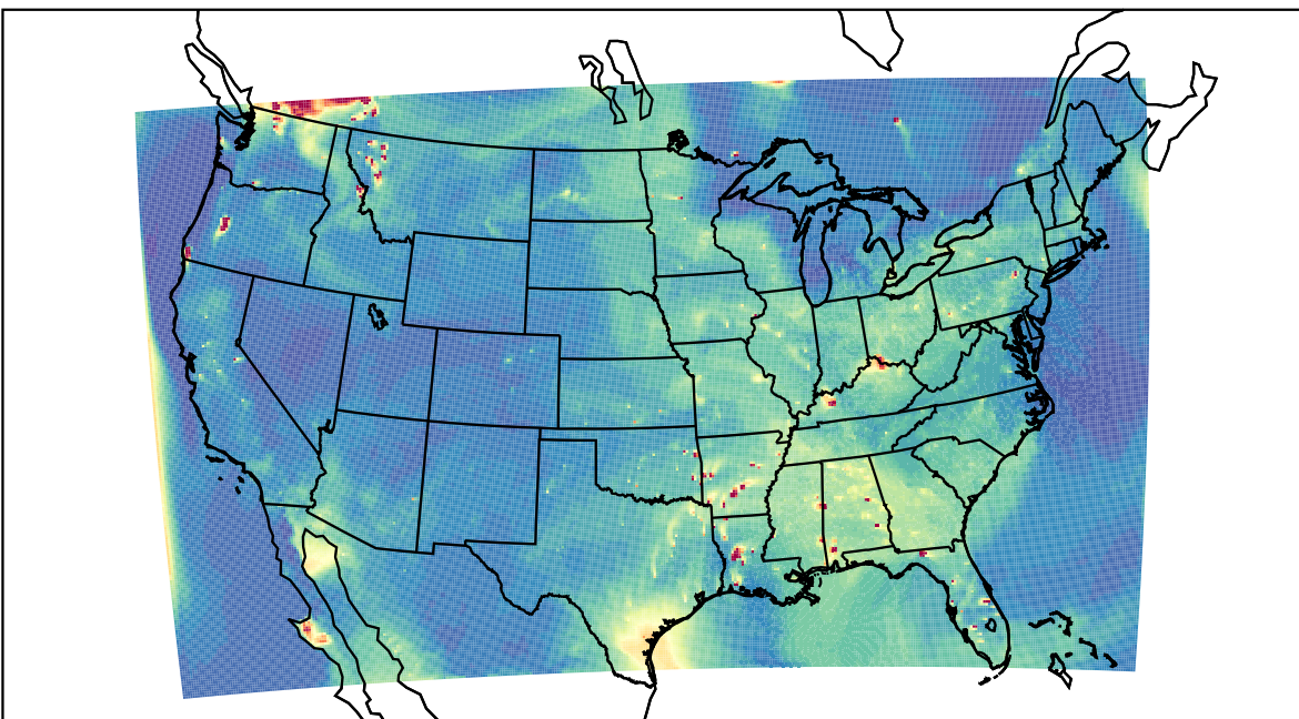
WRF 2023-08-05_00:00:00
