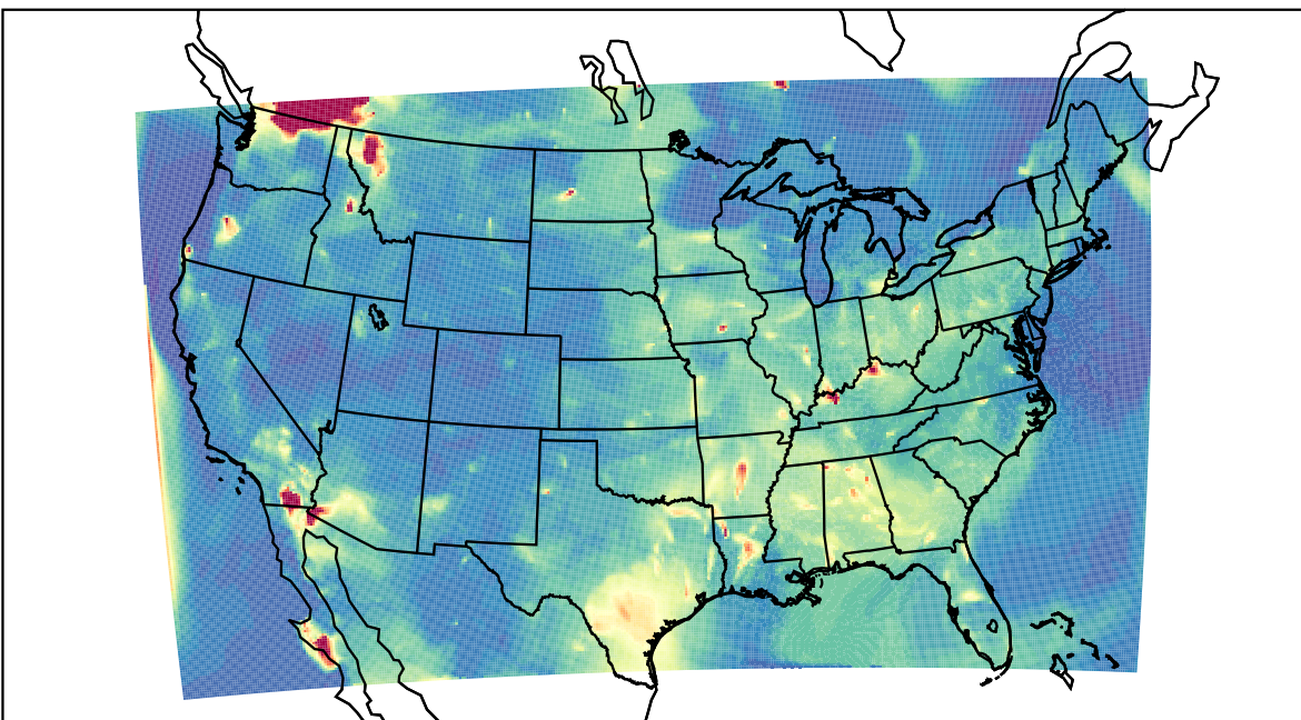
WRF 2023-08-05_05:00:00
