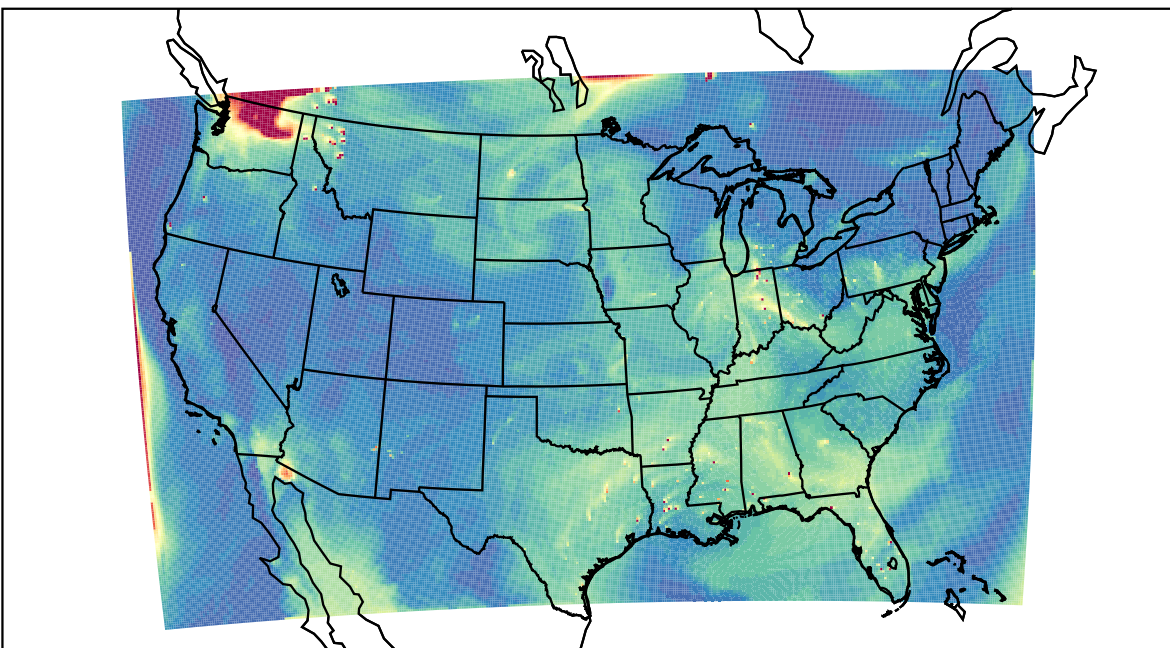
WRF 2023-08-05_21:00:00
