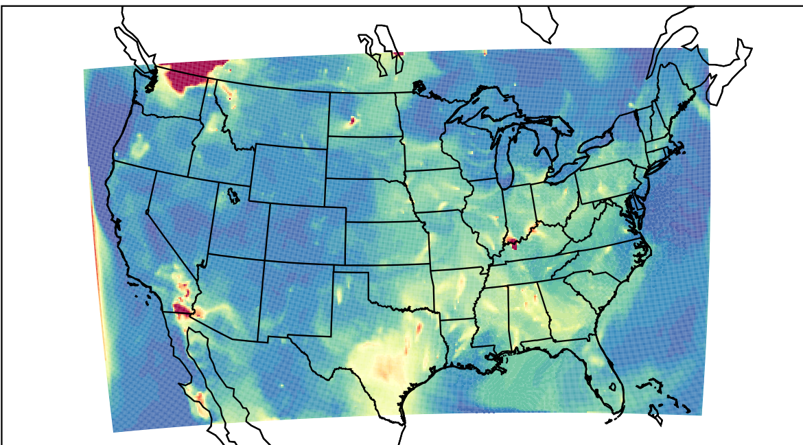
WRF 2023-08-05_08:00:00
