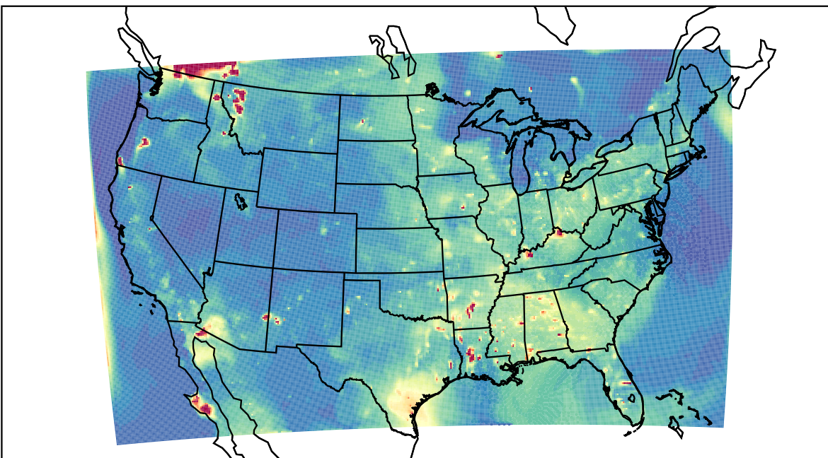
WRF 2023-08-05_02:00:00
