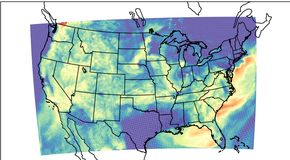
WRF (2023-08-06_11:00:00)
