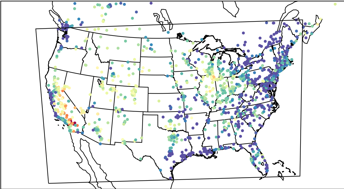
AirNOW (2023-08-06_03:00:00)
