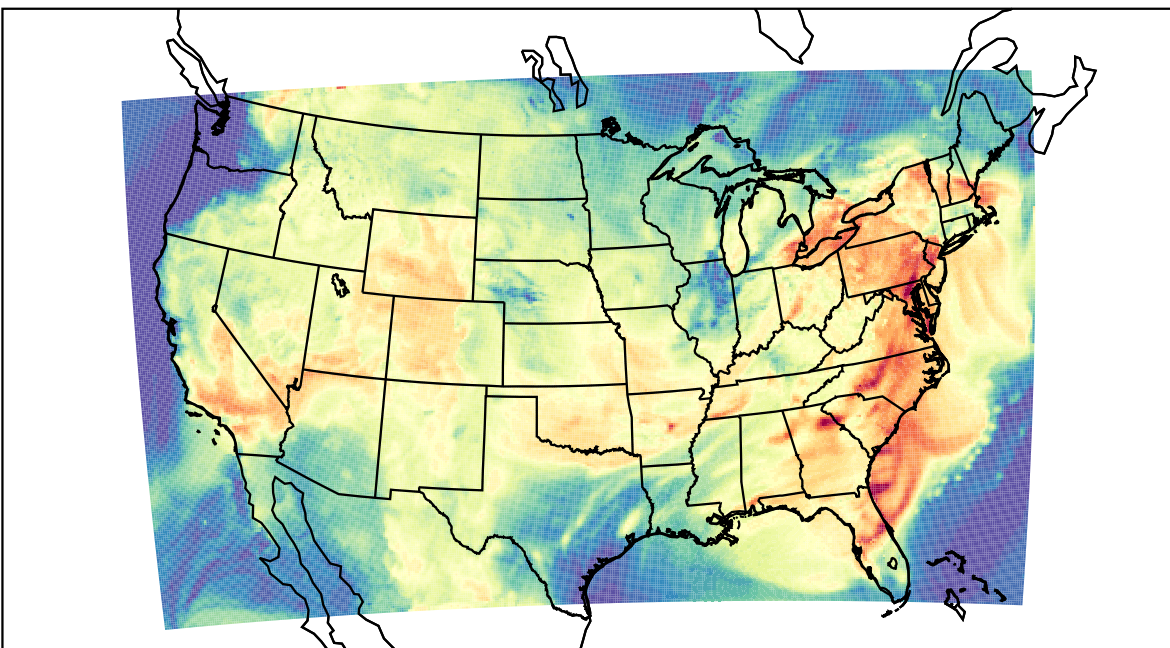
WRF (2023-08-07_17:00:00)
