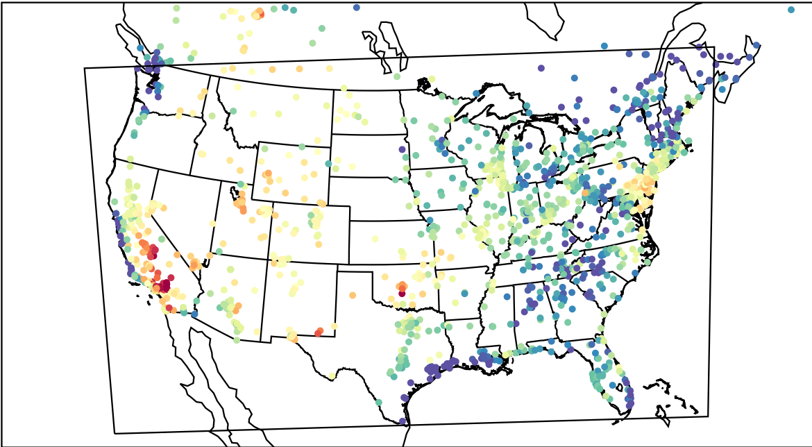
AirNOW (2023-08-07_00:00:00)
