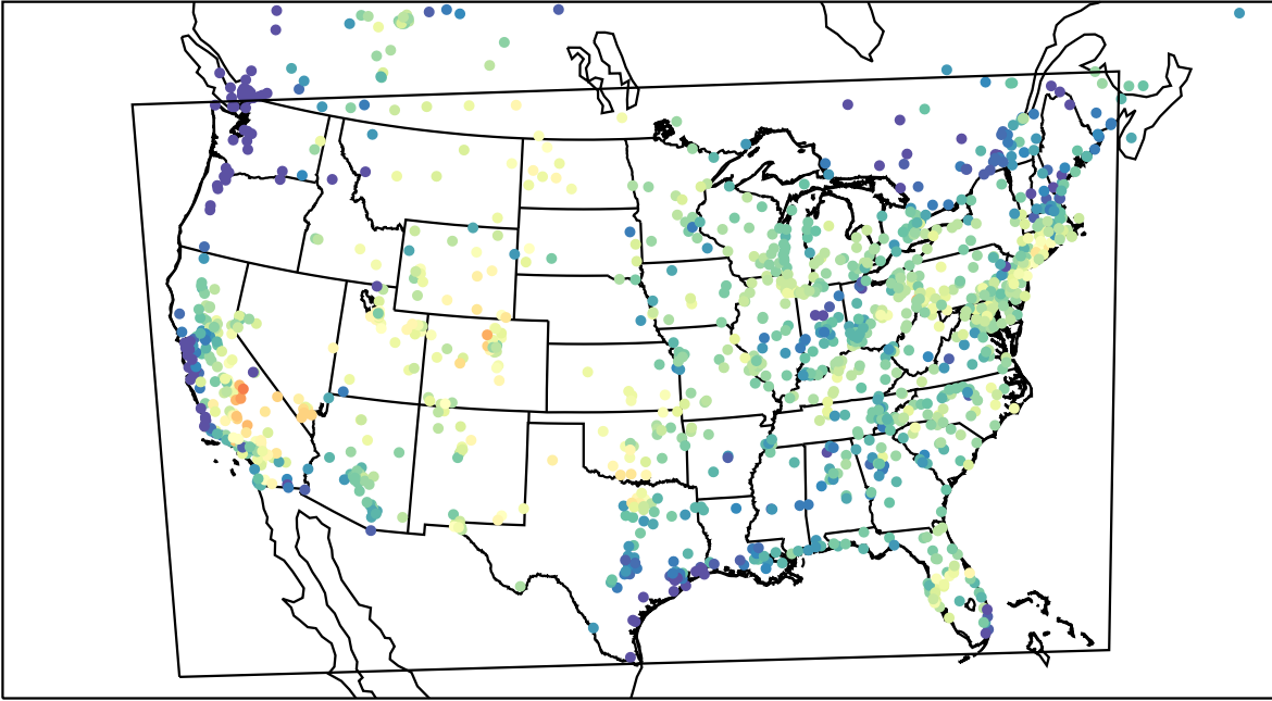
AirNOW (2023-08-07_16:00:00)
