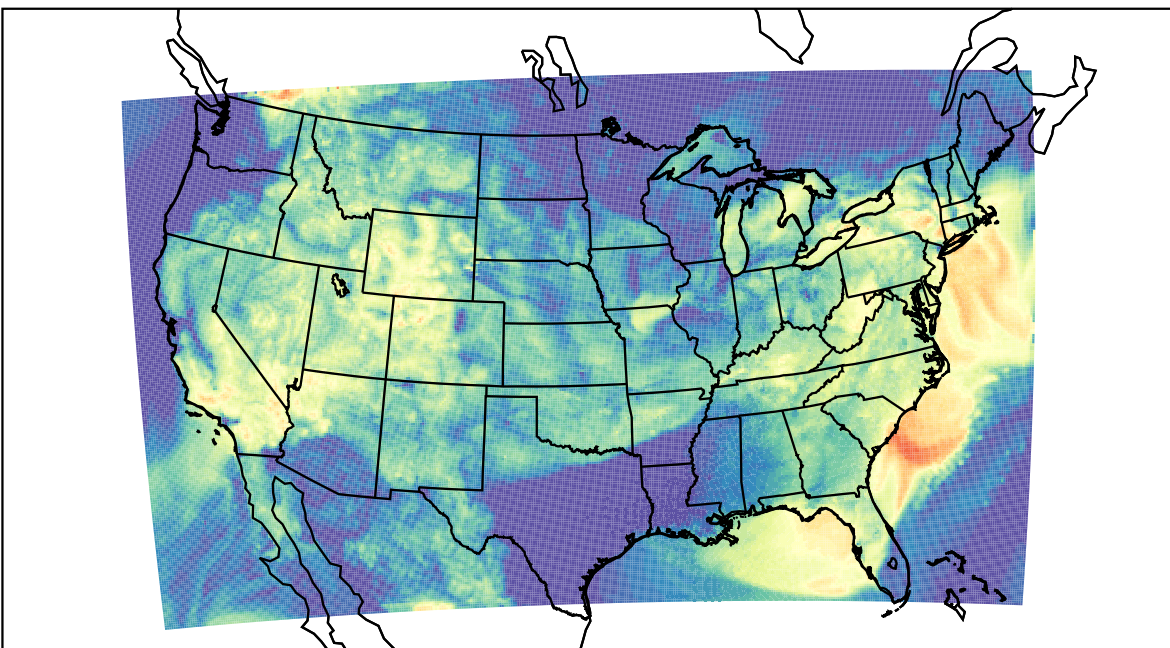
WRF (2023-08-07_13:00:00)
