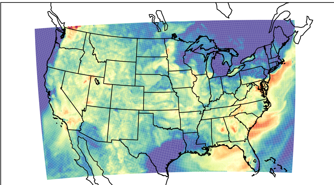
WRF (2023-08-06_06:00:00)
