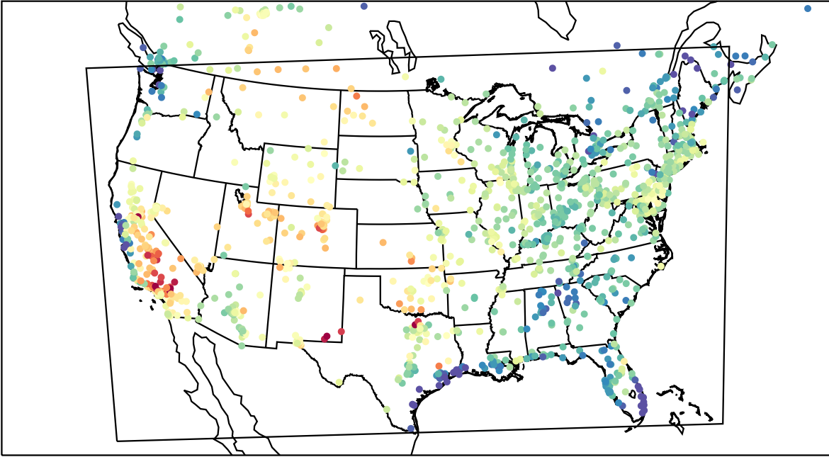
AirNOW (2023-08-07_23:00:00)
