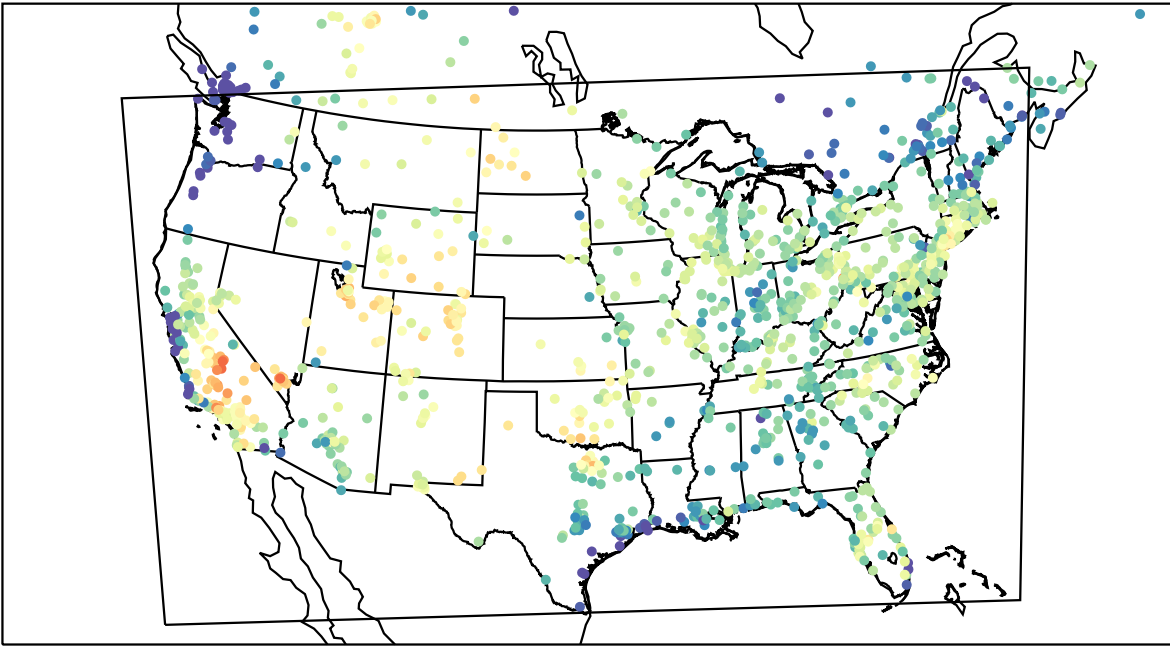
AirNOW (2023-08-07_17:00:00)
