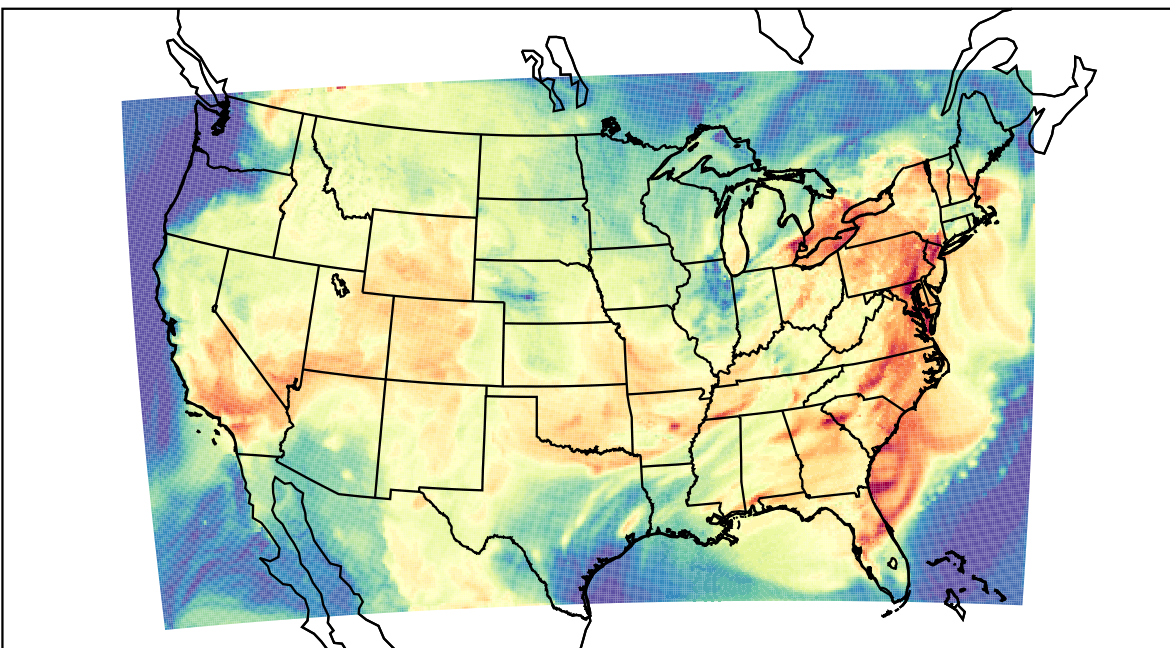
WRF (2023-08-07_18:00:00)
