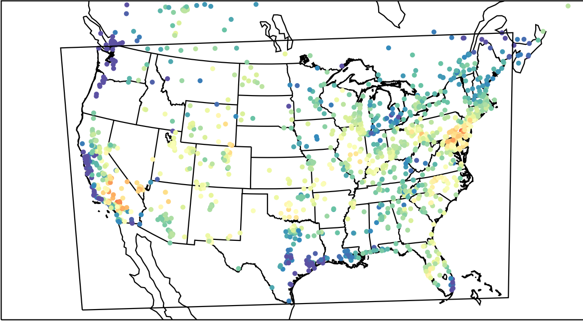
AirNOW (2023-08-06_16:00:00)
