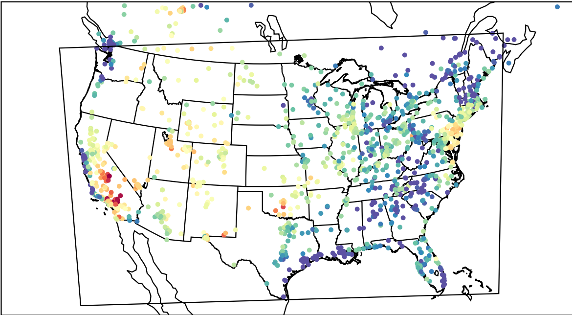
AirNOW (2023-08-07_01:00:00)
