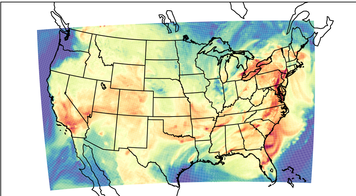
WRF (2023-08-07_19:00:00)
