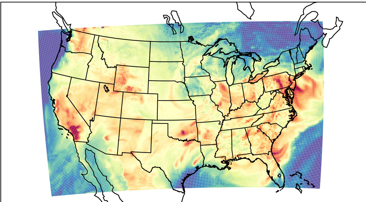
WRF (2023-08-06_23:00:00)
