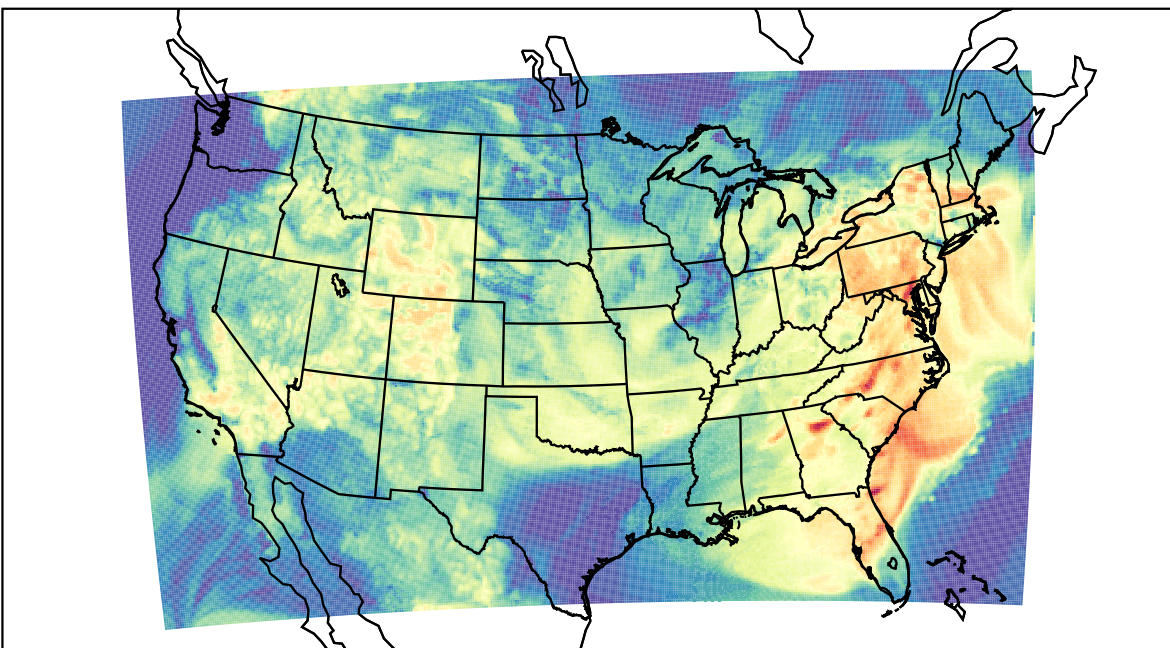
WRF (2023-08-07_15:00:00)
