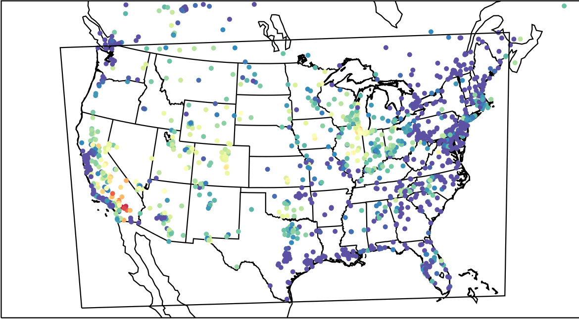
AirNOW (2023-08-06_05:00:00)
