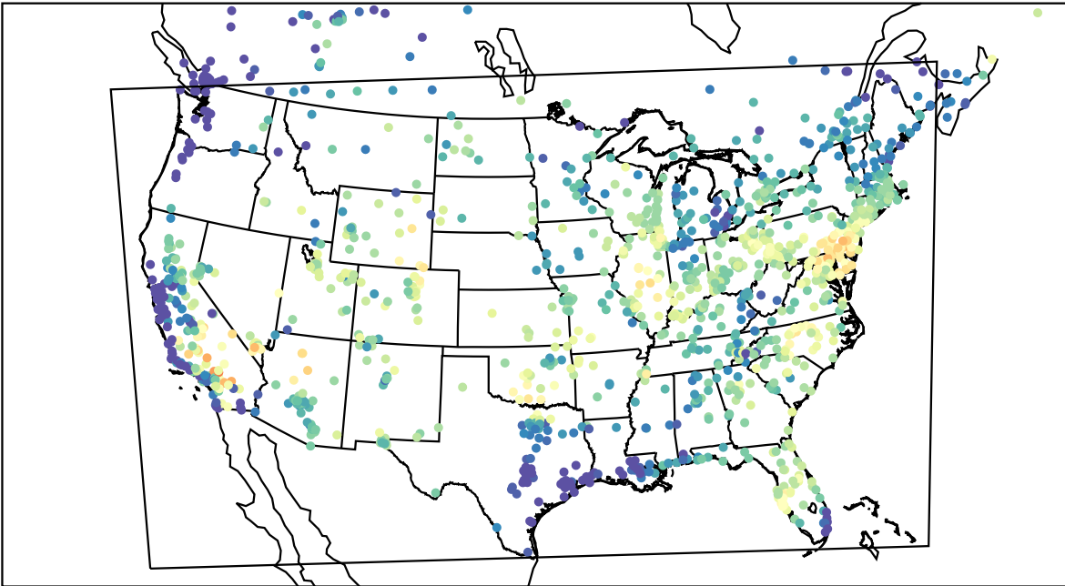
AirNOW (2023-08-06_15:00:00)
