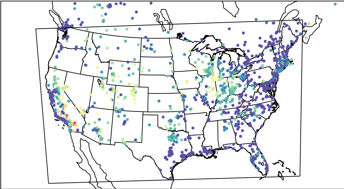
AirNOW (2023-08-06_06:00:00)
