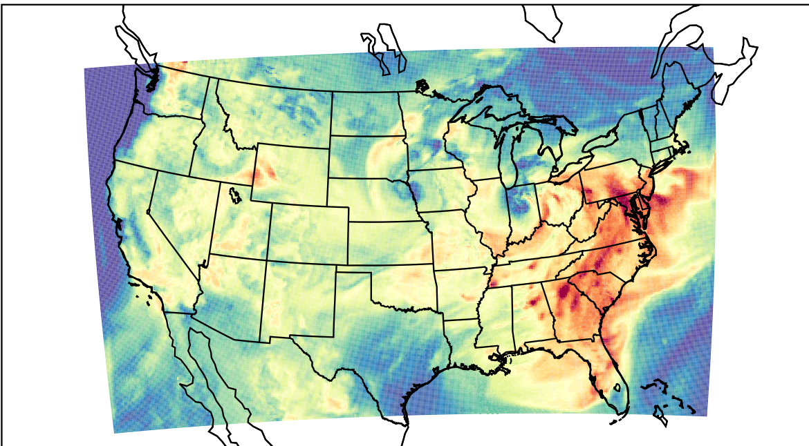
WRF (2023-08-06_16:00:00)
