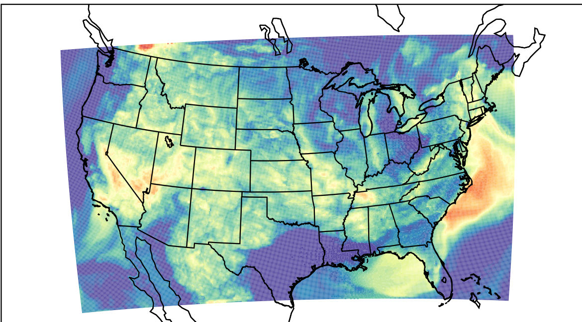
WRF (2023-08-08_09:00:00)
