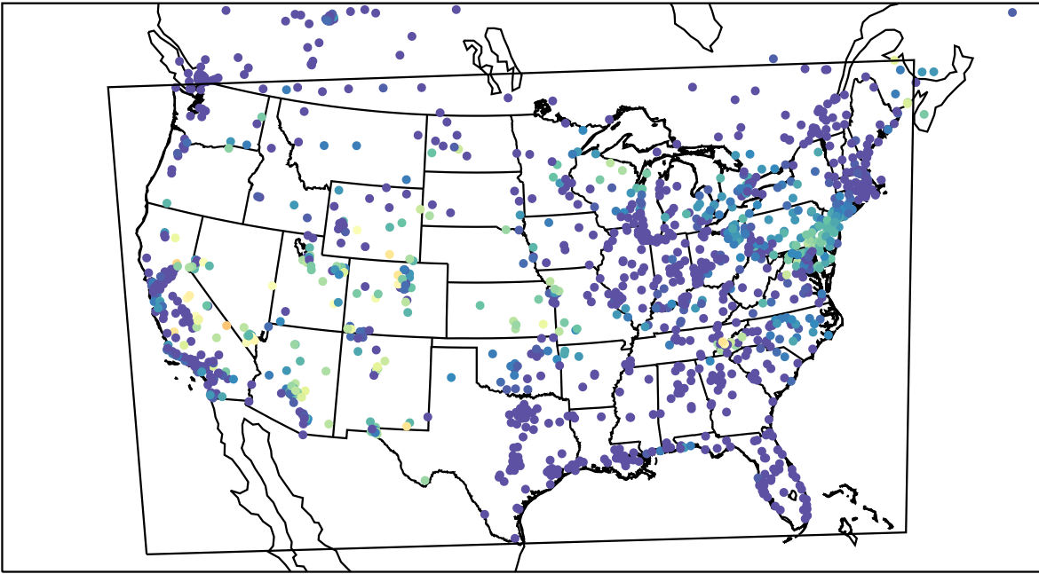
AirNOW (2023-08-09_12:00:00)
