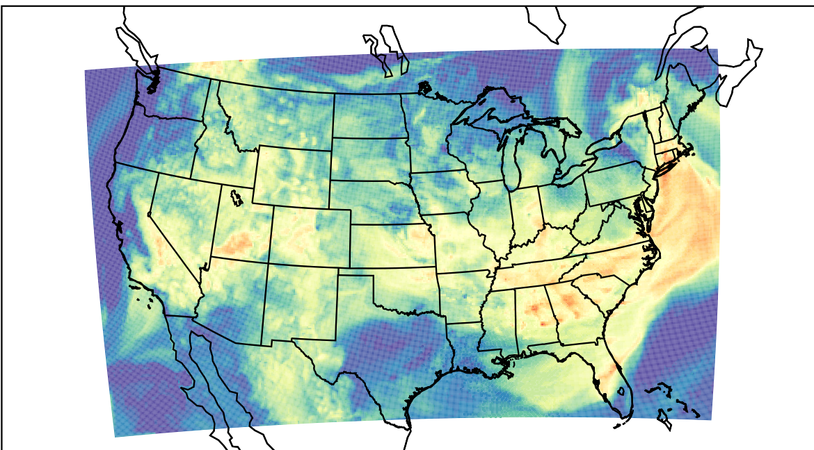
WRF (2023-08-08_15:00:00)
