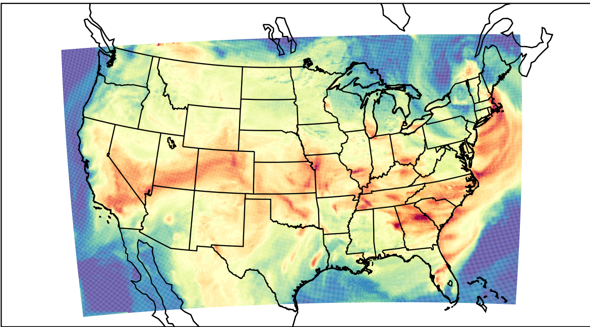
WRF (2023-08-08_21:00:00)
