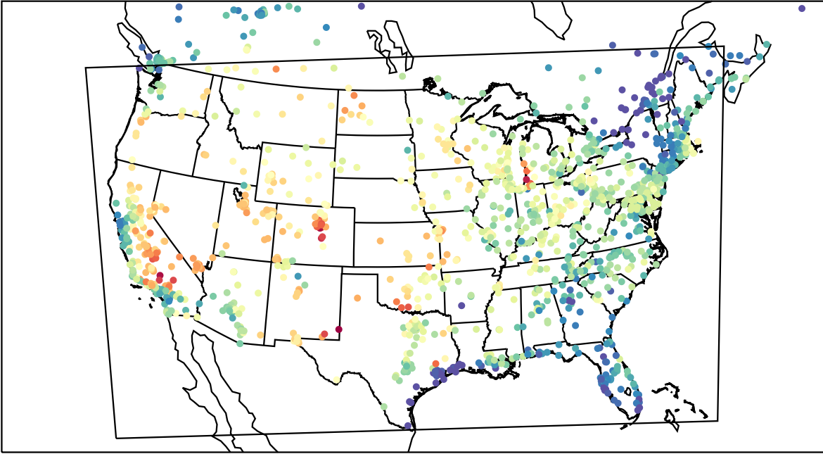
AirNOW (2023-08-08_23:00:00)
