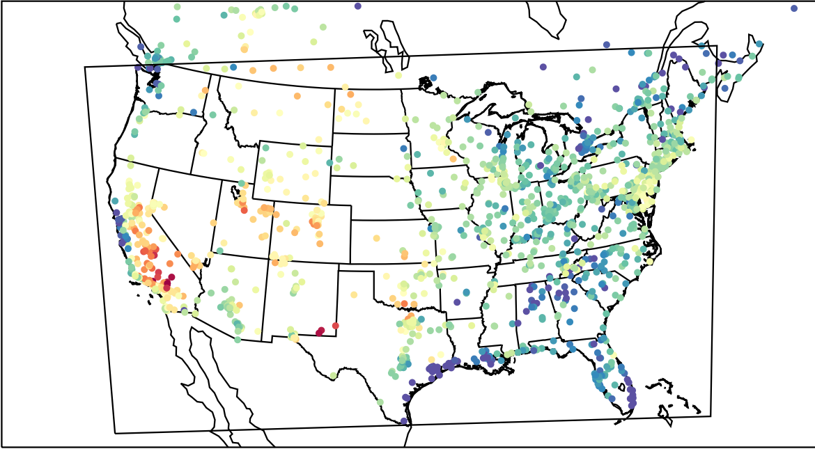
AirNOW (2023-08-08_00:00:00)
