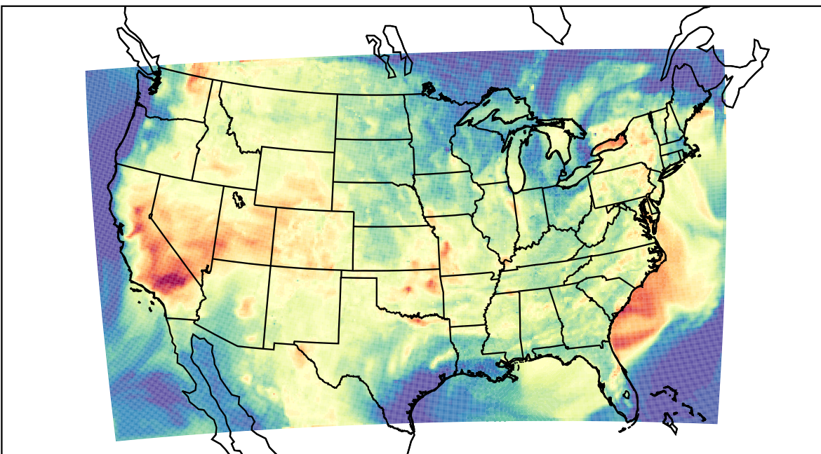
WRF (2023-08-08_01:00:00)
