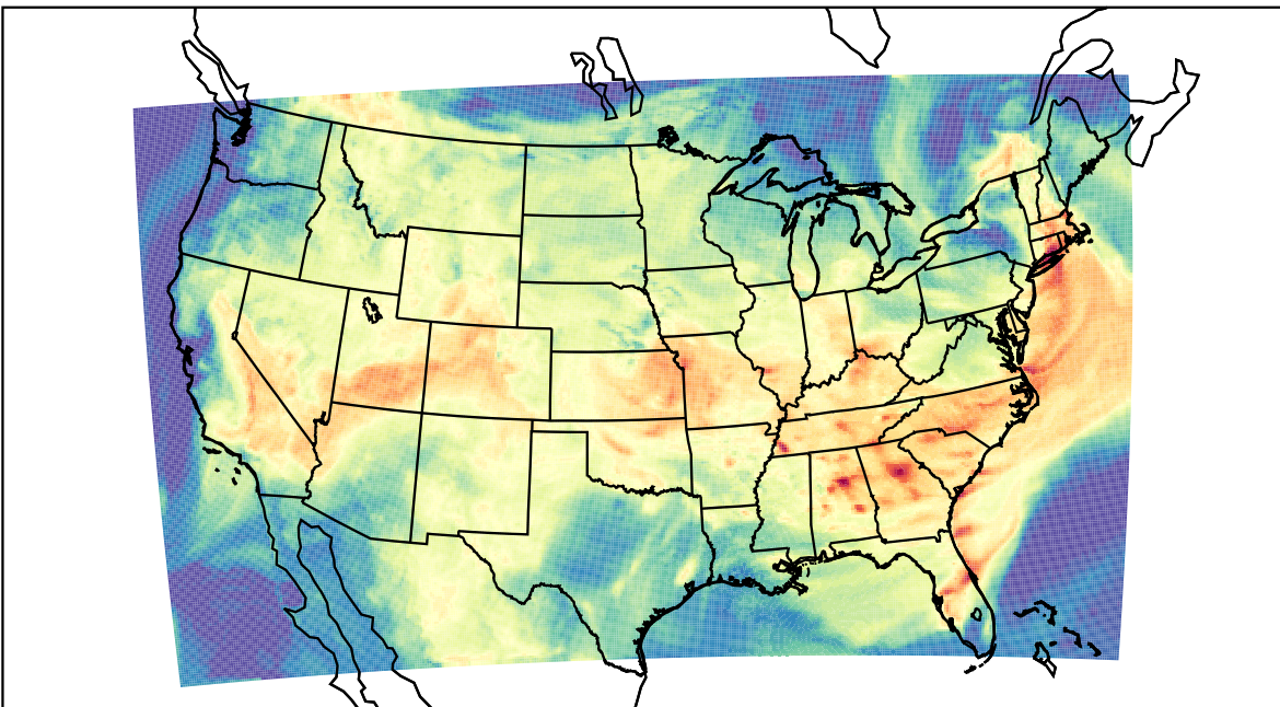
WRF (2023-08-08_17:00:00)
