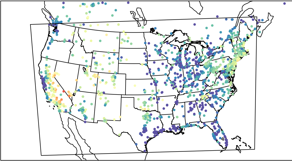
AirNOW (2023-08-08_03:00:00)
