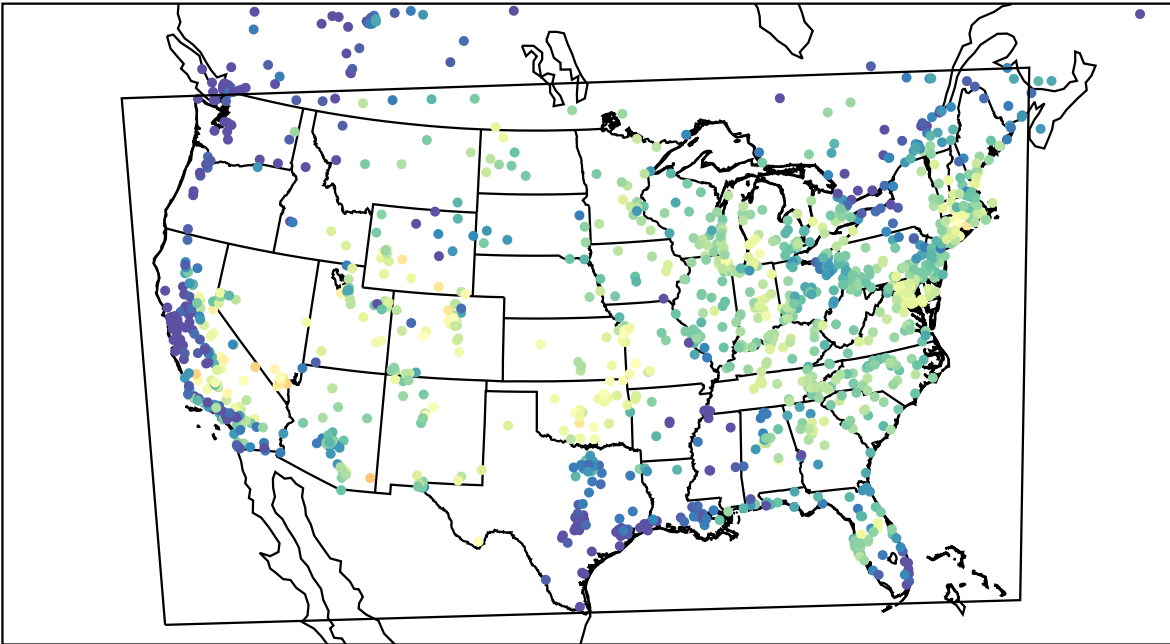
AirNOW (2023-08-08_15:00:00)
