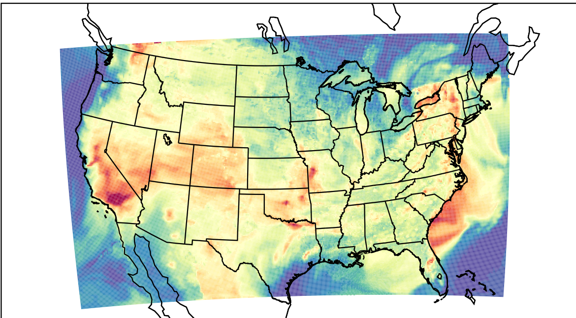
WRF (2023-08-08_00:00:00)
