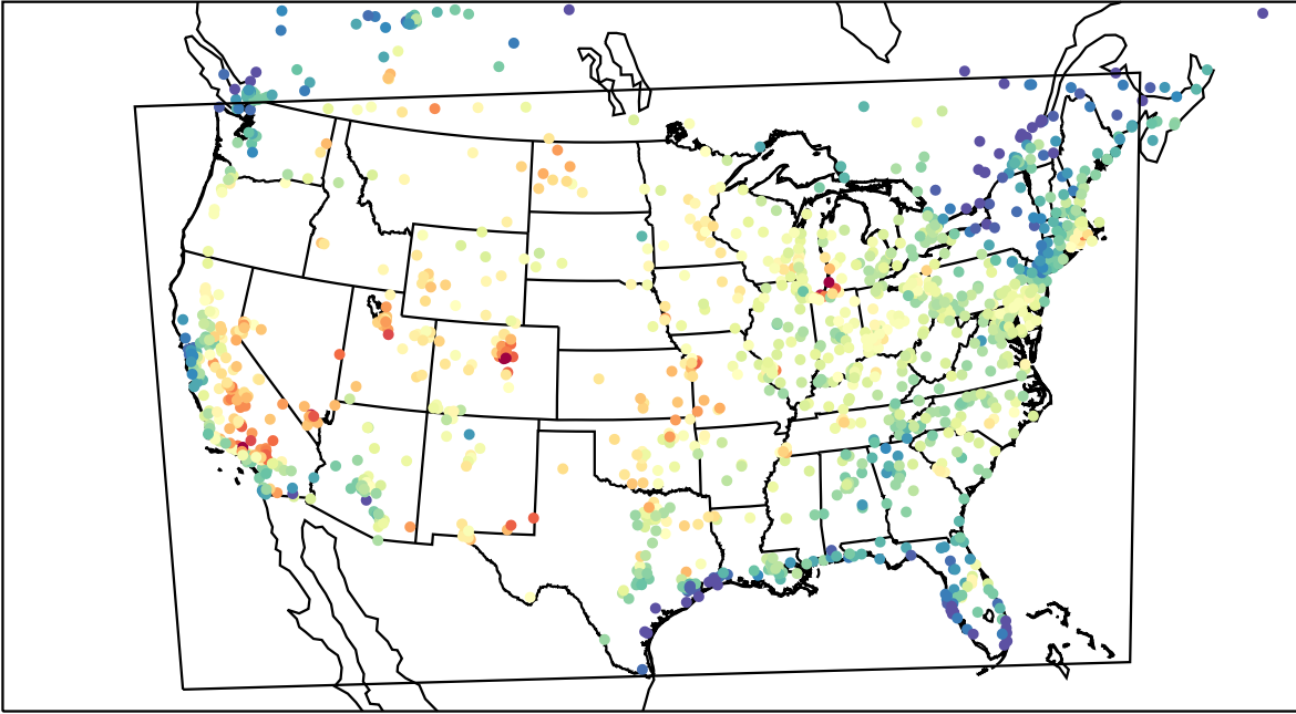
AirNOW (2023-08-08_21:00:00)
