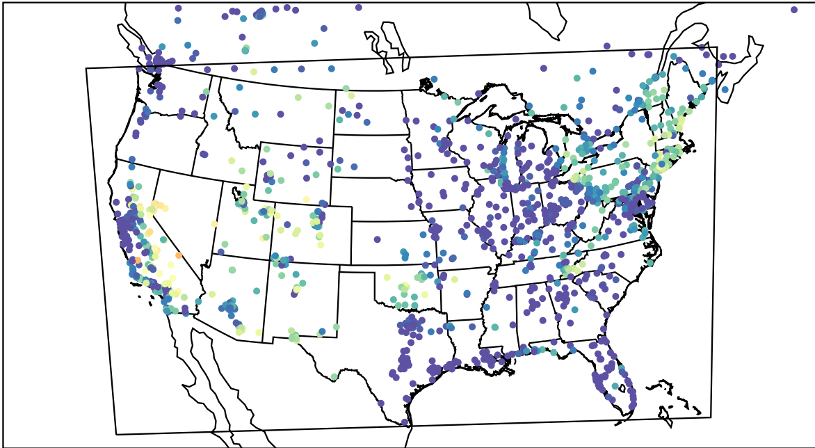
AirNOW (2023-08-08_08:00:00)
