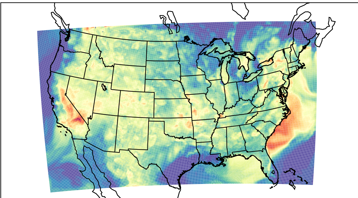
WRF (2023-08-08_03:00:00)
