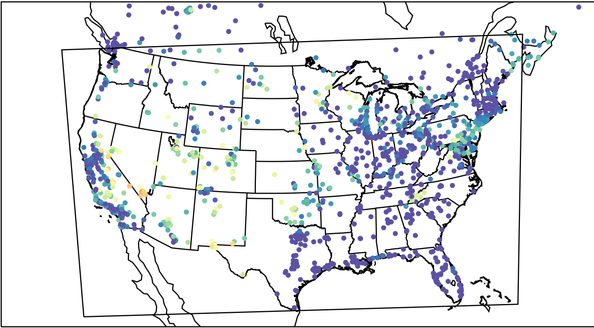
AirNOW (2023-08-09_08:00:00)
