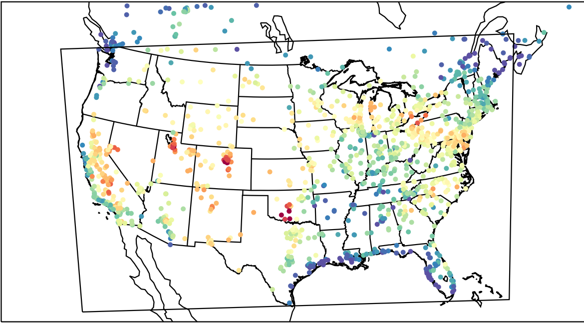
AirNOW (2023-08-09_22:00:00)
