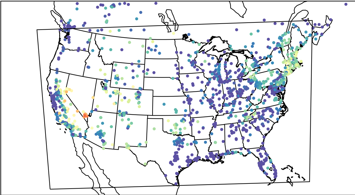
AirNOW (2023-08-08_07:00:00)
