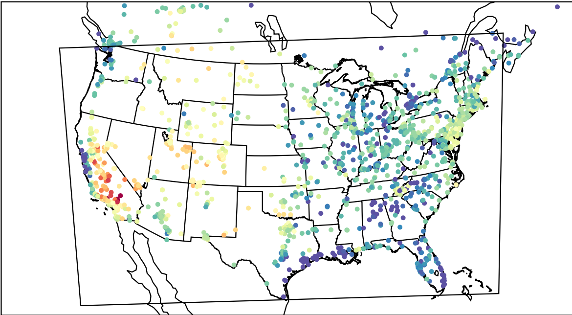
AirNOW (2023-08-08_01:00:00)
