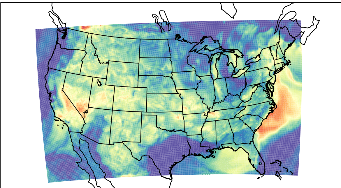
WRF (2023-08-08_07:00:00)
