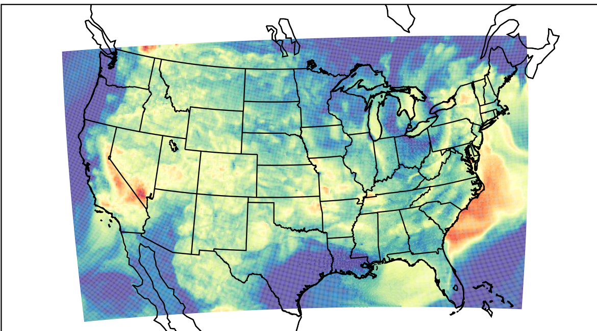
WRF (2023-08-08_05:00:00)
