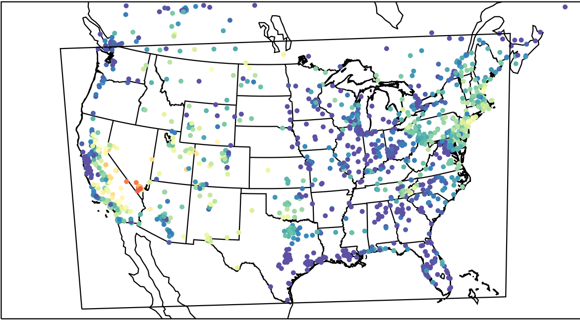
AirNOW (2023-08-08_05:00:00)
