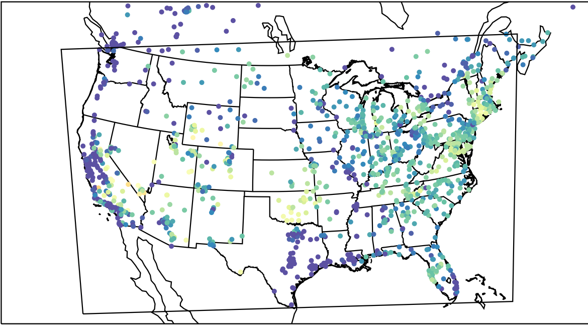
AirNOW (2023-08-08_14:00:00)
