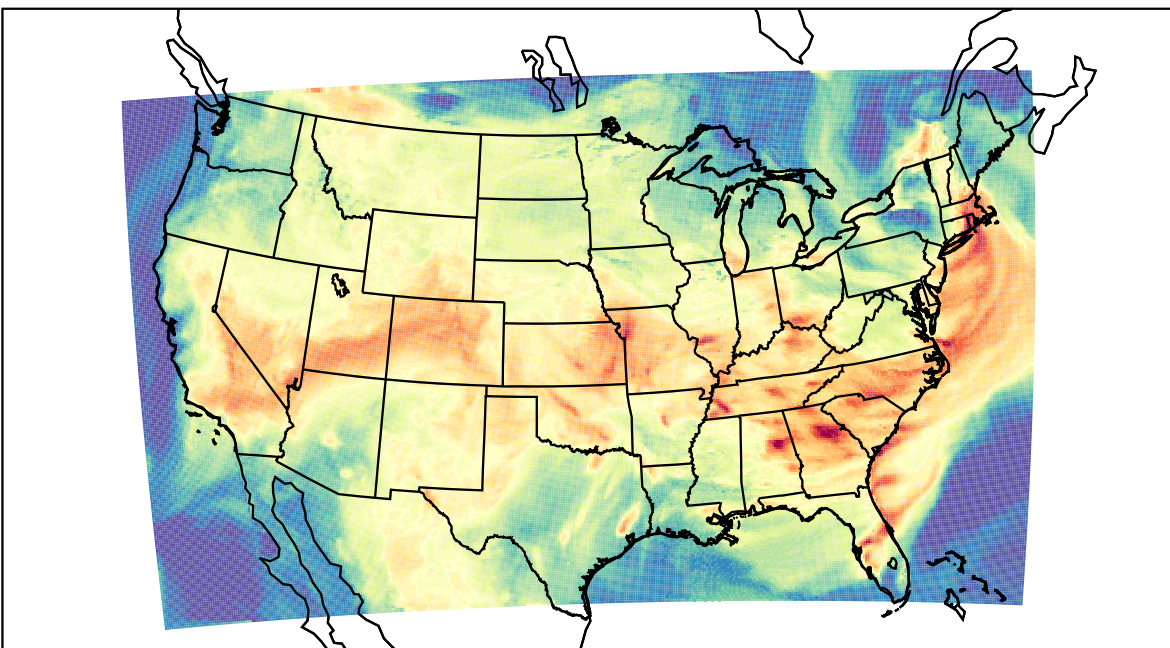
WRF (2023-08-08_19:00:00)
