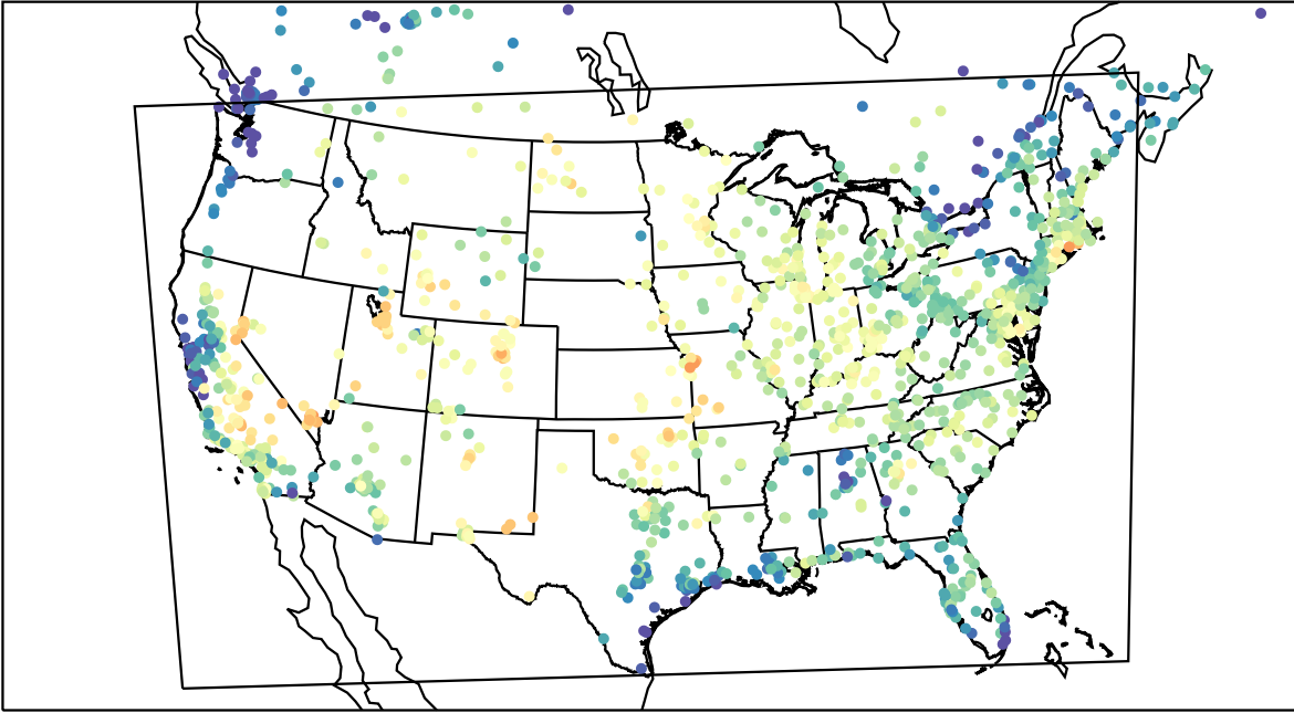
AirNOW (2023-08-08_17:00:00)
