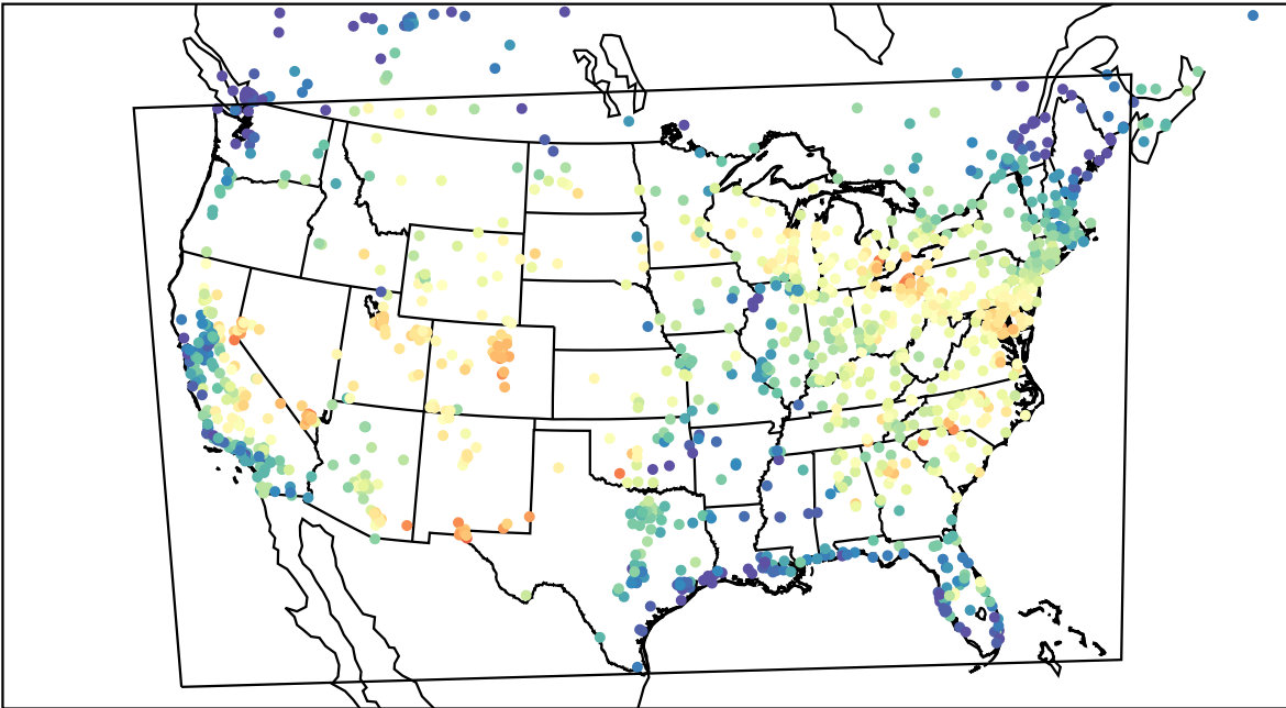
AirNOW (2023-08-09_17:00:00)
