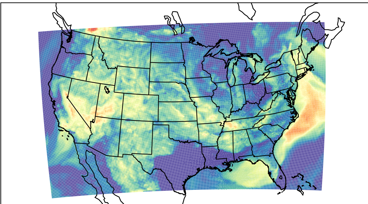
WRF (2023-08-08_11:00:00)
