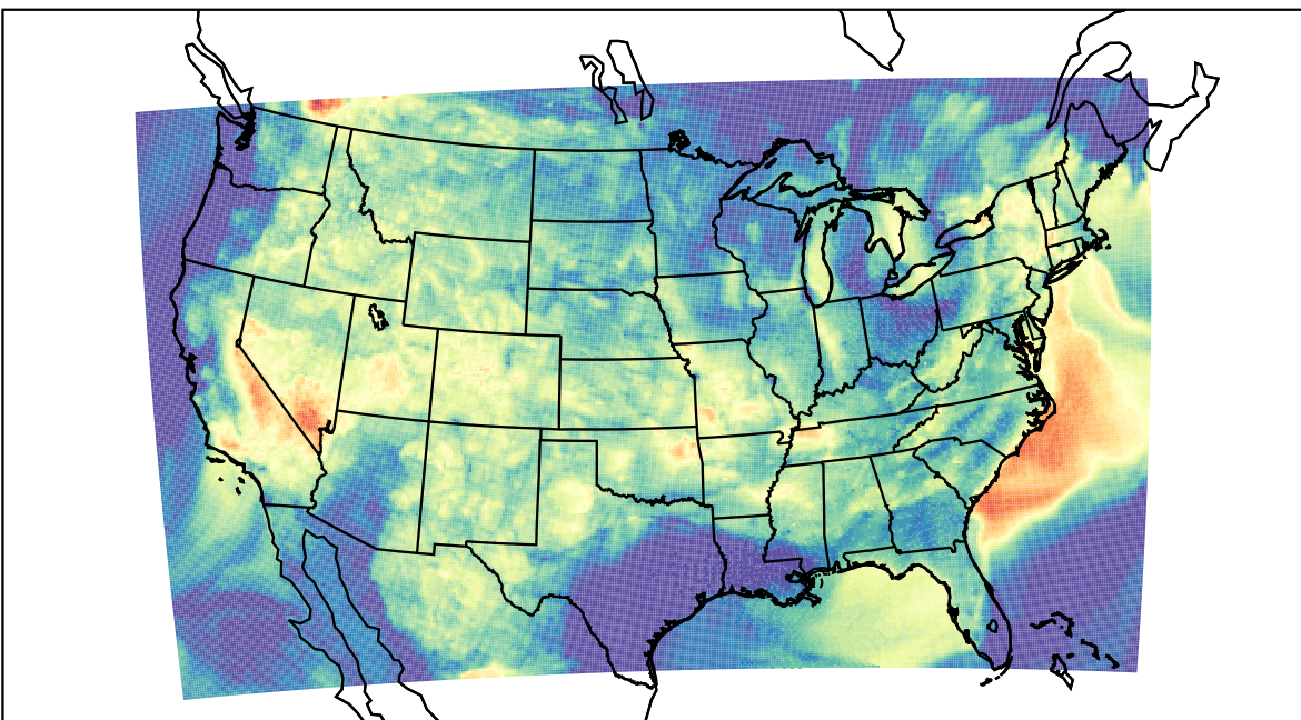
WRF (2023-08-08_06:00:00)
