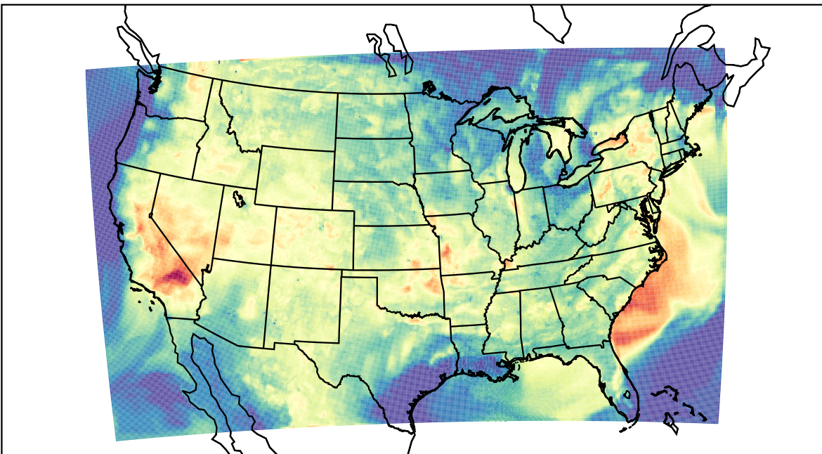
WRF (2023-08-08_02:00:00)
