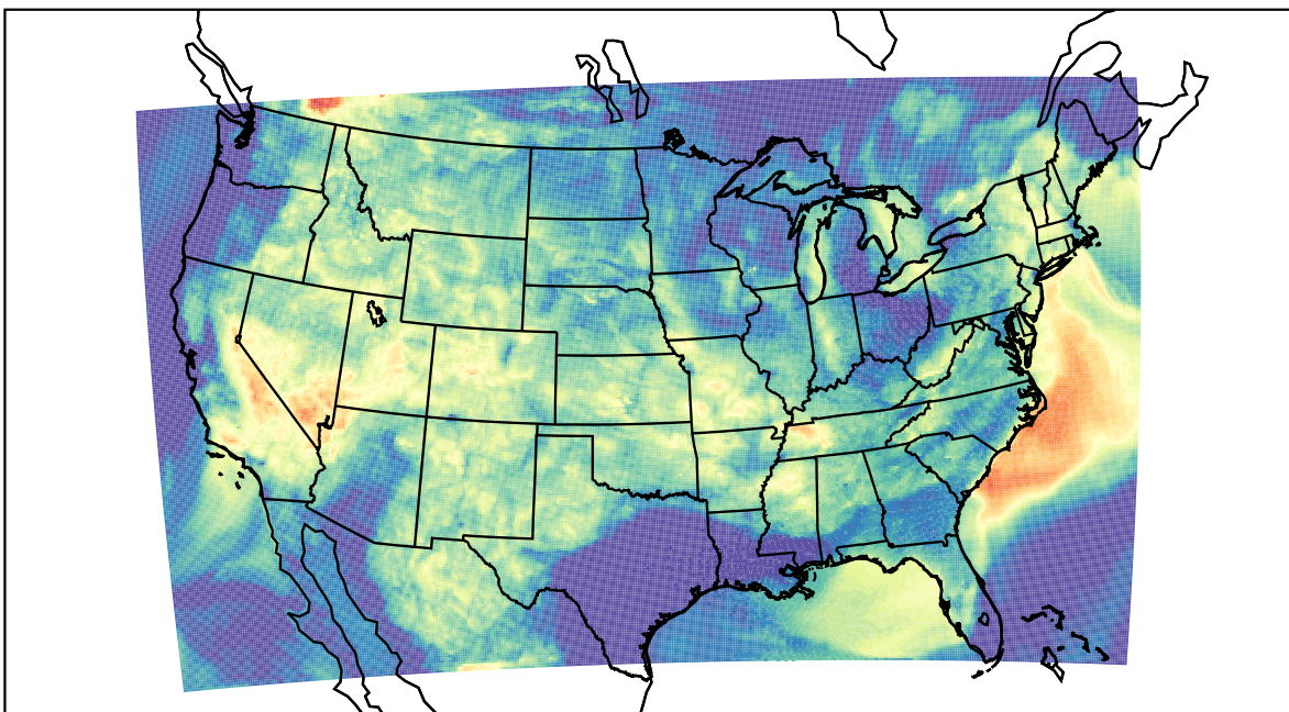
WRF (2023-08-08_08:00:00)
