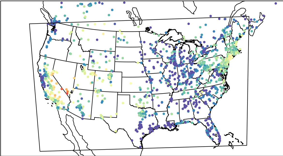
AirNOW (2023-08-08_04:00:00)
