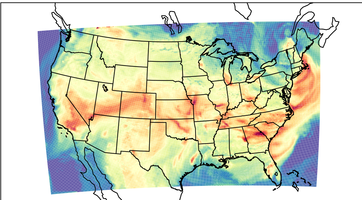
WRF (2023-08-08_22:00:00)
