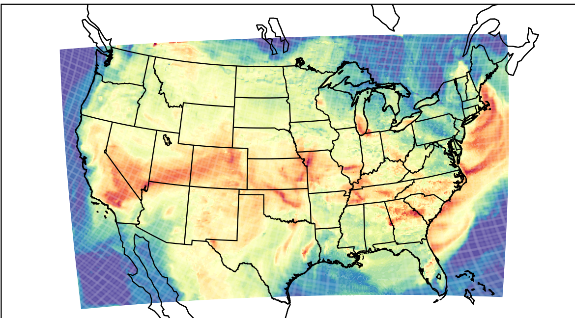
WRF (2023-08-08_23:00:00)
