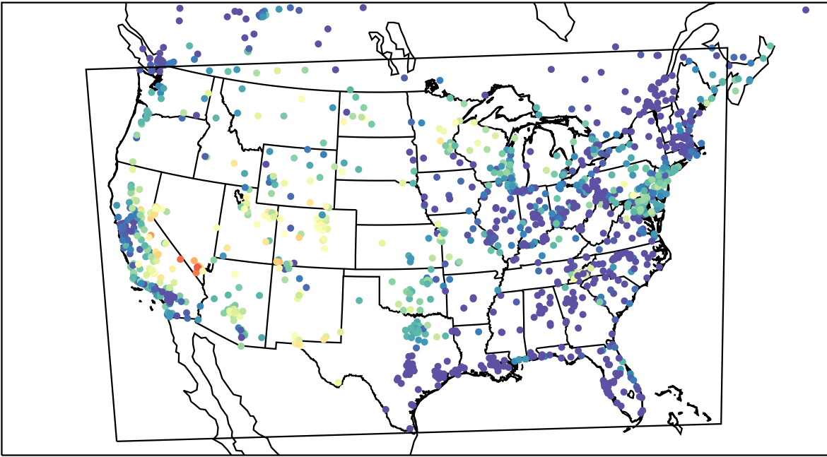
AirNOW (2023-08-09_05:00:00)
