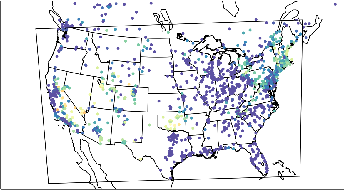
AirNOW (2023-08-08_11:00:00)
