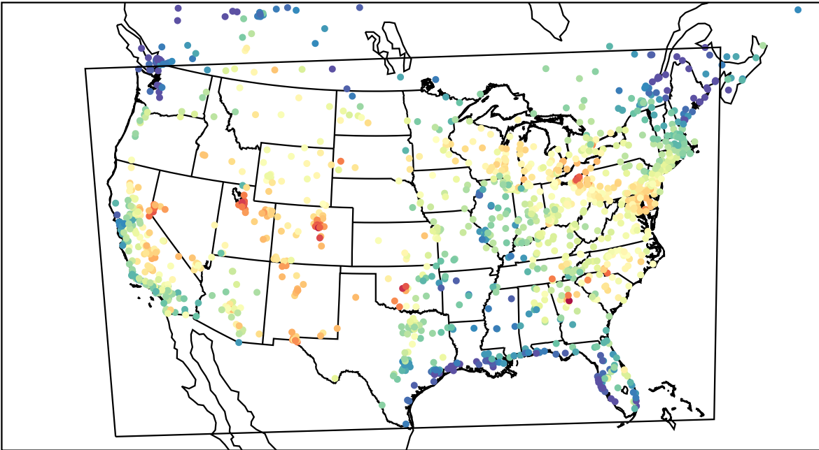
AirNOW (2023-08-09_19:00:00)
