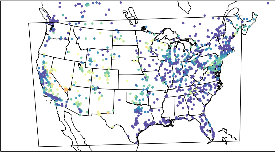
AirNOW (2023-08-09_07:00:00)
