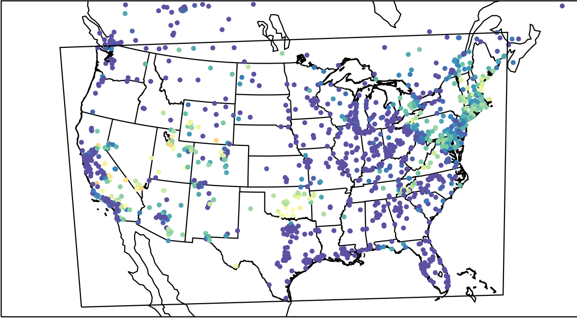
AirNOW (2023-08-08_12:00:00)
