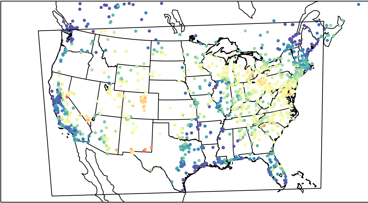
AirNOW (2023-08-09_16:00:00)
