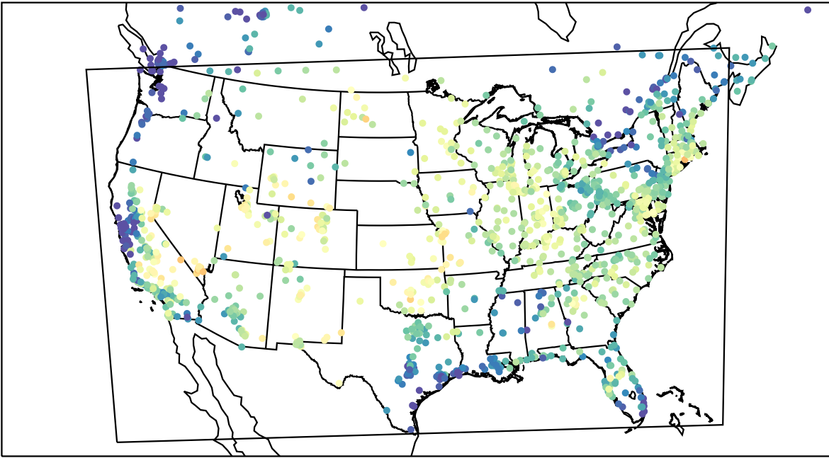
AirNOW (2023-08-08_16:00:00)
