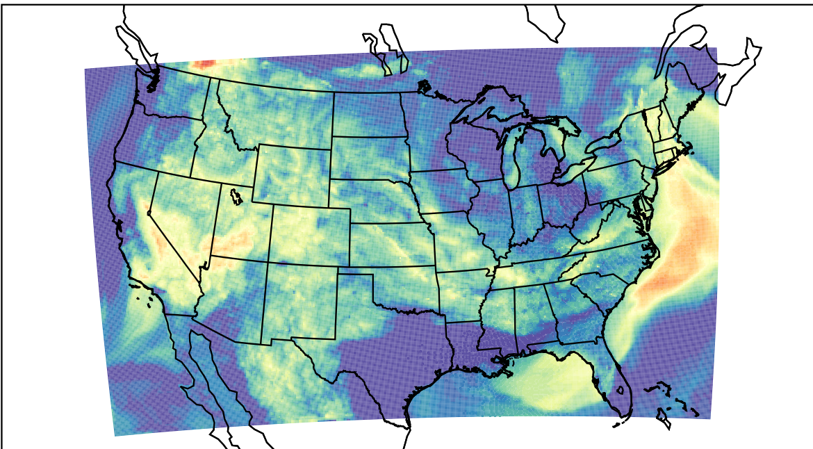
WRF (2023-08-08_12:00:00)
