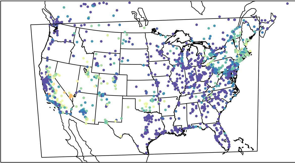
AirNOW (2023-08-08_09:00:00)
