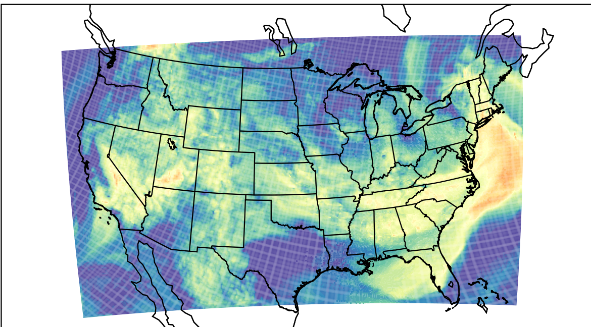
WRF (2023-08-08_14:00:00)
