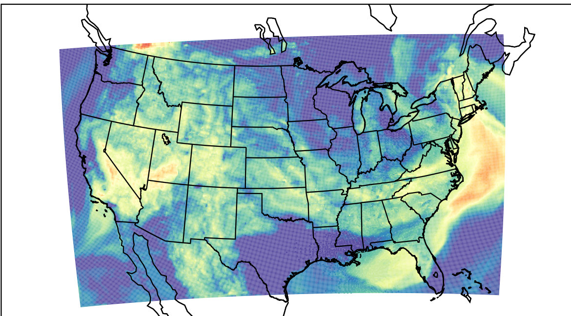
WRF (2023-08-08_13:00:00)
