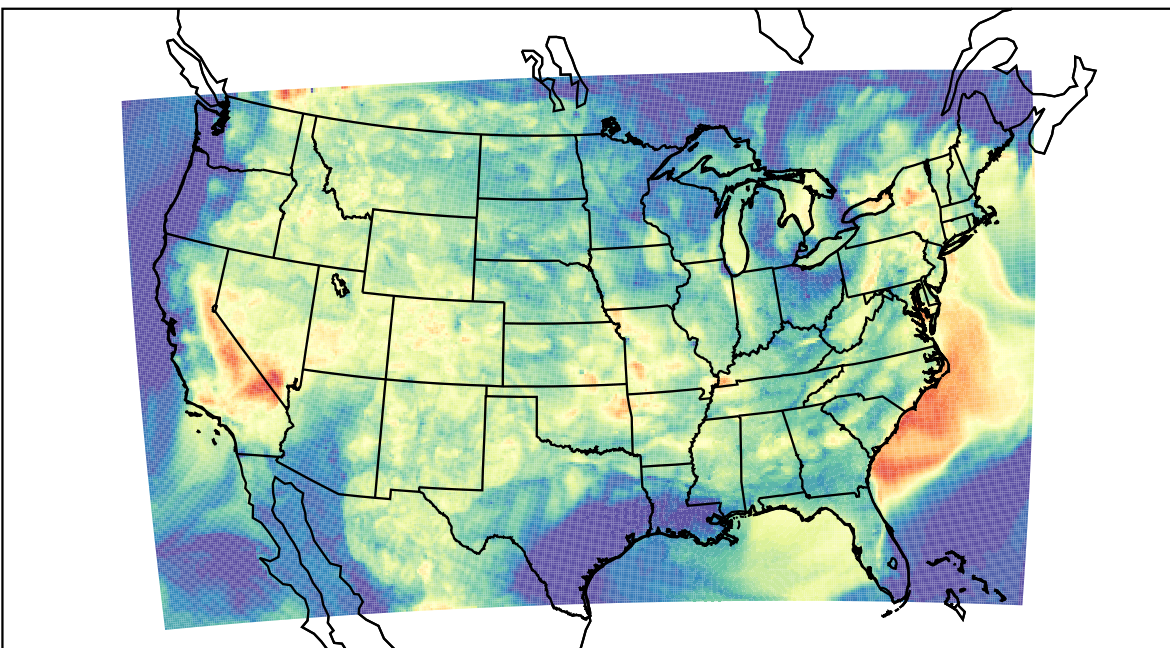
WRF (2023-08-08_04:00:00)
