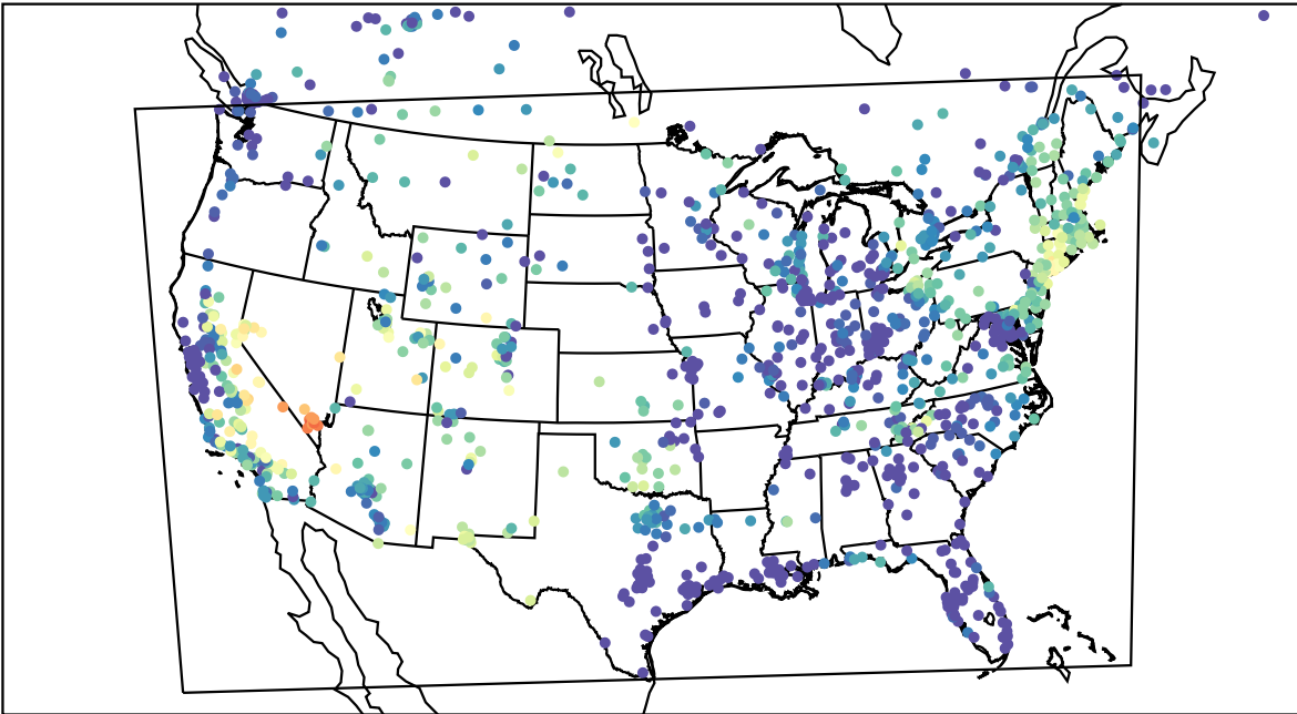
AirNOW (2023-08-08_06:00:00)
