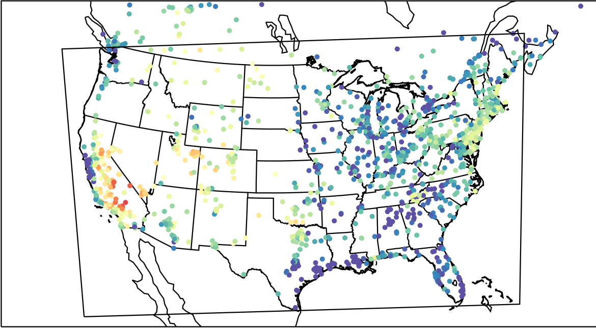
AirNOW (2023-08-08_02:00:00)
