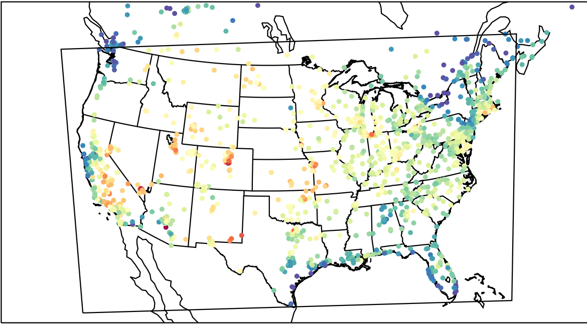
AirNOW (2023-08-08_19:00:00)
