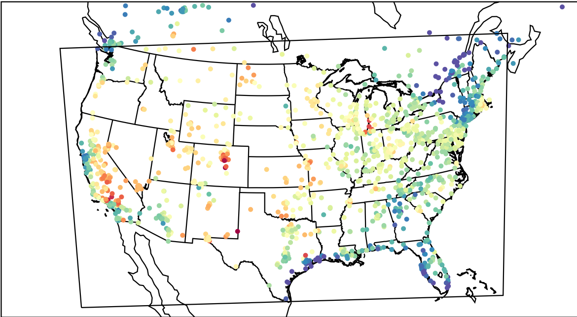
AirNOW (2023-08-08_22:00:00)
