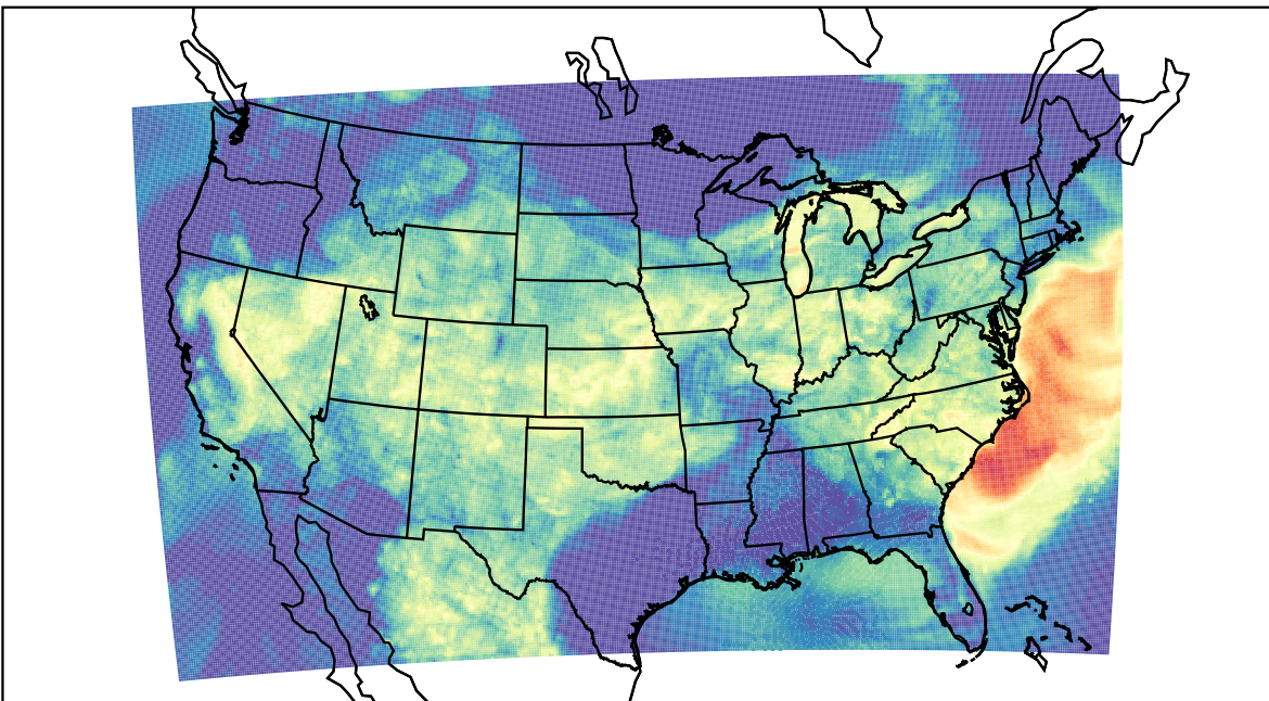
WRF (2023-08-10_08:00:00)
