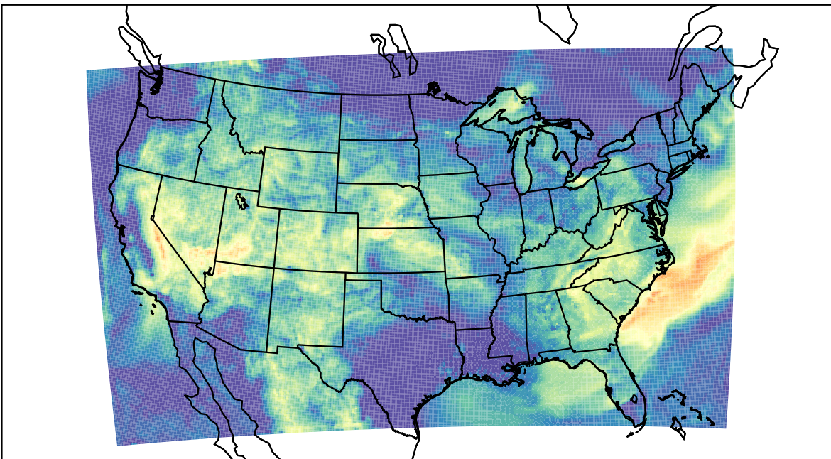
WRF (2023-08-09_13:00:00)
