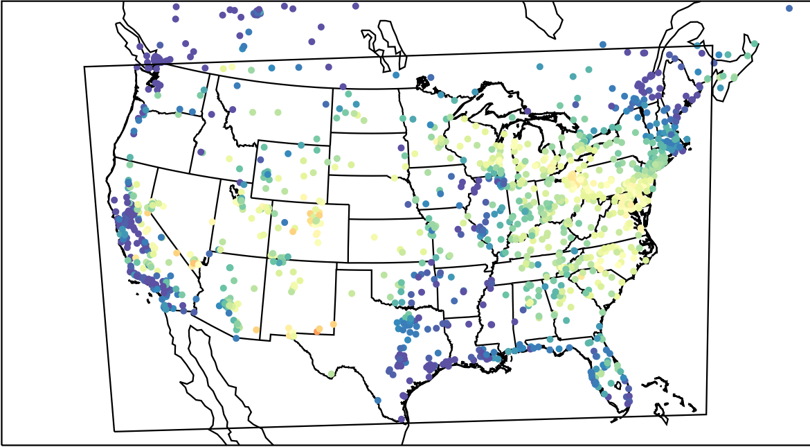
AirNOW (2023-08-09_15:00:00)
