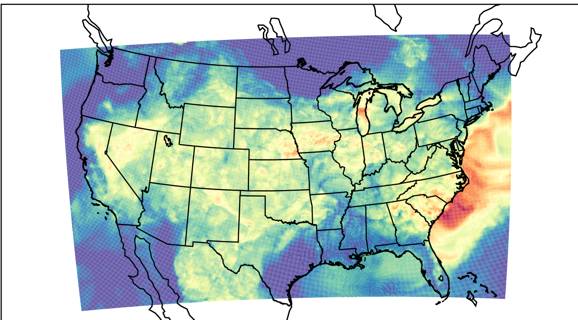
WRF (2023-08-10_04:00:00)
