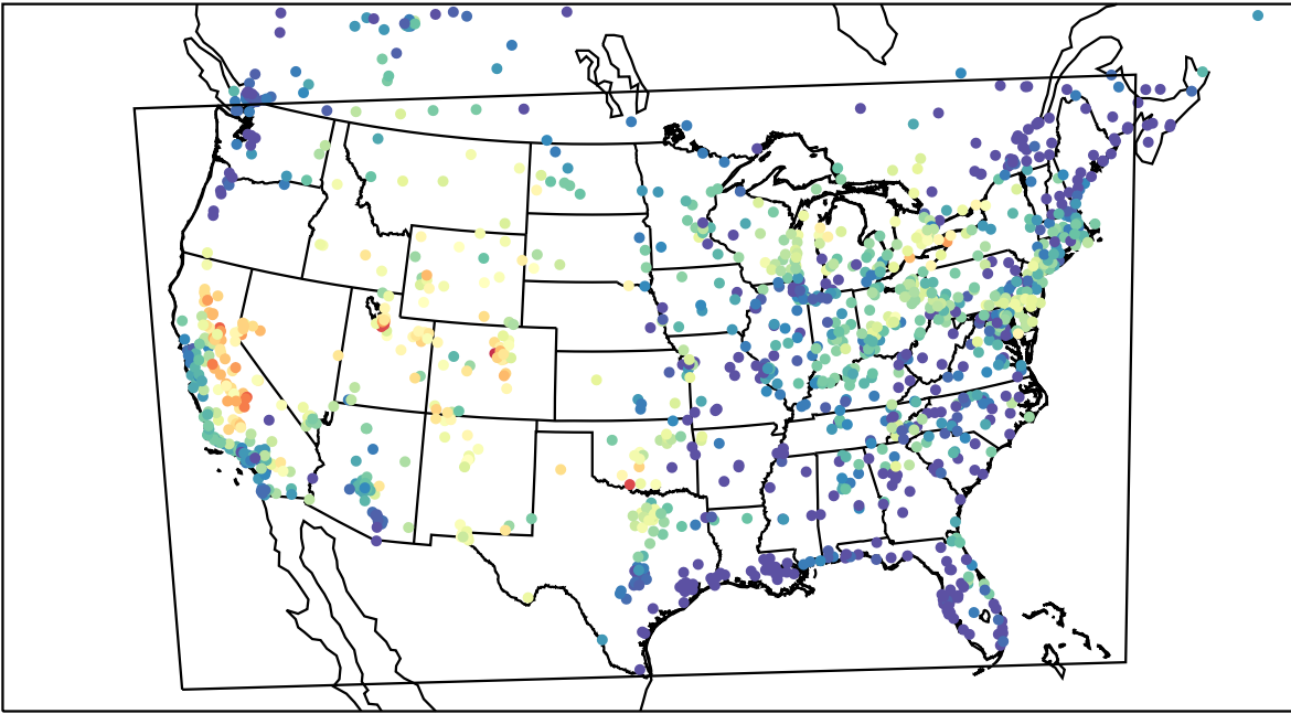
AirNOW (2023-08-10_02:00:00)
