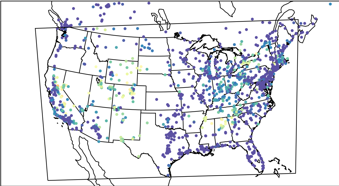
AirNOW (2023-08-10_11:00:00)
