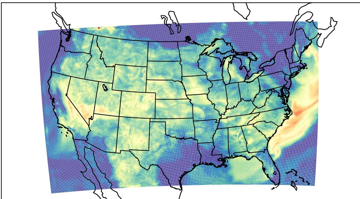
WRF (2023-08-09_07:00:00)
