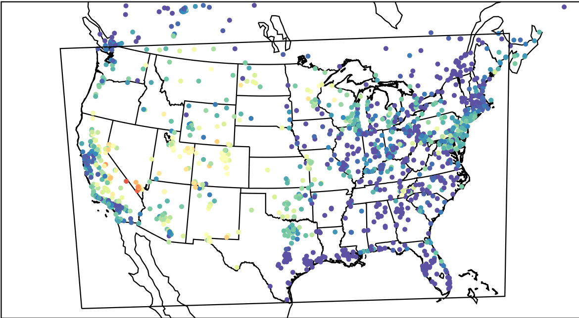
AirNOW (2023-08-09_04:00:00)
