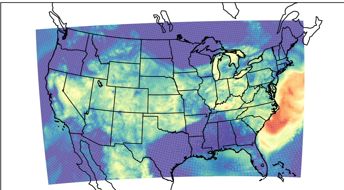
WRF (2023-08-10_11:00:00)
