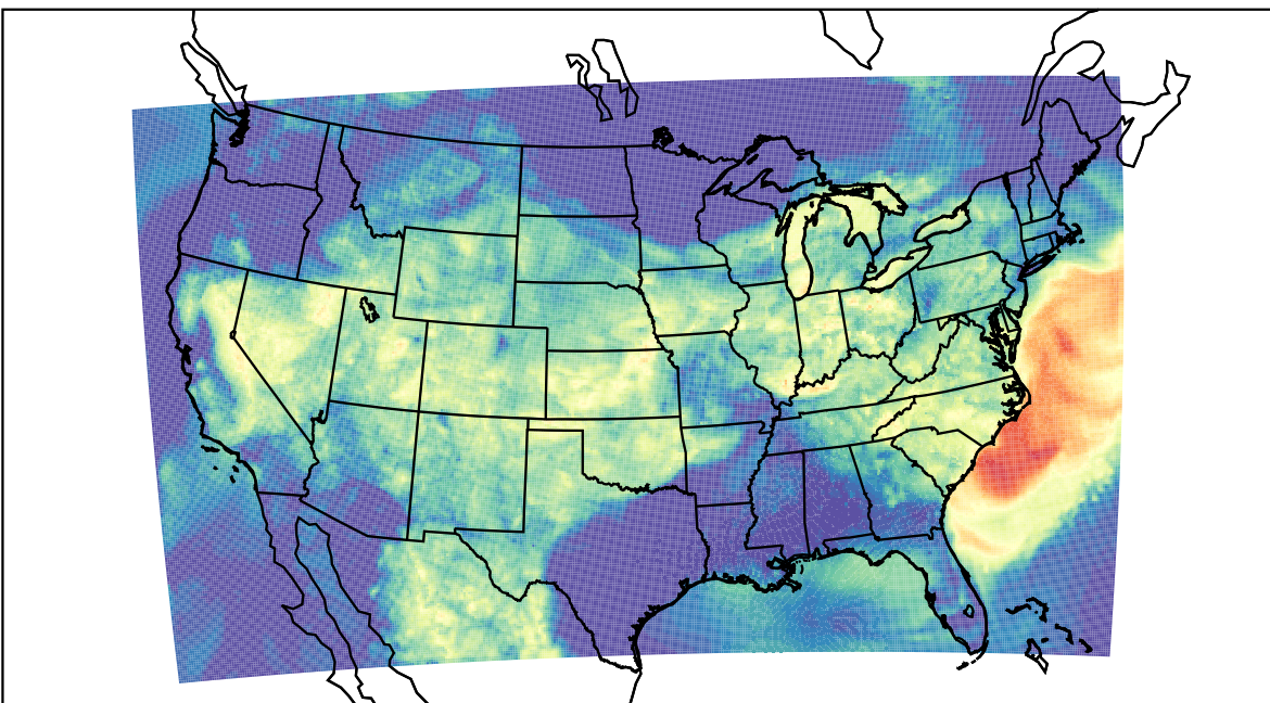
WRF (2023-08-10_09:00:00)
