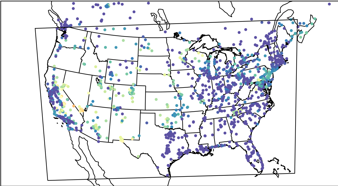
AirNOW (2023-08-09_09:00:00)
