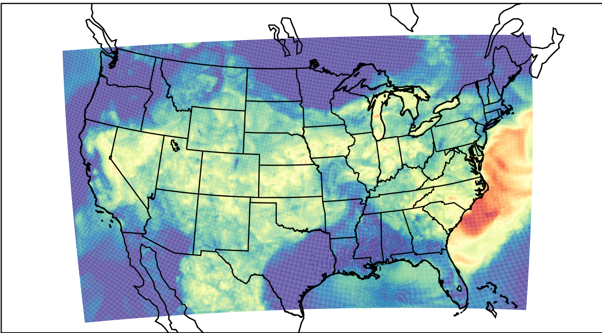
WRF (2023-08-10_07:00:00)
