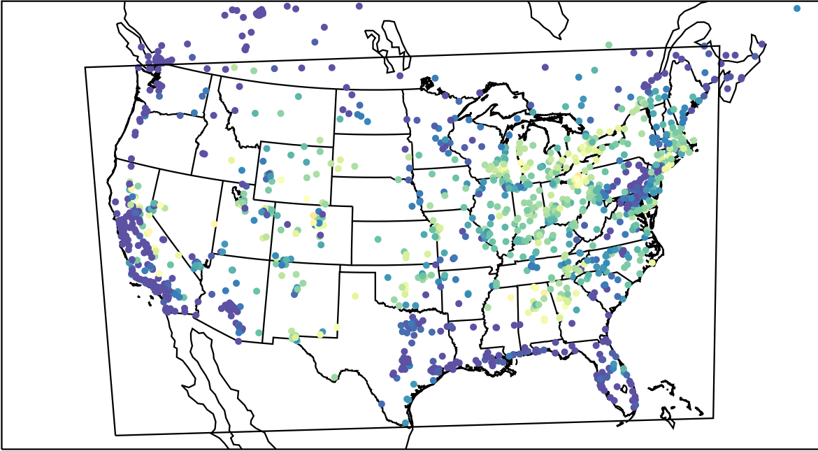
AirNOW (2023-08-10_14:00:00)
