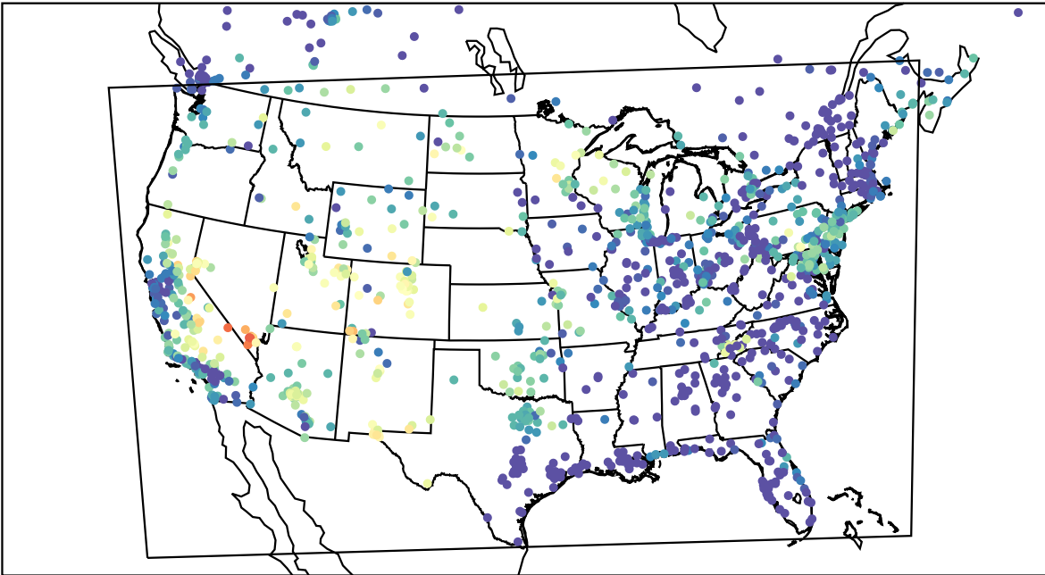
AirNOW (2023-08-09_05:00:00)
