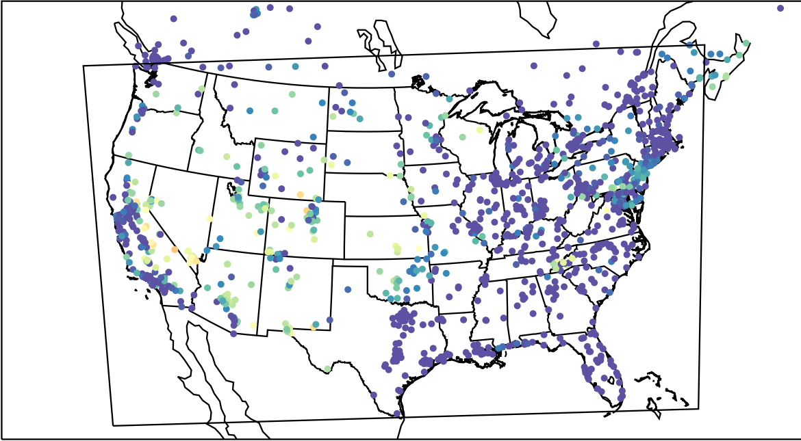
AirNOW (2023-08-09_10:00:00)
