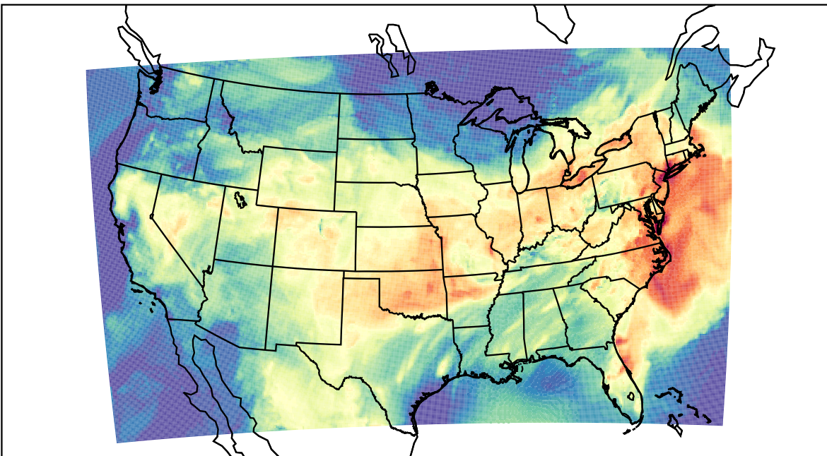
WRF (2023-08-10_17:00:00)
