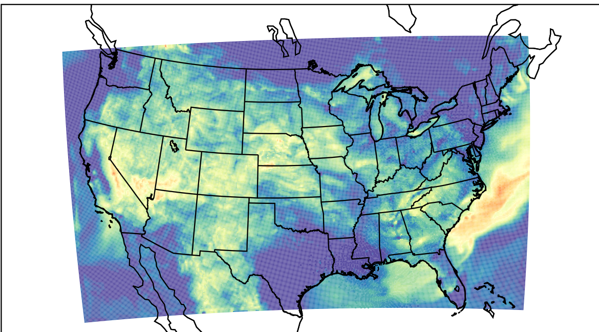
WRF (2023-08-09_11:00:00)
