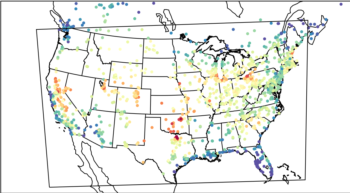
AirNOW (2023-08-10_21:00:00)
