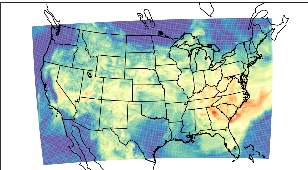
WRF (2023-08-09_15:00:00)
