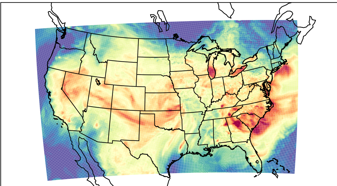
WRF (2023-08-09_22:00:00)
