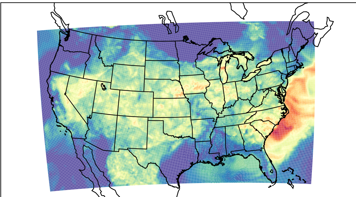
WRF (2023-08-10_05:00:00)
