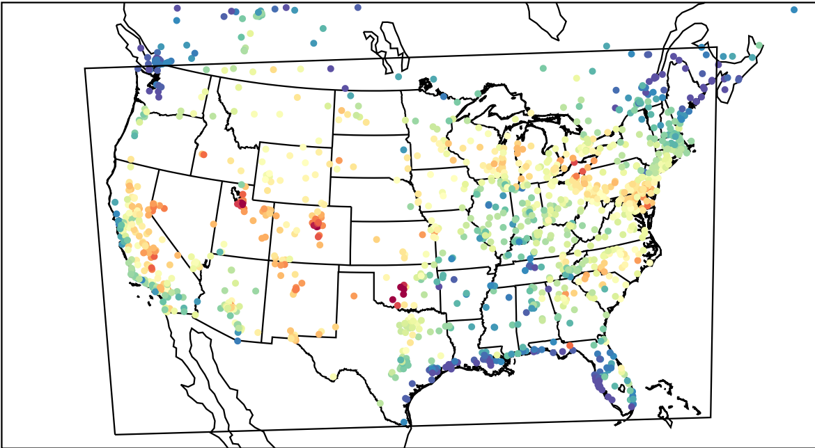
AirNOW (2023-08-09_21:00:00)
