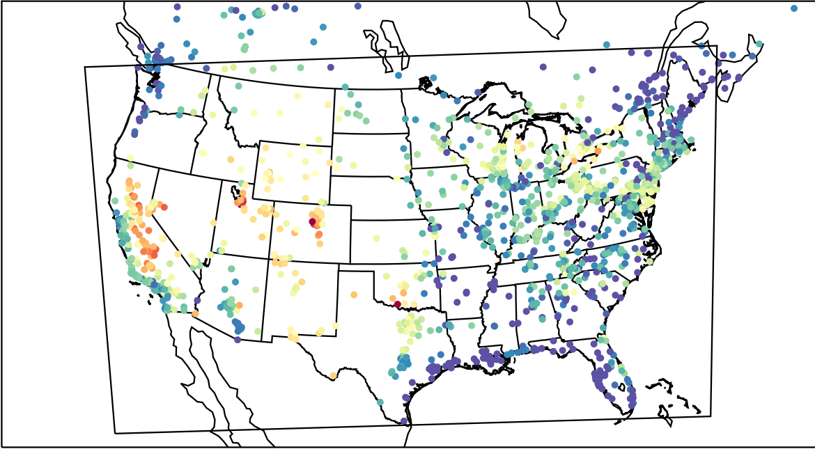
AirNOW (2023-08-10_01:00:00)
