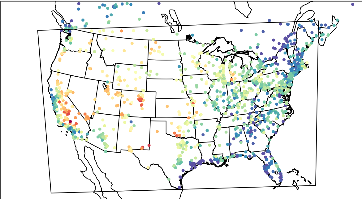
AirNOW (2023-08-09_00:00:00)
