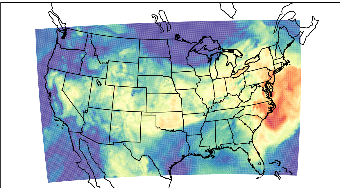
WRF (2023-08-10_15:00:00)
