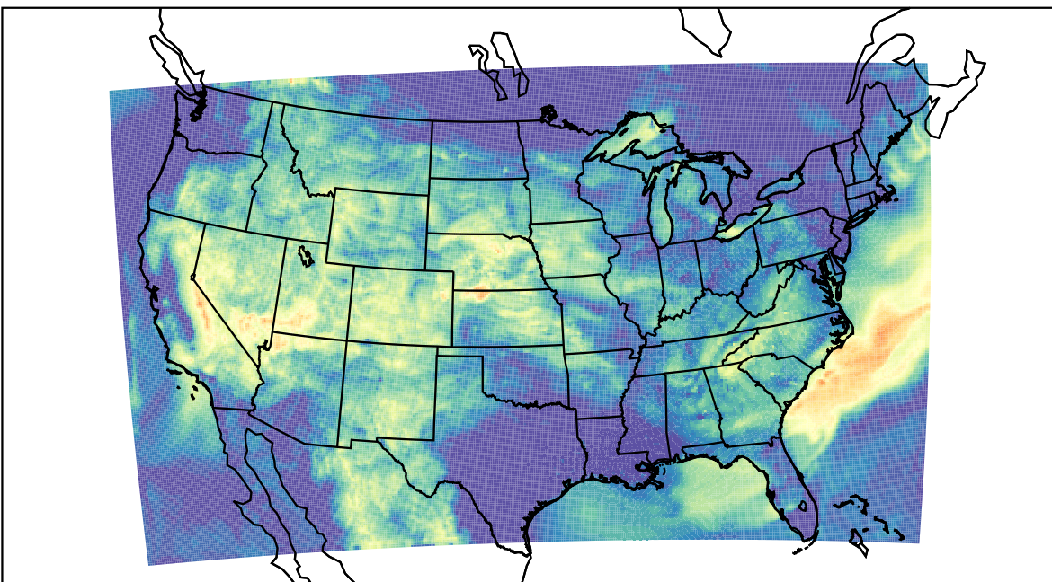
WRF (2023-08-09_12:00:00)
