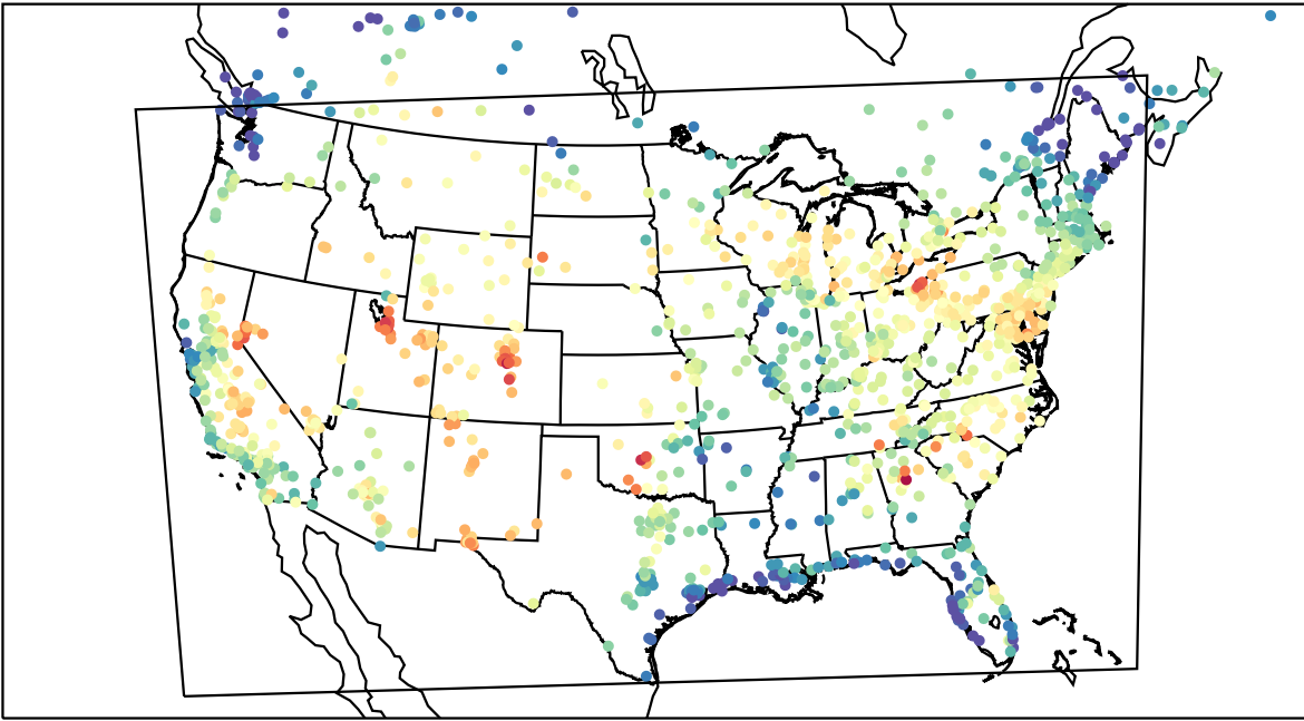
AirNOW (2023-08-09_19:00:00)
