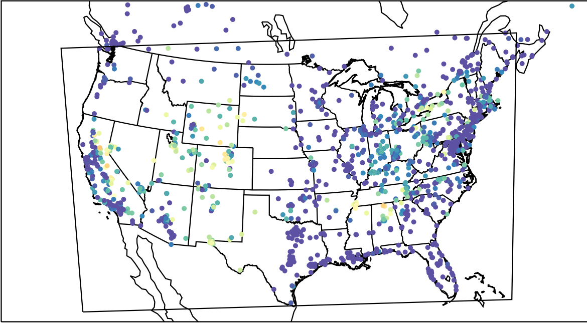
AirNOW (2023-08-10_10:00:00)
