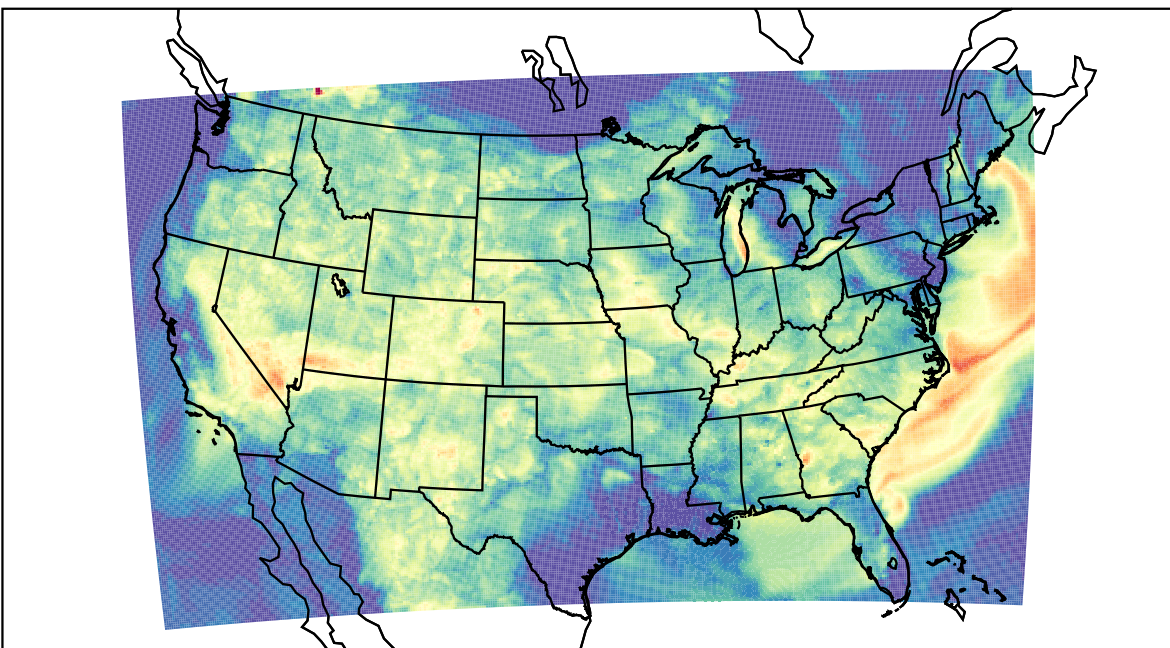
WRF (2023-08-09_05:00:00)
