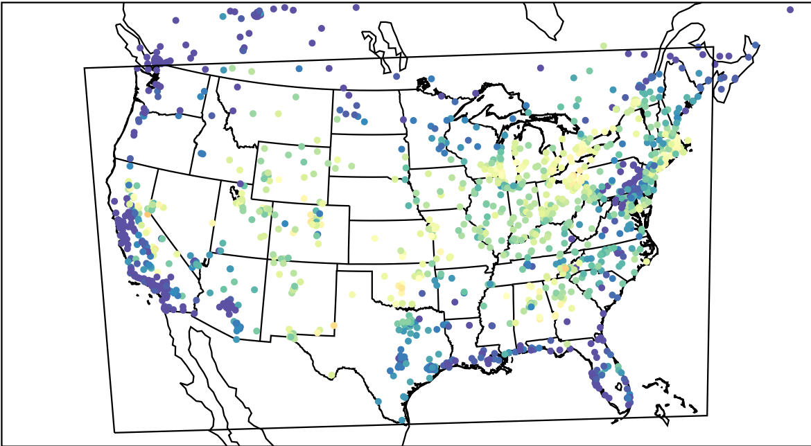
AirNOW (2023-08-10_15:00:00)
