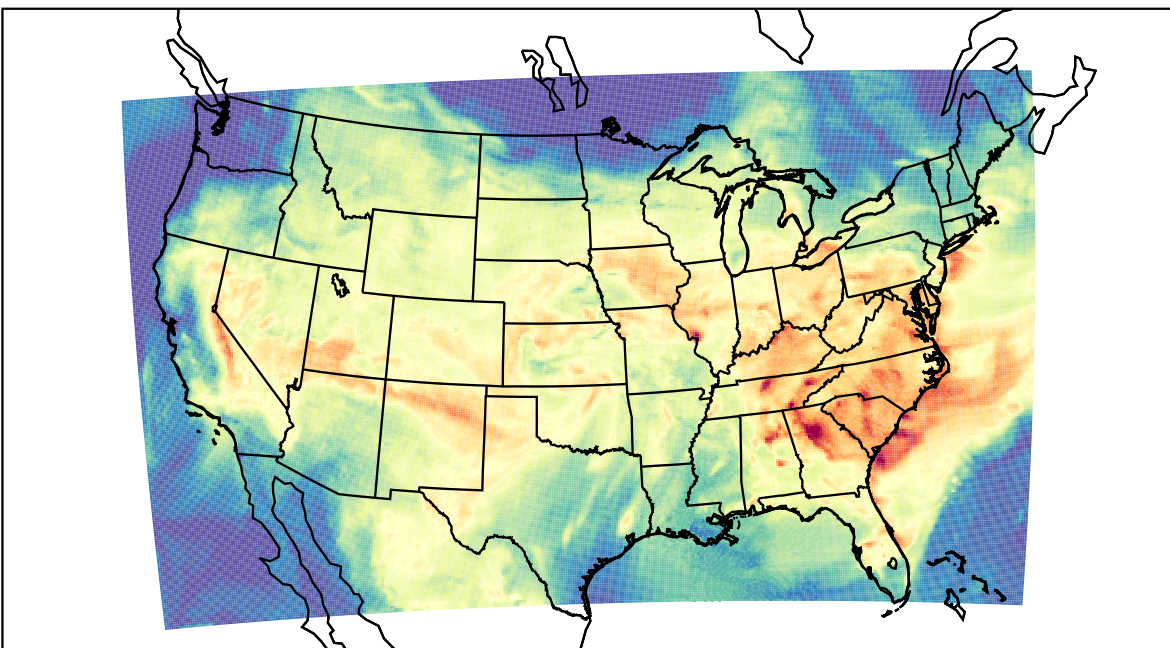
WRF (2023-08-09_17:00:00)
