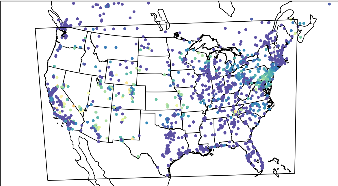
AirNOW (2023-08-09_12:00:00)
