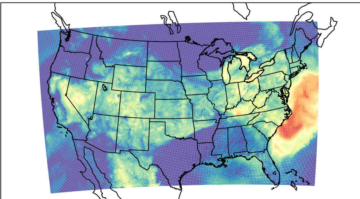
WRF (2023-08-10_13:00:00)
