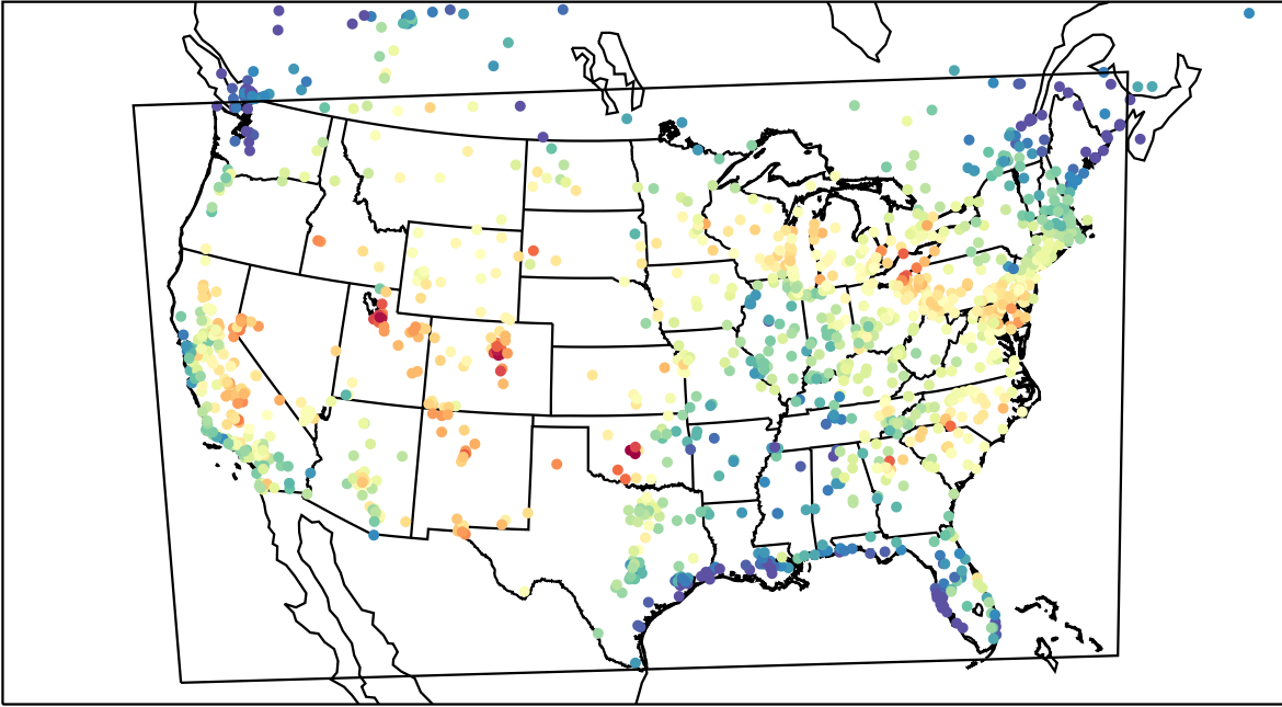
AirNOW (2023-08-09_20:00:00)
