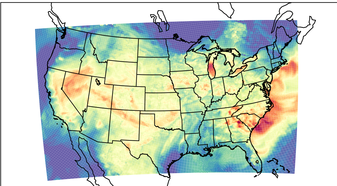
WRF (2023-08-10_01:00:00)
