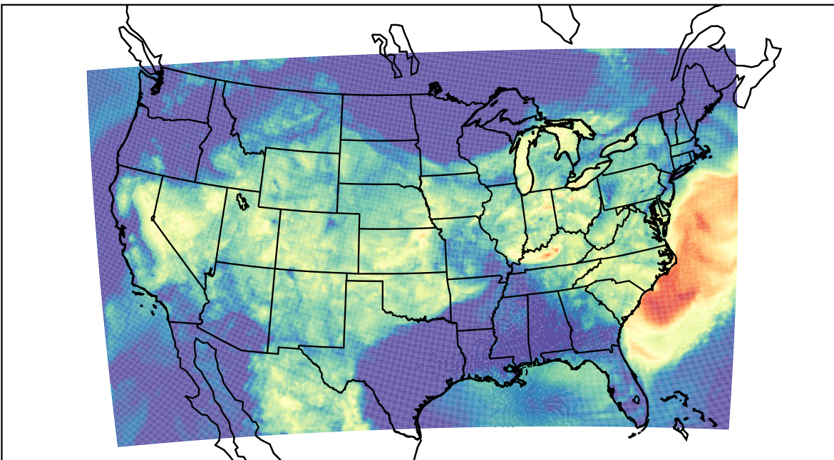
WRF (2023-08-10_10:00:00)
