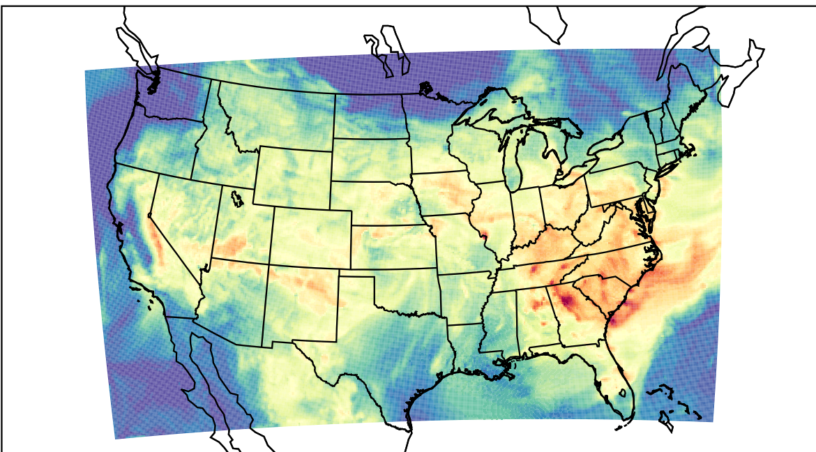
WRF (2023-08-09_16:00:00)
