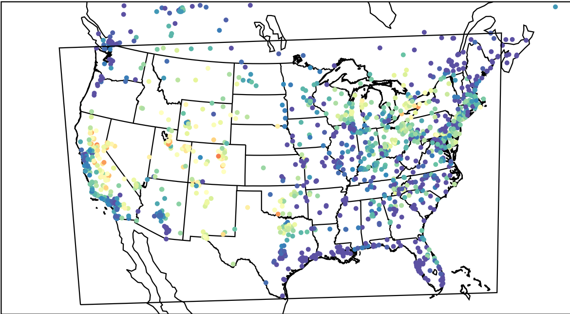
AirNOW (2023-08-10_03:00:00)
