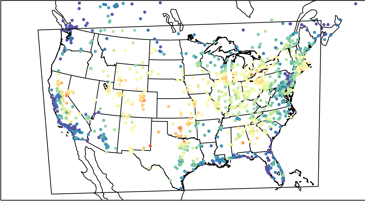
AirNOW (2023-08-10_17:00:00)
