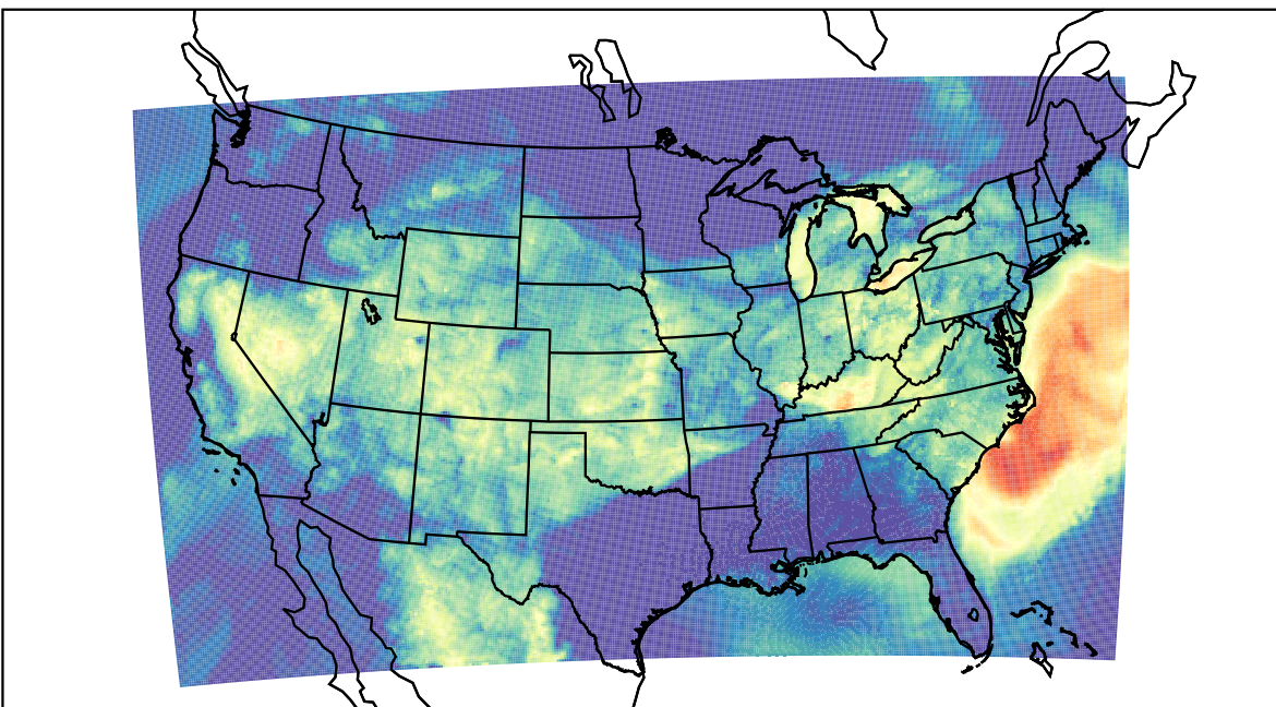
WRF (2023-08-10_12:00:00)
