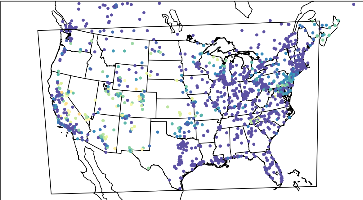
AirNOW (2023-08-09_11:00:00)
