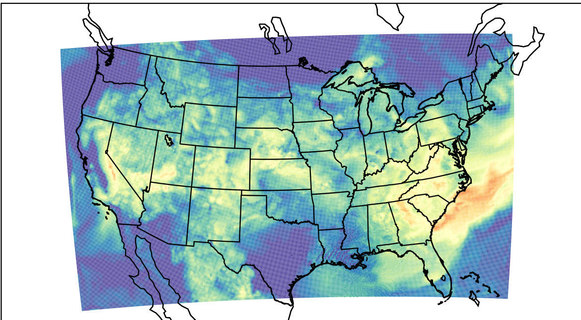
WRF (2023-08-09_14:00:00)
