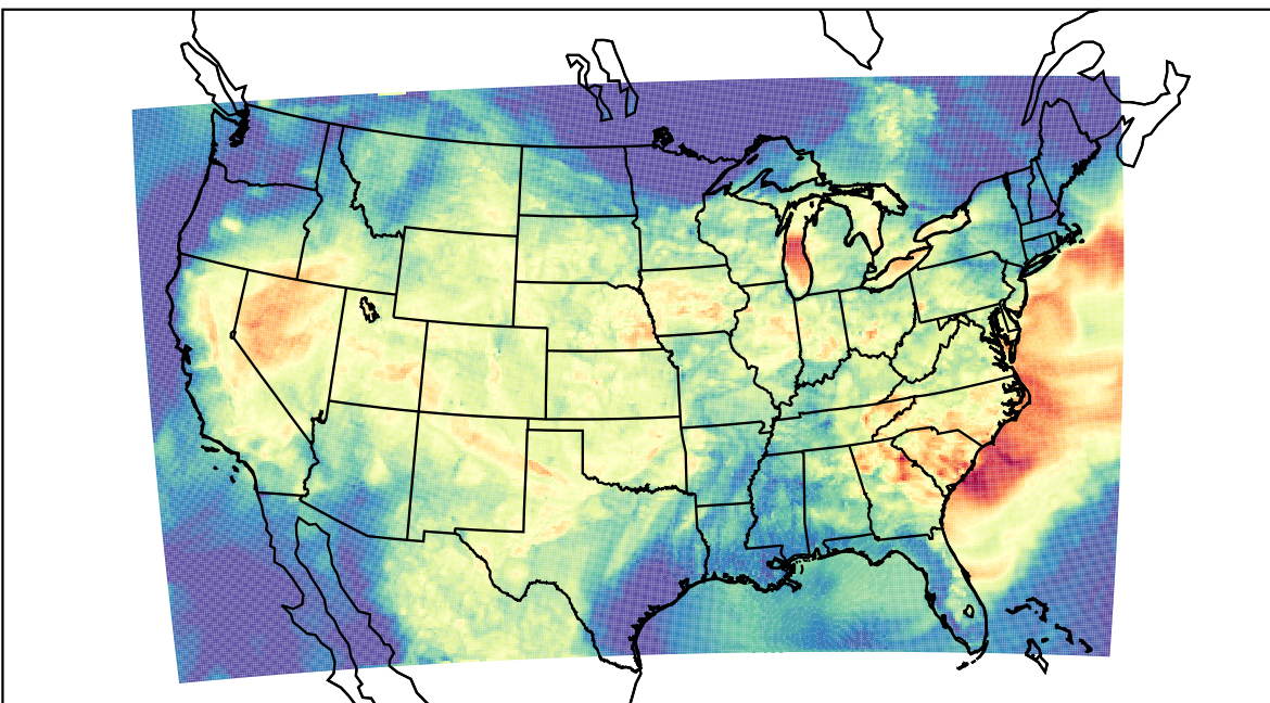
WRF (2023-08-10_02:00:00)
