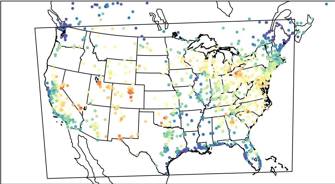
AirNOW (2023-08-09_18:00:00)
