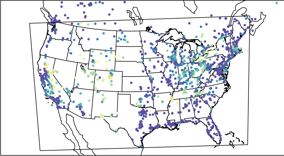
AirNOW (2023-08-10_08:00:00)
