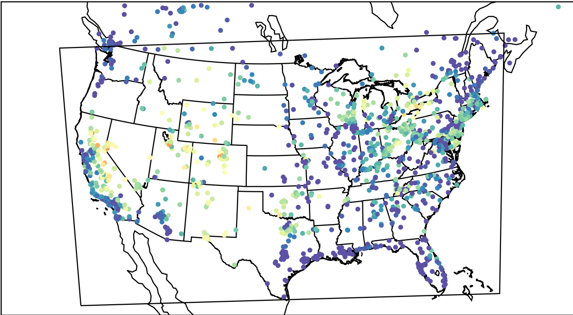
AirNOW (2023-08-10_04:00:00)
