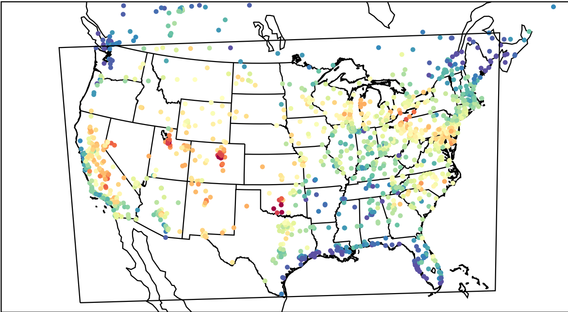
AirNOW (2023-08-09_22:00:00)
