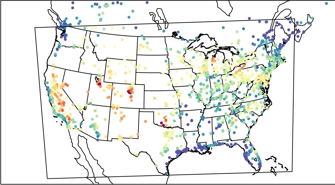
AirNOW (2023-08-09_23:00:00)
