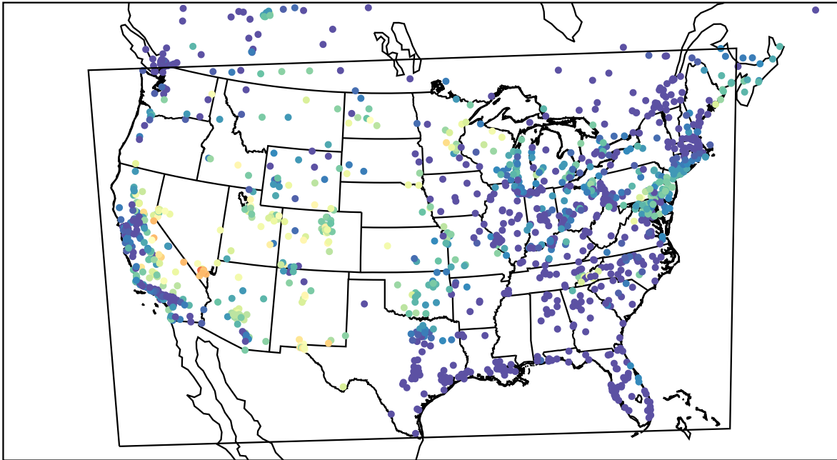
AirNOW (2023-08-09_07:00:00)
