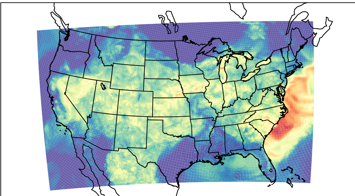
WRF (2023-08-10_06:00:00)
