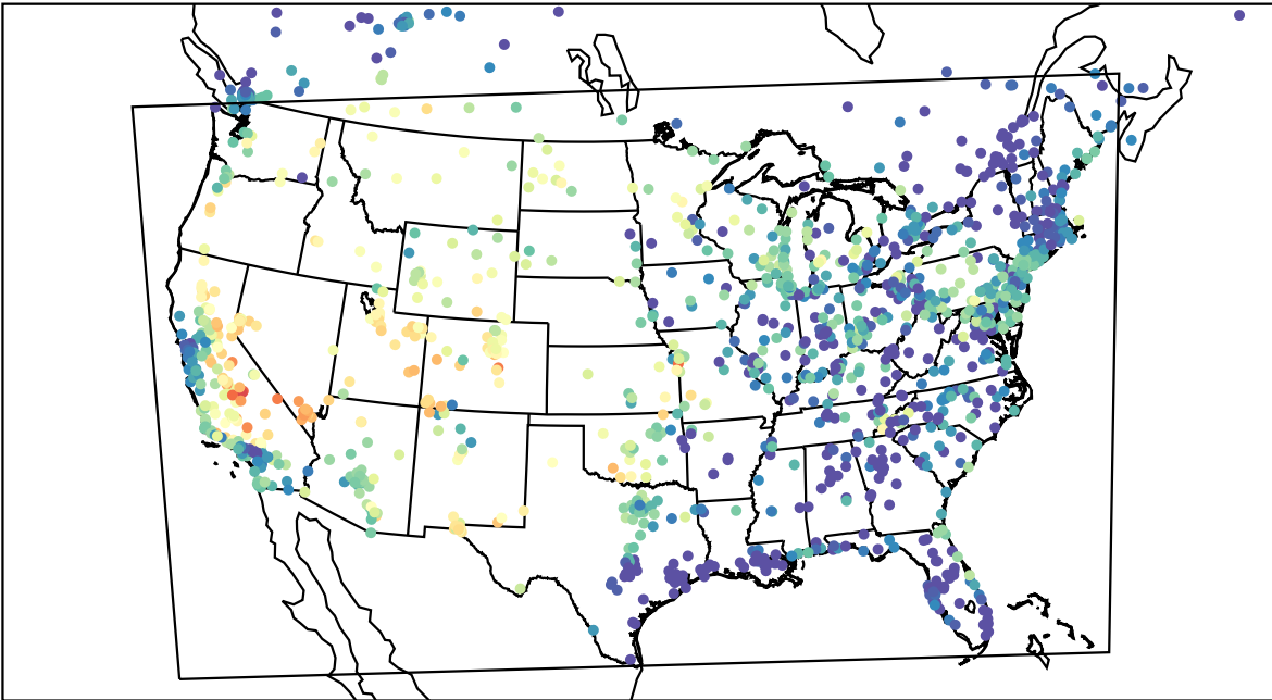
AirNOW (2023-08-09_02:00:00)
