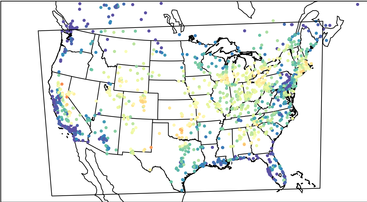
AirNOW (2023-08-10_16:00:00)
