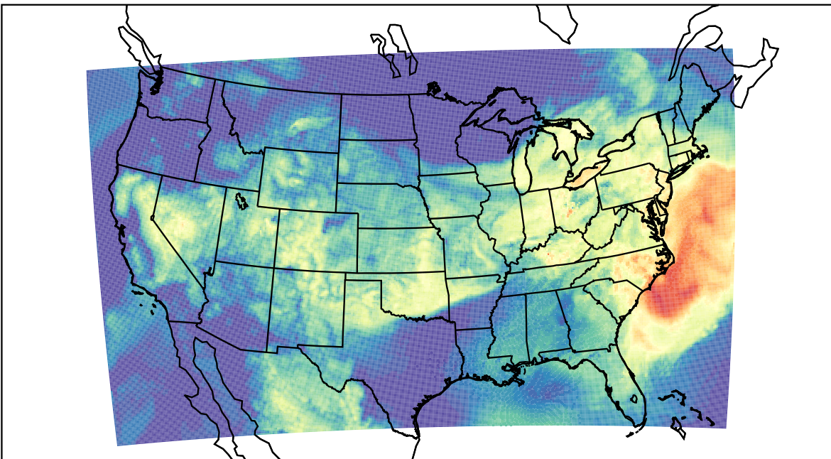
WRF (2023-08-10_14:00:00)
