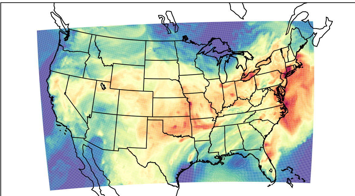
WRF (2023-08-10_19:00:00)
