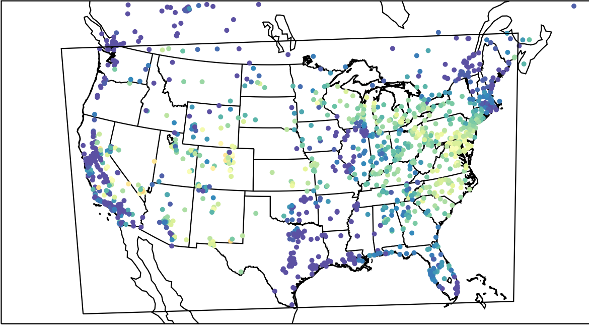
AirNOW (2023-08-09_14:00:00)
