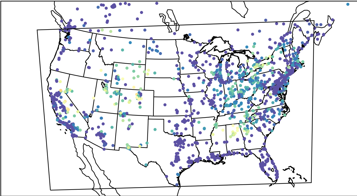
AirNOW (2023-08-10_12:00:00)
