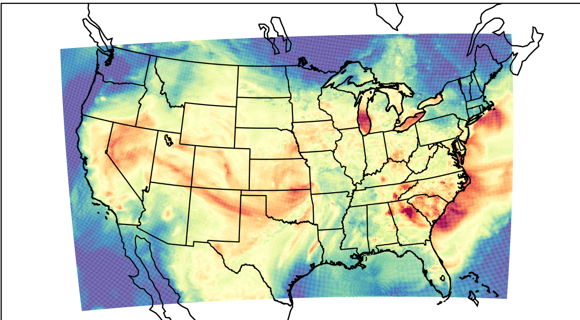
WRF (2023-08-09_23:00:00)
