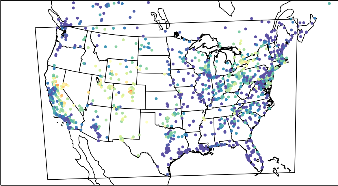
AirNOW (2023-08-10_05:00:00)
