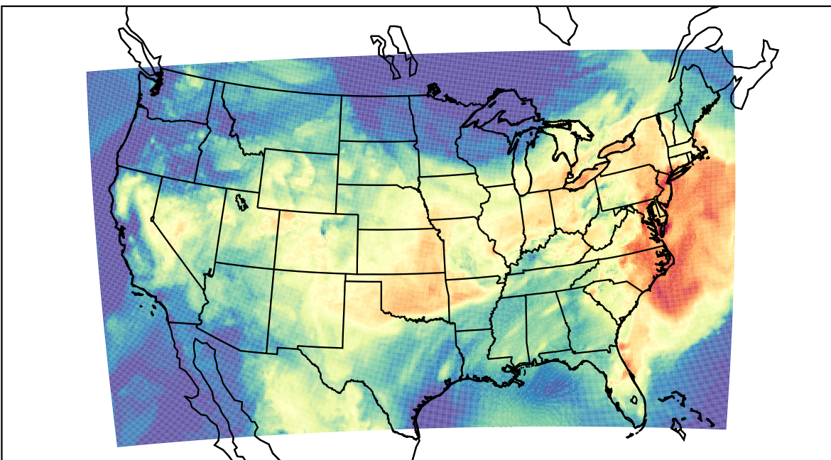
WRF (2023-08-10_16:00:00)
