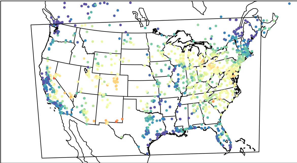
AirNOW (2023-08-09_16:00:00)
