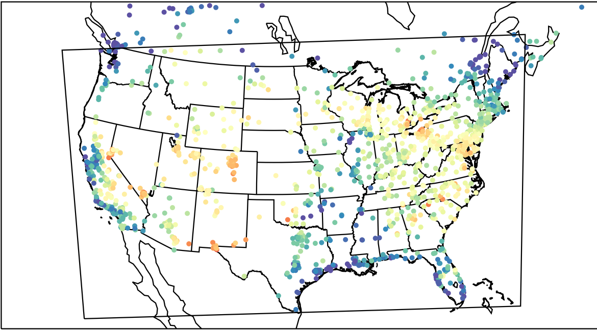
AirNOW (2023-08-09_17:00:00)
