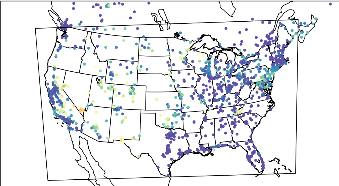
AirNOW (2023-08-09_08:00:00)
