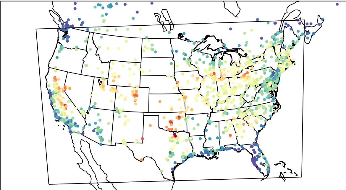
AirNOW (2023-08-10_19:00:00)
