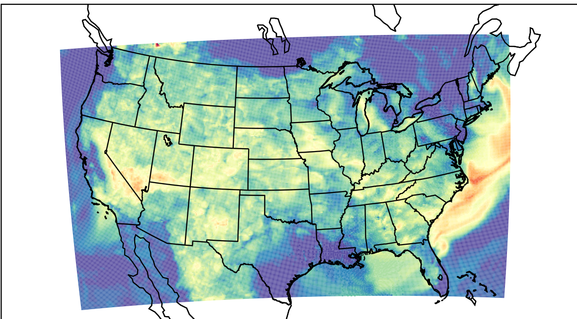
WRF (2023-08-09_06:00:00)
