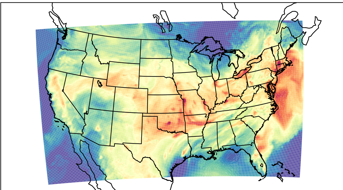
WRF (2023-08-10_21:00:00)
