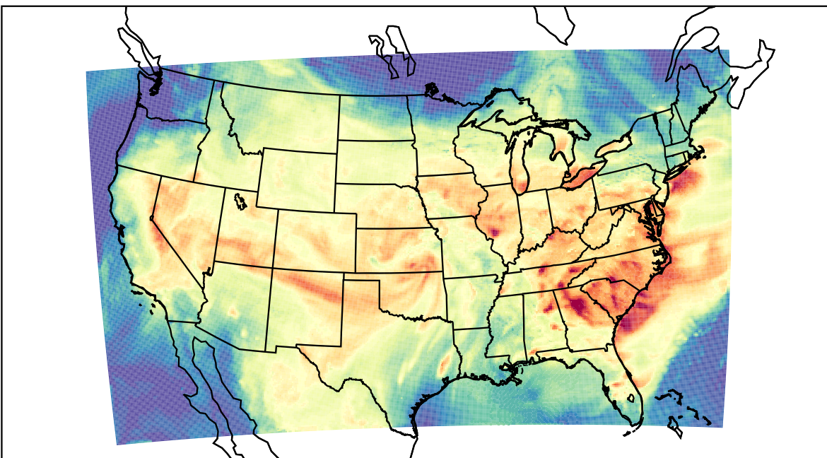
WRF (2023-08-09_19:00:00)
