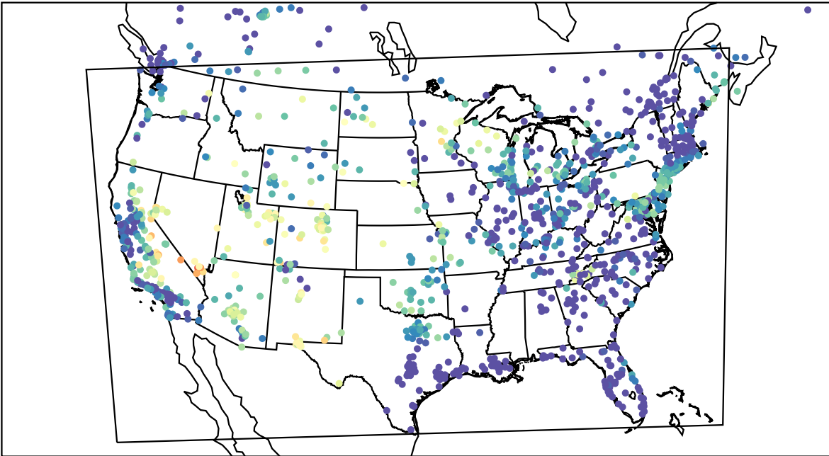
AirNOW (2023-08-09_06:00:00)
