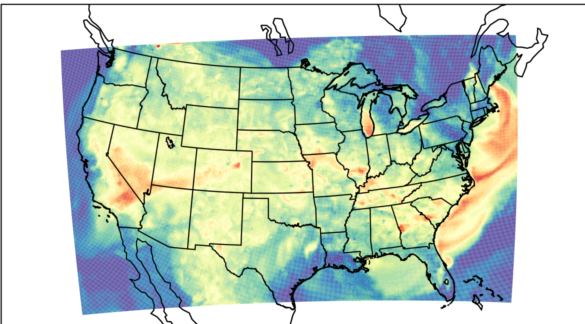
WRF (2023-08-09_02:00:00)
