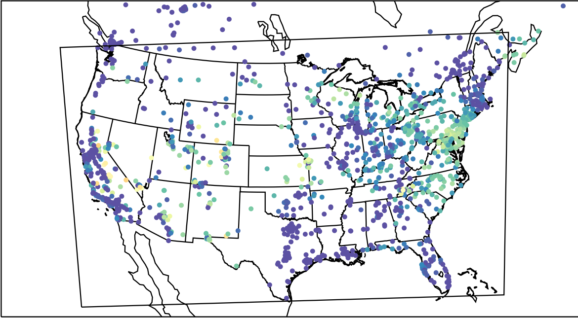
AirNOW (2023-08-09_13:00:00)
