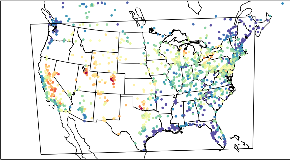
AirNOW (2023-08-10_00:00:00)
