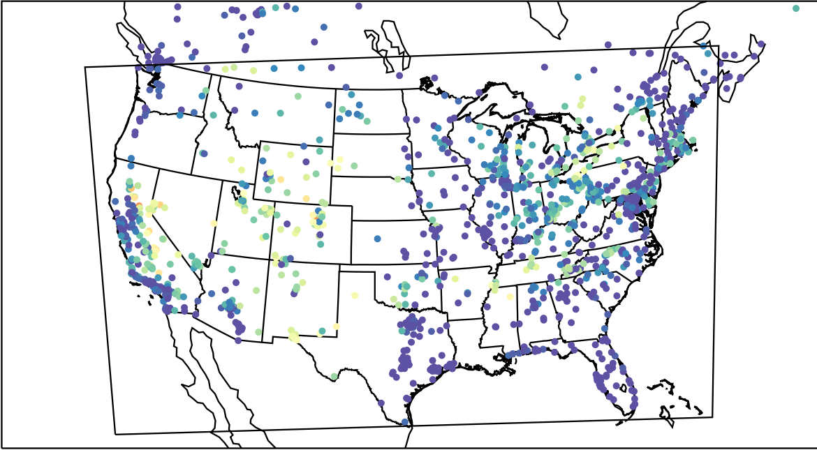
AirNOW (2023-08-10_07:00:00)
