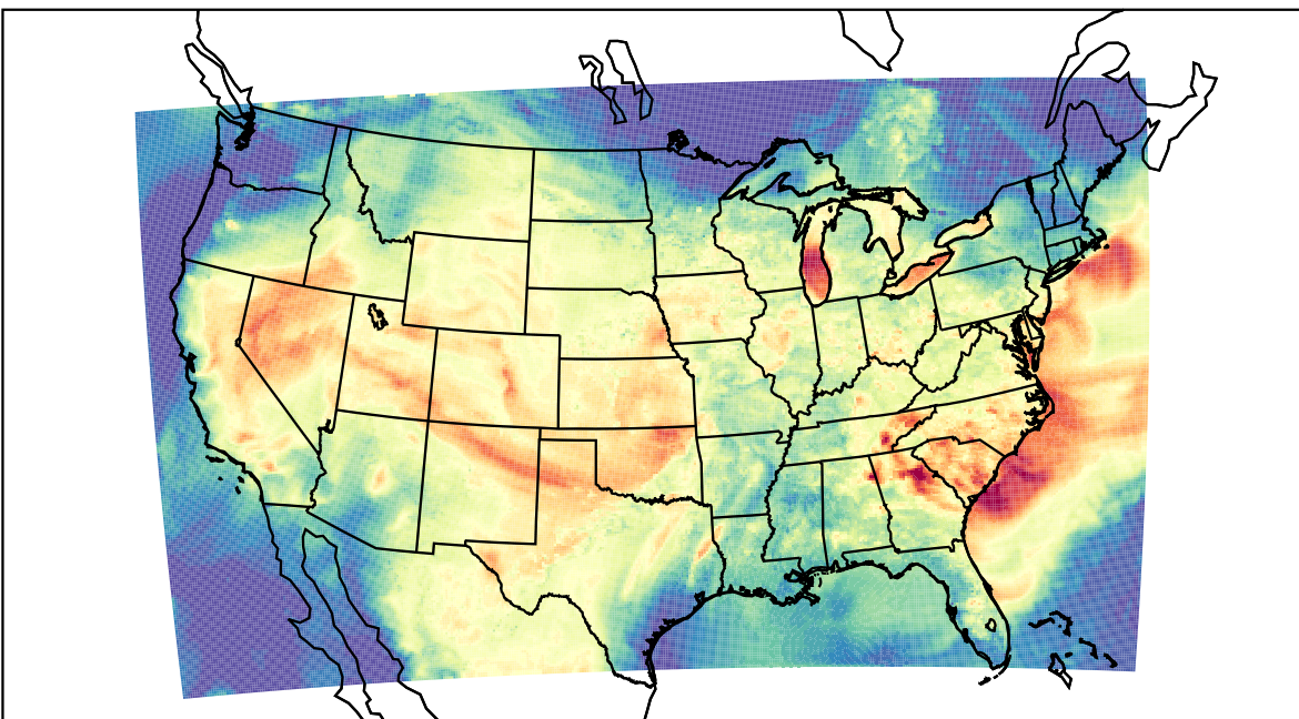
WRF (2023-08-10_00:00:00)
