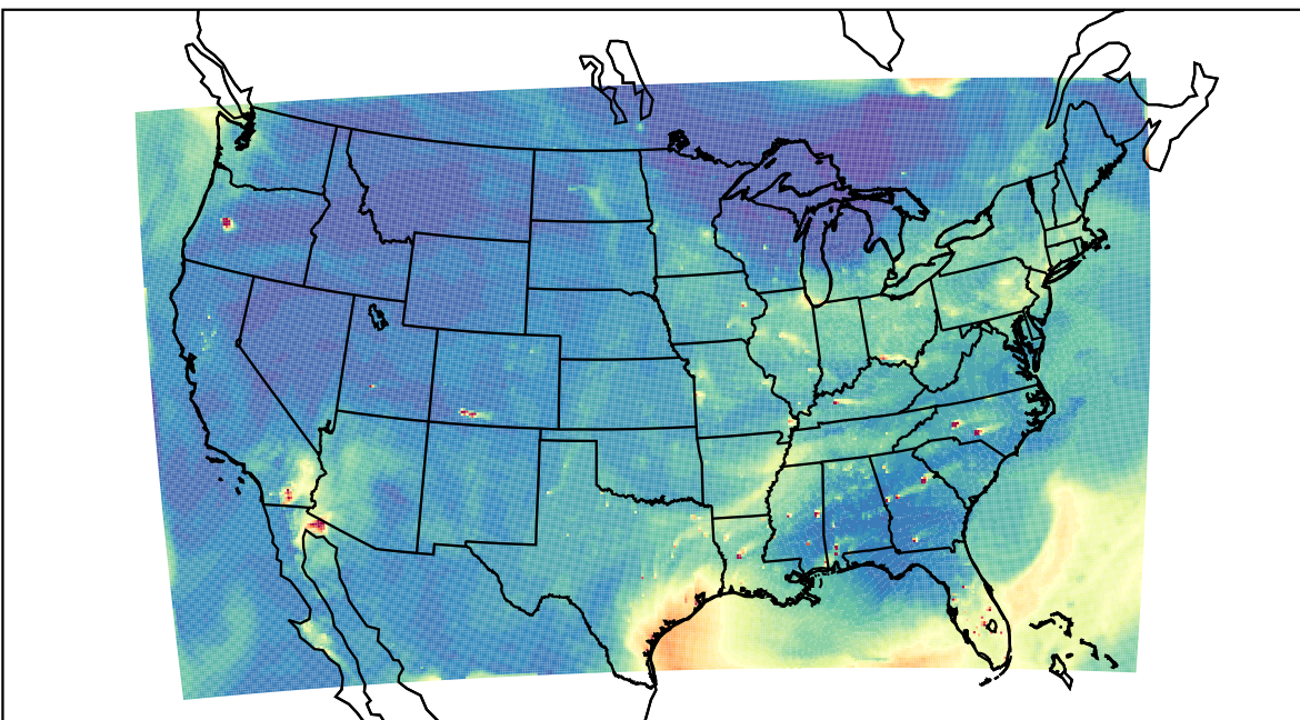
WRF 2023-08-11_00:00:00
