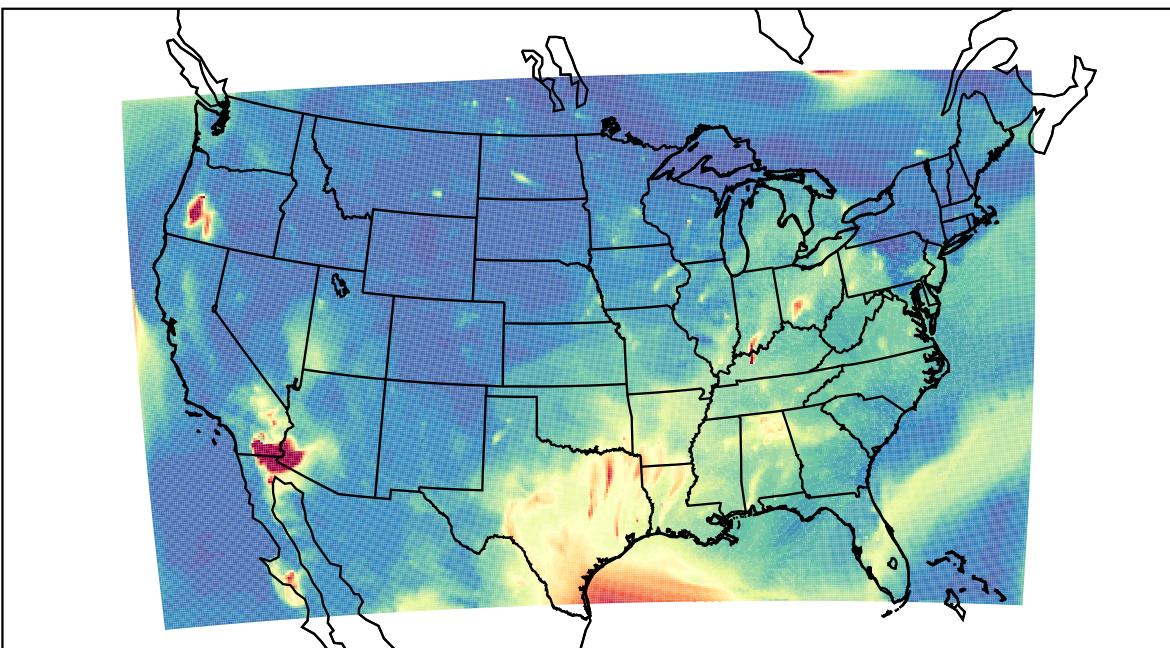
WRF 2023-08-12_07:00:00
