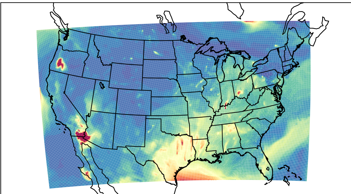
WRF 2023-08-12_06:00:00
