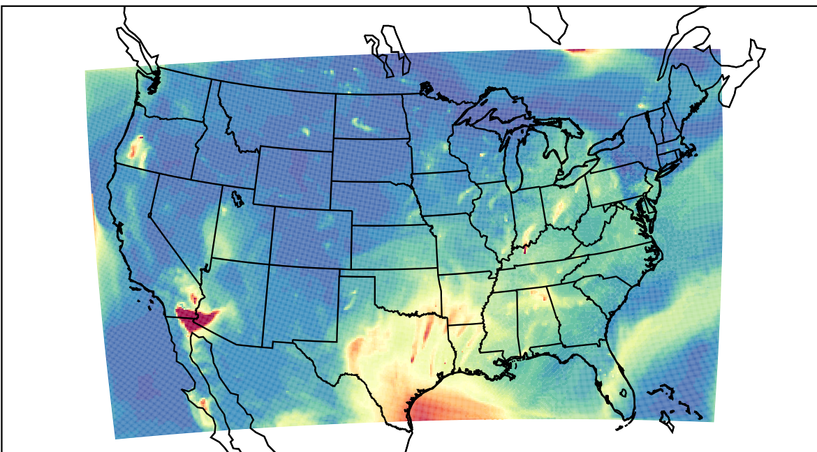
WRF 2023-08-12_09:00:00
