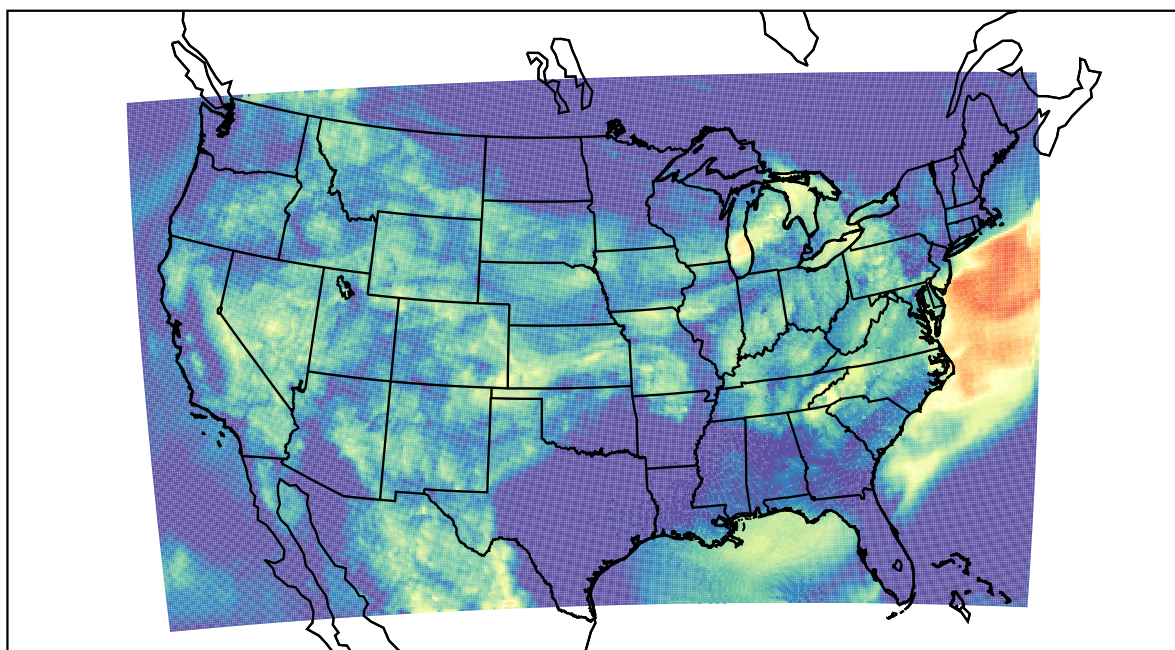
WRF (2023-08-12_12:00:00)
