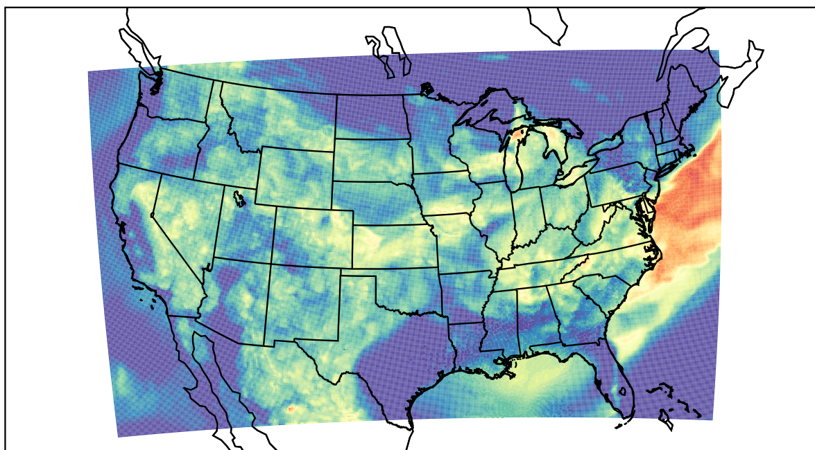
WRF (2023-08-12_07:00:00)
