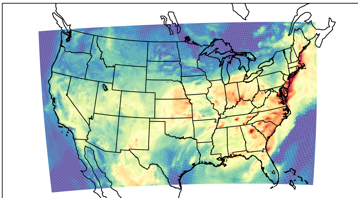
WRF (2023-08-13_17:00:00)
