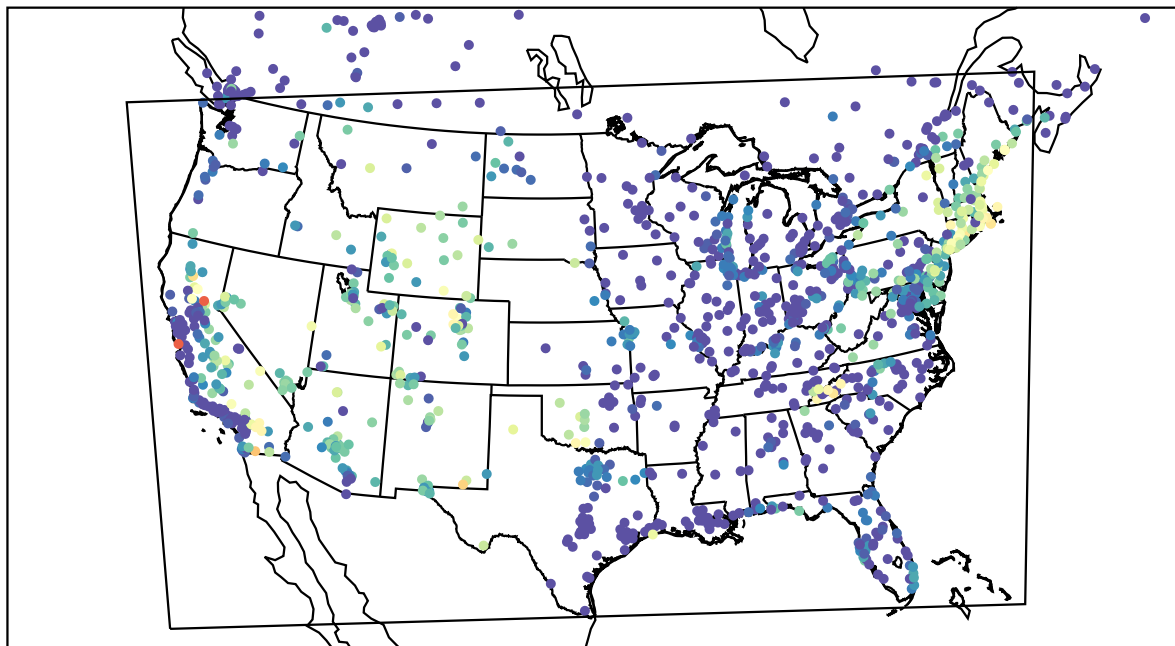
AirNOW (2023-08-13_07:00:00)
