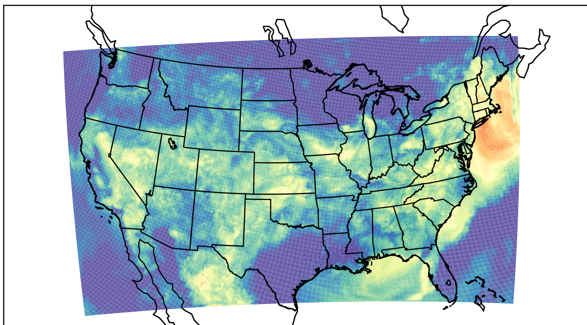
WRF (2023-08-13_07:00:00)
