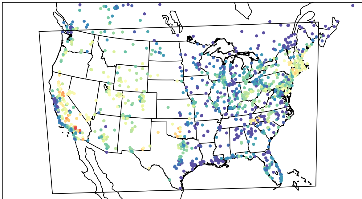
AirNOW (2023-08-13_02:00:00)
