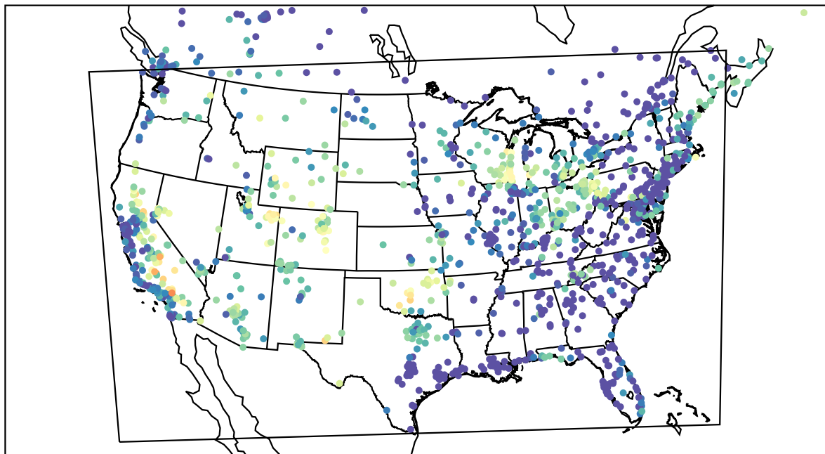
AirNOW (2023-08-12_04:00:00)
