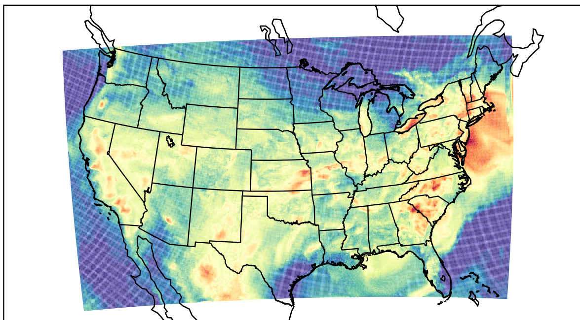
WRF (2023-08-13_01:00:00)
