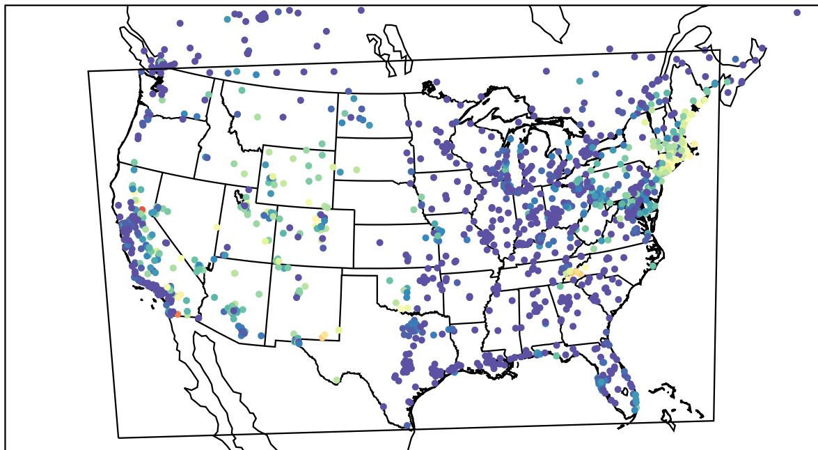
AirNOW (2023-08-13_08:00:00)
