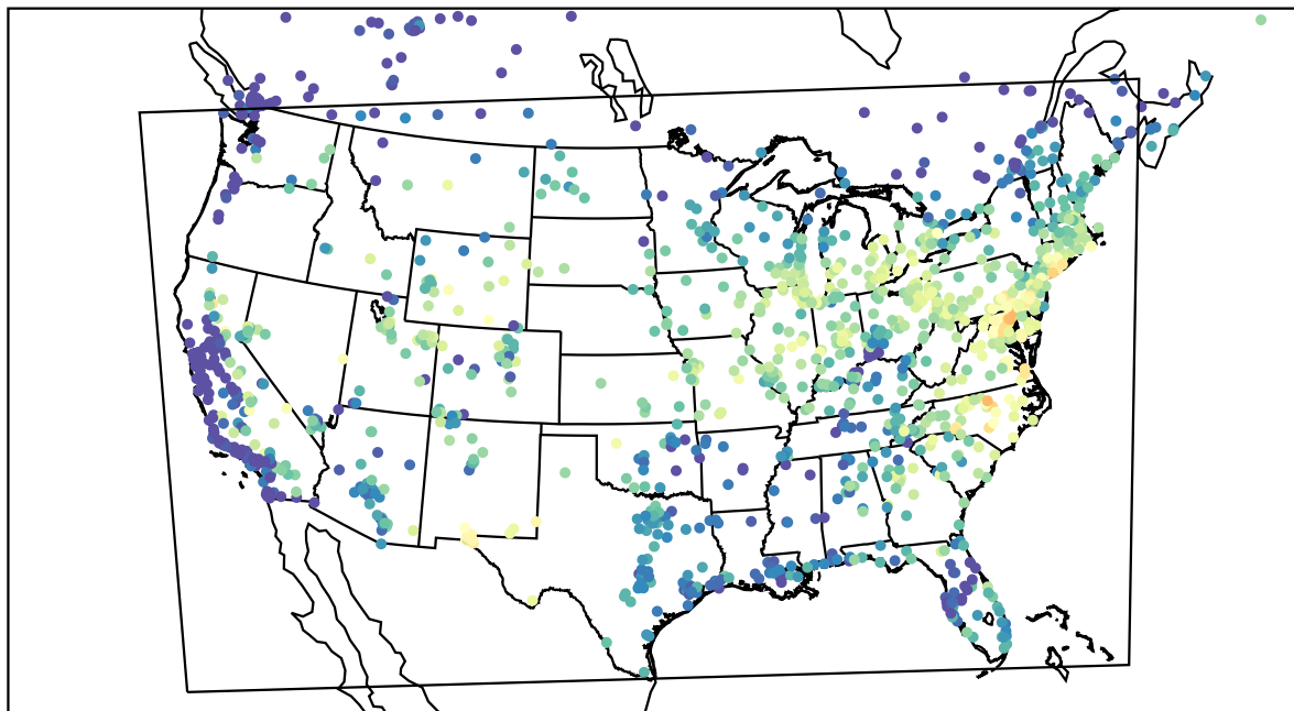
AirNOW (2023-08-12_15:00:00)
