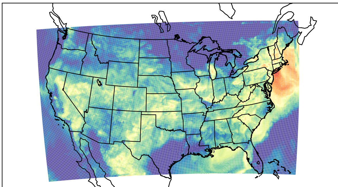
WRF (2023-08-13_05:00:00)
