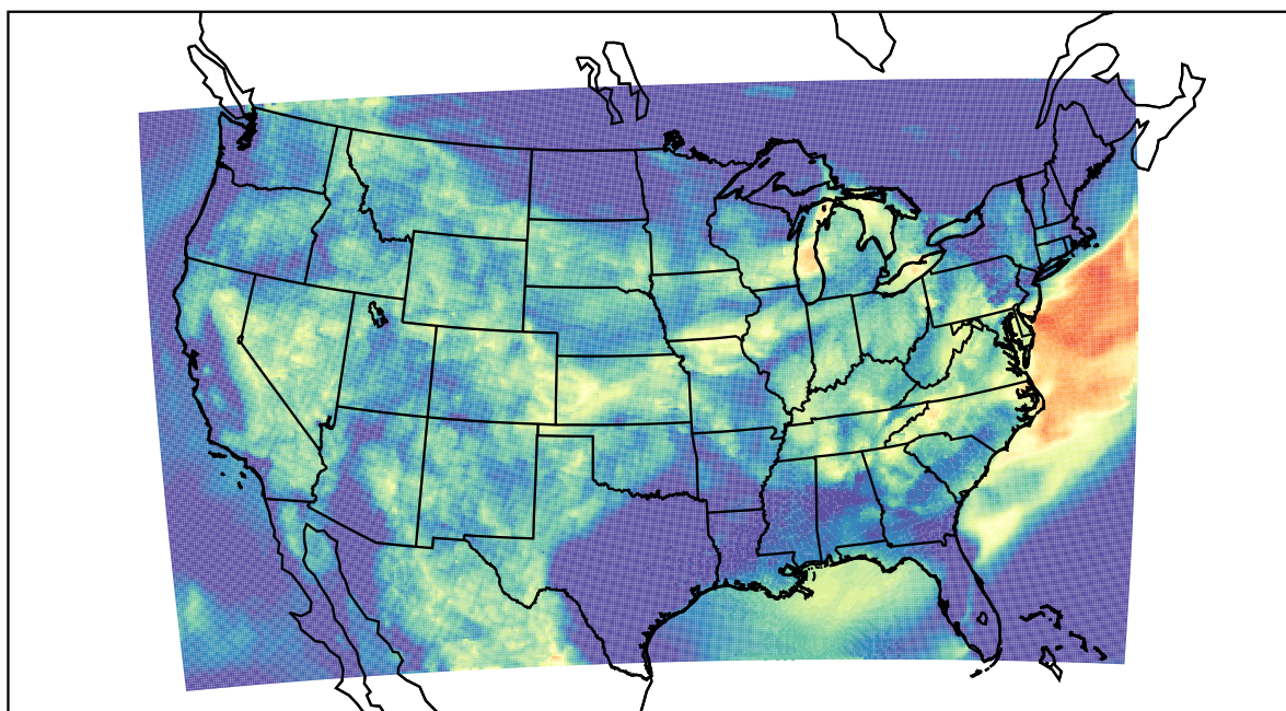
WRF (2023-08-12_09:00:00)
