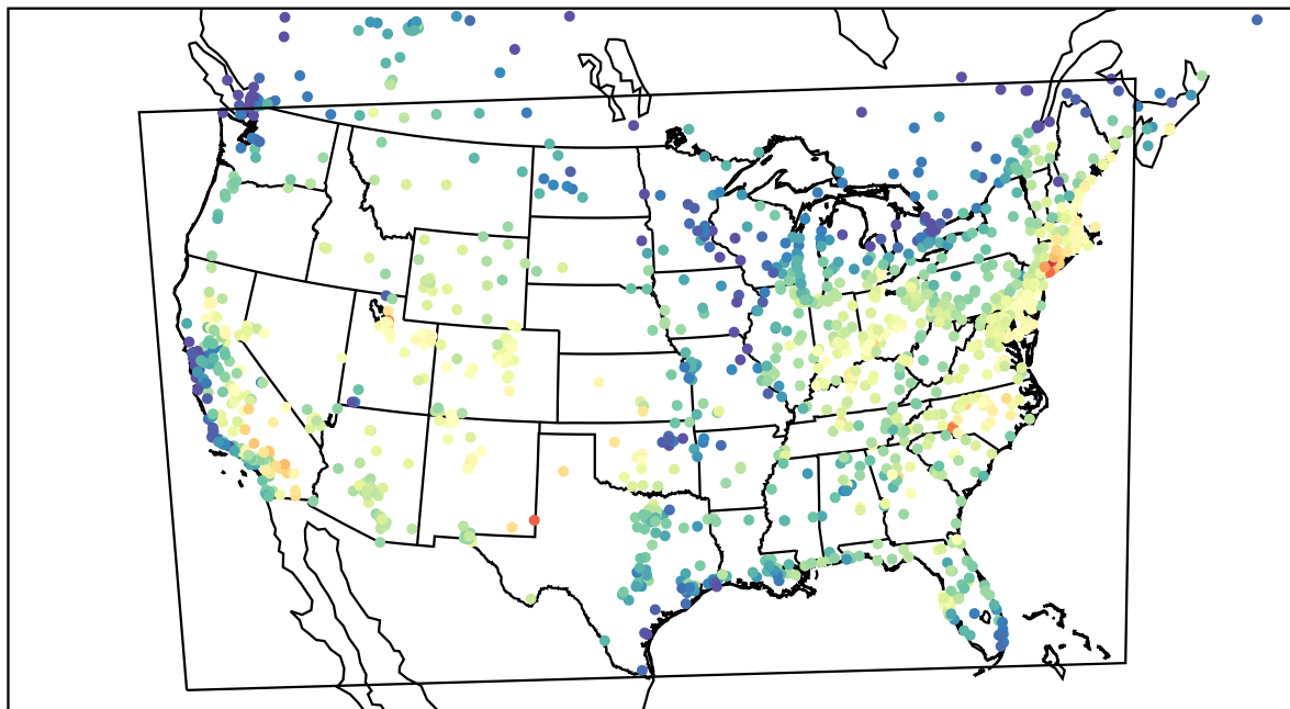
AirNOW (2023-08-13_17:00:00)
