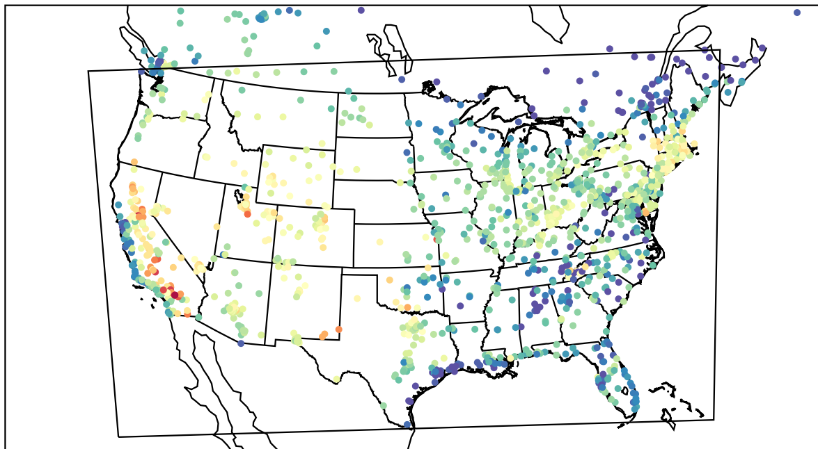
AirNOW (2023-08-13_00:00:00)
