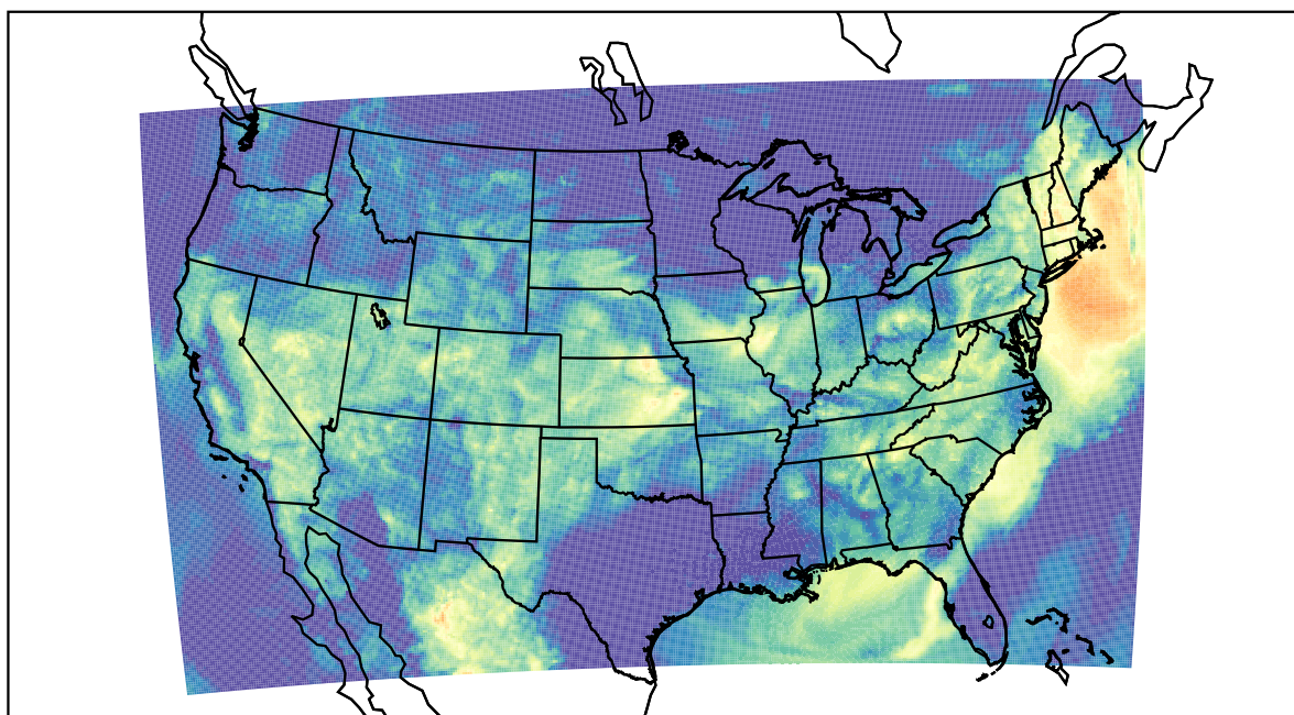
WRF (2023-08-13_09:00:00)
