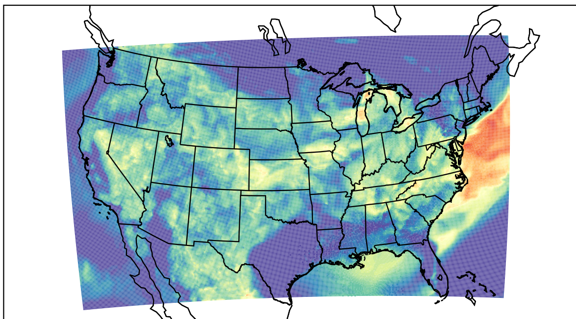
WRF (2023-08-12_08:00:00)
