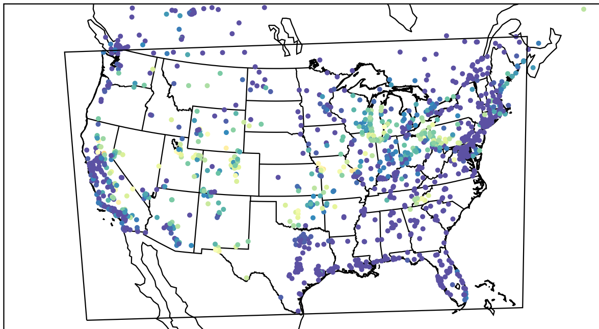
AirNOW (2023-08-12_08:00:00)
