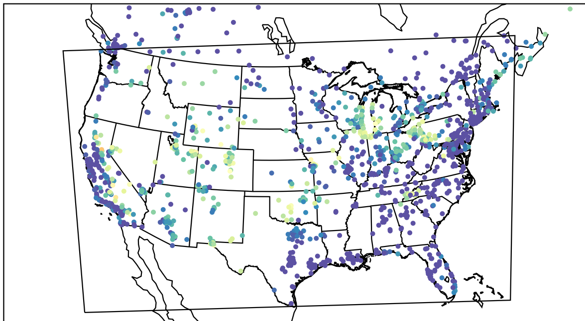
AirNOW (2023-08-12_07:00:00)
