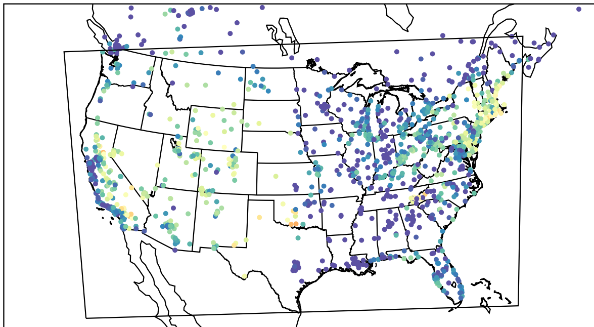
AirNOW (2023-08-13_04:00:00)
