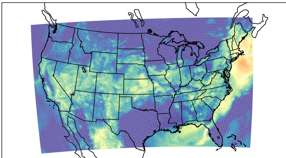
WRF (2023-08-13_11:00:00)
