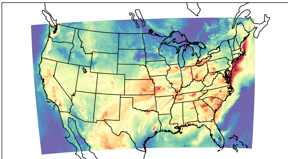
WRF (2023-08-13_21:00:00)
