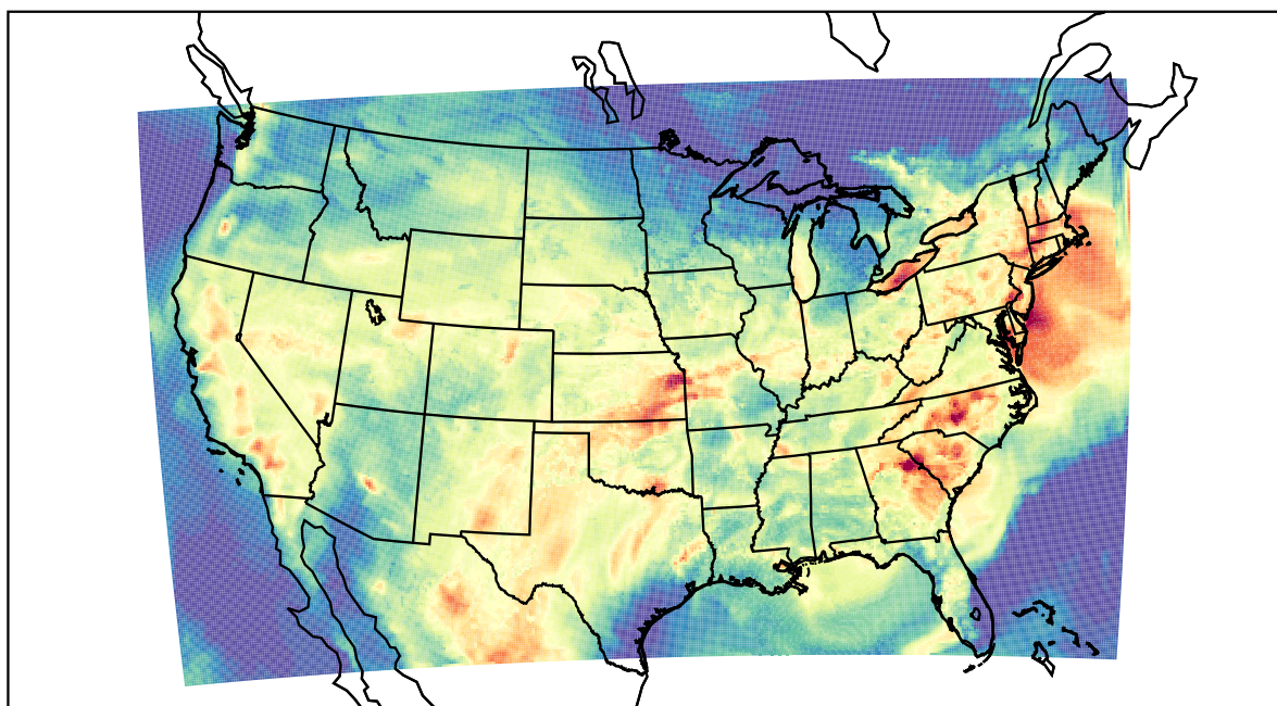
WRF (2023-08-13_00:00:00)
