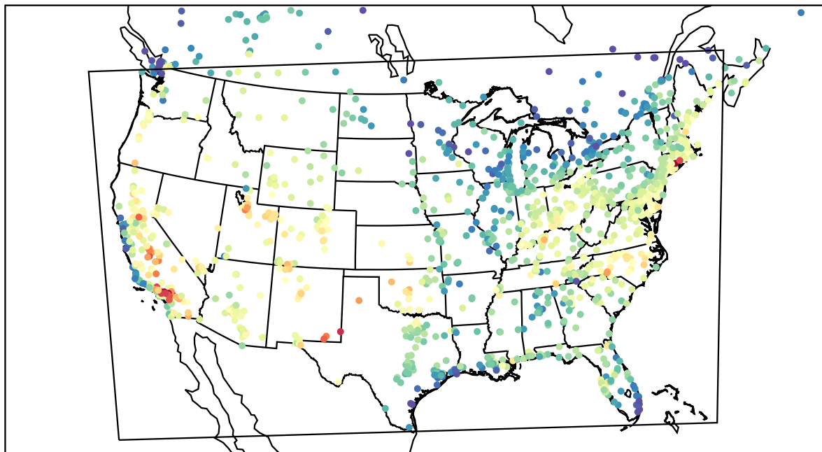
AirNOW (2023-08-13_20:00:00)
