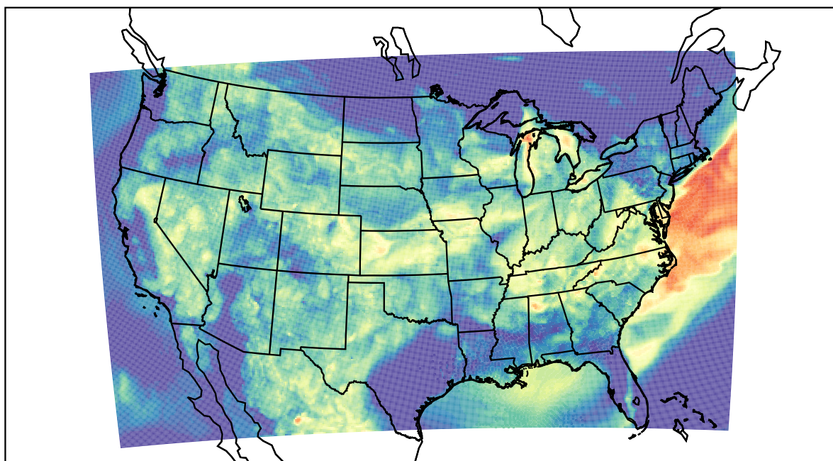
WRF (2023-08-12_06:00:00)
