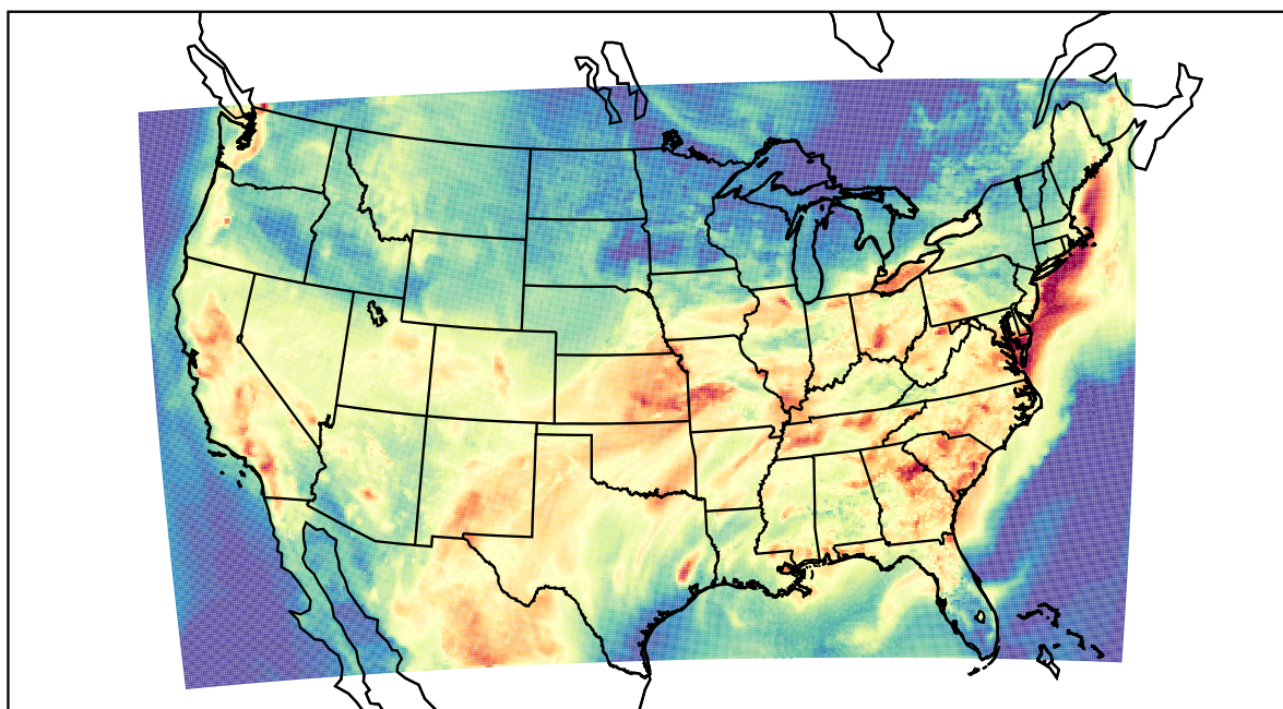
WRF (2023-08-13_22:00:00)
