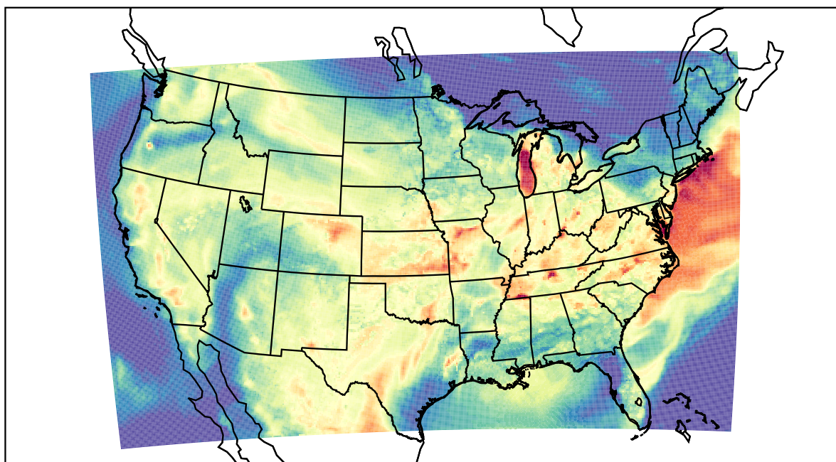
WRF (2023-08-12_00:00:00)
