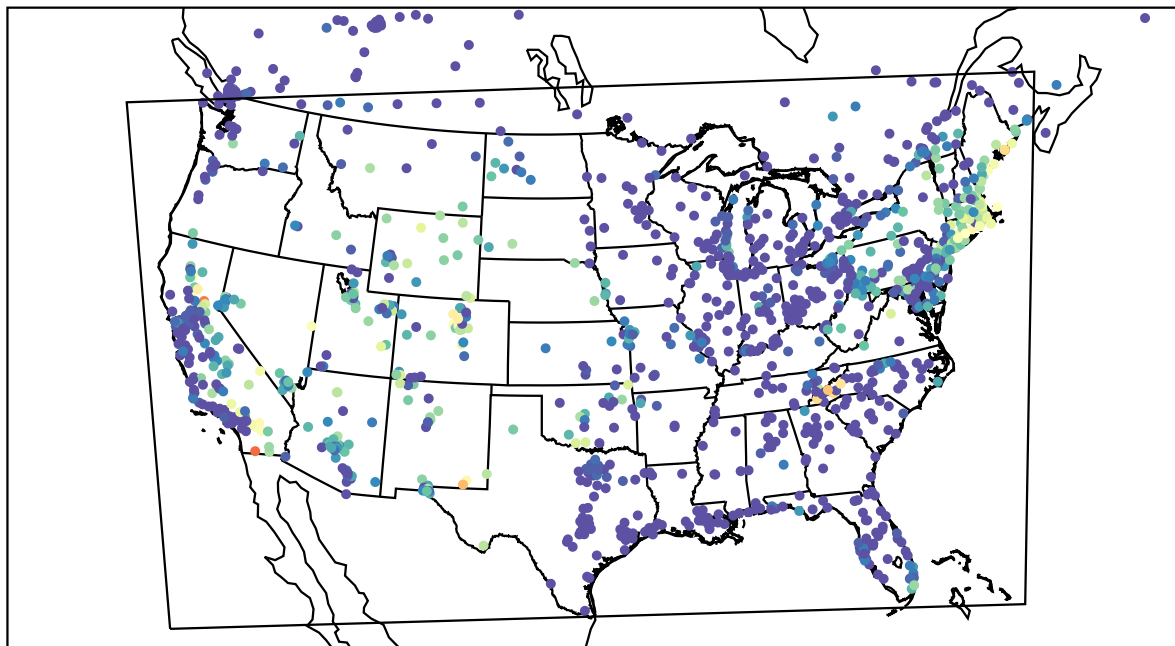
AirNOW (2023-08-13_09:00:00)
