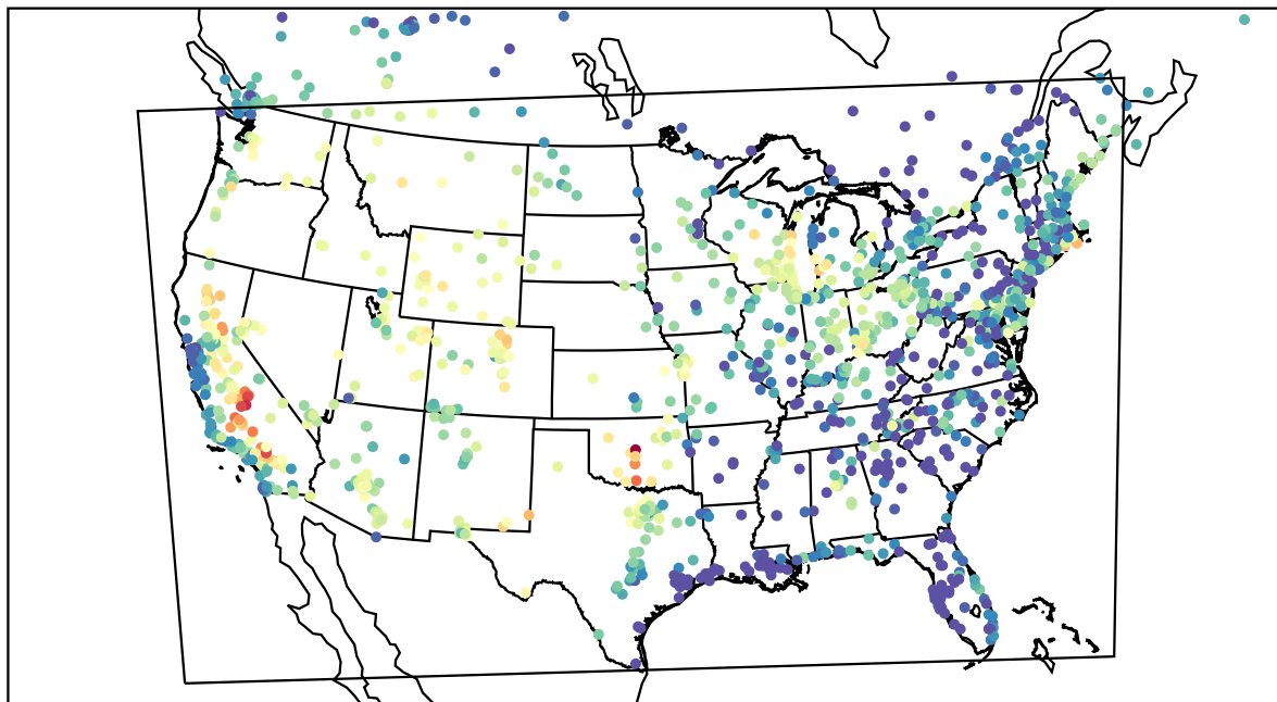
AirNOW (2023-08-12_01:00:00)
