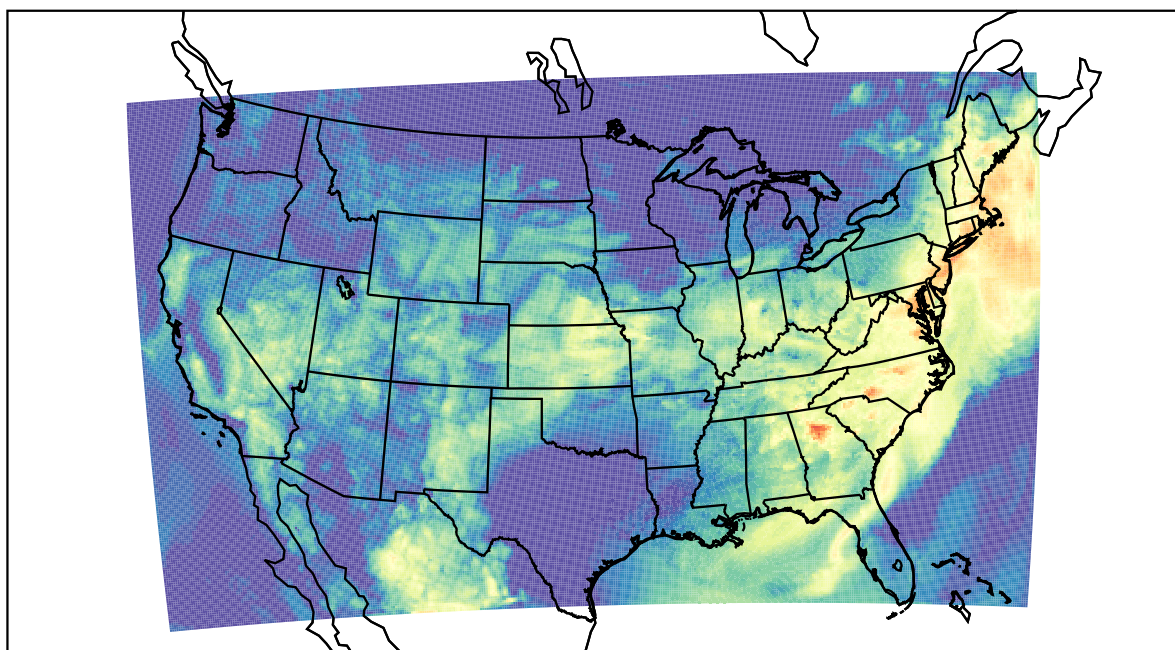
WRF (2023-08-13_14:00:00)
