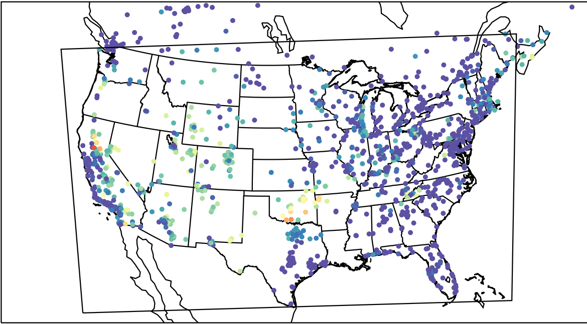
AirNOW (2023-08-14_07:00:00)
