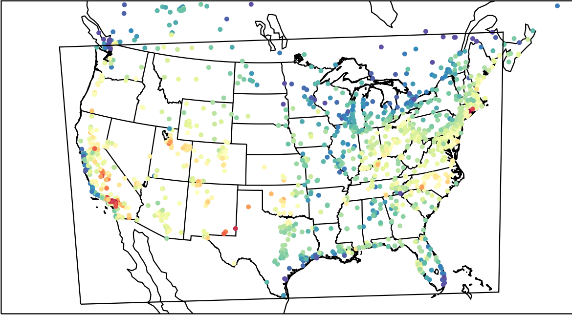
AirNOW (2023-08-13_20:00:00)
