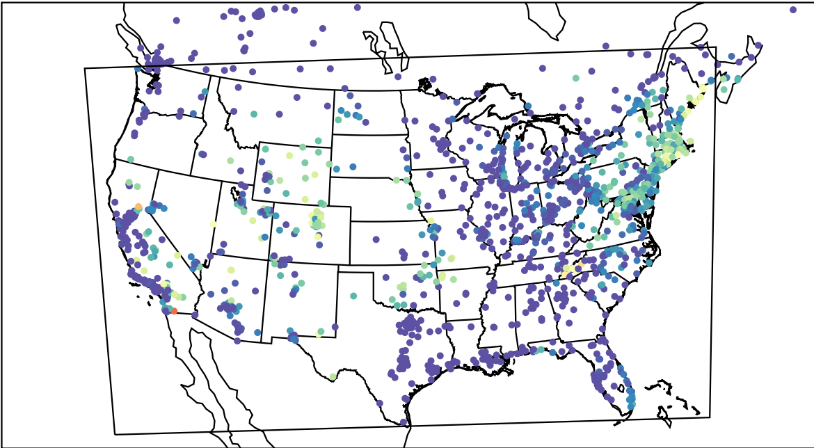
AirNOW (2023-08-13_12:00:00)
