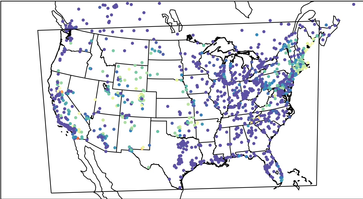
AirNOW (2023-08-13_11:00:00)
