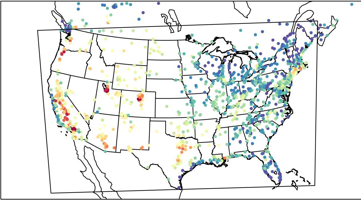
AirNOW (2023-08-14_23:00:00)
