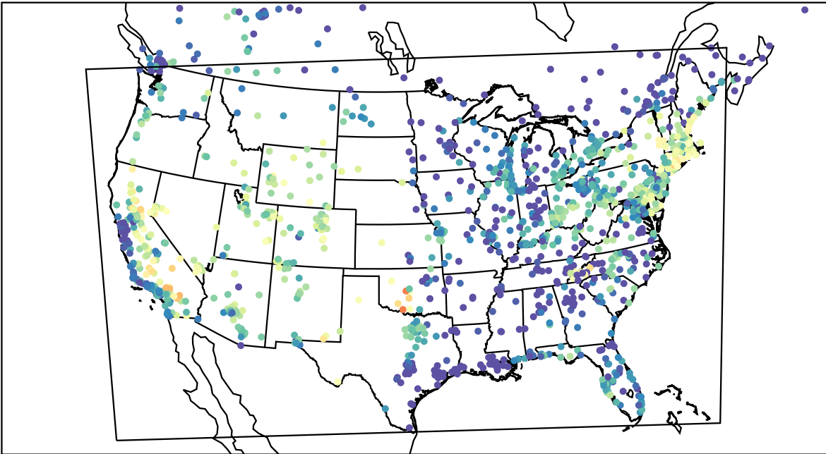
AirNOW (2023-08-13_03:00:00)
