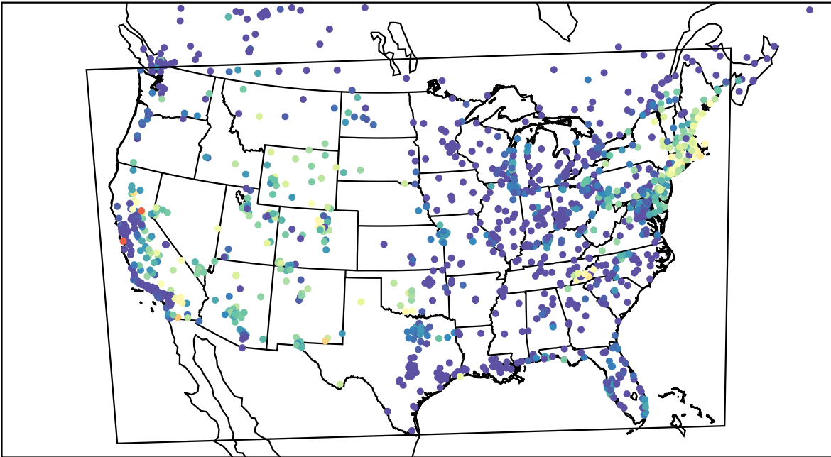
AirNOW (2023-08-13_07:00:00)
