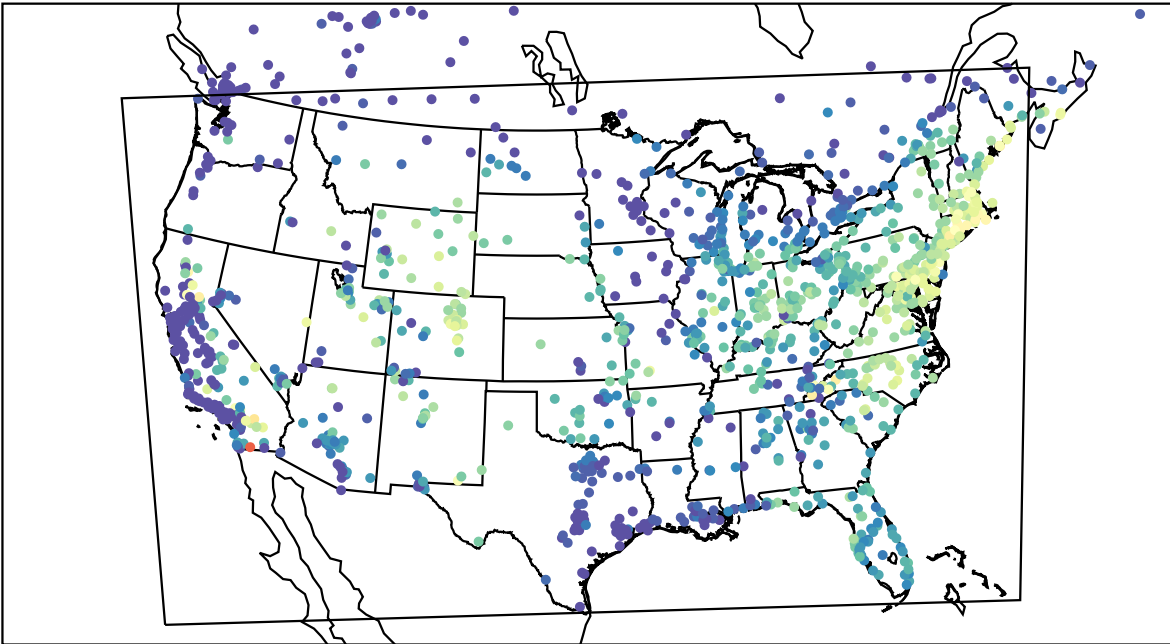
AirNOW (2023-08-13_14:00:00)
