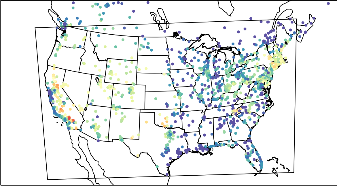
AirNOW (2023-08-13_02:00:00)
