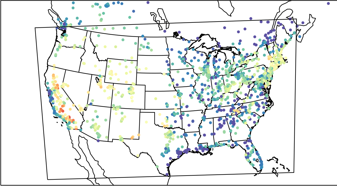
AirNOW (2023-08-13_01:00:00)
