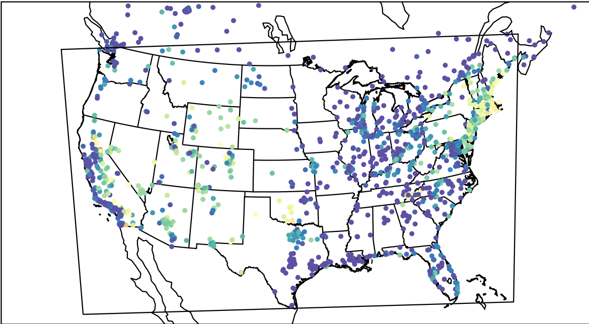
AirNOW (2023-08-13_06:00:00)
