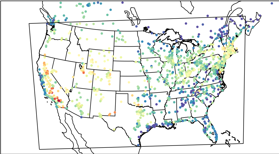
AirNOW (2023-08-13_00:00:00)
