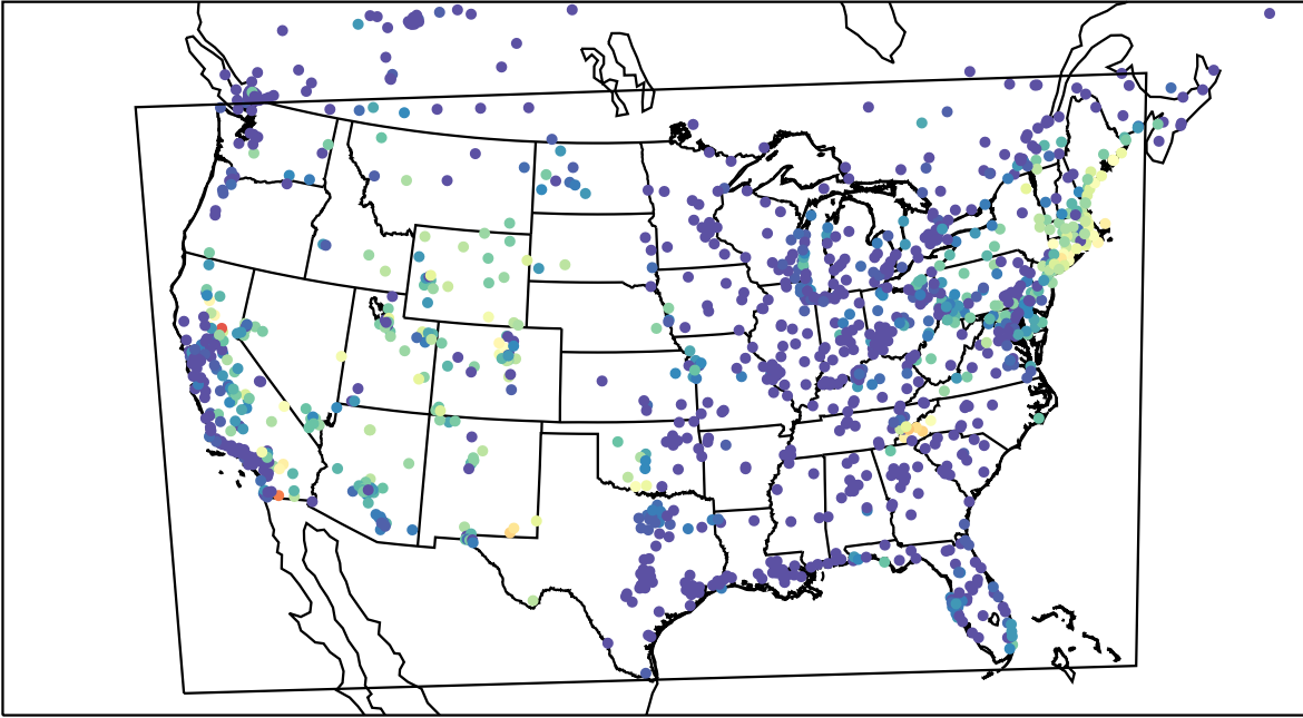
AirNOW (2023-08-13_08:00:00)
