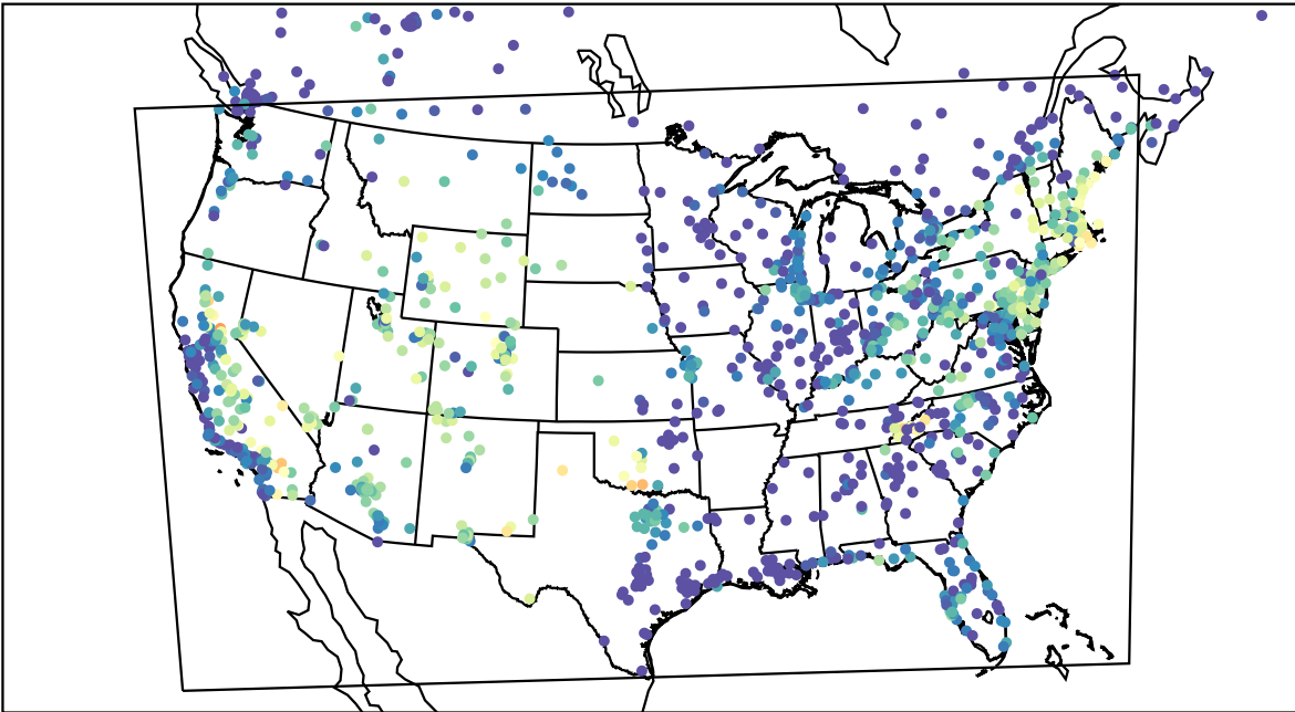
AirNOW (2023-08-13_05:00:00)
