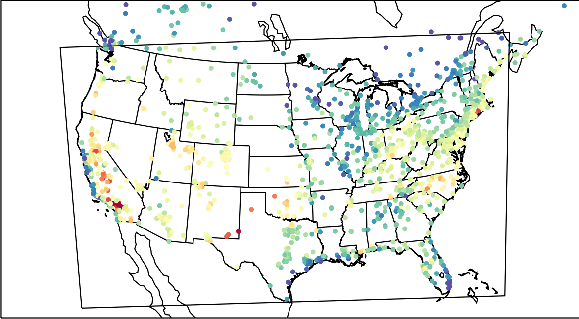
AirNOW (2023-08-13_21:00:00)
