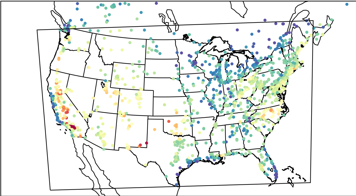
AirNOW (2023-08-13_22:00:00)
