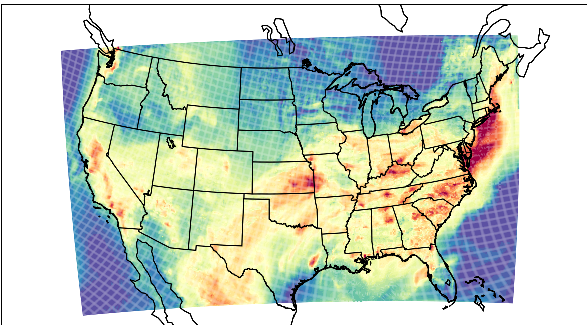
WRF (2023-08-13_22:00:00)
