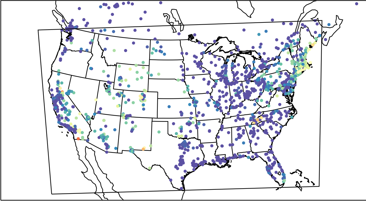
AirNOW (2023-08-13_09:00:00)
