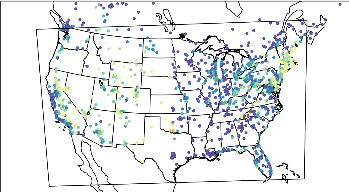
AirNOW (2023-08-13_04:00:00)
