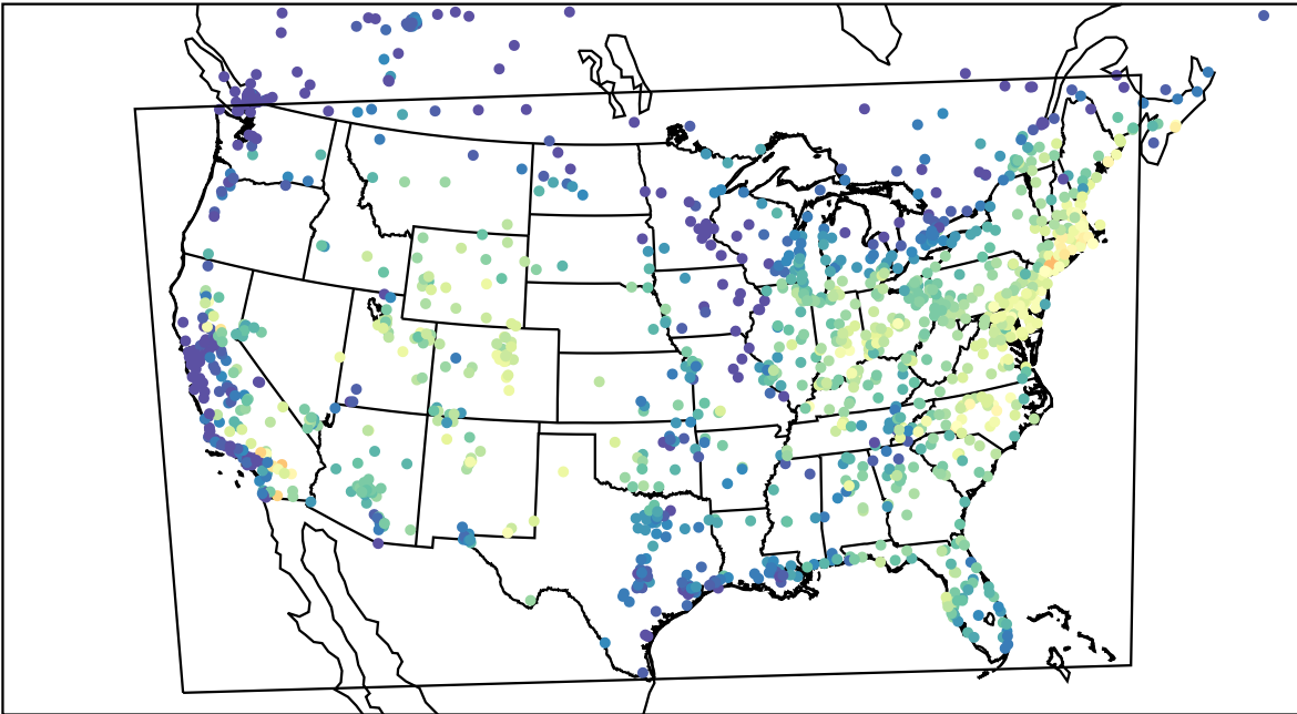
AirNOW (2023-08-13_15:00:00)
