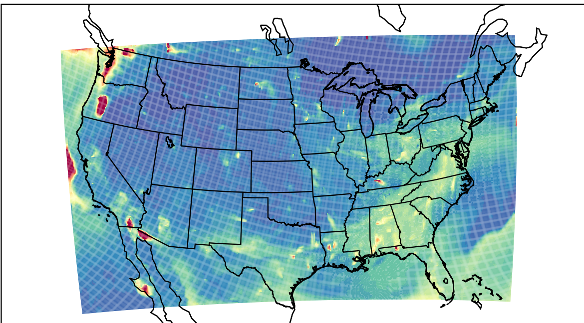
WRF 2023-08-15_04:00:00
