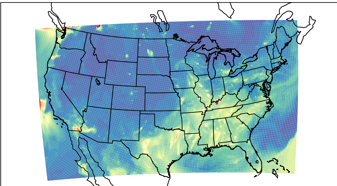
WRF 2023-08-14_09:00:00
