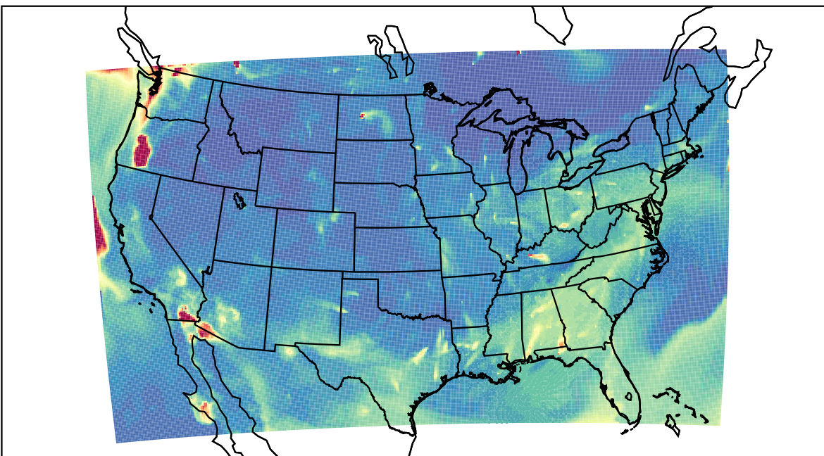
WRF 2023-08-15_06:00:00
