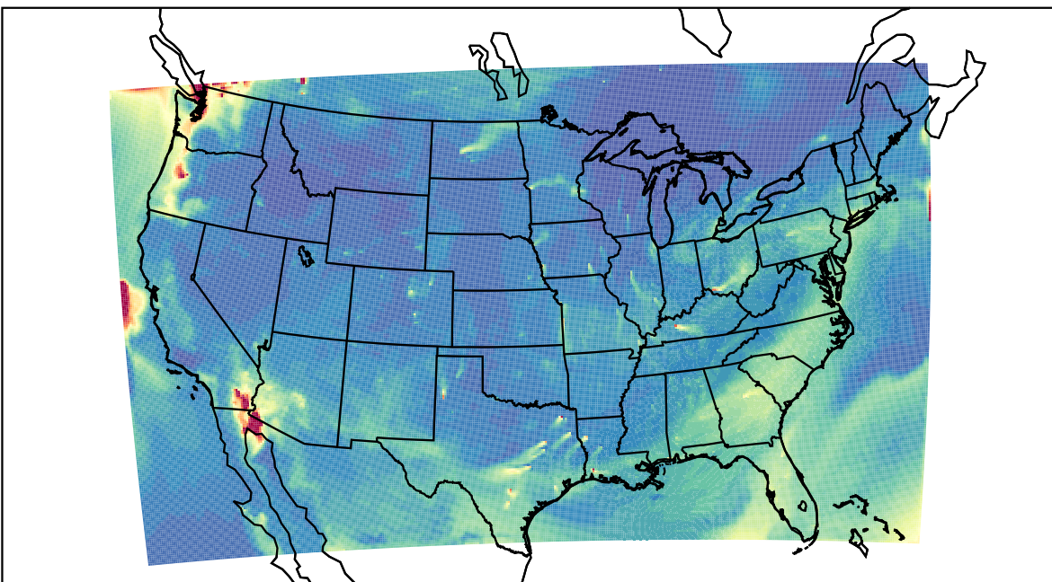
WRF 2023-08-15_15:00:00
