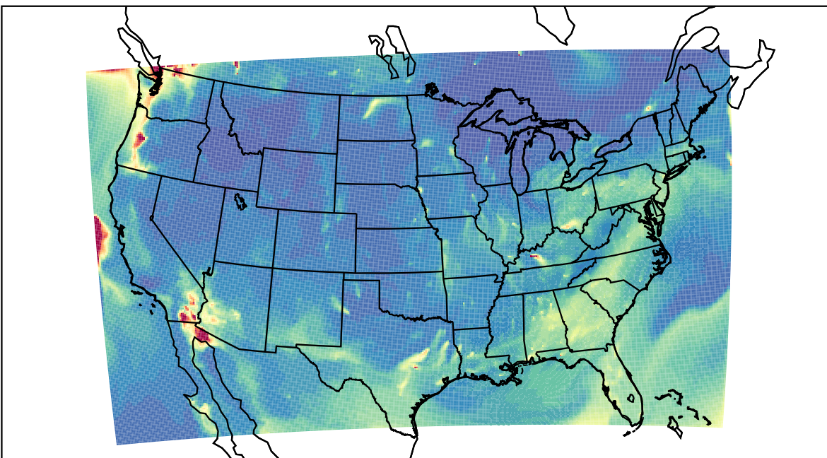
WRF 2023-08-15_11:00:00
