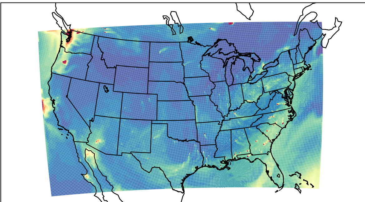
WRF 2023-08-15_23:00:00
