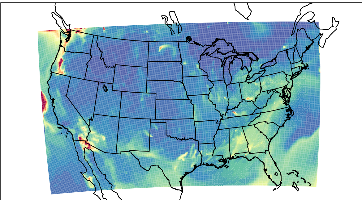
WRF 2023-08-15_09:00:00
