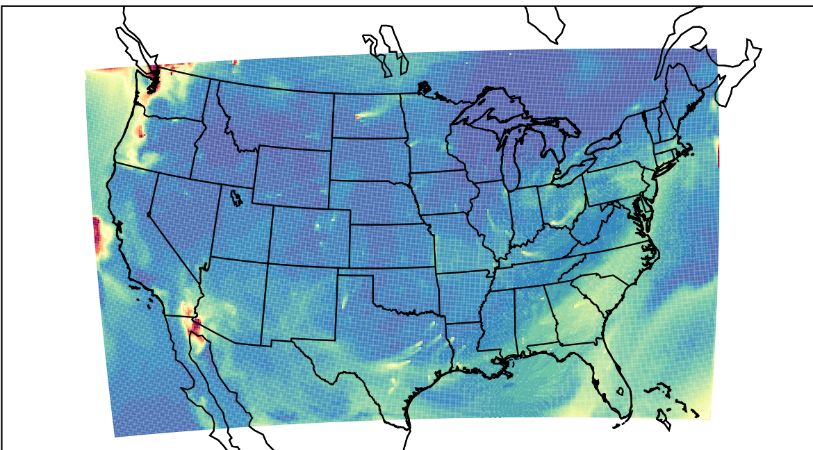
WRF 2023-08-15_16:00:00
