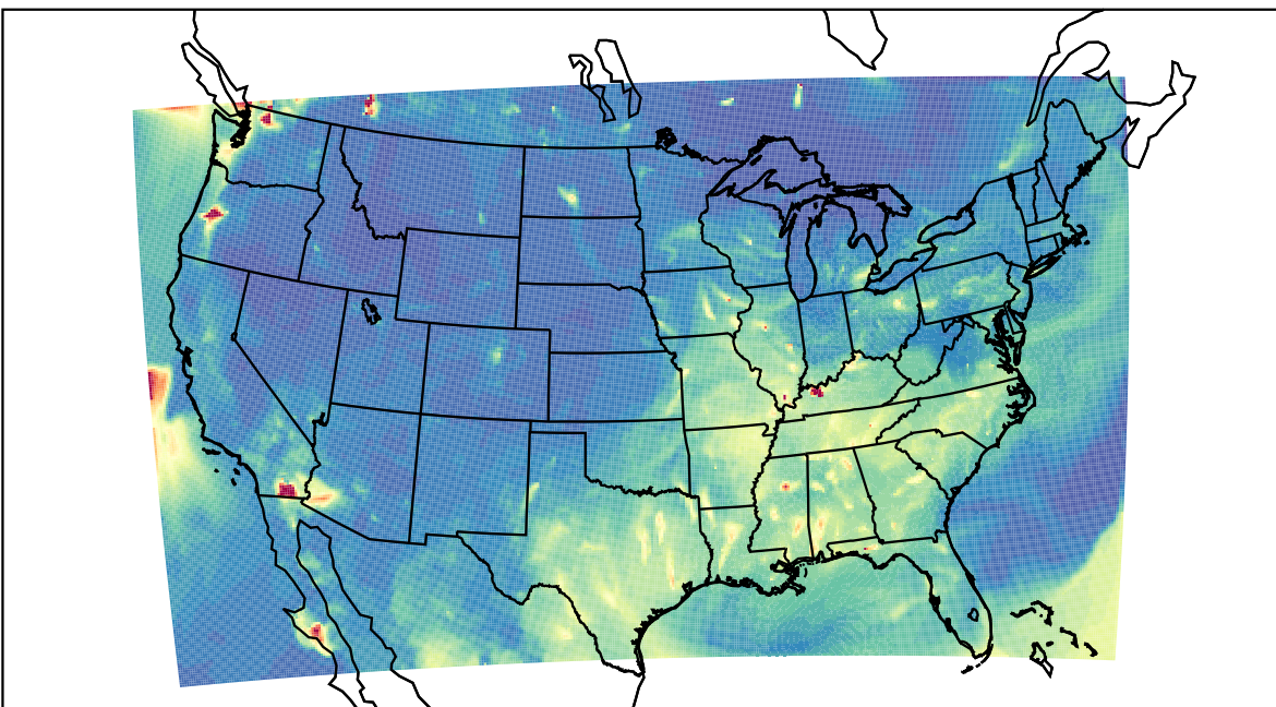
WRF 2023-08-14_06:00:00
