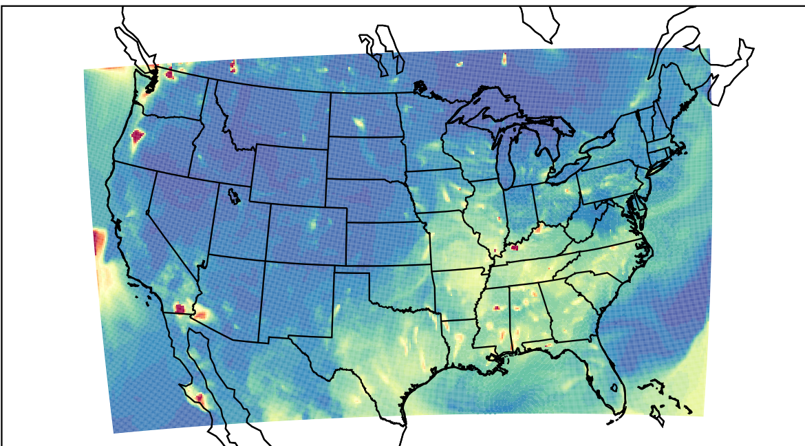
WRF 2023-08-14_05:00:00
