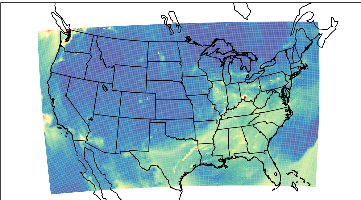
WRF 2023-08-14_16:00:00
