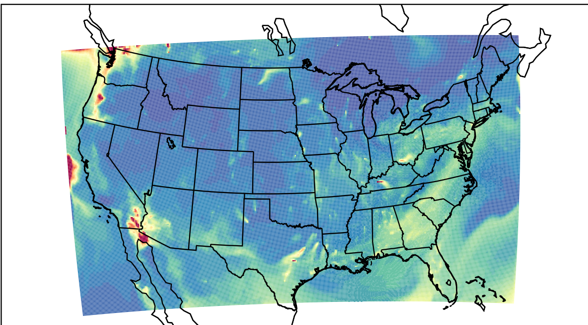
WRF 2023-08-15_12:00:00
