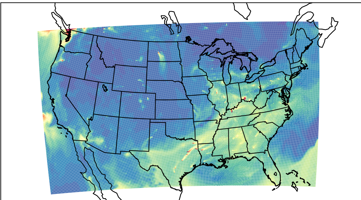
WRF 2023-08-14_15:00:00
