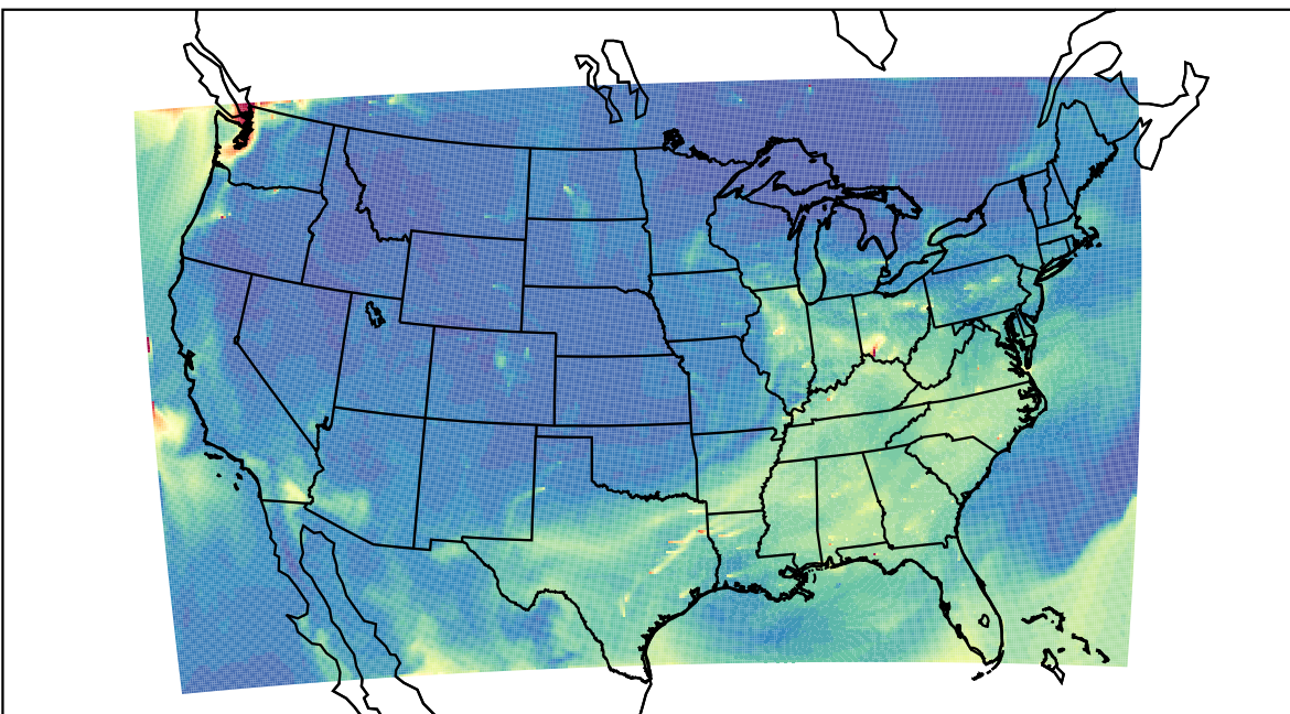
WRF 2023-08-14_17:00:00
