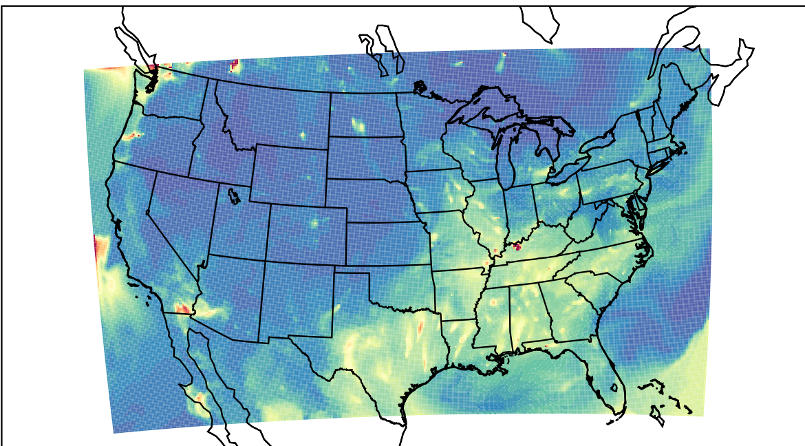
WRF 2023-08-14_08:00:00
