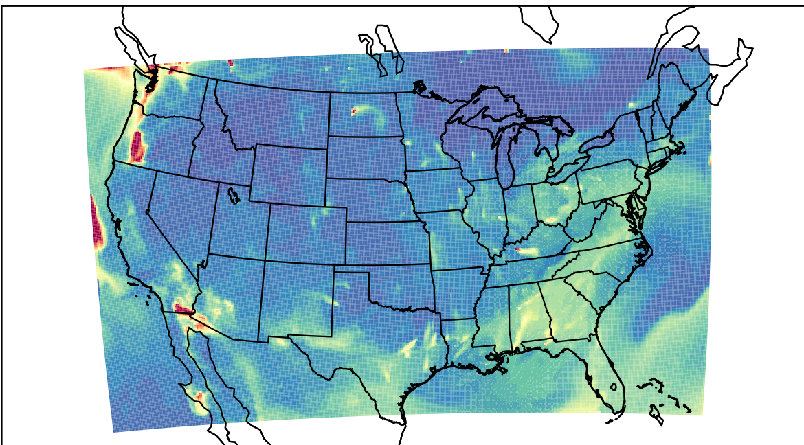
WRF 2023-08-15_07:00:00
