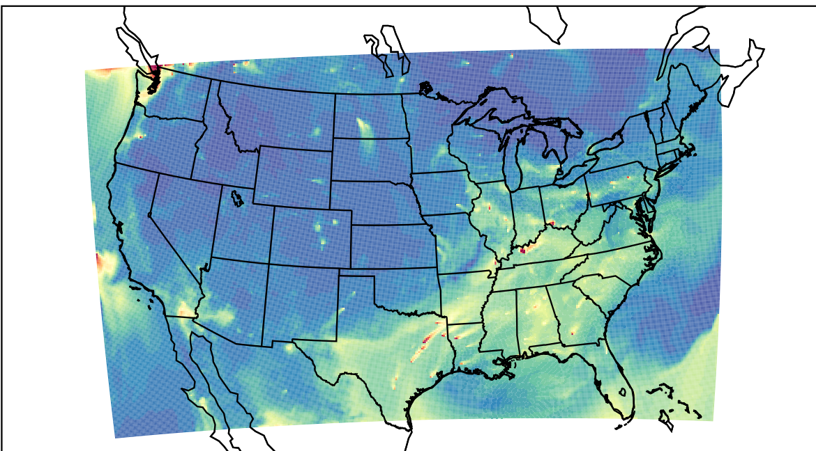
WRF 2023-08-14_14:00:00
