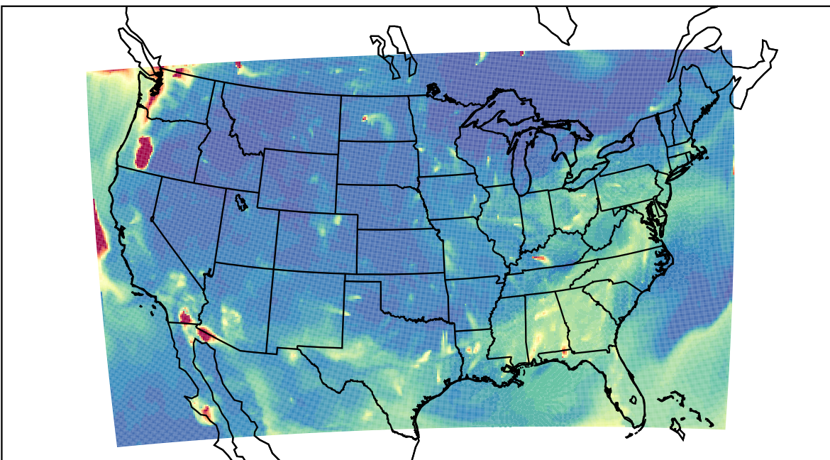
WRF 2023-08-15_05:00:00
