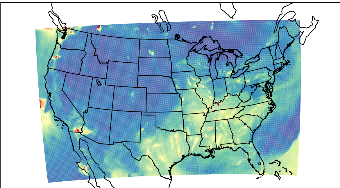
WRF 2023-08-14_07:00:00
