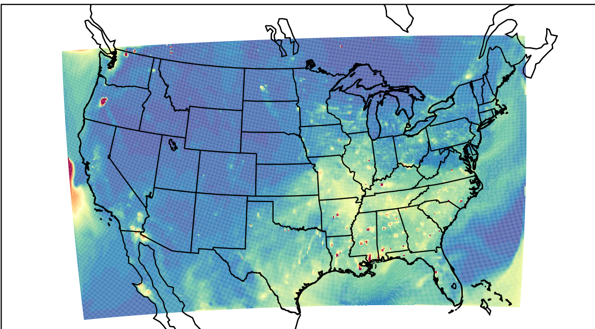
WRF 2023-08-14_01:00:00
