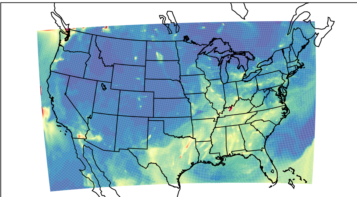
WRF 2023-08-14_11:00:00
