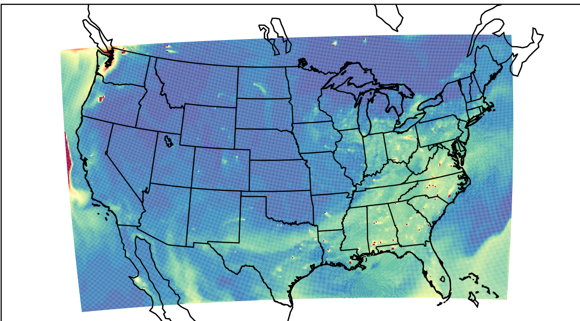
WRF 2023-08-14_23:00:00
