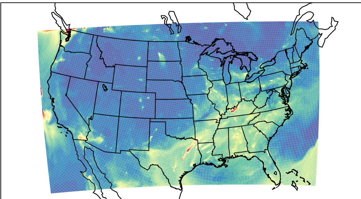
WRF 2023-08-14_13:00:00
