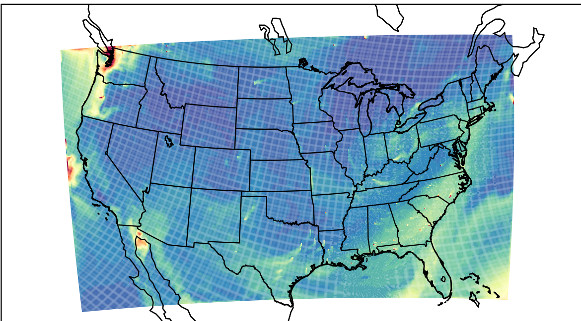
WRF 2023-08-15_19:00:00
