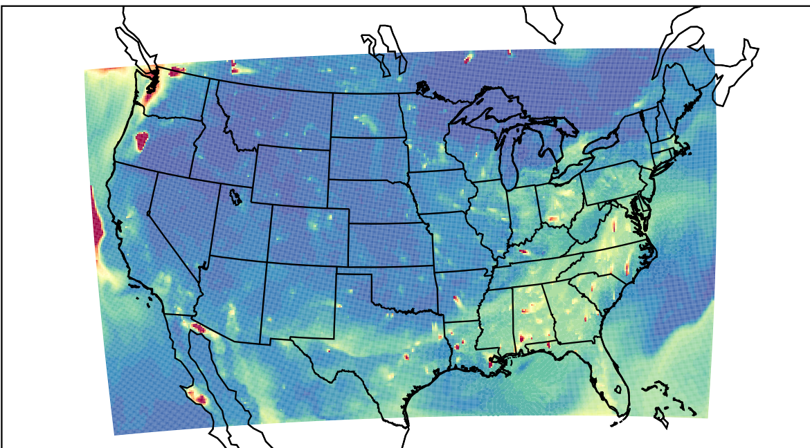
WRF 2023-08-15_02:00:00
