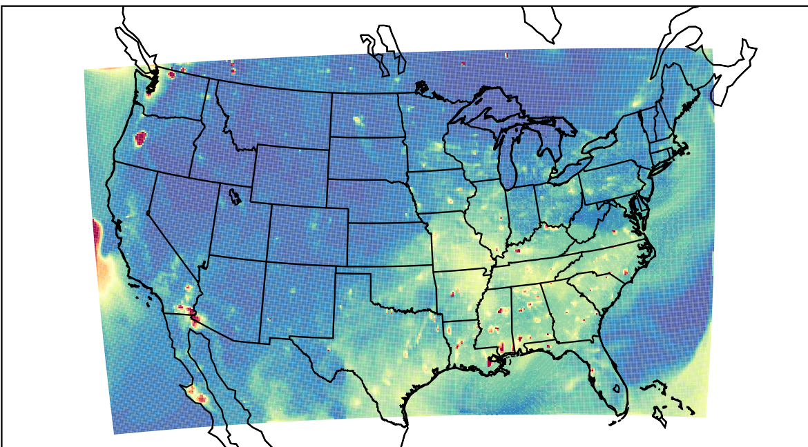
WRF 2023-08-14_02:00:00
