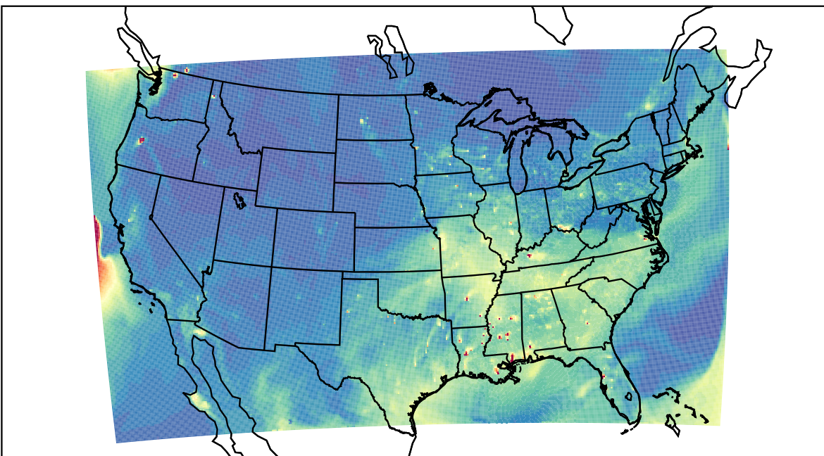
WRF 2023-08-14_00:00:00
