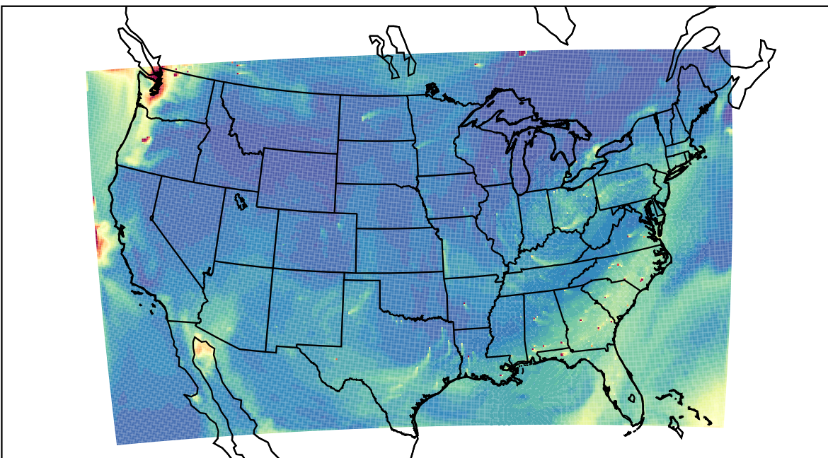
WRF 2023-08-15_21:00:00
