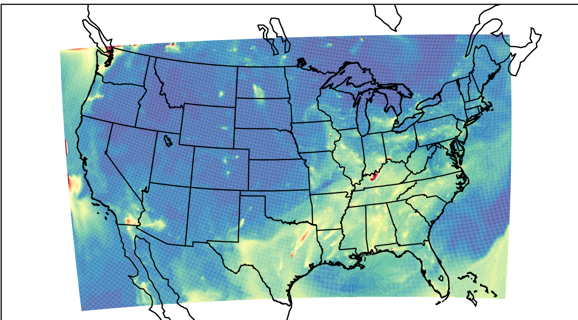
WRF 2023-08-14_12:00:00
