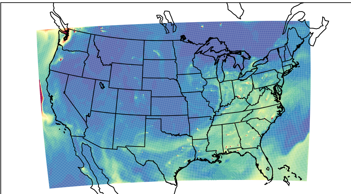
WRF 2023-08-14_22:00:00
