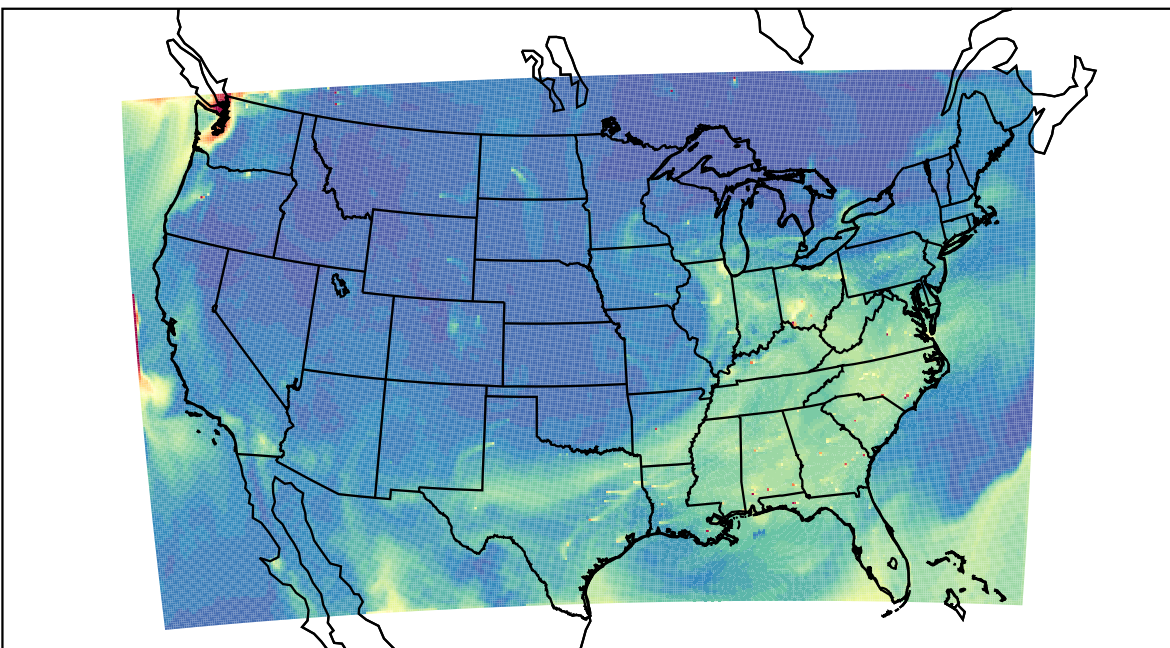
WRF 2023-08-14_19:00:00
