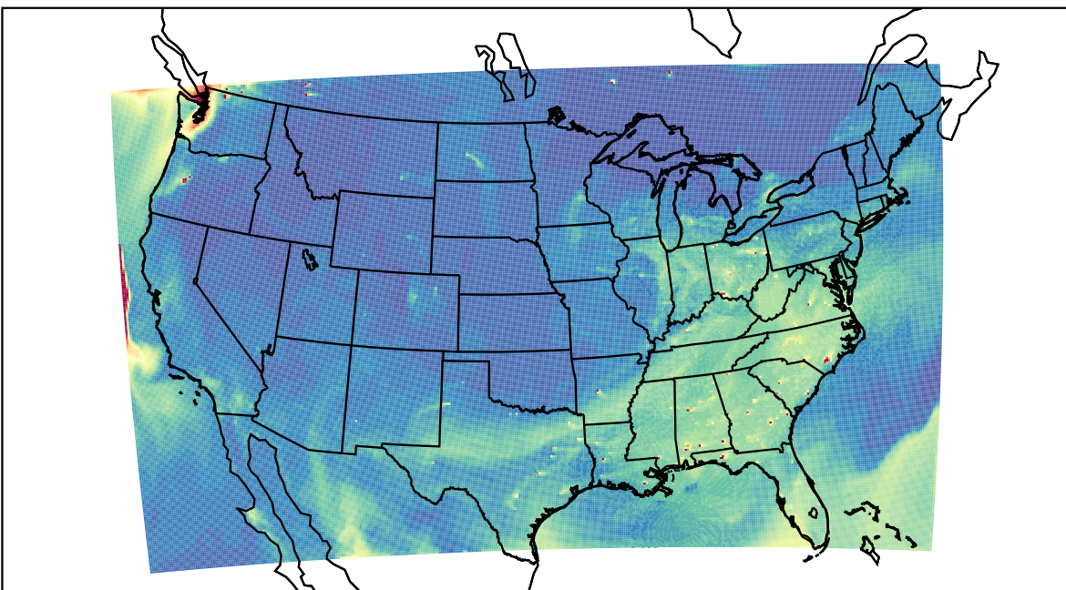
WRF 2023-08-14_21:00:00
