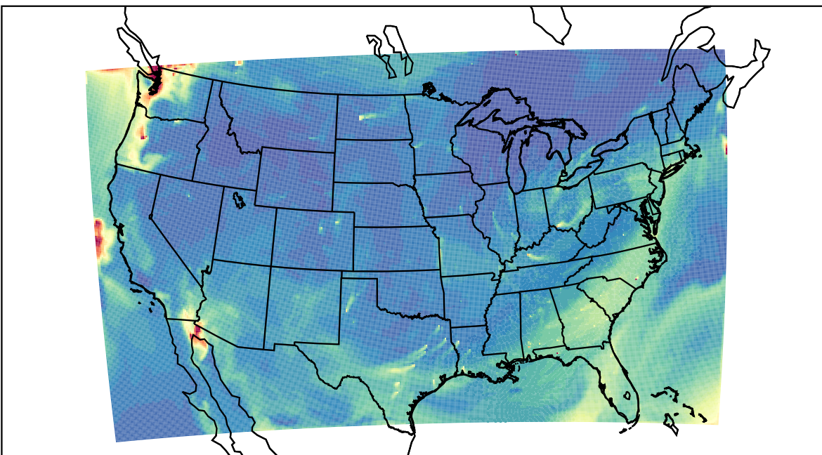
WRF 2023-08-15_17:00:00
