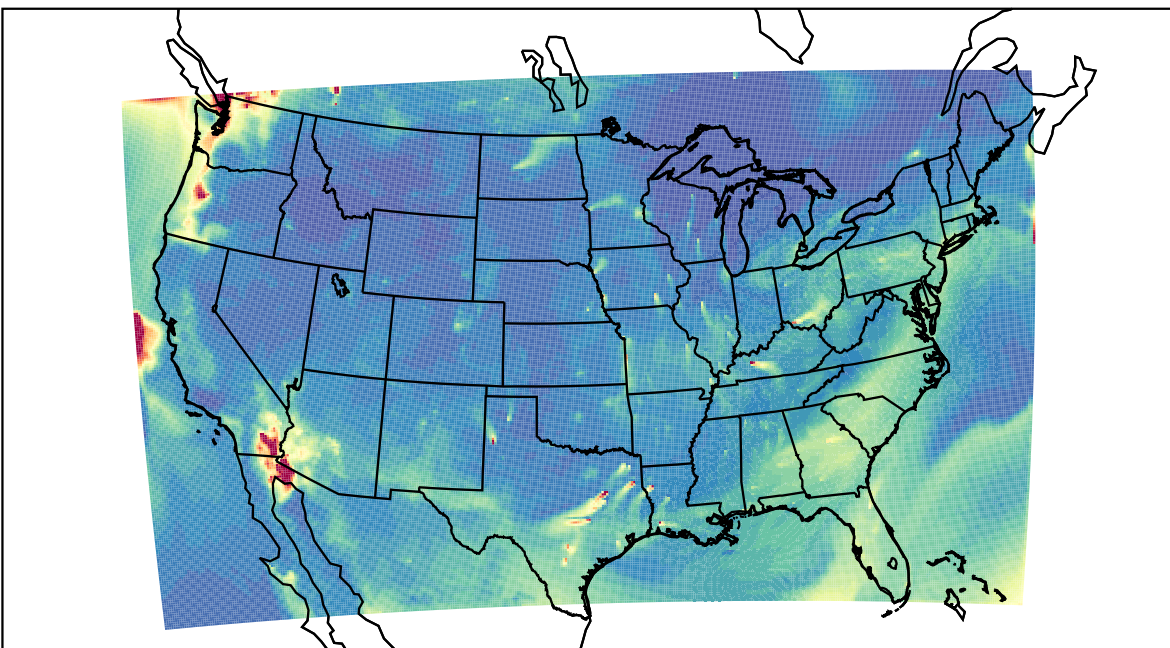
WRF 2023-08-15_14:00:00
