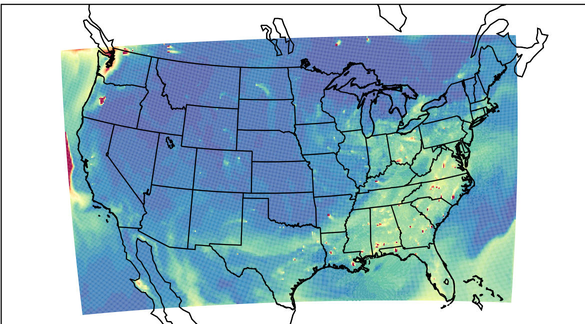
WRF 2023-08-15_00:00:00
