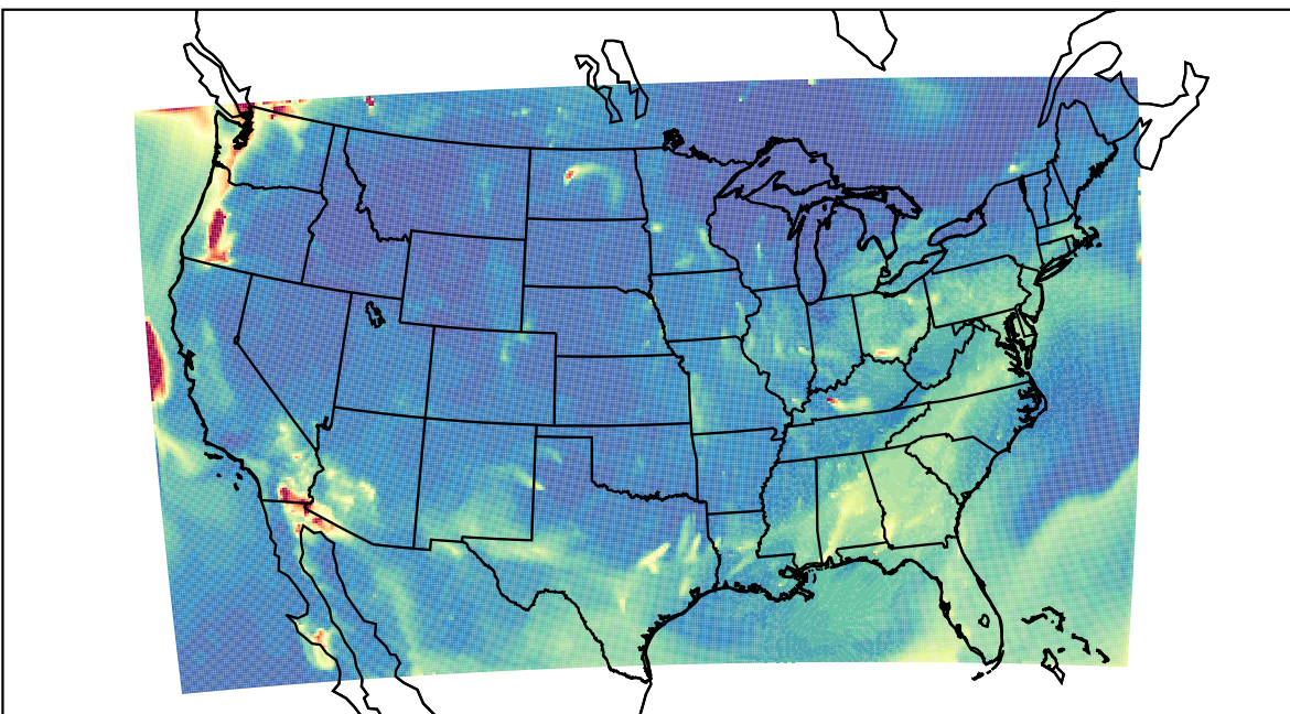
WRF 2023-08-15_08:00:00
