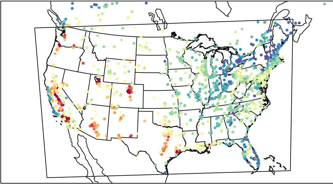
AirNOW (2023-08-15_21:00:00)
