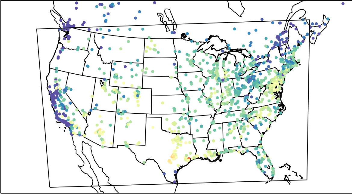
AirNOW (2023-08-16_15:00:00)
