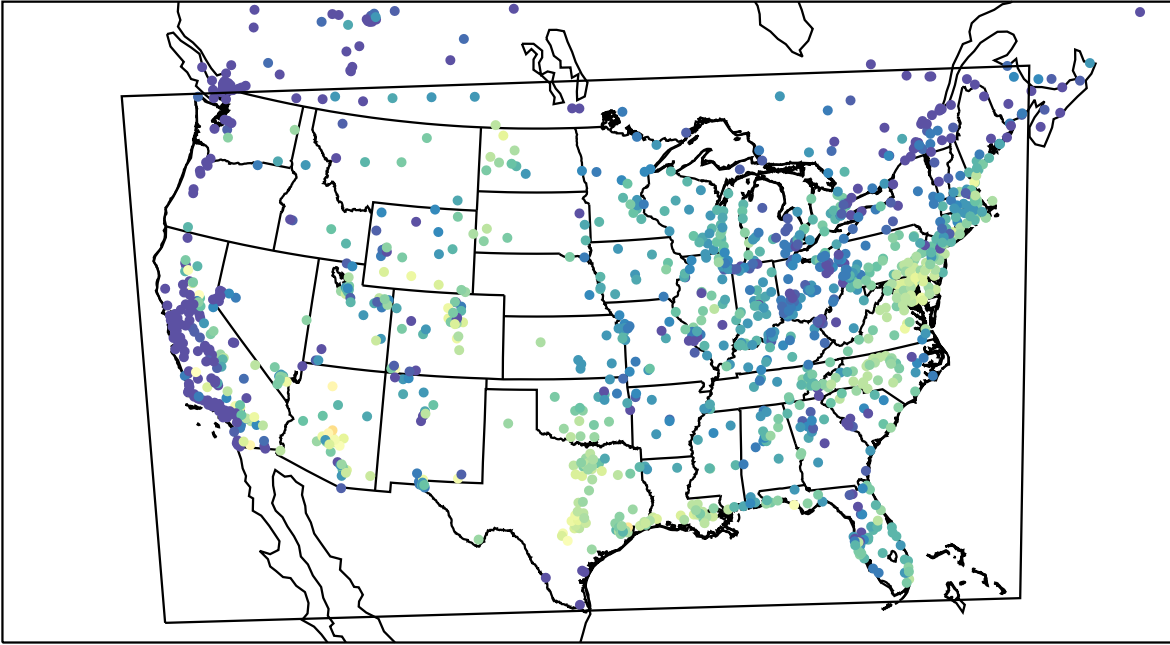
AirNOW (2023-08-16_14:00:00)
