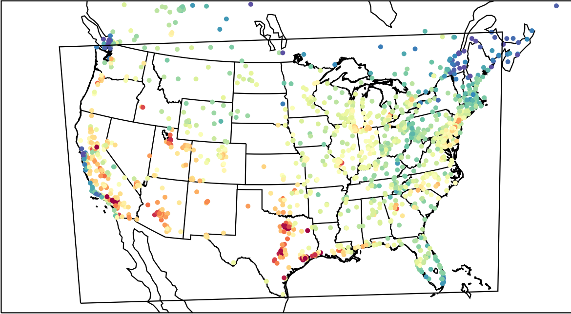
AirNOW (2023-08-16_19:00:00)
