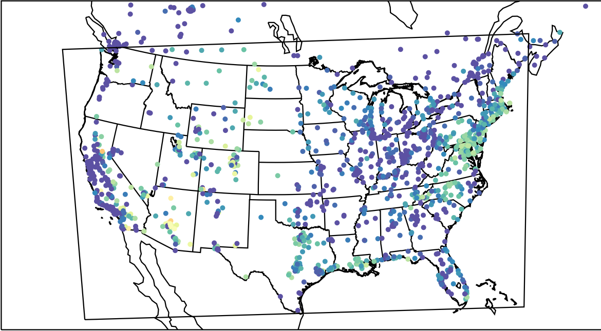
AirNOW (2023-08-16_13:00:00)
