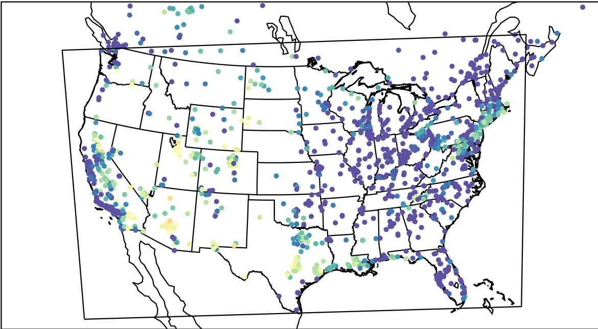
AirNOW (2023-08-16_07:00:00)
