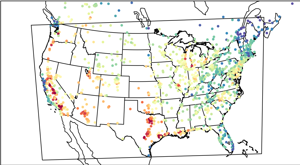
AirNOW (2023-08-16_22:00:00)
