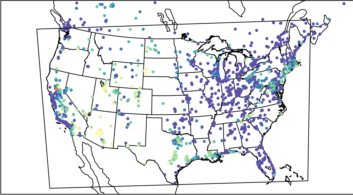
AirNOW (2023-08-16_08:00:00)
