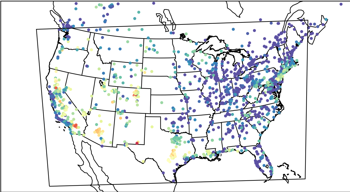
AirNOW (2023-08-16_04:00:00)
