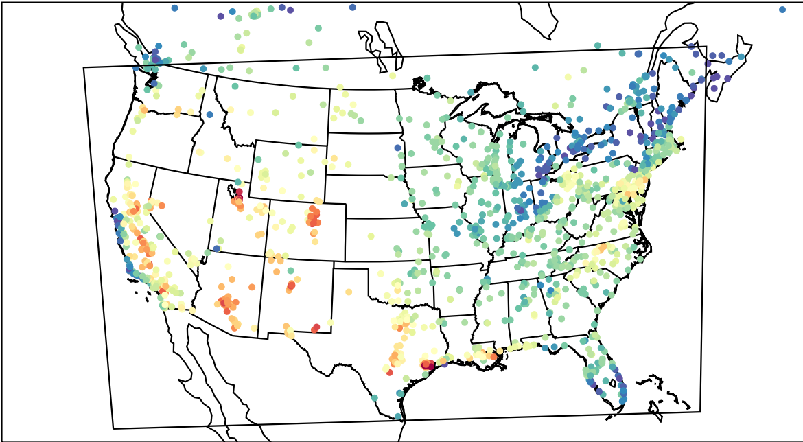
AirNOW (2023-08-15_18:00:00)
