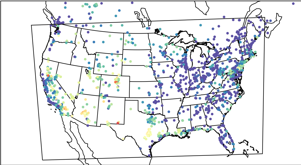
AirNOW (2023-08-16_05:00:00)
