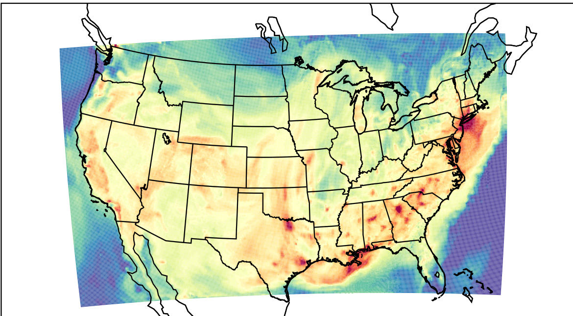
WRF (2023-08-16_19:00:00)
