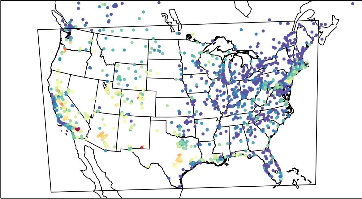
AirNOW (2023-08-16_03:00:00)
