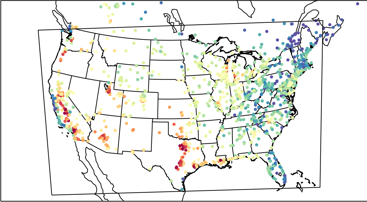
AirNOW (2023-08-16_23:00:00)
