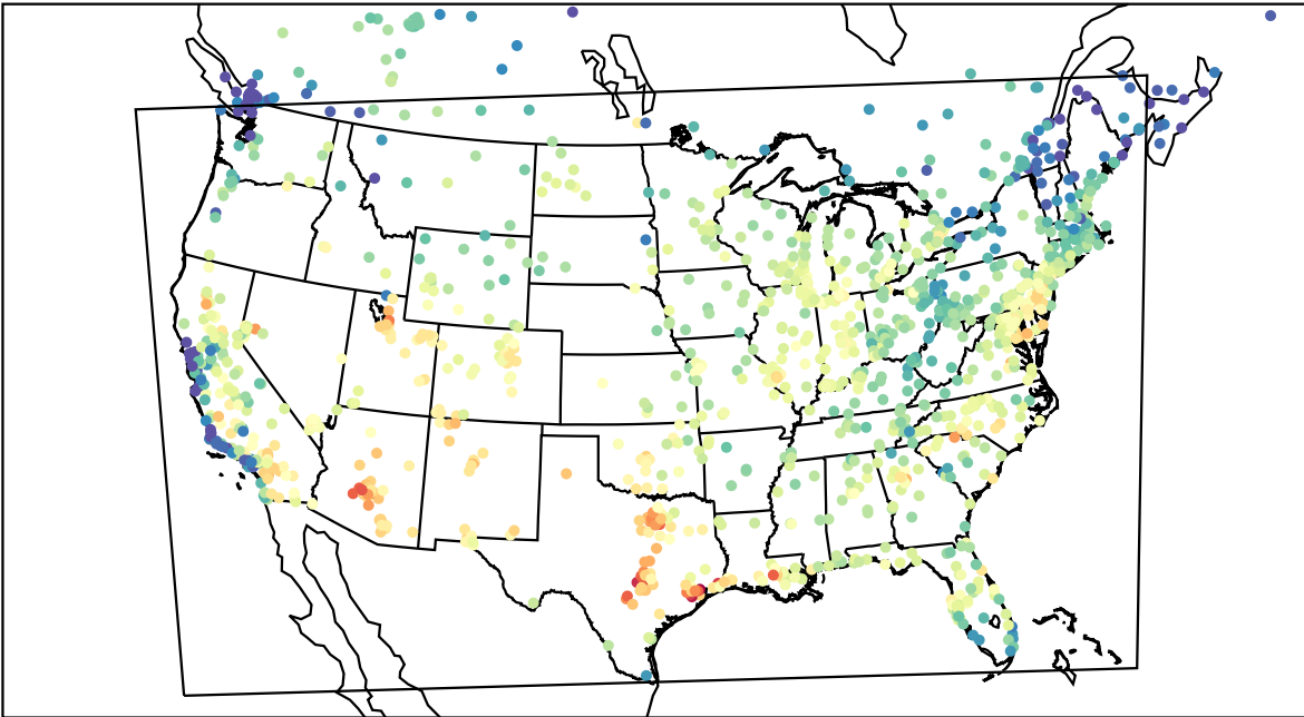
AirNOW (2023-08-16_17:00:00)
