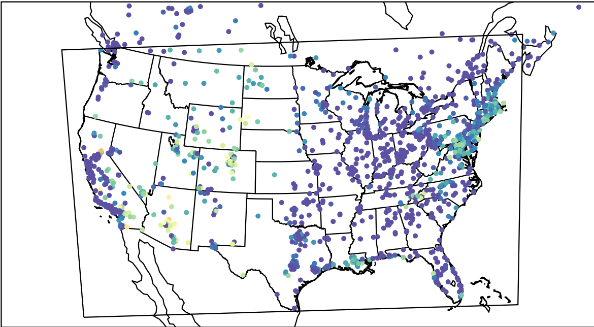
AirNOW (2023-08-16_12:00:00)
