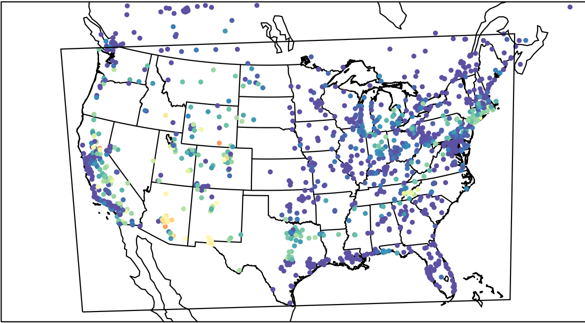
AirNOW (2023-08-15_08:00:00)
