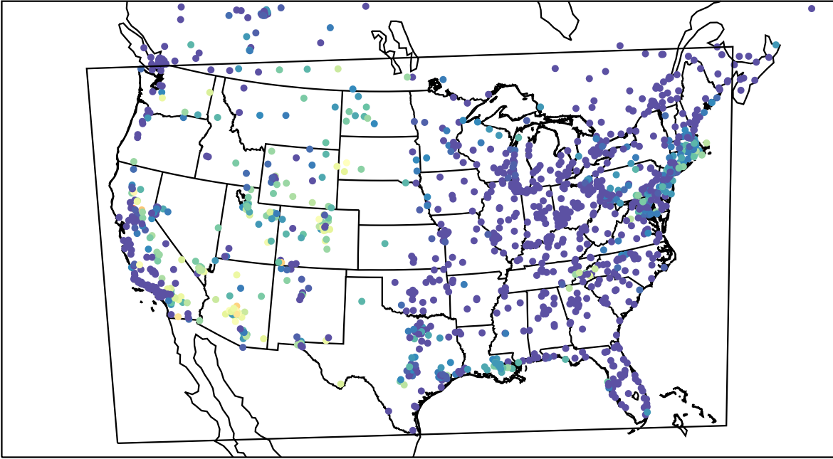
AirNOW (2023-08-16_11:00:00)
