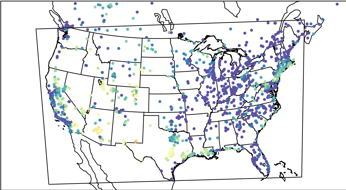
AirNOW (2023-08-16_06:00:00)
