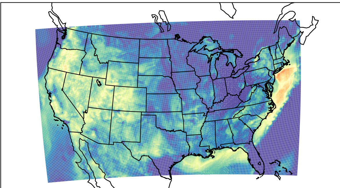
WRF (2023-08-16_12:00:00)
