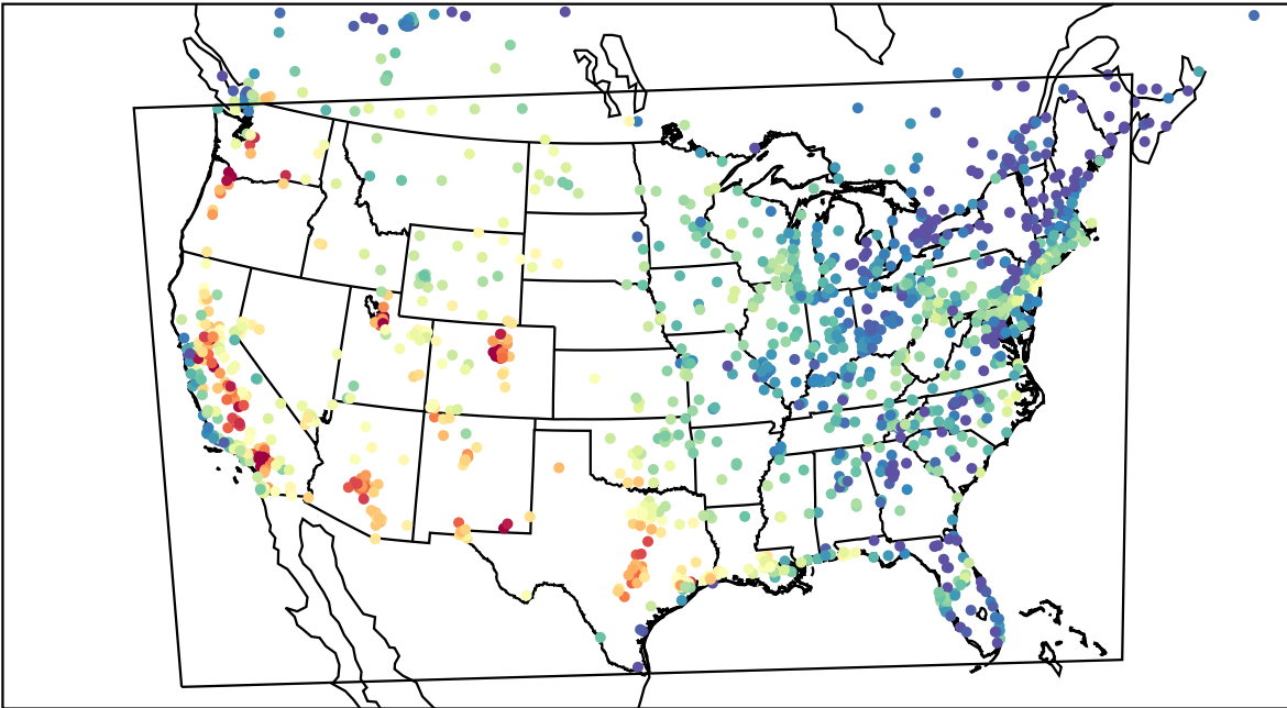
AirNOW (2023-08-16_00:00:00)
