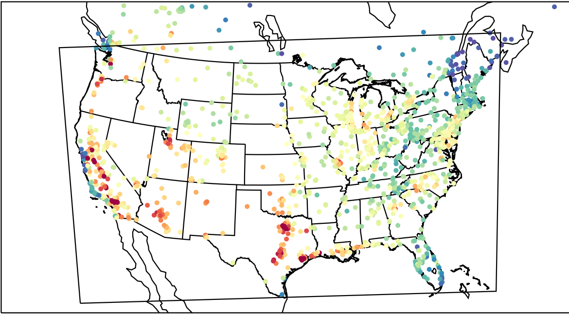
AirNOW (2023-08-16_21:00:00)
