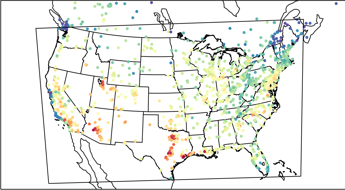
AirNOW (2023-08-16_18:00:00)
