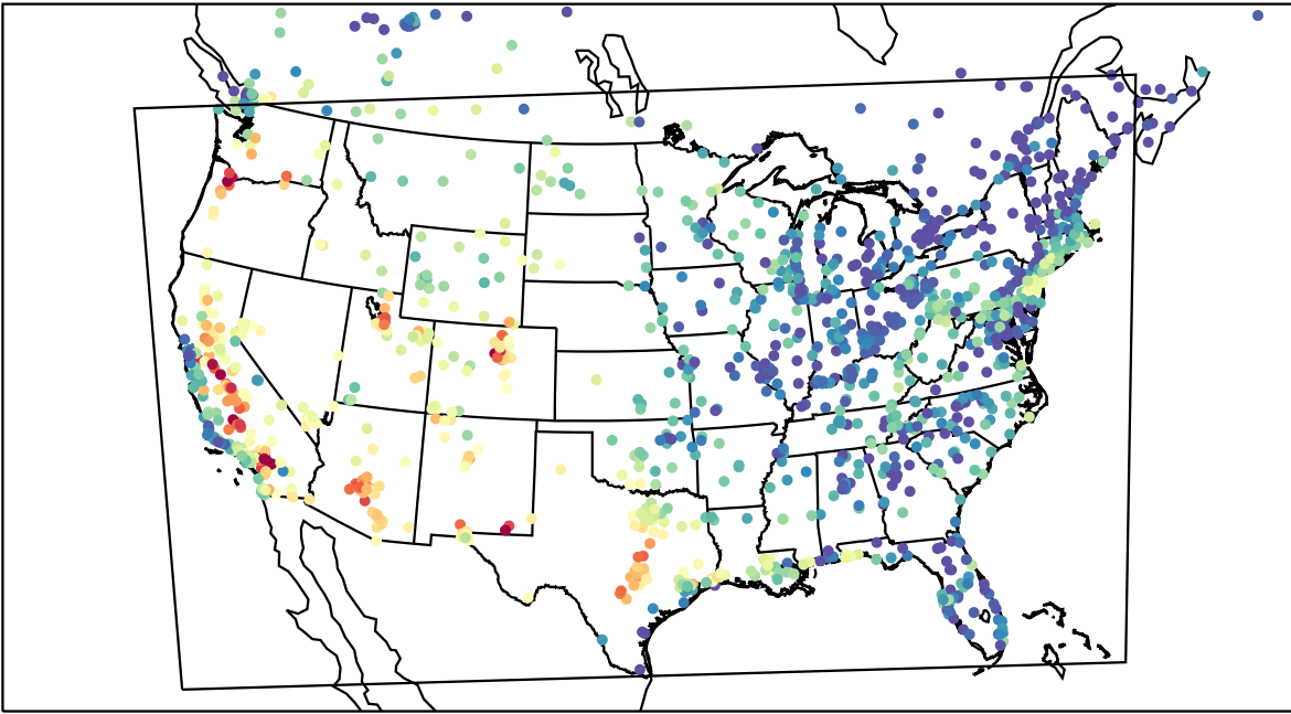
AirNOW (2023-08-16_01:00:00)
