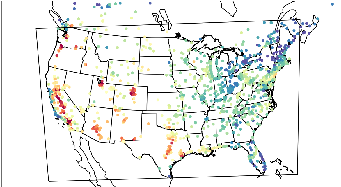
AirNOW (2023-08-15_22:00:00)
