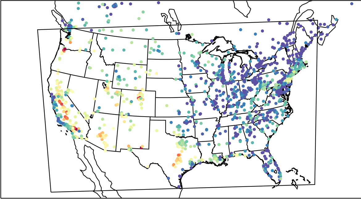
AirNOW (2023-08-16_02:00:00)
