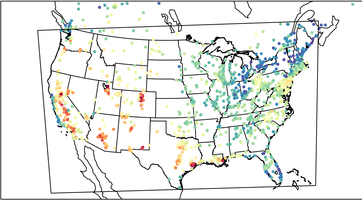
AirNOW (2023-08-15_19:00:00)
