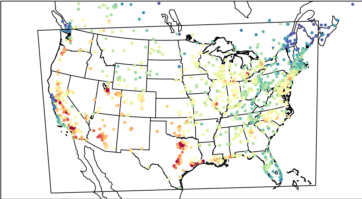
AirNOW (2023-08-16_20:00:00)
