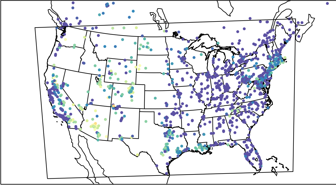
AirNOW (2023-08-16_10:00:00)
