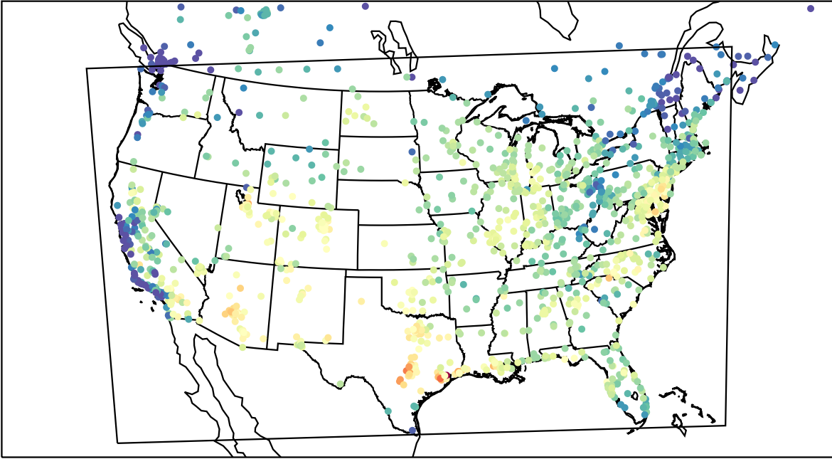
AirNOW (2023-08-16_16:00:00)
