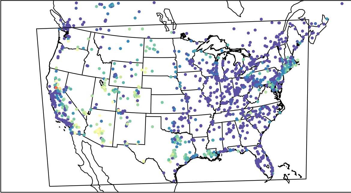
AirNOW (2023-08-16_09:00:00)
