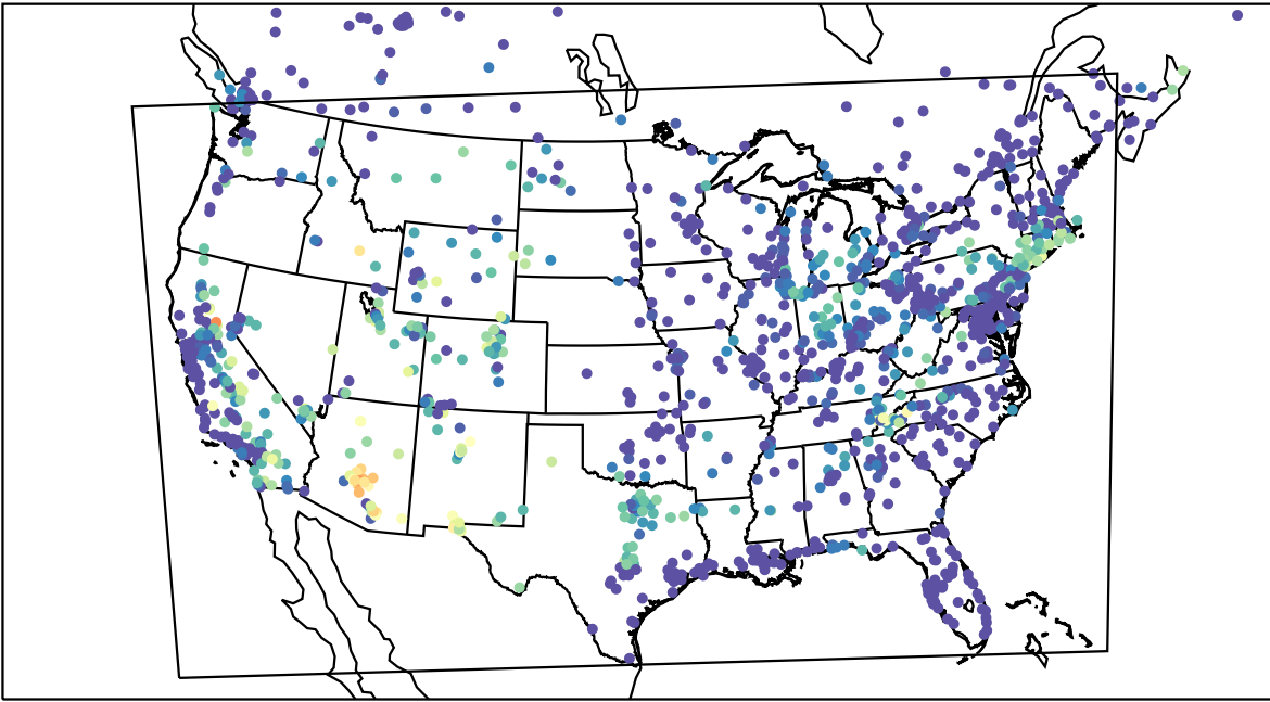
AirNOW (2023-08-15_09:00:00)
