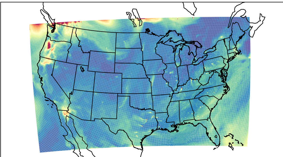
WRF 2023-08-16_17:00:00
