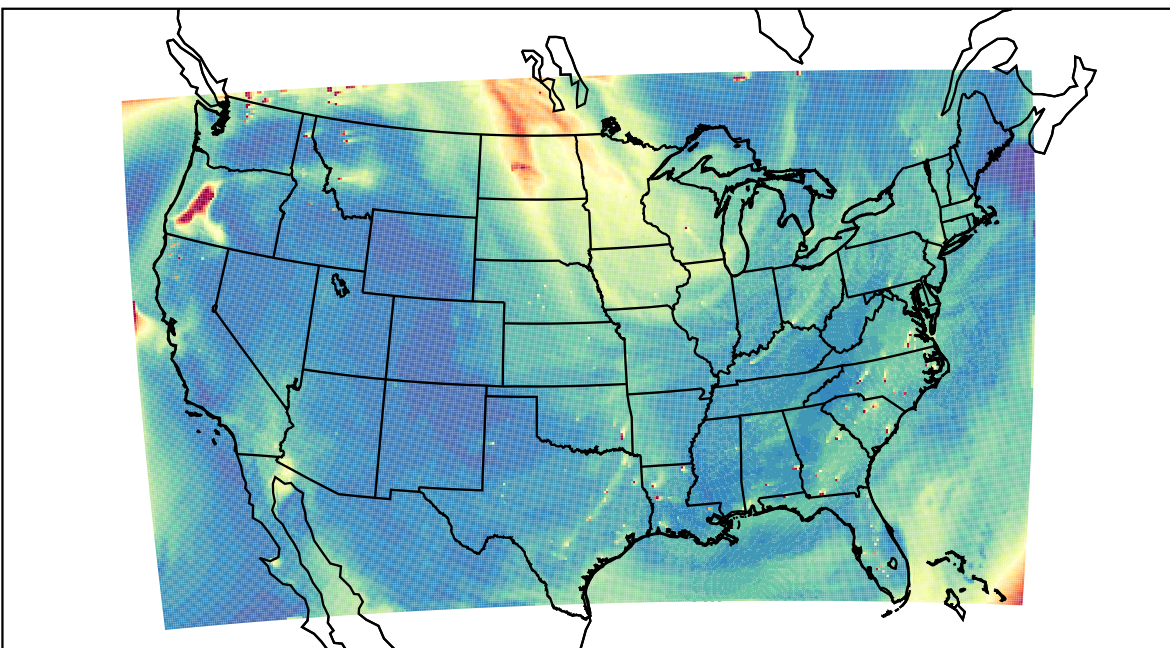
WRF 2023-08-17_21:00:00
