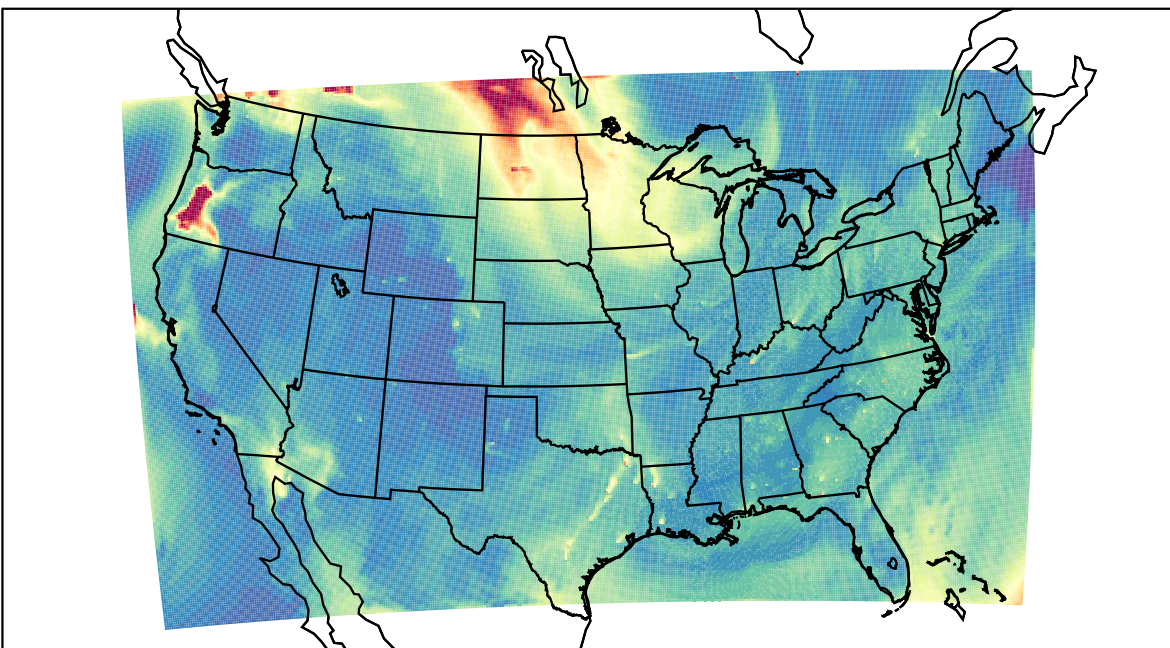
WRF 2023-08-17_17:00:00
