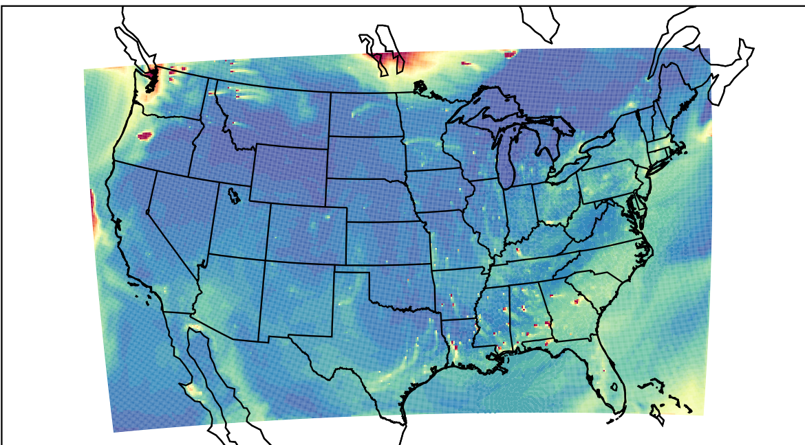
WRF 2023-08-16_00:00:00
