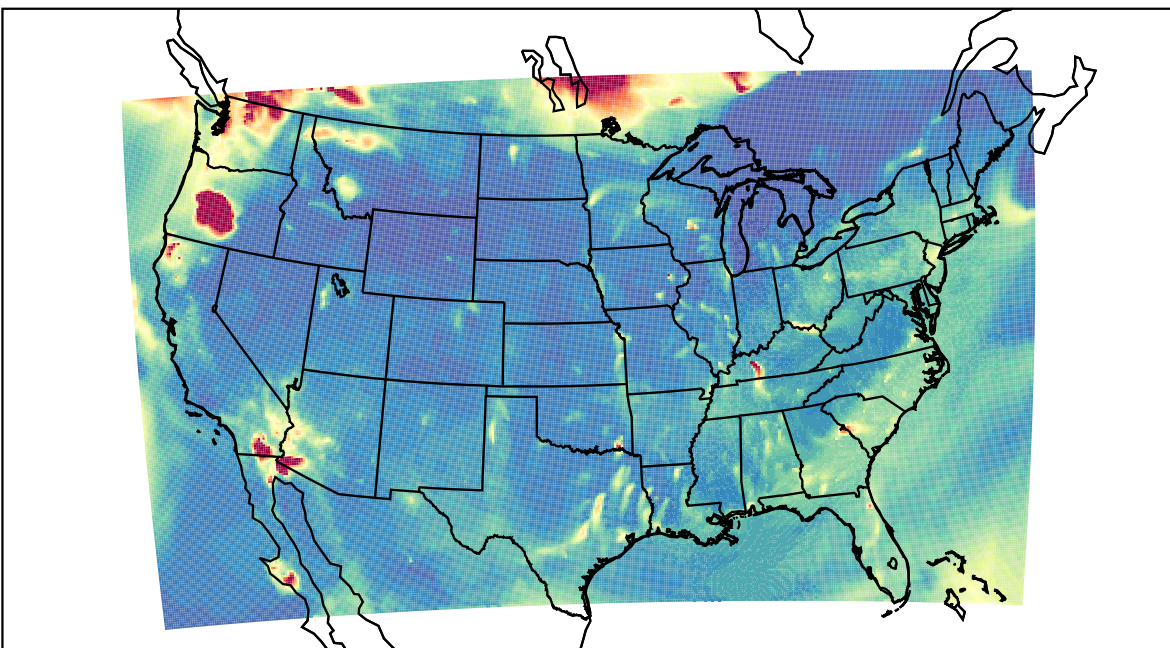
WRF 2023-08-16_05:00:00
