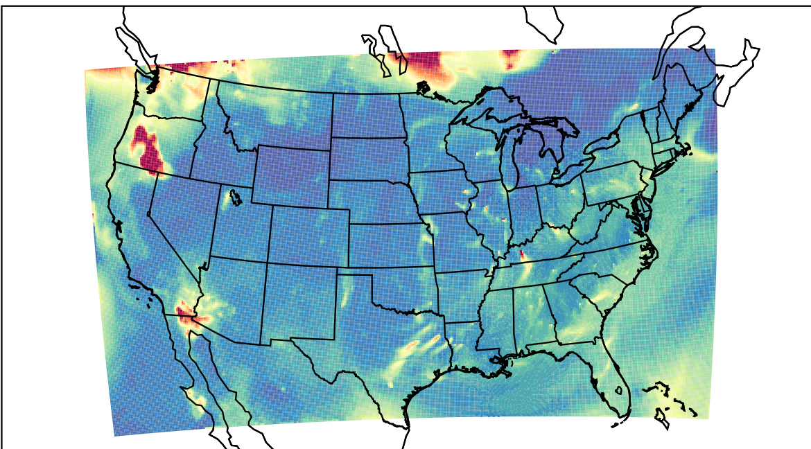
WRF 2023-08-16_09:00:00
