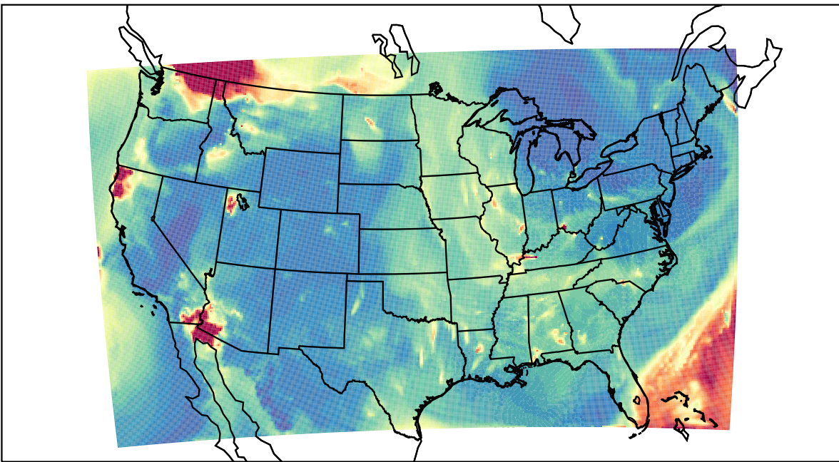
WRF 2023-08-19_06:00:00
