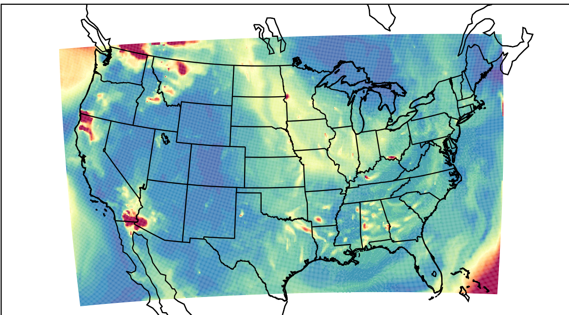
WRF 2023-08-18_06:00:00
