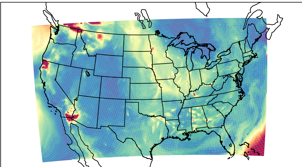
WRF 2023-08-18_08:00:00
