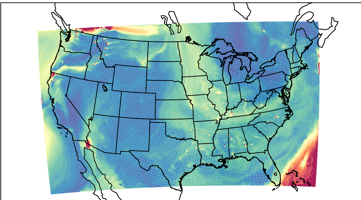
WRF 2023-08-18_21:00:00
