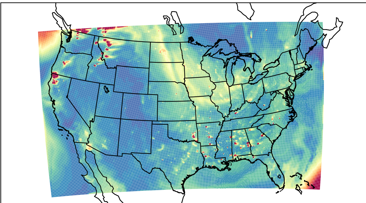
WRF 2023-08-18_01:00:00
