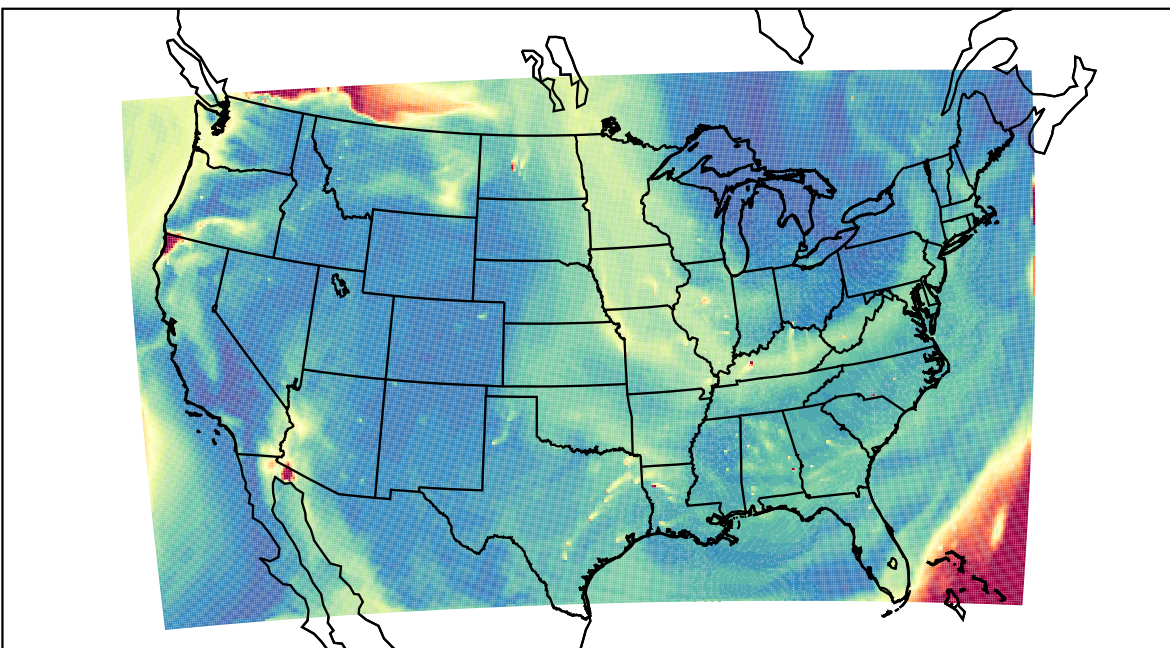
WRF 2023-08-18_17:00:00
