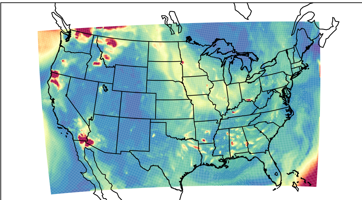
WRF 2023-08-18_05:00:00
