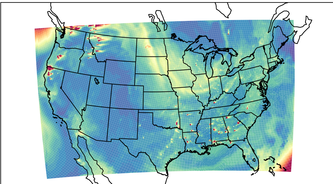
WRF 2023-08-18_00:00:00
