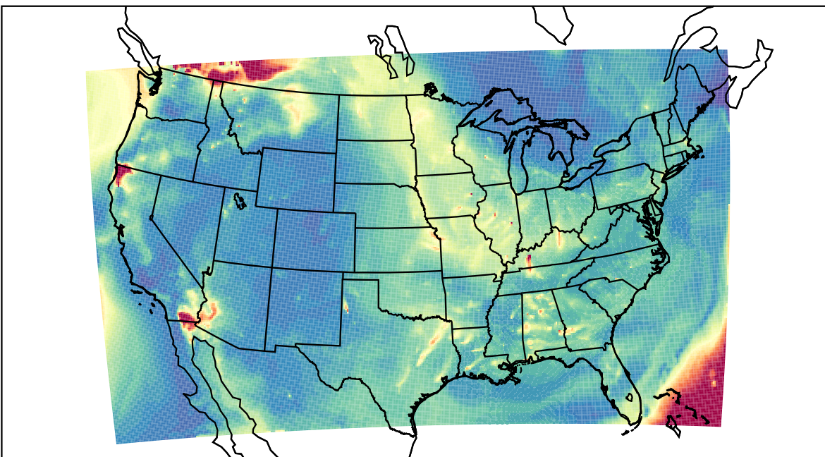
WRF 2023-08-18_12:00:00
