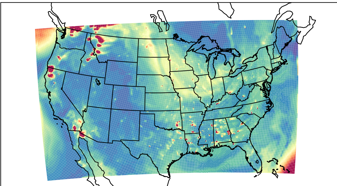
WRF 2023-08-18_02:00:00
