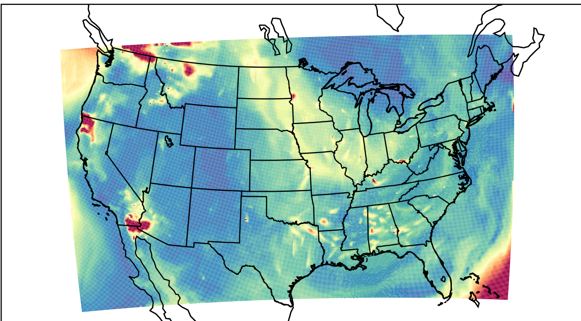
WRF 2023-08-18_07:00:00
