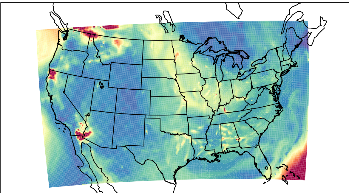
WRF 2023-08-18_09:00:00
