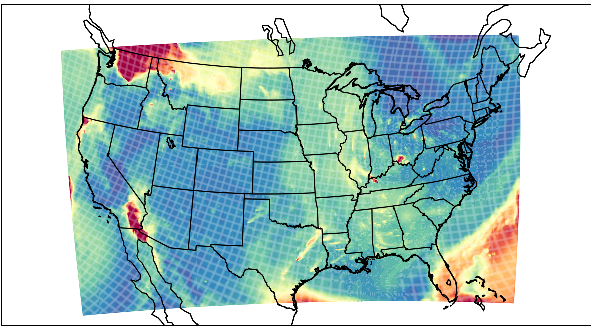
WRF 2023-08-19_13:00:00
