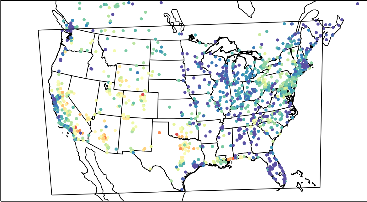
AirNOW (2023-08-18_03:00:00)
