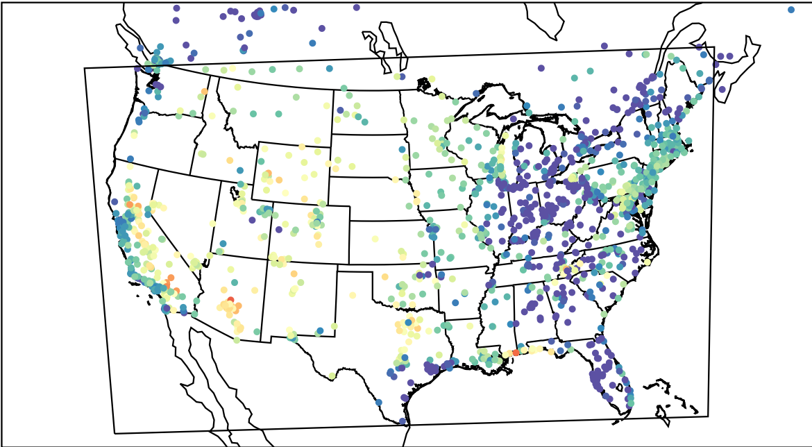
AirNOW (2023-08-19_03:00:00)
