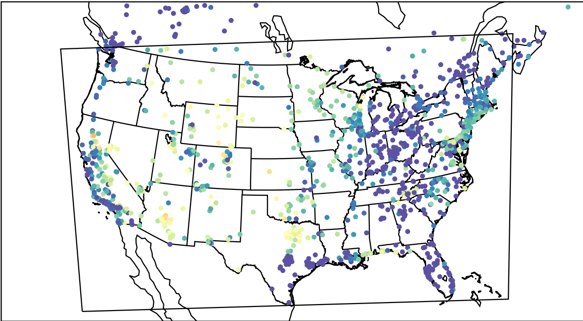
AirNOW (2023-08-19_06:00:00)
