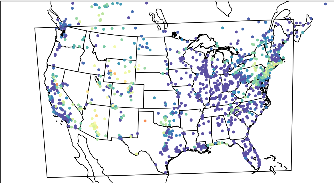
AirNOW (2023-08-18_11:00:00)
