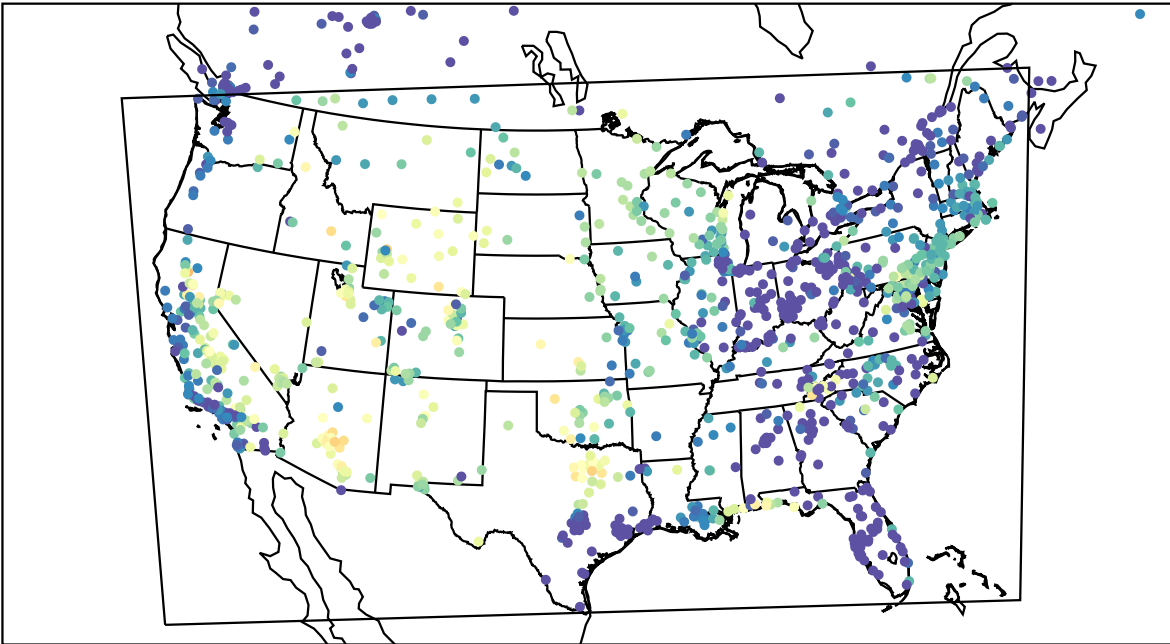
AirNOW (2023-08-19_05:00:00)
