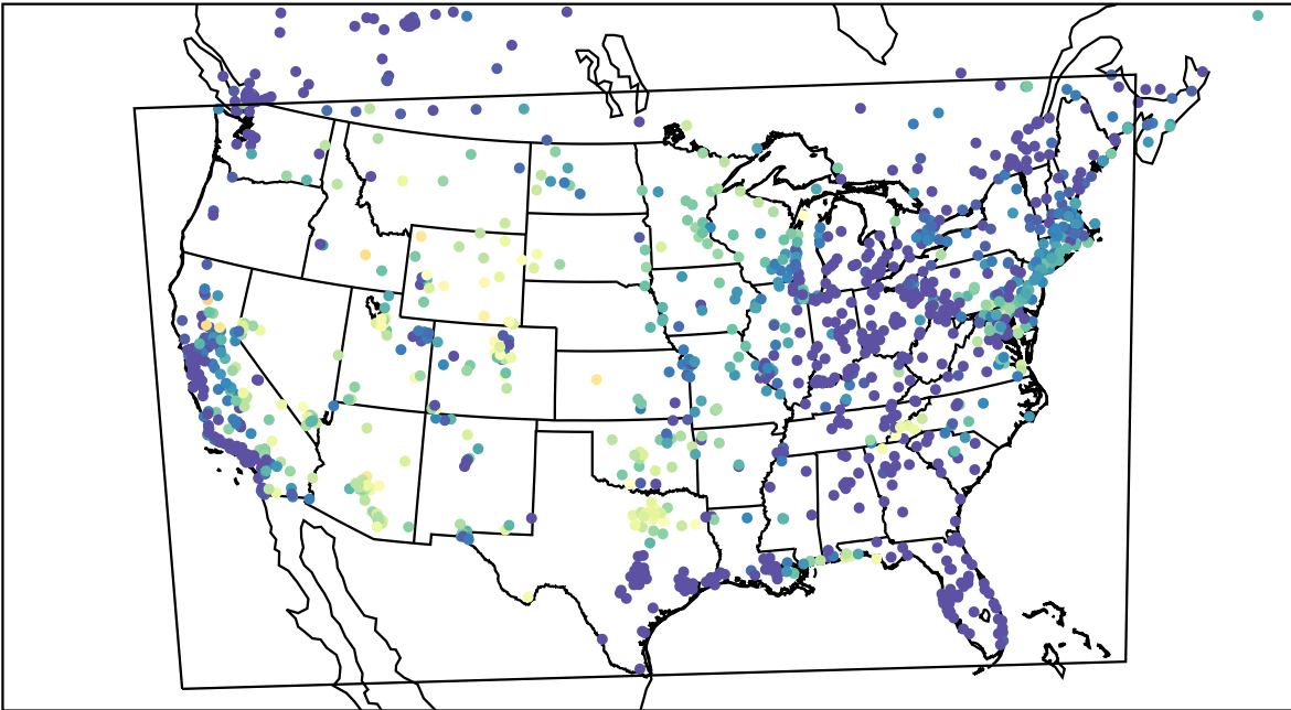
AirNOW (2023-08-19_08:00:00)
