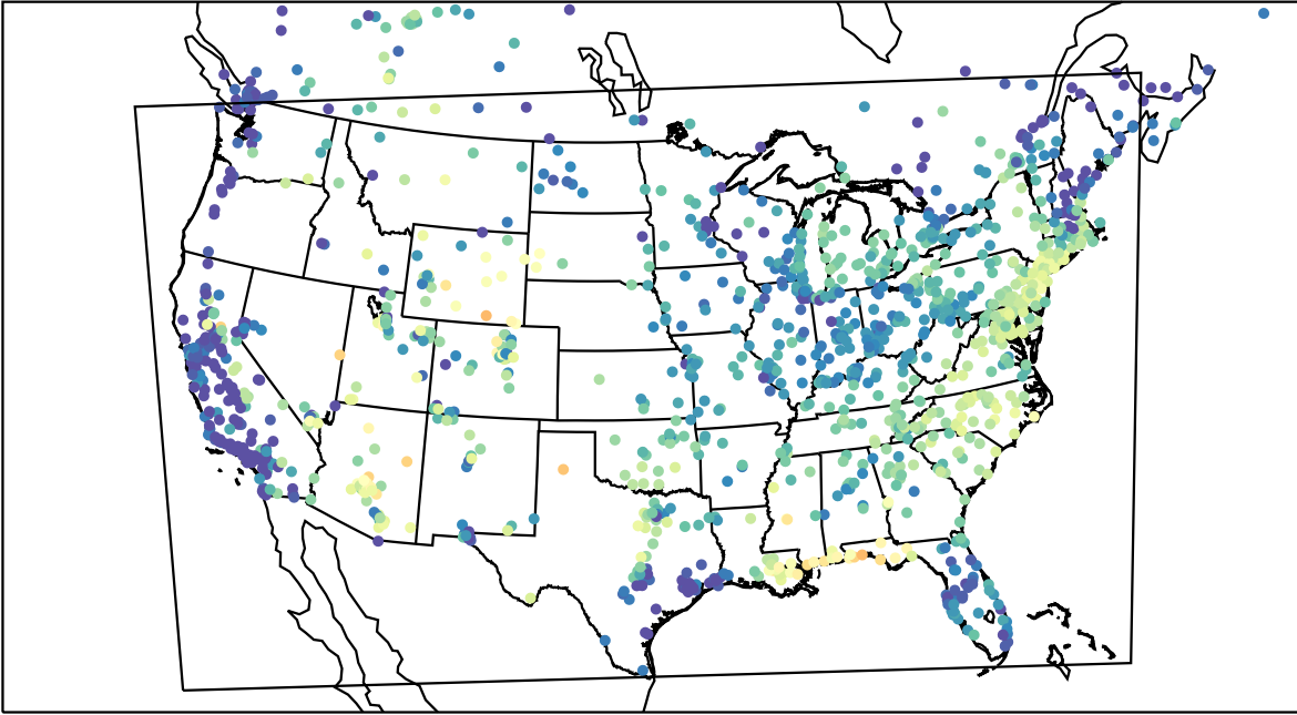
AirNOW (2023-08-18_14:00:00)
