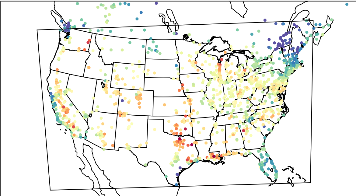
AirNOW (2023-08-19_22:00:00)
