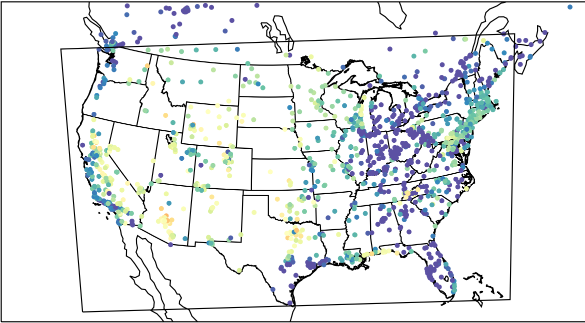
AirNOW (2023-08-19_04:00:00)
