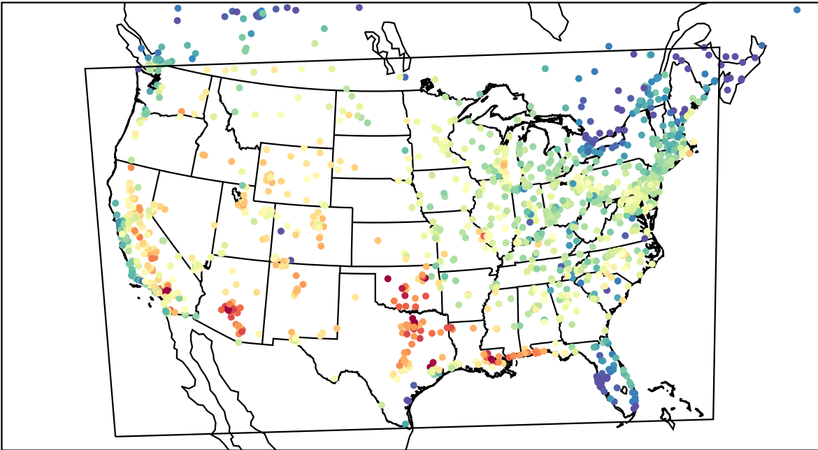
AirNOW (2023-08-18_23:00:00)
