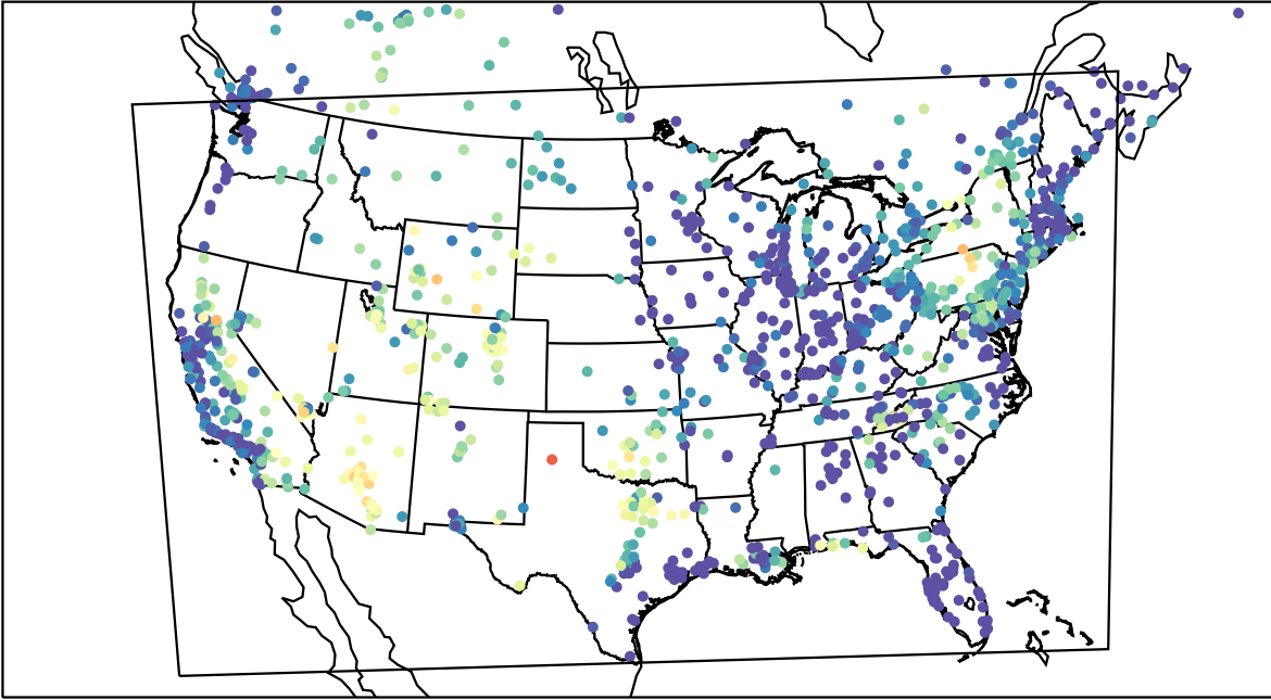
AirNOW (2023-08-18_07:00:00)
