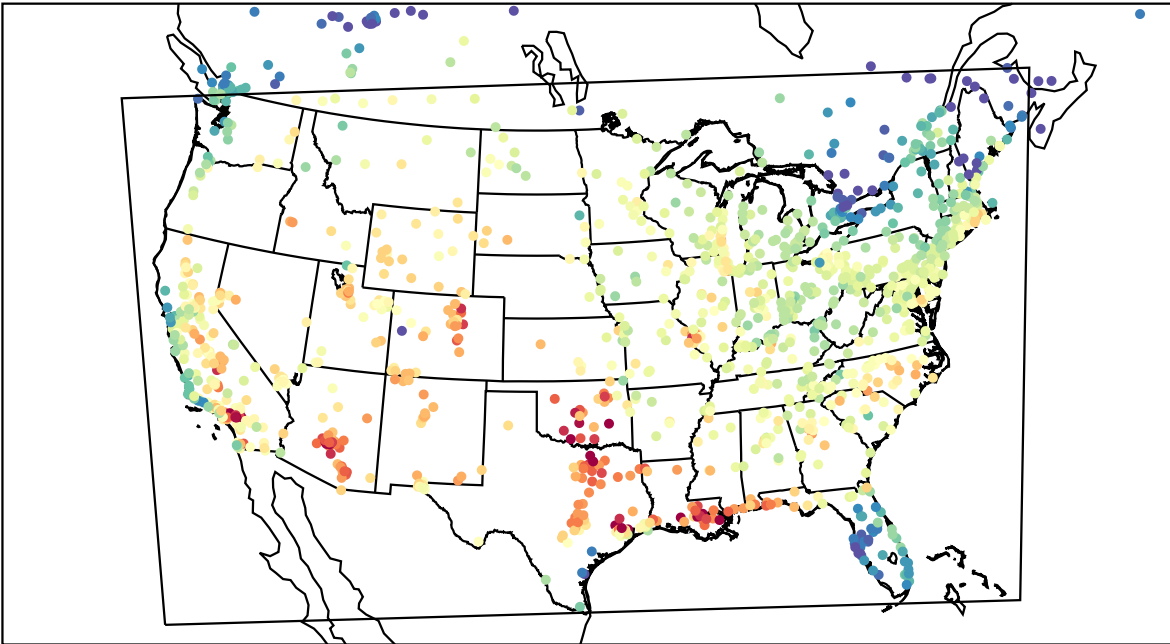
AirNOW (2023-08-18_21:00:00)
