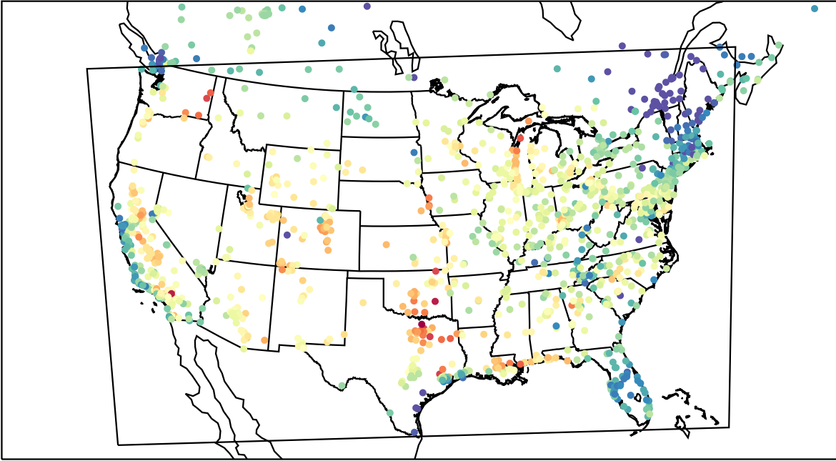
AirNOW (2023-08-19_23:00:00)
