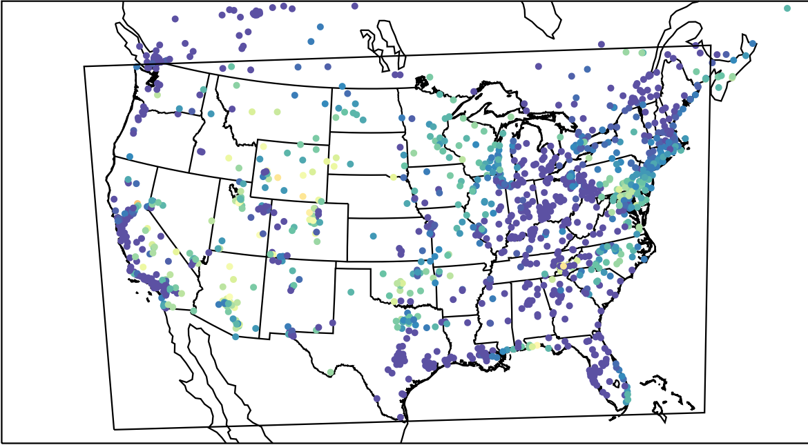
AirNOW (2023-08-19_12:00:00)
