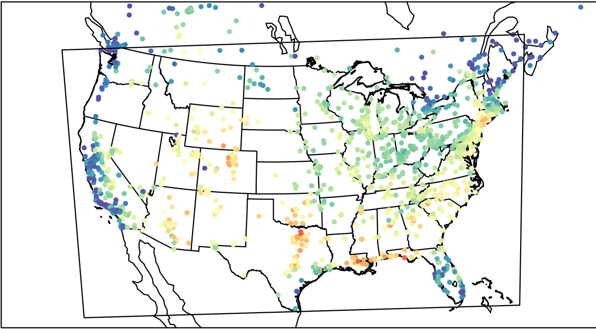
AirNOW (2023-08-18_16:00:00)
