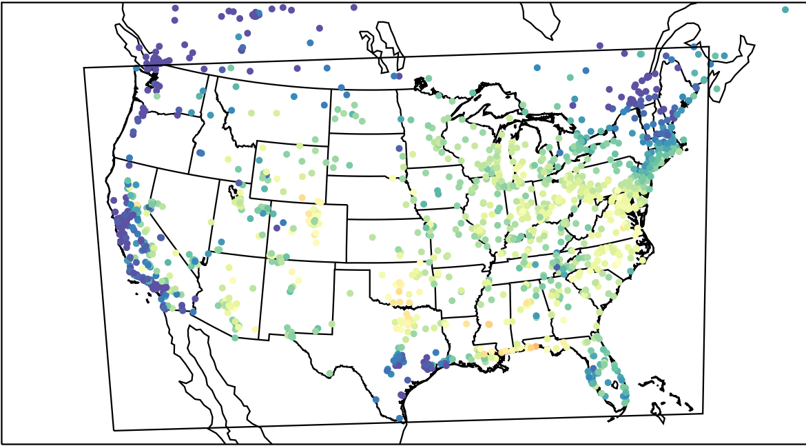
AirNOW (2023-08-19_15:00:00)
