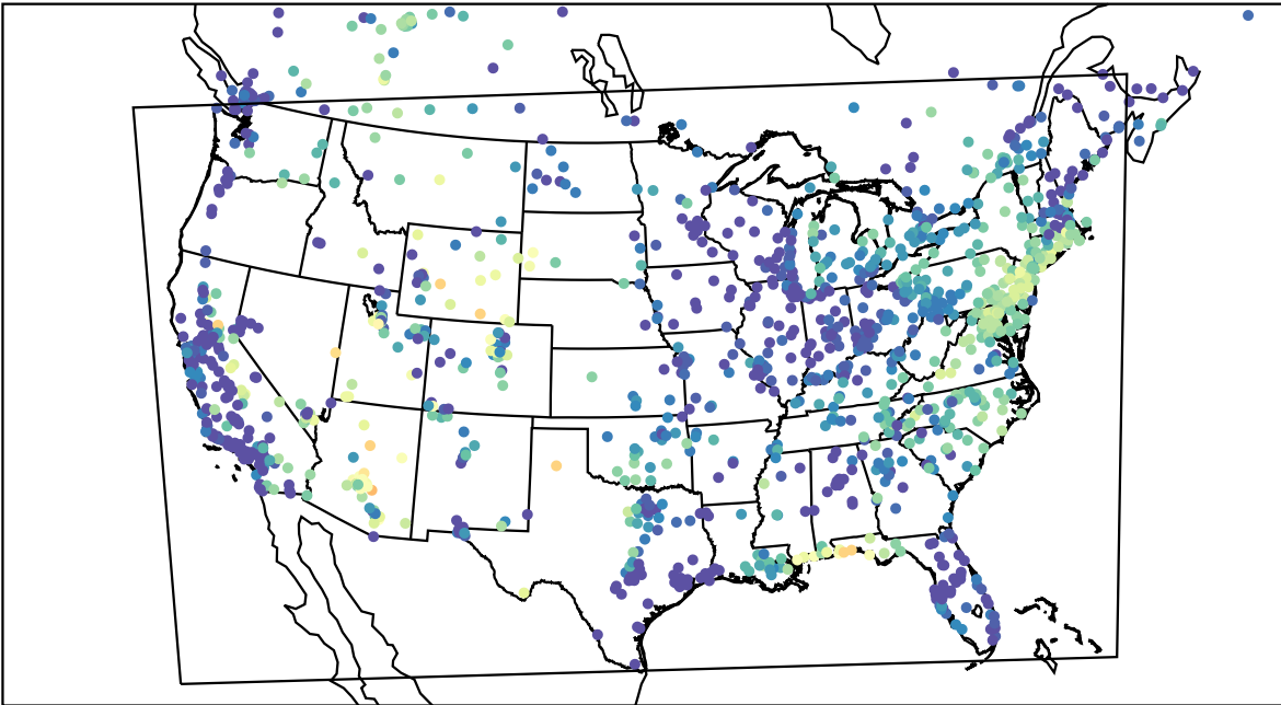
AirNOW (2023-08-18_13:00:00)
