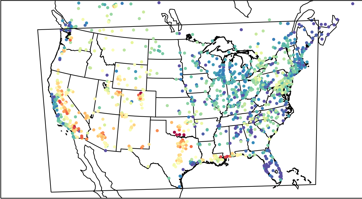
AirNOW (2023-08-18_01:00:00)
