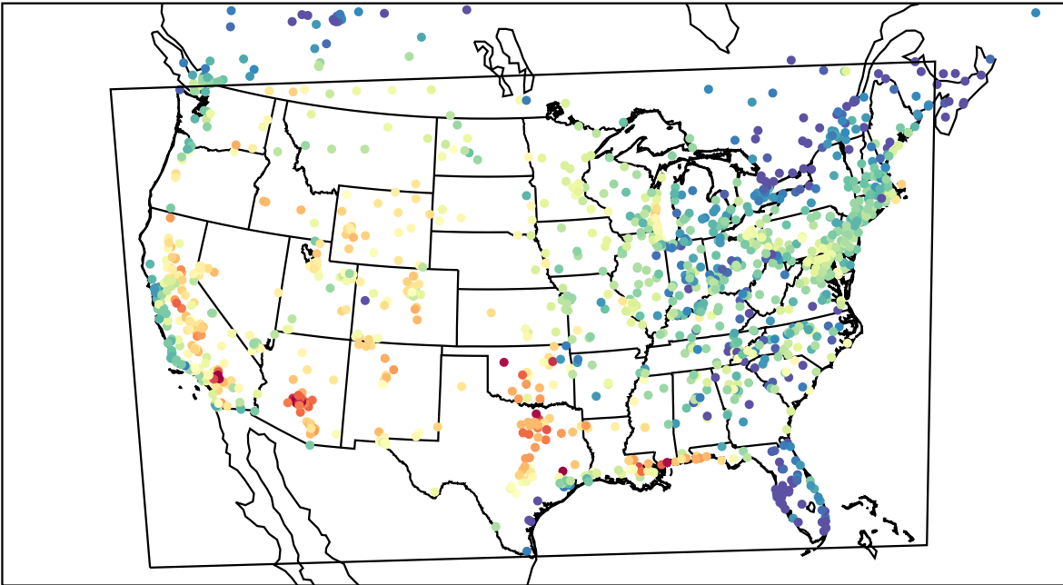
AirNOW (2023-08-19_00:00:00)
