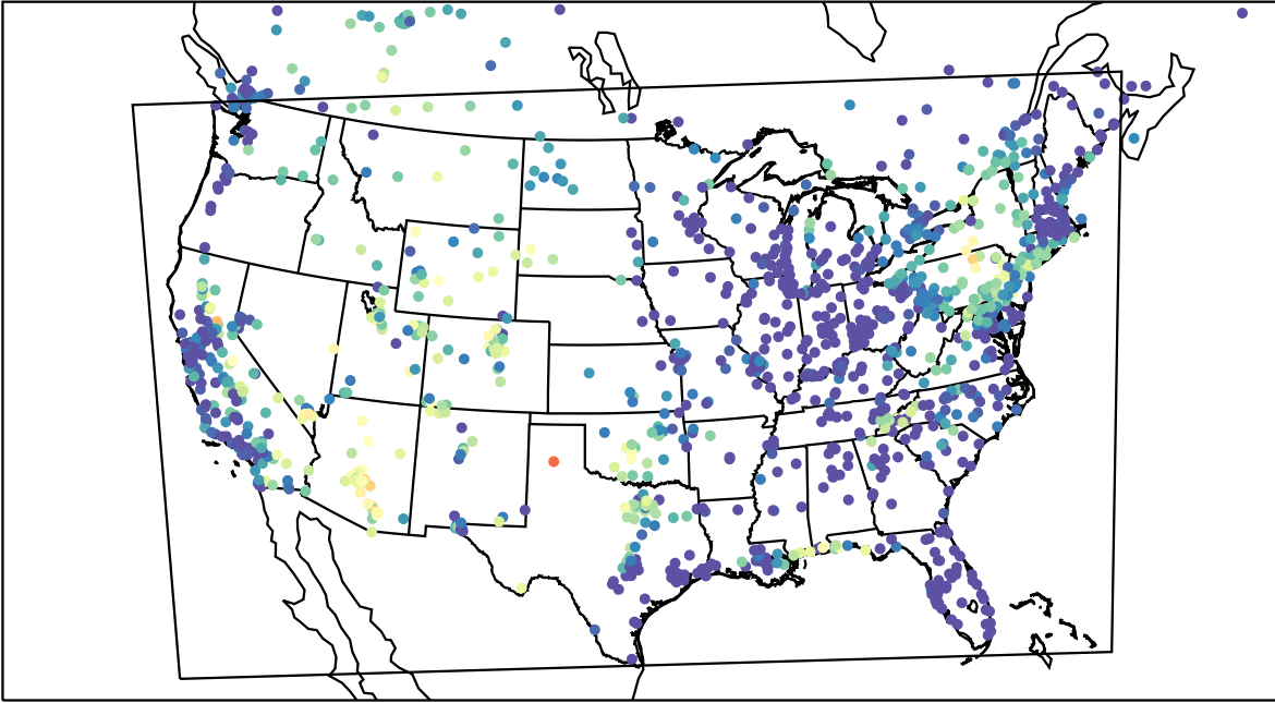
AirNOW (2023-08-18_09:00:00)
