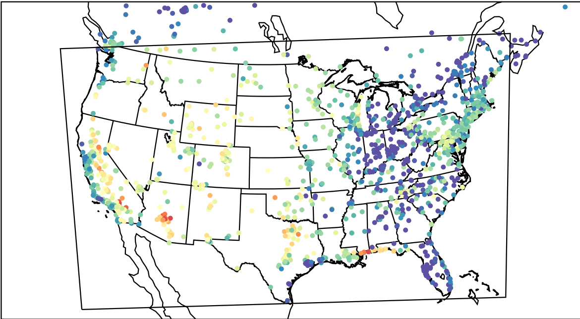
AirNOW (2023-08-19_02:00:00)
