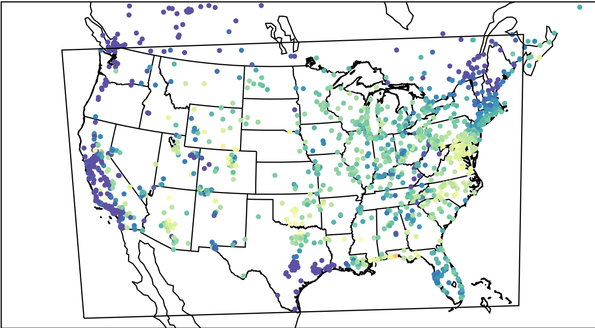
AirNOW (2023-08-19_14:00:00)
