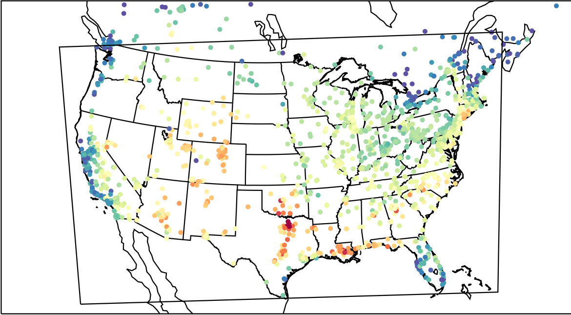
AirNOW (2023-08-18_17:00:00)
