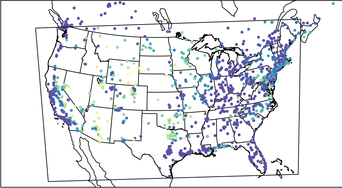
AirNOW (2023-08-19_10:00:00)
