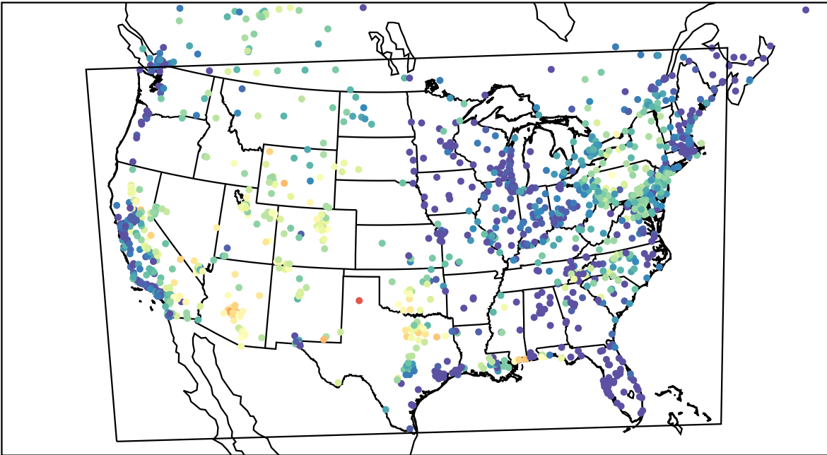
AirNOW (2023-08-18_05:00:00)
