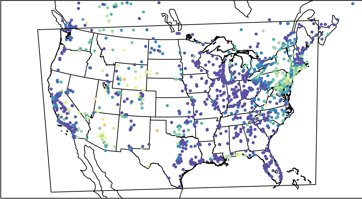
AirNOW (2023-08-18_12:00:00)
