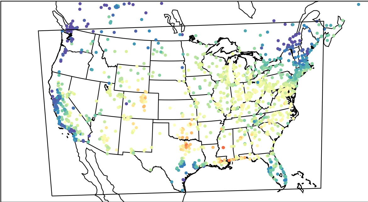
AirNOW (2023-08-19_16:00:00)
