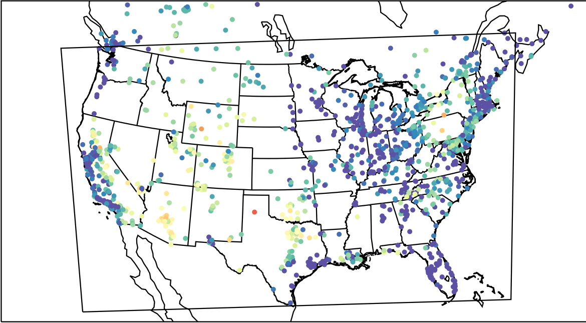
AirNOW (2023-08-18_06:00:00)
