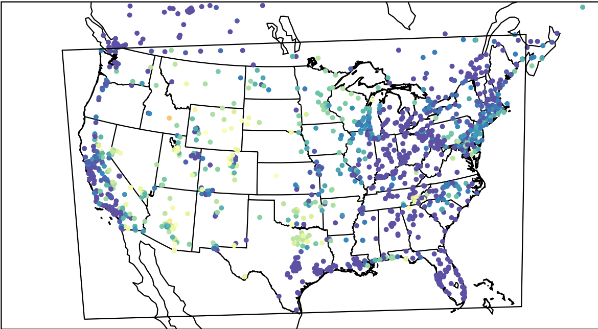
AirNOW (2023-08-19_09:00:00)
