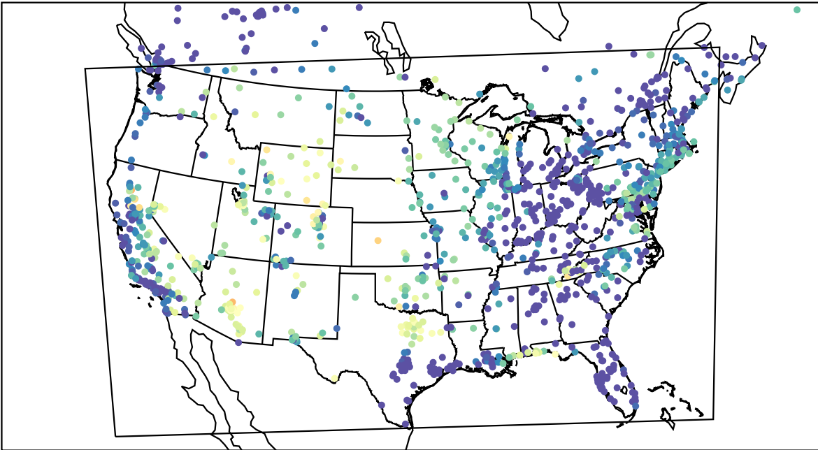
AirNOW (2023-08-19_07:00:00)
