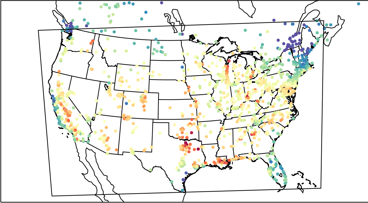
AirNOW (2023-08-19_21:00:00)
