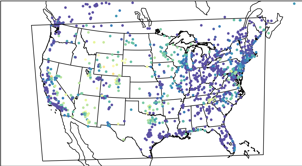
AirNOW (2023-08-19_11:00:00)
