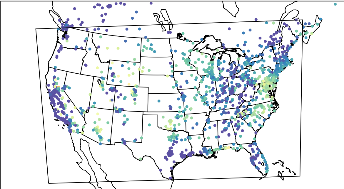
AirNOW (2023-08-19_13:00:00)
