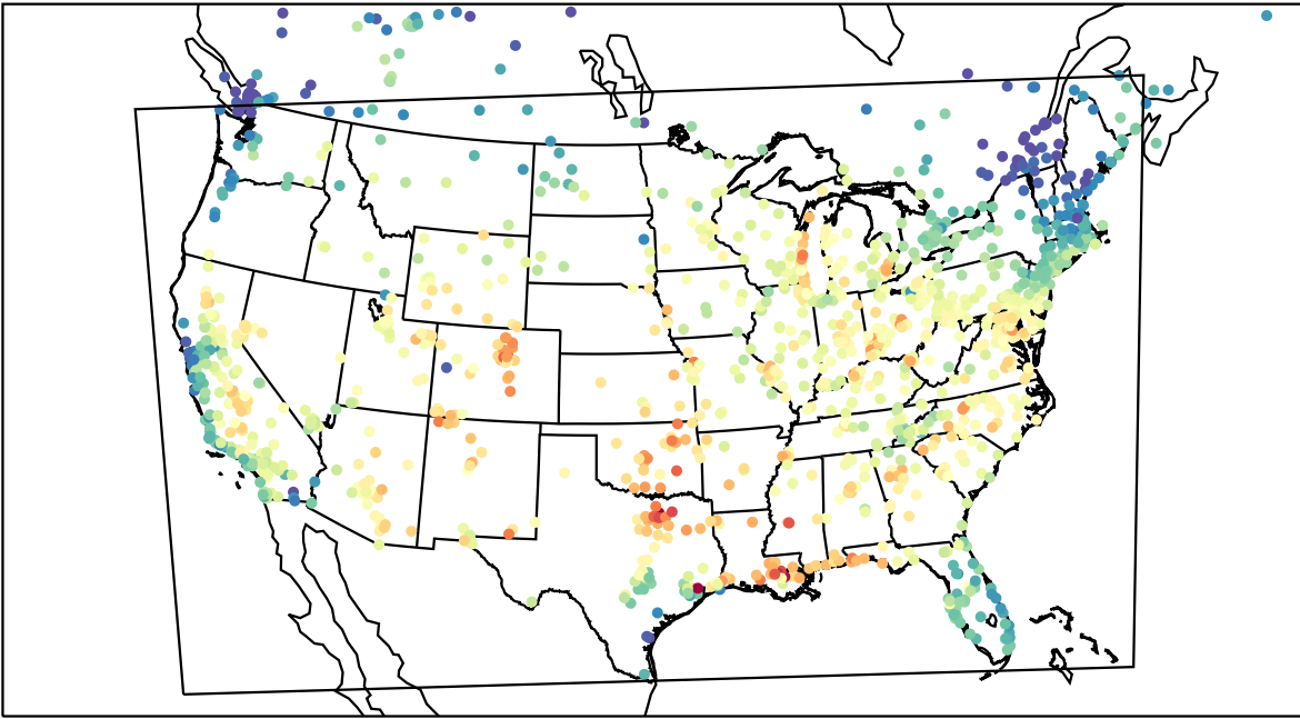
AirNOW (2023-08-19_18:00:00)
