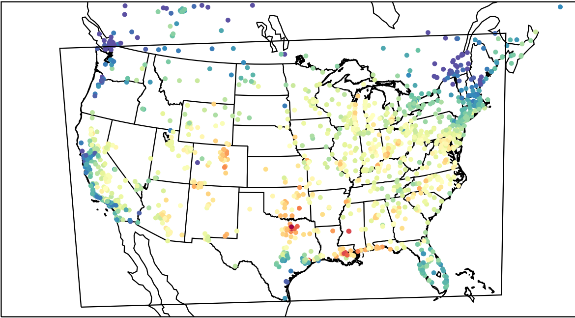
AirNOW (2023-08-19_17:00:00)
