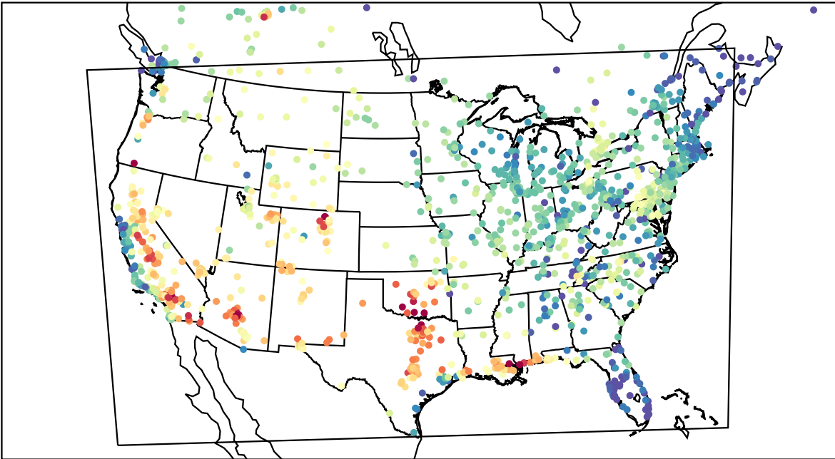
AirNOW (2023-08-18_00:00:00)
