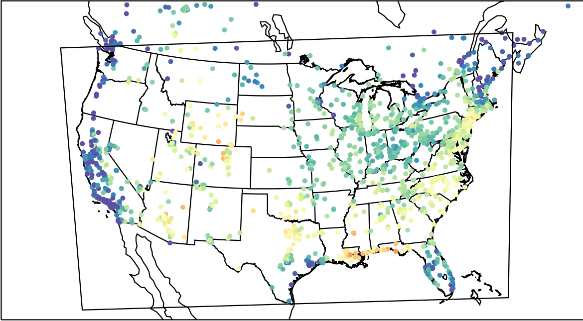
AirNOW (2023-08-18_15:00:00)
