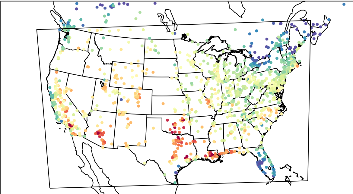
AirNOW (2023-08-18_22:00:00)
