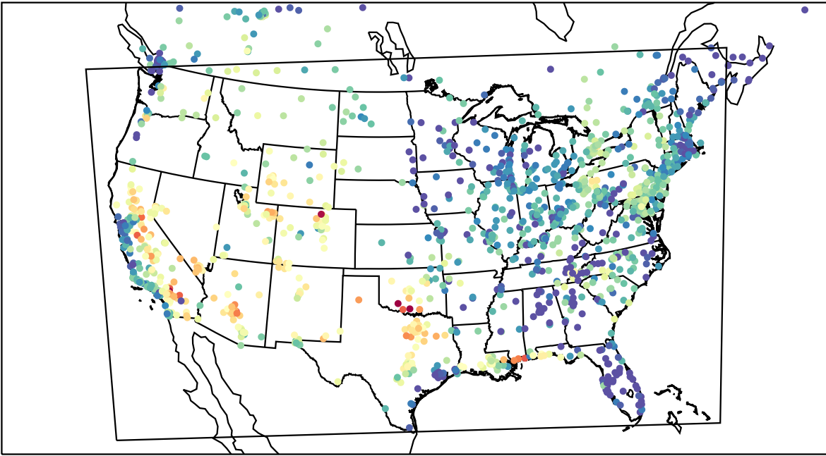
AirNOW (2023-08-18_02:00:00)
