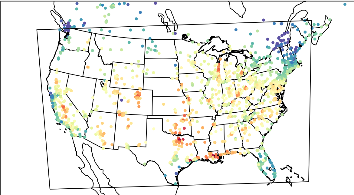
AirNOW (2023-08-19_19:00:00)
