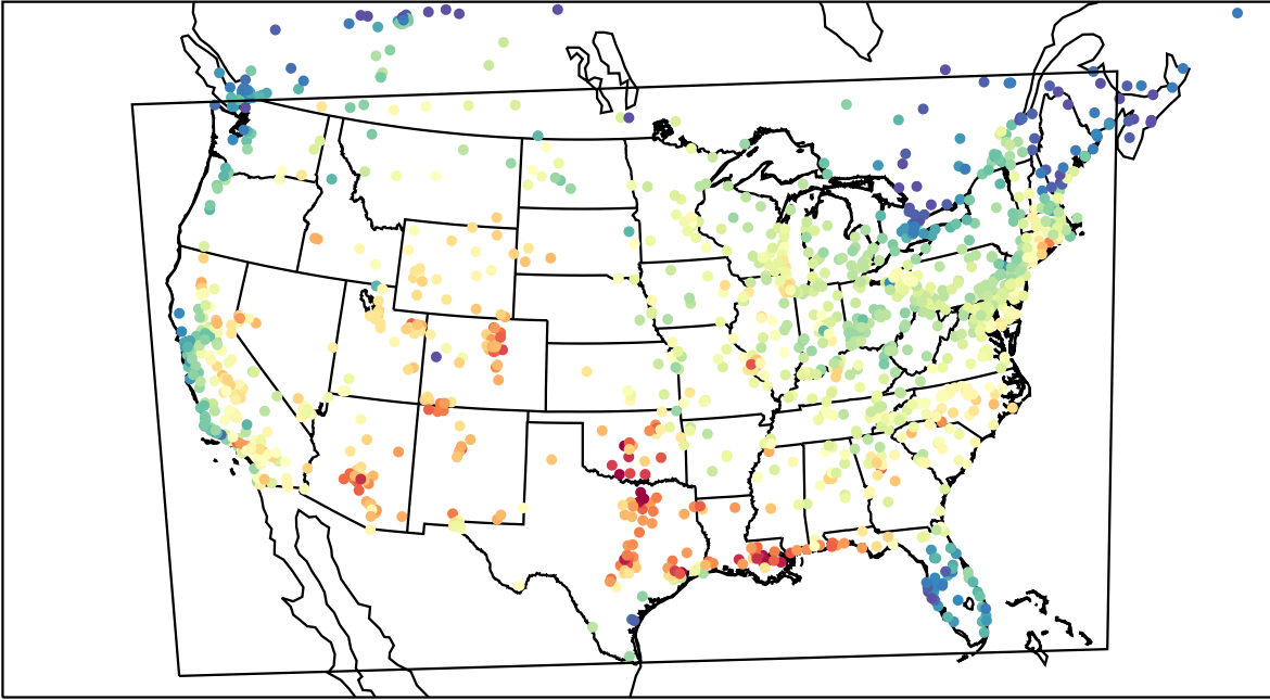
AirNOW (2023-08-18_19:00:00)
