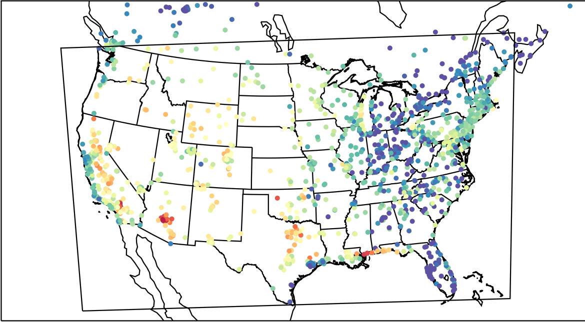
AirNOW (2023-08-19_01:00:00)
