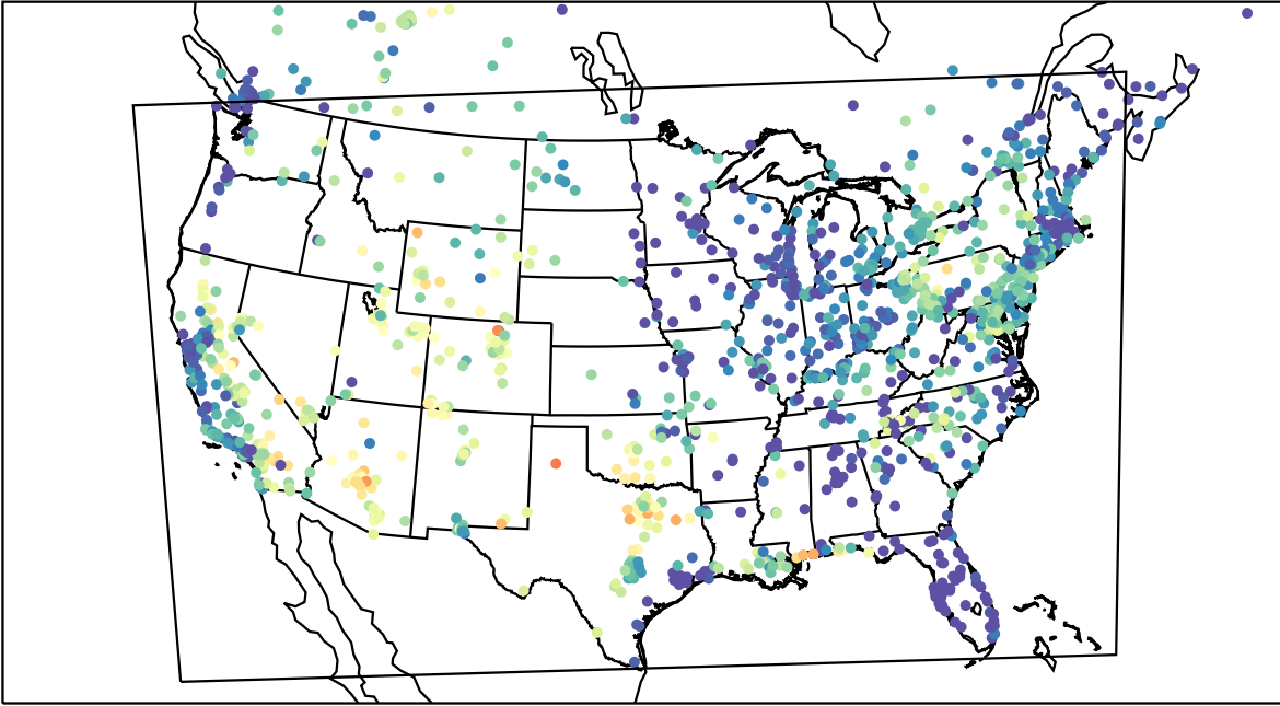
AirNOW (2023-08-18_04:00:00)
