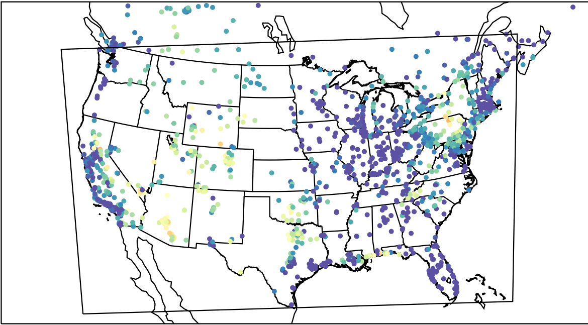
AirNOW (2023-08-18_08:00:00)
