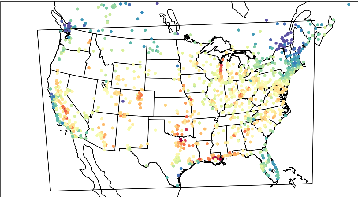
AirNOW (2023-08-19_20:00:00)
