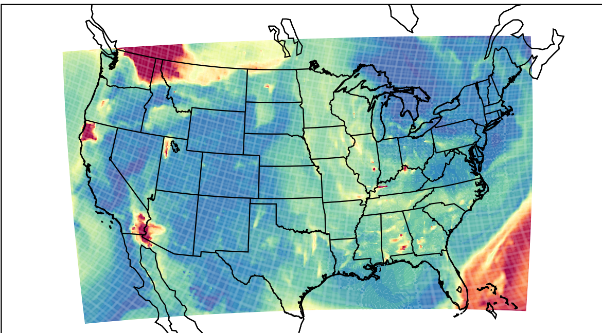
WRF 2023-08-19_07:00:00
