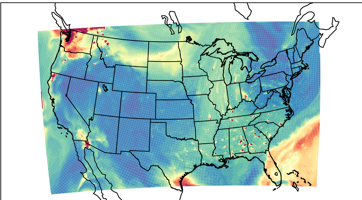
WRF 2023-08-19_23:00:00
