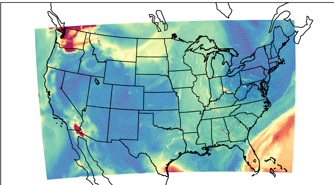
WRF 2023-08-19_19:00:00
