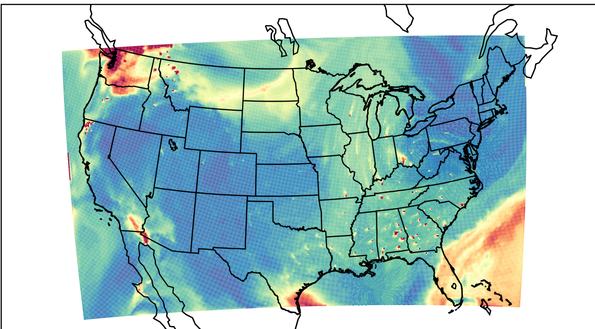
WRF 2023-08-19_22:00:00
