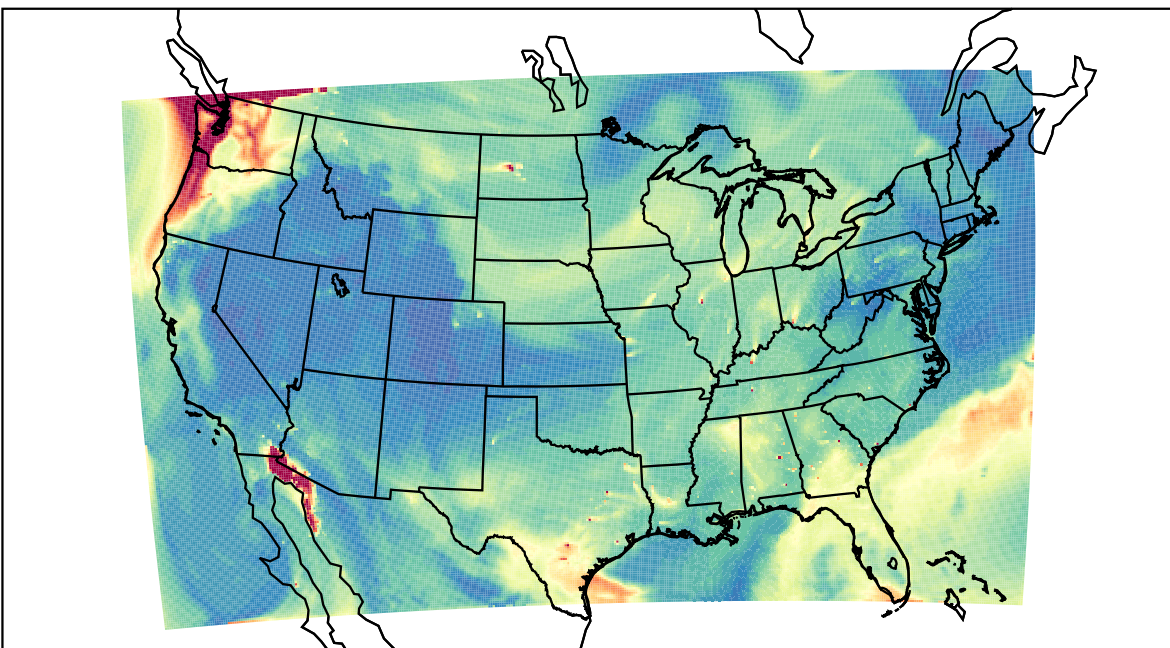
WRF 2023-08-20_17:00:00
