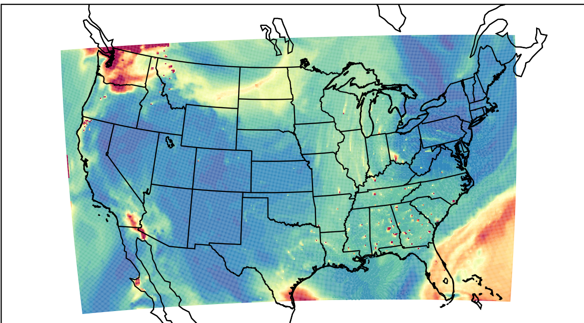
WRF 2023-08-19_21:00:00
