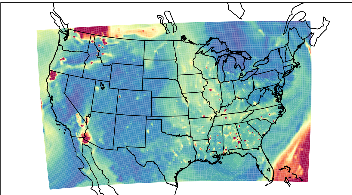
WRF 2023-08-19_02:00:00
