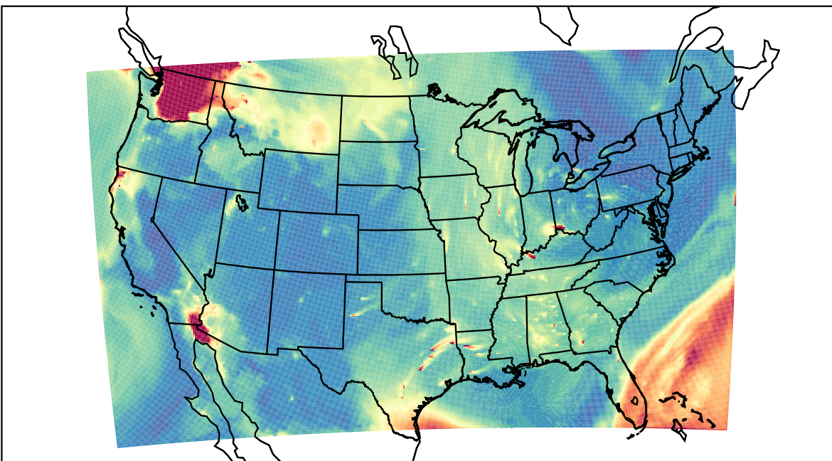
WRF 2023-08-19_14:00:00
