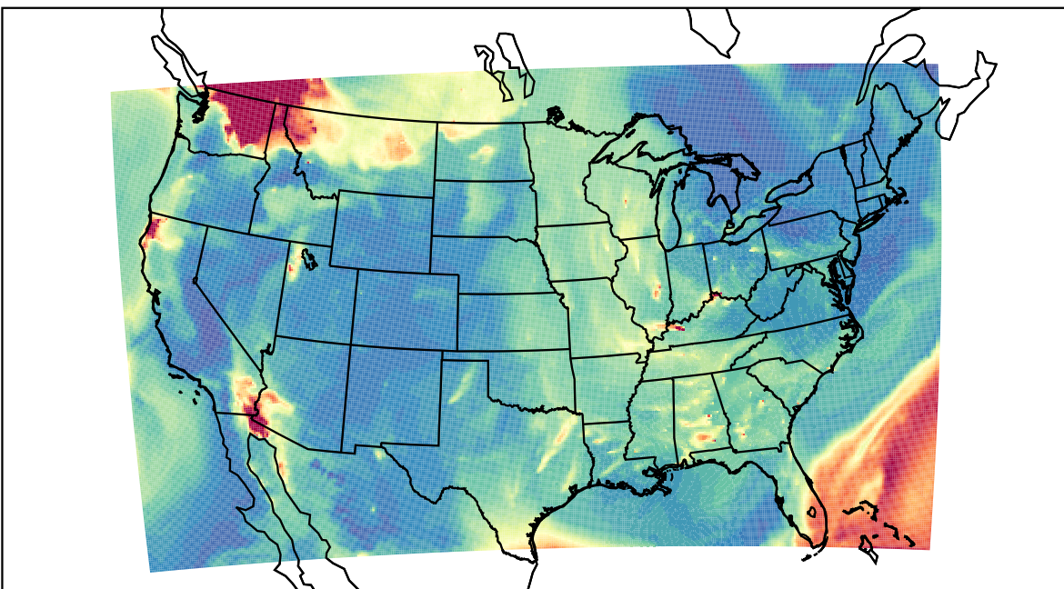
WRF 2023-08-19_10:00:00
