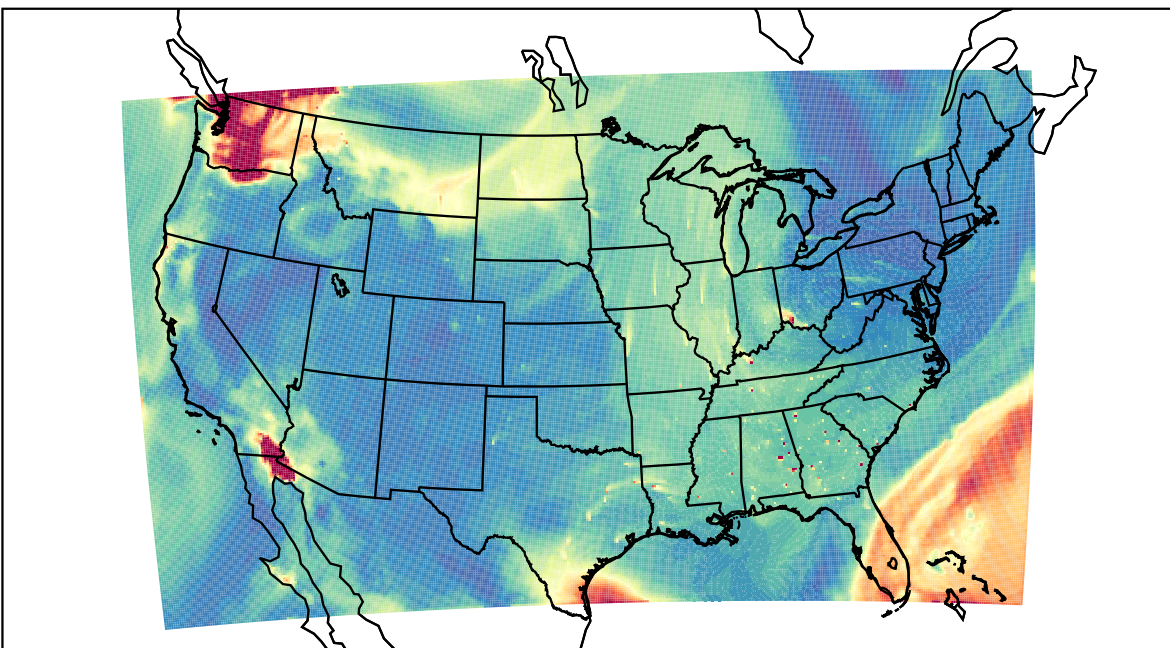
WRF 2023-08-19_18:00:00
