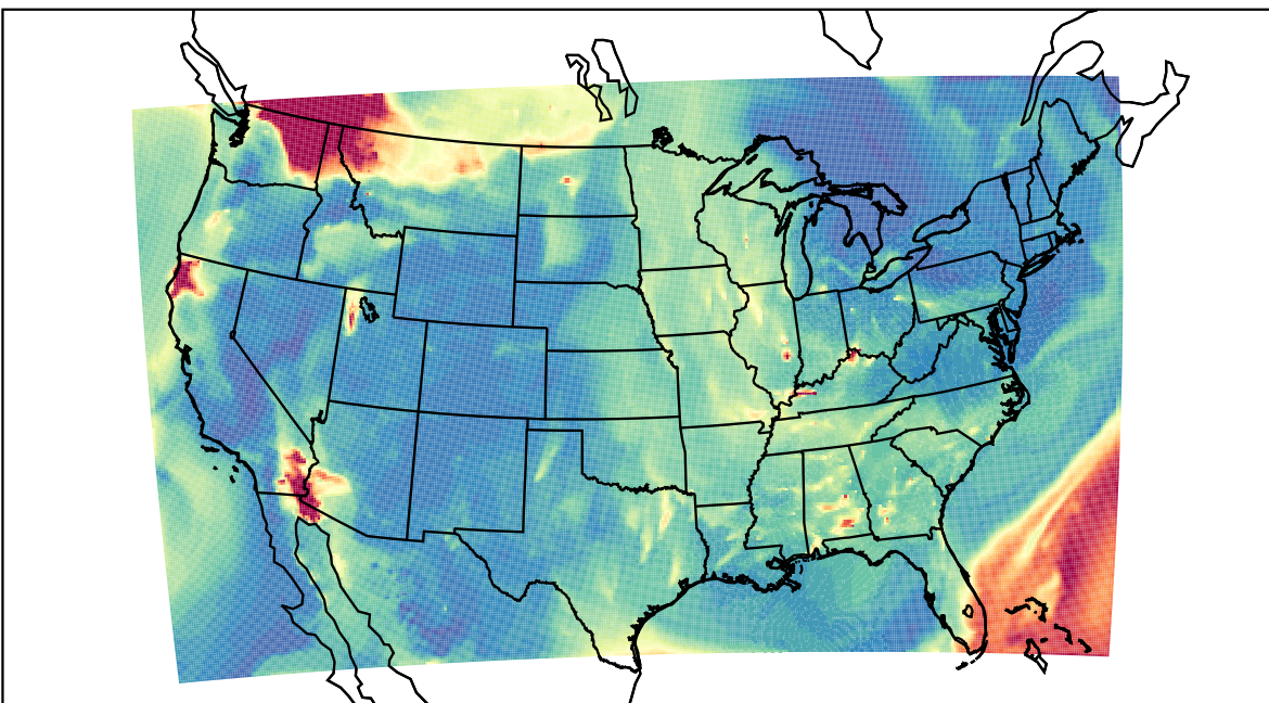
WRF 2023-08-19_08:00:00
