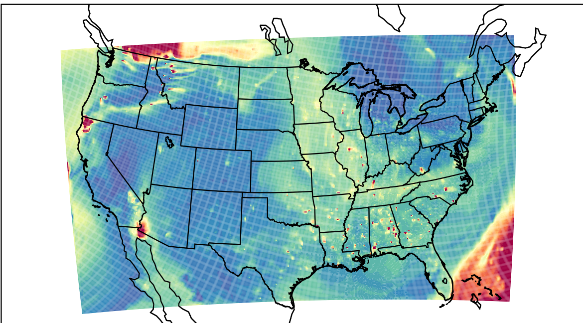
WRF 2023-08-19_01:00:00
