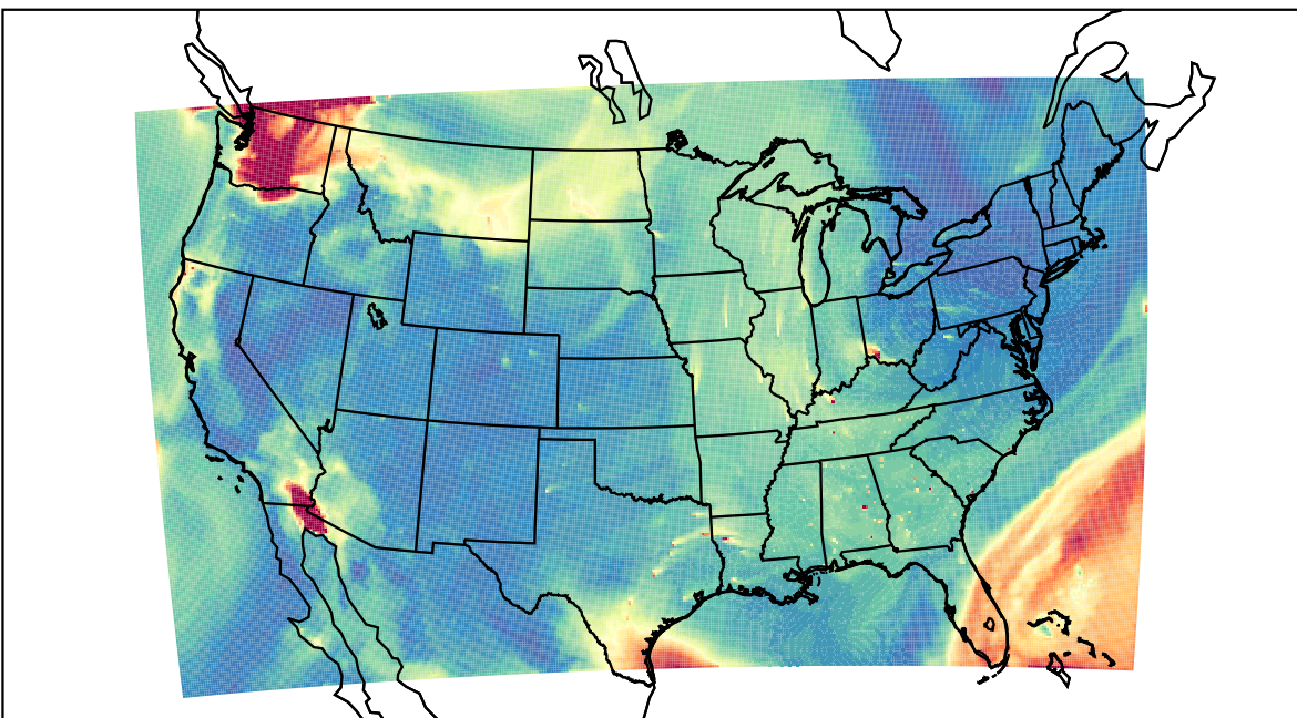
WRF 2023-08-19_17:00:00
