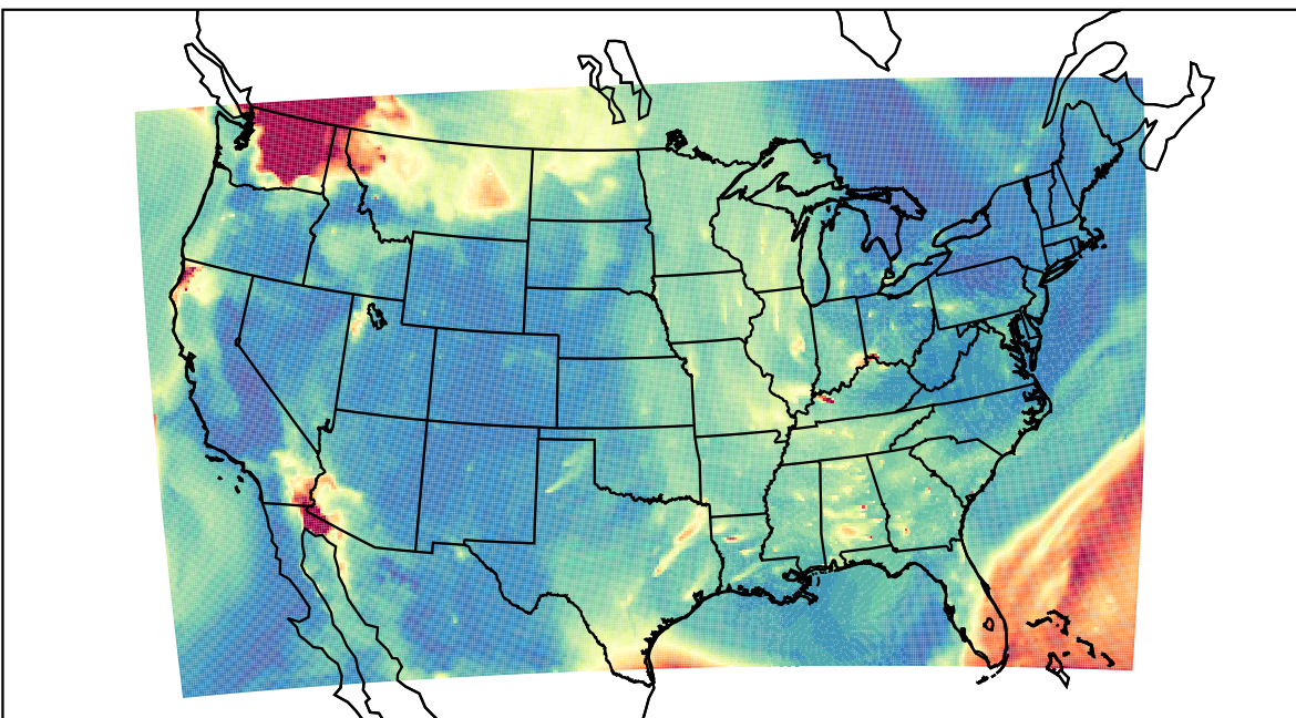
WRF 2023-08-19_12:00:00
