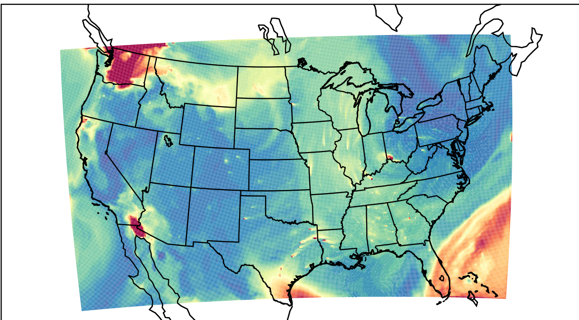
WRF 2023-08-19_16:00:00
