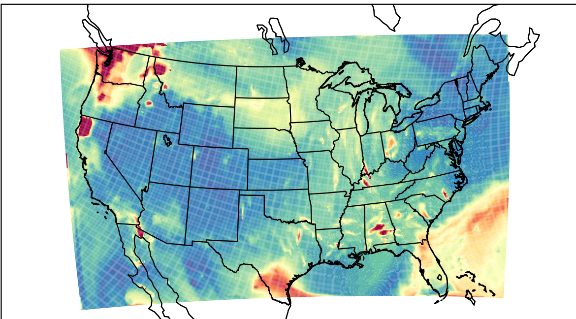
WRF 2023-08-20_05:00:00
