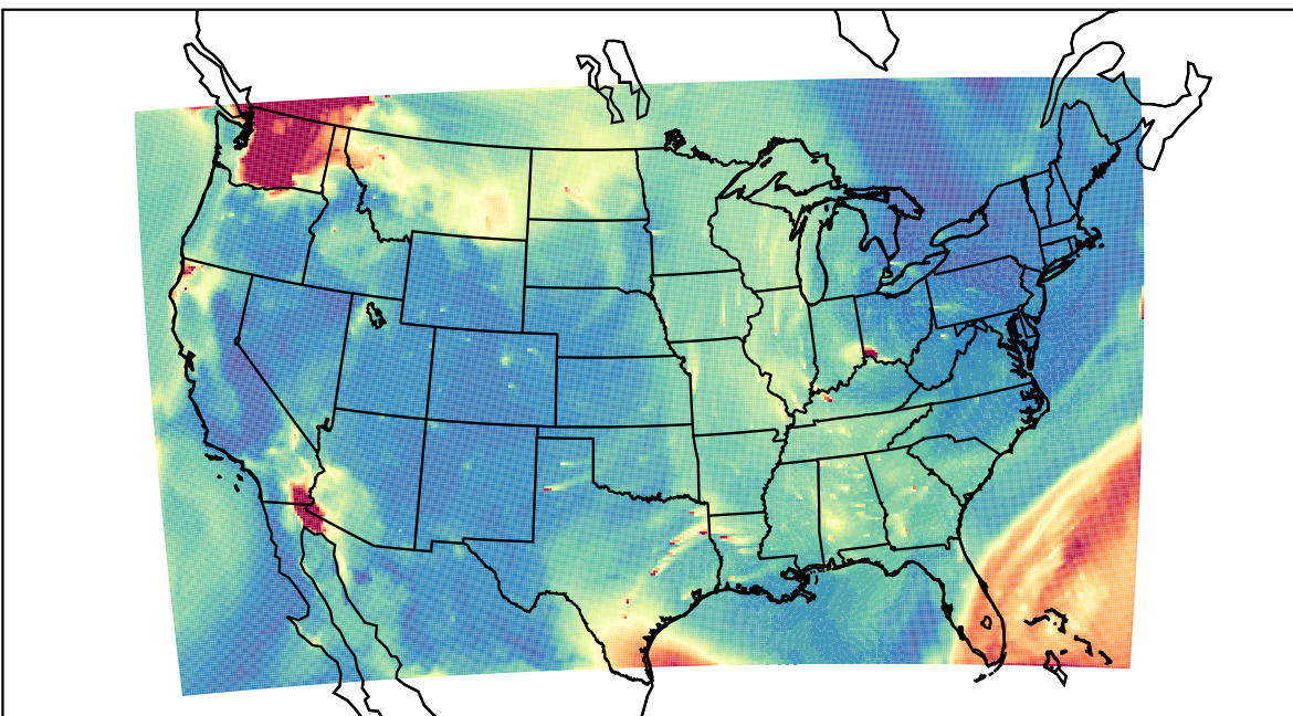
WRF 2023-08-19_15:00:00
