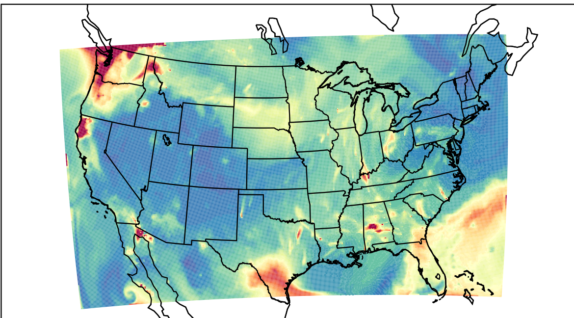
WRF 2023-08-20_07:00:00
