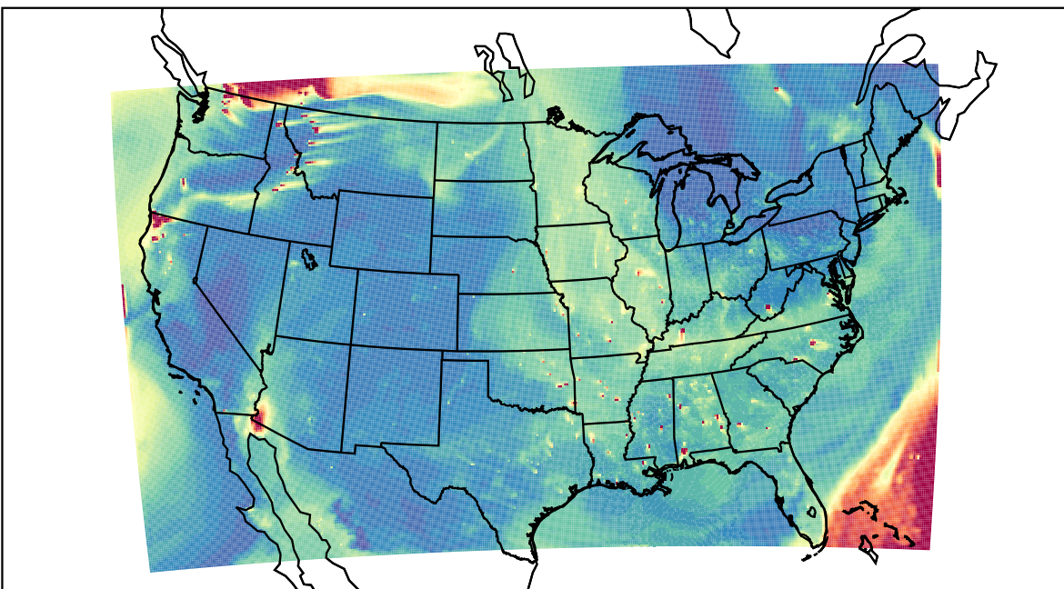
WRF 2023-08-19_00:00:00
