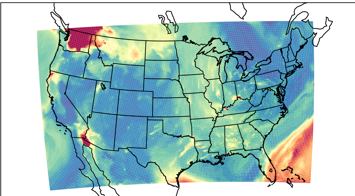
WRF 2023-08-19_13:00:00
