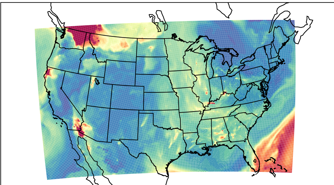
WRF 2023-08-19_09:00:00
