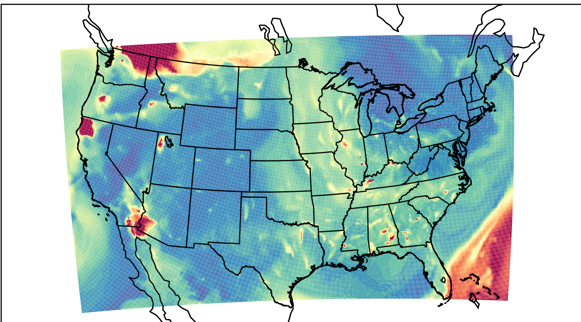
WRF 2023-08-19_05:00:00
