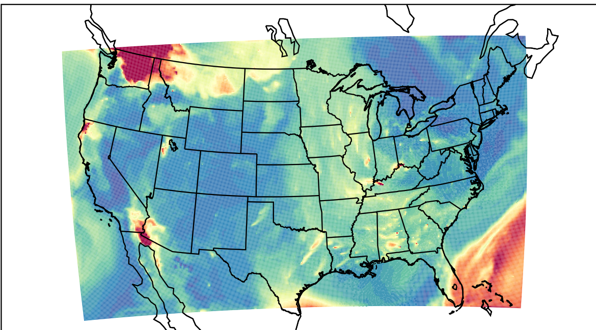
WRF 2023-08-19_11:00:00
