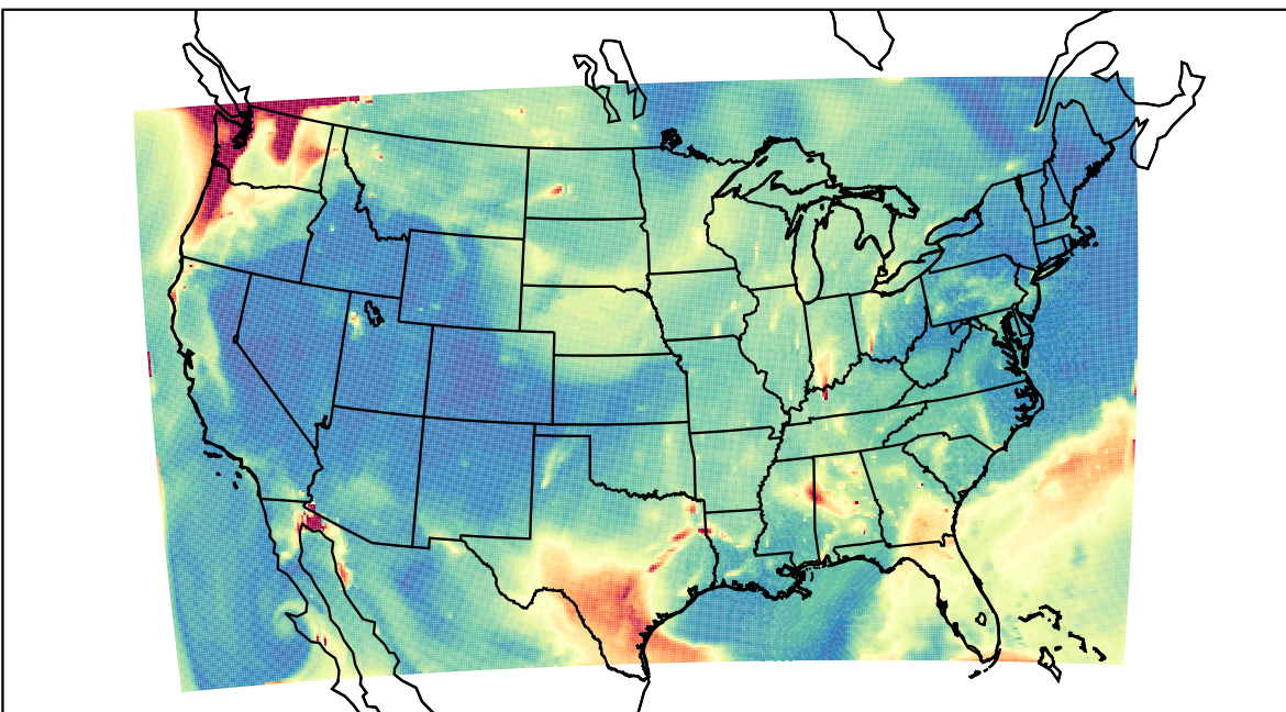
WRF 2023-08-20_12:00:00
