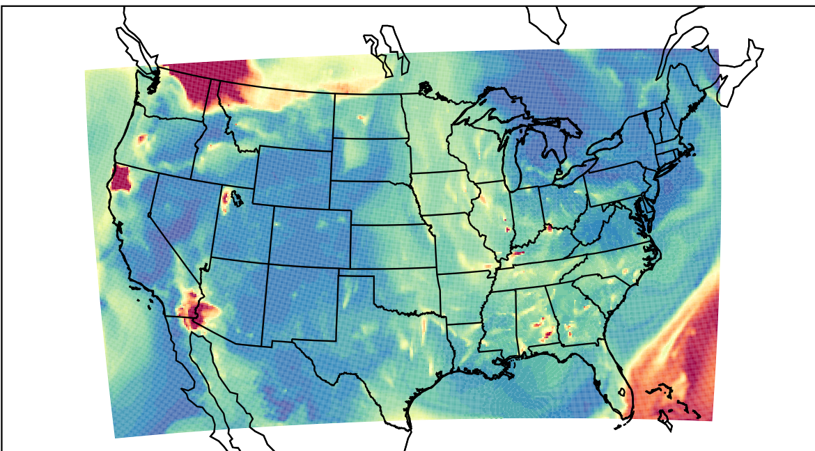
WRF 2023-08-19_06:00:00
