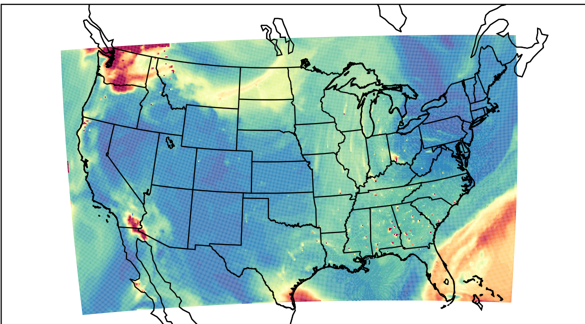
WRF 2023-08-19_20:00:00
