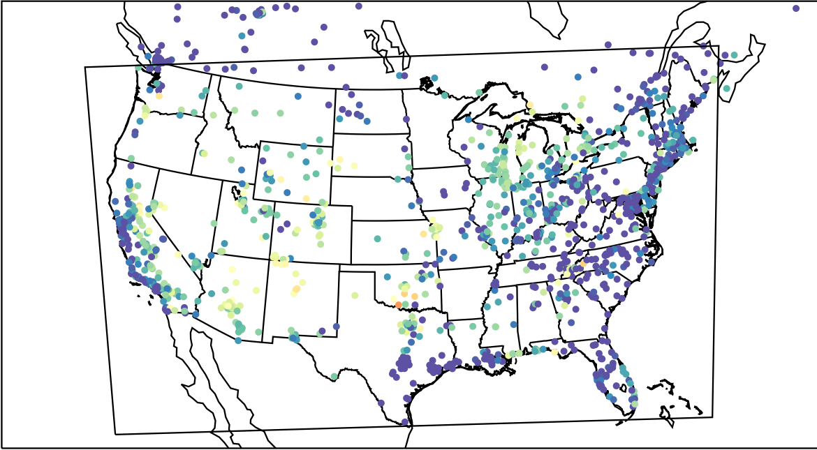
AirNOW (2023-08-20_06:00:00)
