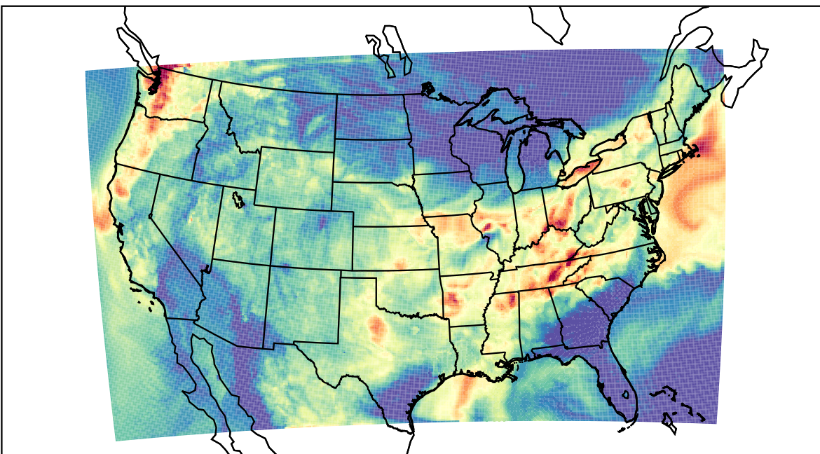
WRF (2023-08-21_05:00:00)
