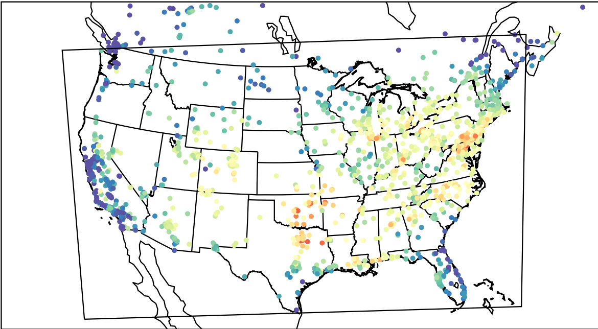
AirNOW (2023-08-20_16:00:00)
