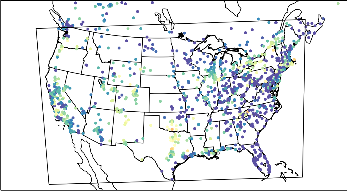
AirNOW (2023-08-21_04:00:00)
