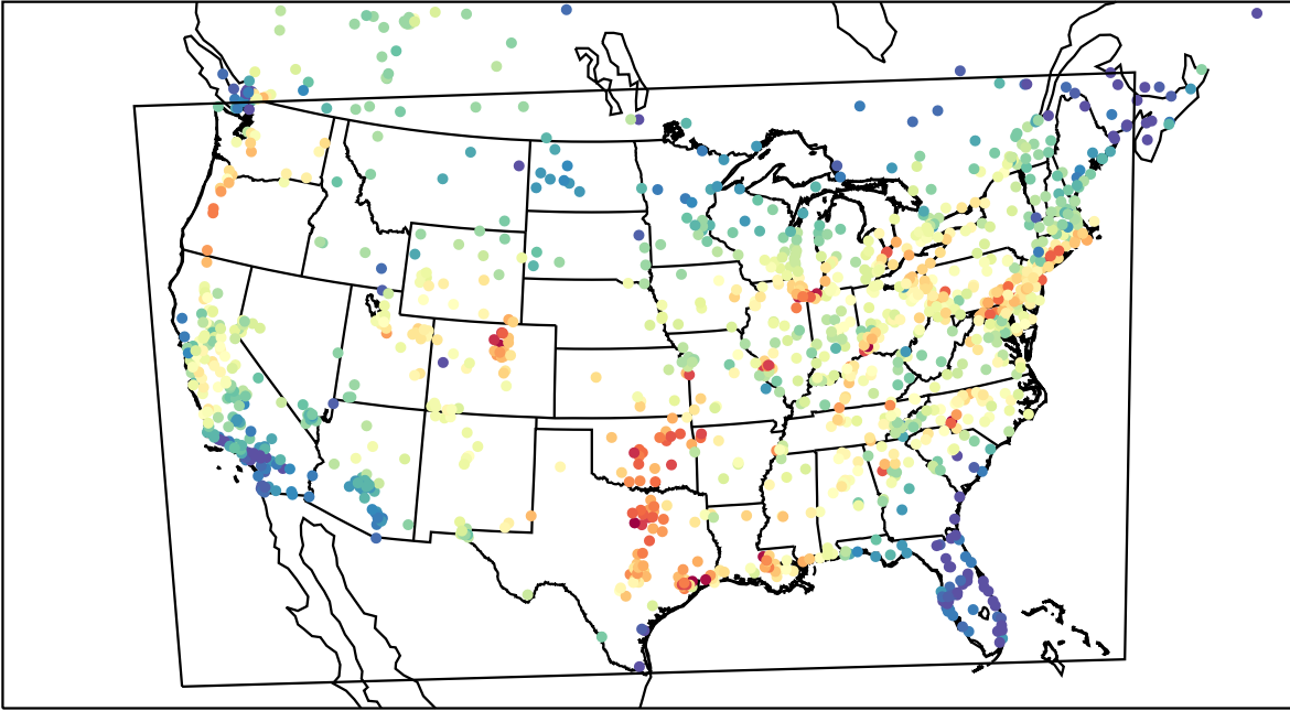
AirNOW (2023-08-20_22:00:00)
