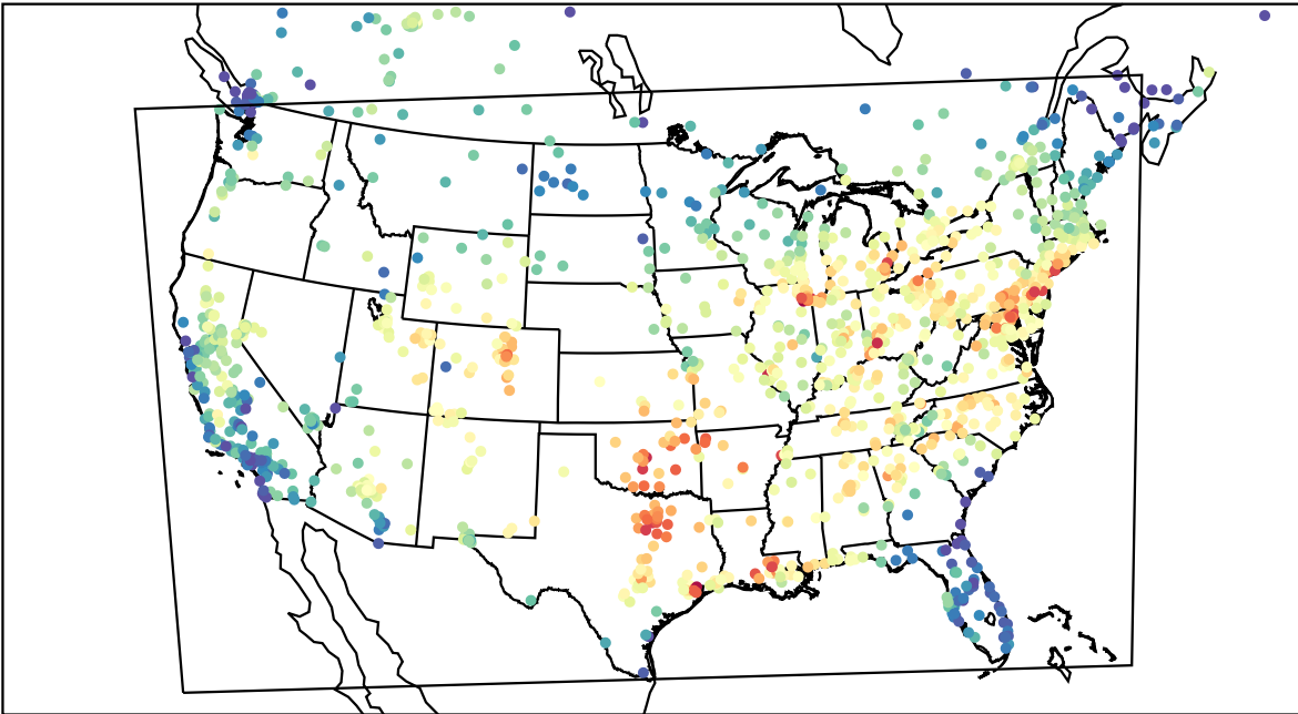
AirNOW (2023-08-20_18:00:00)
