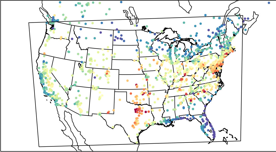
AirNOW (2023-08-21_21:00:00)
