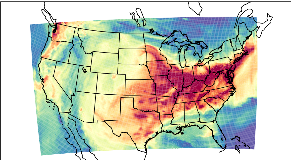
WRF (2023-08-21_21:00:00)
