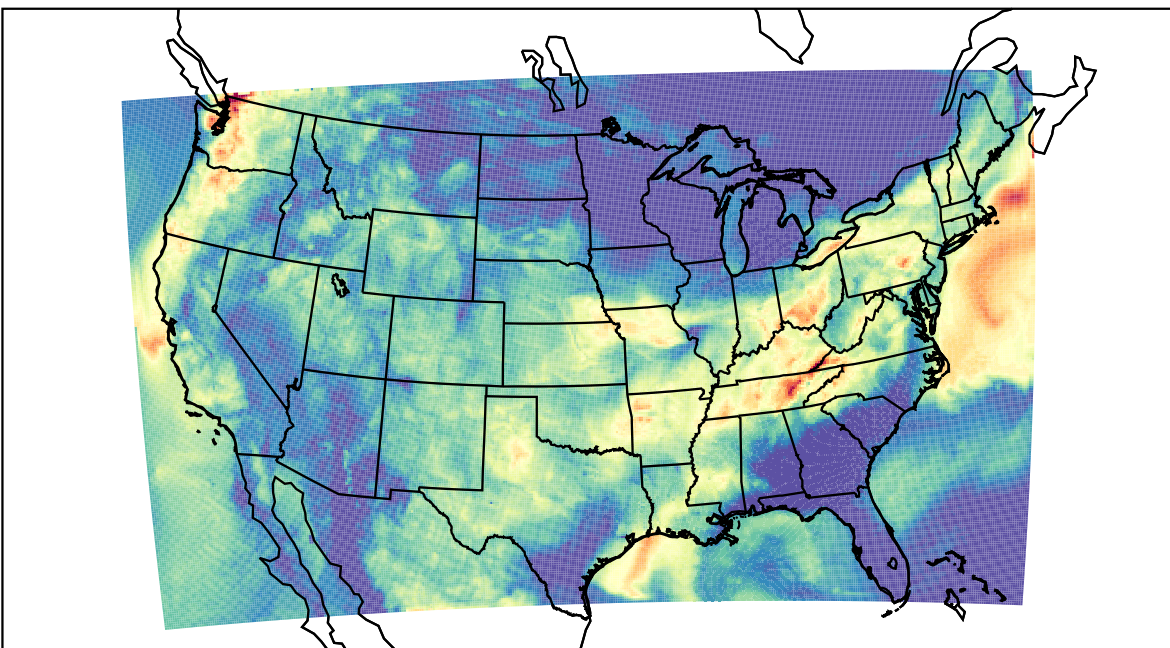
WRF (2023-08-21_09:00:00)
