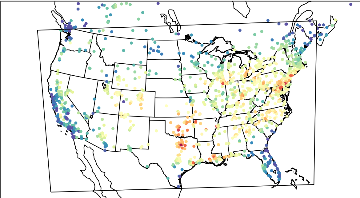
AirNOW (2023-08-20_17:00:00)
