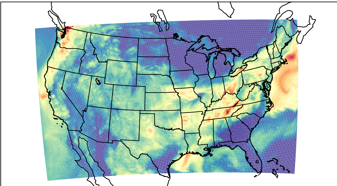
WRF (2023-08-21_08:00:00)
