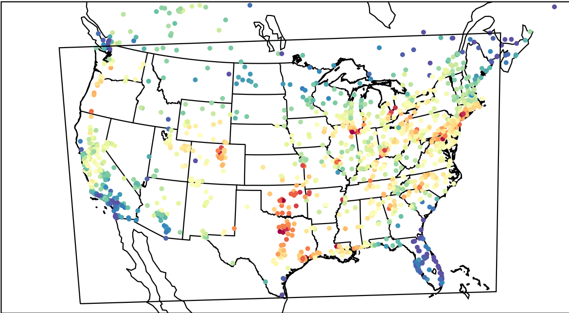
AirNOW (2023-08-20_21:00:00)
