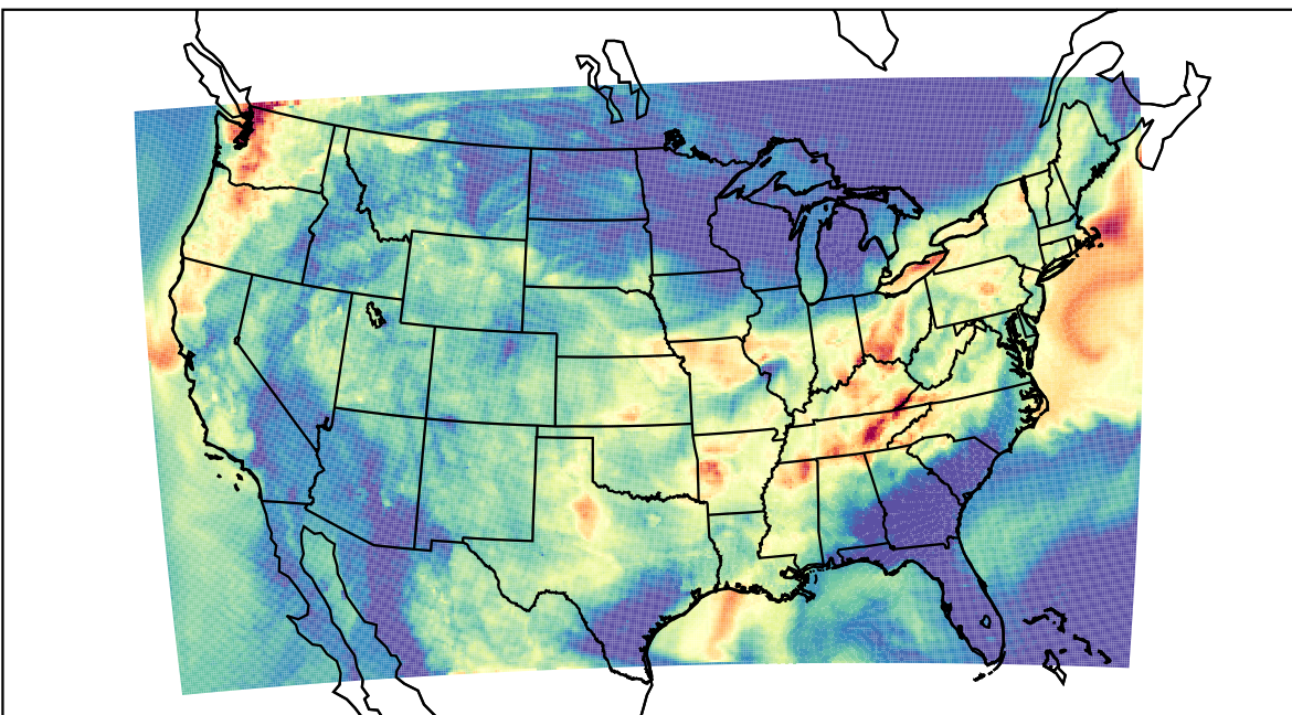
WRF (2023-08-21_06:00:00)
