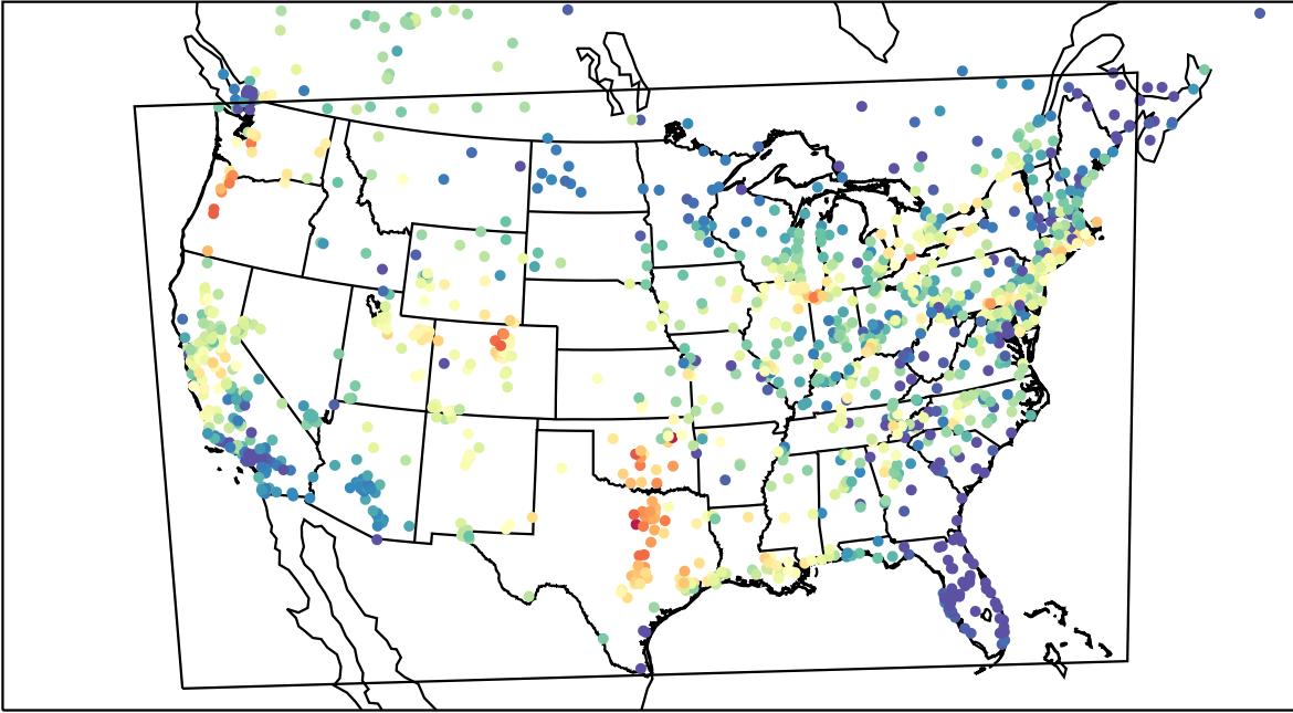
AirNOW (2023-08-21_00:00:00)
