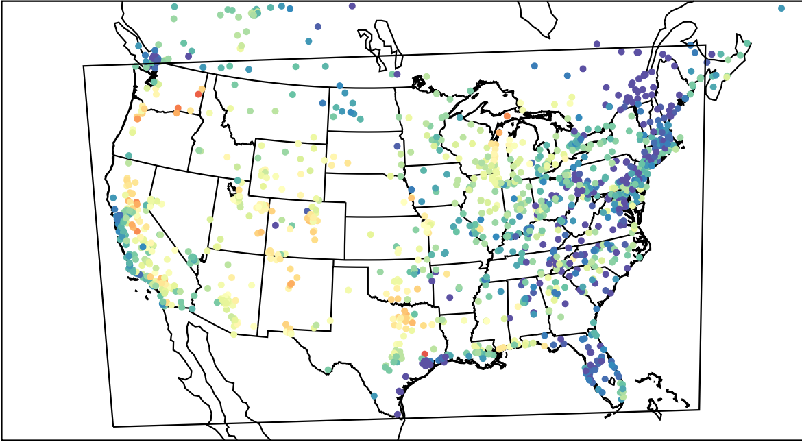
AirNOW (2023-08-20_01:00:00)
