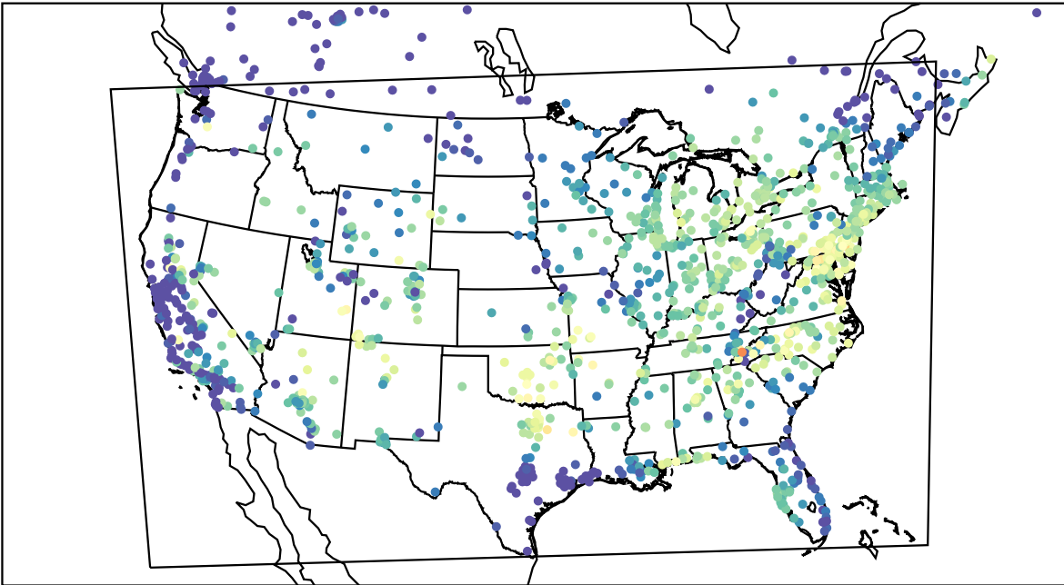
AirNOW (2023-08-20_14:00:00)
