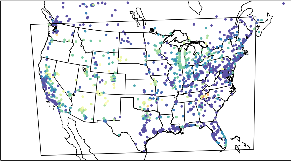
AirNOW (2023-08-20_08:00:00)
