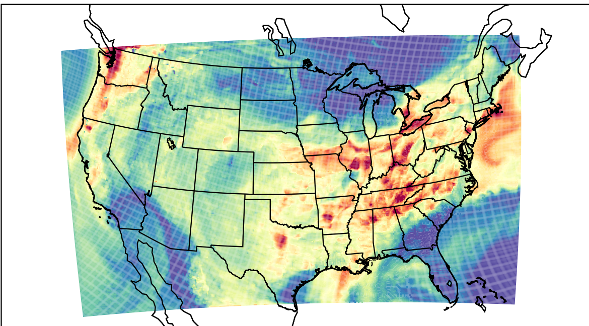
WRF (2023-08-21_02:00:00)
