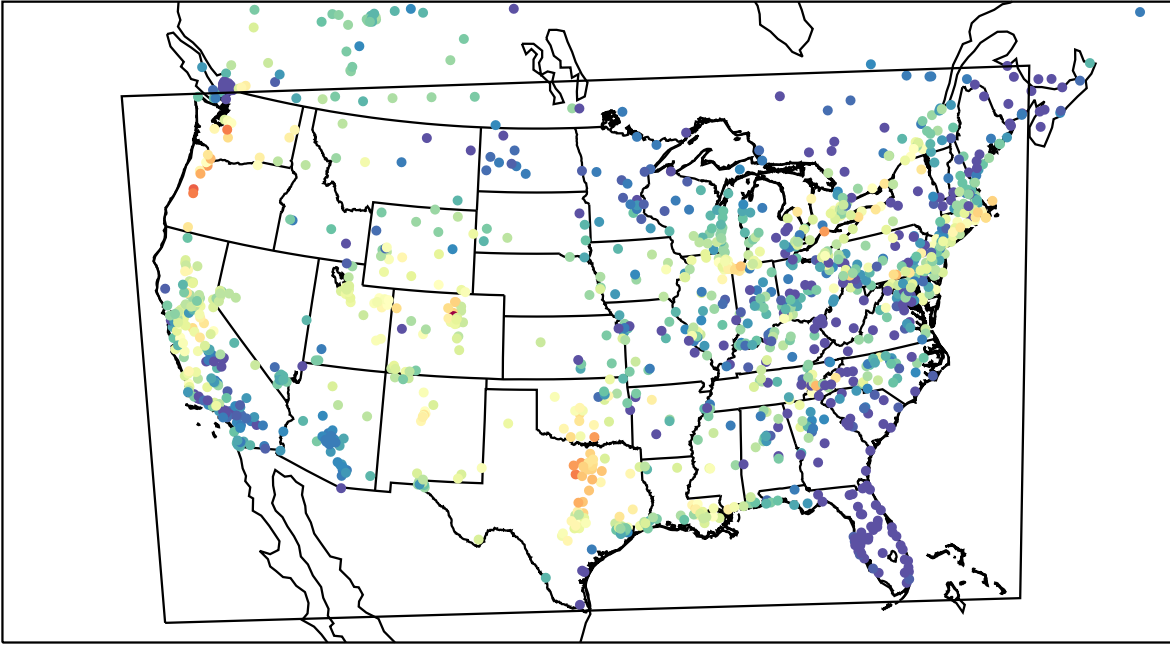
AirNOW (2023-08-21_01:00:00)
