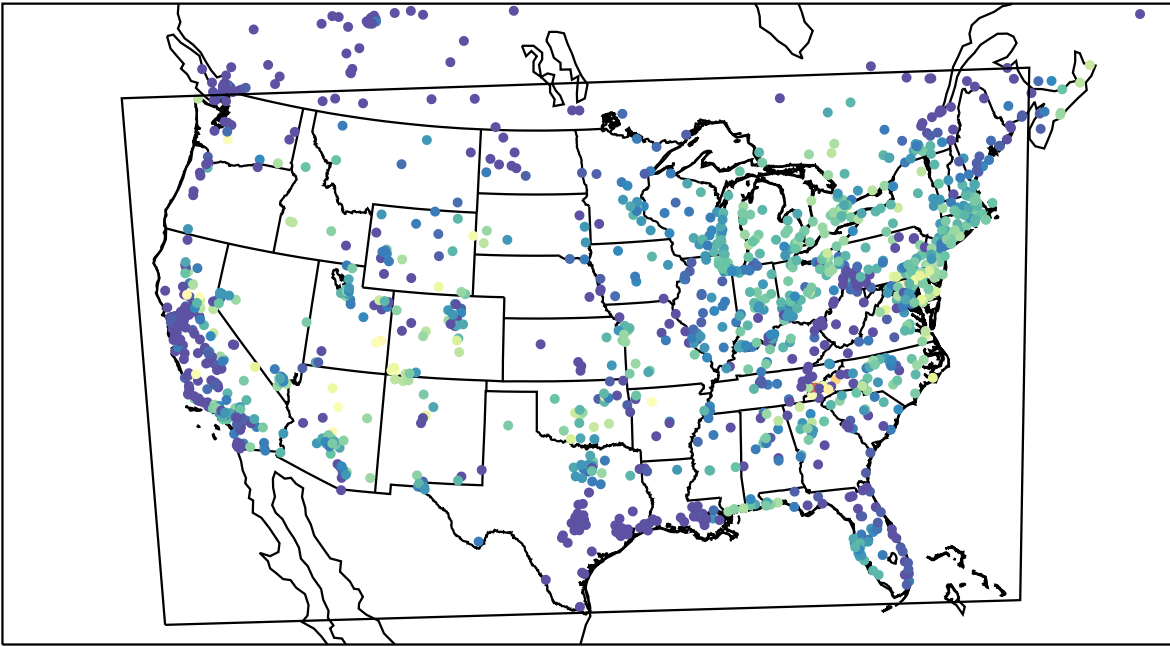
AirNOW (2023-08-20_13:00:00)
