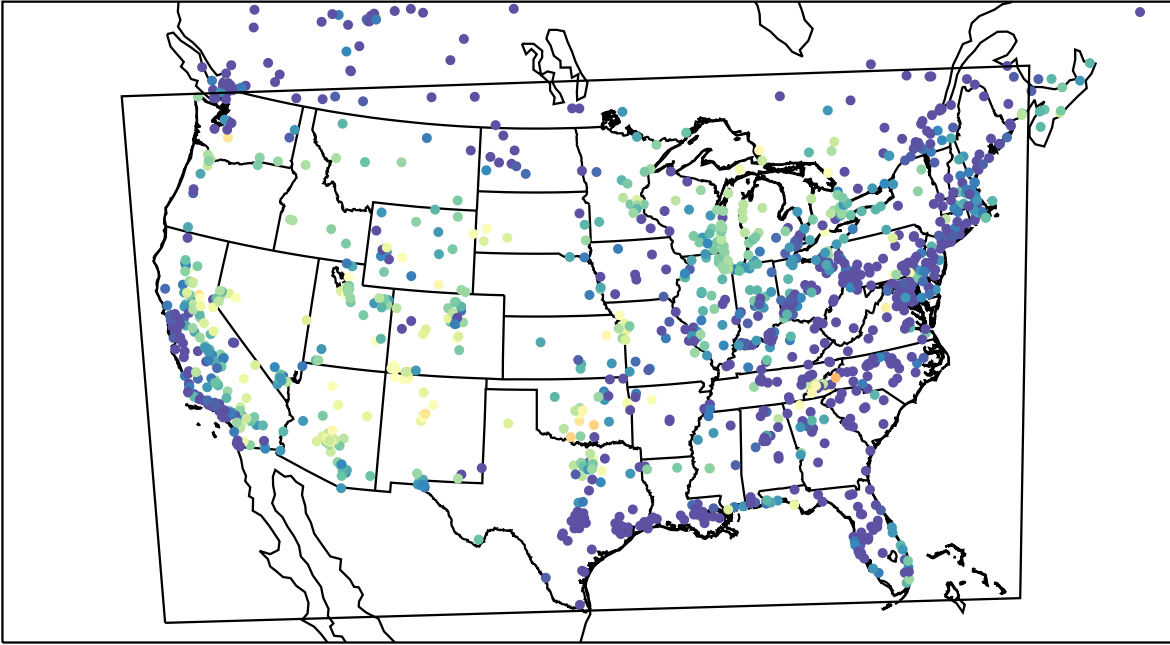
AirNOW (2023-08-20_07:00:00)
