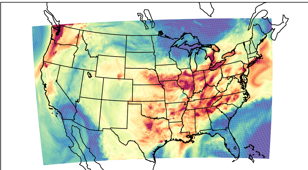
WRF (2023-08-21_00:00:00)
