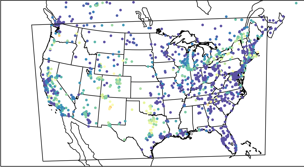
AirNOW (2023-08-21_06:00:00)
