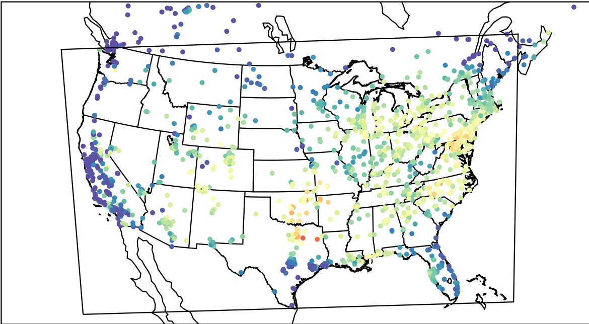
AirNOW (2023-08-20_15:00:00)
