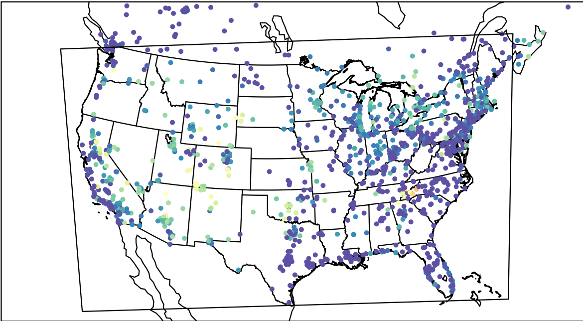
AirNOW (2023-08-20_11:00:00)
