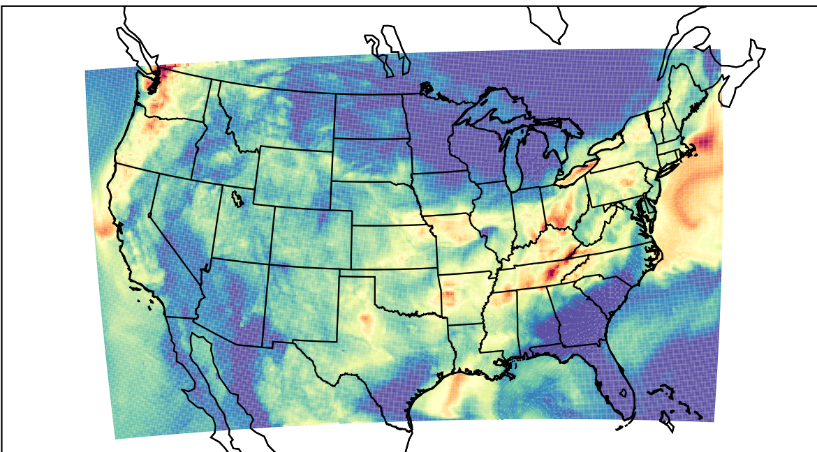
WRF (2023-08-21_07:00:00)
