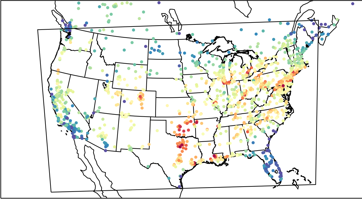
AirNOW (2023-08-20_19:00:00)
