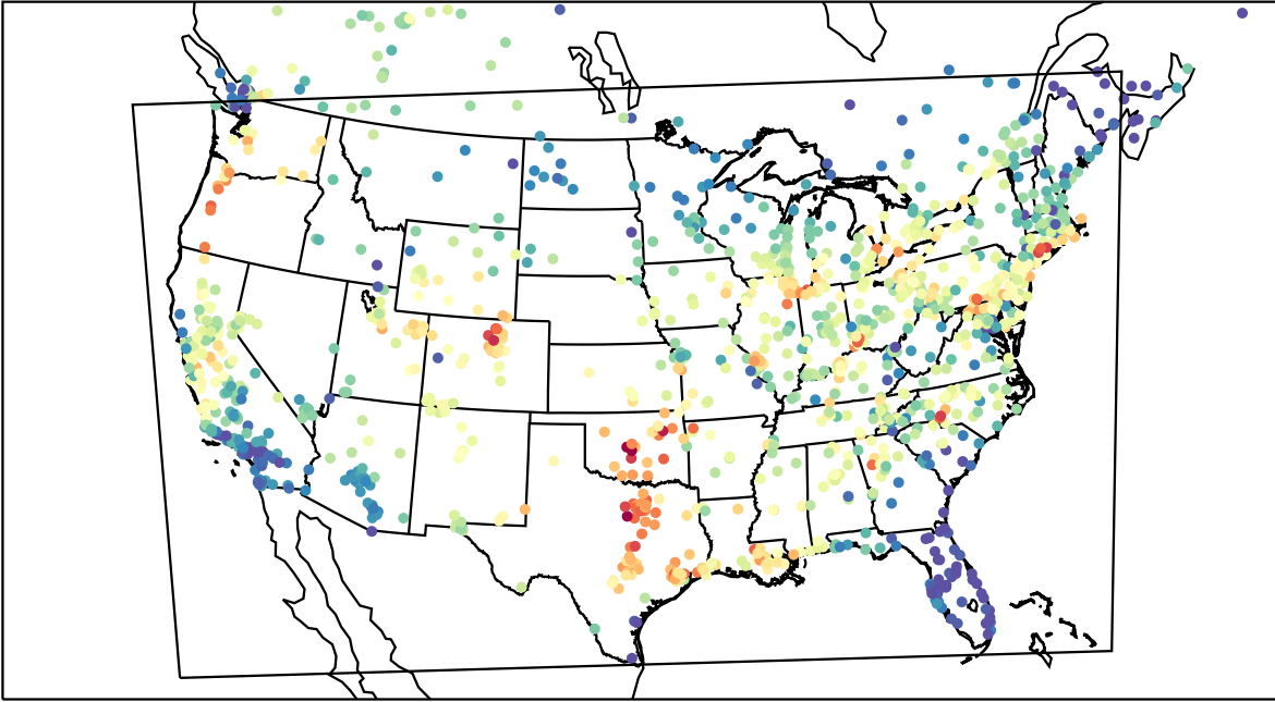
AirNOW (2023-08-20_23:00:00)
