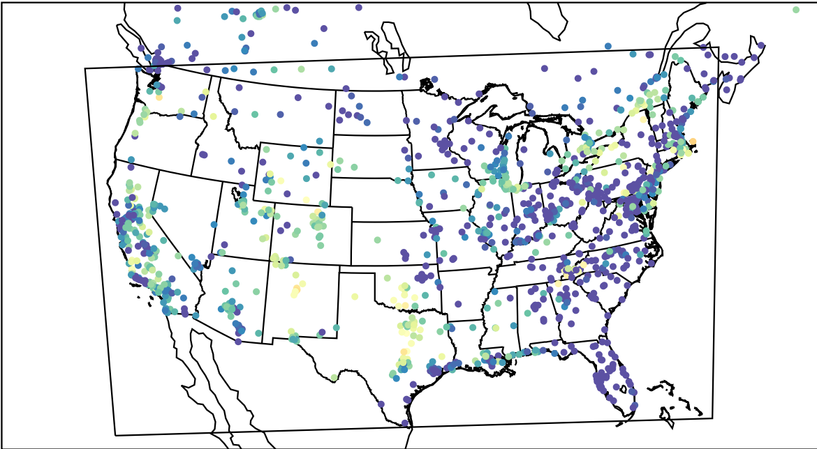
AirNOW (2023-08-21_05:00:00)
