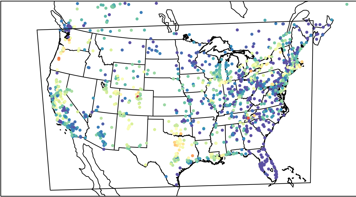
AirNOW (2023-08-21_02:00:00)
