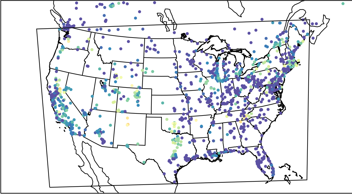
AirNOW (2023-08-21_08:00:00)
