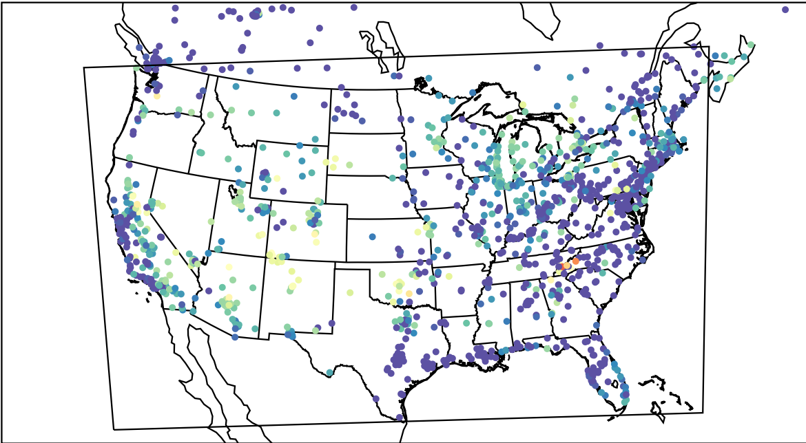
AirNOW (2023-08-20_09:00:00)
