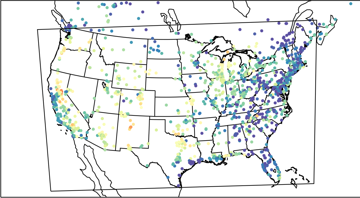
AirNOW (2023-08-20_02:00:00)
