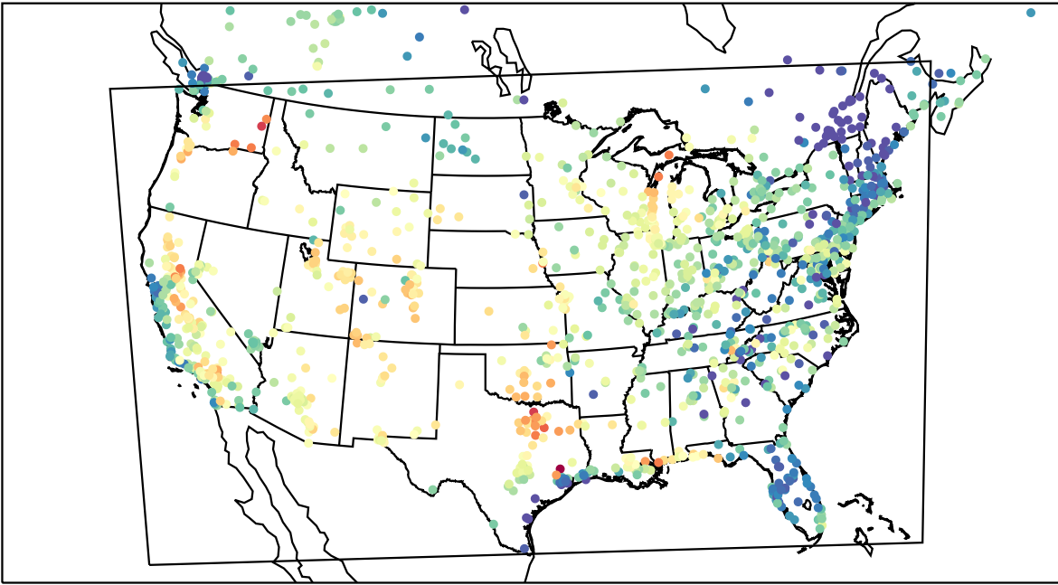
AirNOW (2023-08-20_00:00:00)
