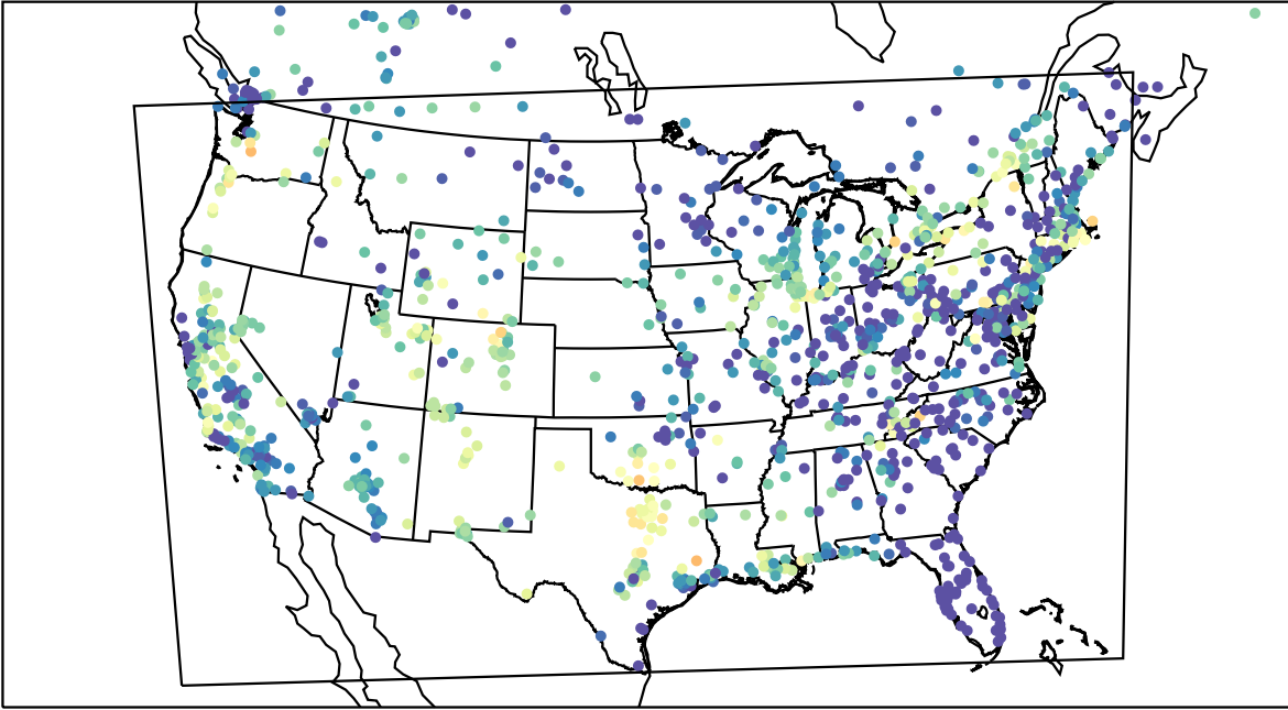
AirNOW (2023-08-21_03:00:00)
