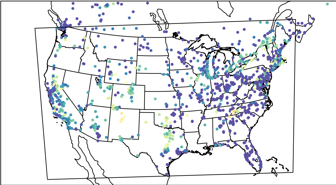
AirNOW (2023-08-21_07:00:00)
