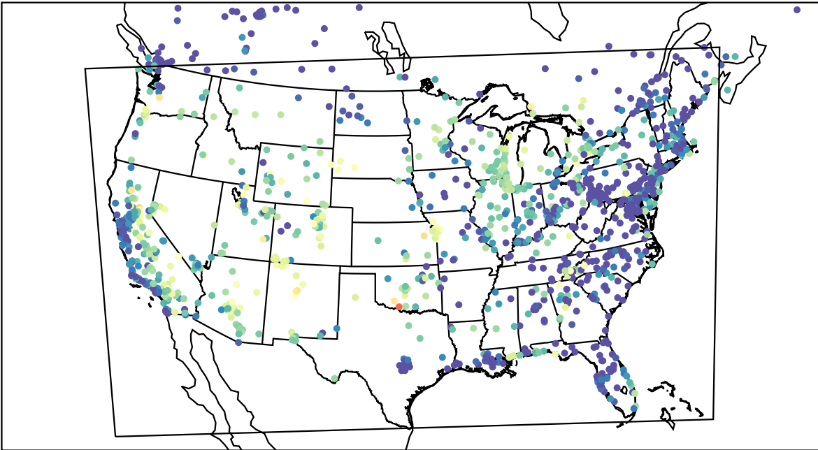
AirNOW (2023-08-20_05:00:00)
