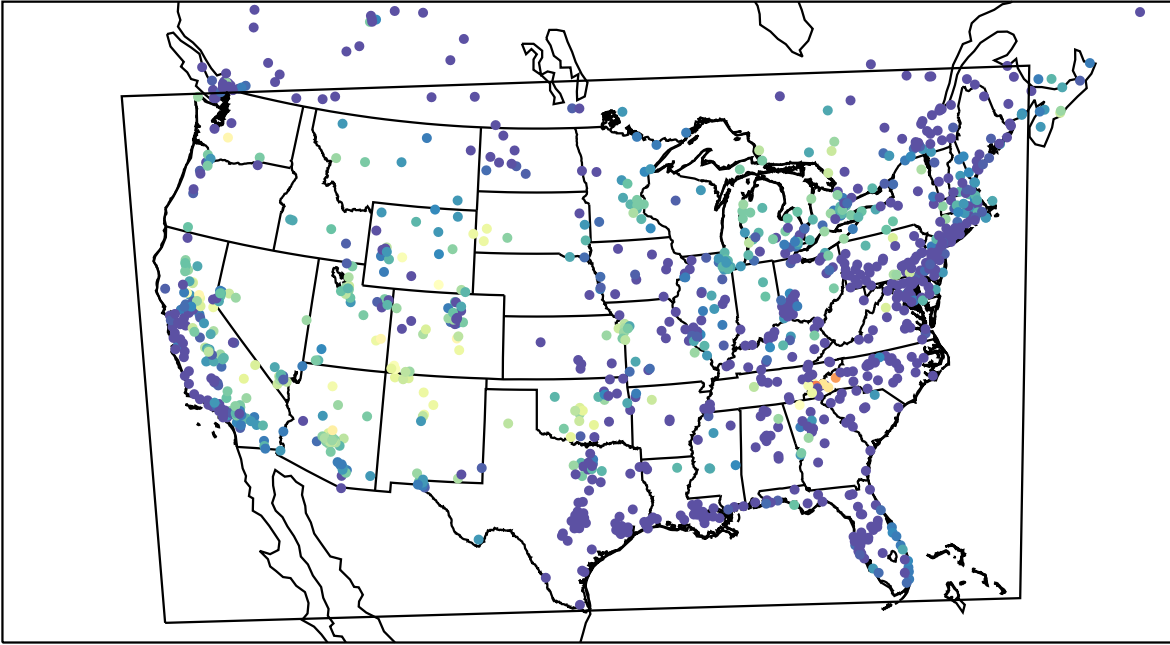
AirNOW (2023-08-20_10:00:00)
