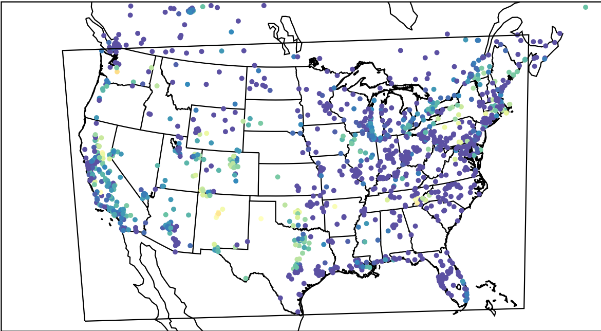
AirNOW (2023-08-21_09:00:00)
