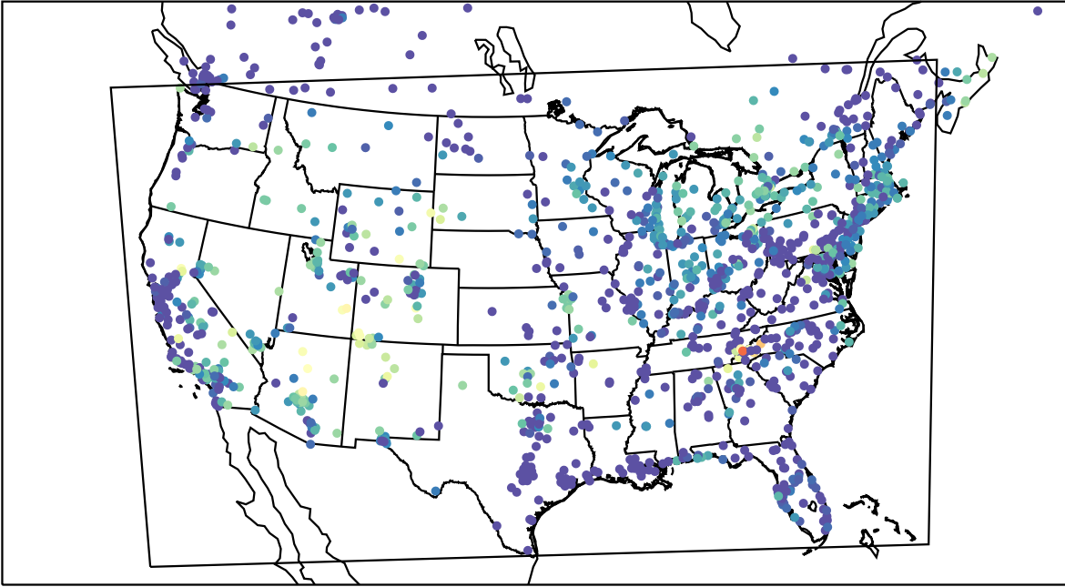
AirNOW (2023-08-20_12:00:00)
