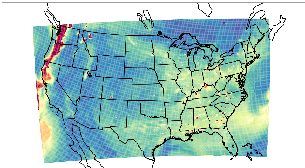
WRF 2023-08-22_00:00:00
