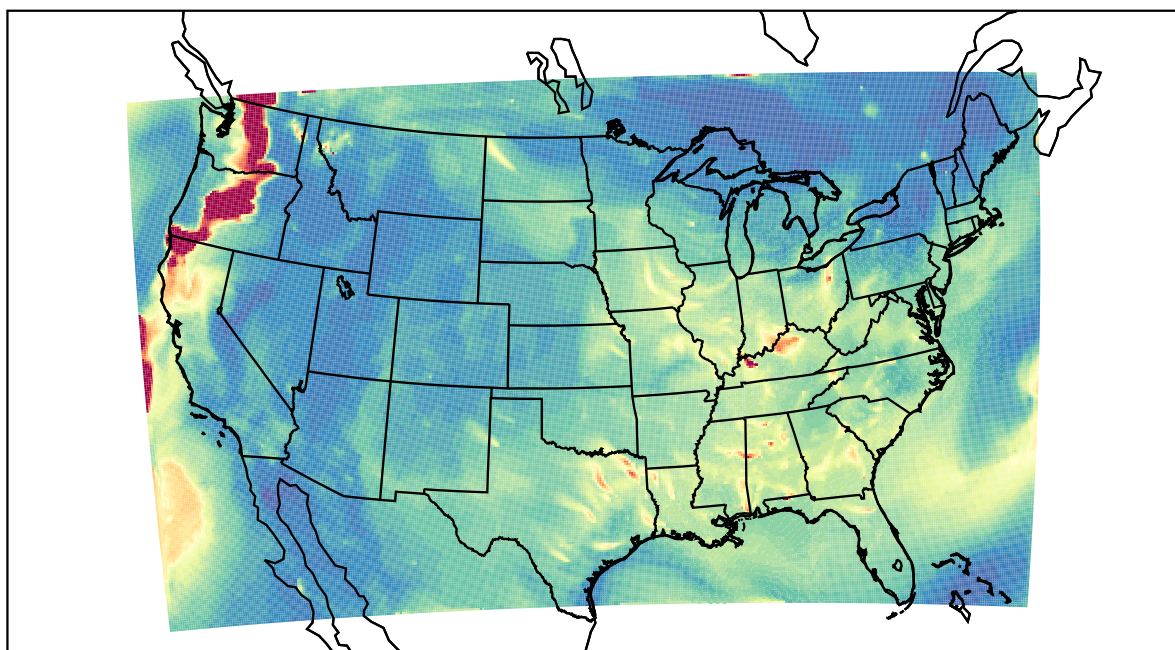
WRF 2023-08-22_07:00:00
