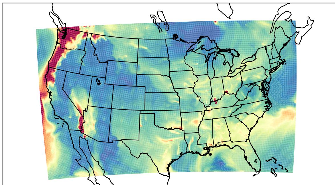
WRF 2023-08-21_09:00:00
