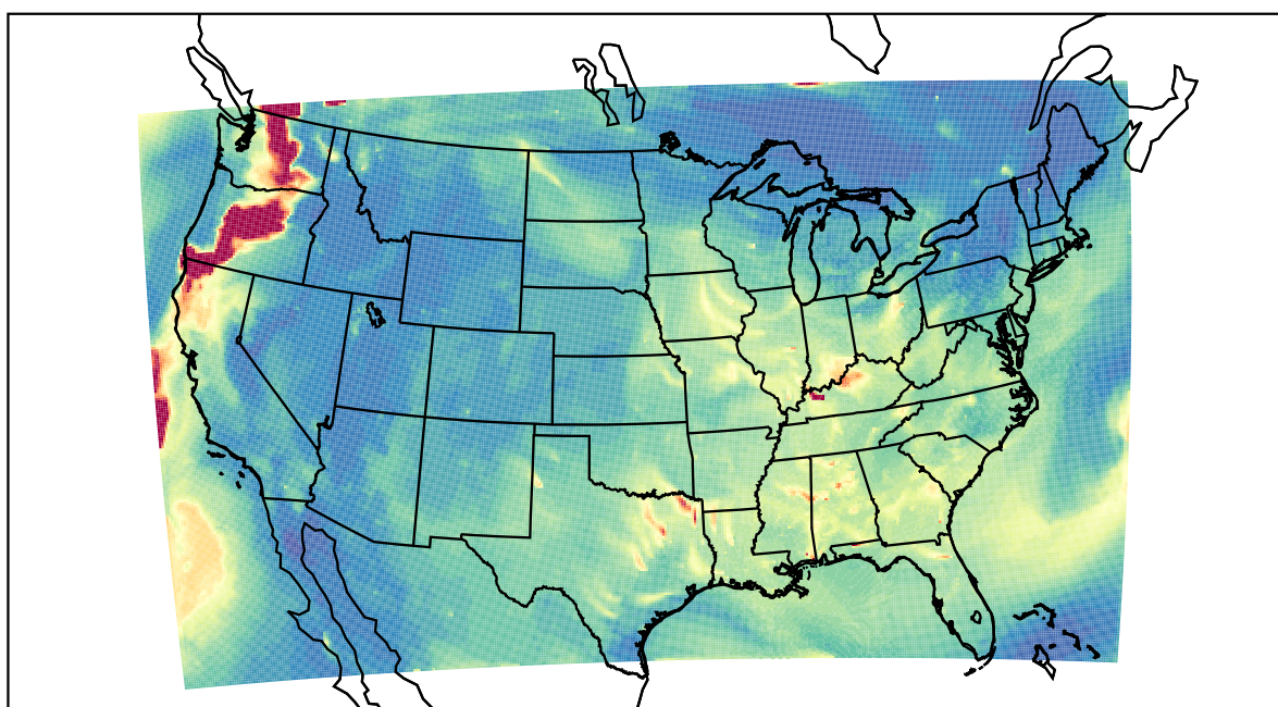
WRF 2023-08-22_09:00:00
