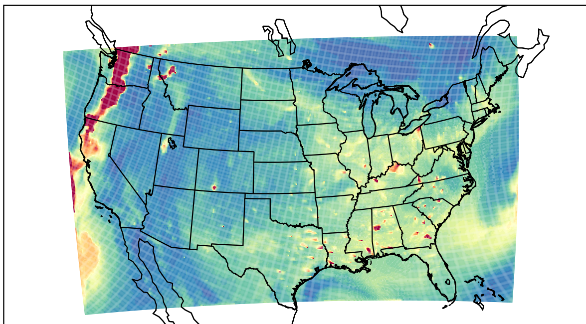
WRF 2023-08-22_02:00:00
