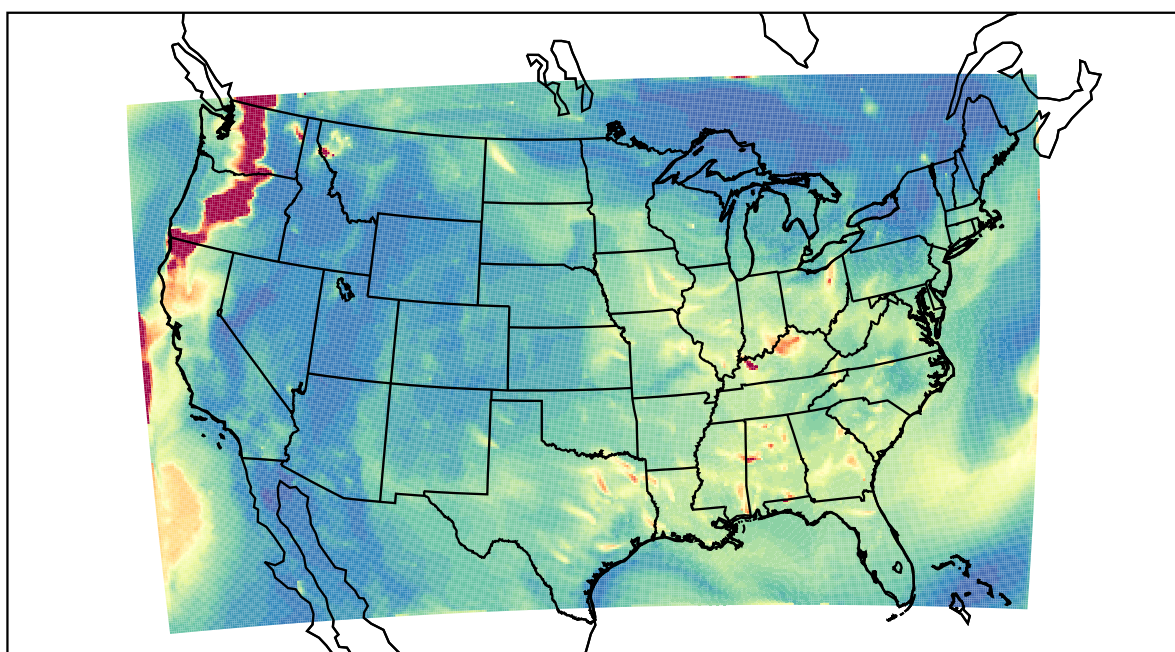
WRF 2023-08-22_06:00:00
