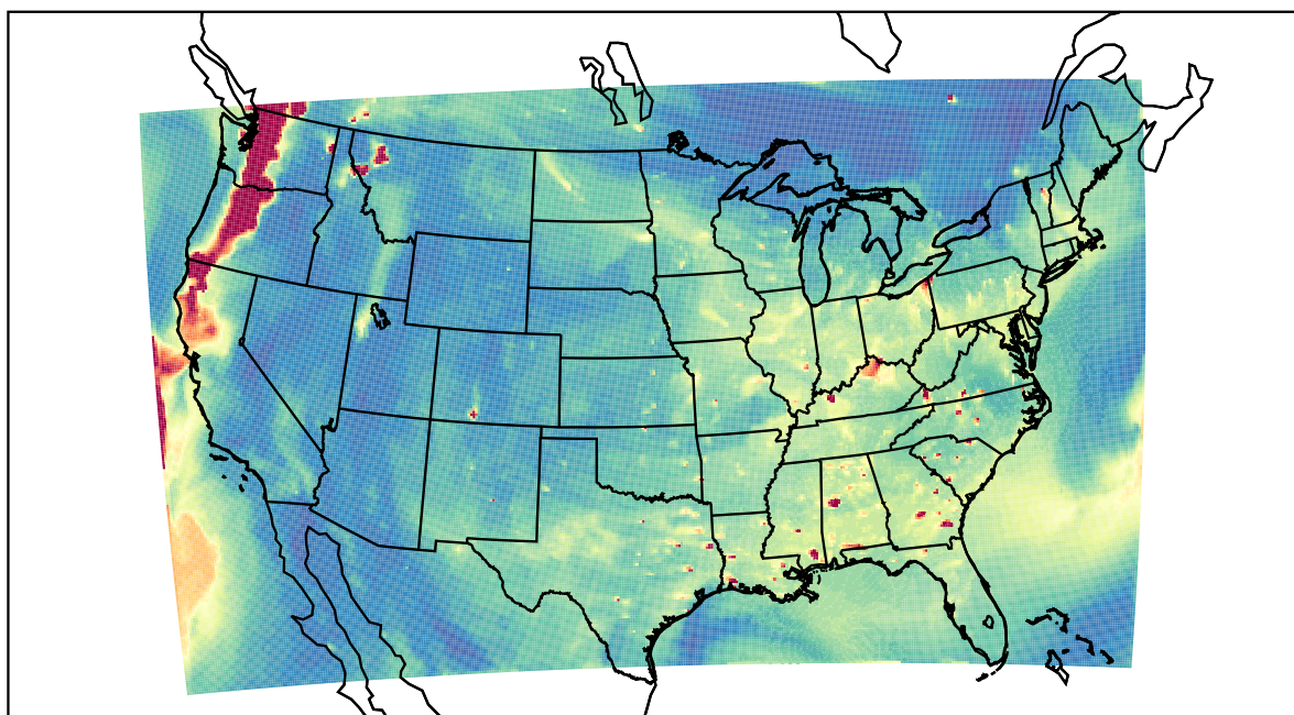
WRF 2023-08-22_01:00:00
