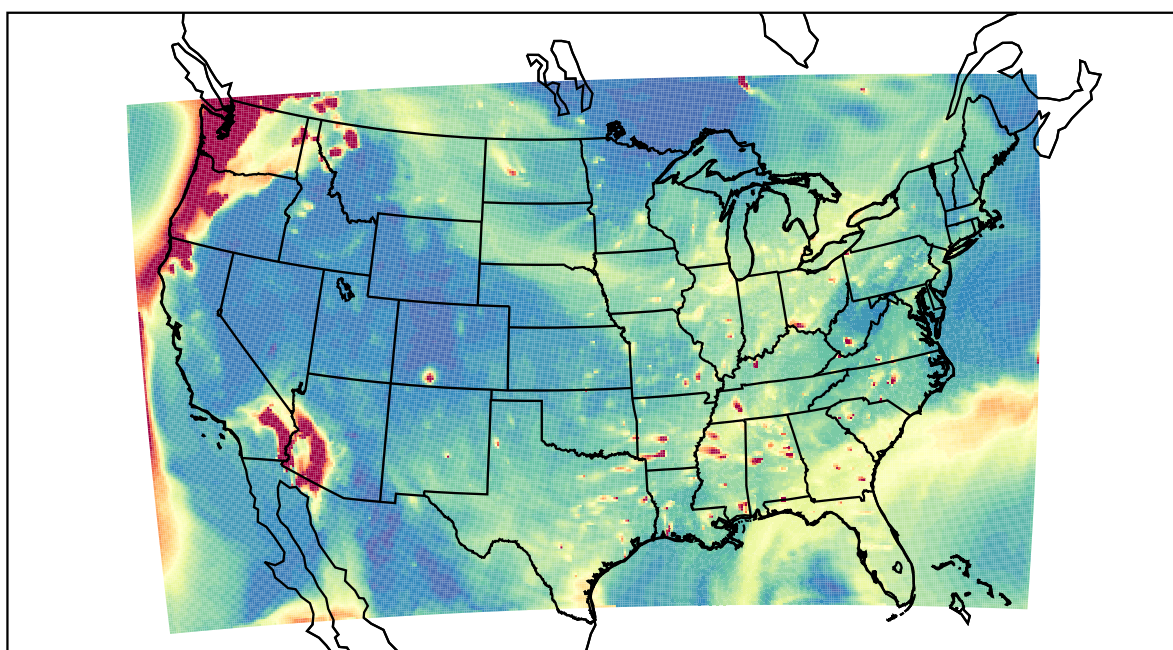
WRF 2023-08-21_02:00:00
