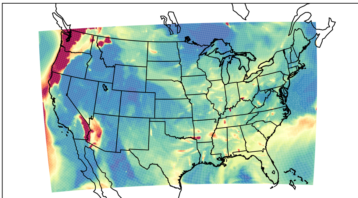
WRF 2023-08-21_05:00:00
