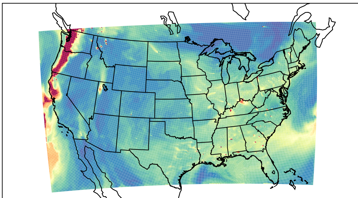
WRF 2023-08-21_21:00:00
