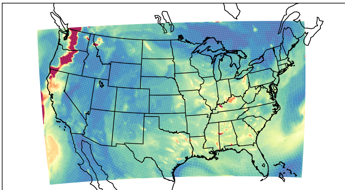
WRF 2023-08-22_05:00:00
