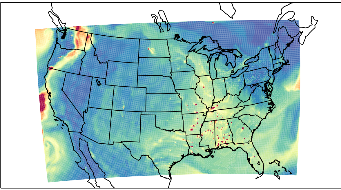
WRF 2023-08-23_00:00:00
