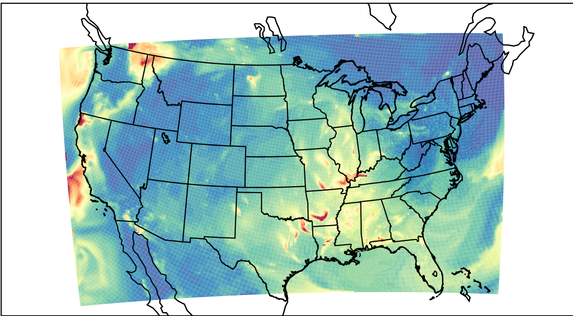
WRF 2023-08-23_08:00:00
