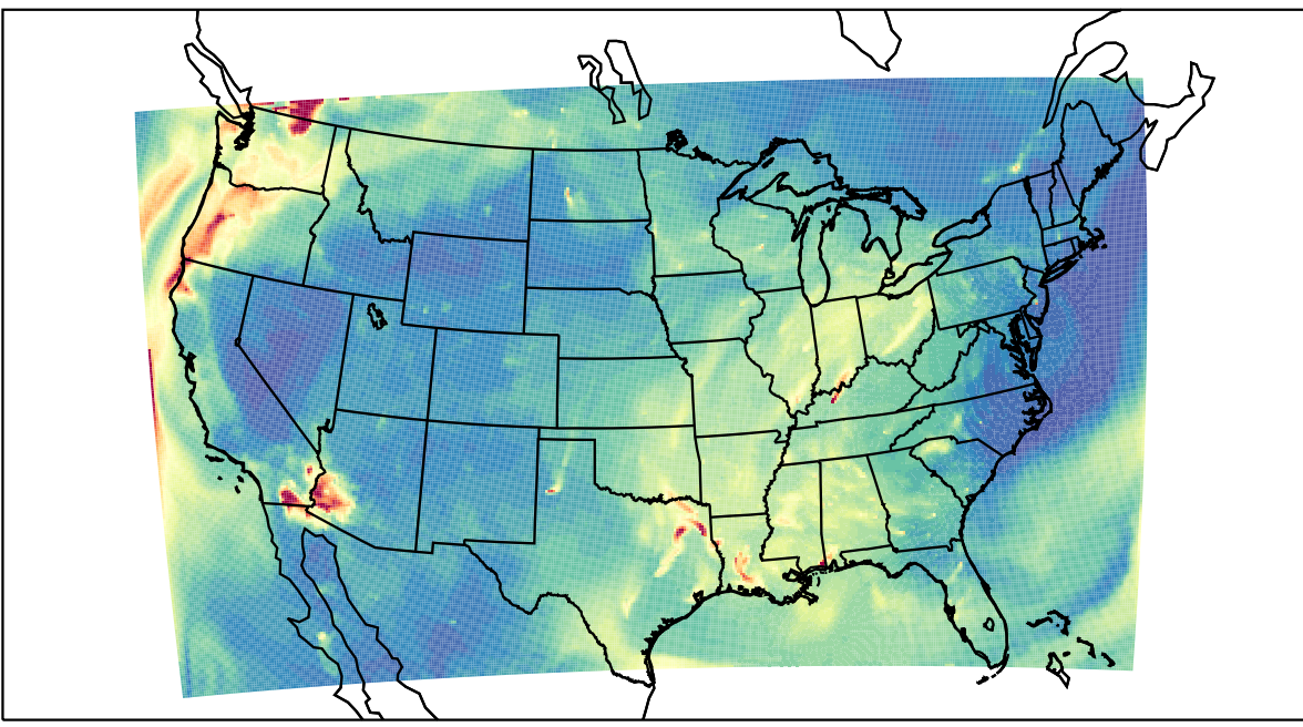
WRF 2023-08-24_09:00:00
