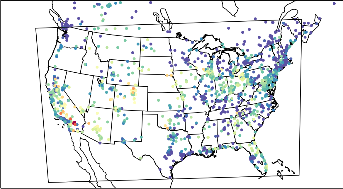
AirNOW (2023-08-24_04:00:00)
