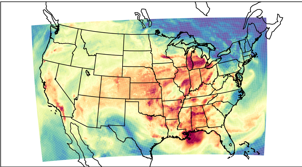
WRF (2023-08-24_00:00:00)
