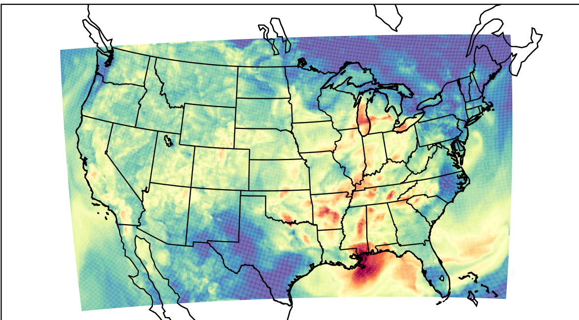
WRF (2023-08-24_05:00:00)
