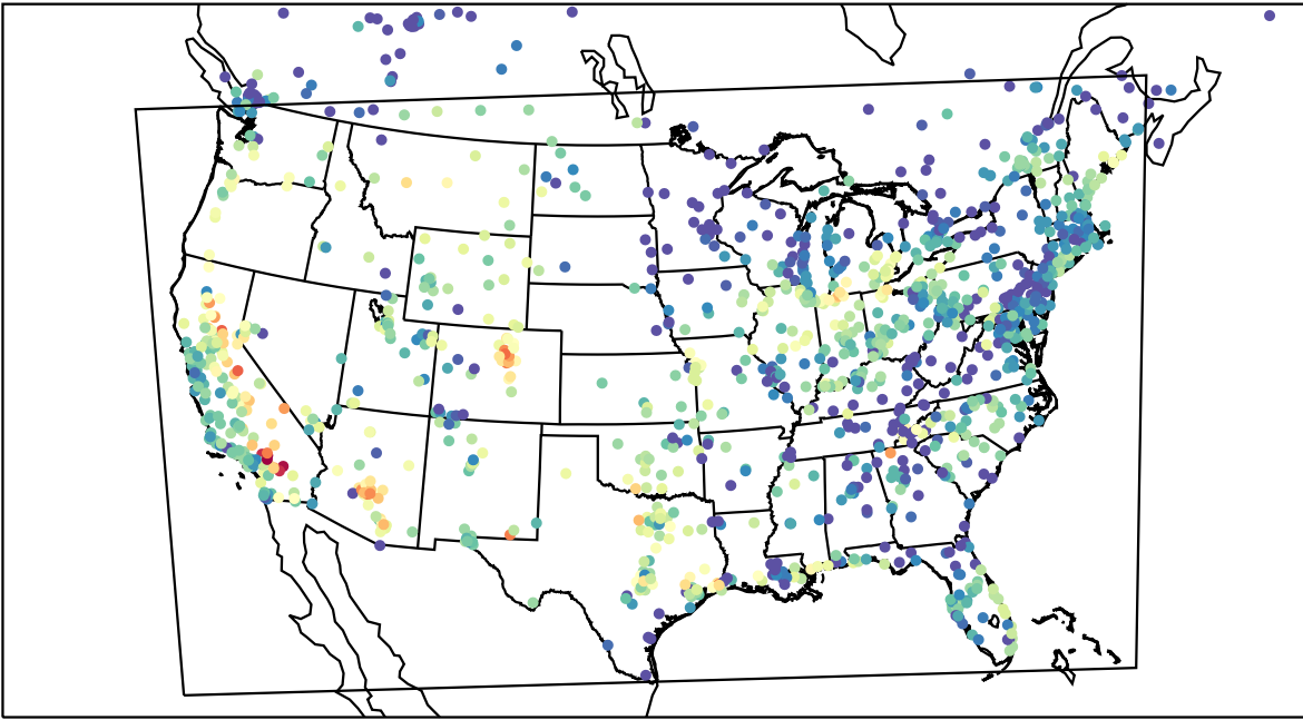
AirNOW (2023-08-25_03:00:00)
