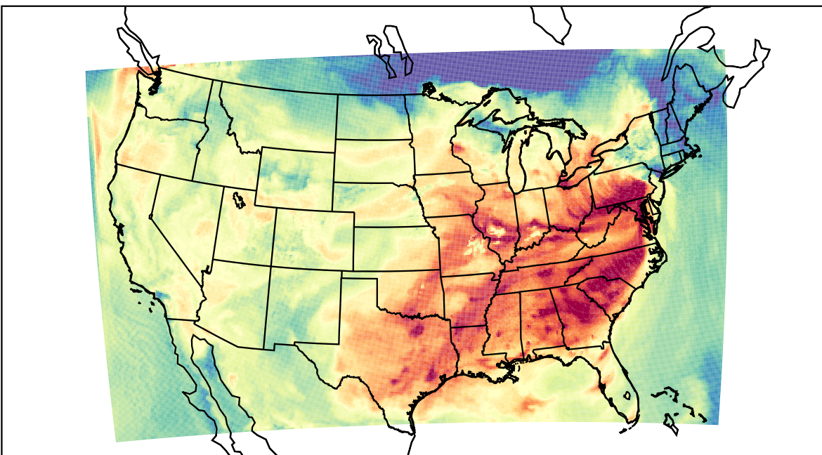
WRF (2023-08-25_18:00:00)
