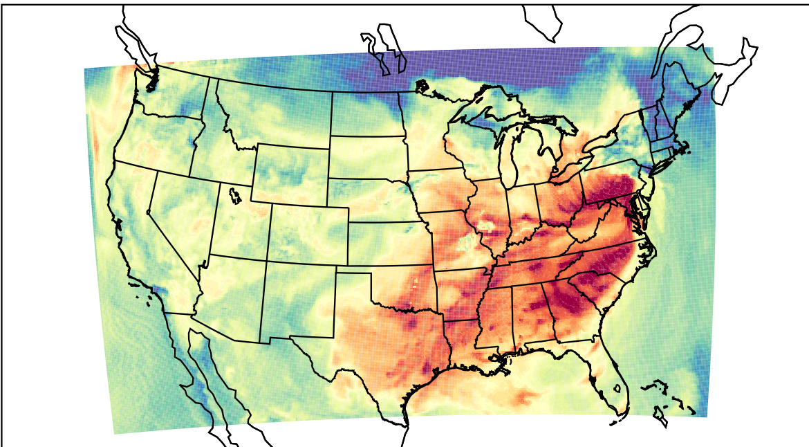
WRF (2023-08-25_17:00:00)
