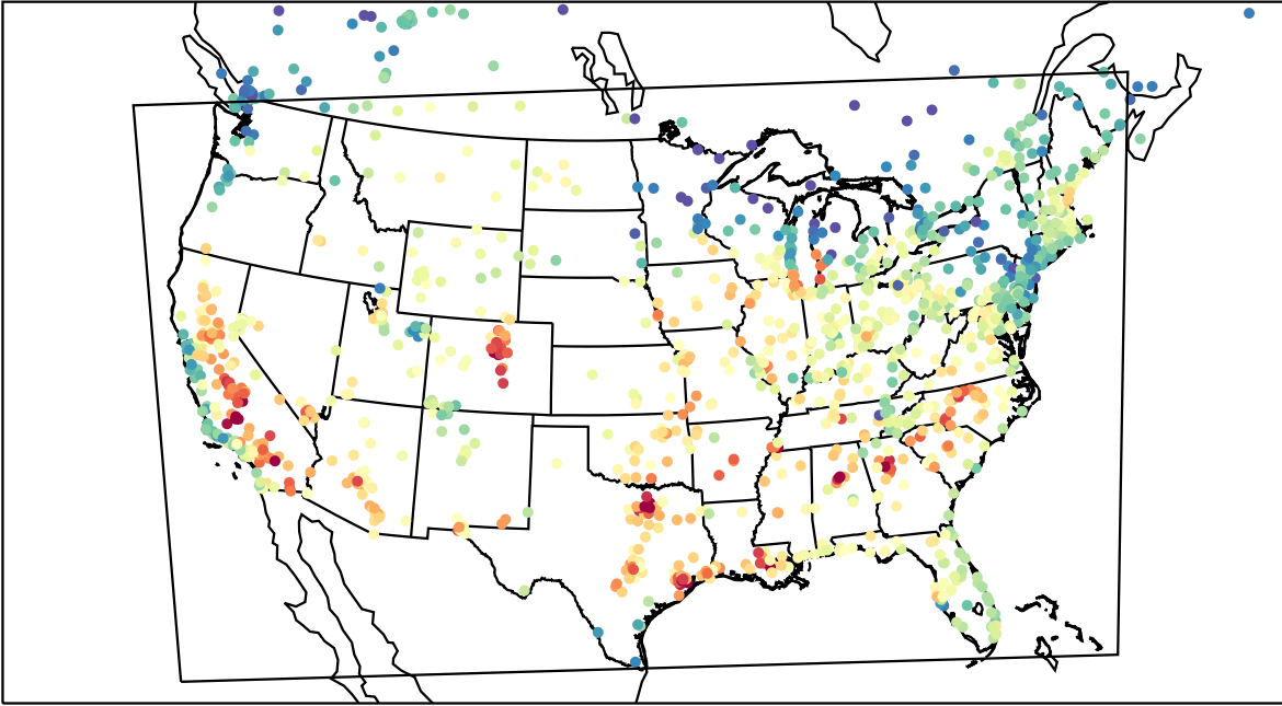
AirNOW (2023-08-24_19:00:00)
