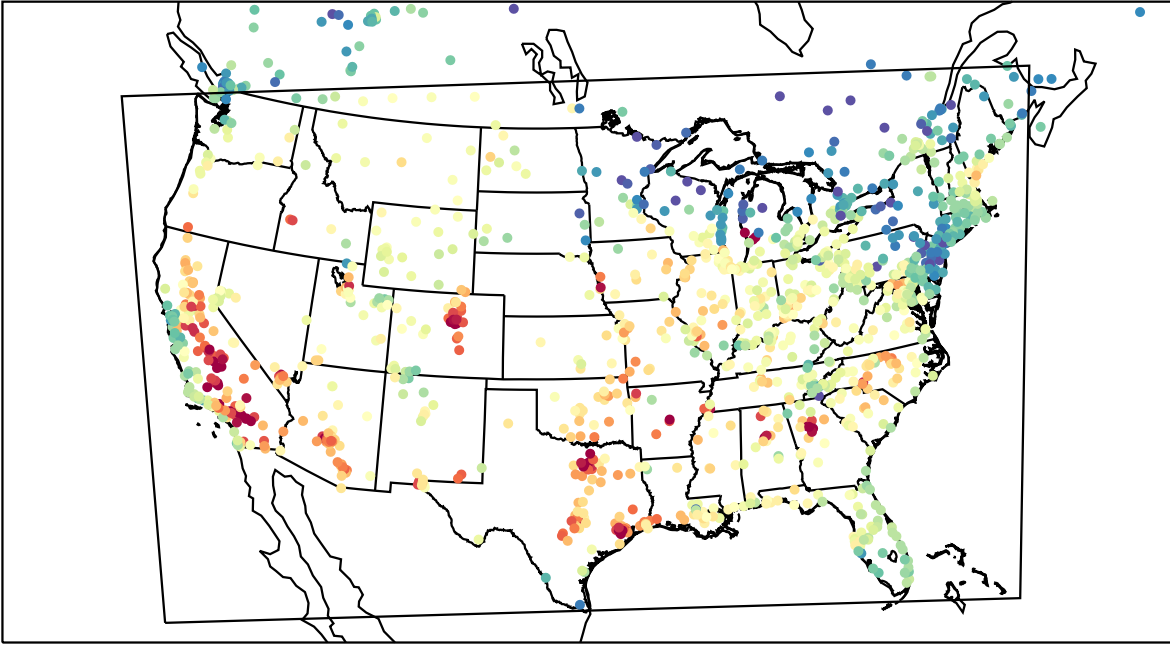
AirNOW (2023-08-24_21:00:00)
