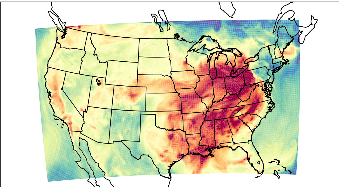
WRF (2023-08-24_20:00:00)
