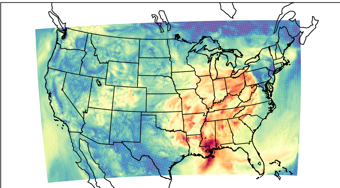
WRF (2023-08-24_15:00:00)
