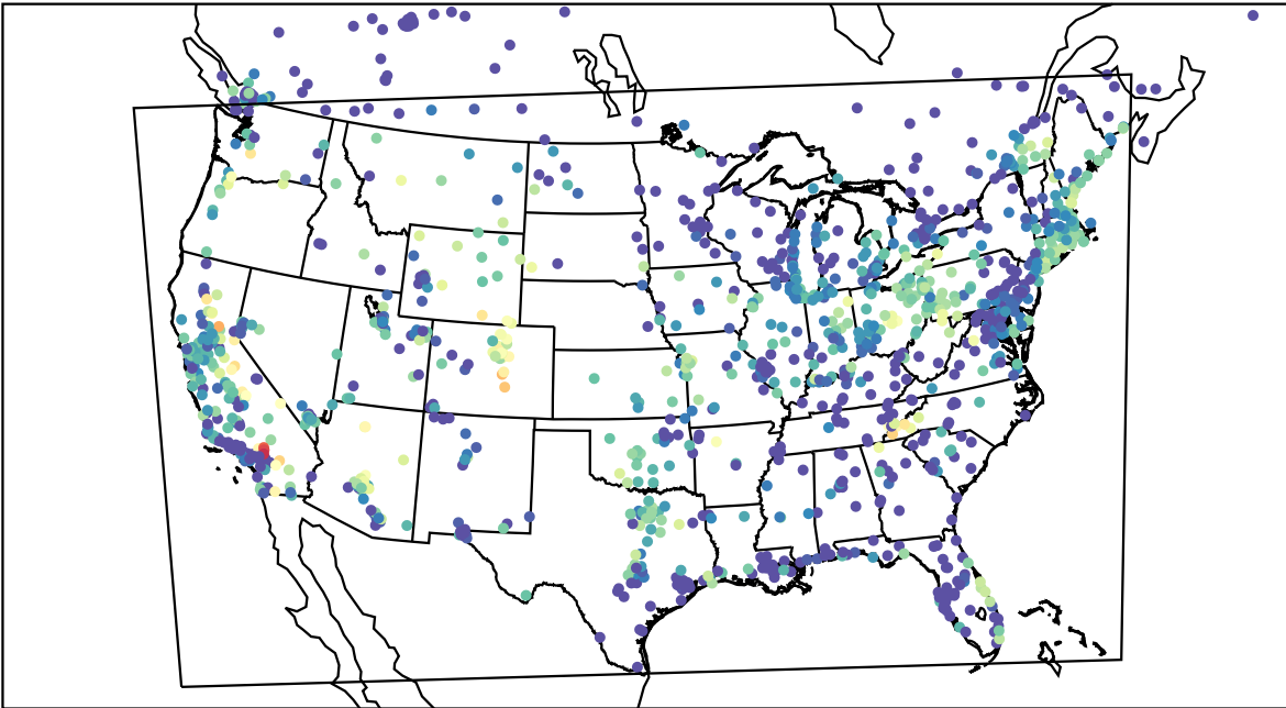
AirNOW (2023-08-25_08:00:00)
