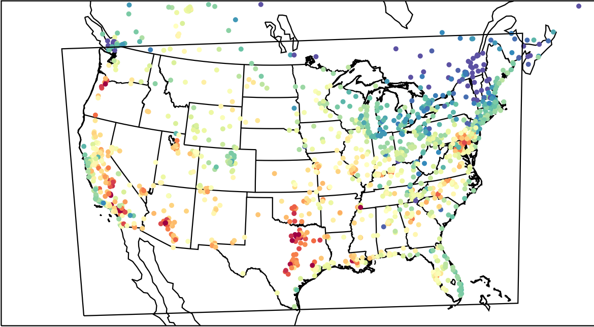
AirNOW (2023-08-25_22:00:00)
