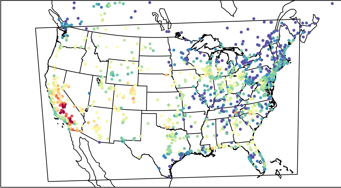
AirNOW (2023-08-24_01:00:00)
