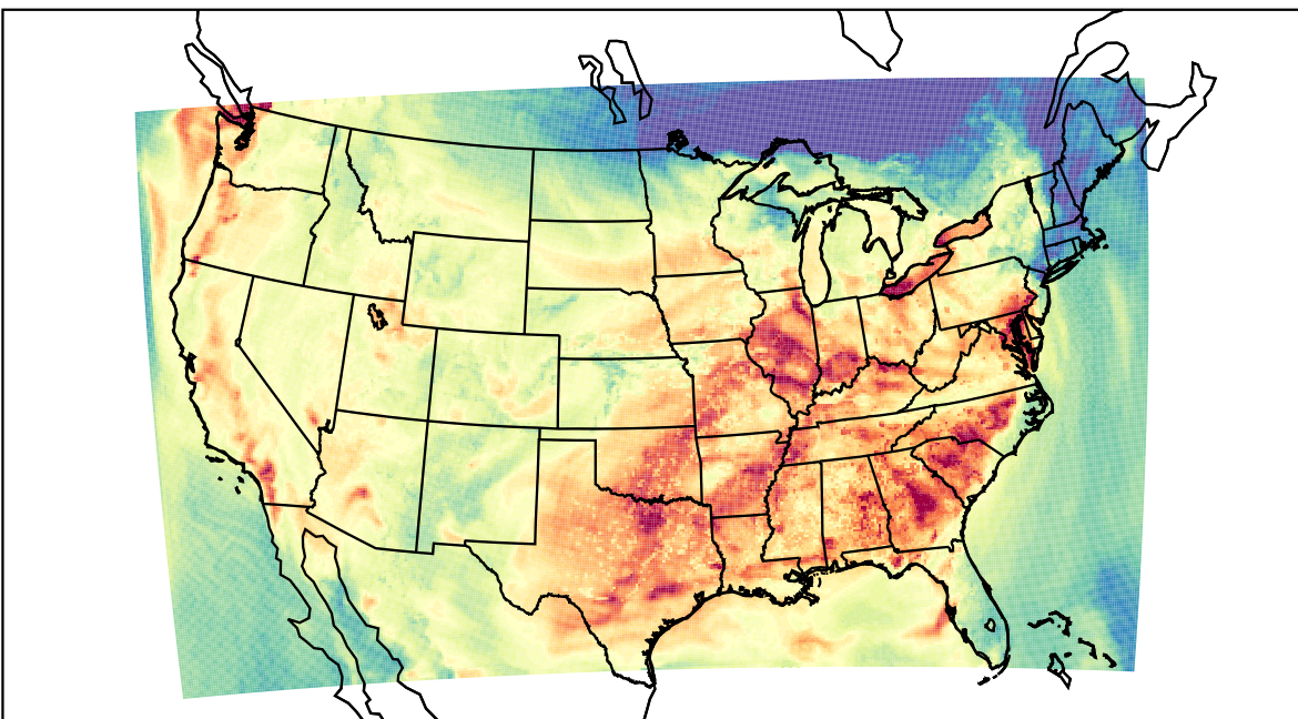
WRF (2023-08-25_23:00:00)
