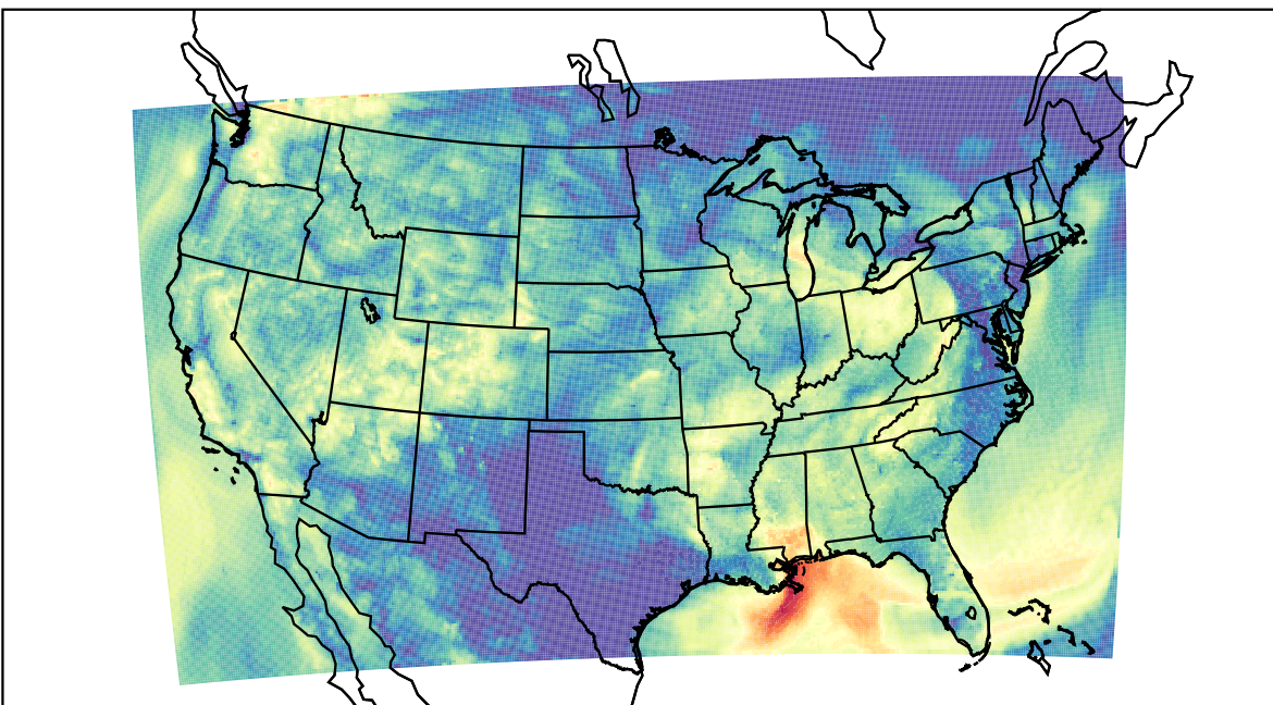
WRF (2023-08-24_13:00:00)
