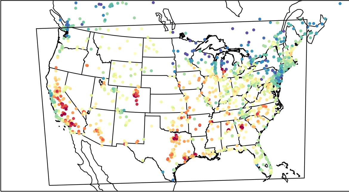
AirNOW (2023-08-24_20:00:00)
