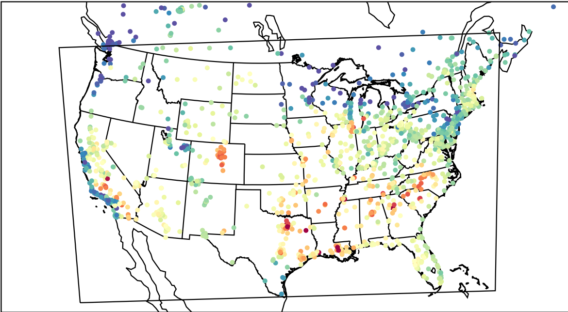
AirNOW (2023-08-24_17:00:00)
