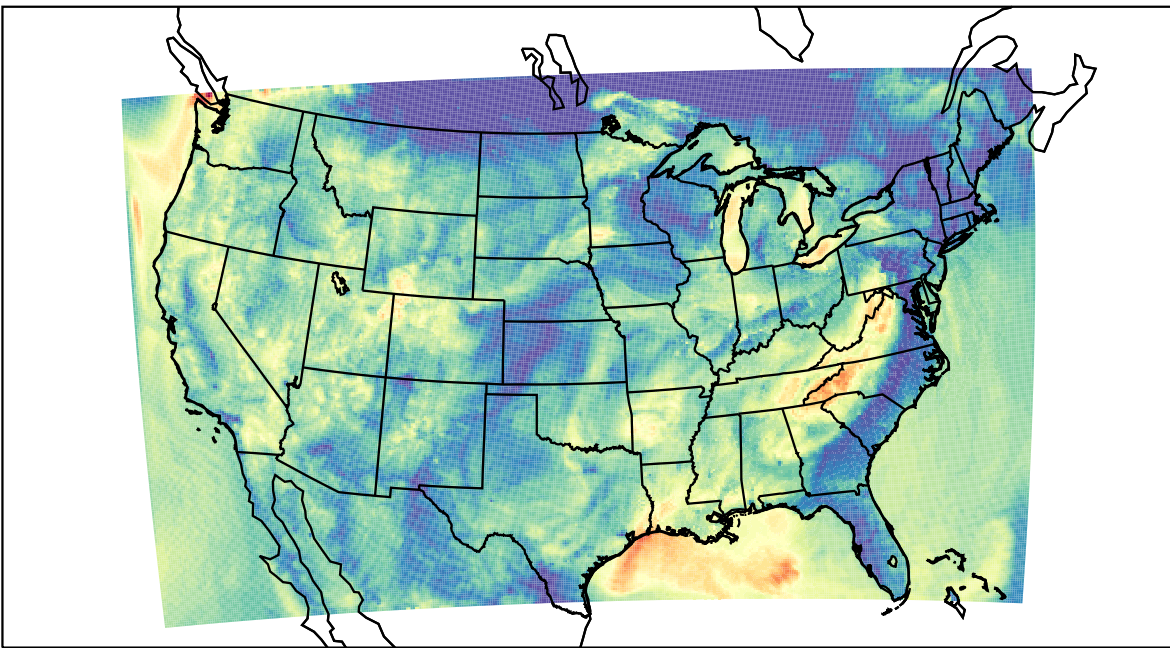
WRF (2023-08-25_11:00:00)
