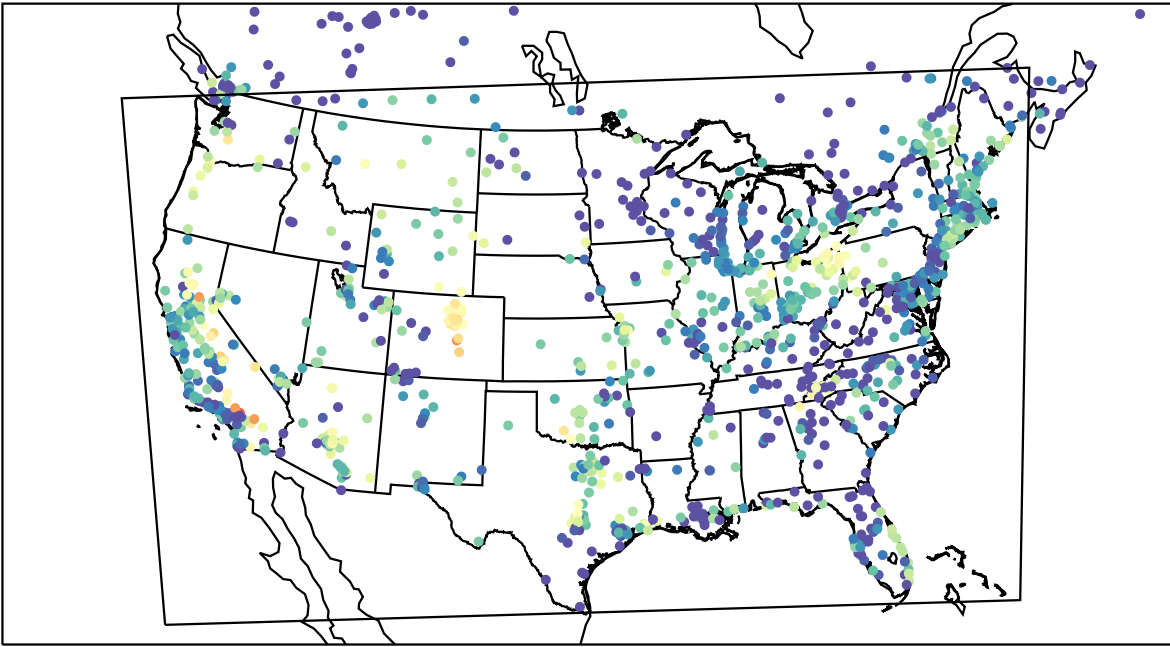
AirNOW (2023-08-25_06:00:00)
