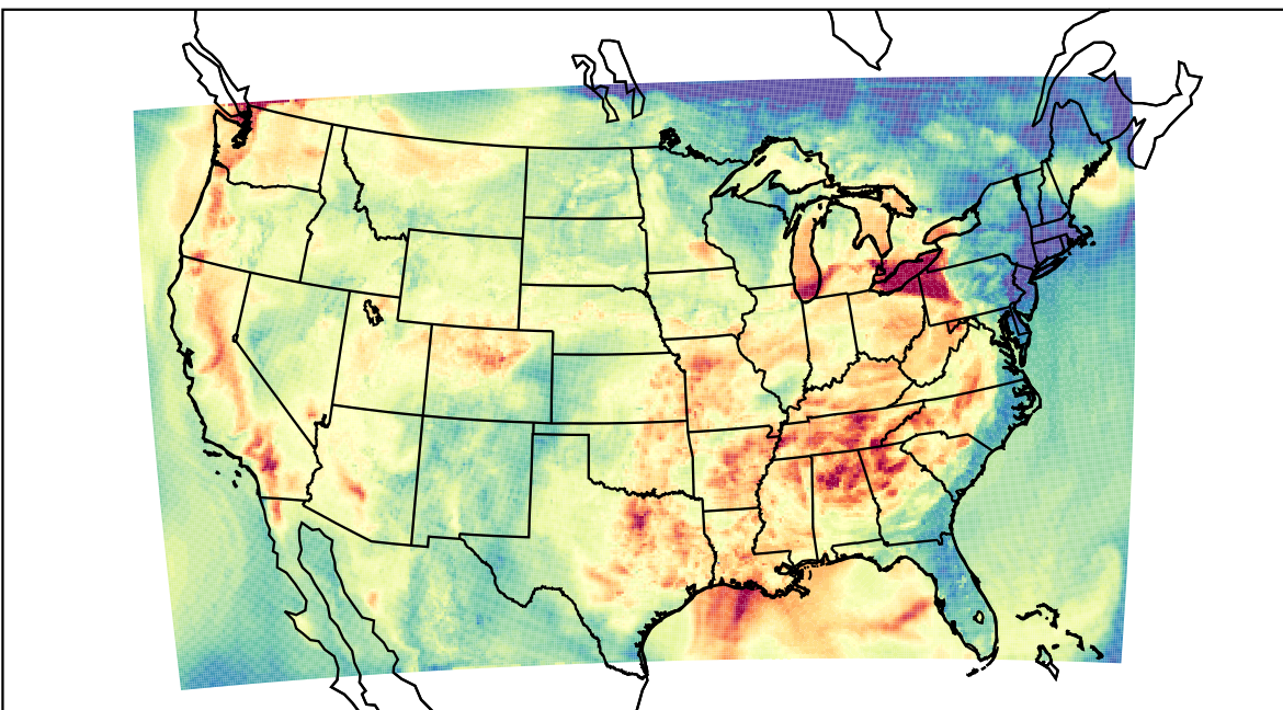
WRF (2023-08-25_01:00:00)
