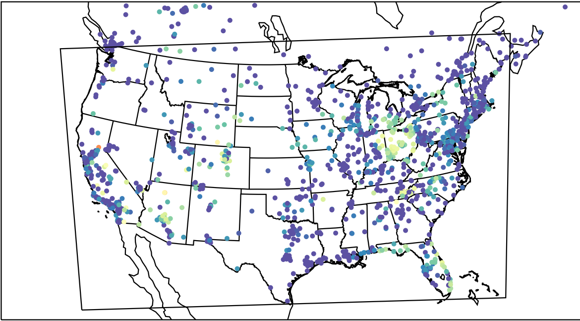
AirNOW (2023-08-24_12:00:00)
