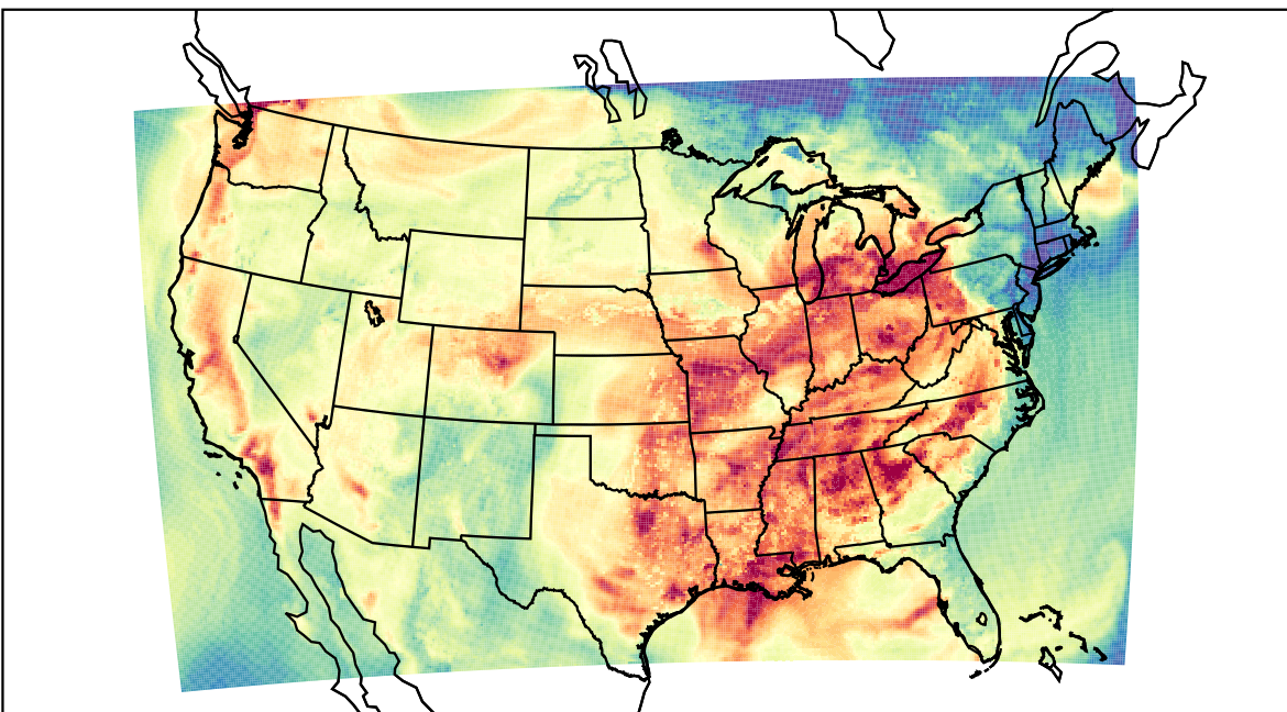
WRF (2023-08-24_23:00:00)
