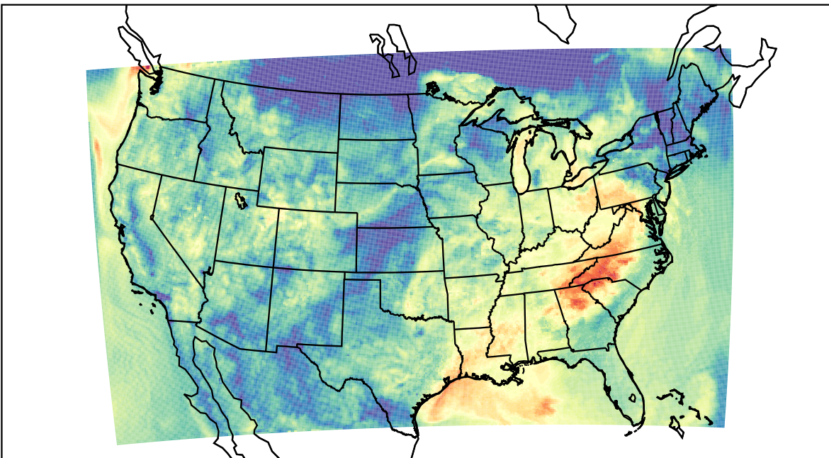
WRF (2023-08-25_14:00:00)
