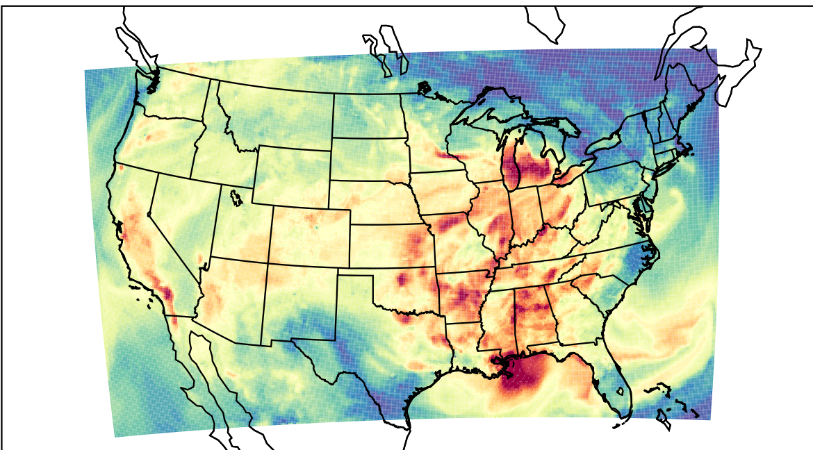
WRF (2023-08-24_01:00:00)
