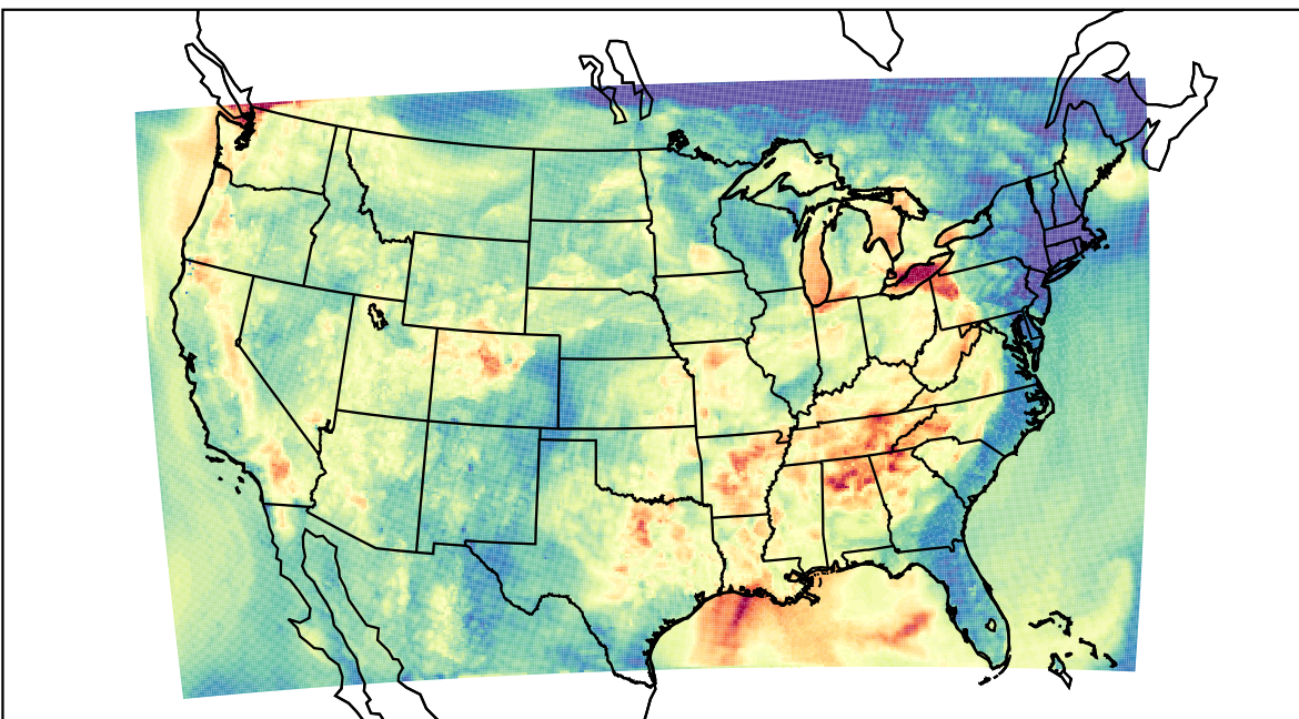
WRF (2023-08-25_03:00:00)
