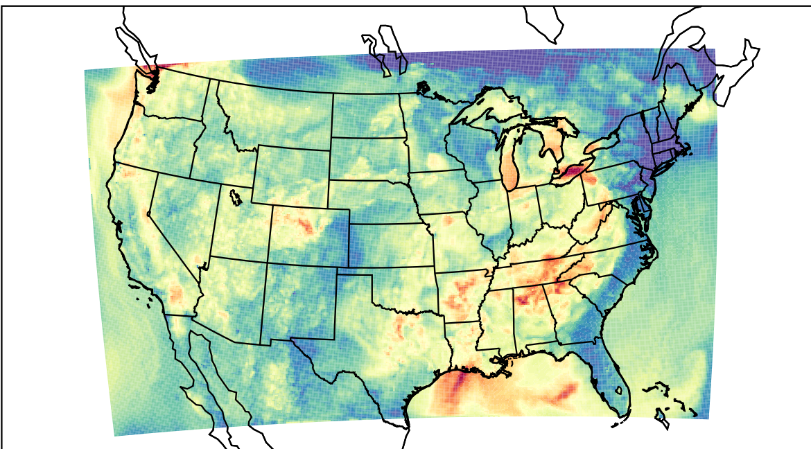
WRF (2023-08-25_04:00:00)
