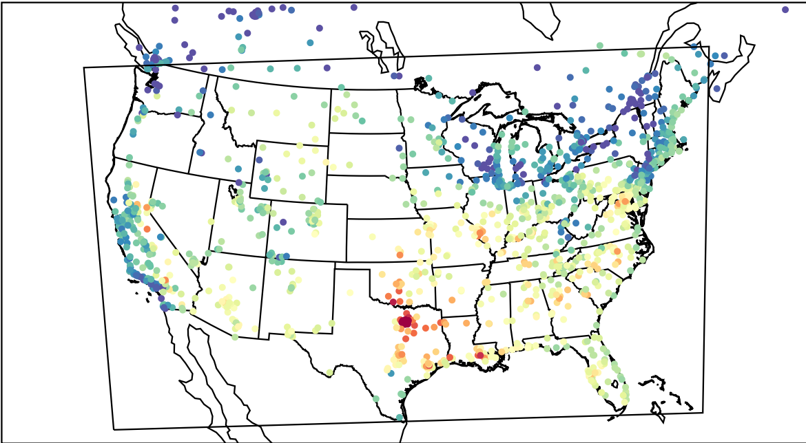
AirNOW (2023-08-25_16:00:00)
