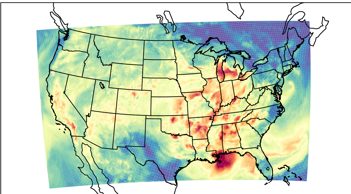
WRF (2023-08-24_02:00:00)
