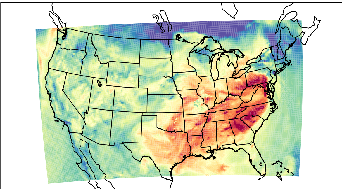
WRF (2023-08-25_16:00:00)
