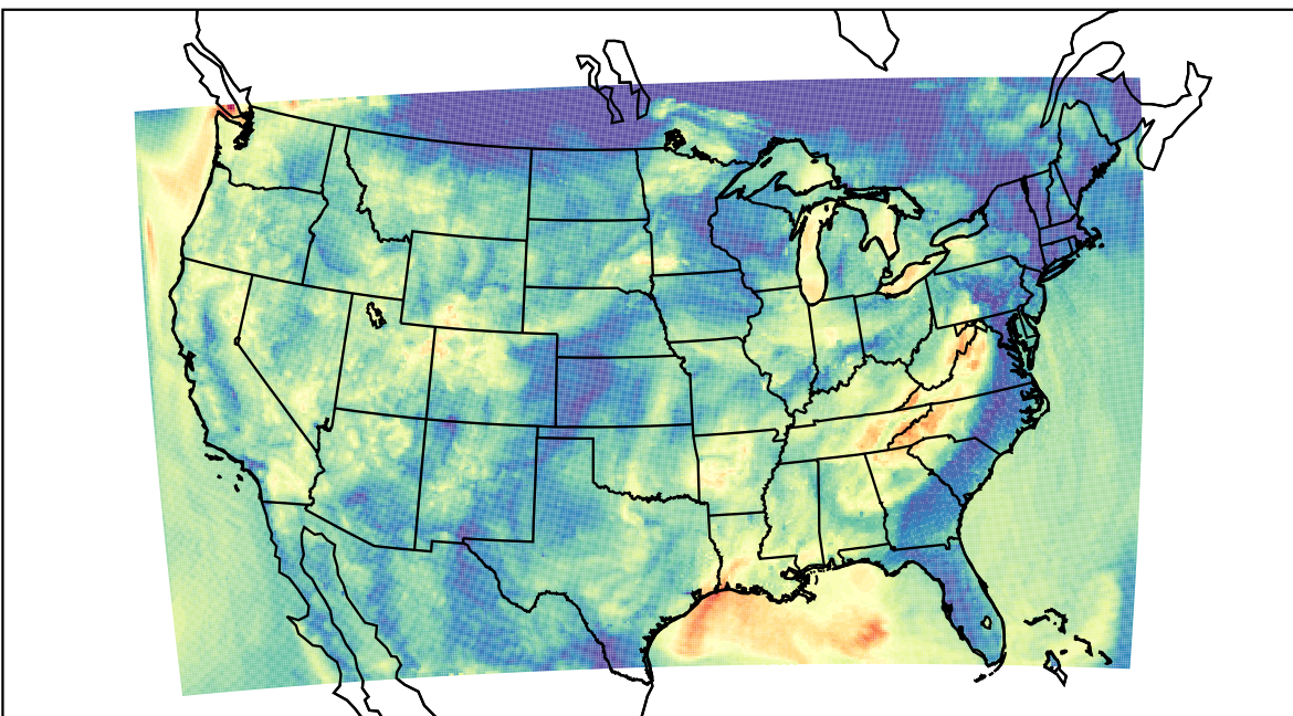
WRF (2023-08-25_10:00:00)
