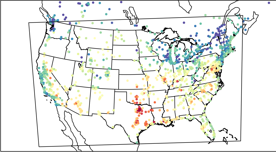
AirNOW (2023-08-25_17:00:00)
