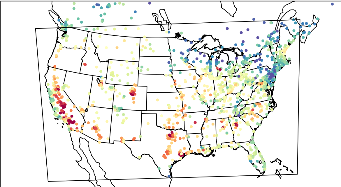
AirNOW (2023-08-24_22:00:00)
