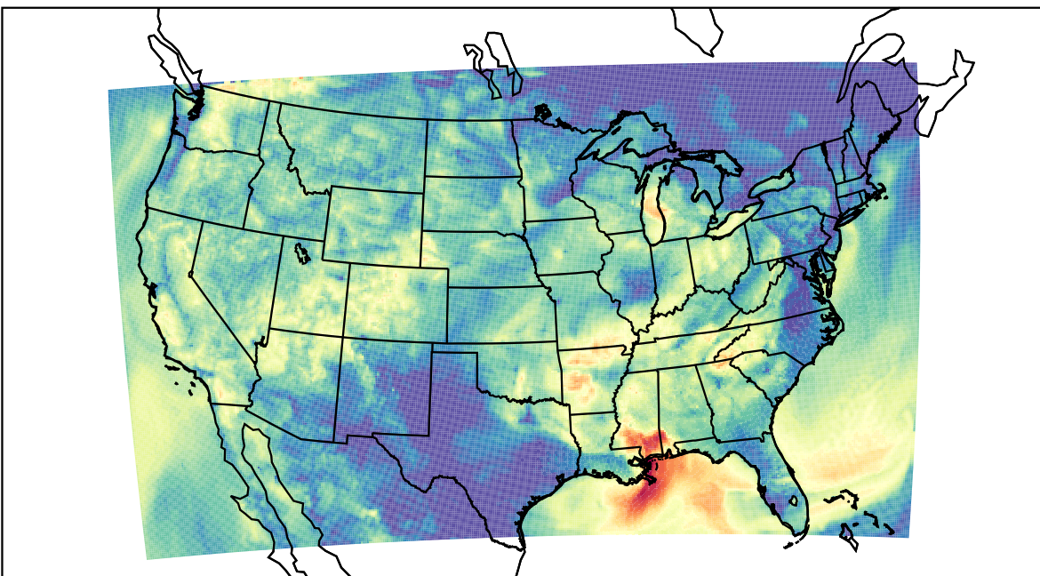
WRF (2023-08-24_11:00:00)
