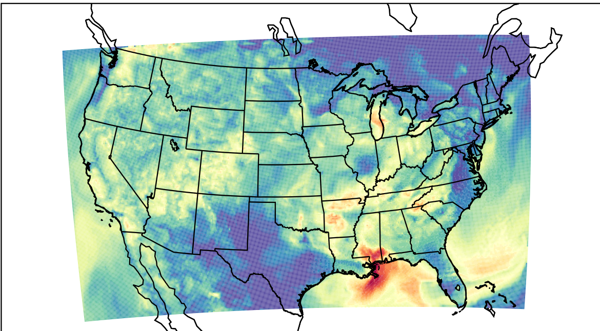
WRF (2023-08-24_10:00:00)
