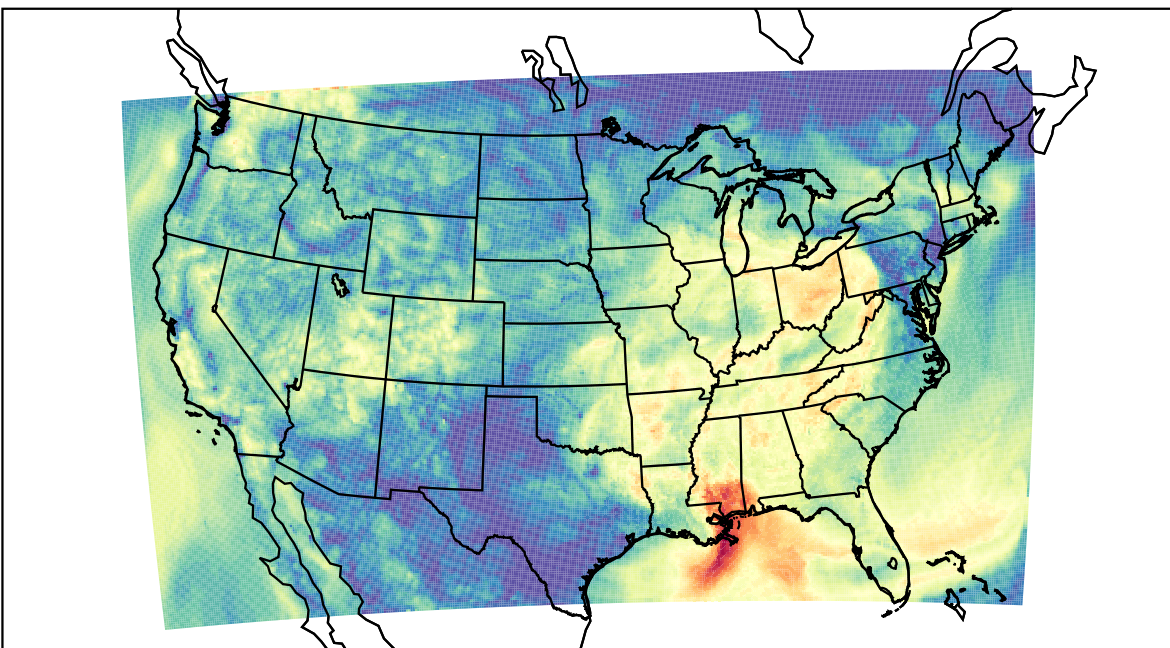
WRF (2023-08-24_14:00:00)
