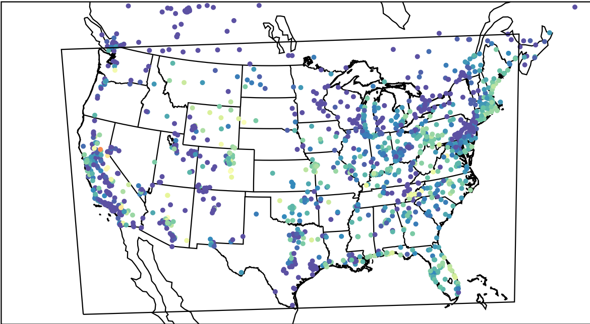
AirNOW (2023-08-25_13:00:00)
