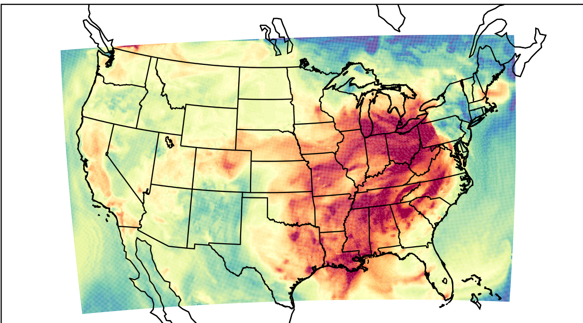
WRF (2023-08-24_19:00:00)
