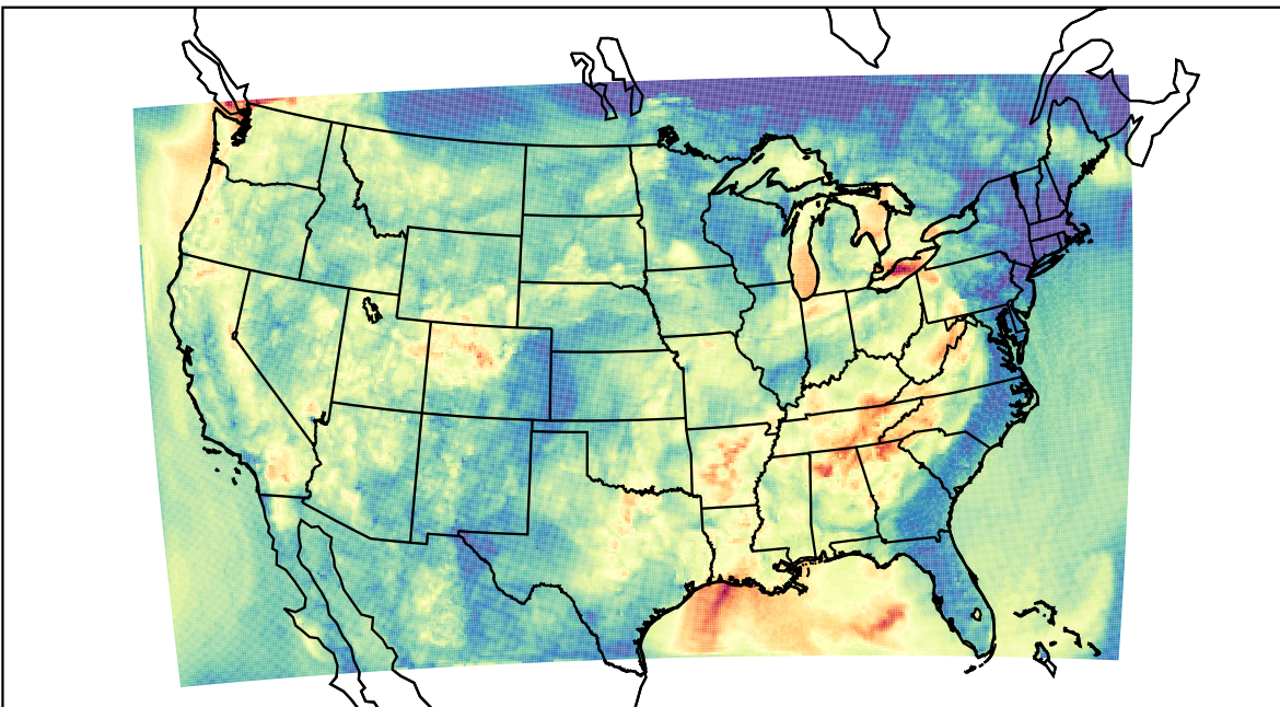
WRF (2023-08-25_05:00:00)
