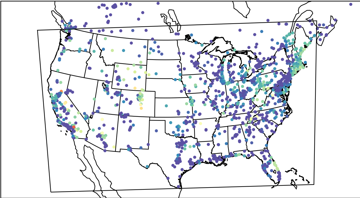
AirNOW (2023-08-25_12:00:00)
