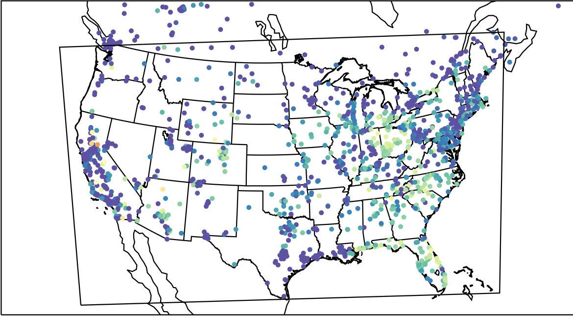
AirNOW (2023-08-24_13:00:00)
