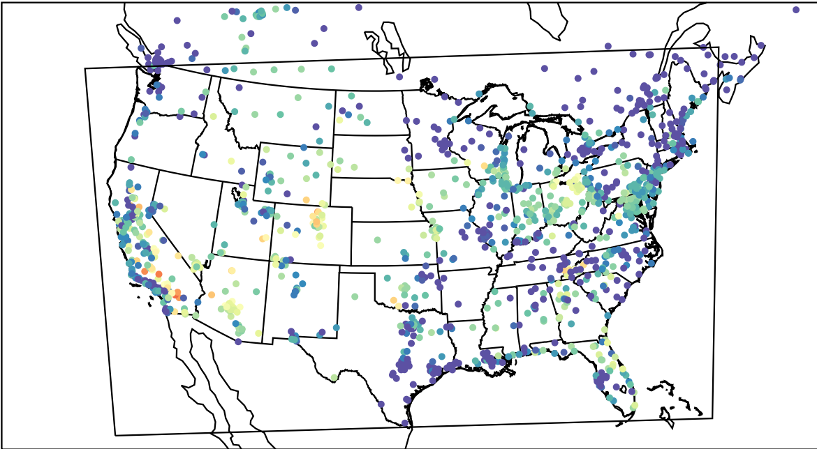
AirNOW (2023-08-24_05:00:00)
