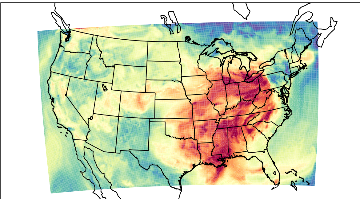
WRF (2023-08-24_17:00:00)
