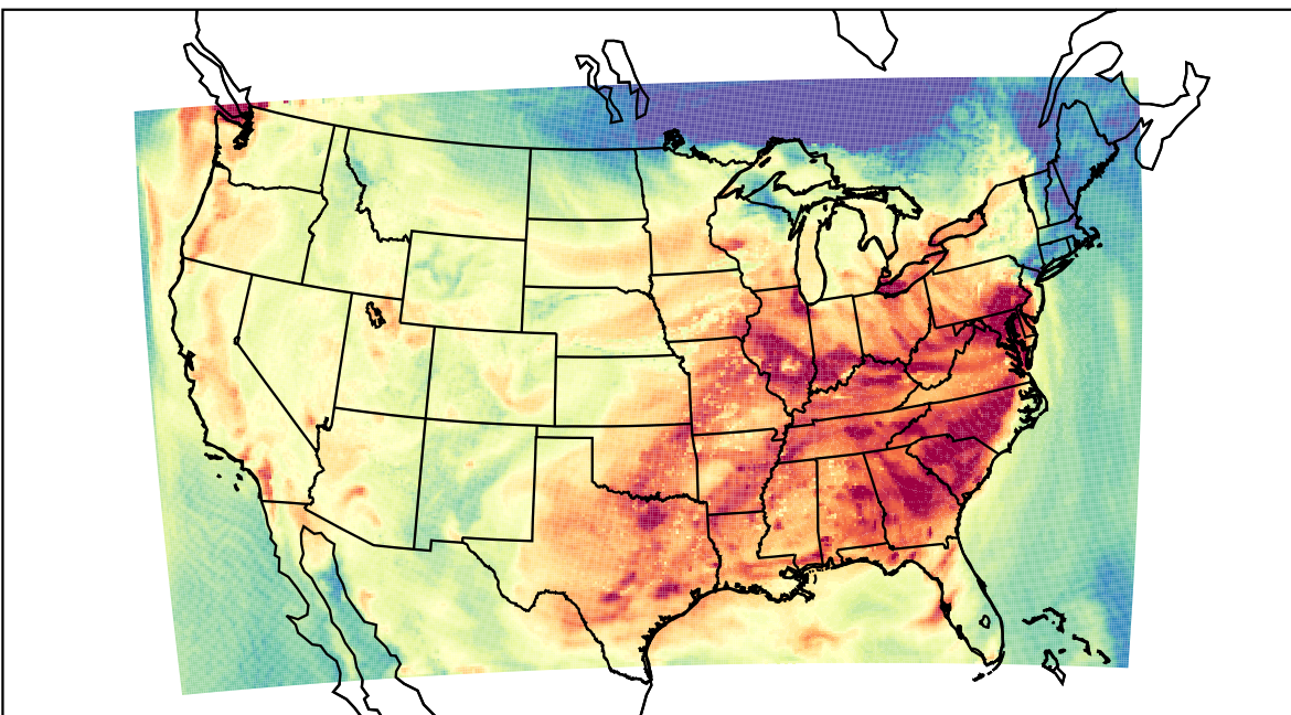
WRF (2023-08-25_21:00:00)
