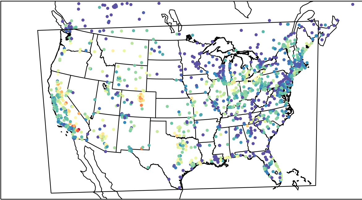
AirNOW (2023-08-25_04:00:00)
