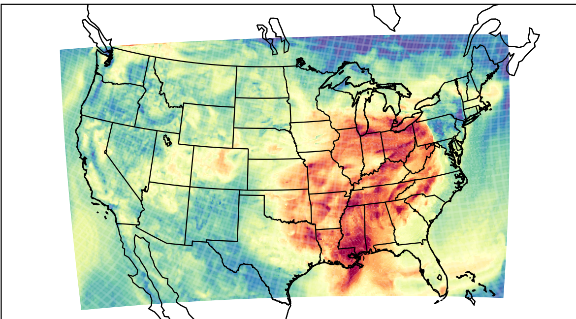
WRF (2023-08-24_16:00:00)
