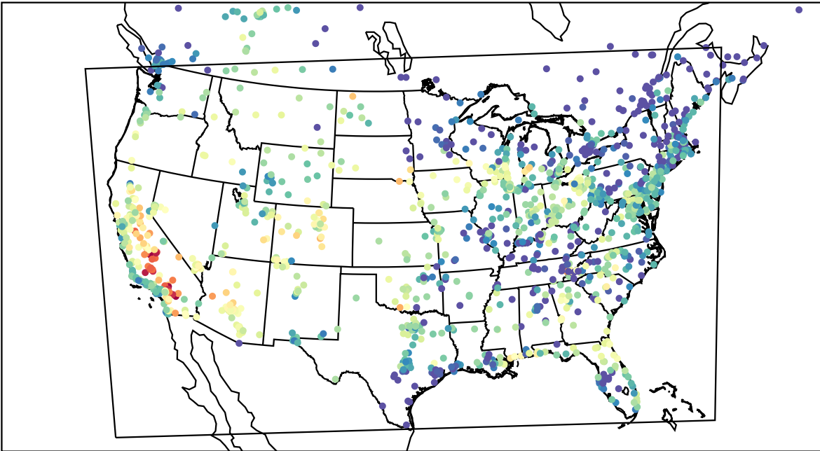
AirNOW (2023-08-24_02:00:00)
