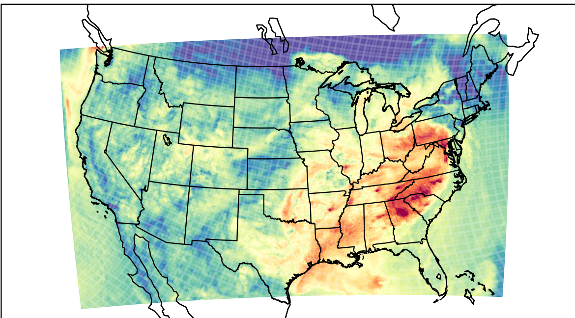
WRF (2023-08-25_15:00:00)
