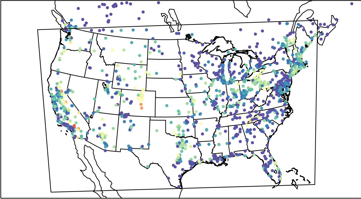
AirNOW (2023-08-25_07:00:00)
