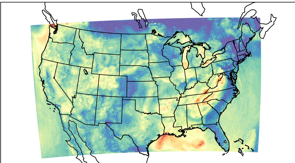
WRF (2023-08-25_08:00:00)
