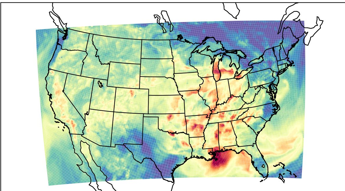
WRF (2023-08-24_03:00:00)
