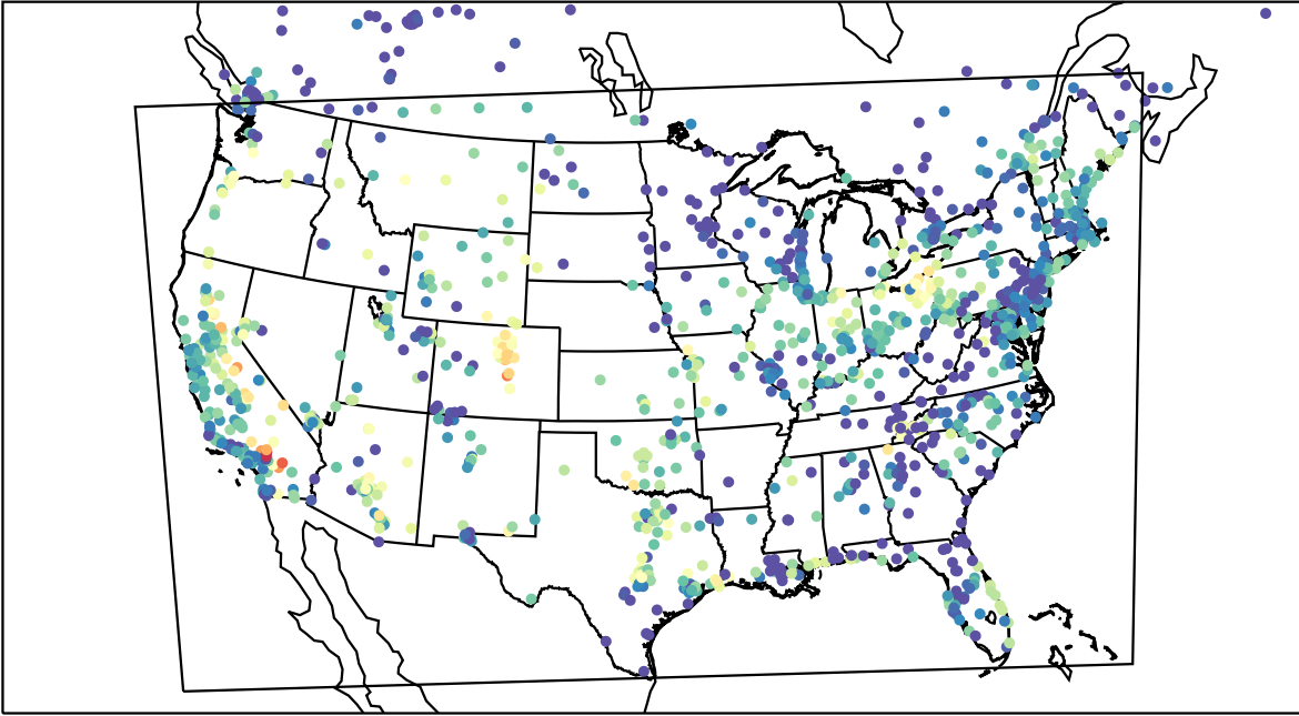
AirNOW (2023-08-25_05:00:00)
