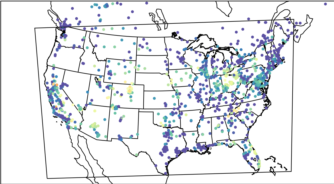
AirNOW (2023-08-24_08:00:00)
