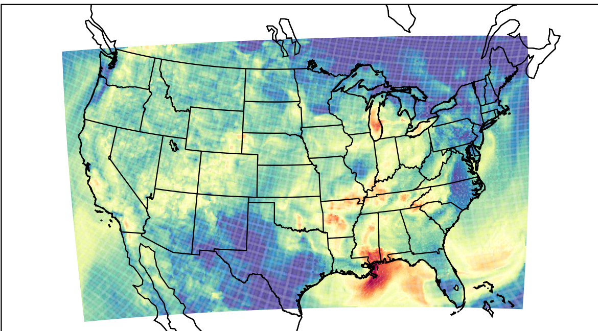
WRF (2023-08-24_08:00:00)
