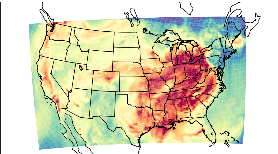
WRF (2023-08-24_22:00:00)
