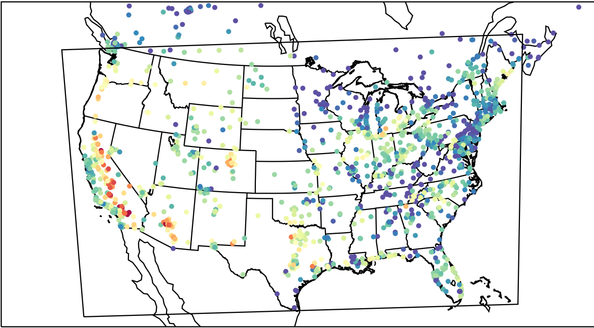
AirNOW (2023-08-25_02:00:00)
