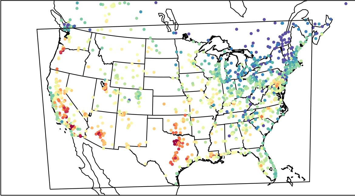
AirNOW (2023-08-25_23:00:00)
