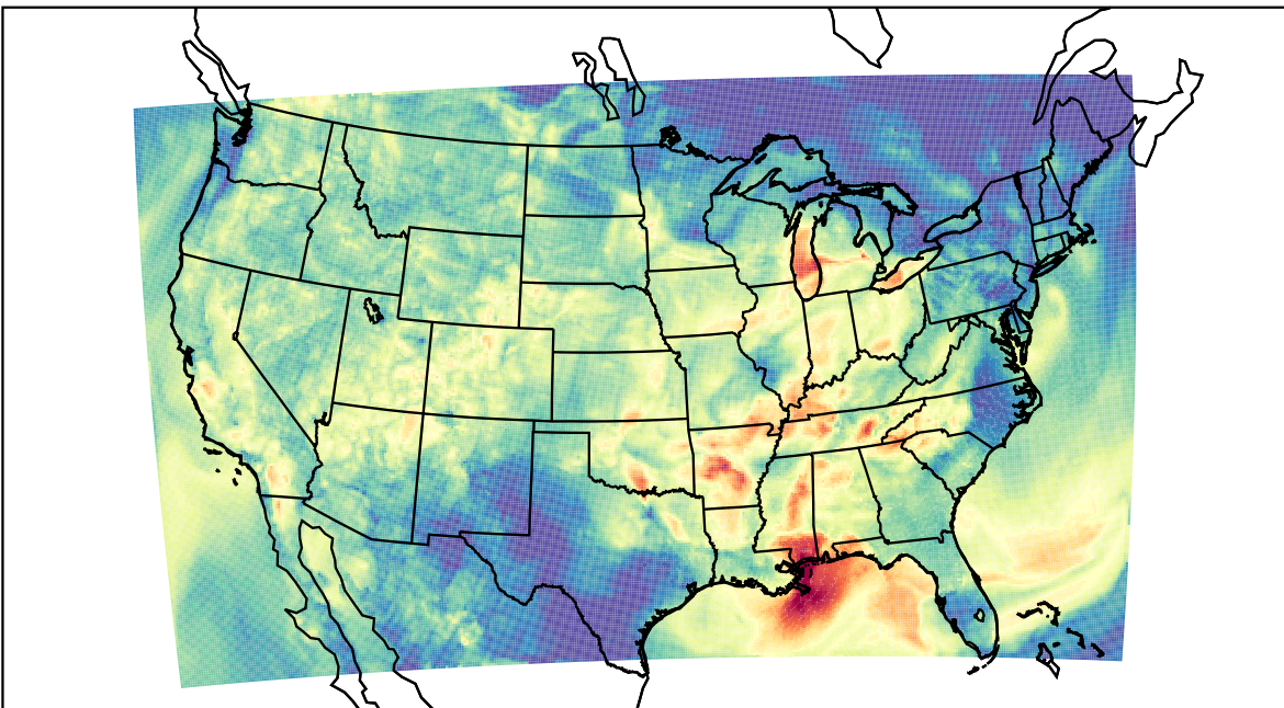
WRF (2023-08-24_06:00:00)
