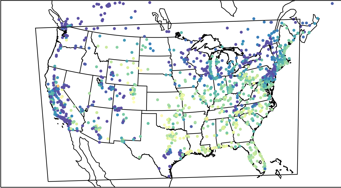
AirNOW (2023-08-25_14:00:00)
