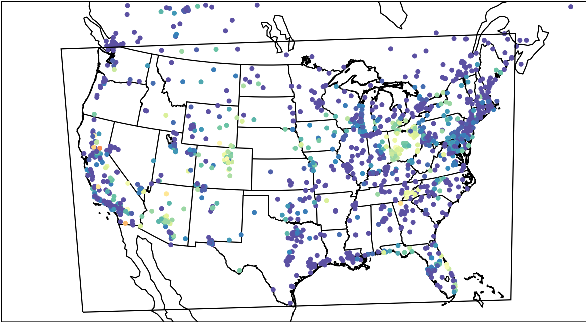
AirNOW (2023-08-24_11:00:00)
