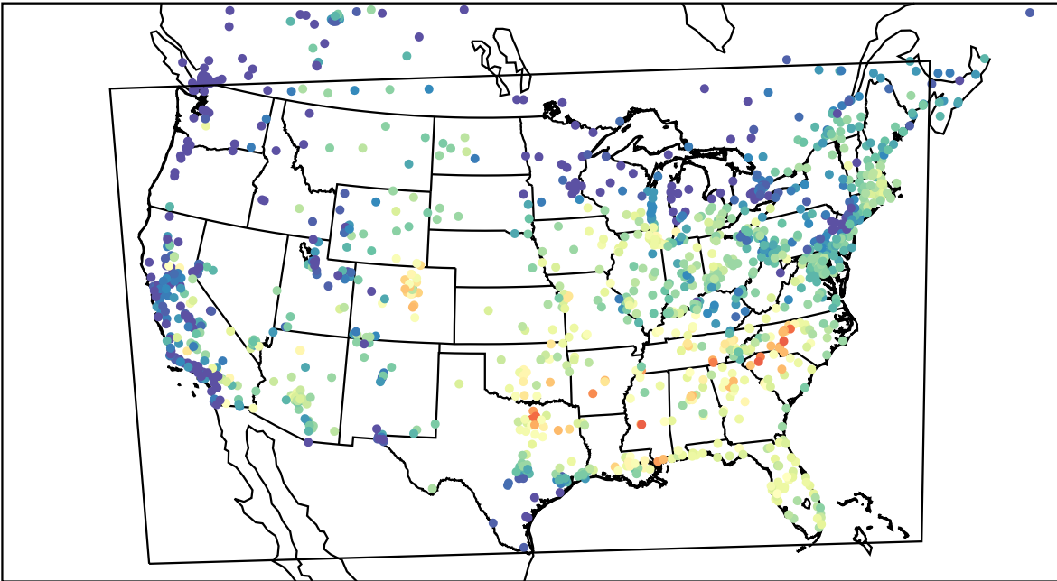
AirNOW (2023-08-24_15:00:00)
