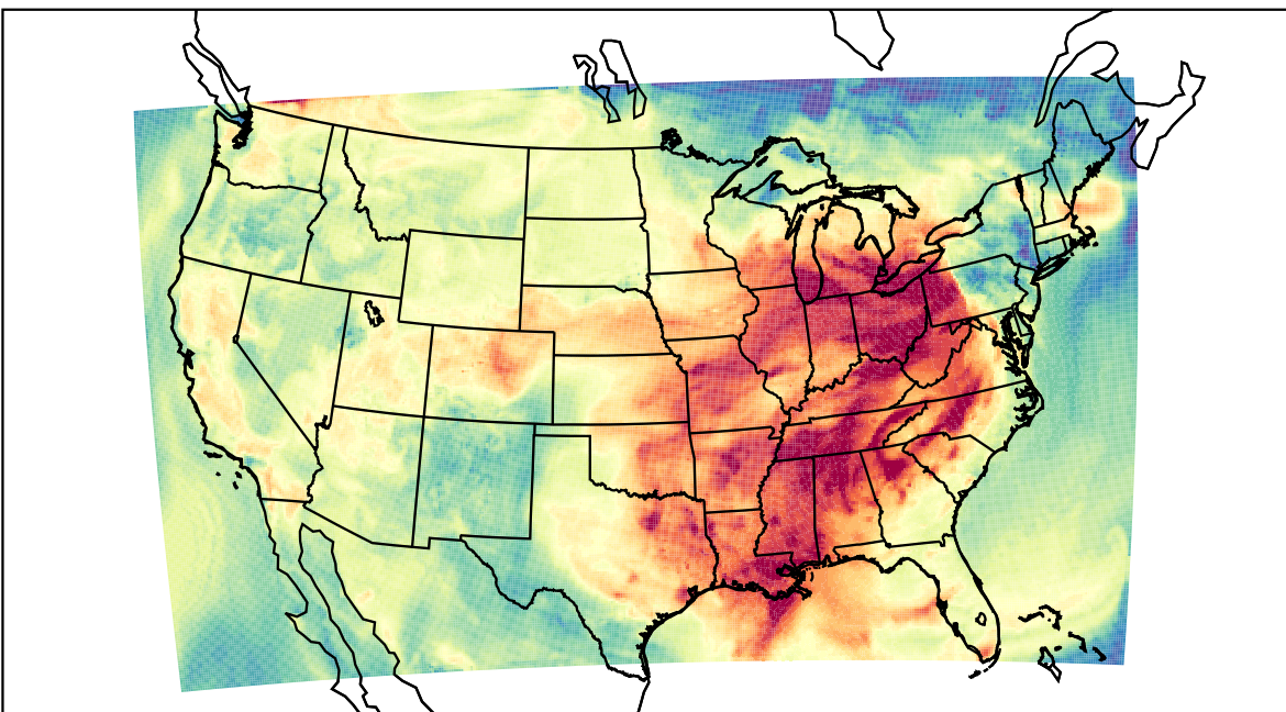
WRF (2023-08-24_18:00:00)
