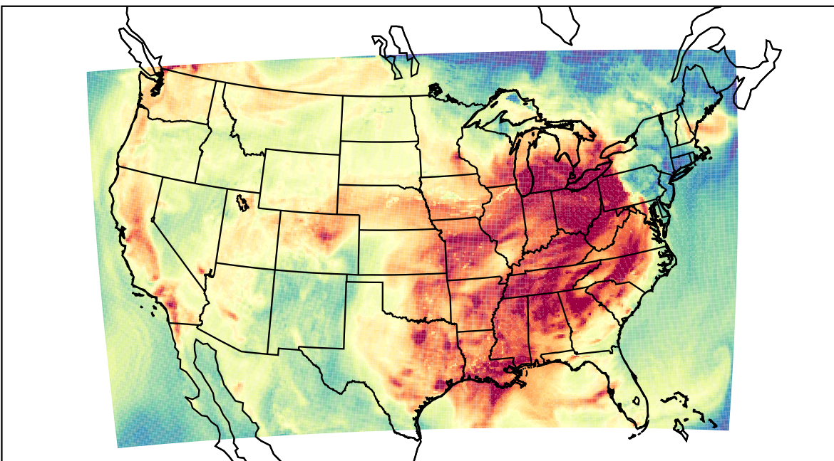
WRF (2023-08-24_21:00:00)
