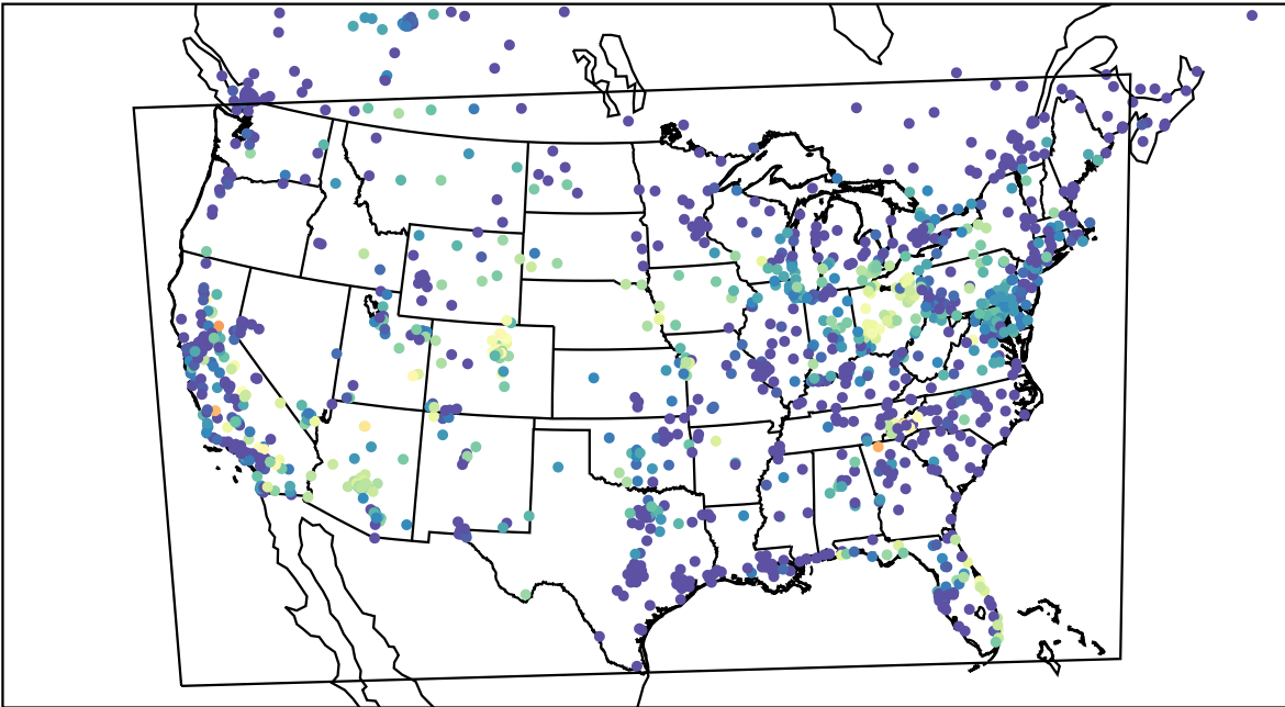
AirNOW (2023-08-24_09:00:00)
