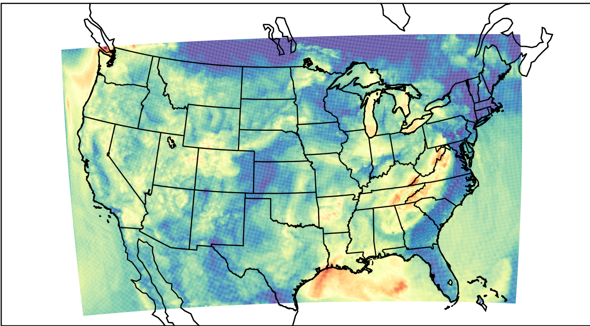
WRF (2023-08-25_09:00:00)
