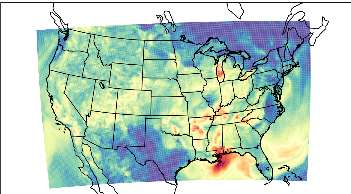
WRF (2023-08-24_07:00:00)
