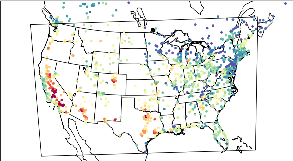
AirNOW (2023-08-25_00:00:00)
