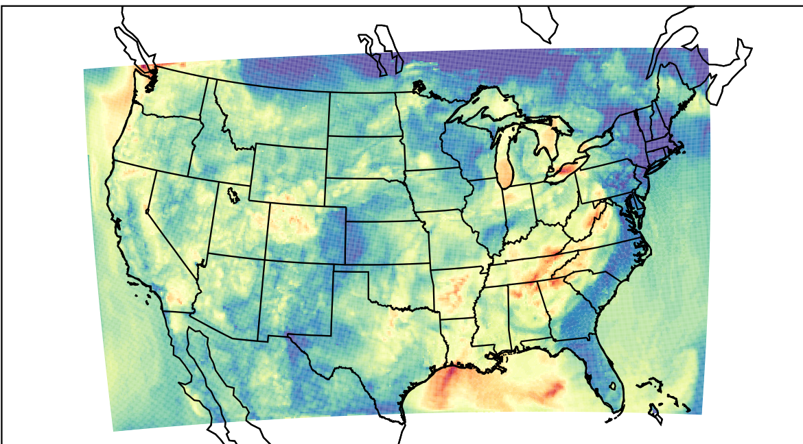
WRF (2023-08-25_06:00:00)
