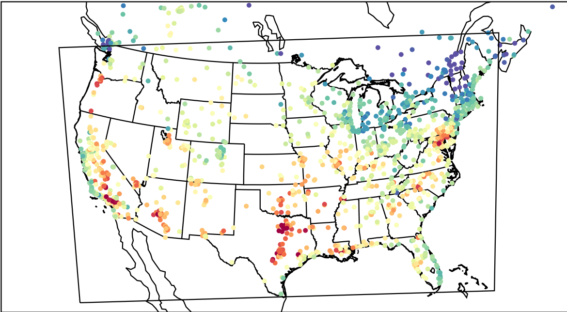
AirNOW (2023-08-25_21:00:00)
