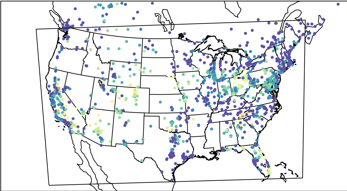
AirNOW (2023-08-24_07:00:00)
