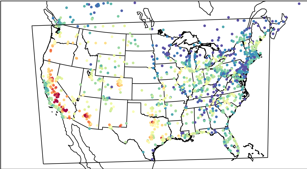
AirNOW (2023-08-25_01:00:00)
