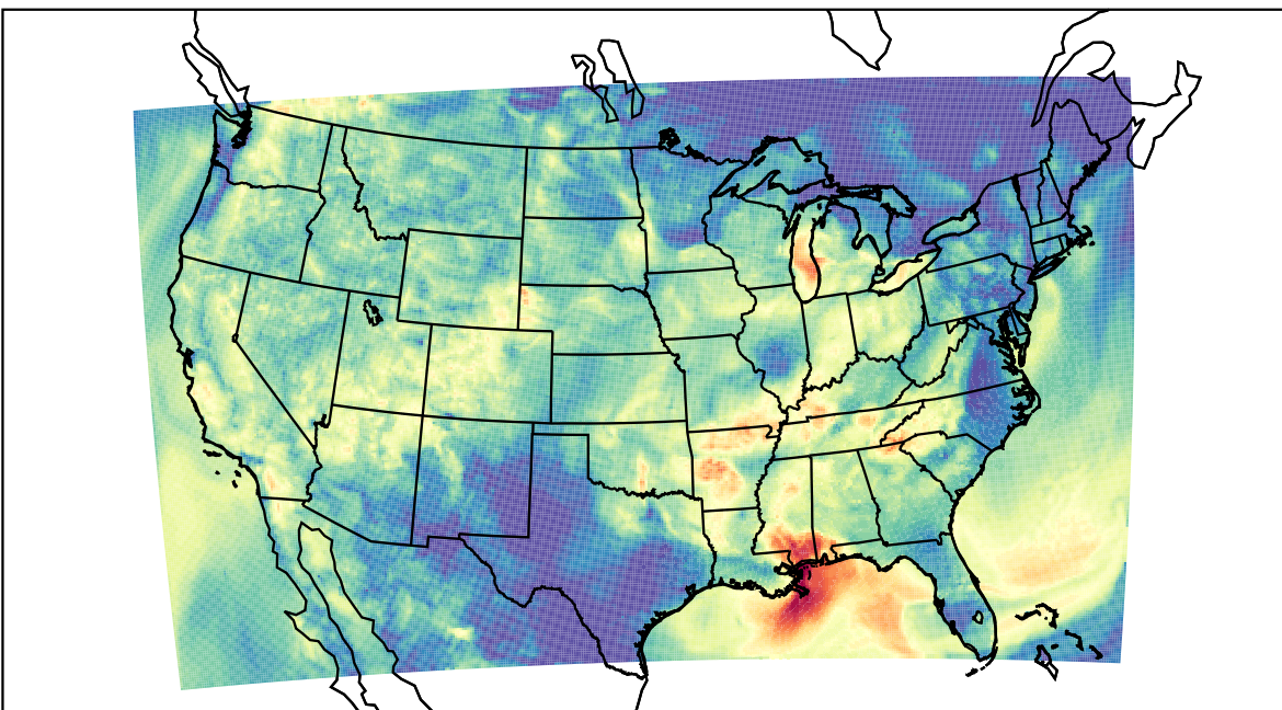
WRF (2023-08-24_09:00:00)
