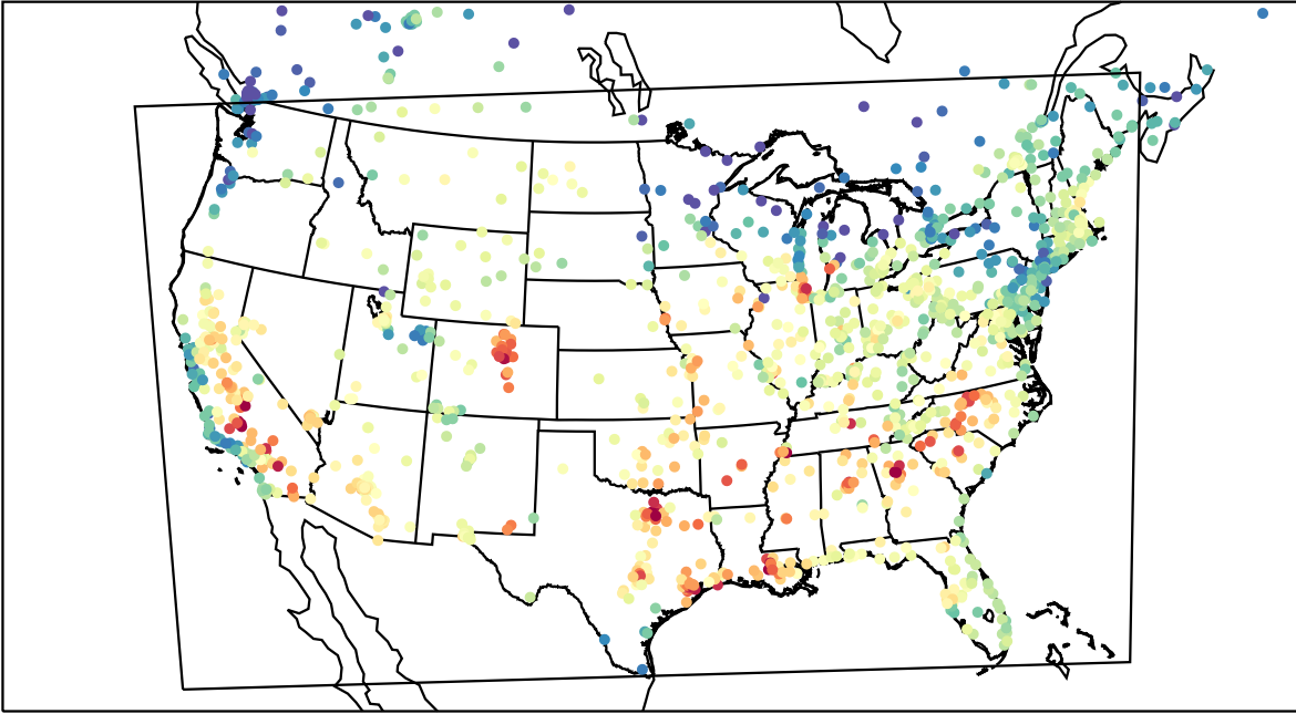
AirNOW (2023-08-24_18:00:00)
