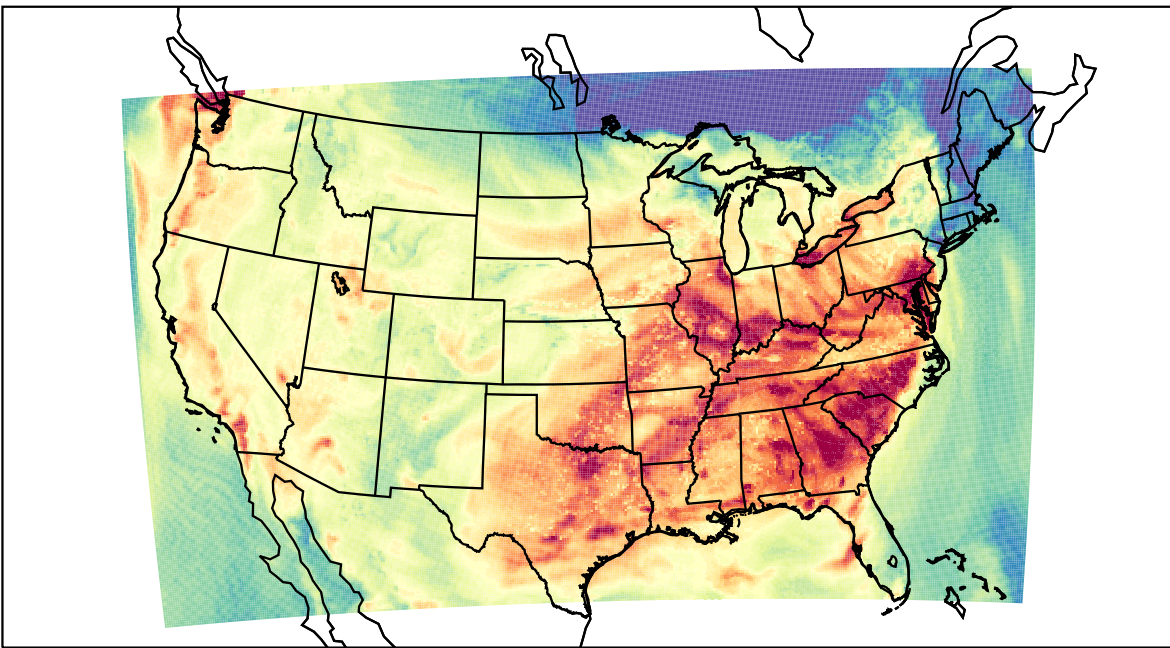
WRF (2023-08-25_22:00:00)
