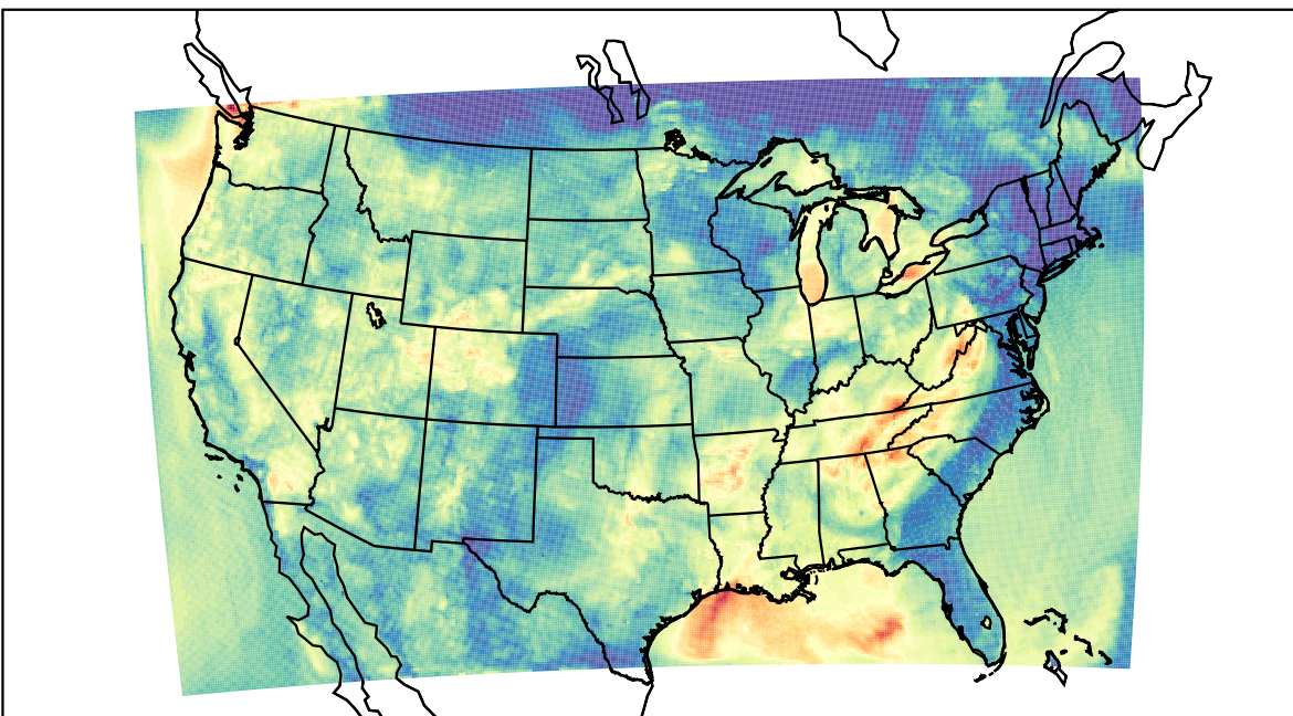
WRF (2023-08-25_07:00:00)
