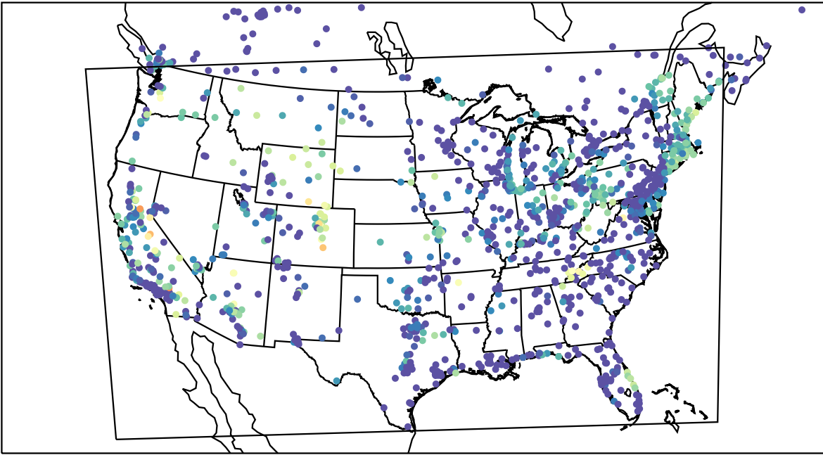
AirNOW (2023-08-25_11:00:00)
