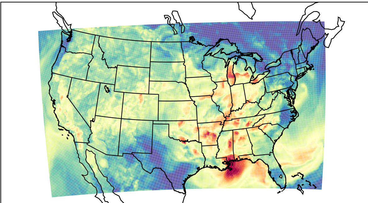
WRF (2023-08-24_04:00:00)
