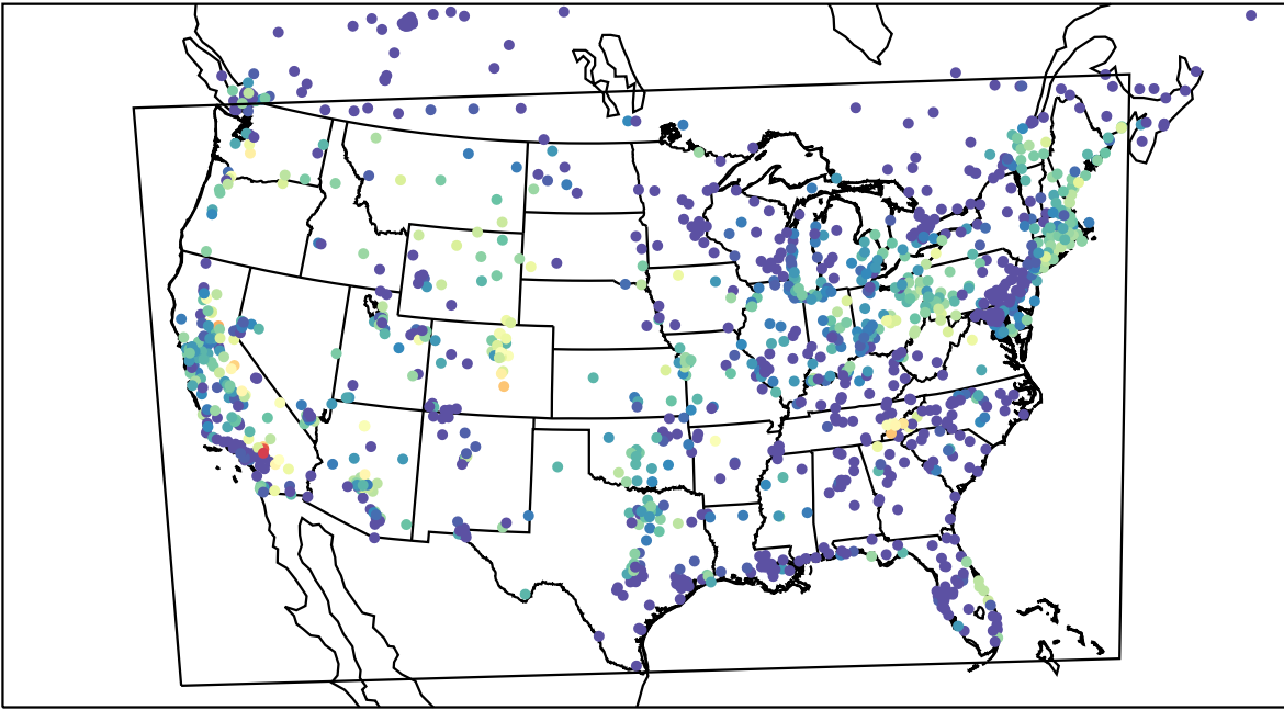
AirNOW (2023-08-25_09:00:00)
