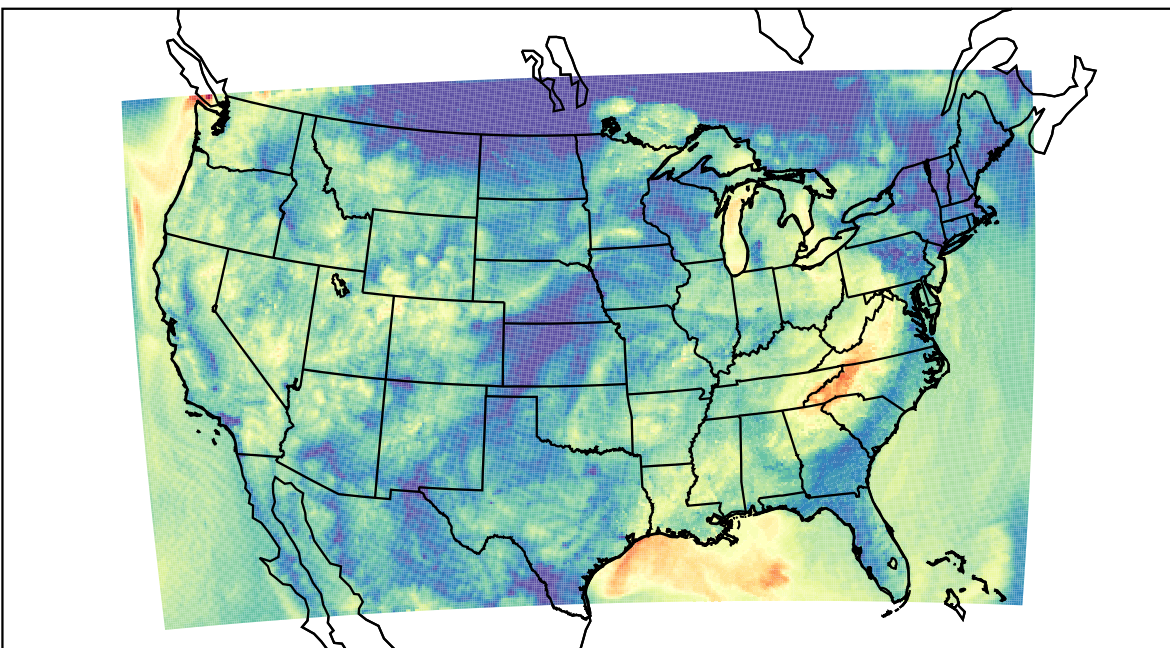
WRF (2023-08-25_13:00:00)
