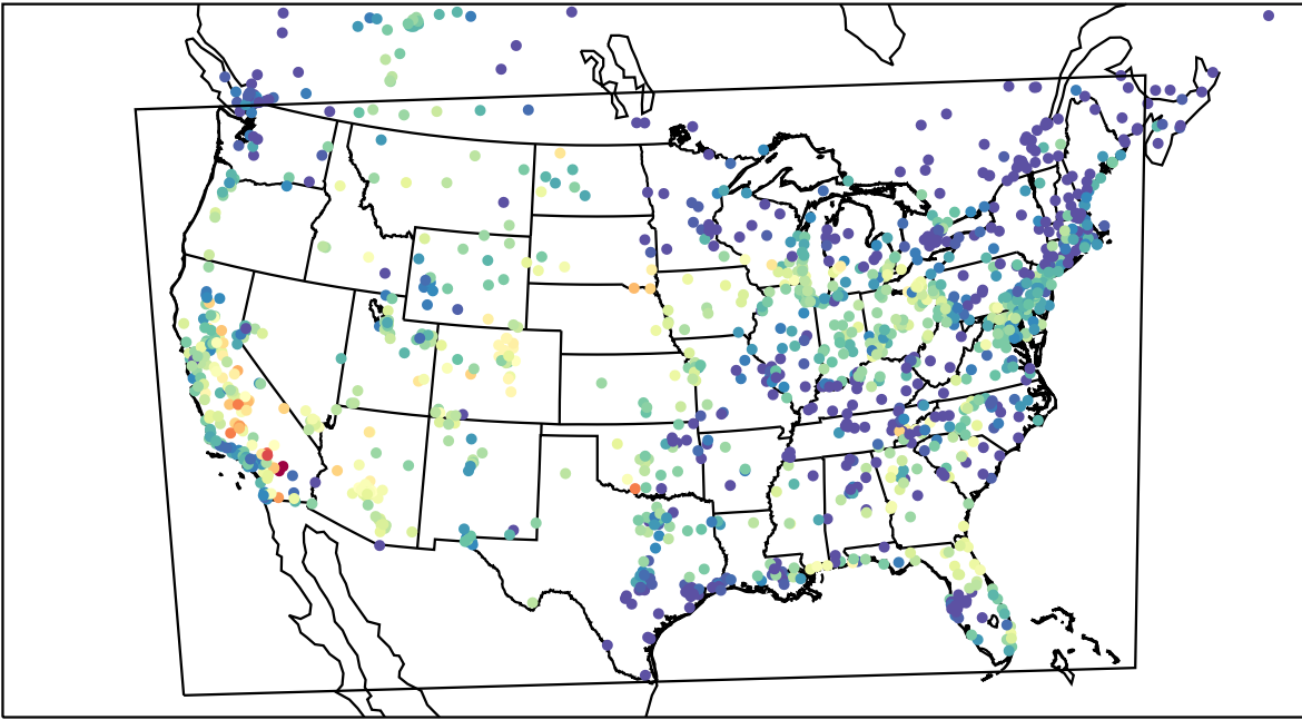
AirNOW (2023-08-24_03:00:00)
