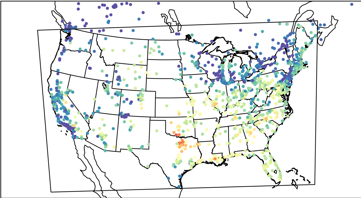
AirNOW (2023-08-25_15:00:00)
