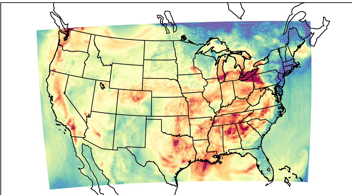
WRF (2023-08-25_00:00:00)
