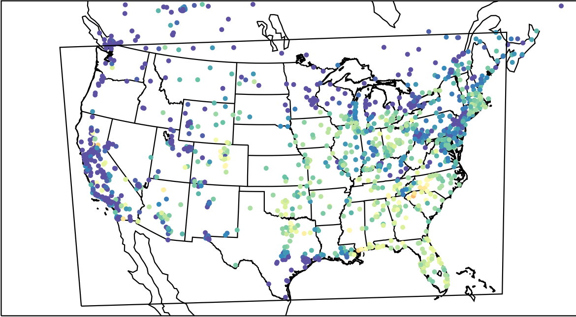
AirNOW (2023-08-24_14:00:00)
