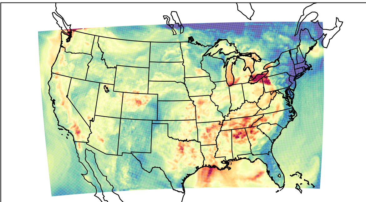
WRF (2023-08-25_02:00:00)
