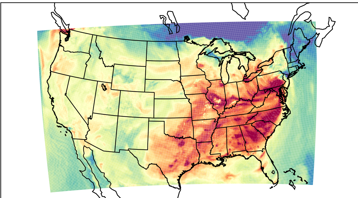
WRF (2023-08-25_19:00:00)
