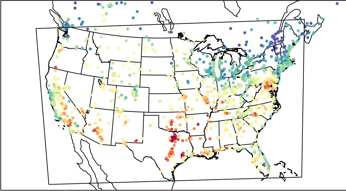
AirNOW (2023-08-25_19:00:00)
