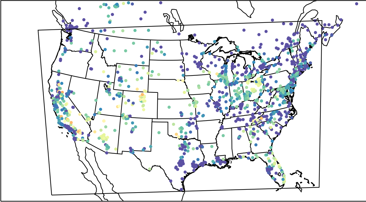
AirNOW (2023-08-24_06:00:00)
