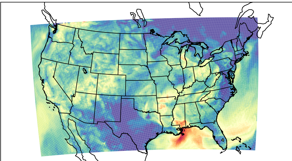
WRF (2023-08-24_12:00:00)
