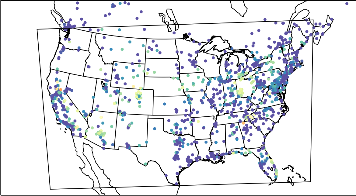
AirNOW (2023-08-24_10:00:00)
