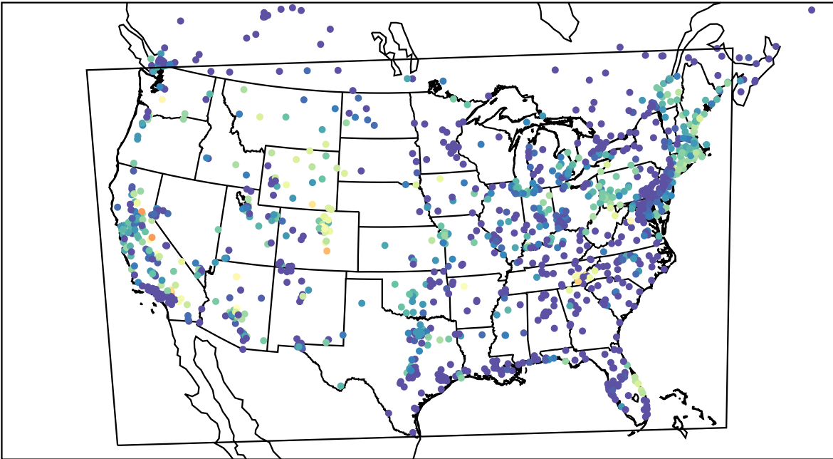
AirNOW (2023-08-25_10:00:00)
