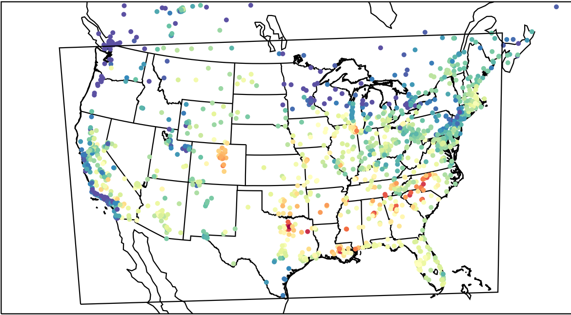
AirNOW (2023-08-24_16:00:00)
