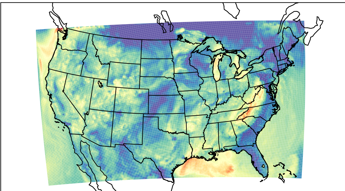
WRF (2023-08-25_12:00:00)
