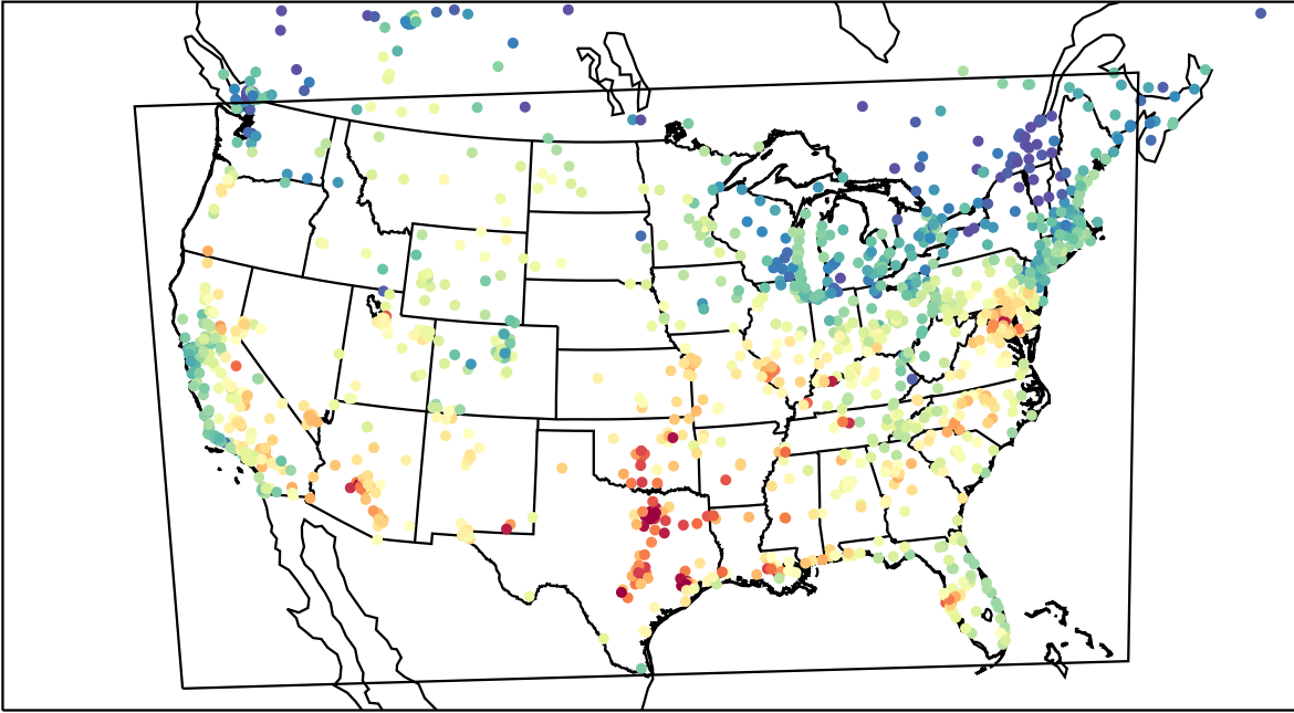
AirNOW (2023-08-25_18:00:00)
