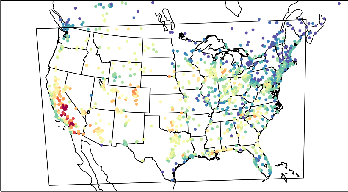
AirNOW (2023-08-24_00:00:00)
