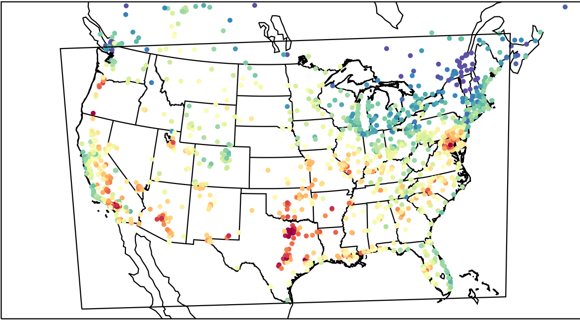
AirNOW (2023-08-25_20:00:00)
