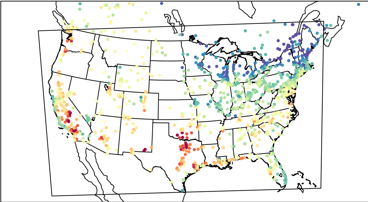
AirNOW (2023-08-26_21:00:00)
