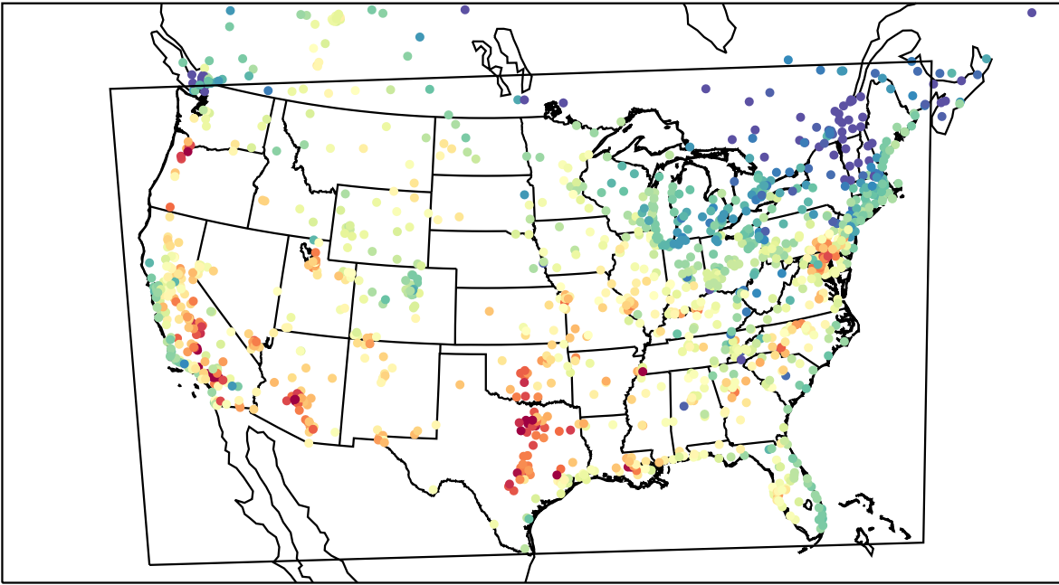
AirNOW (2023-08-25_22:00:00)
