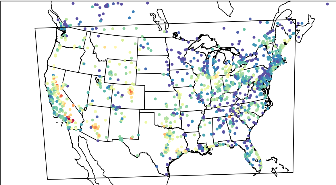
AirNOW (2023-08-25_03:00:00)
