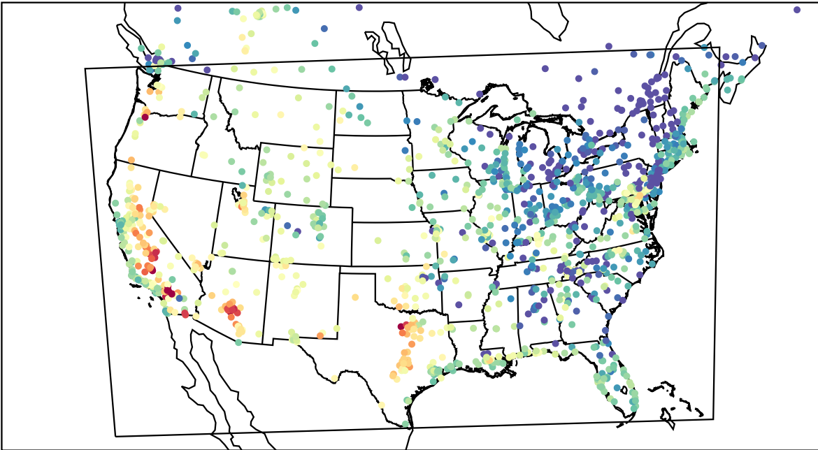
AirNOW (2023-08-26_01:00:00)
