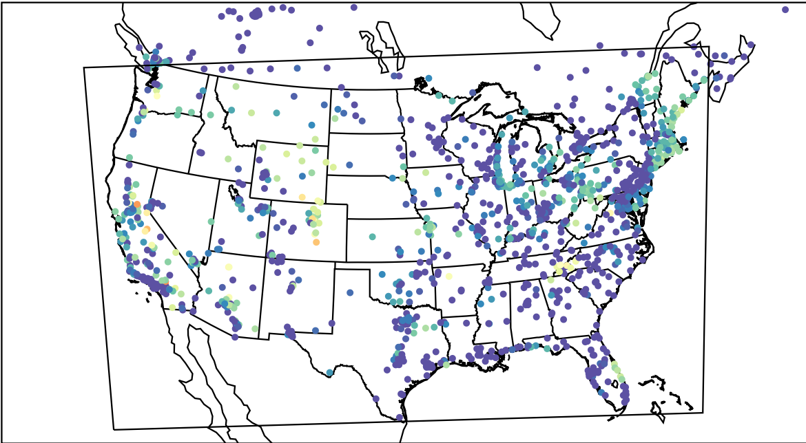
AirNOW (2023-08-25_11:00:00)
