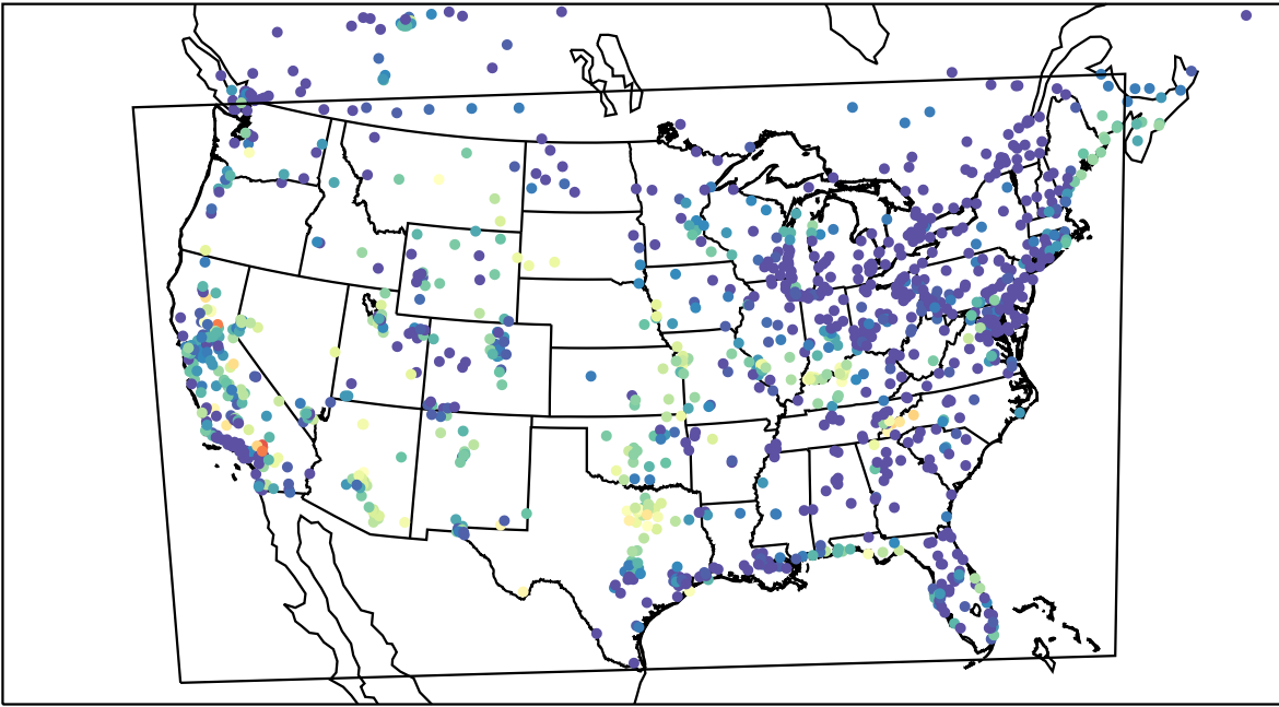
AirNOW (2023-08-26_08:00:00)
