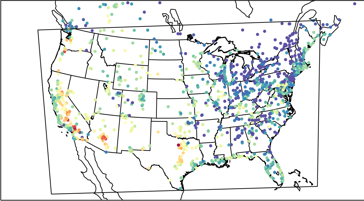
AirNOW (2023-08-26_02:00:00)
