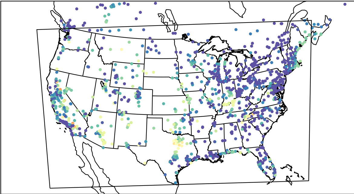
AirNOW (2023-08-26_07:00:00)
