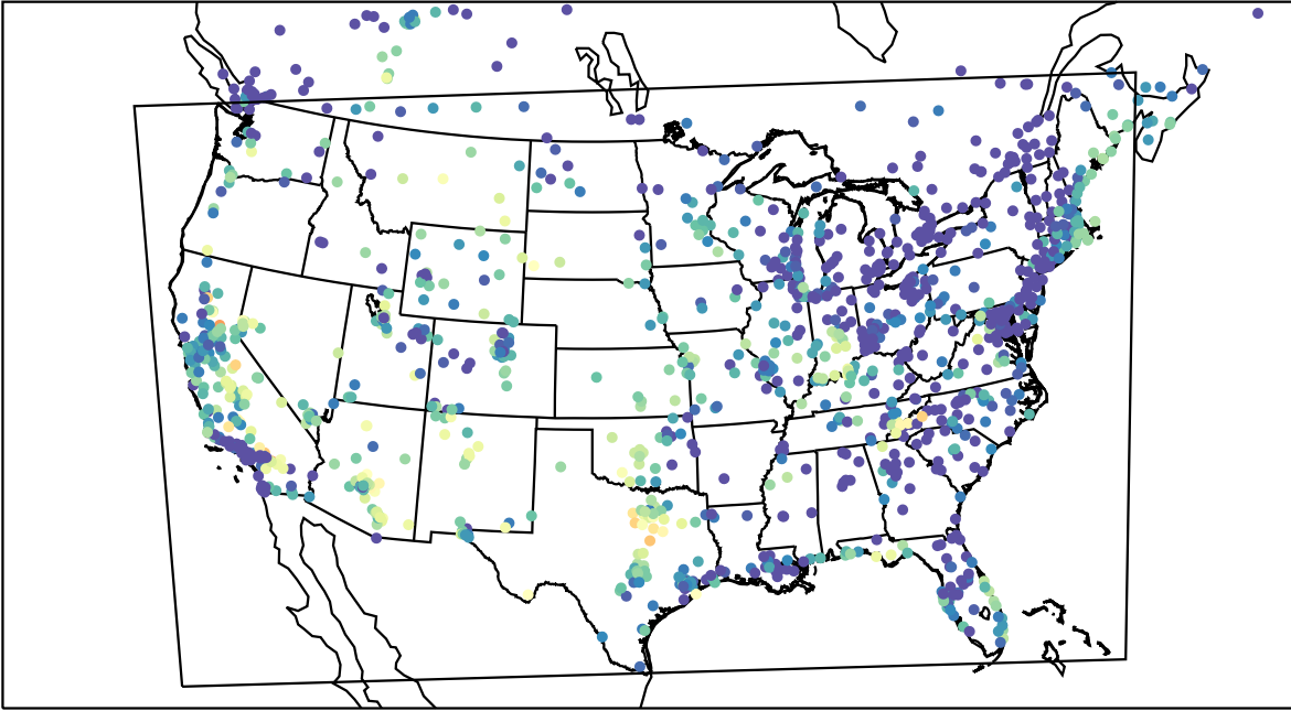
AirNOW (2023-08-26_06:00:00)
