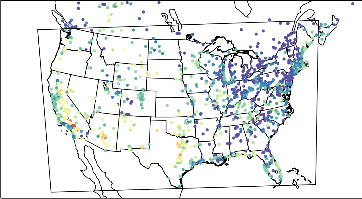
AirNOW (2023-08-26_03:00:00)
