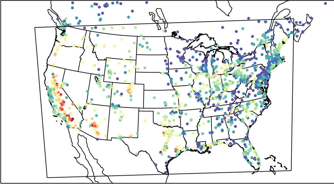
AirNOW (2023-08-25_02:00:00)
