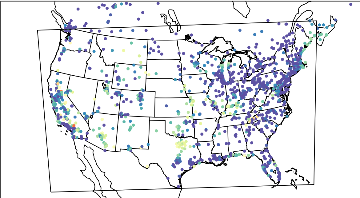
AirNOW (2023-08-26_09:00:00)
