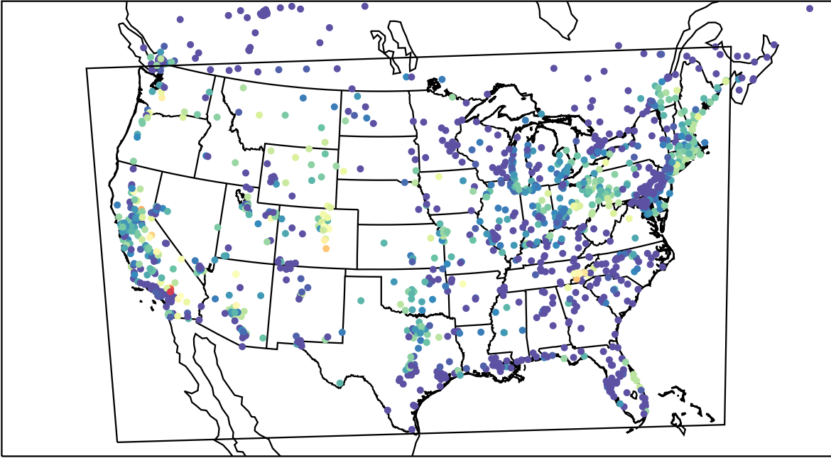
AirNOW (2023-08-25_09:00:00)
