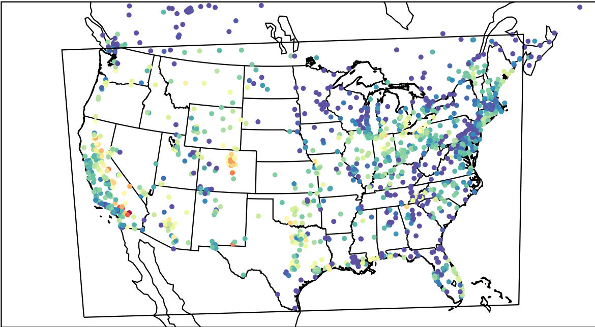
AirNOW (2023-08-25_04:00:00)
