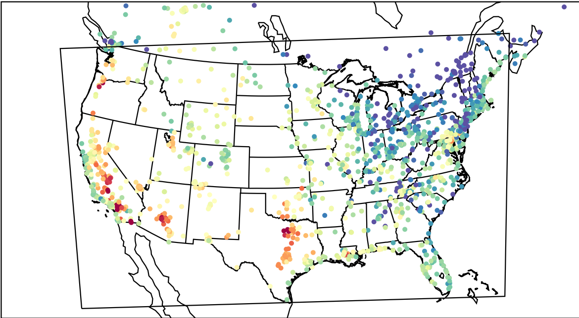
AirNOW (2023-08-26_00:00:00)
