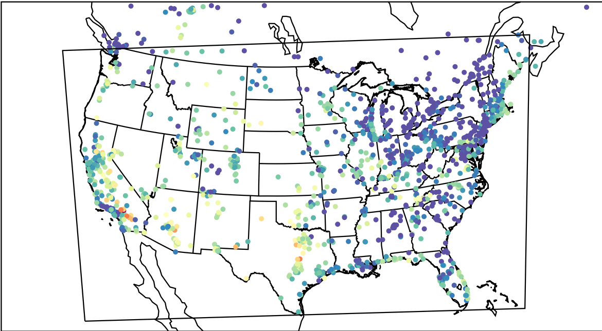
AirNOW (2023-08-26_04:00:00)
