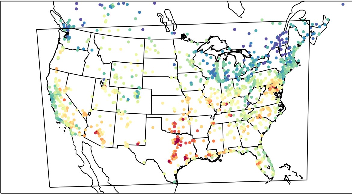
AirNOW (2023-08-25_18:00:00)
