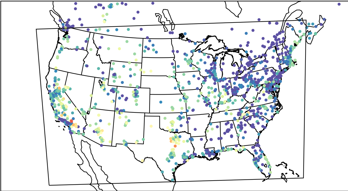
AirNOW (2023-08-26_05:00:00)
