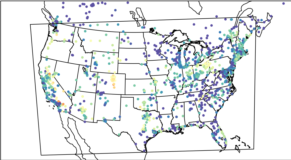
AirNOW (2023-08-25_06:00:00)
