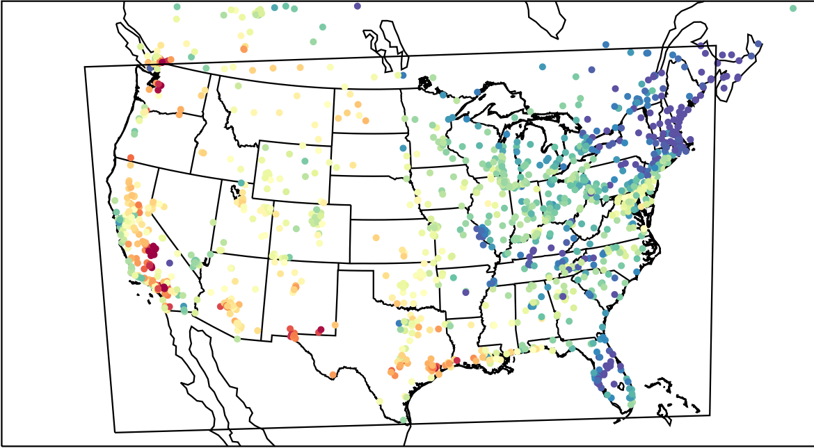
AirNOW (2023-08-27_23:00:00)
