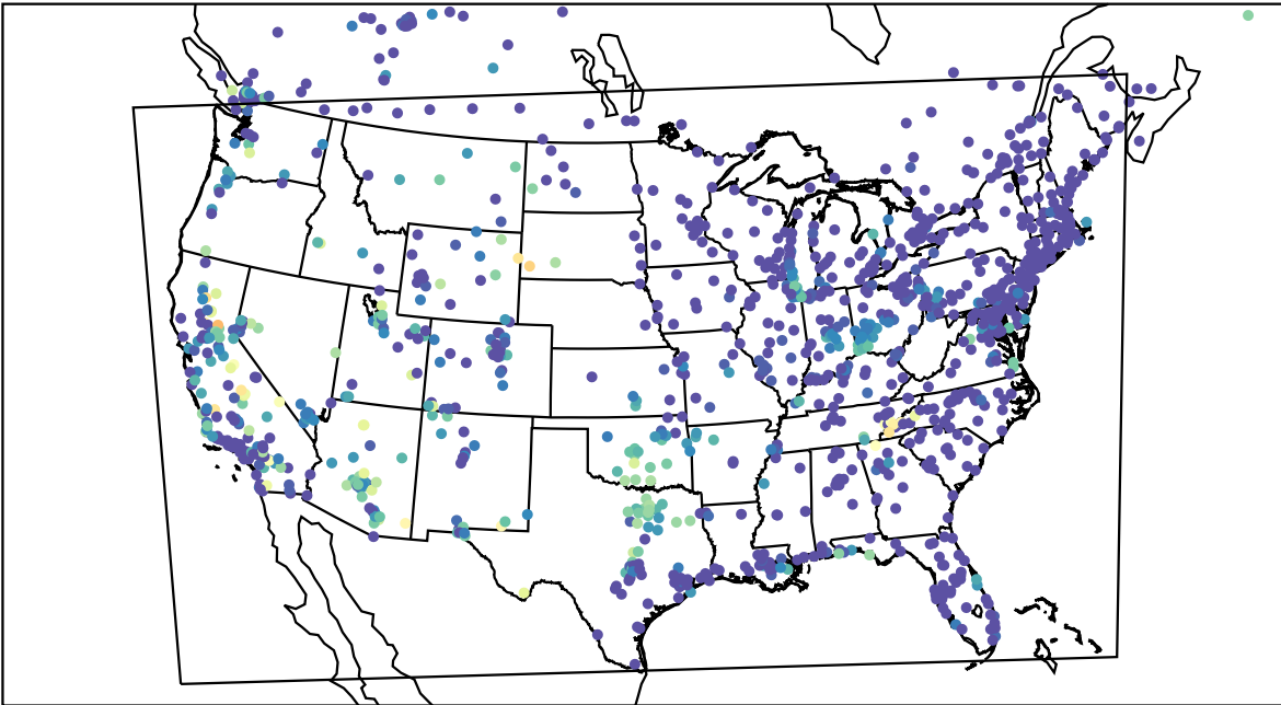
AirNOW (2023-08-27_11:00:00)
