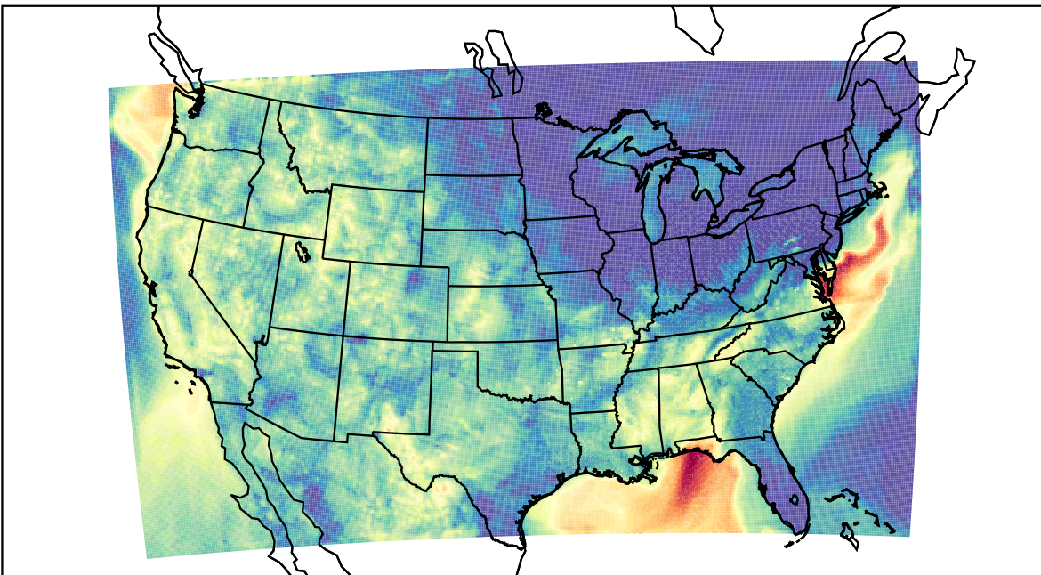
WRF (2023-08-27_12:00:00)
