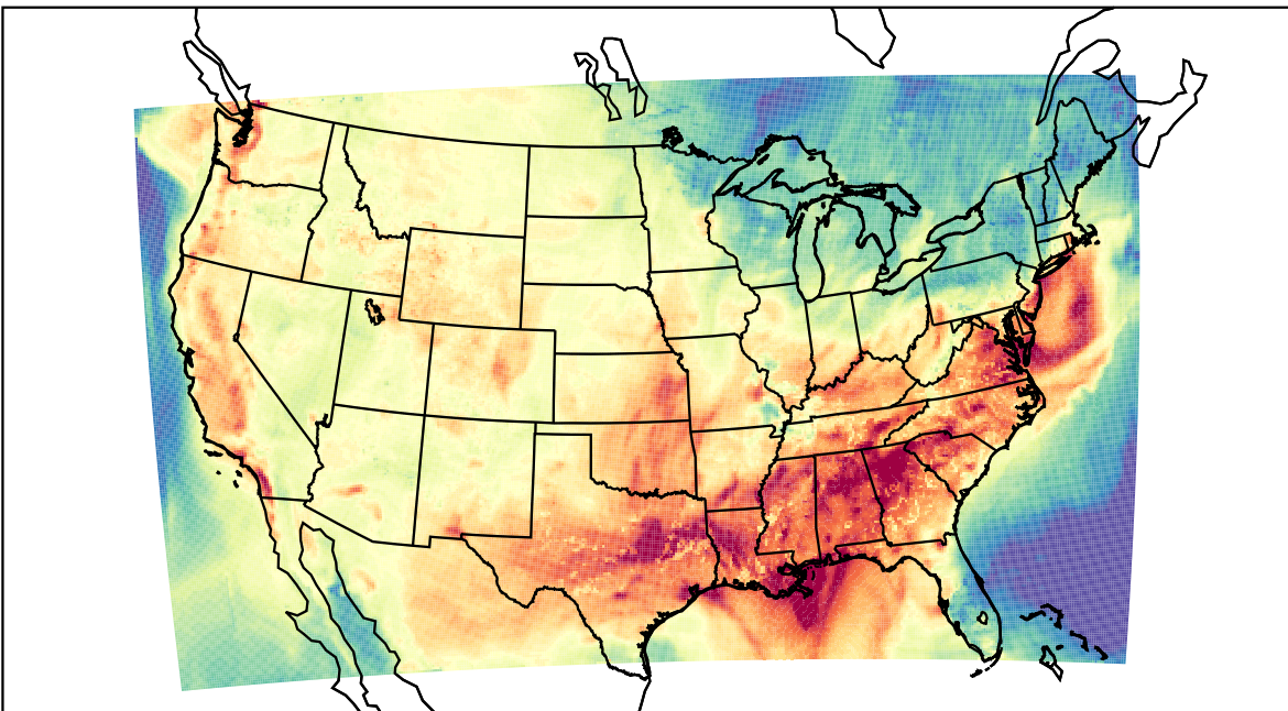
WRF (2023-08-27_21:00:00)
