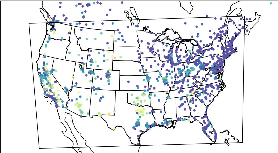
AirNOW (2023-08-27_07:00:00)
