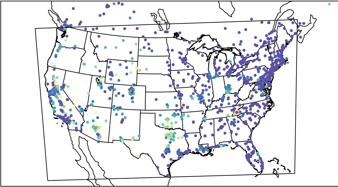
AirNOW (2023-08-27_10:00:00)
