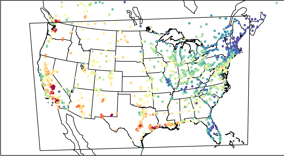
AirNOW (2023-08-27_22:00:00)
