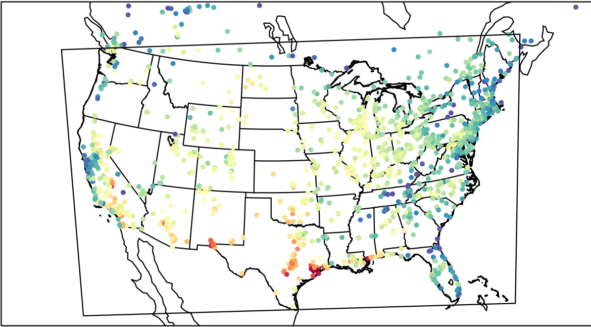
AirNOW (2023-08-28_17:00:00)
