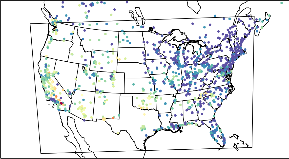
AirNOW (2023-08-27_04:00:00)
