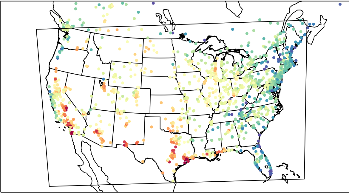
AirNOW (2023-08-28_19:00:00)
