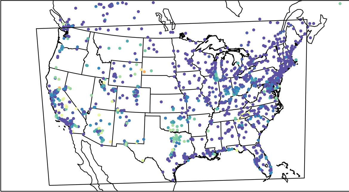
AirNOW (2023-08-27_12:00:00)
