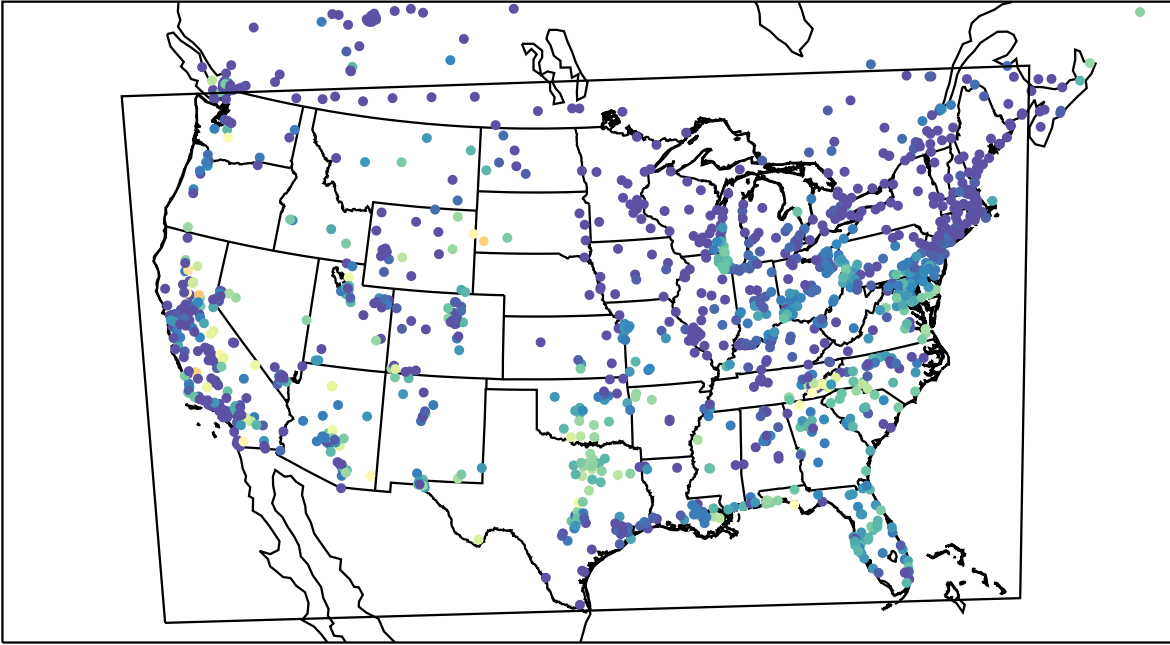
AirNOW (2023-08-27_13:00:00)
