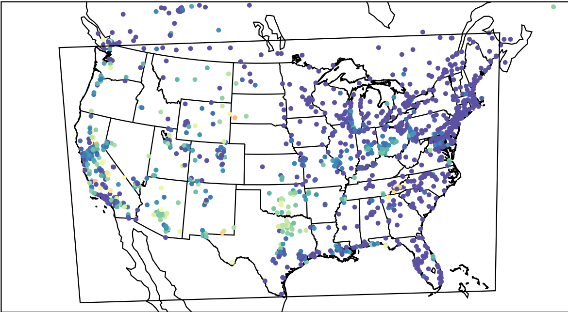
AirNOW (2023-08-27_09:00:00)
