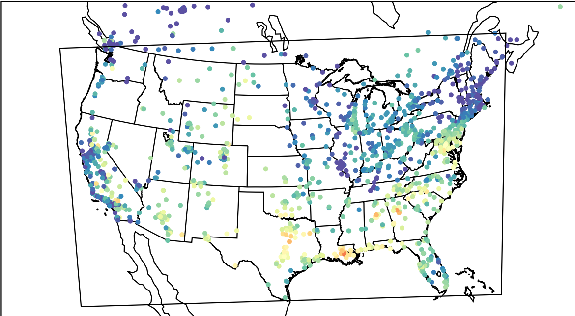
AirNOW (2023-08-27_15:00:00)
