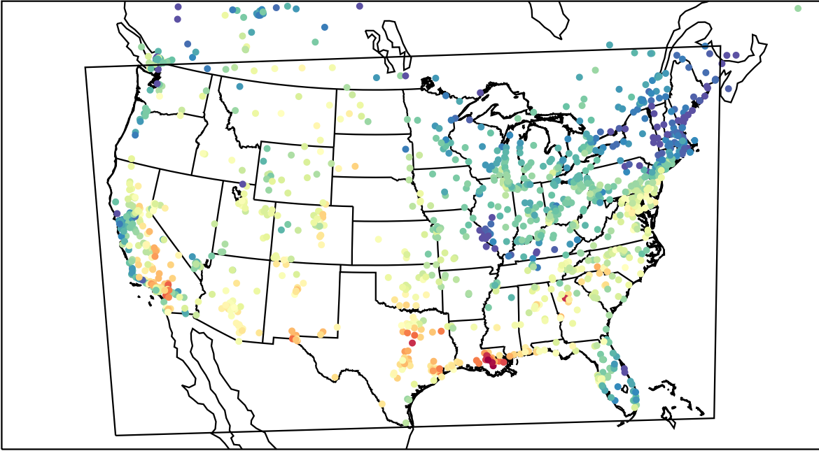
AirNOW (2023-08-27_17:00:00)
