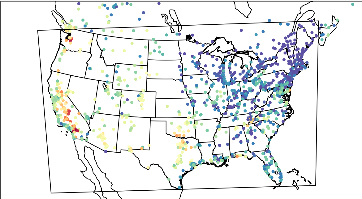
AirNOW (2023-08-27_02:00:00)
