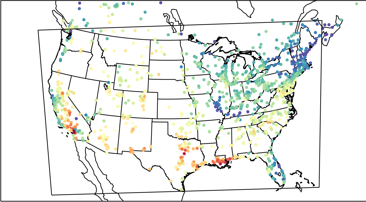
AirNOW (2023-08-27_18:00:00)
