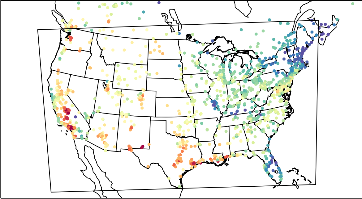
AirNOW (2023-08-27_21:00:00)
