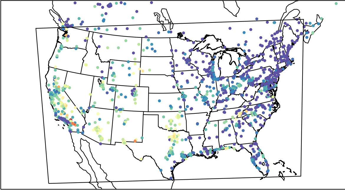
AirNOW (2023-08-27_05:00:00)
