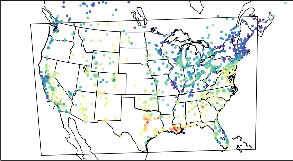
AirNOW (2023-08-27_16:00:00)
