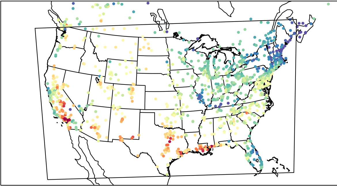
AirNOW (2023-08-27_19:00:00)
