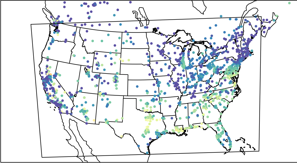
AirNOW (2023-08-27_14:00:00)
