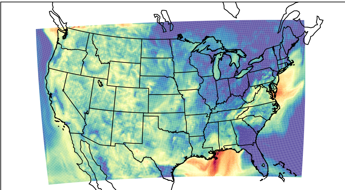
WRF (2023-08-28_12:00:00)
