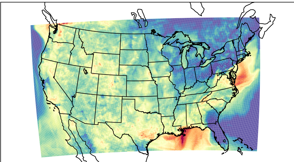
WRF (2023-08-28_06:00:00)
