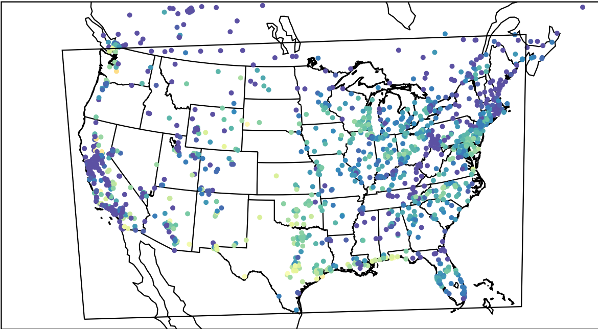
AirNOW (2023-08-28_14:00:00)
