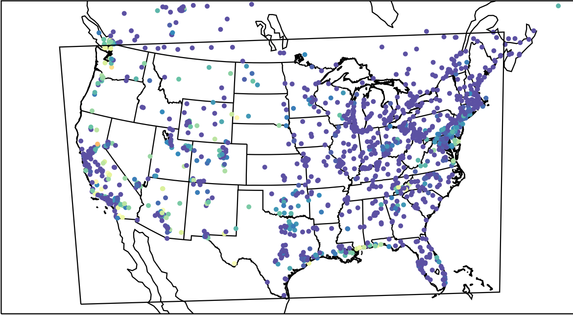
AirNOW (2023-08-28_12:00:00)
