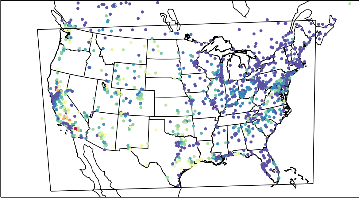
AirNOW (2023-08-28_05:00:00)
