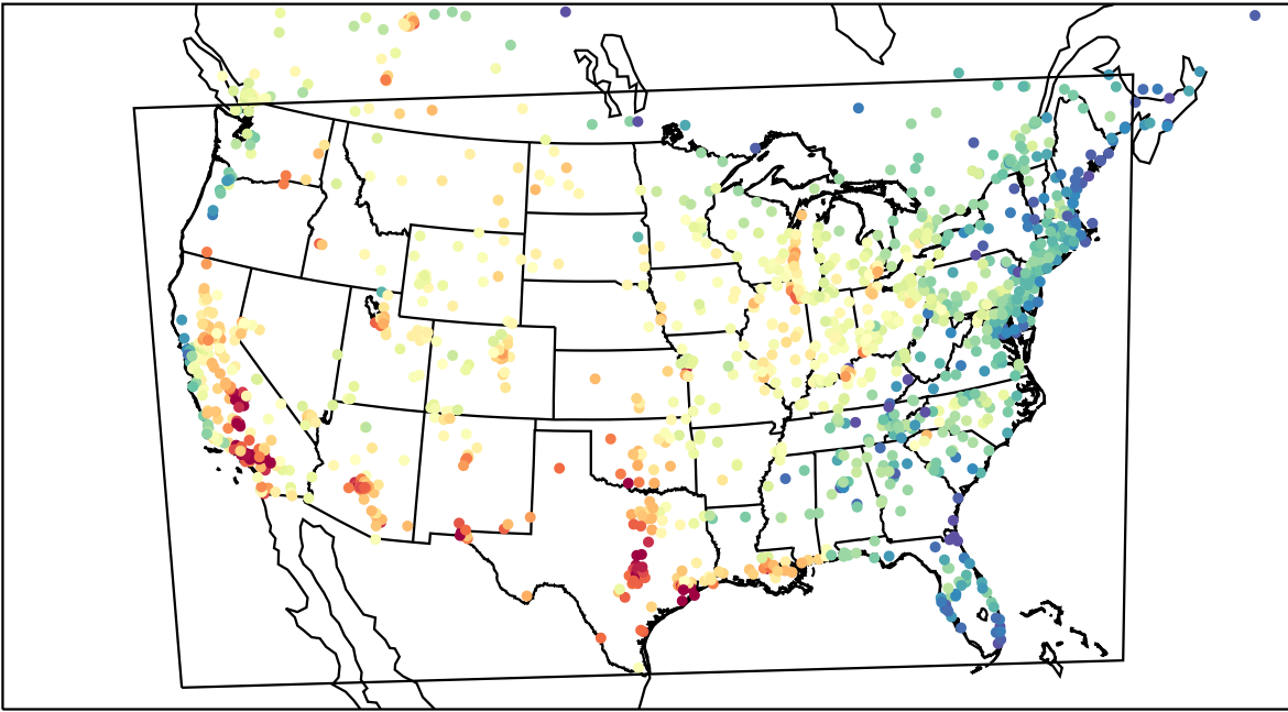
AirNOW (2023-08-28_21:00:00)
