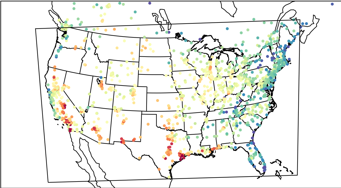
AirNOW (2023-08-28_19:00:00)
