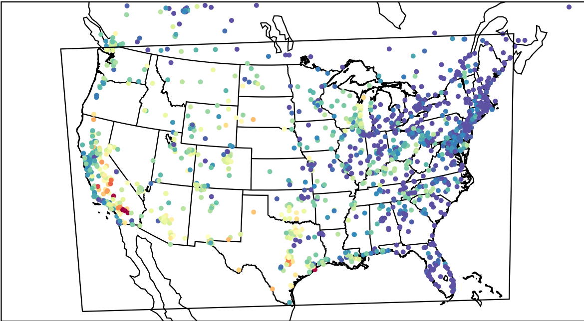
AirNOW (2023-08-29_03:00:00)
