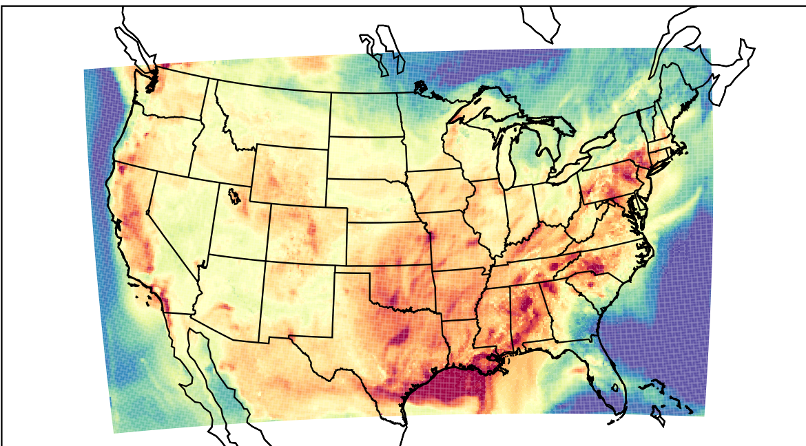
WRF (2023-08-28_21:00:00)
