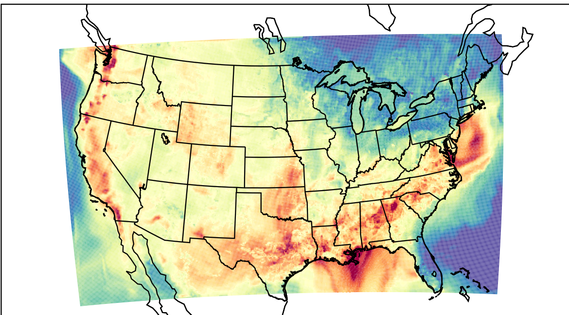
WRF (2023-08-28_00:00:00)
