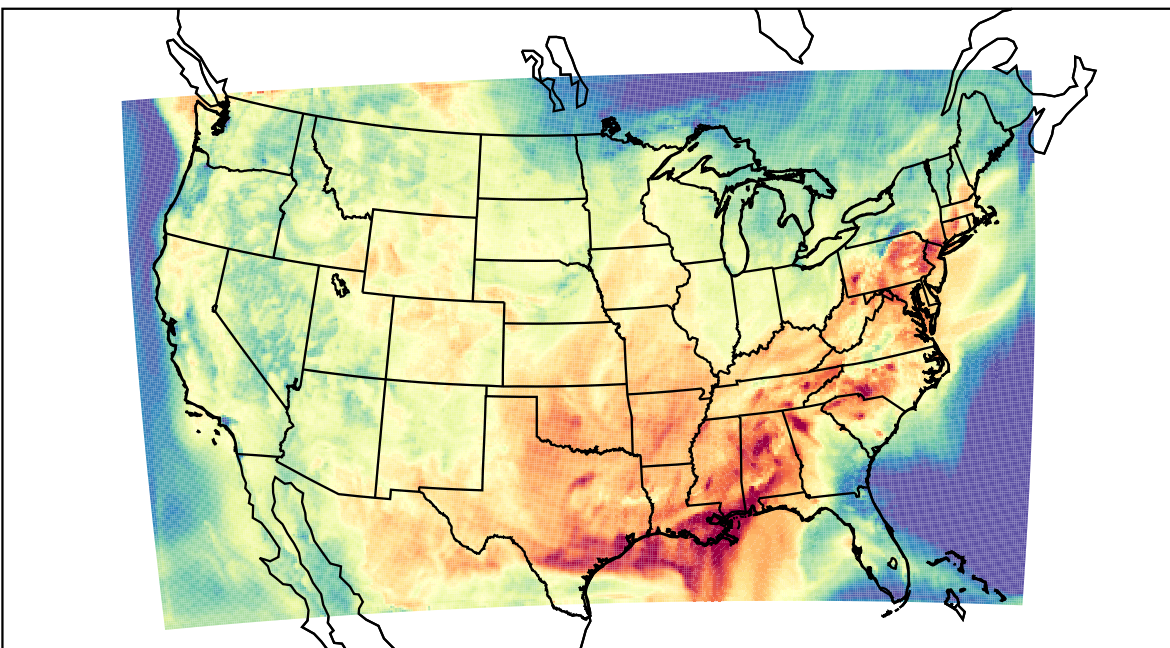
WRF (2023-08-28_17:00:00)
