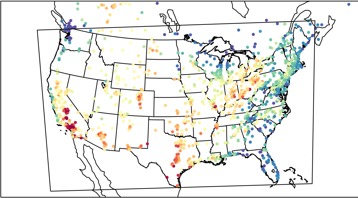
AirNOW (2023-08-29_21:00:00)
