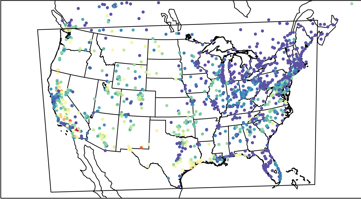
AirNOW (2023-08-28_04:00:00)
