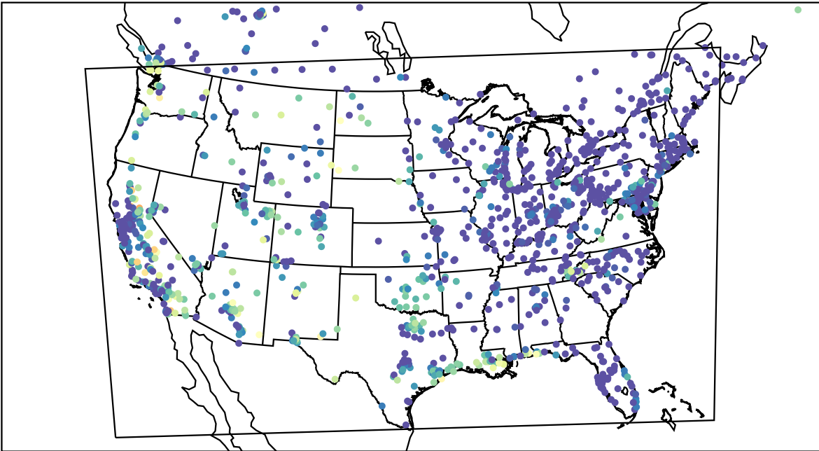
AirNOW (2023-08-28_09:00:00)
