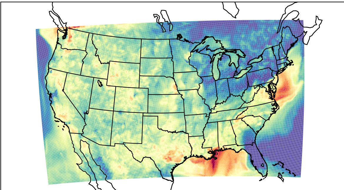
WRF (2023-08-28_05:00:00)
