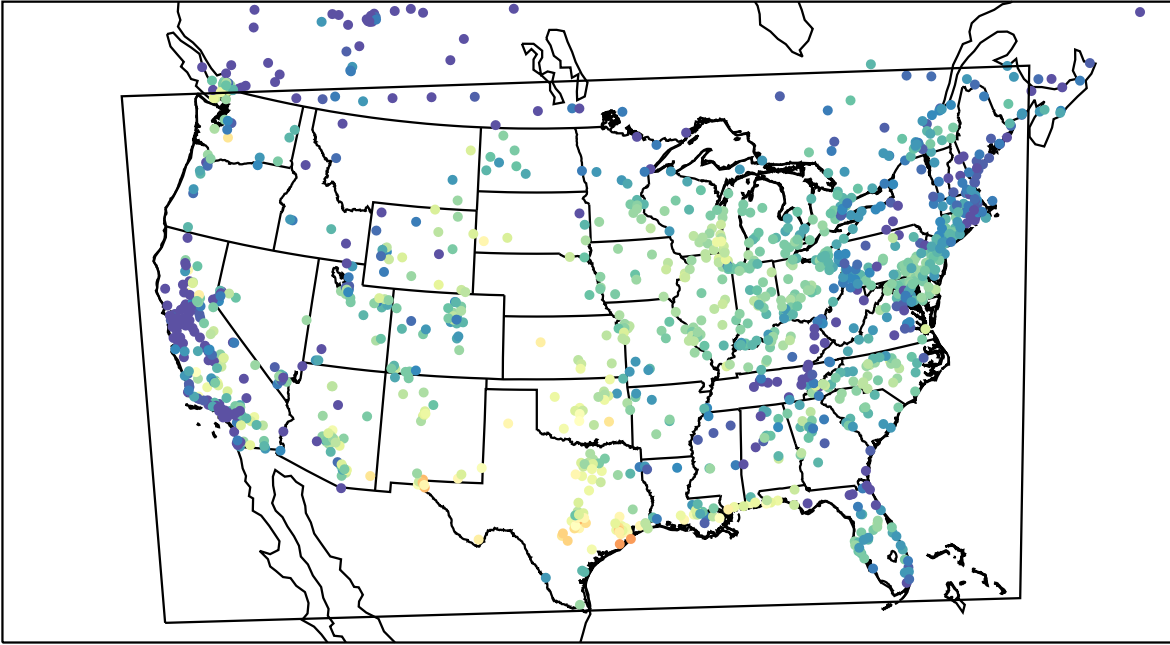
AirNOW (2023-08-28_15:00:00)
