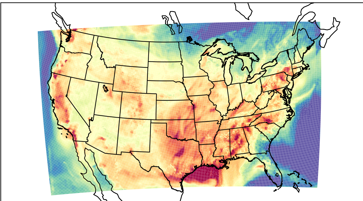
WRF (2023-08-28_22:00:00)
