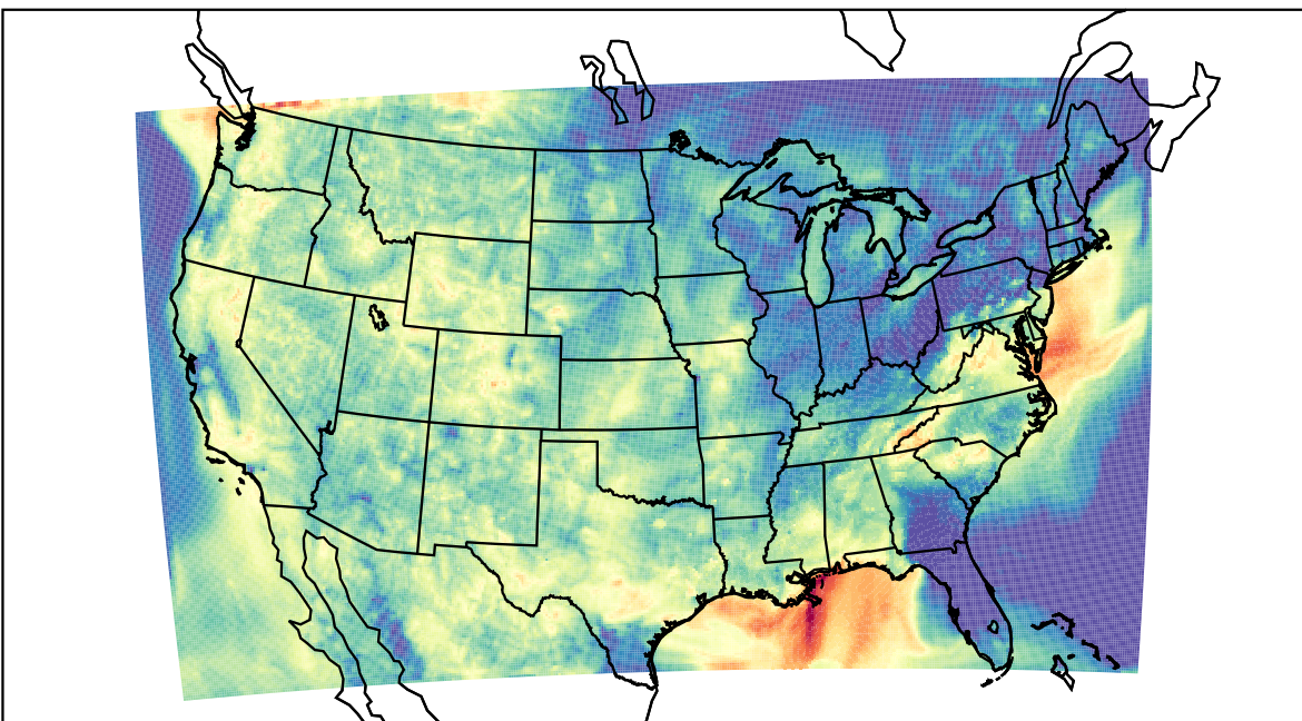
WRF (2023-08-28_09:00:00)
