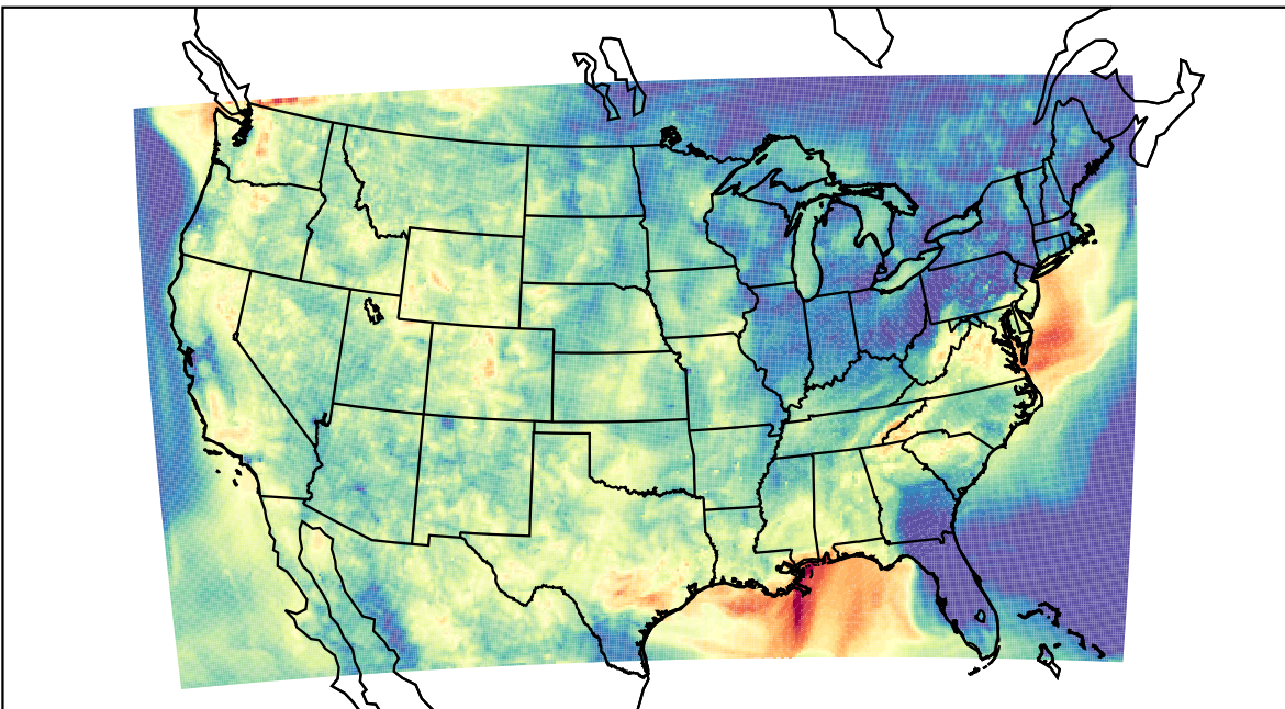
WRF (2023-08-28_07:00:00)
