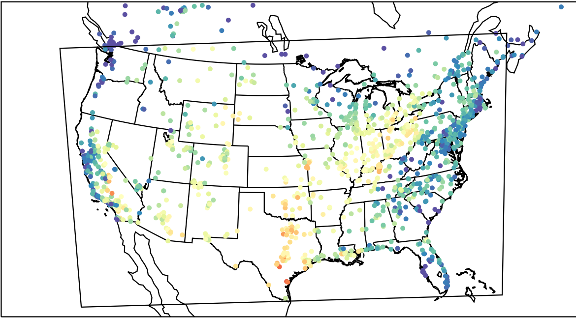
AirNOW (2023-08-29_16:00:00)
