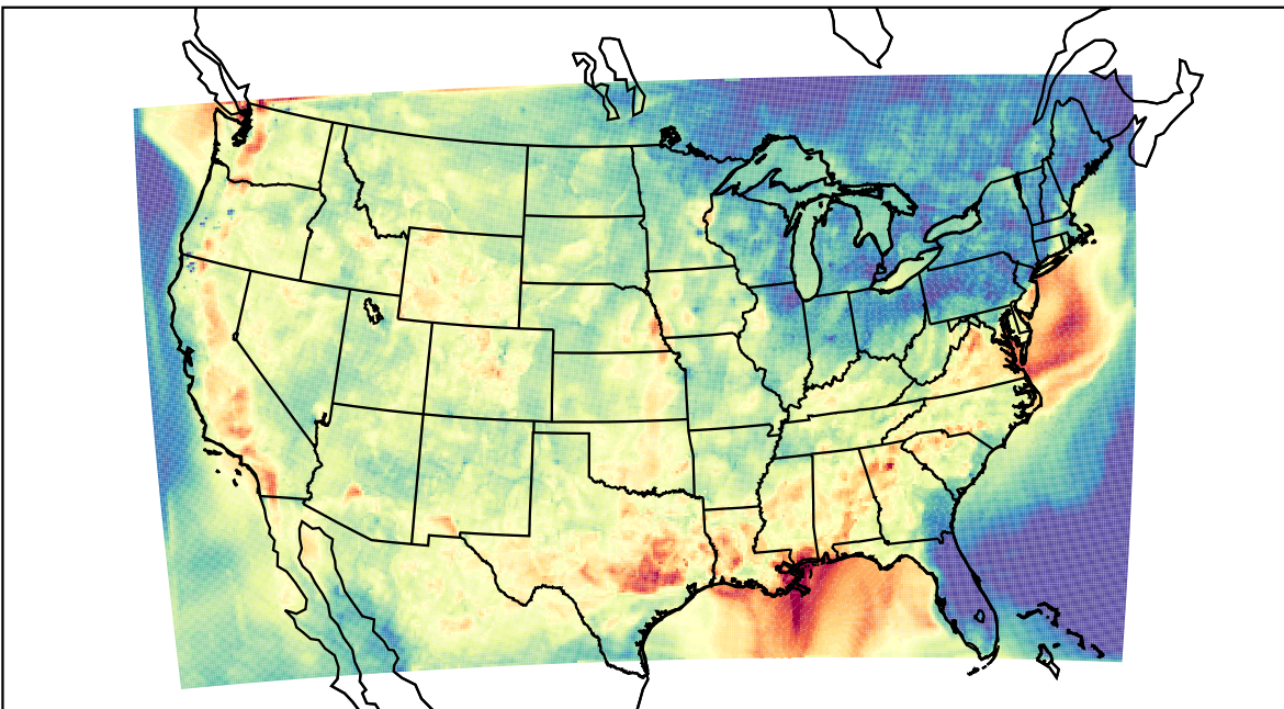
WRF (2023-08-28_02:00:00)
