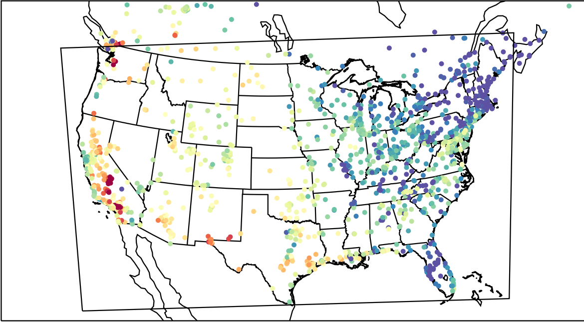
AirNOW (2023-08-28_00:00:00)
