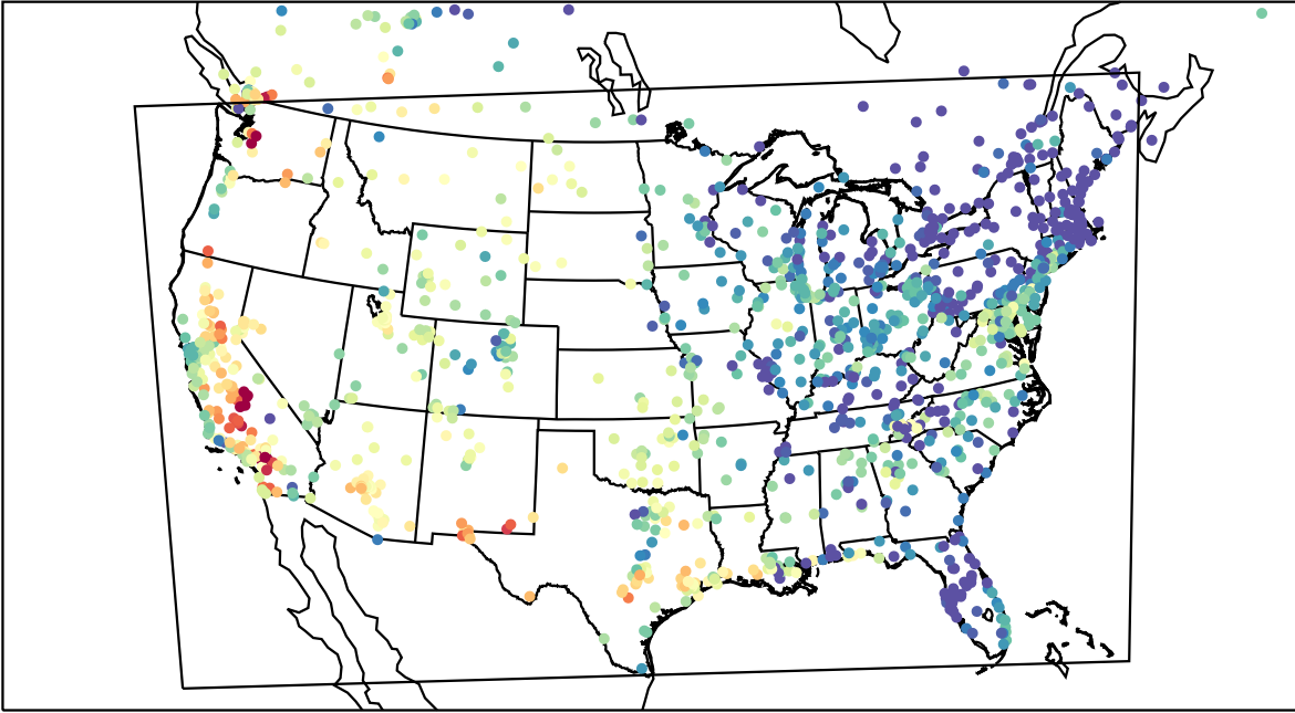
AirNOW (2023-08-28_01:00:00)
