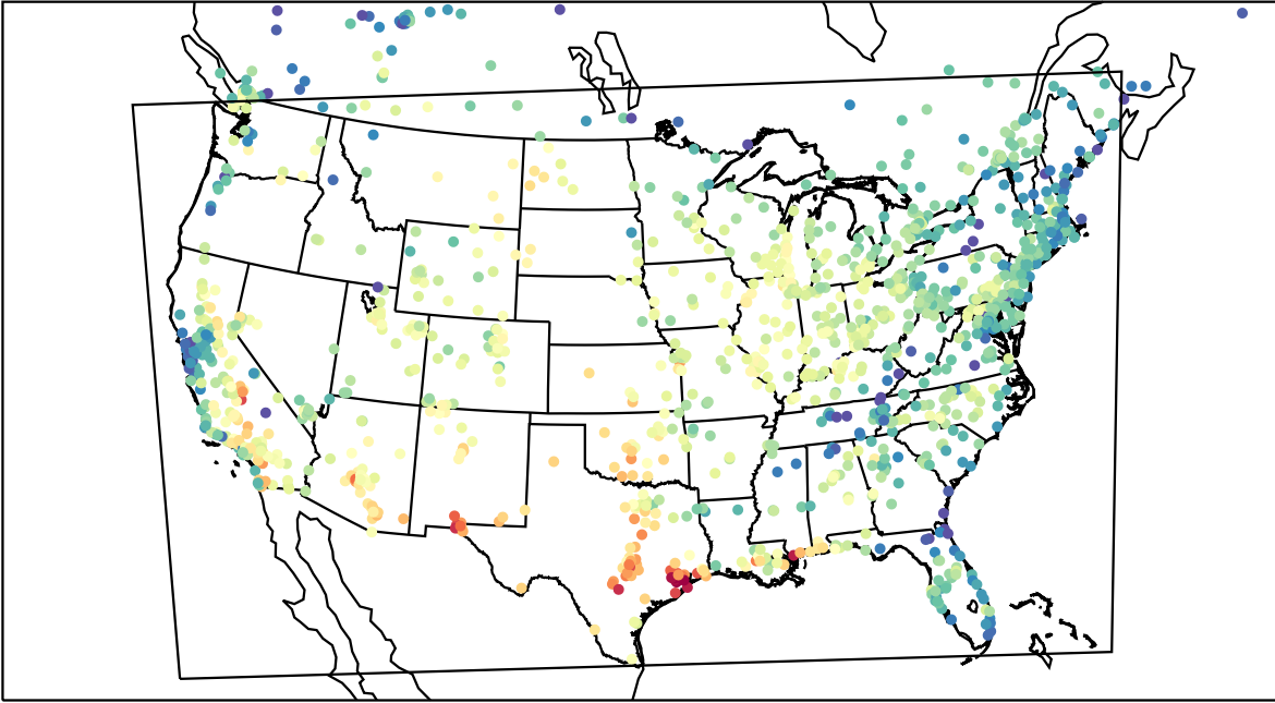
AirNOW (2023-08-28_17:00:00)
