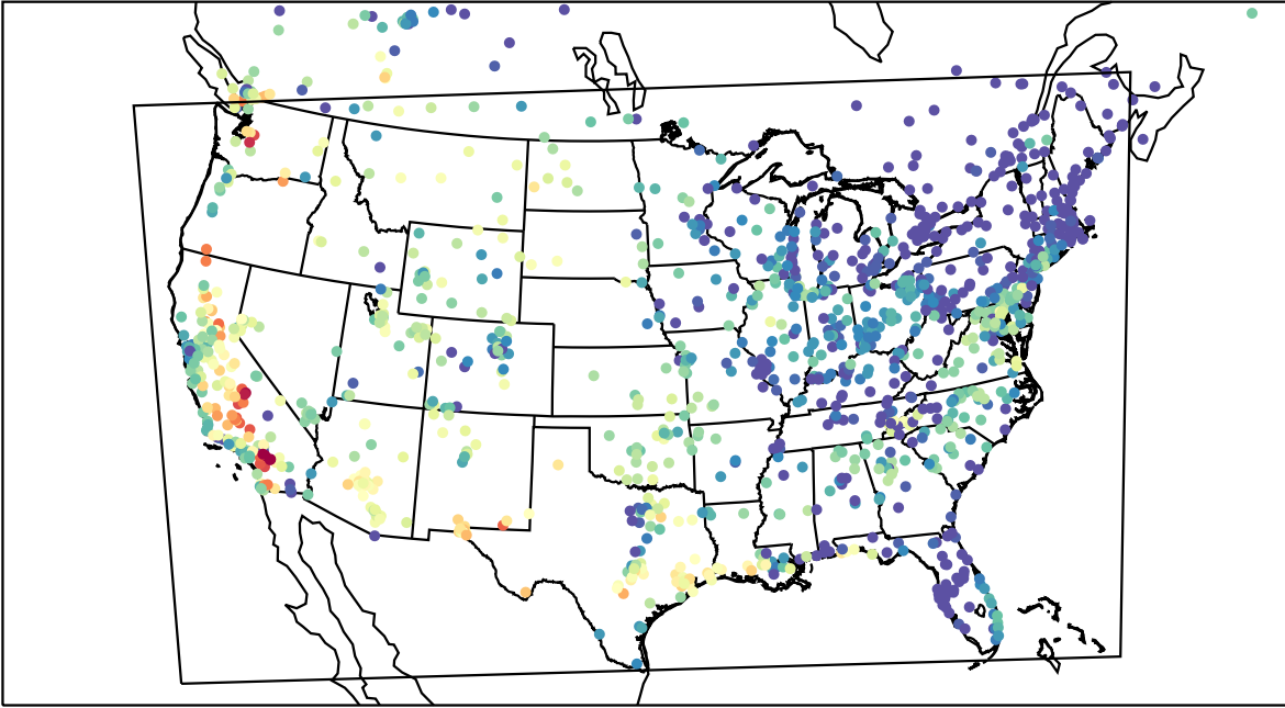
AirNOW (2023-08-28_02:00:00)
