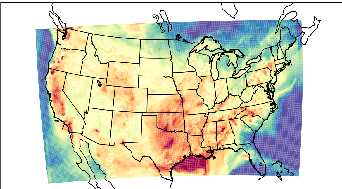
WRF (2023-08-28_23:00:00)
