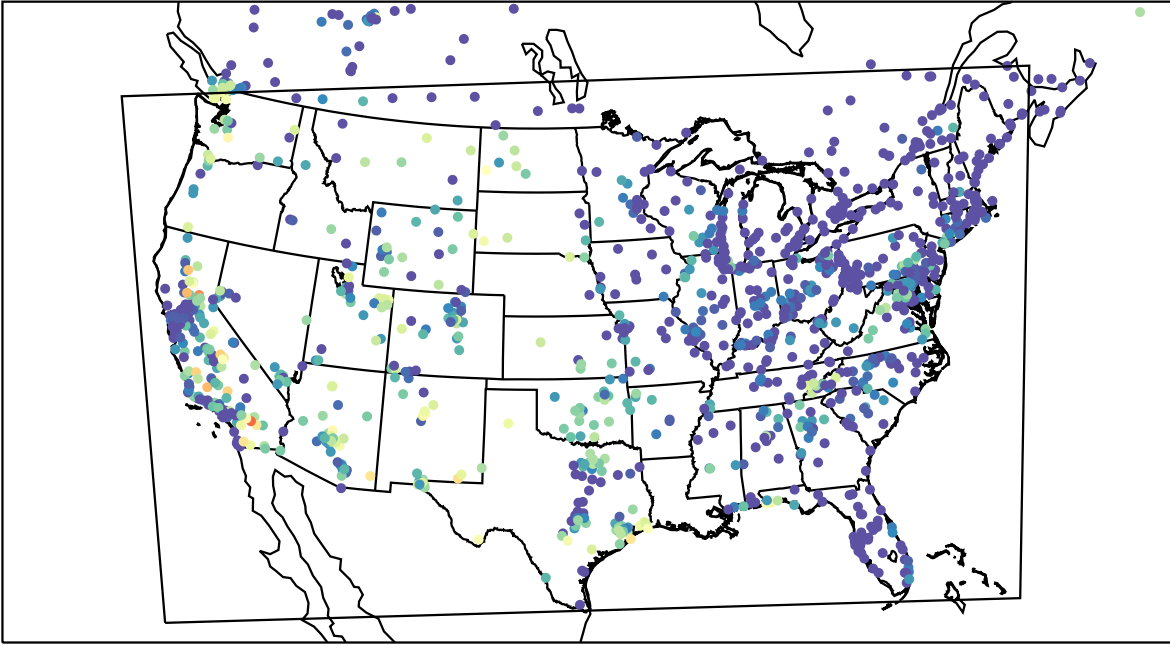
AirNOW (2023-08-28_07:00:00)
