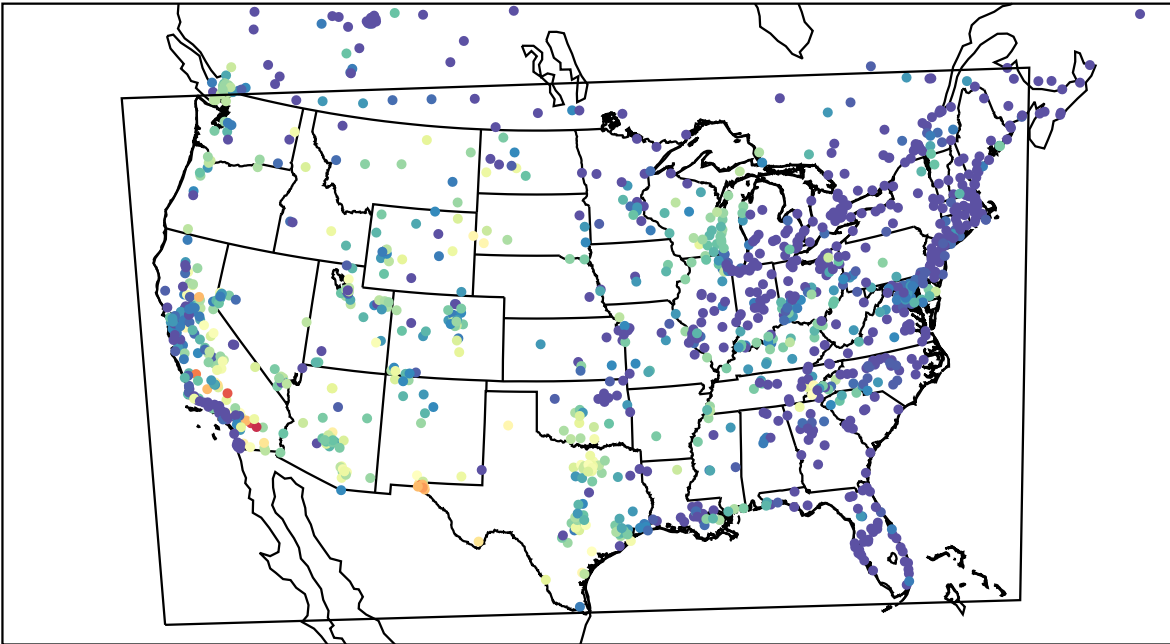
AirNOW (2023-08-29_06:00:00)
