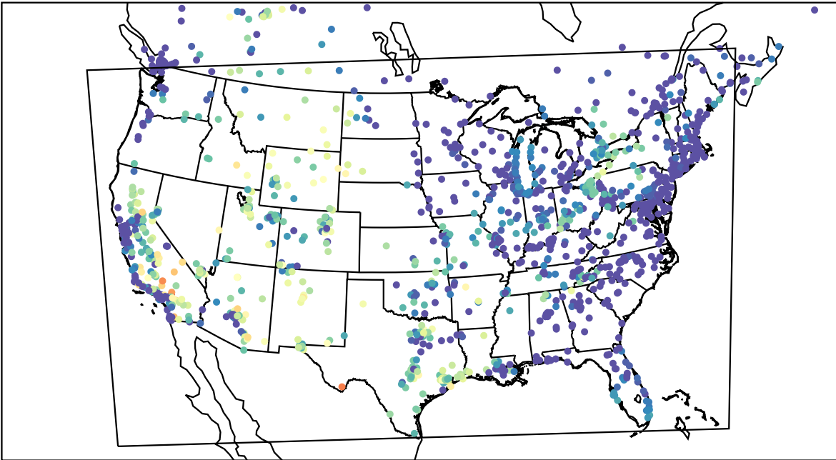
AirNOW (2023-08-30_07:00:00)
