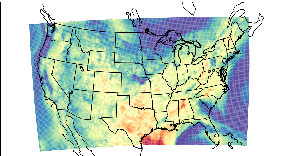
WRF (2023-08-29_15:00:00)
