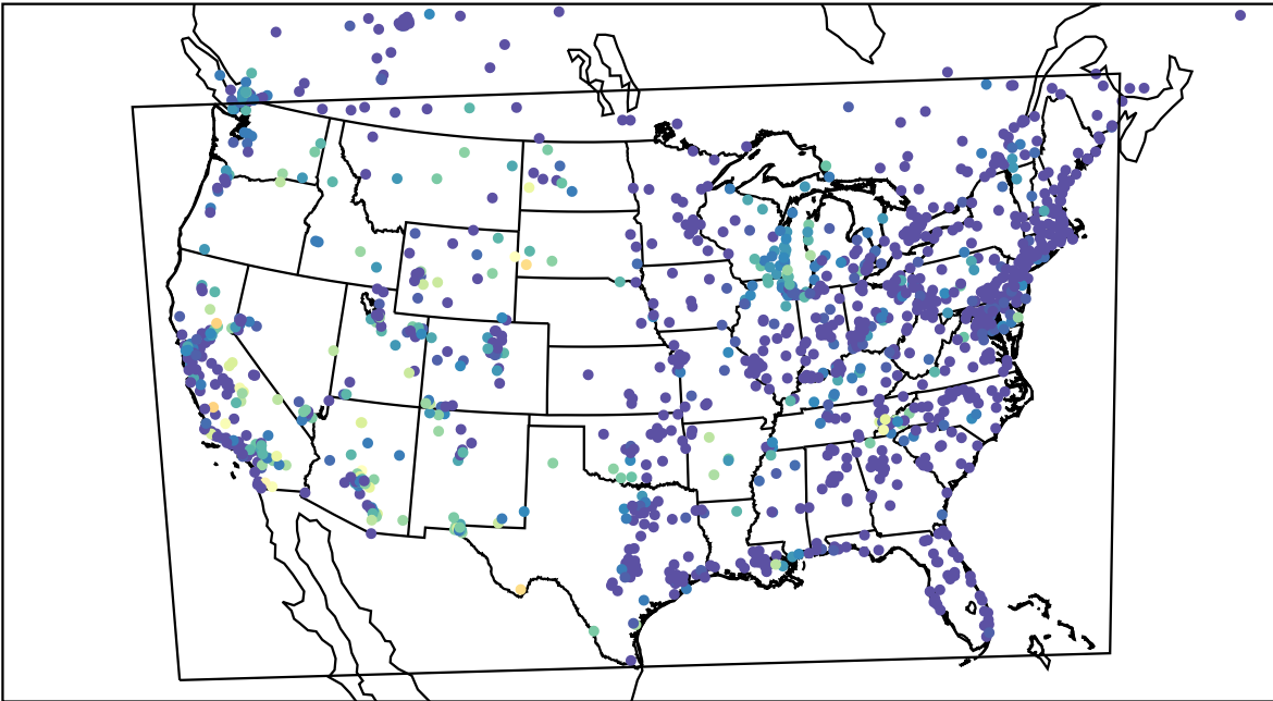
AirNOW (2023-08-29_12:00:00)
