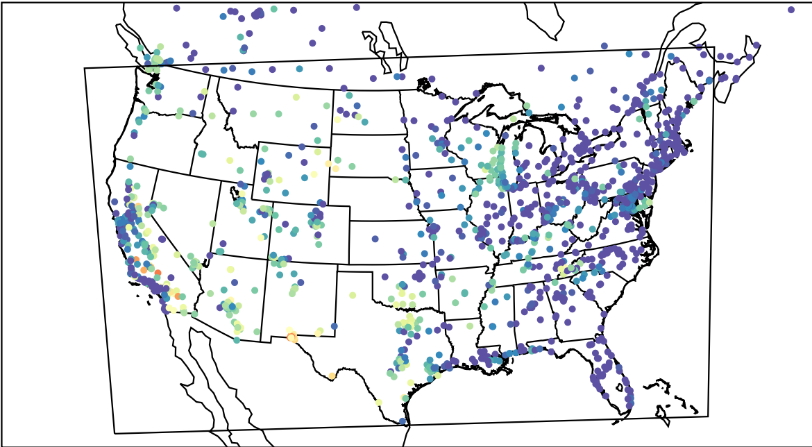
AirNOW (2023-08-29_07:00:00)
