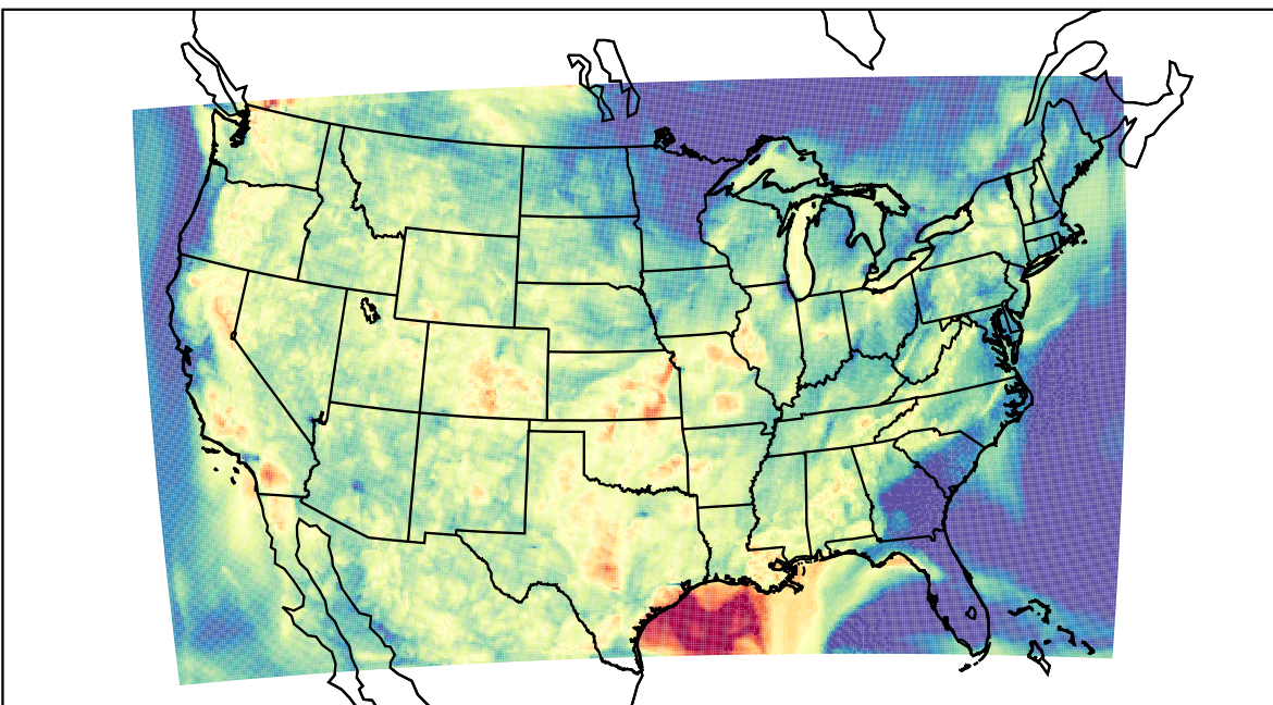
WRF (2023-08-29_05:00:00)
