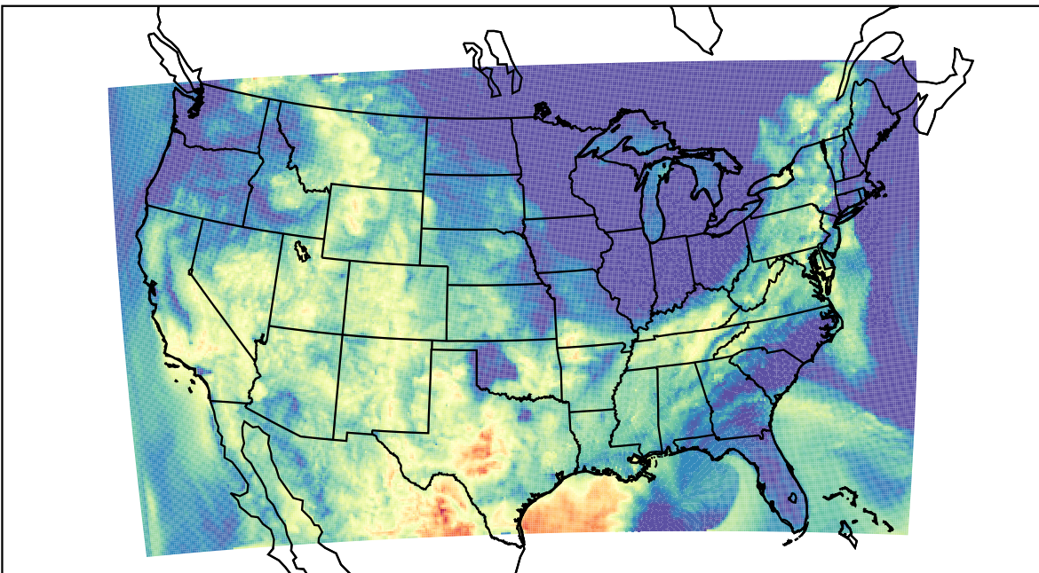
WRF (2023-08-30_12:00:00)
