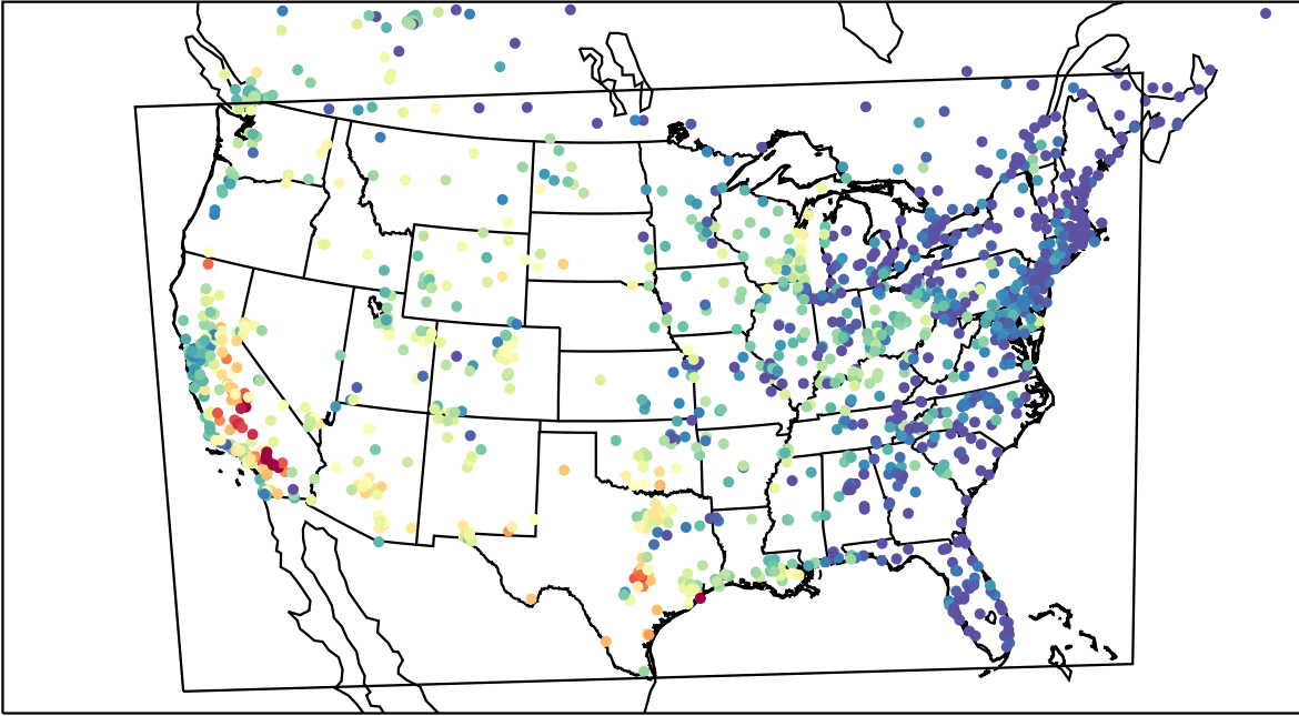
AirNOW (2023-08-29_02:00:00)
