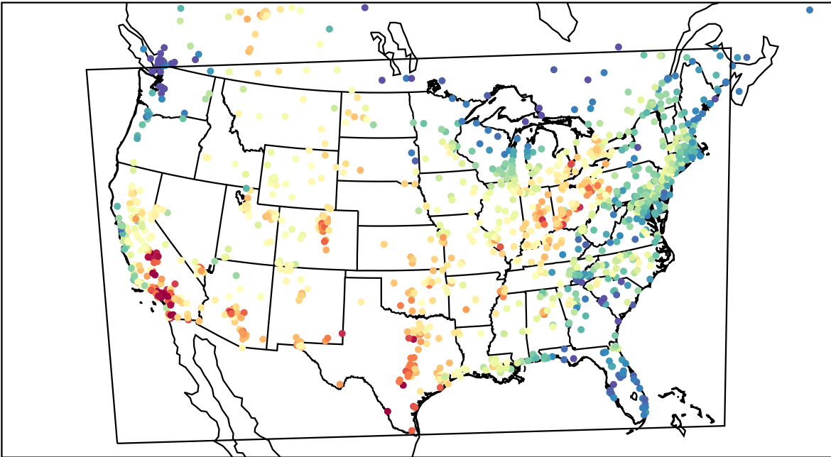
AirNOW (2023-08-29_20:00:00)
