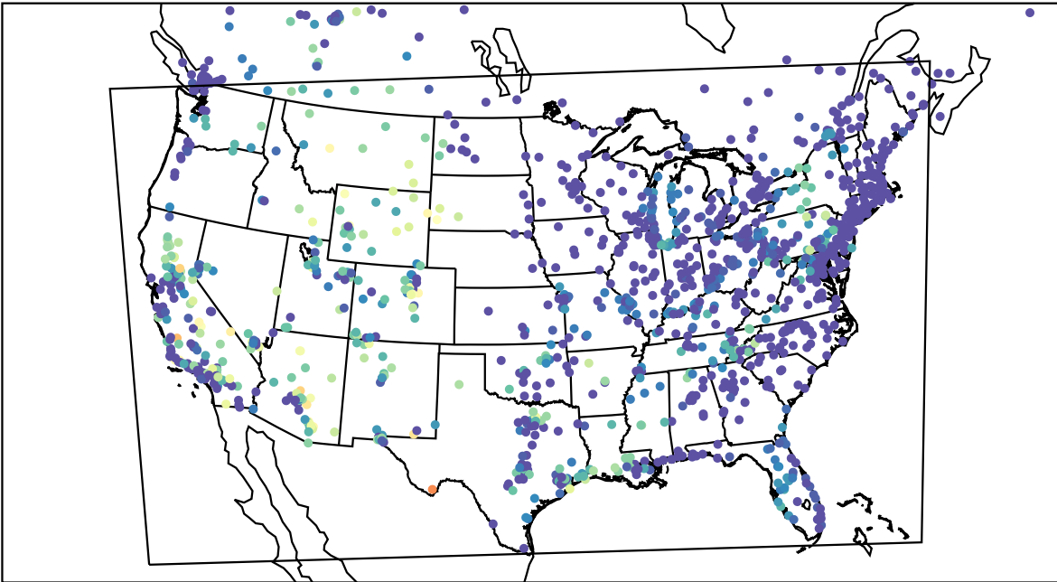
AirNOW (2023-08-30_11:00:00)
