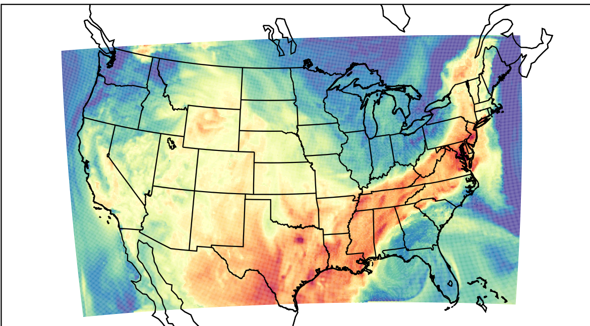
WRF (2023-08-30_17:00:00)
