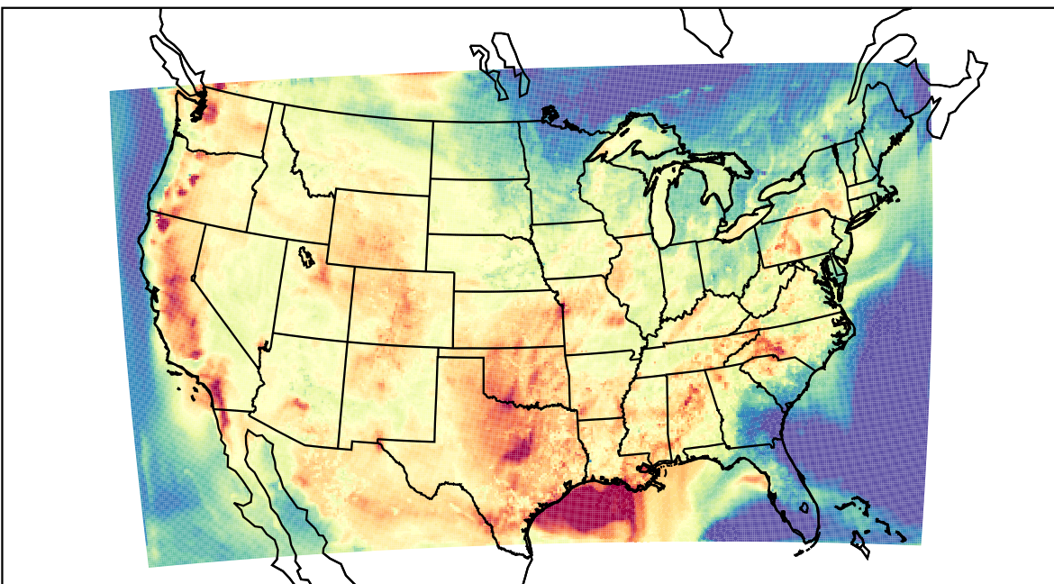
WRF (2023-08-29_00:00:00)
