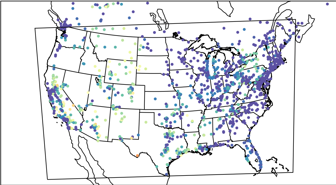
AirNOW (2023-08-30_09:00:00)
