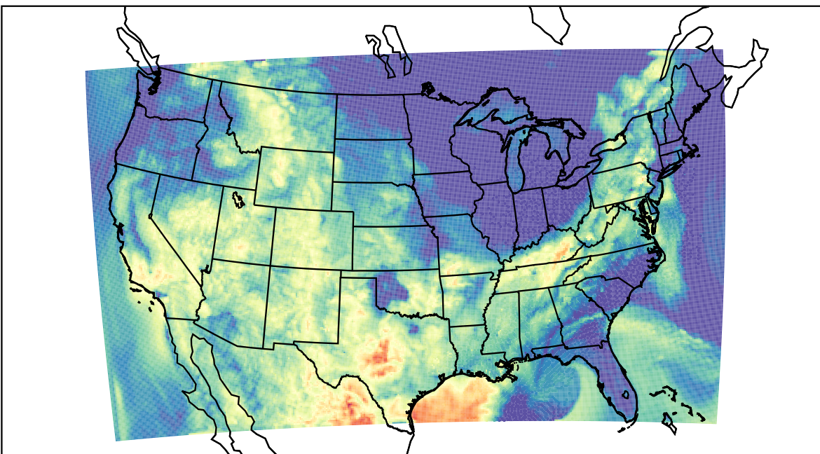
WRF (2023-08-30_11:00:00)
