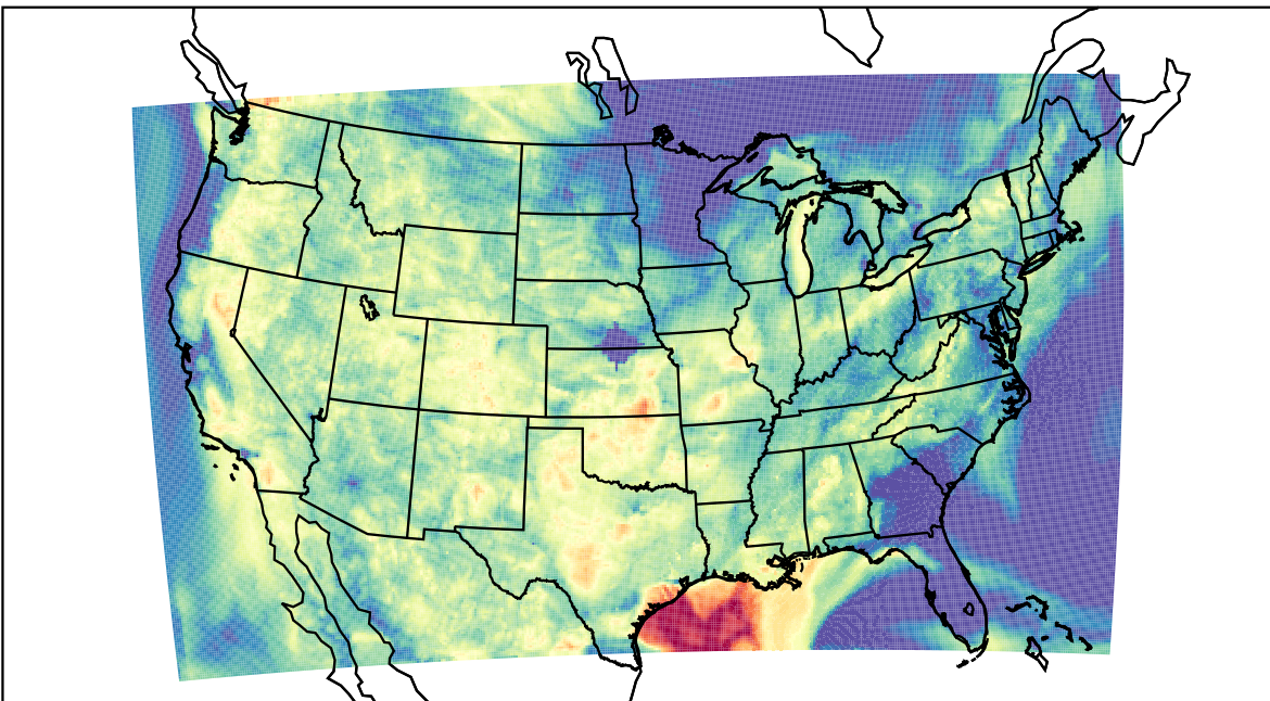
WRF (2023-08-29_08:00:00)
