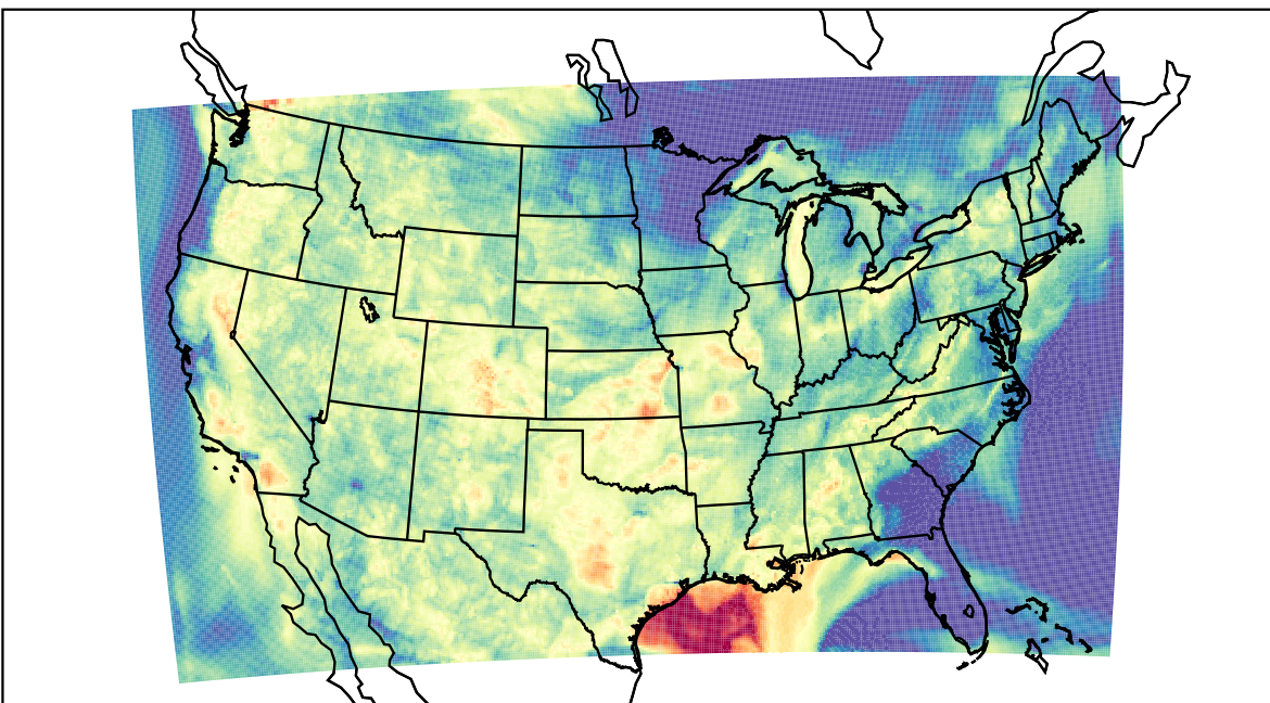
WRF (2023-08-29_06:00:00)
