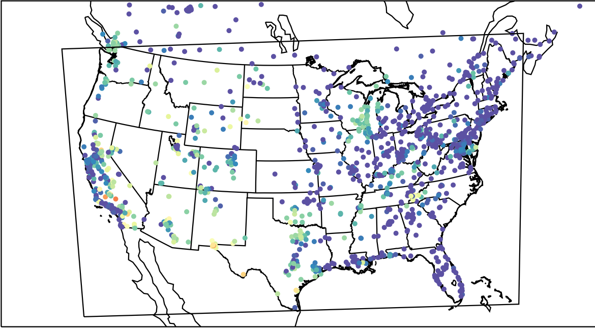
AirNOW (2023-08-29_08:00:00)
