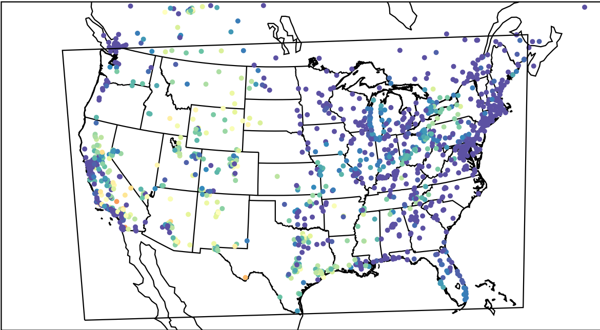
AirNOW (2023-08-30_08:00:00)
