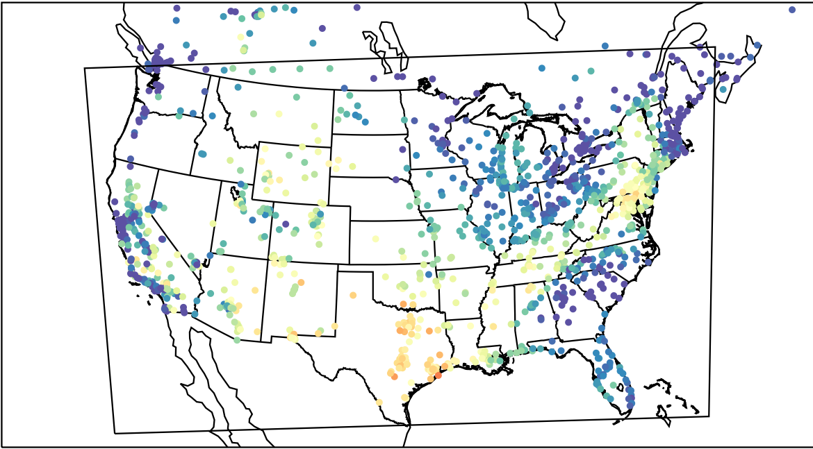
AirNOW (2023-08-30_15:00:00)
