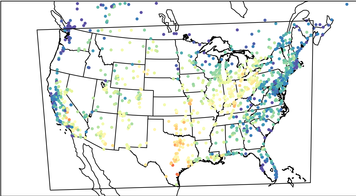
AirNOW (2023-08-29_16:00:00)
