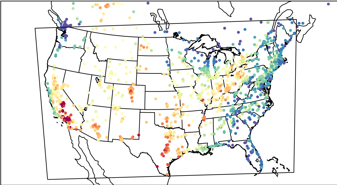
AirNOW (2023-08-29_22:00:00)
