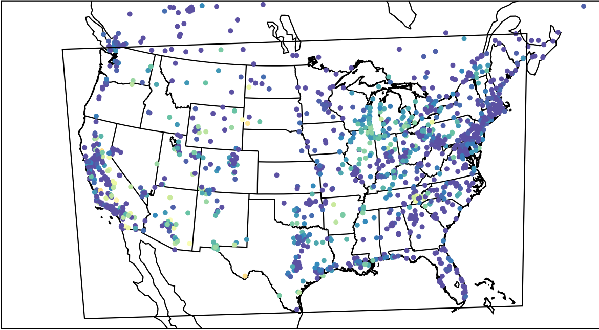
AirNOW (2023-08-29_13:00:00)
