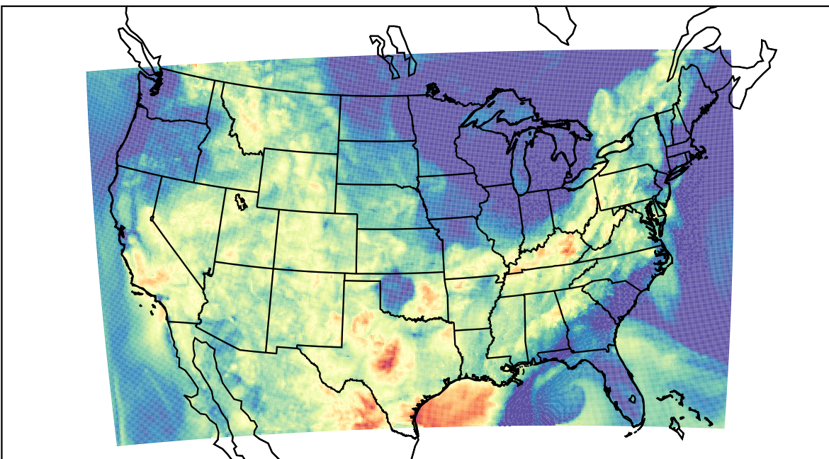
WRF (2023-08-30_07:00:00)
