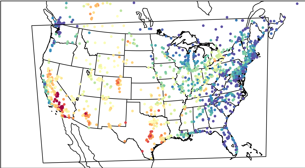
AirNOW (2023-08-30_00:00:00)
