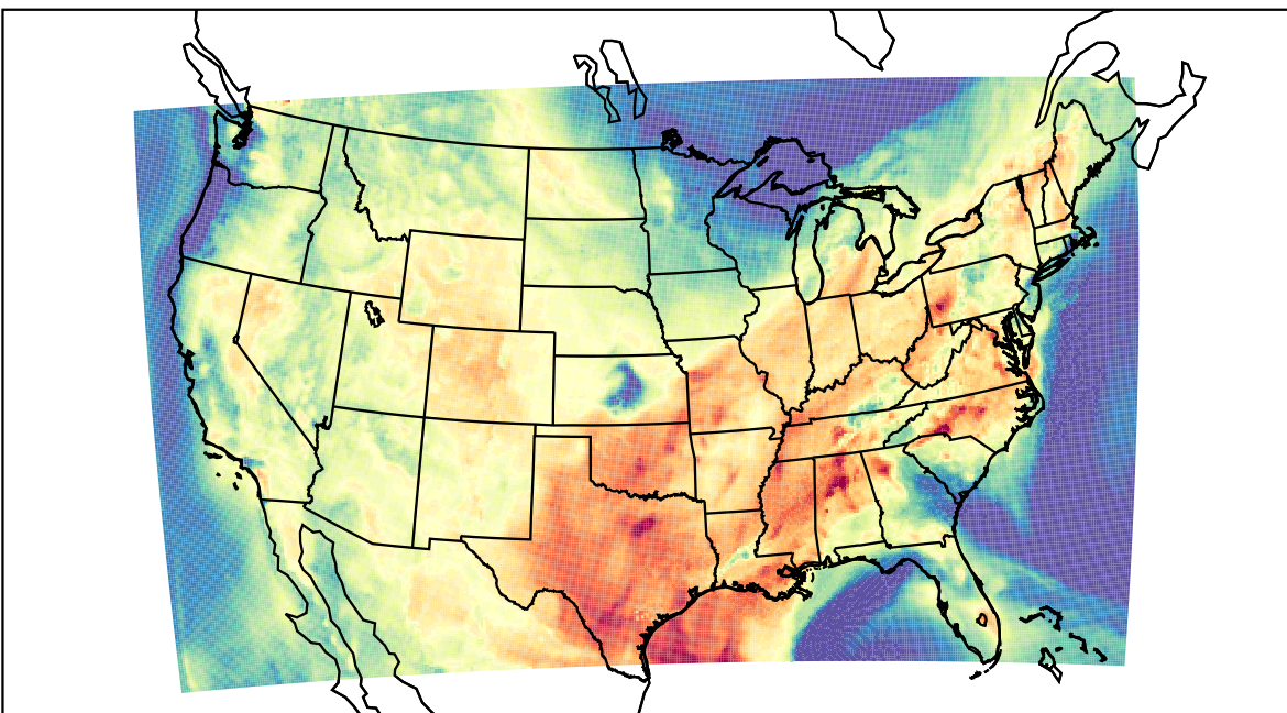
WRF (2023-08-29_17:00:00)
