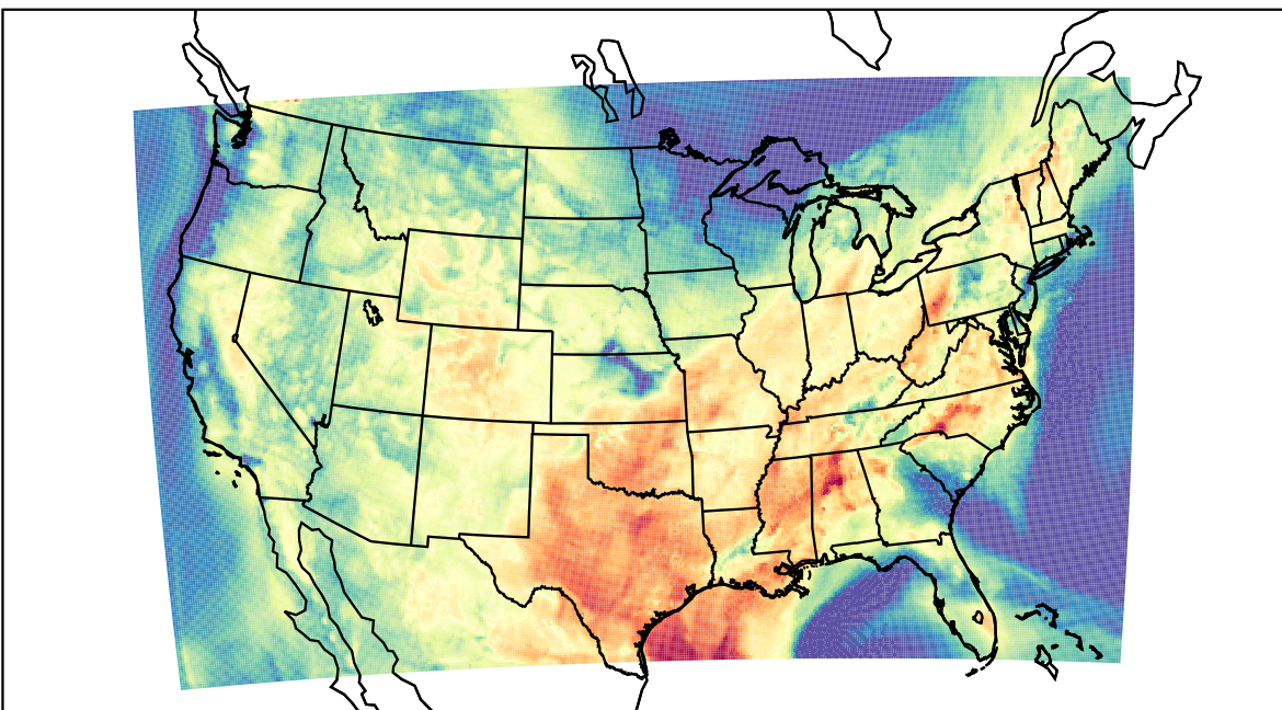
WRF (2023-08-29_16:00:00)
