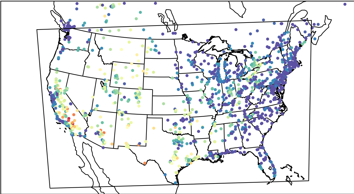
AirNOW (2023-08-30_04:00:00)
