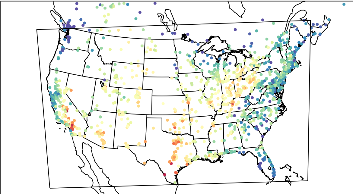
AirNOW (2023-08-29_17:00:00)
