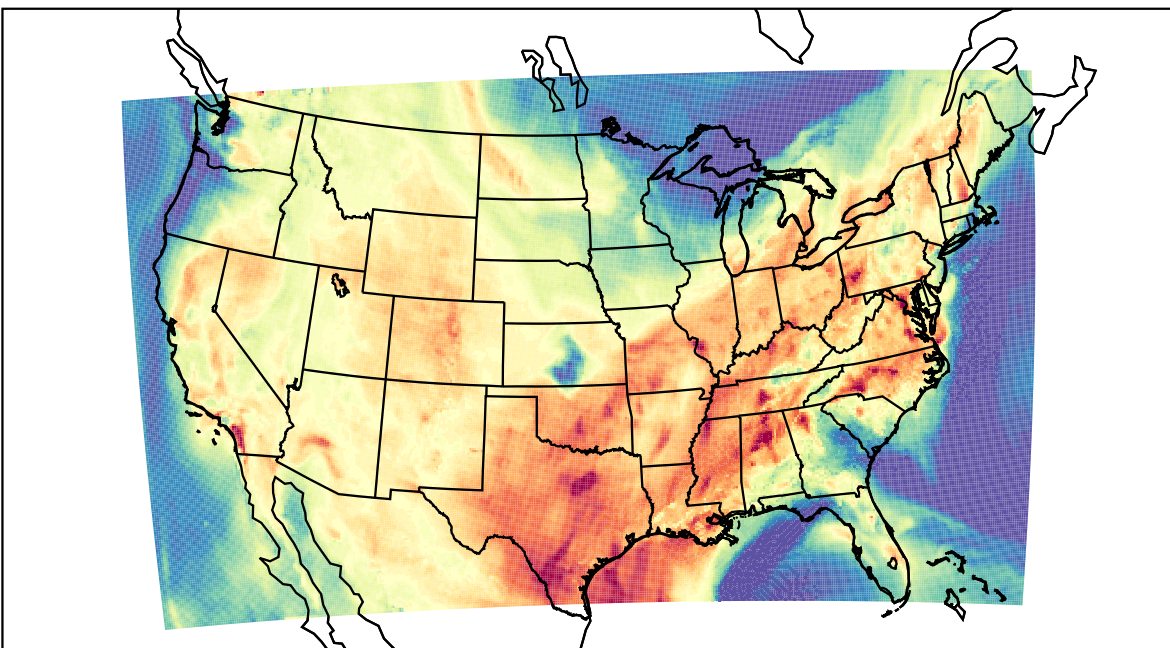
WRF (2023-08-29_19:00:00)
