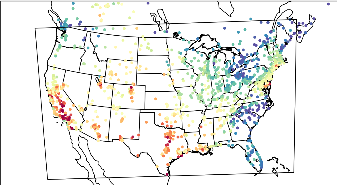
AirNOW (2023-08-30_21:00:00)
