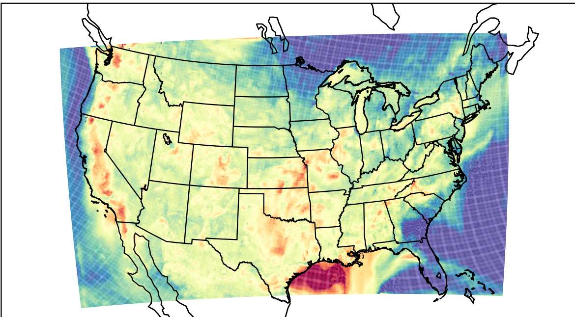
WRF (2023-08-29_02:00:00)
