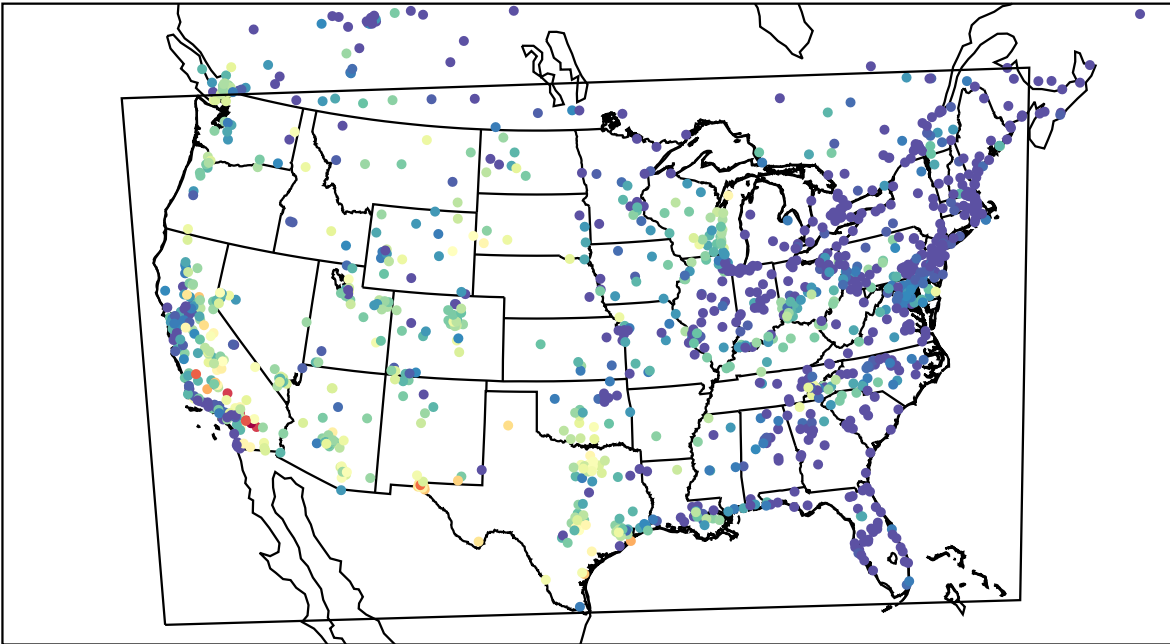
AirNOW (2023-08-29_05:00:00)
