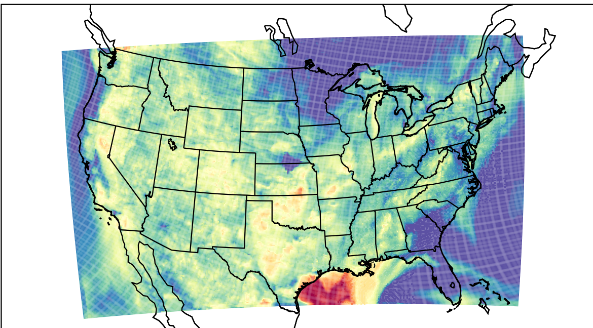
WRF (2023-08-29_09:00:00)
