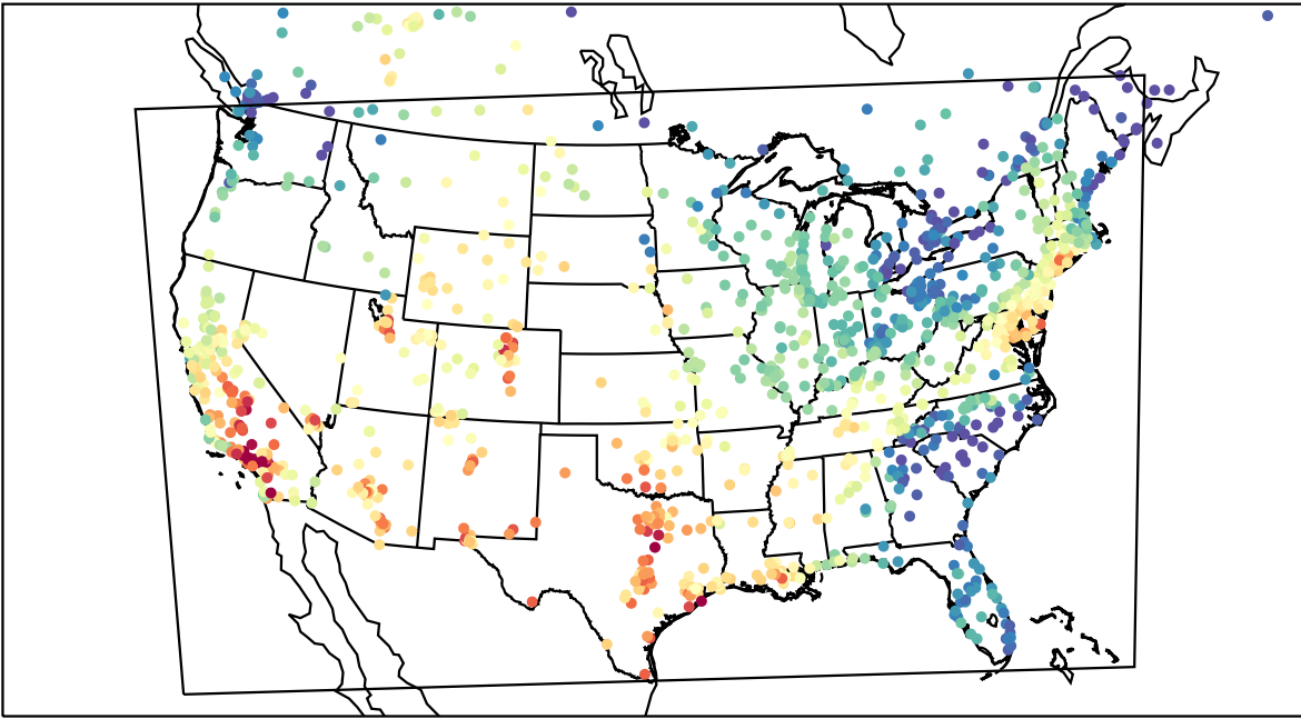
AirNOW (2023-08-30_19:00:00)
