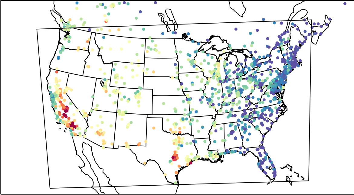
AirNOW (2023-08-29_01:00:00)
