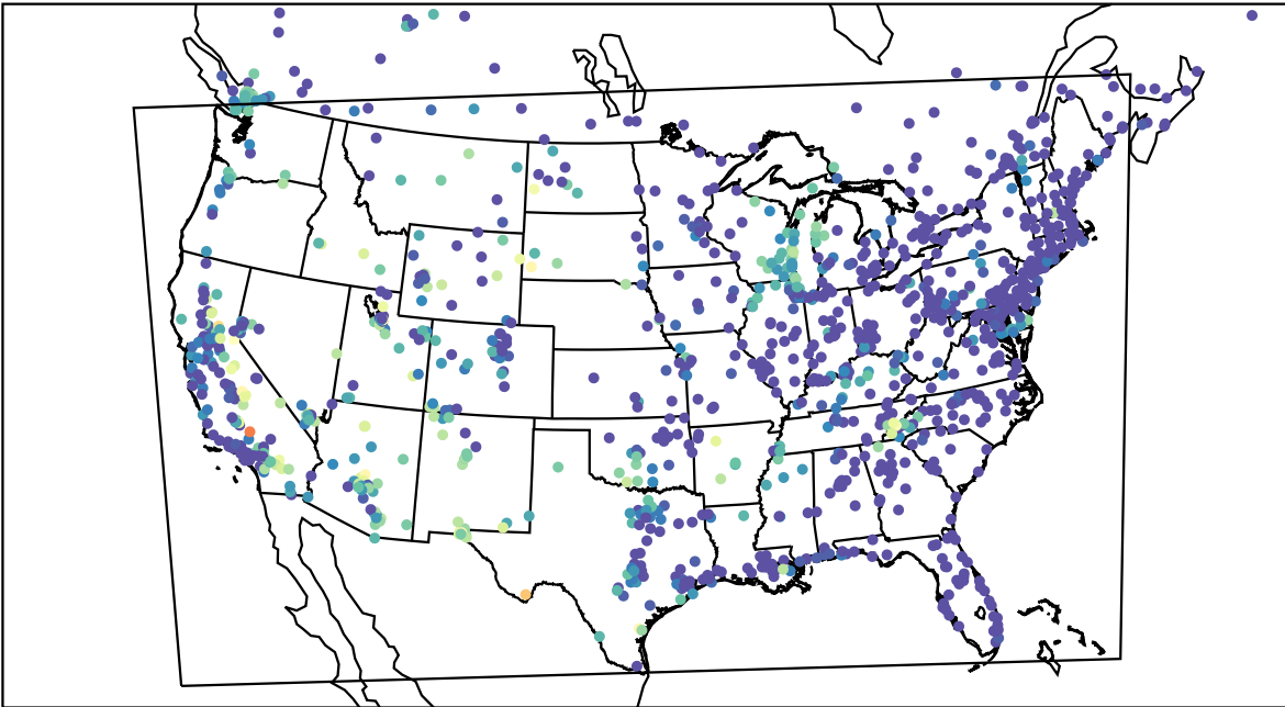
AirNOW (2023-08-29_10:00:00)
