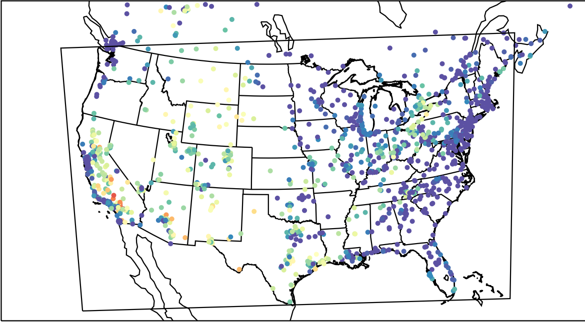
AirNOW (2023-08-30_05:00:00)
