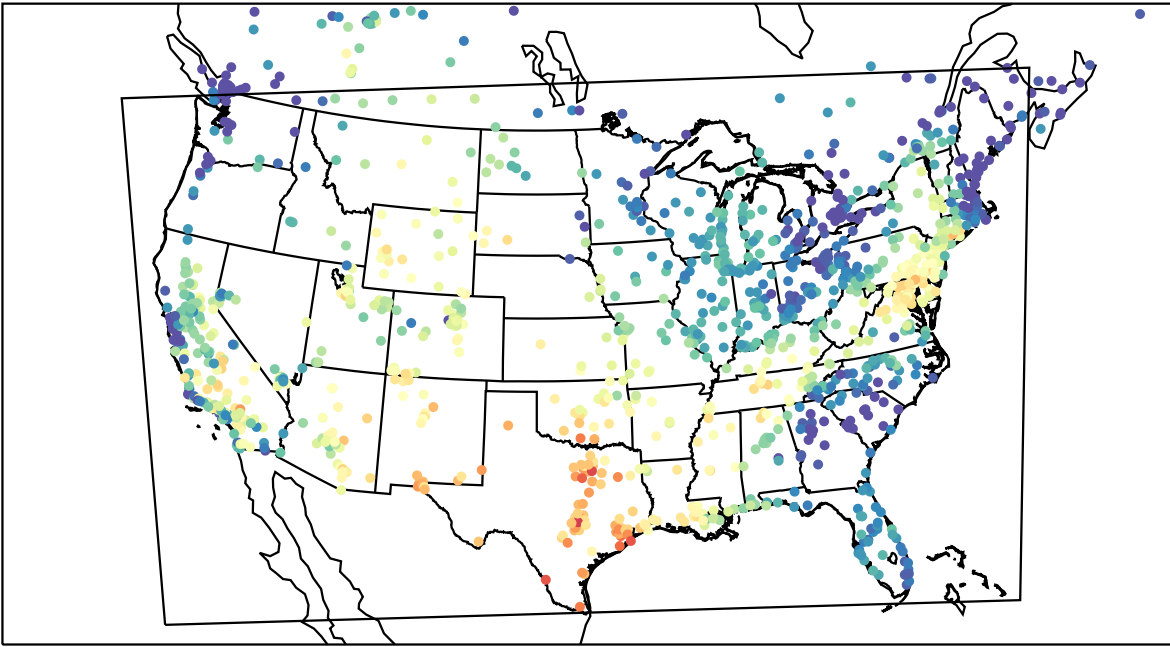
AirNOW (2023-08-30_16:00:00)
