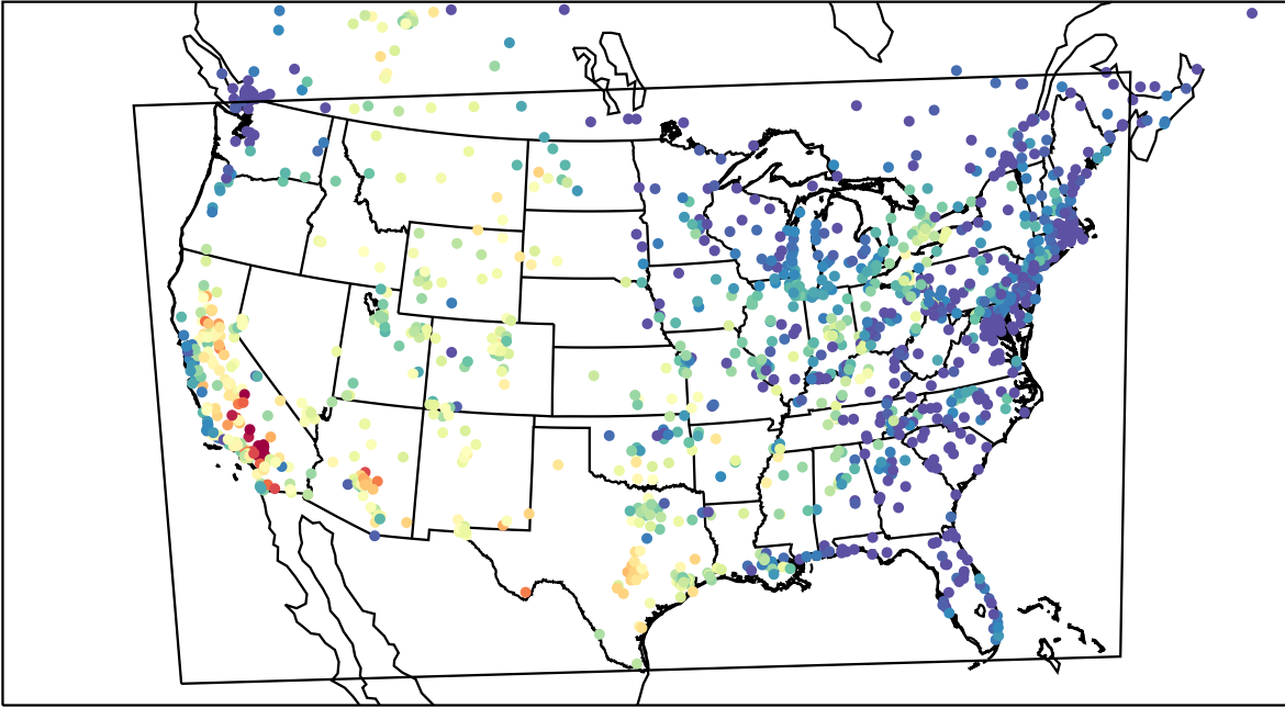
AirNOW (2023-08-30_02:00:00)
