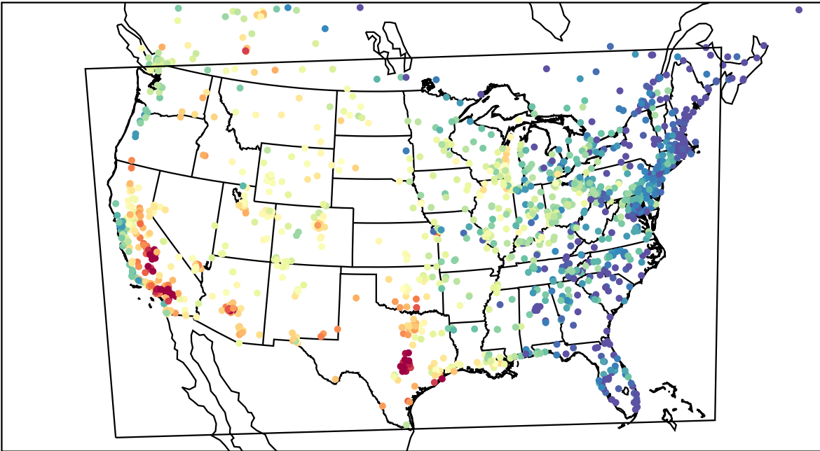
AirNOW (2023-08-29_00:00:00)
