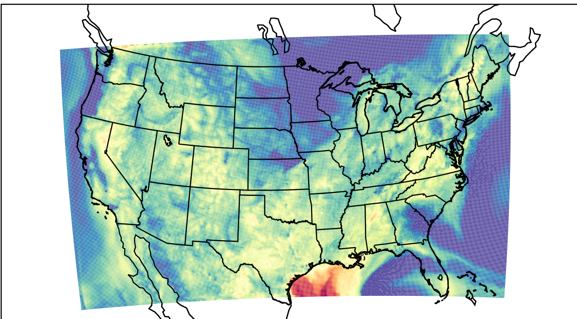
WRF (2023-08-29_14:00:00)
