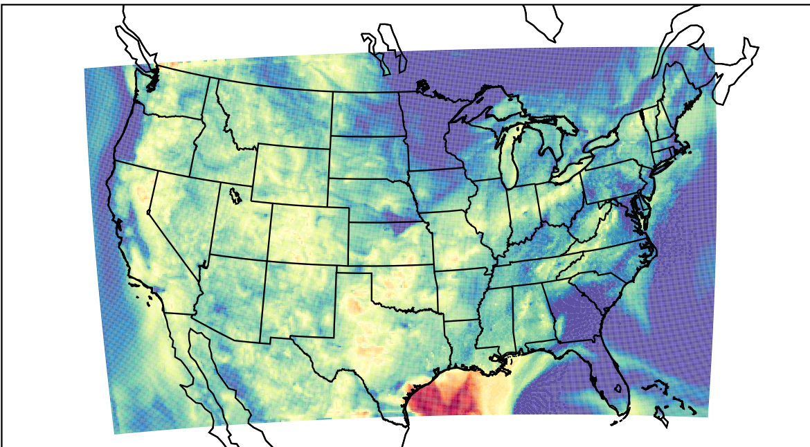
WRF (2023-08-29_11:00:00)
