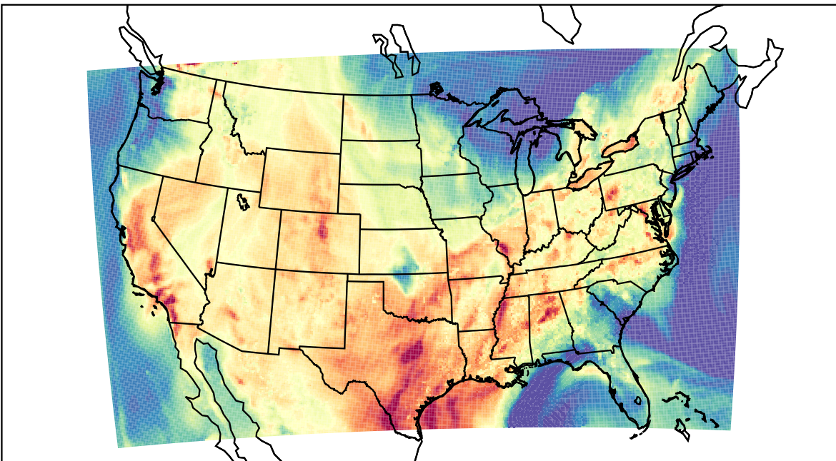
WRF (2023-08-29_23:00:00)
