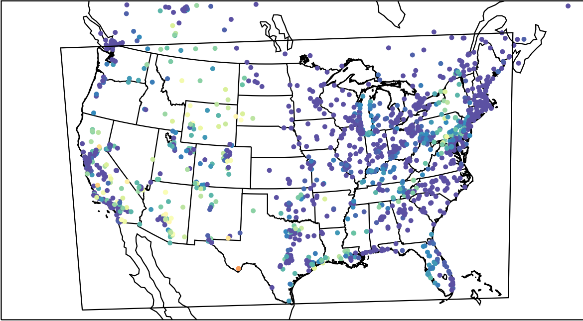
AirNOW (2023-08-30_12:00:00)
