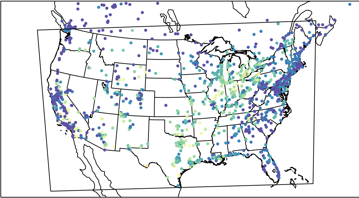
AirNOW (2023-08-29_14:00:00)
