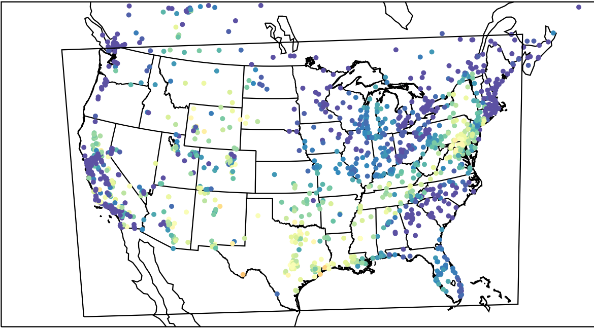
AirNOW (2023-08-30_14:00:00)
