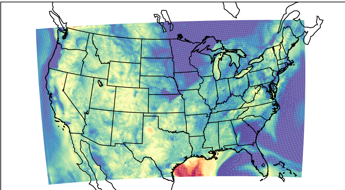
WRF (2023-08-29_13:00:00)
