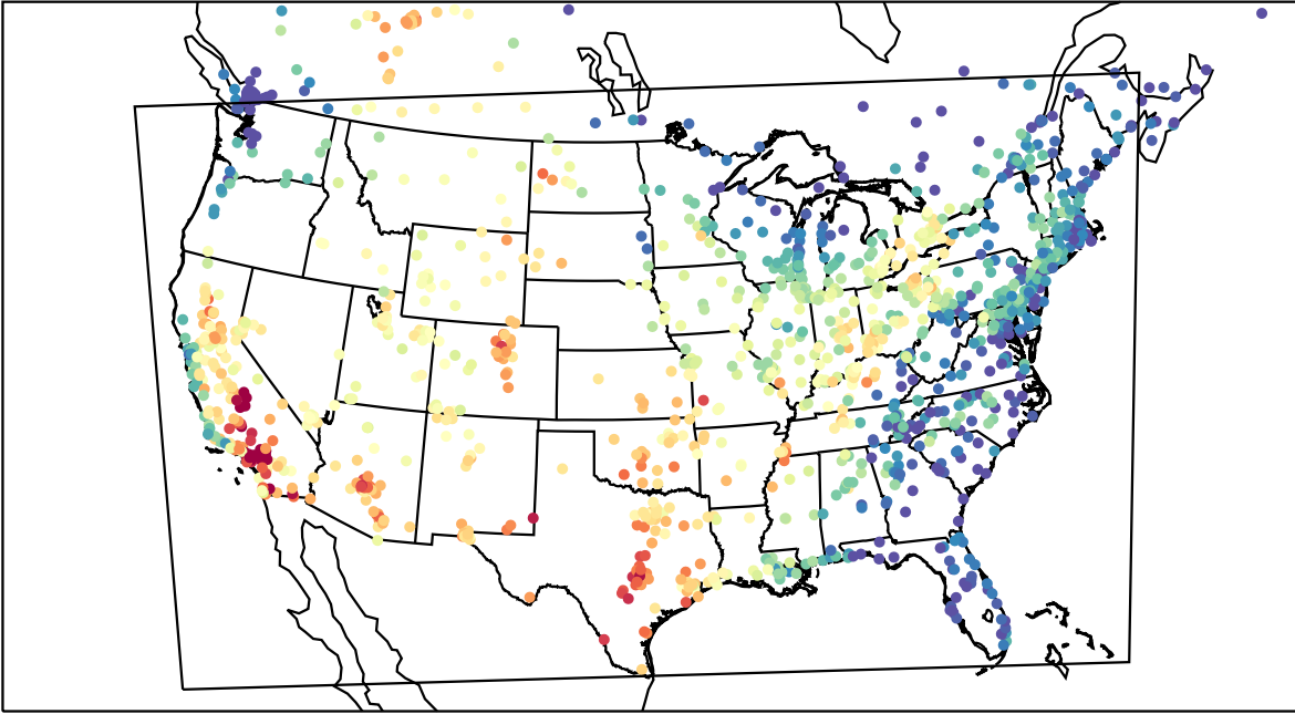
AirNOW (2023-08-29_23:00:00)
