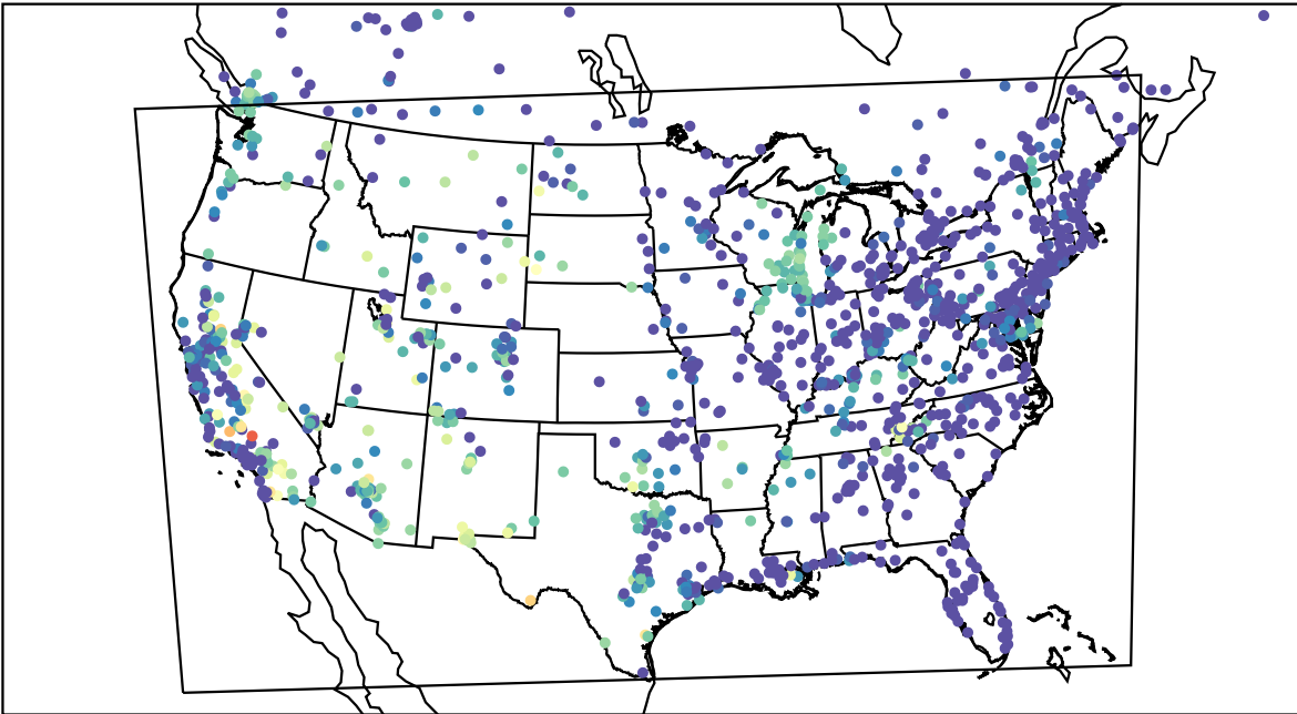
AirNOW (2023-08-29_09:00:00)
