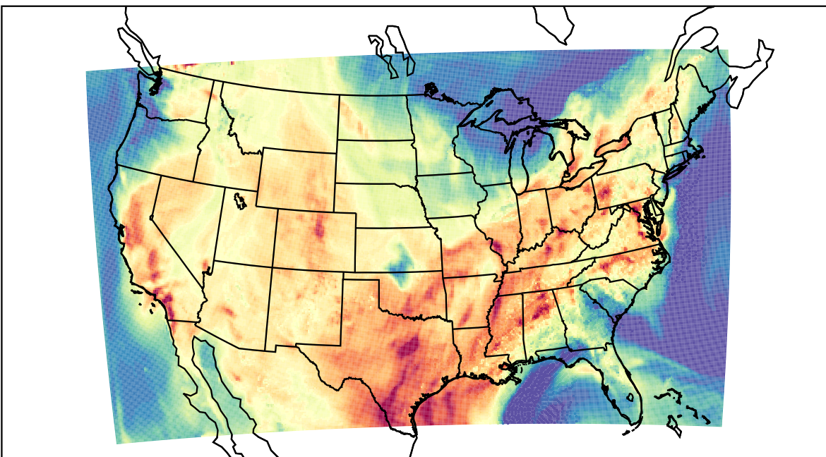
WRF (2023-08-29_22:00:00)
