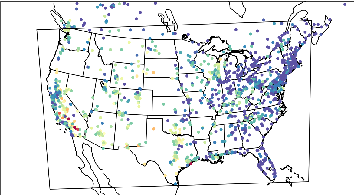
AirNOW (2023-08-29_04:00:00)
