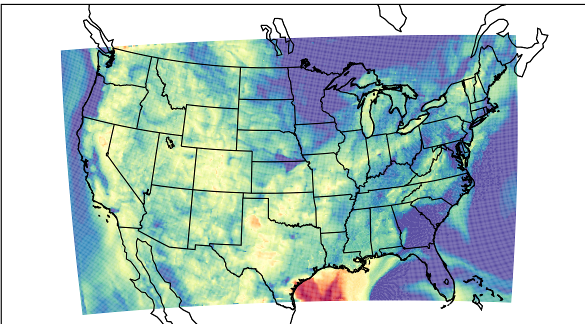
WRF (2023-08-29_12:00:00)
