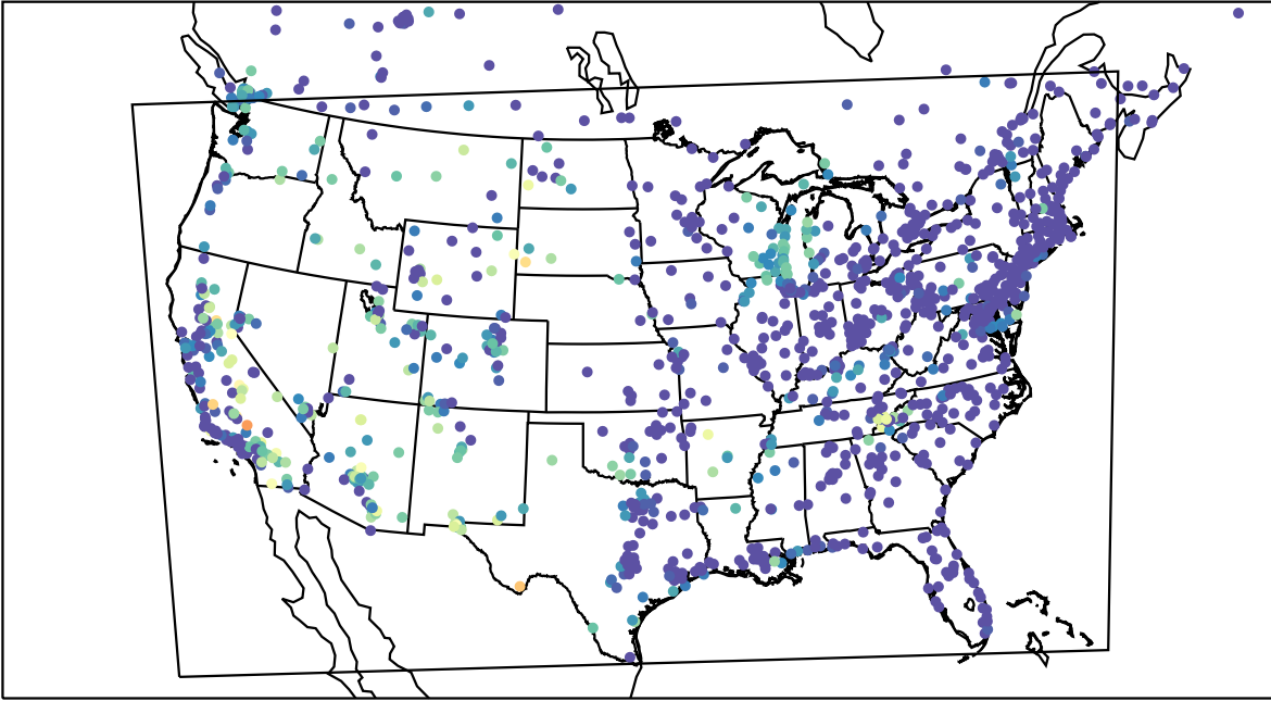
AirNOW (2023-08-29_11:00:00)
