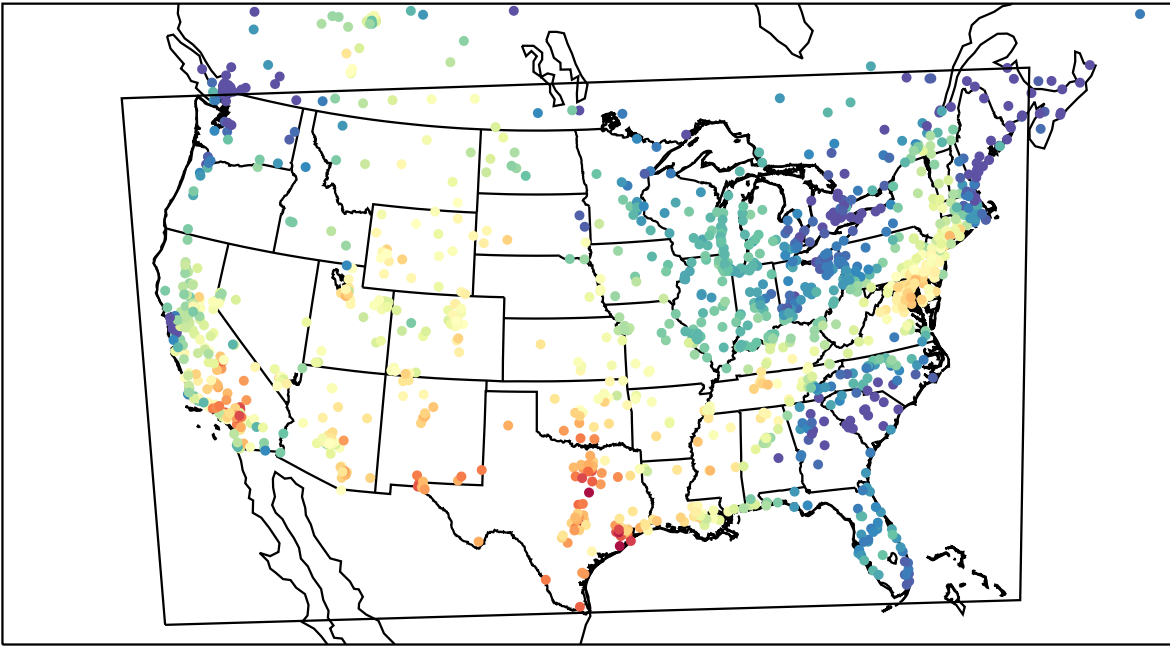
AirNOW (2023-08-30_17:00:00)
