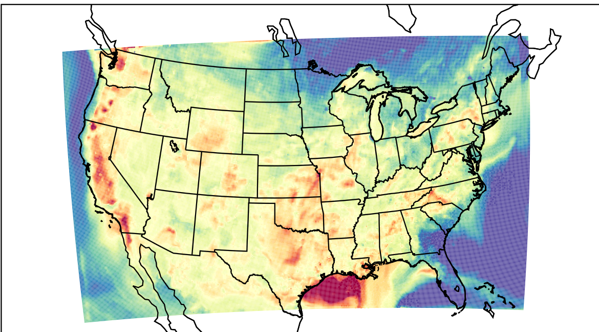
WRF (2023-08-29_01:00:00)
