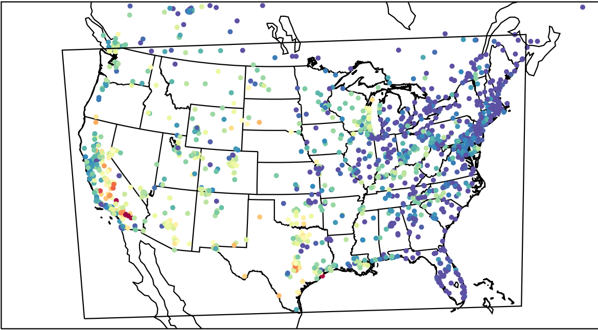
AirNOW (2023-08-29_03:00:00)
