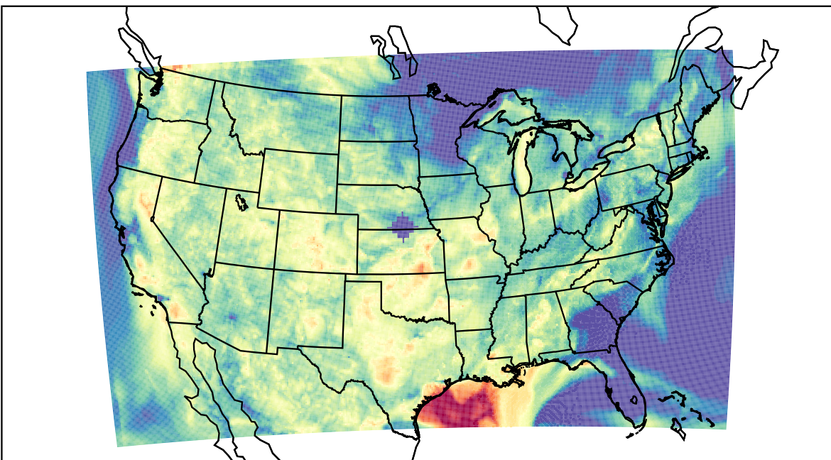
WRF (2023-08-29_07:00:00)
