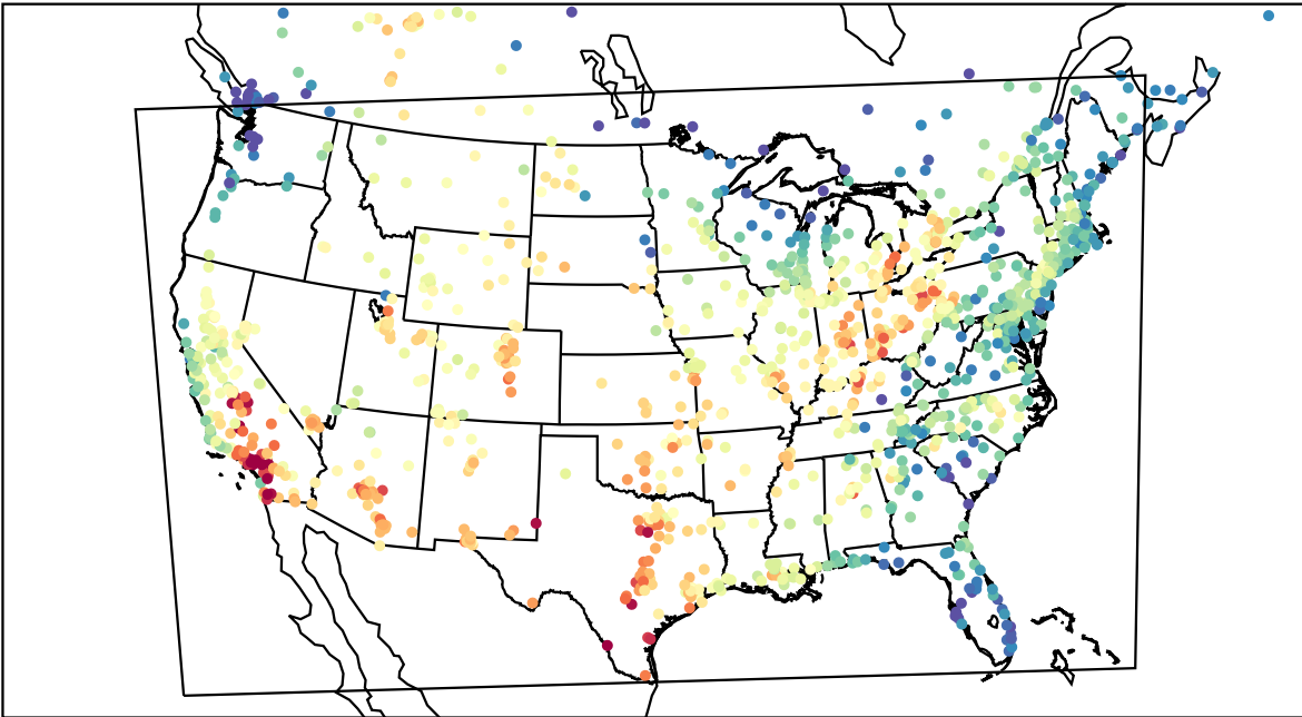
AirNOW (2023-08-29_19:00:00)
