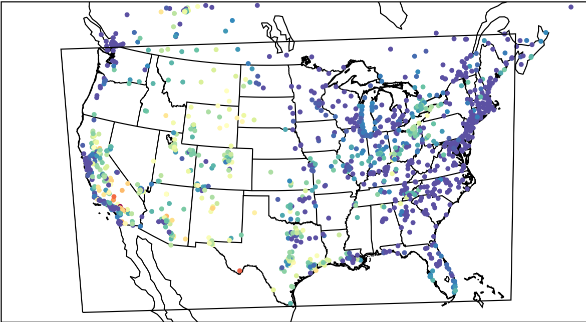
AirNOW (2023-08-30_06:00:00)
