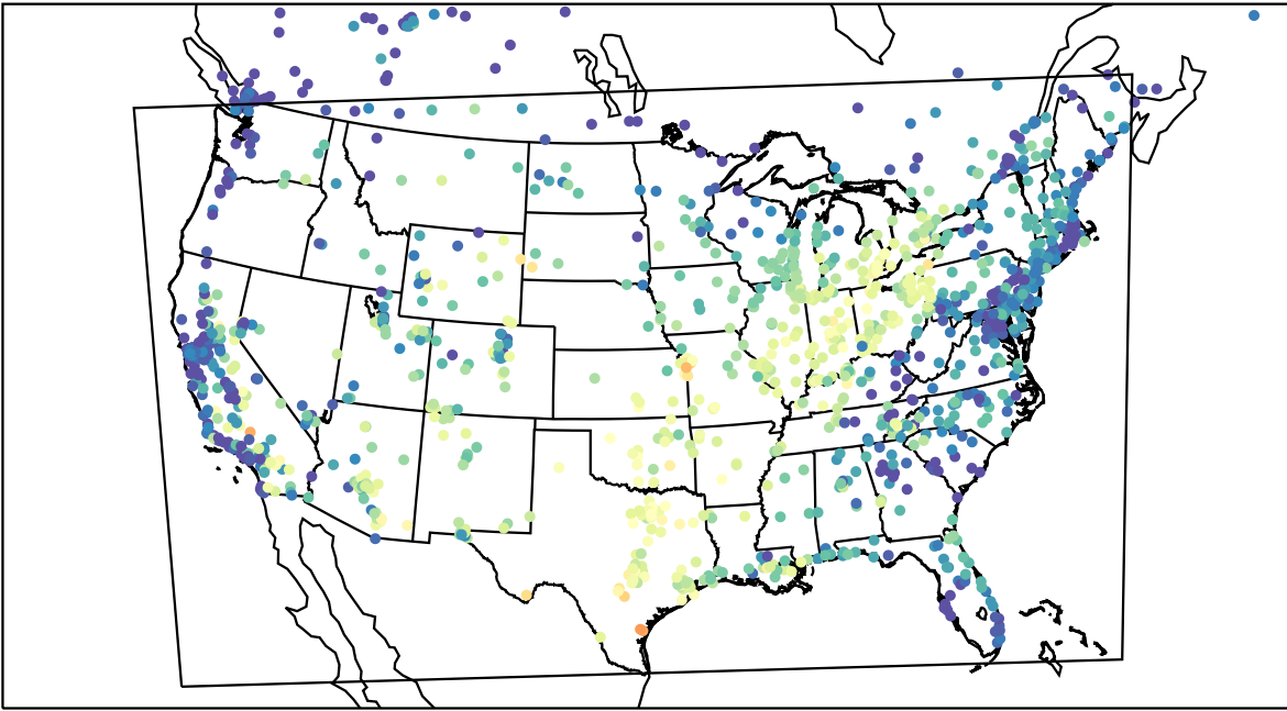
AirNOW (2023-08-29_15:00:00)
