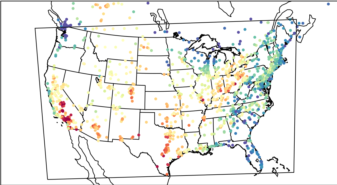
AirNOW (2023-08-29_21:00:00)
