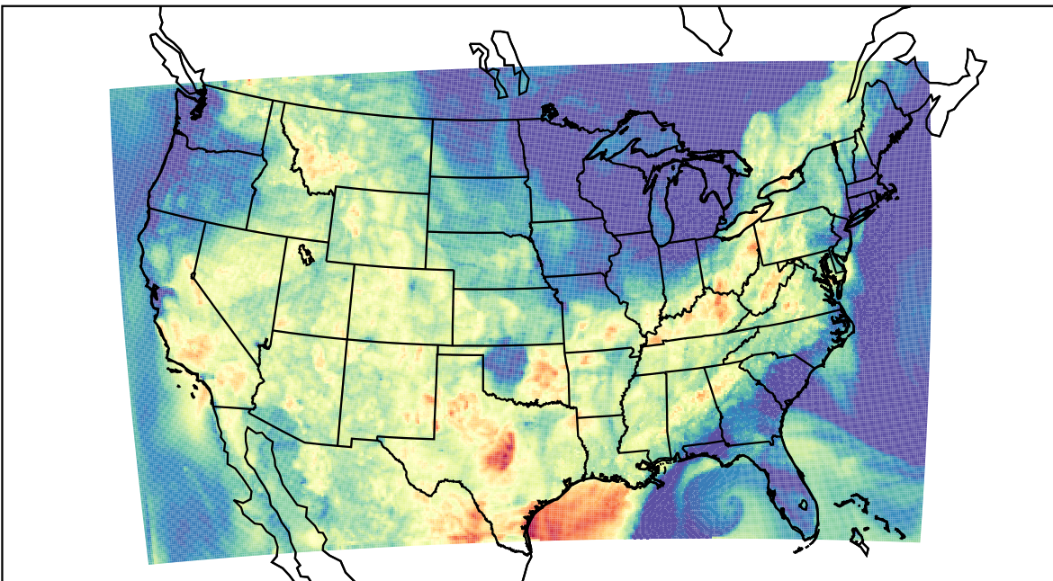
WRF (2023-08-30_05:00:00)
