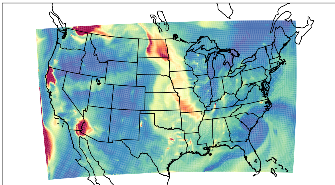
WRF 2023-08-31_05:00:00
