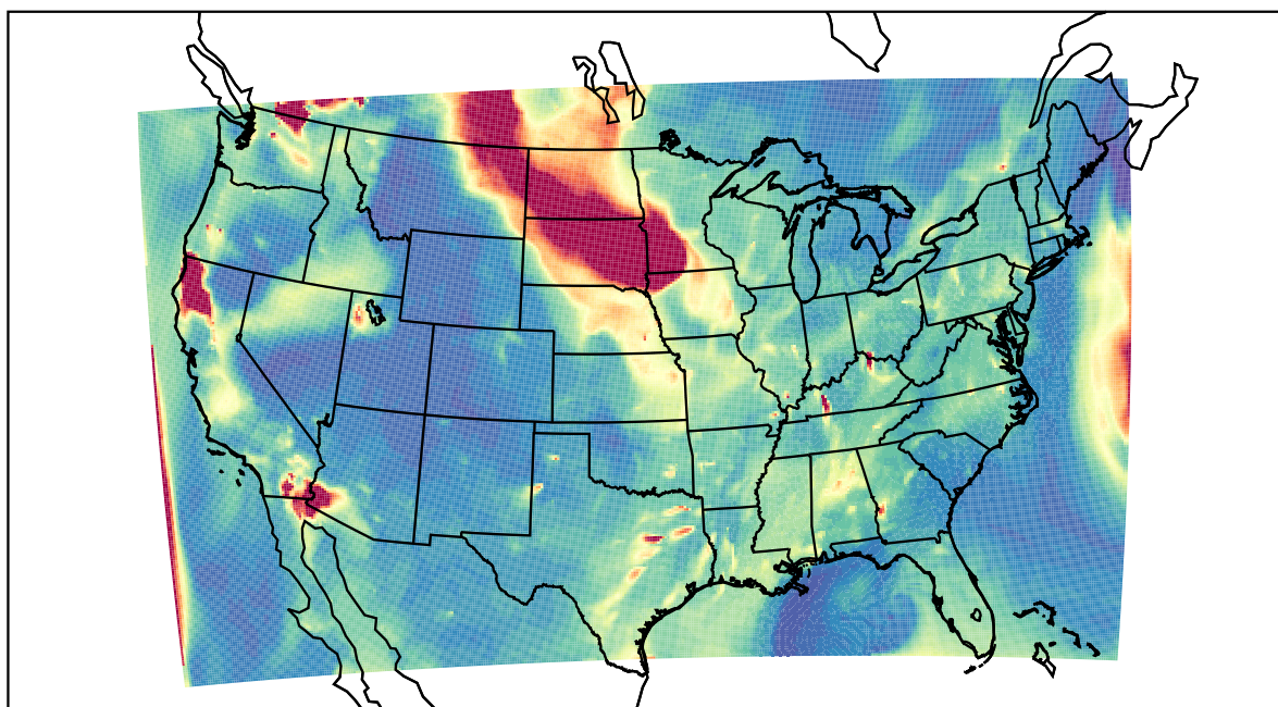
WRF 2023-08-30_05:00:00
