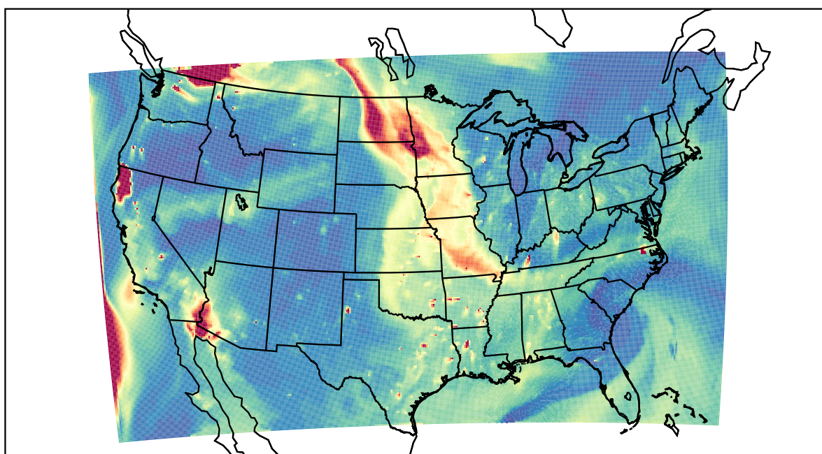
WRF 2023-08-31_02:00:00
