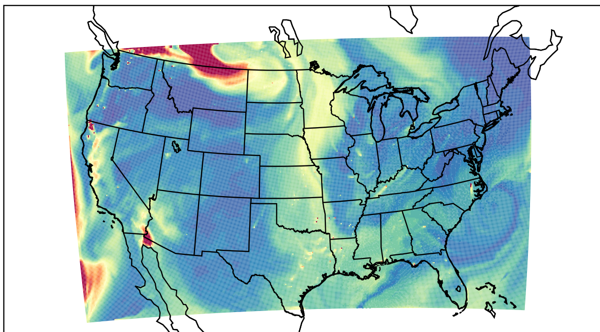
WRF 2023-08-31_21:00:00
