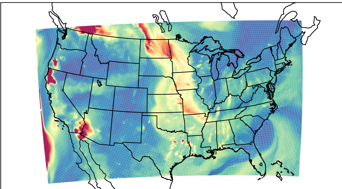
WRF 2023-08-31_05:00:00
