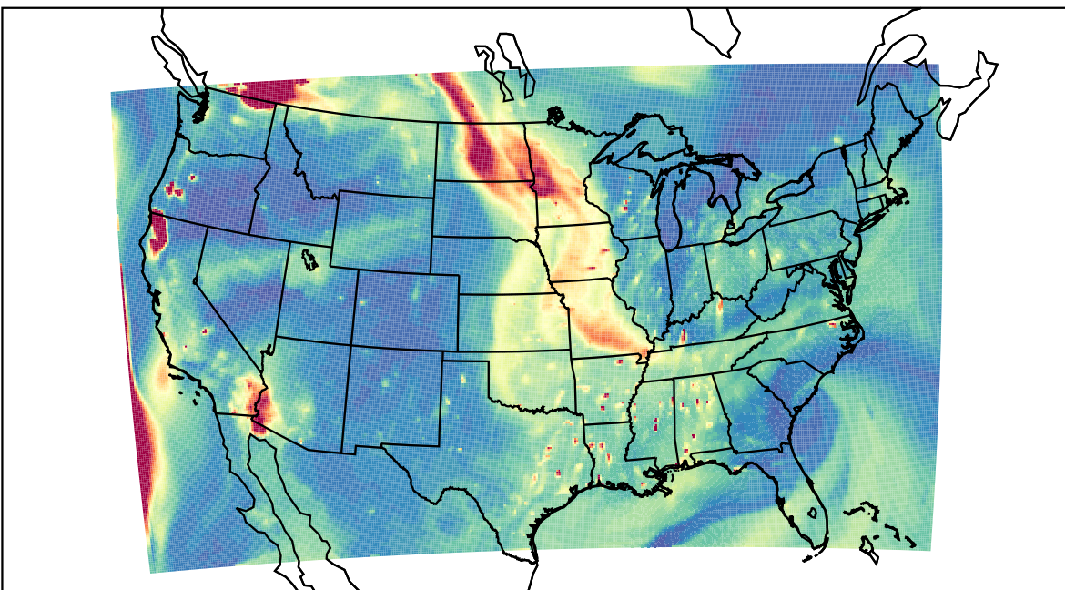
WRF 2023-08-31_02:00:00
