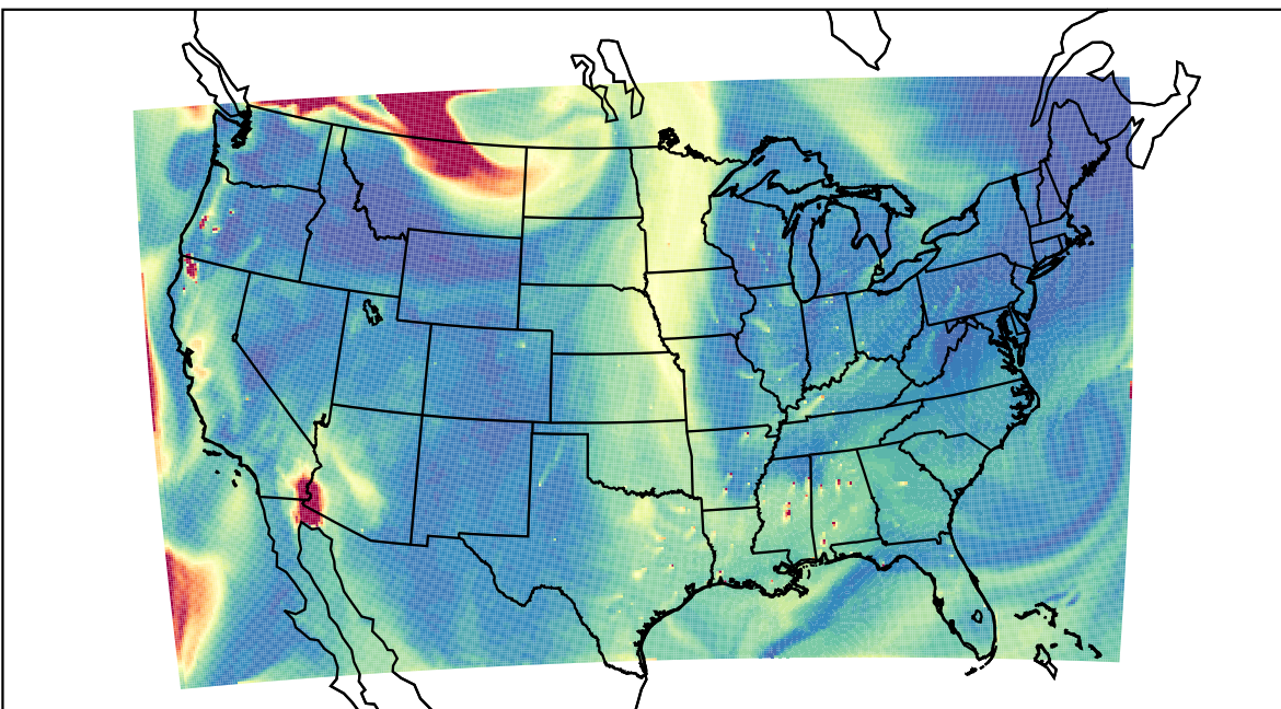
WRF 2023-08-31_21:00:00
