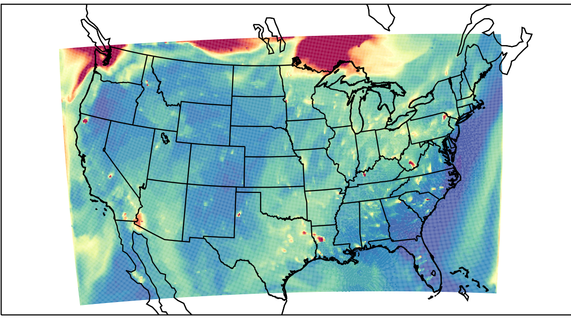
WRF 2023-09-03_02:00:00
