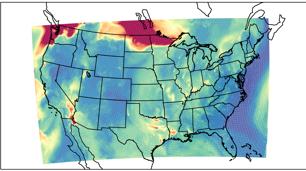
WRF 2023-09-02_09:00:00
