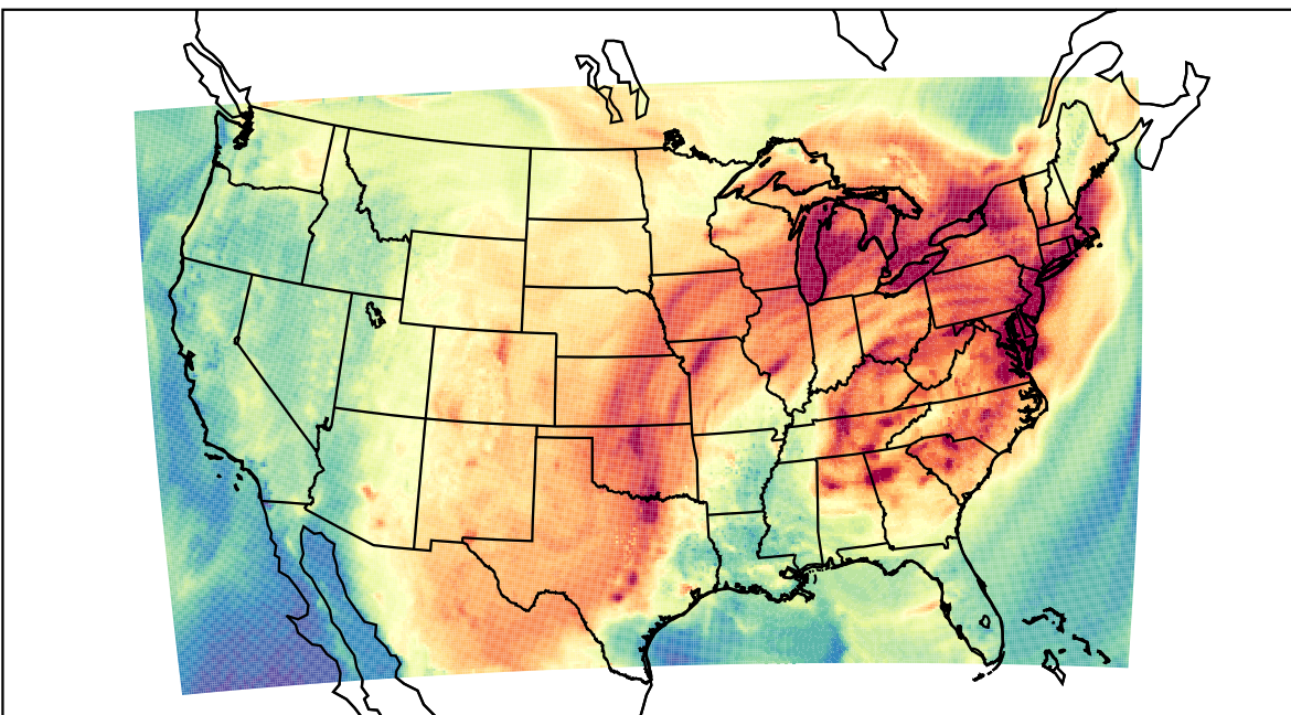
WRF (2023-09-03_20:00:00)
