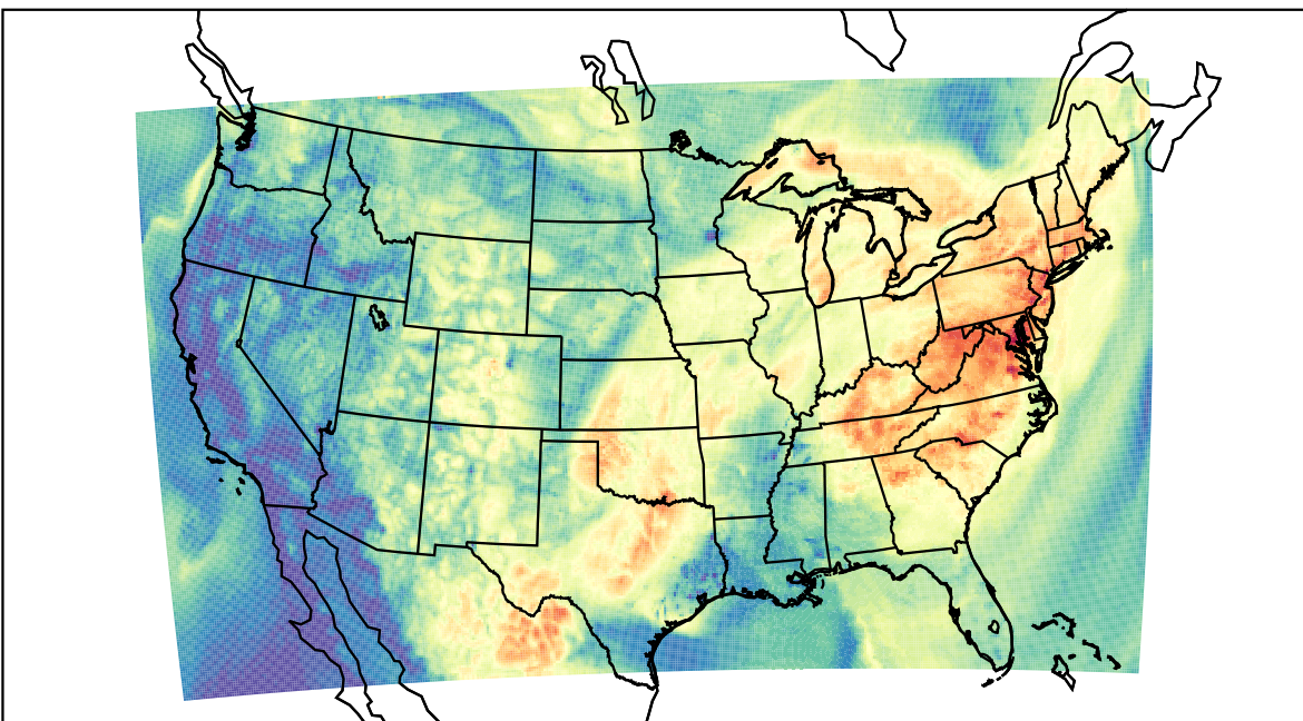
WRF (2023-09-03_15:00:00)
