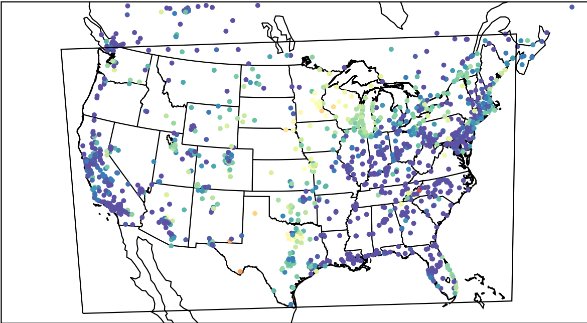
AirNOW (2023-09-03_09:00:00)
