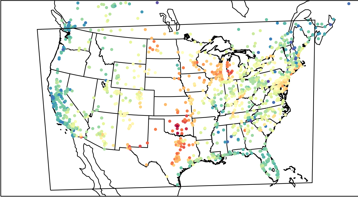
AirNOW (2023-09-03_22:00:00)
