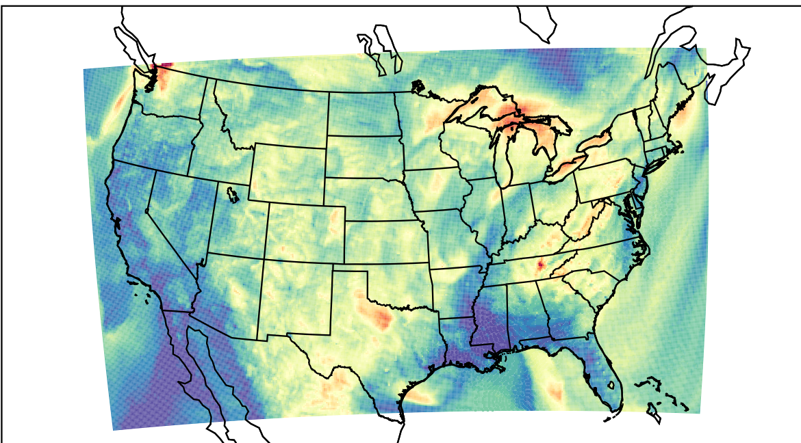
WRF (2023-09-03_06:00:00)
