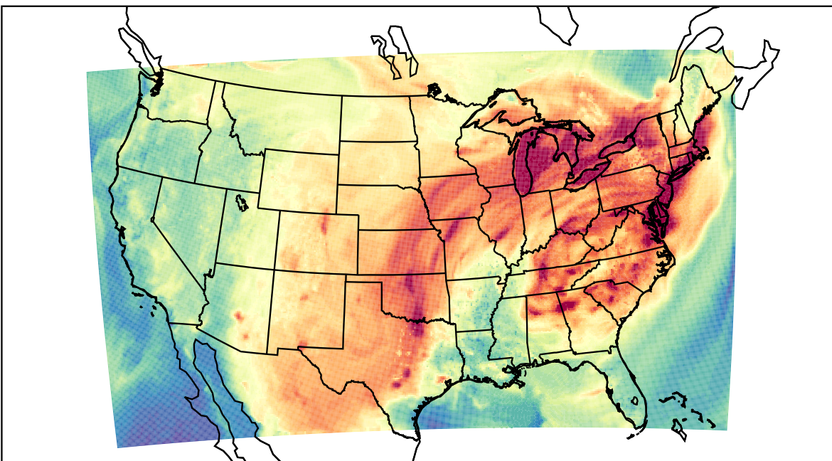
WRF (2023-09-03_21:00:00)
