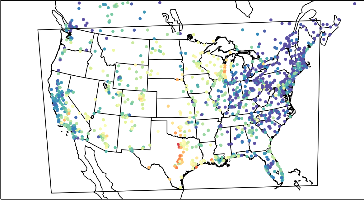
AirNOW (2023-09-02_02:00:00)
