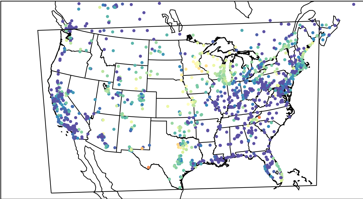
AirNOW (2023-09-03_08:00:00)
