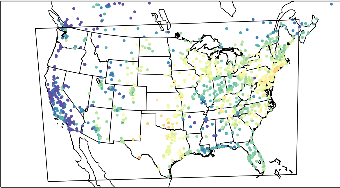
AirNOW (2023-09-03_15:00:00)
