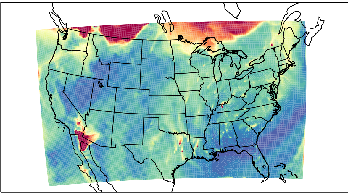
WRF 2023-09-04_12:00:00
