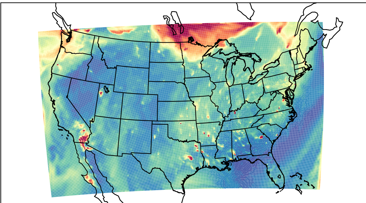
WRF 2023-09-04_02:00:00
