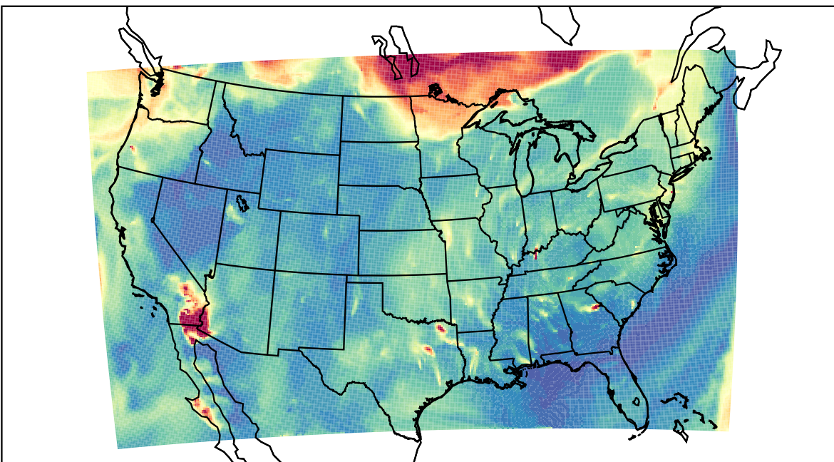
WRF 2023-09-04_05:00:00
