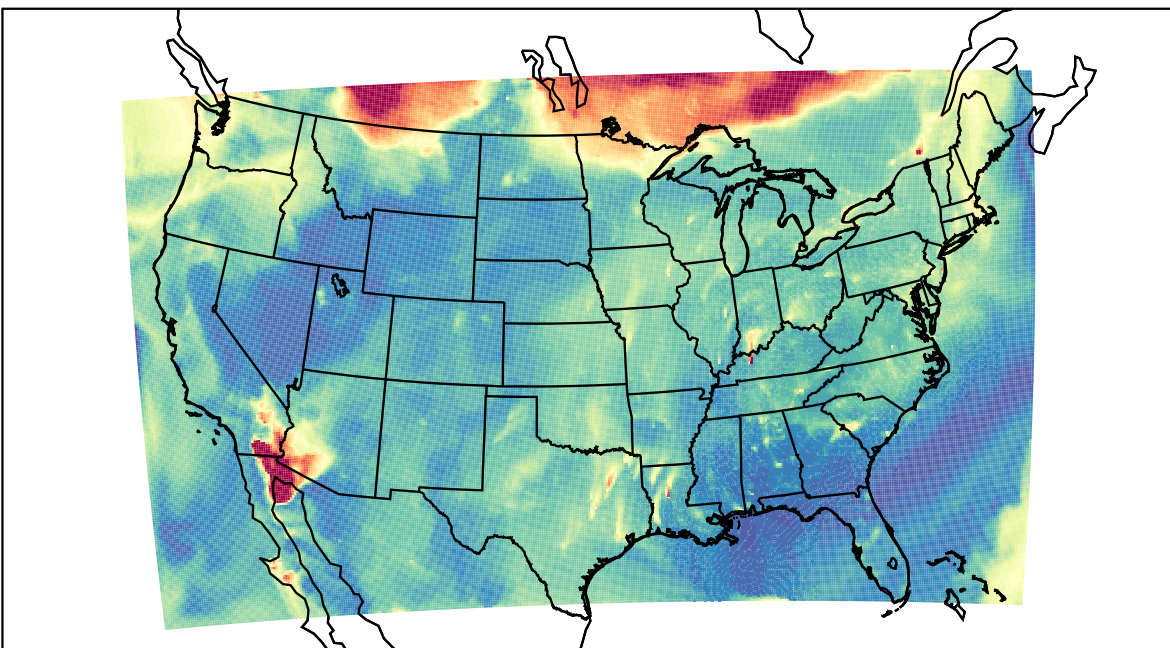
WRF 2023-09-04_12:00:00
