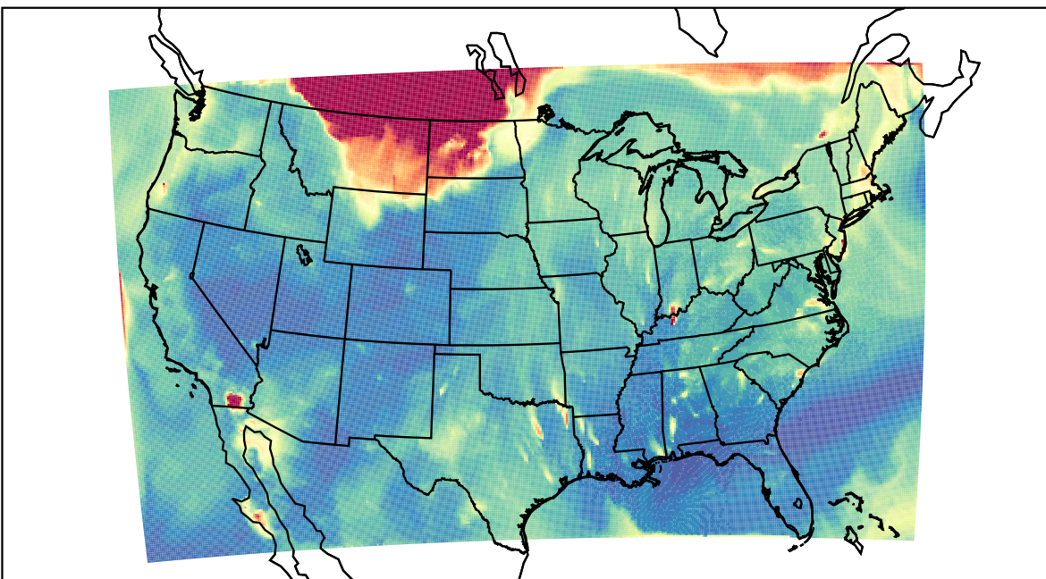
WRF 2023-09-05_05:00:00
