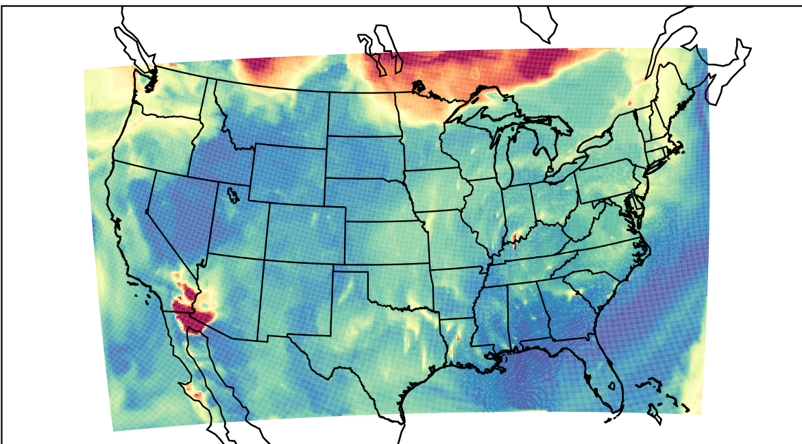
WRF 2023-09-04_09:00:00
