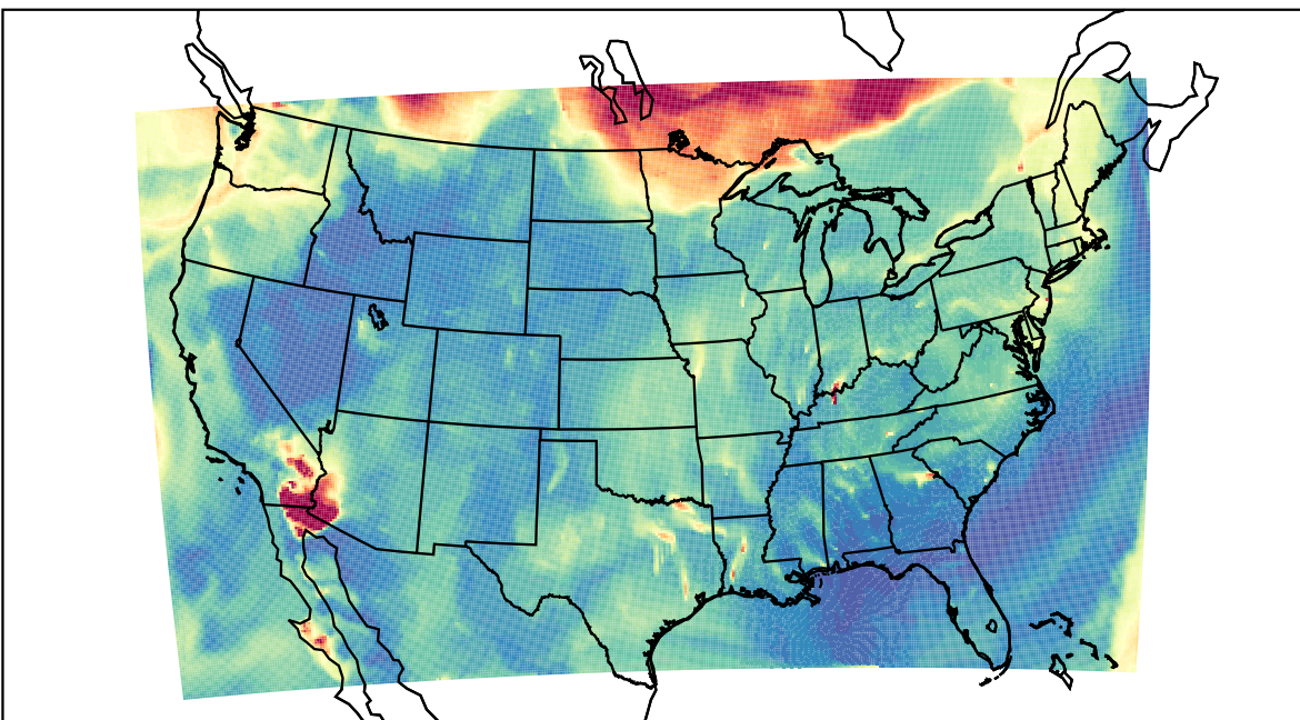
WRF 2023-09-04_07:00:00
