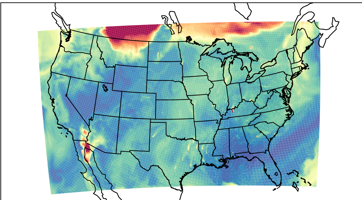
WRF 2023-09-04_17:00:00
