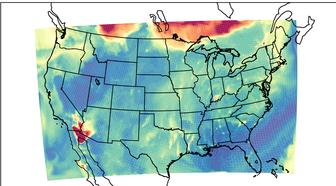
WRF 2023-09-04_11:00:00
