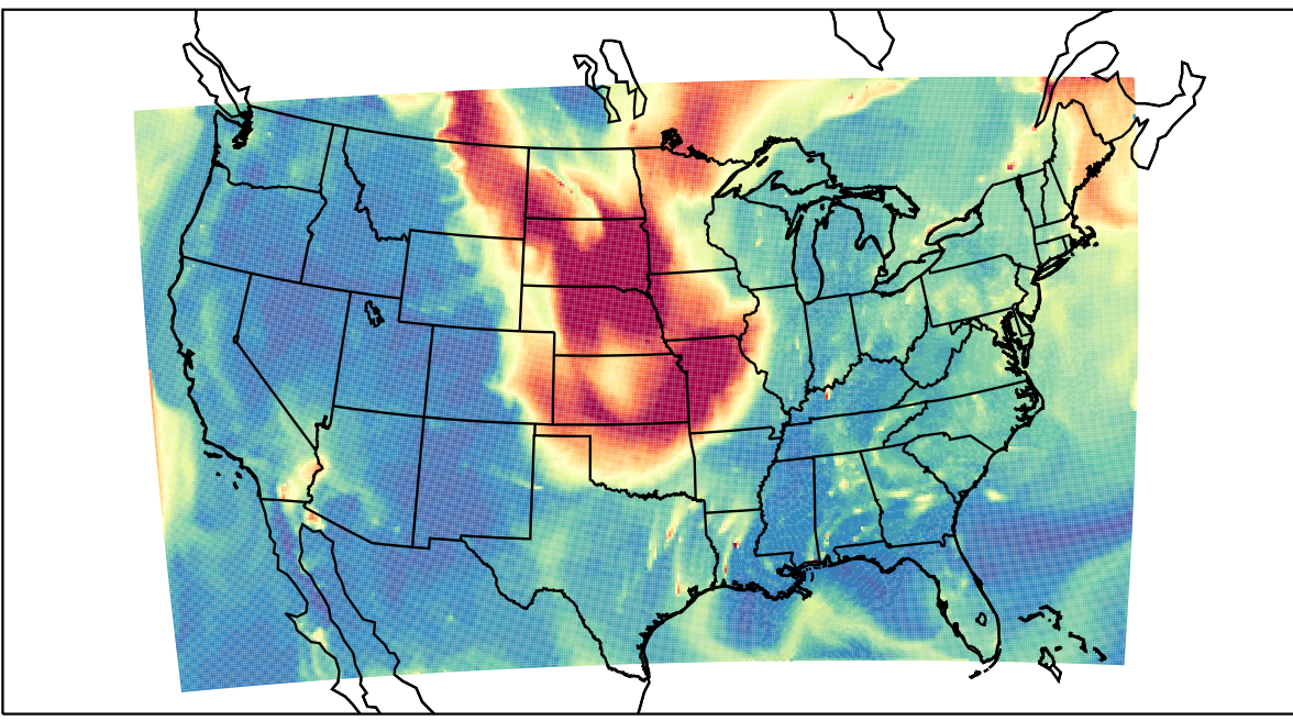
WRF 2023-09-06_12:00:00
