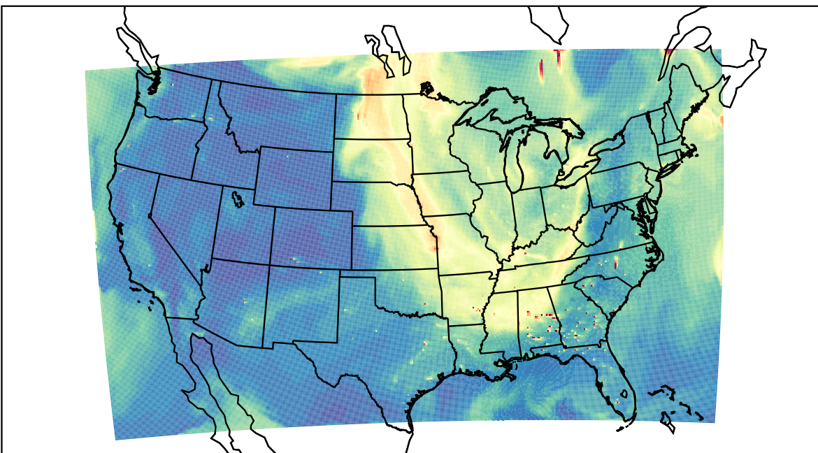
WRF 2023-09-07_21:00:00
