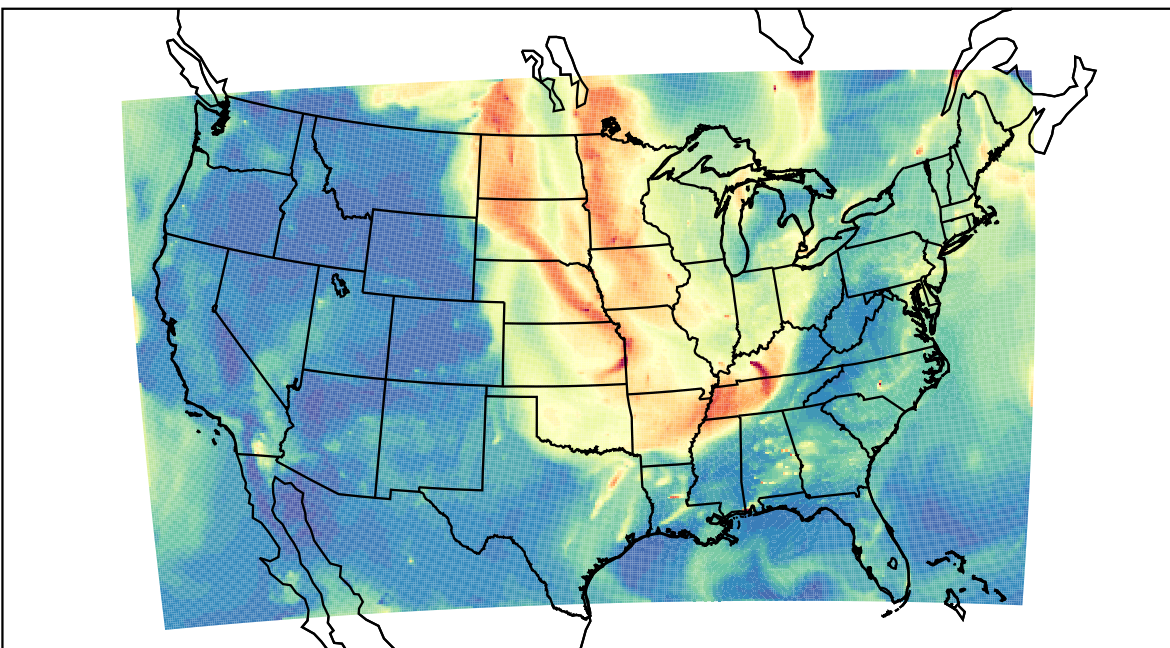
WRF 2023-09-07_11:00:00
