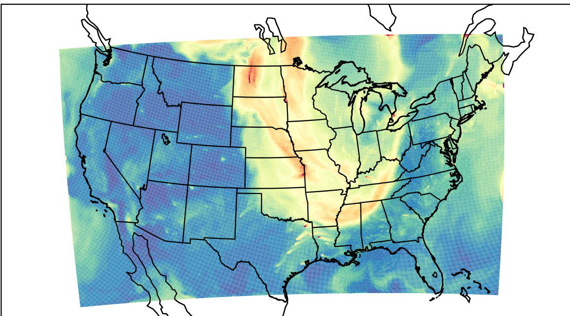
WRF 2023-09-07_16:00:00
