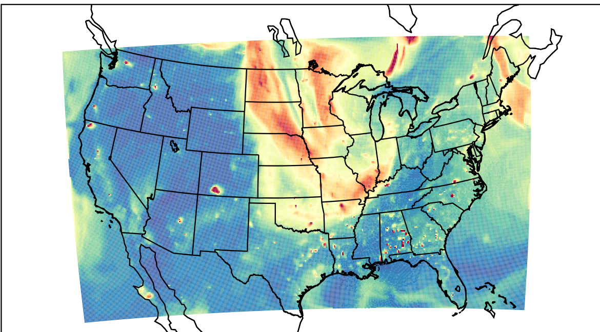
WRF 2023-09-07_02:00:00
