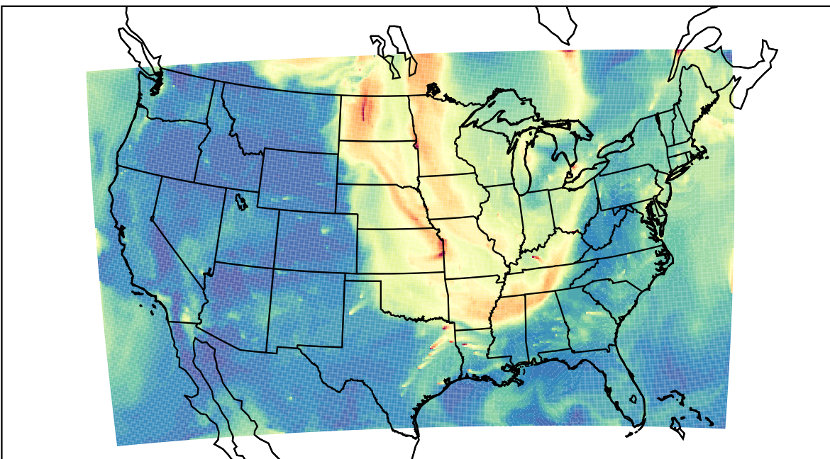
WRF 2023-09-07_15:00:00
