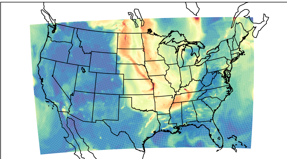
WRF 2023-09-07_13:00:00
