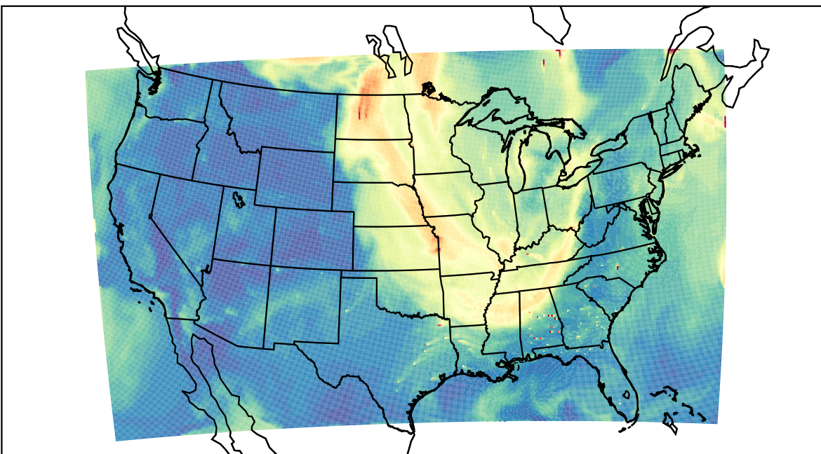
WRF 2023-09-07_18:00:00
