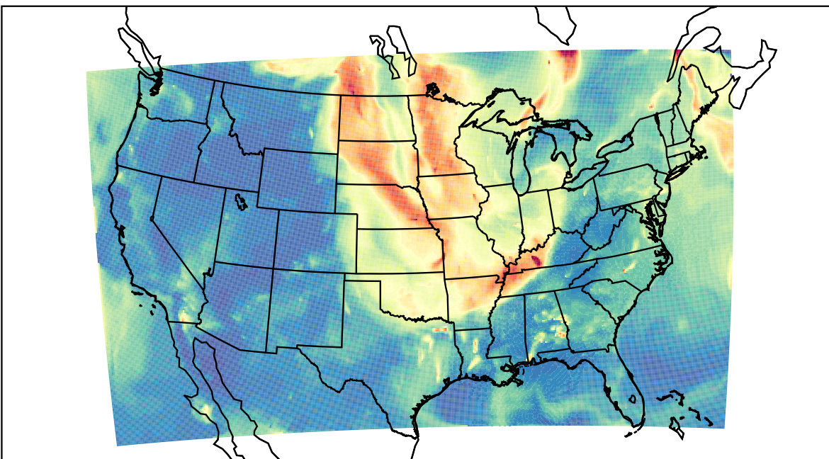
WRF 2023-09-07_07:00:00
