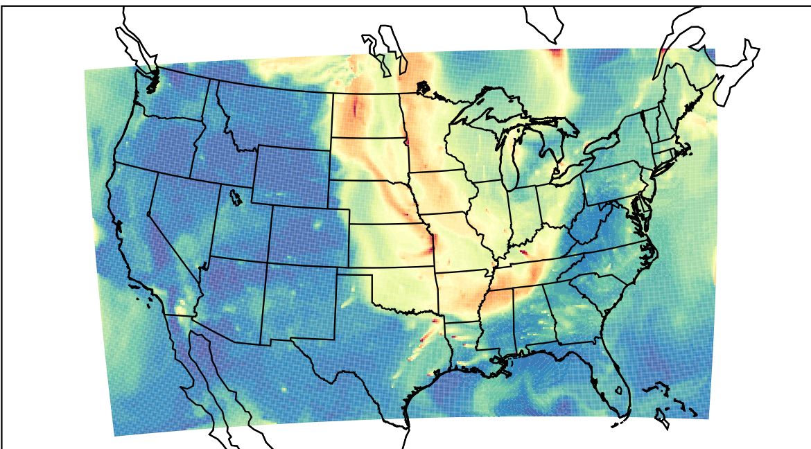
WRF 2023-09-07_14:00:00
