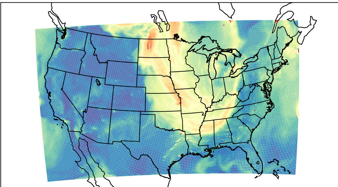
WRF 2023-09-07_17:00:00
