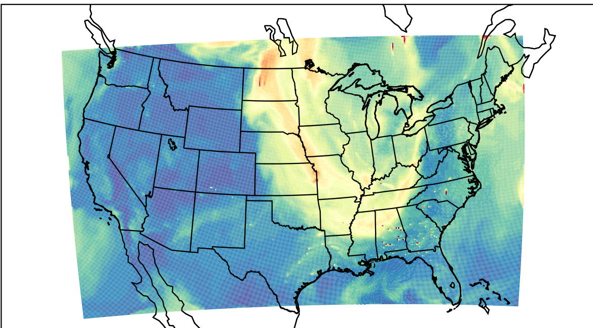
WRF 2023-09-07_19:00:00
