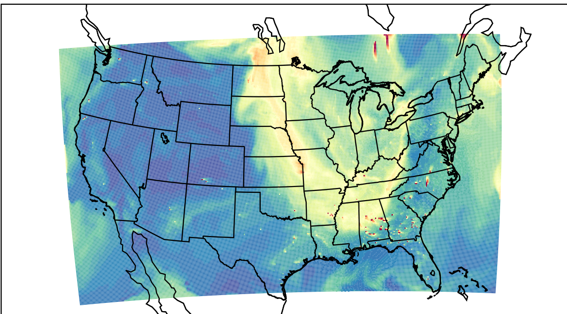
WRF 2023-09-07_22:00:00
