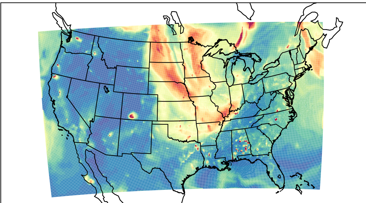
WRF 2023-09-07_03:00:00
