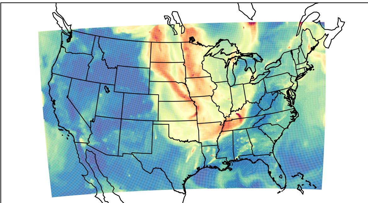
WRF 2023-09-07_10:00:00
