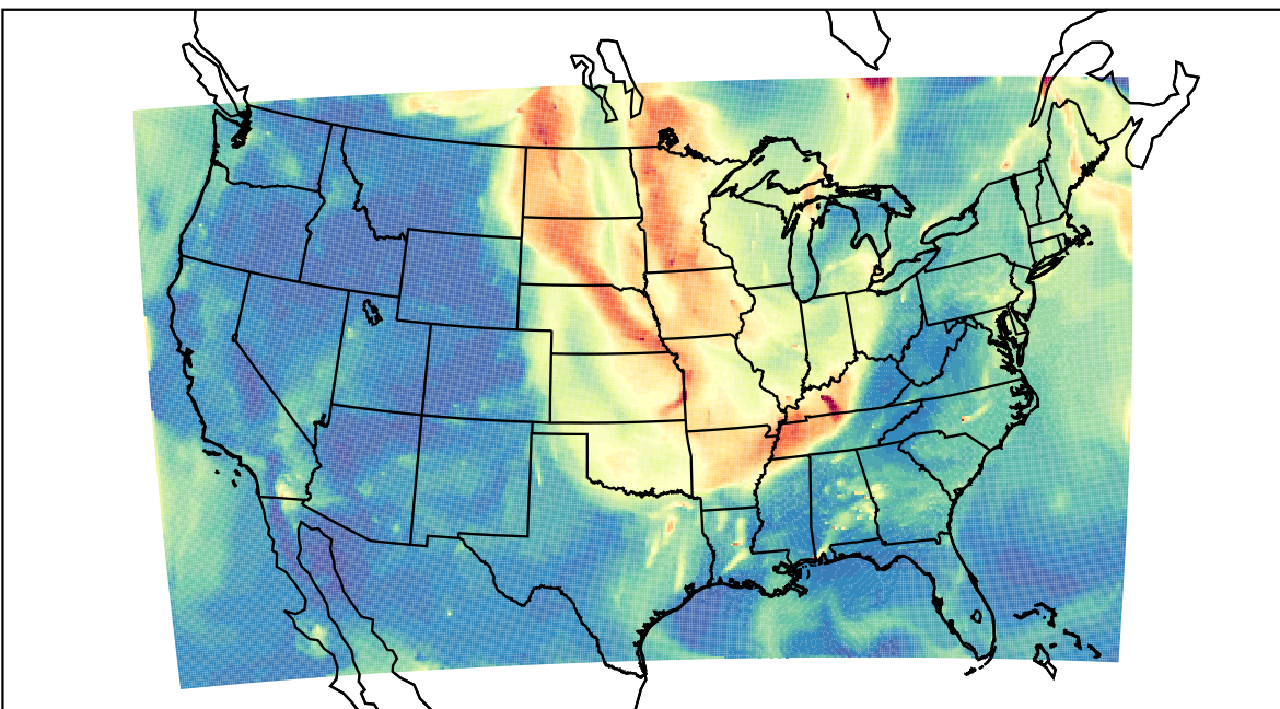
WRF 2023-09-07_09:00:00
