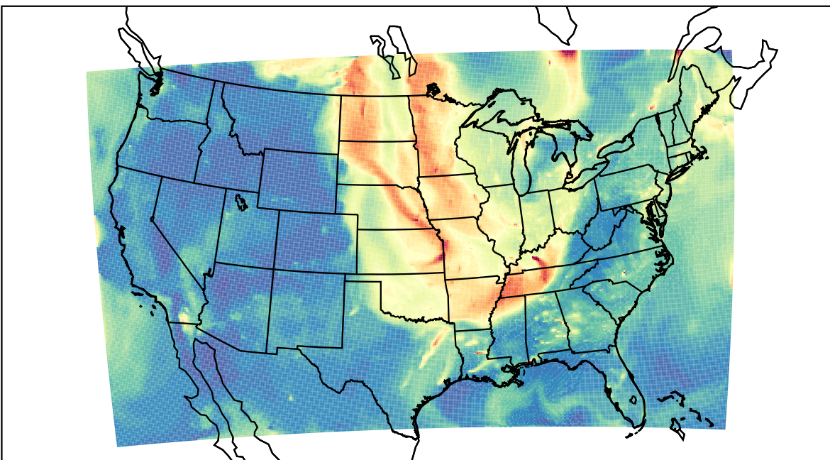
WRF 2023-09-07_12:00:00
