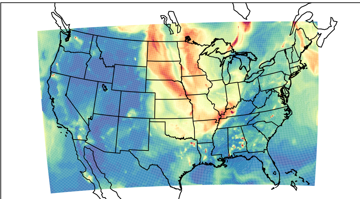
WRF 2023-09-07_05:00:00
