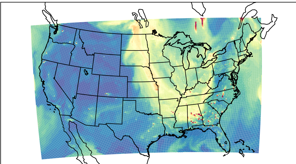
WRF 2023-09-07_23:00:00
