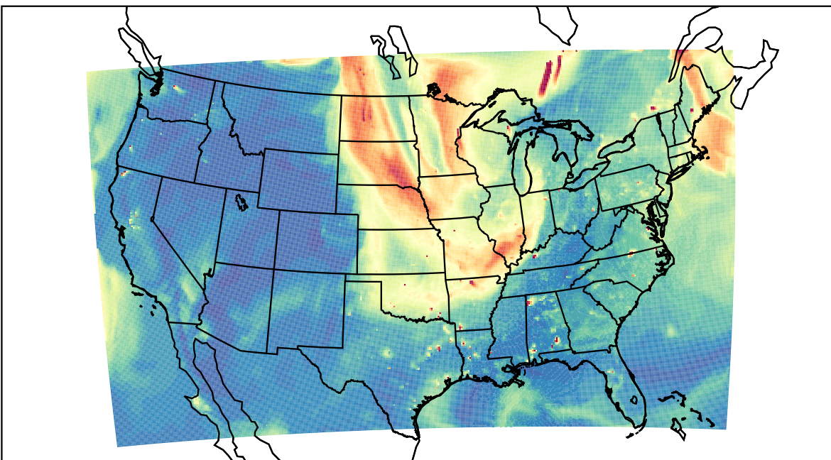
WRF 2023-09-07_00:00:00
