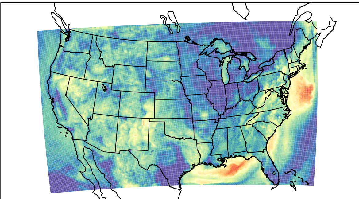
WRF (2023-09-09_13:00:00)
