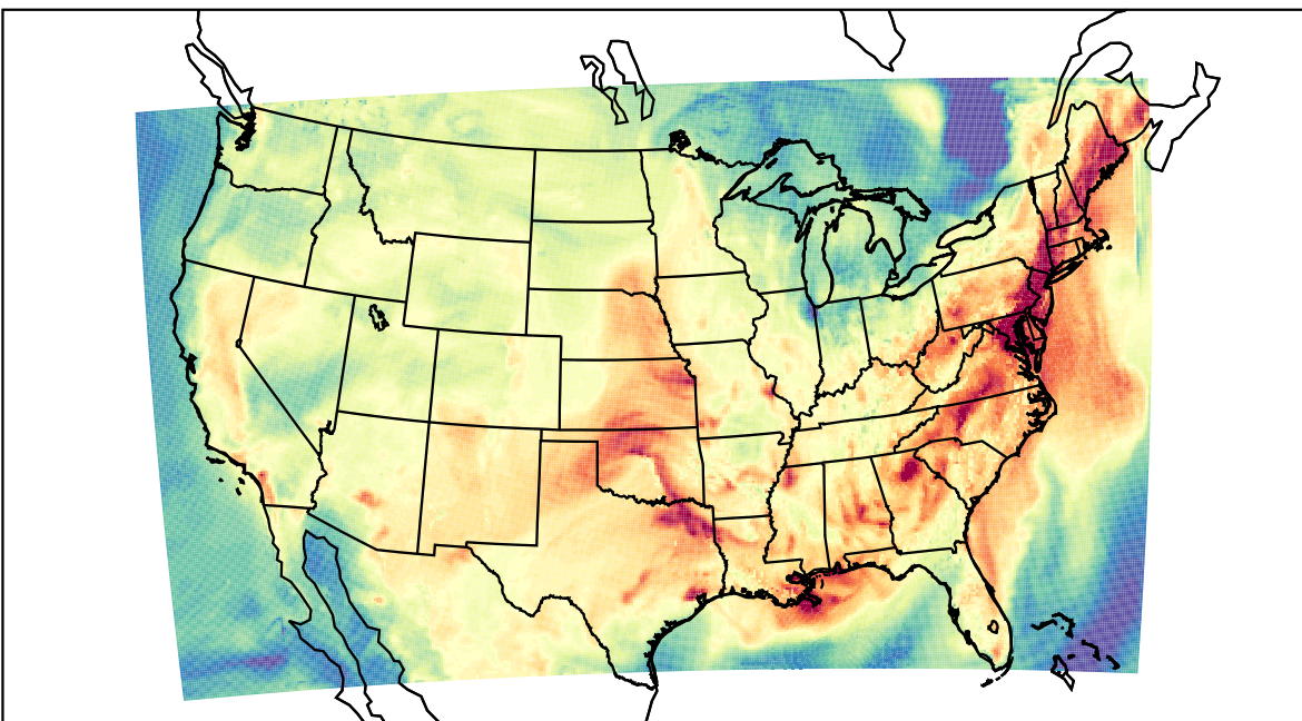
WRF (2023-09-08_21:00:00)
