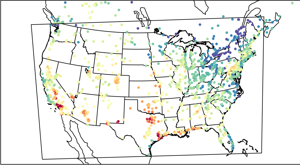
AirNOW (2023-09-09_20:00:00)
