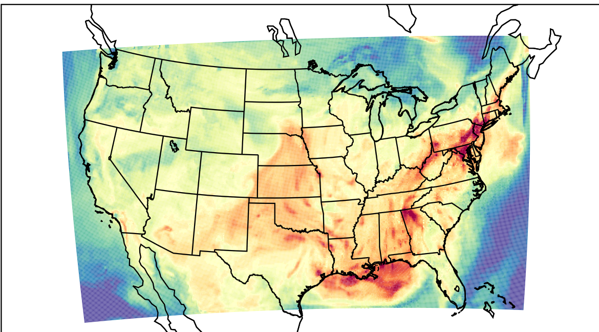
WRF (2023-09-09_19:00:00)
