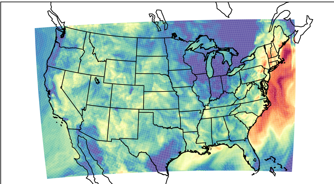
WRF (2023-09-08_07:00:00)
