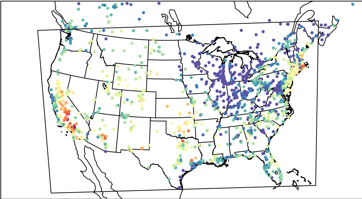
AirNOW (2023-09-08_01:00:00)
