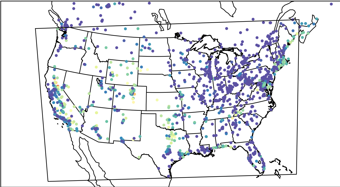
AirNOW (2023-09-09_08:00:00)
