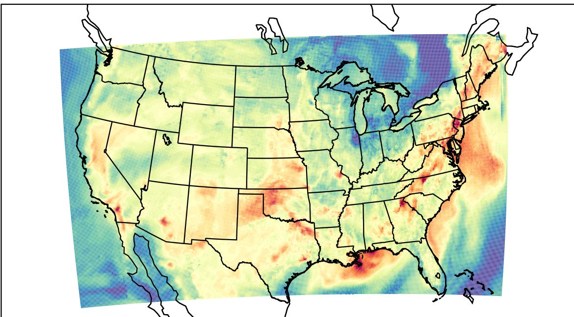
WRF (2023-09-09_00:00:00)
