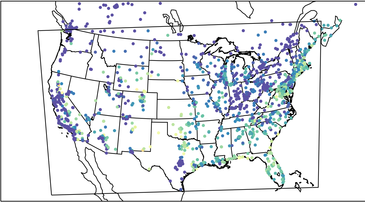
AirNOW (2023-09-09_14:00:00)
