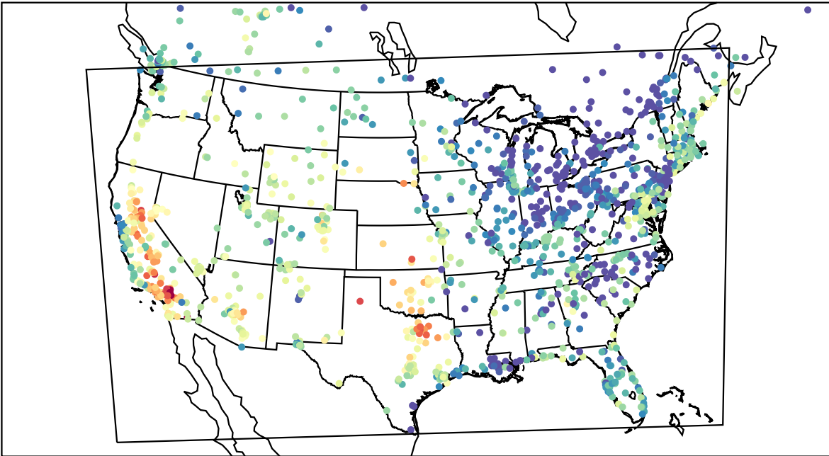
AirNOW (2023-09-09_01:00:00)
