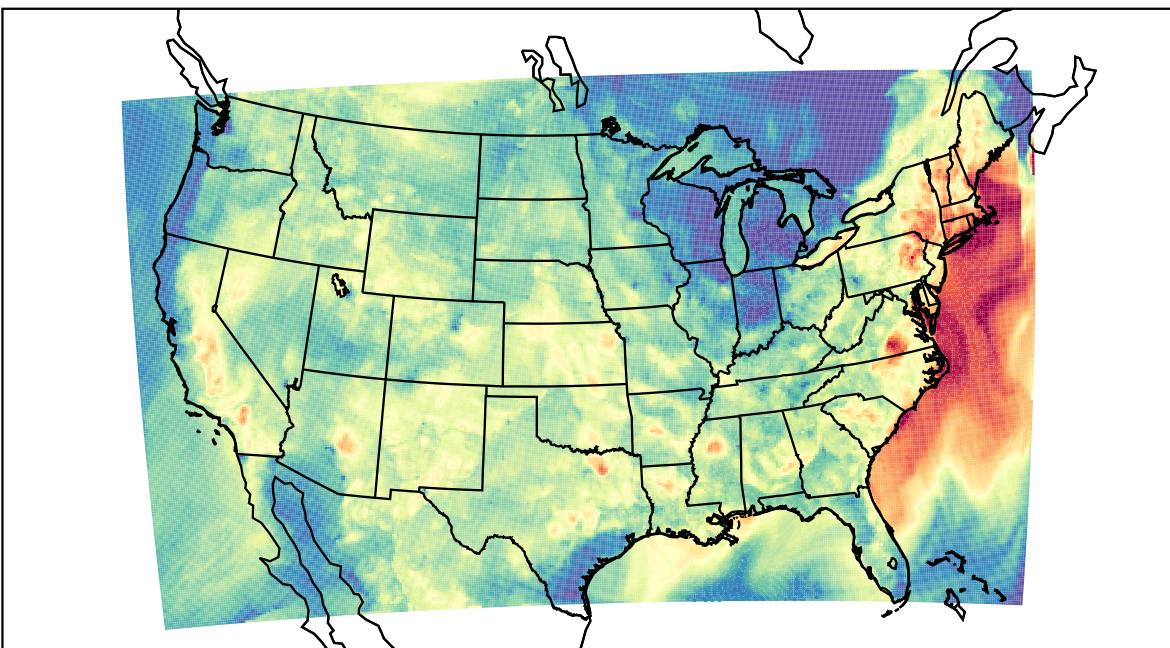
WRF (2023-09-08_02:00:00)
