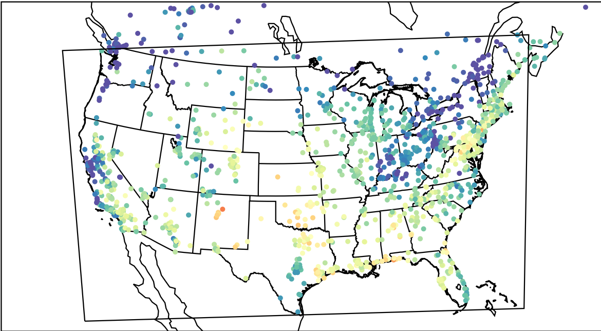
AirNOW (2023-09-09_16:00:00)
