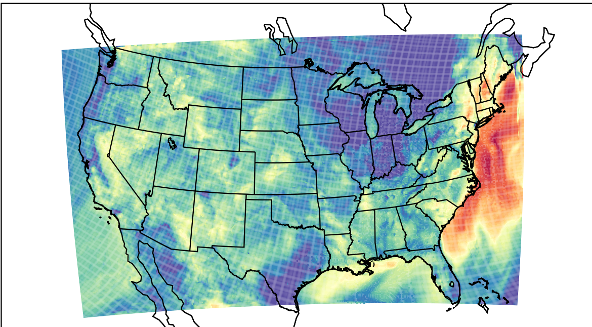
WRF (2023-09-08_09:00:00)
