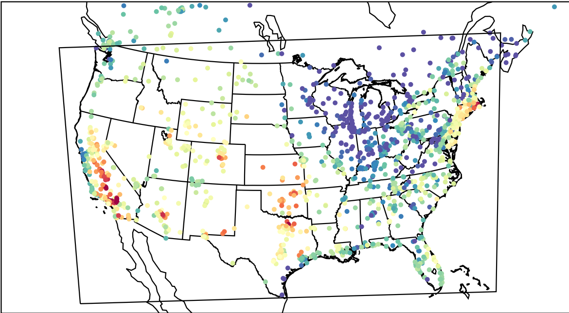
AirNOW (2023-09-08_00:00:00)
