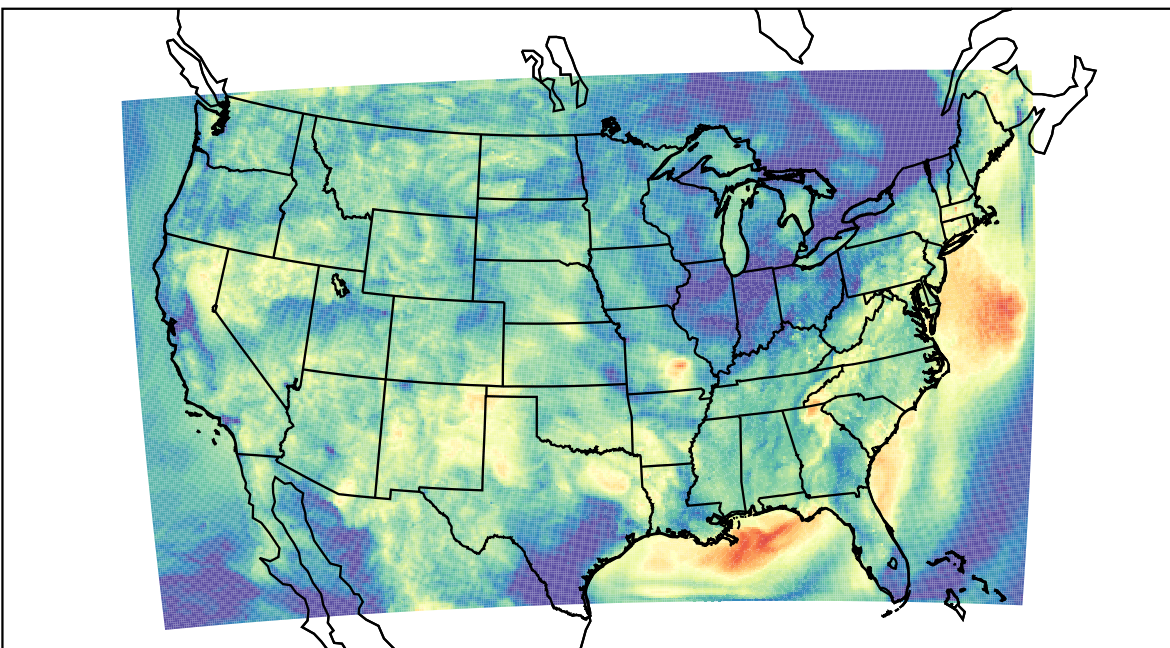
WRF (2023-09-09_08:00:00)
