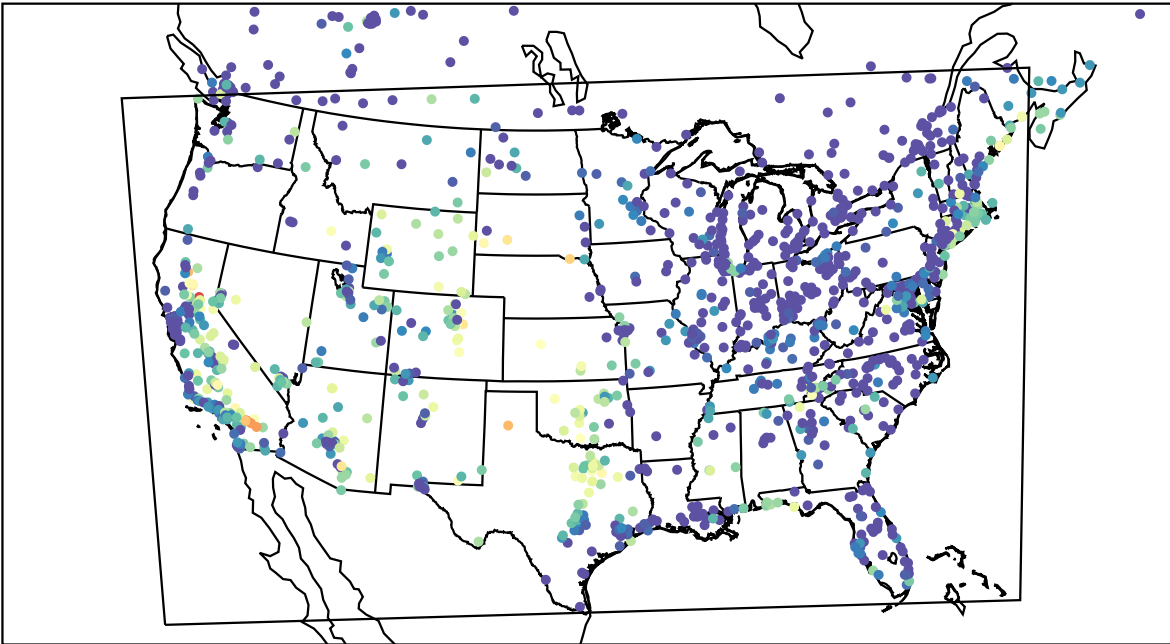
AirNOW (2023-09-09_06:00:00)
