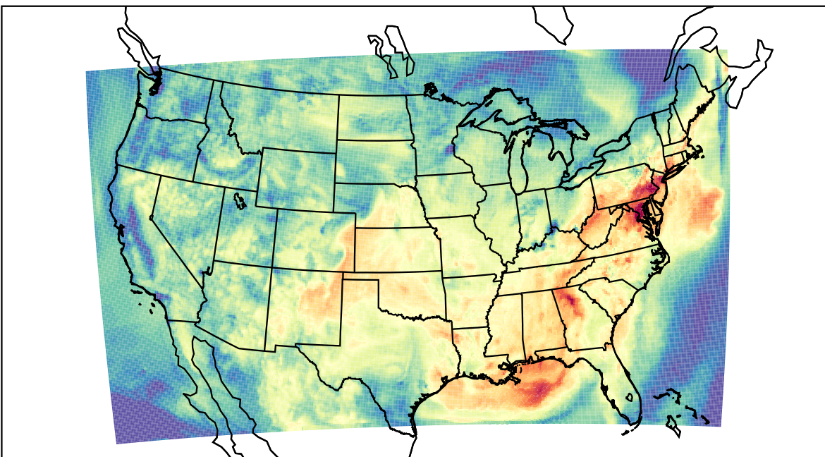
WRF (2023-09-09_16:00:00)
