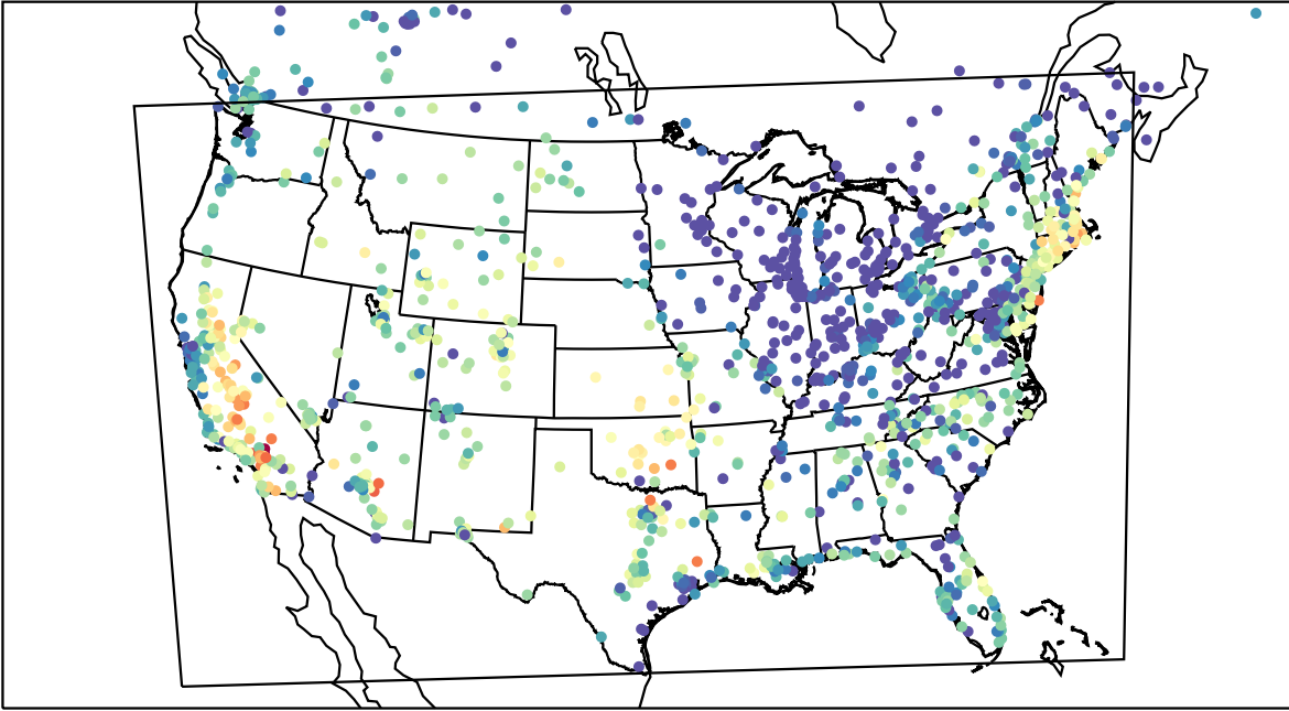
AirNOW (2023-09-08_02:00:00)
