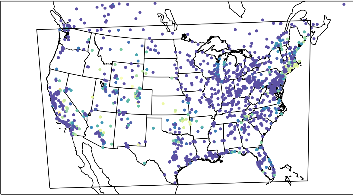
AirNOW (2023-09-08_12:00:00)
