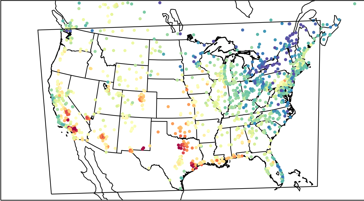
AirNOW (2023-09-09_21:00:00)
