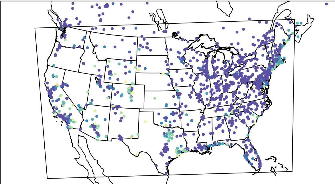
AirNOW (2023-09-09_12:00:00)
