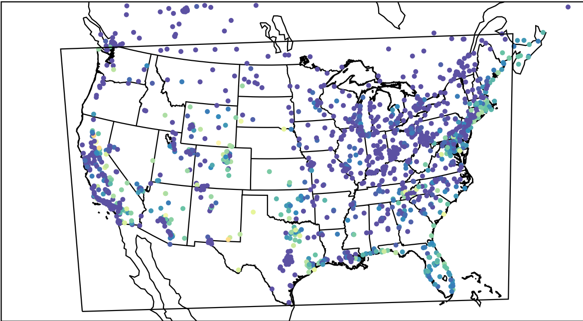
AirNOW (2023-09-09_13:00:00)
