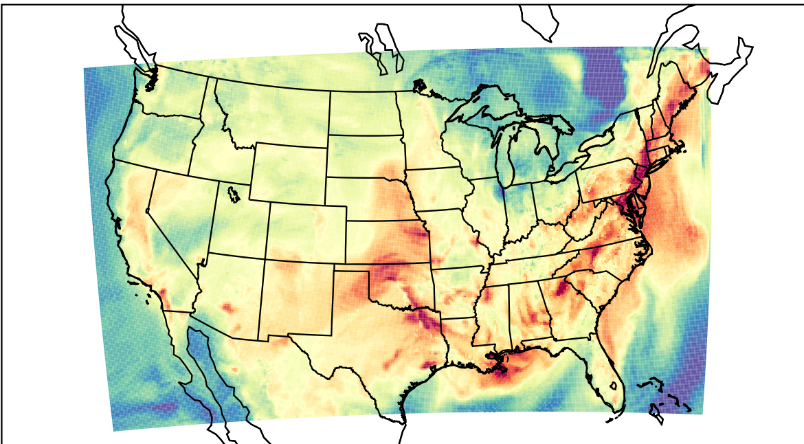
WRF (2023-09-08_22:00:00)
