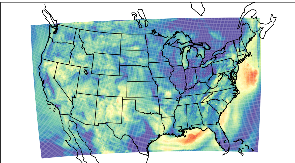
WRF (2023-09-09_12:00:00)
