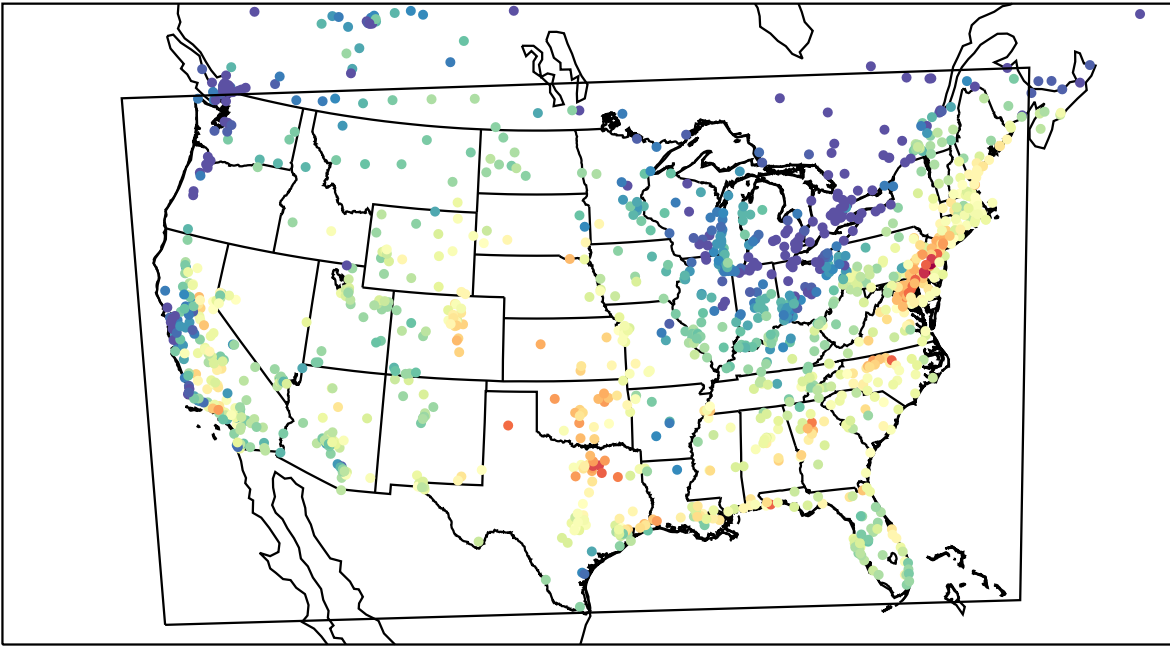
AirNOW (2023-09-08_17:00:00)
