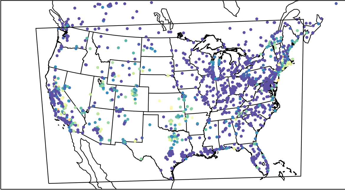
AirNOW (2023-09-08_09:00:00)
