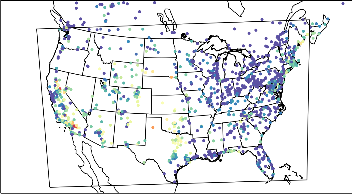
AirNOW (2023-09-09_05:00:00)
