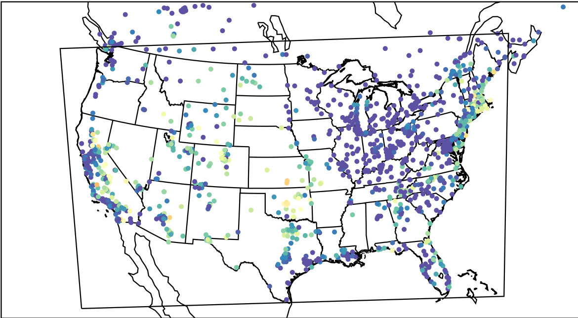
AirNOW (2023-09-08_06:00:00)
