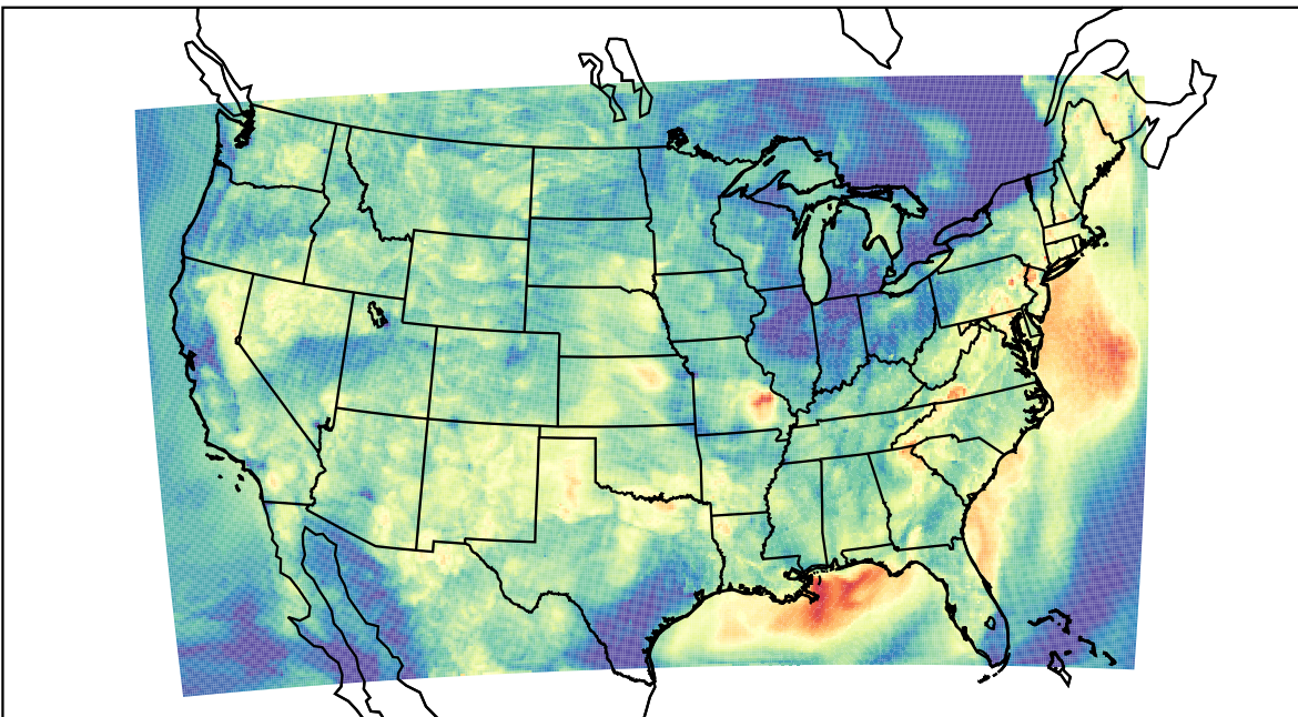
WRF (2023-09-09_05:00:00)
