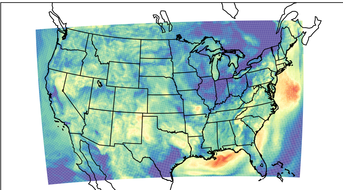
WRF (2023-09-09_09:00:00)
