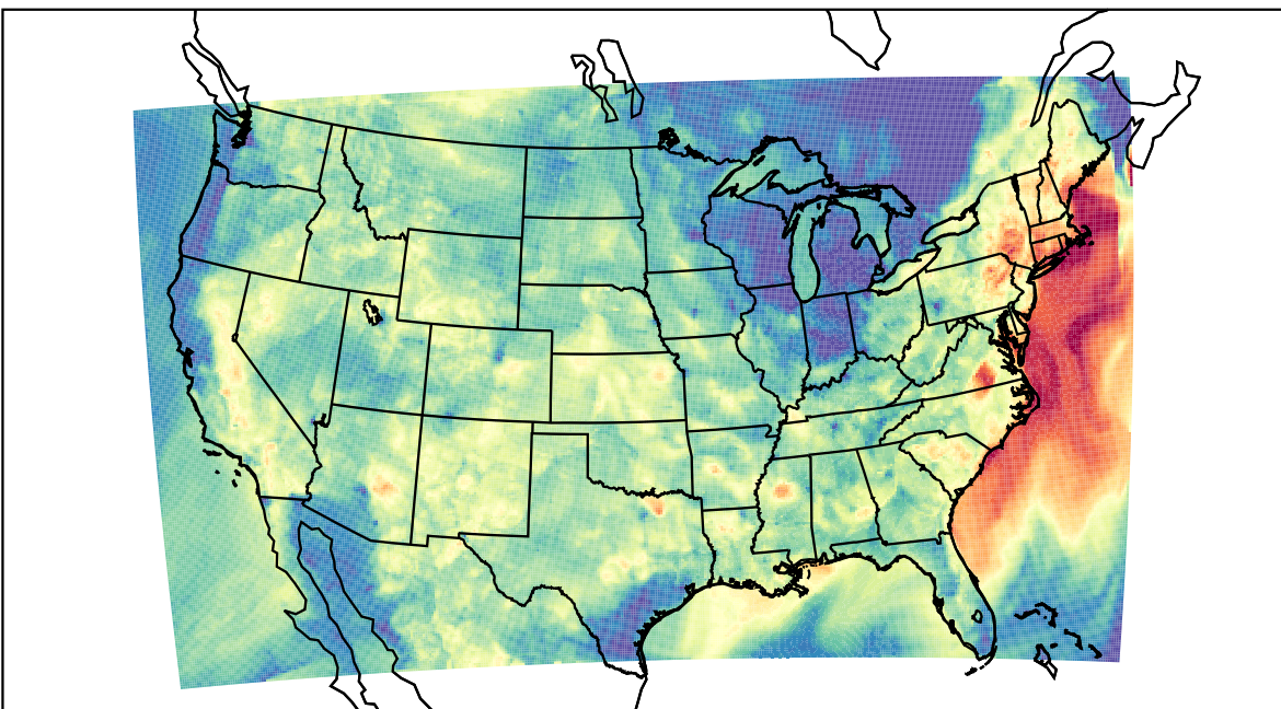
WRF (2023-09-08_03:00:00)
