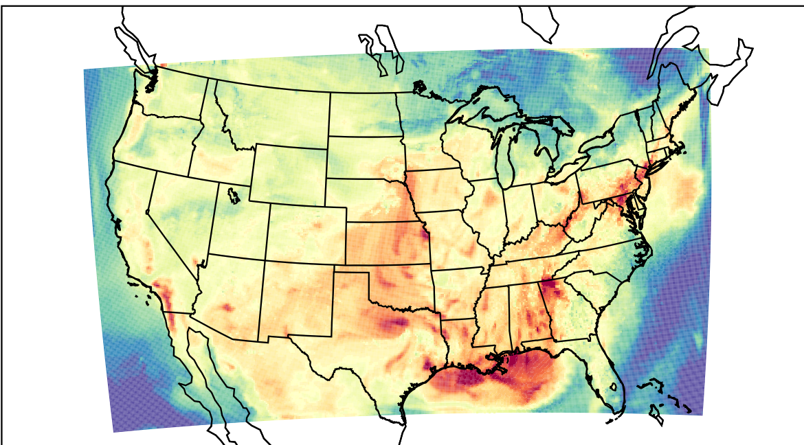
WRF (2023-09-09_22:00:00)
