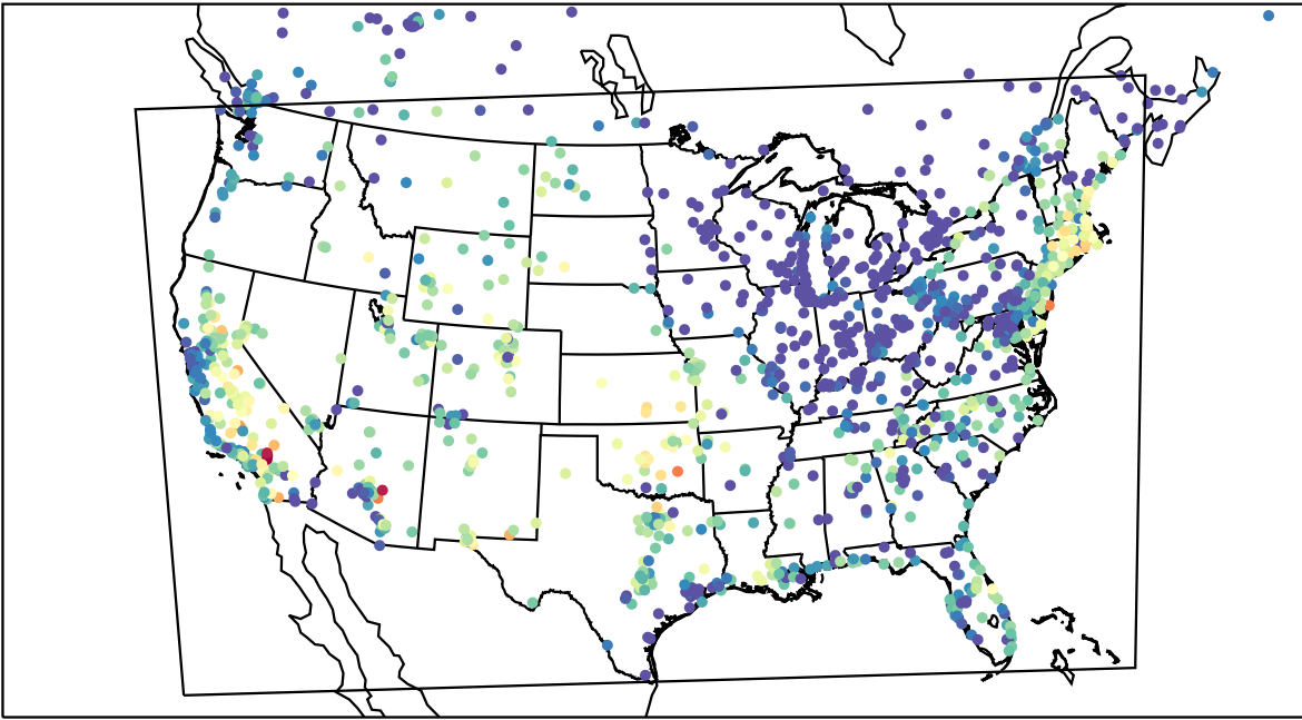
AirNOW (2023-09-08_03:00:00)
