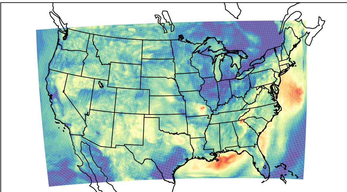
WRF (2023-09-09_07:00:00)
