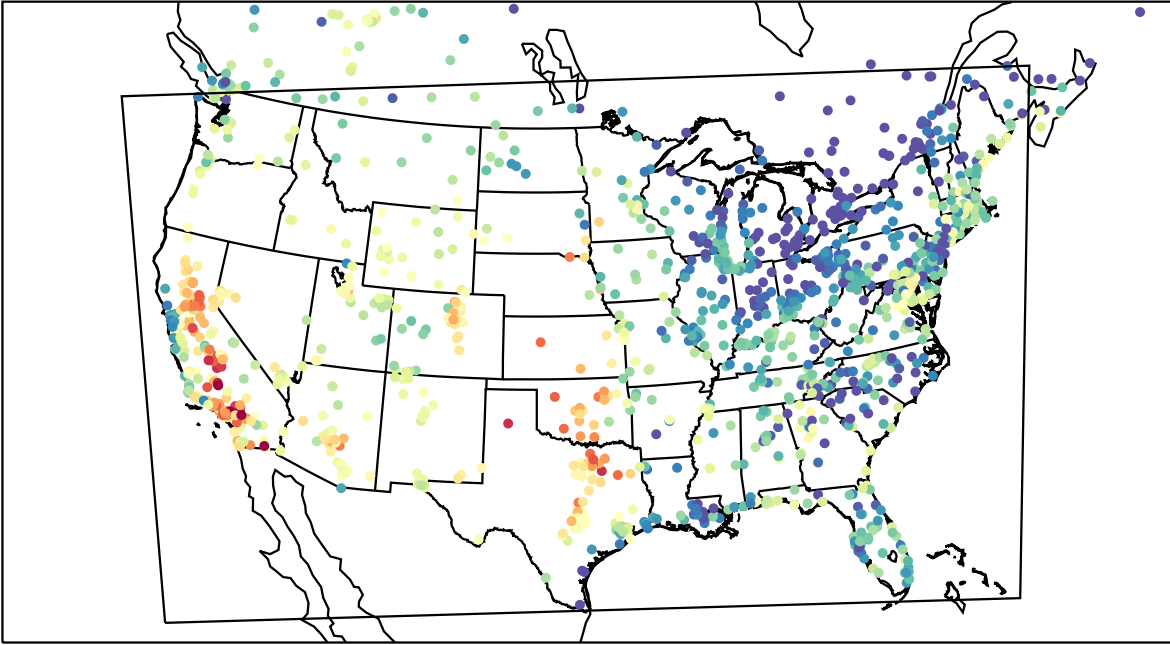
AirNOW (2023-09-09_00:00:00)
