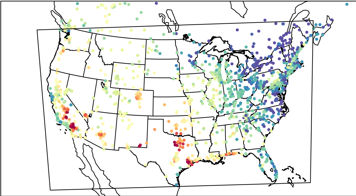
AirNOW (2023-09-09_23:00:00)
