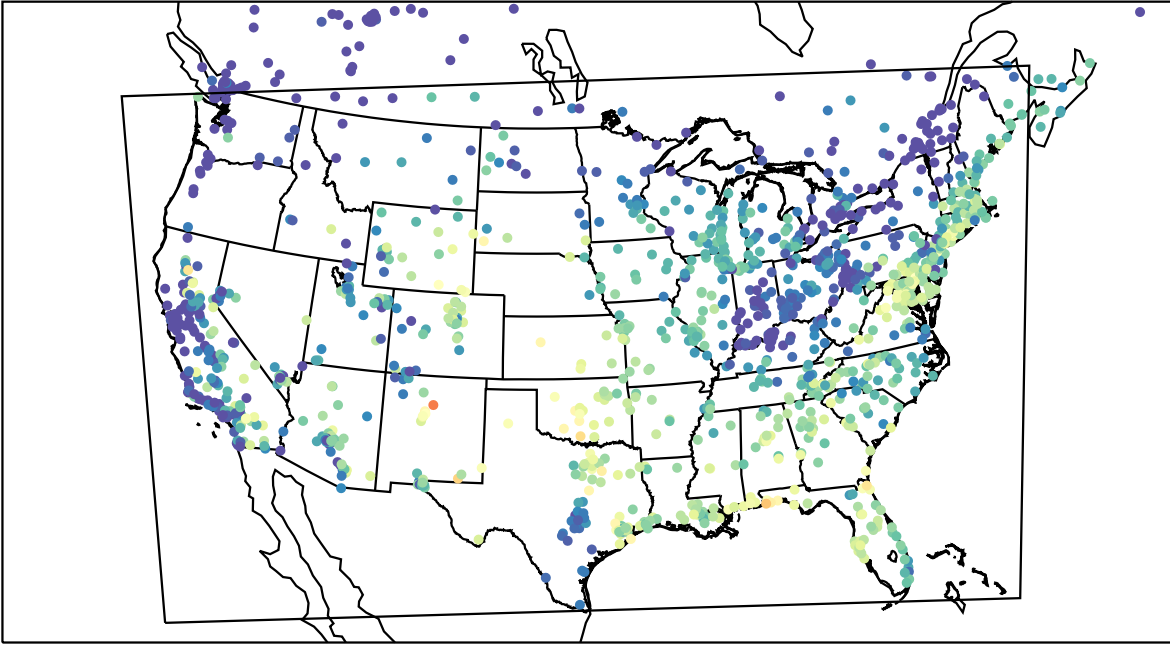
AirNOW (2023-09-09_15:00:00)
