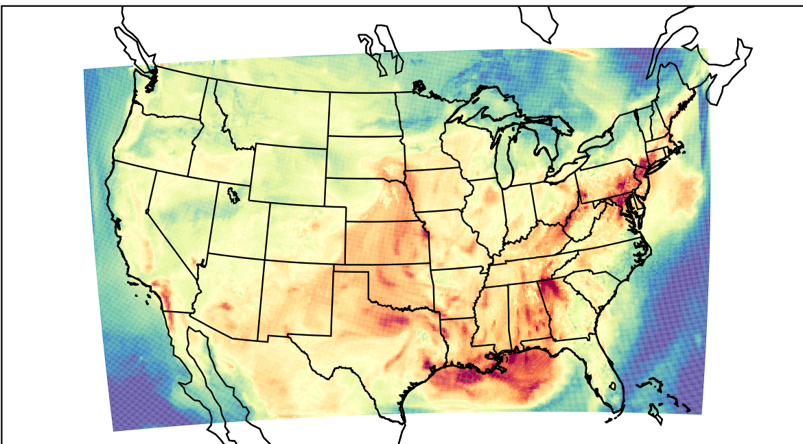
WRF (2023-09-09_21:00:00)
