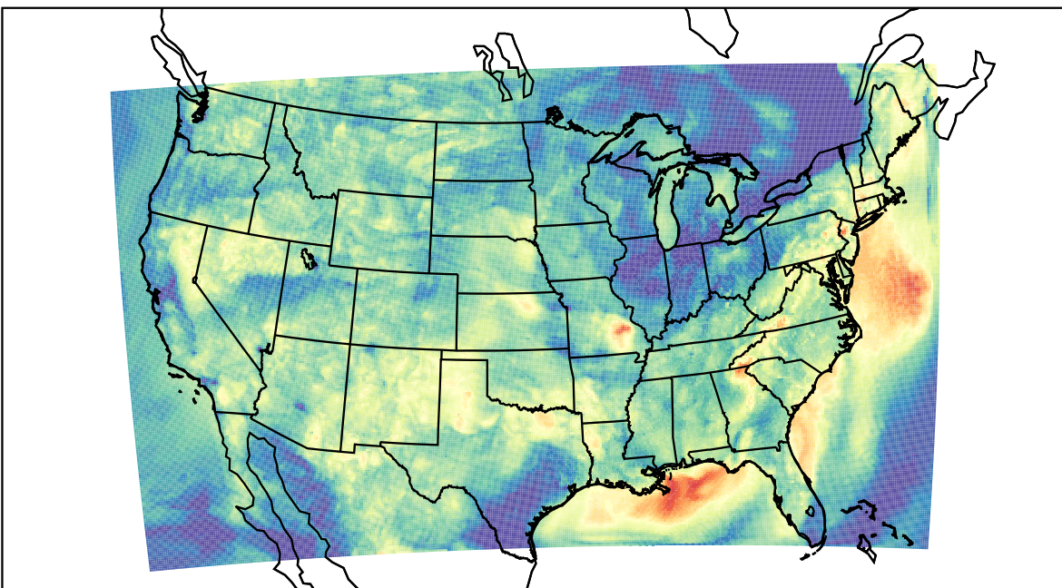
WRF (2023-09-09_06:00:00)
