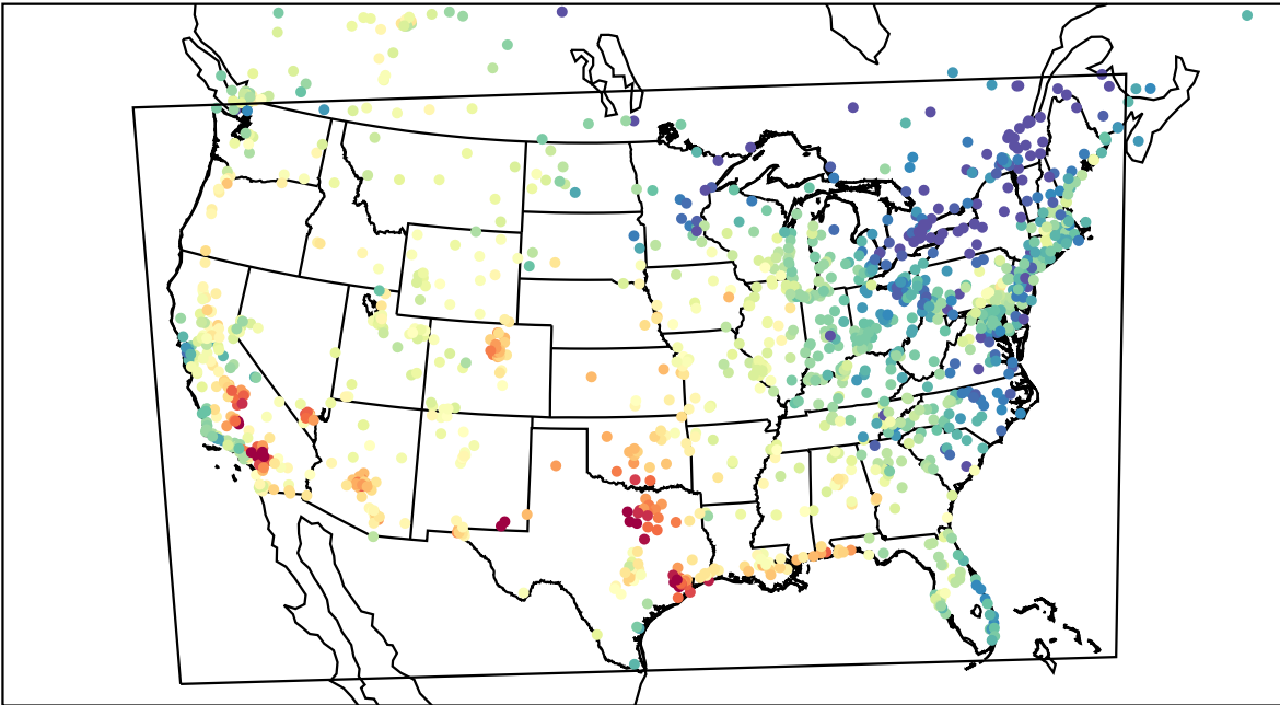
AirNOW (2023-09-09_22:00:00)
