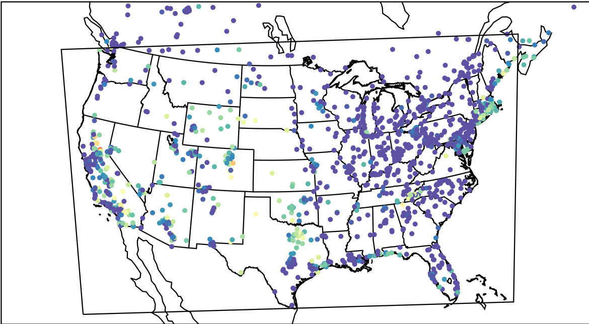
AirNOW (2023-09-09_09:00:00)
