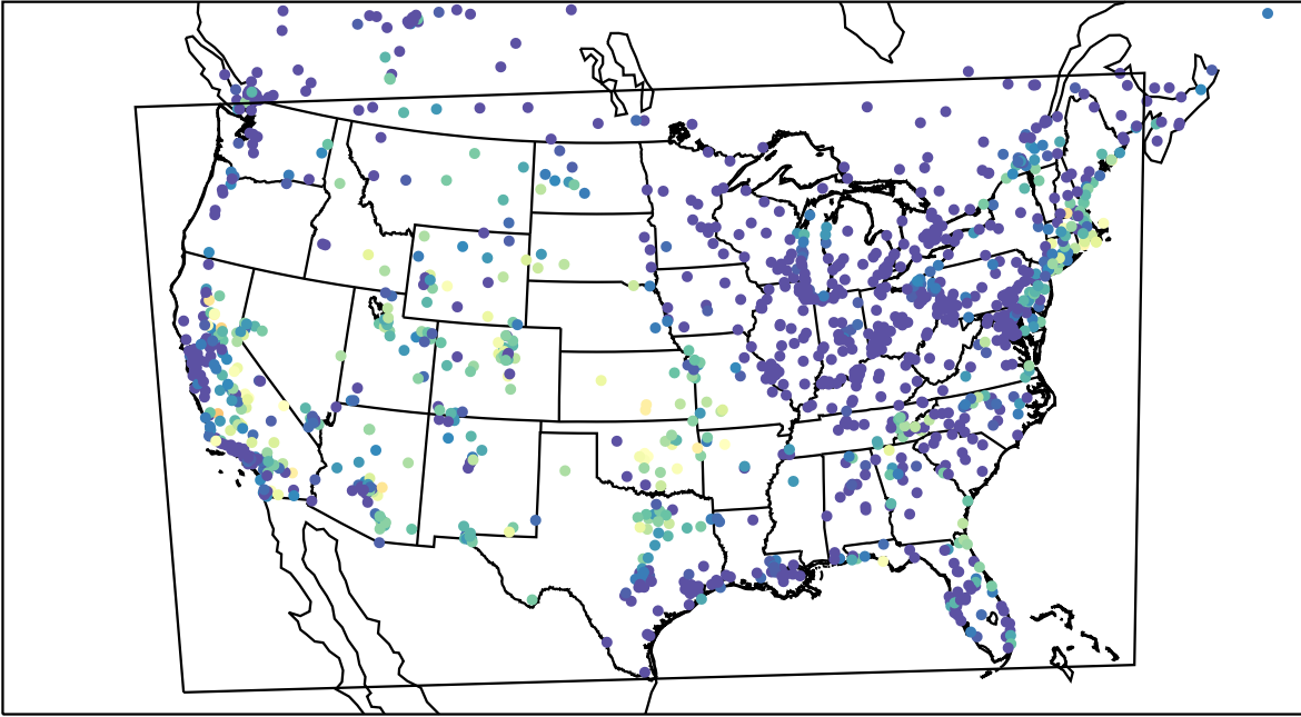
AirNOW (2023-09-08_07:00:00)
