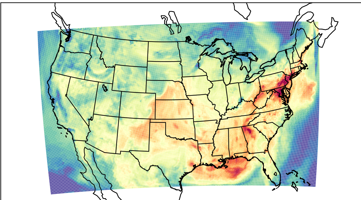
WRF (2023-09-09_17:00:00)
