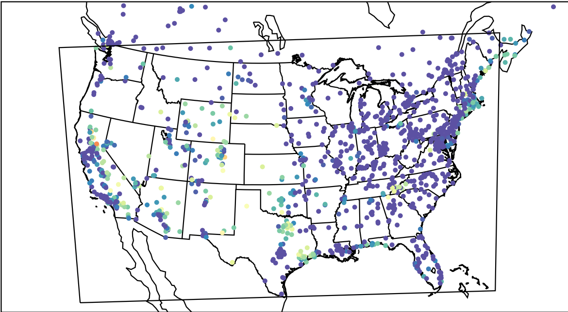
AirNOW (2023-09-09_10:00:00)
