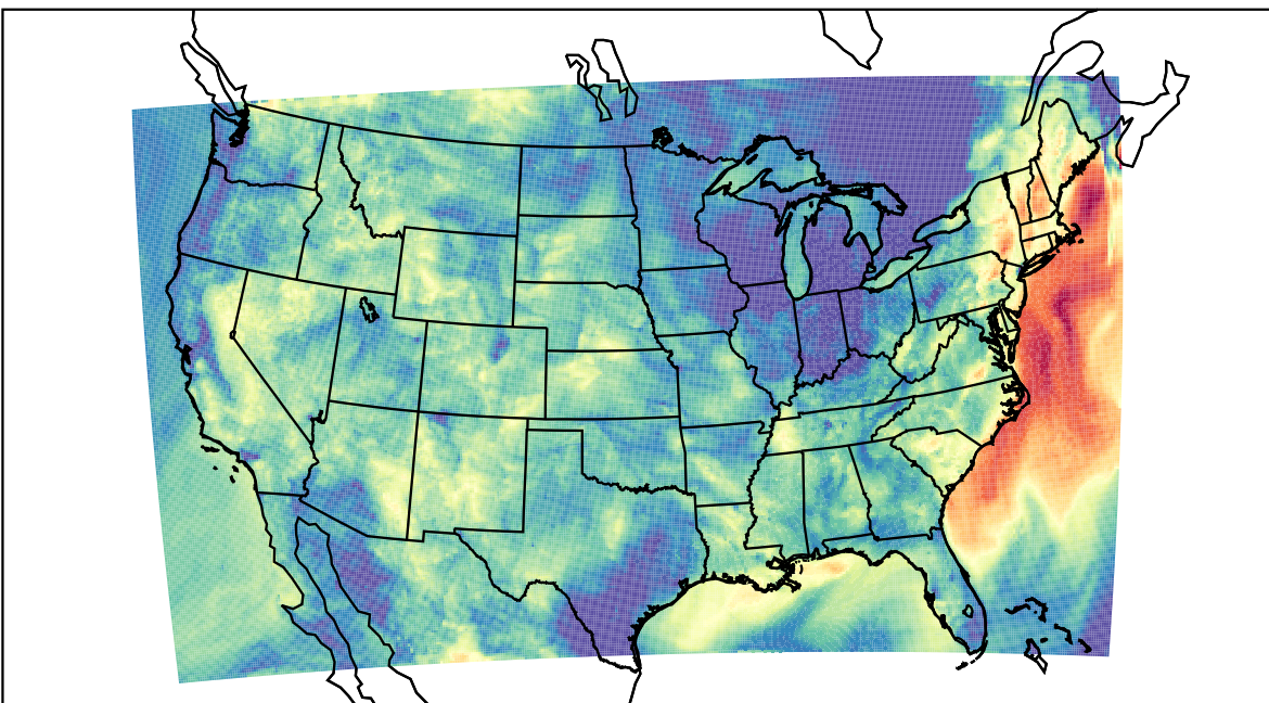
WRF (2023-09-08_08:00:00)
