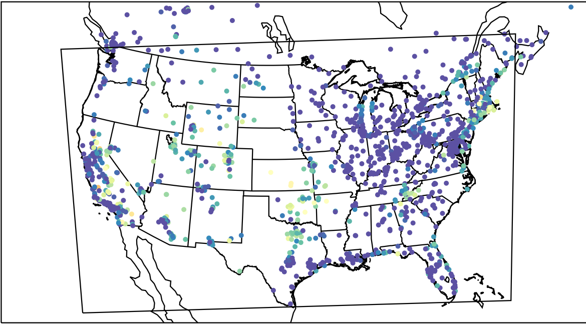
AirNOW (2023-09-08_08:00:00)
