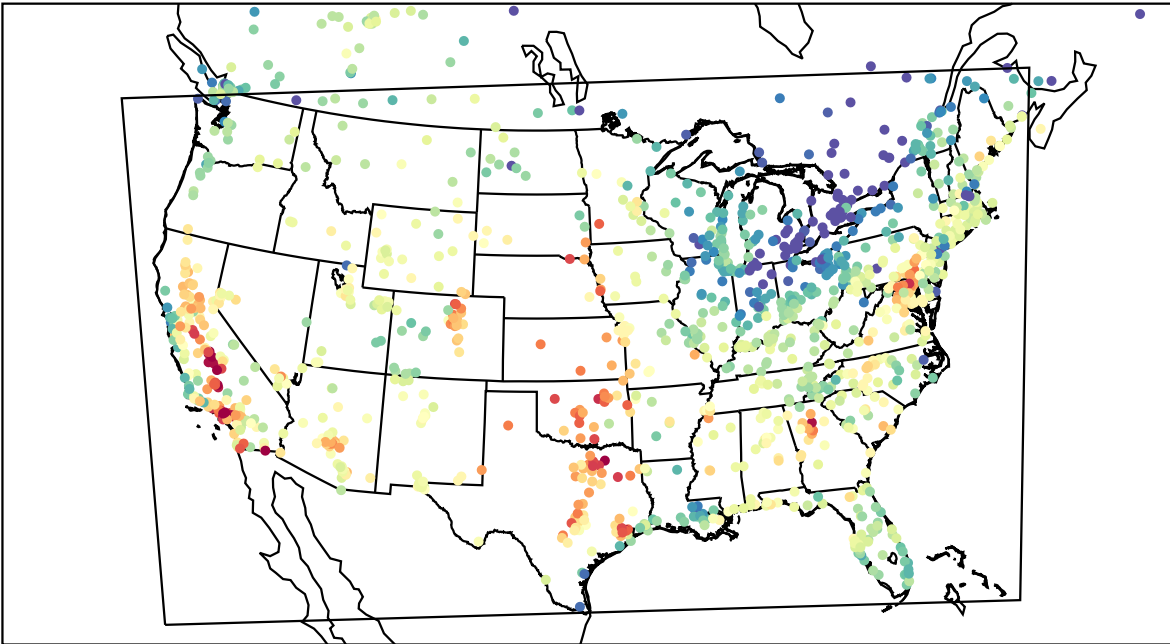
AirNOW (2023-09-08_21:00:00)
