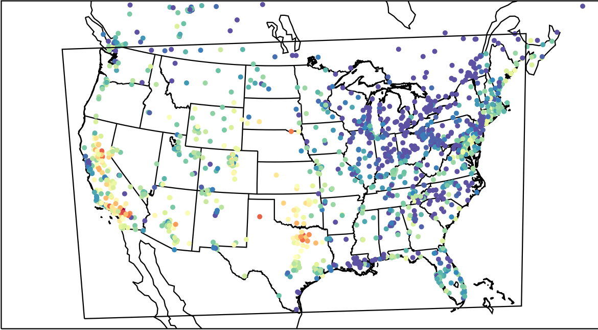
AirNOW (2023-09-09_02:00:00)
