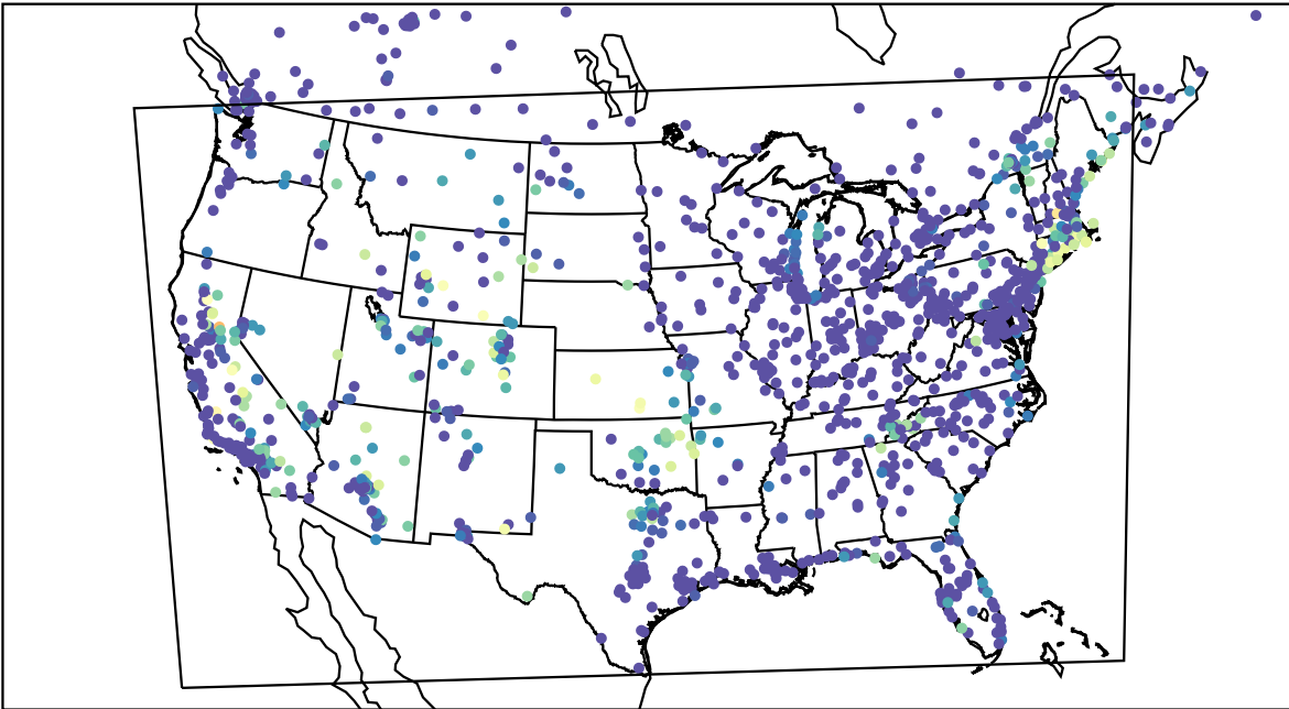
AirNOW (2023-09-08_11:00:00)
