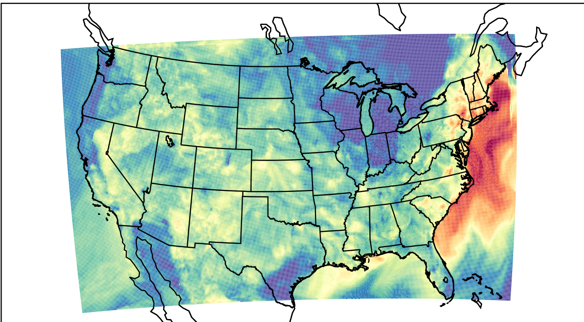
WRF (2023-09-08_05:00:00)
