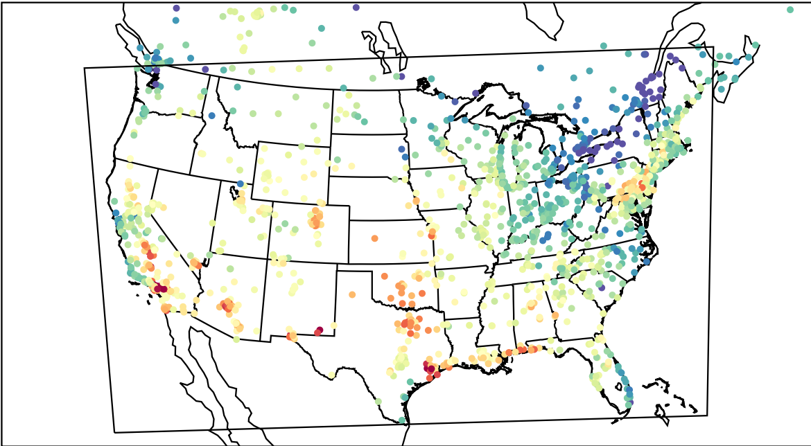
AirNOW (2023-09-09_19:00:00)
