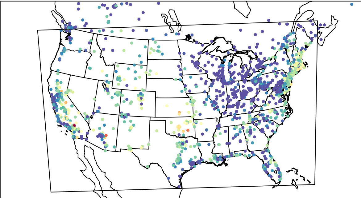
AirNOW (2023-09-08_04:00:00)
