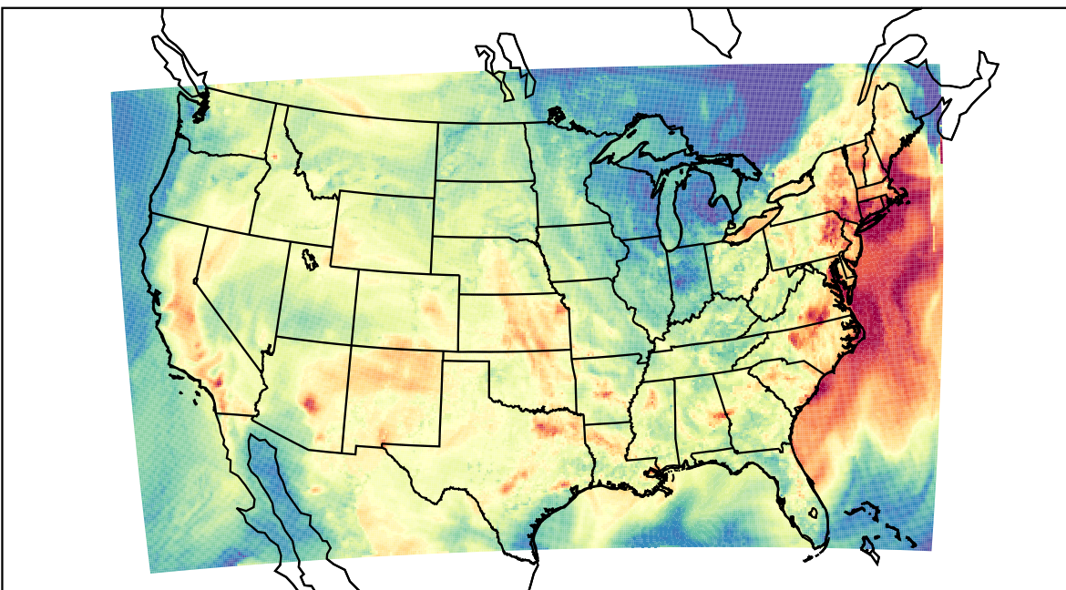
WRF (2023-09-08_00:00:00)
