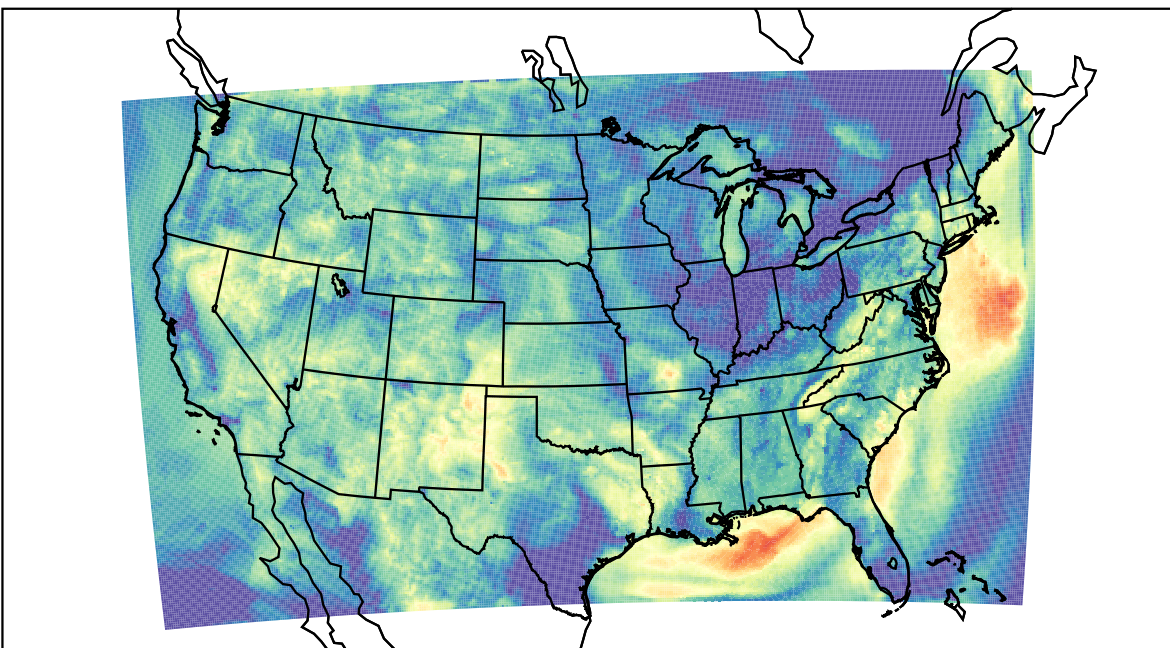
WRF (2023-09-09_11:00:00)
