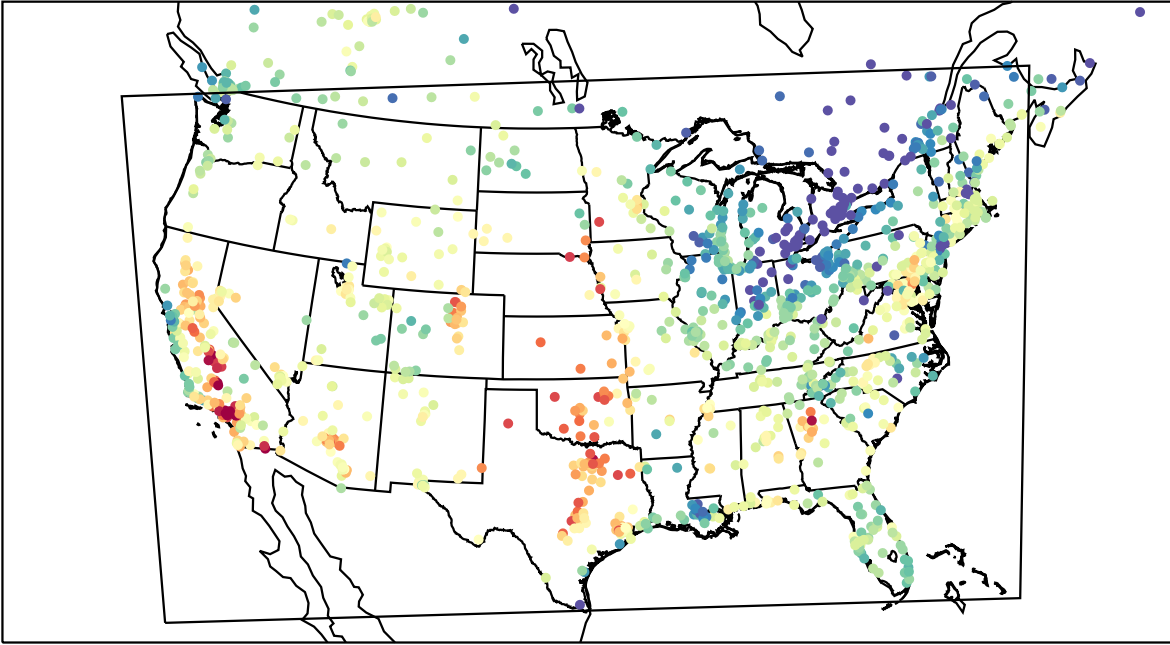
AirNOW (2023-09-08_22:00:00)
