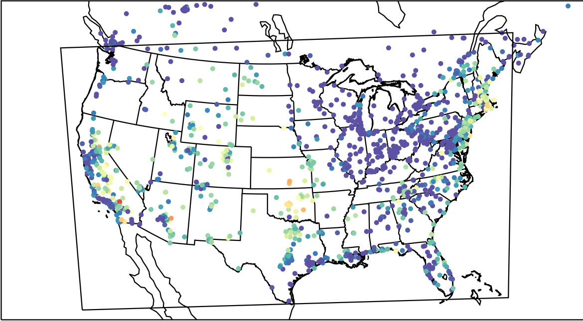
AirNOW (2023-09-08_05:00:00)
