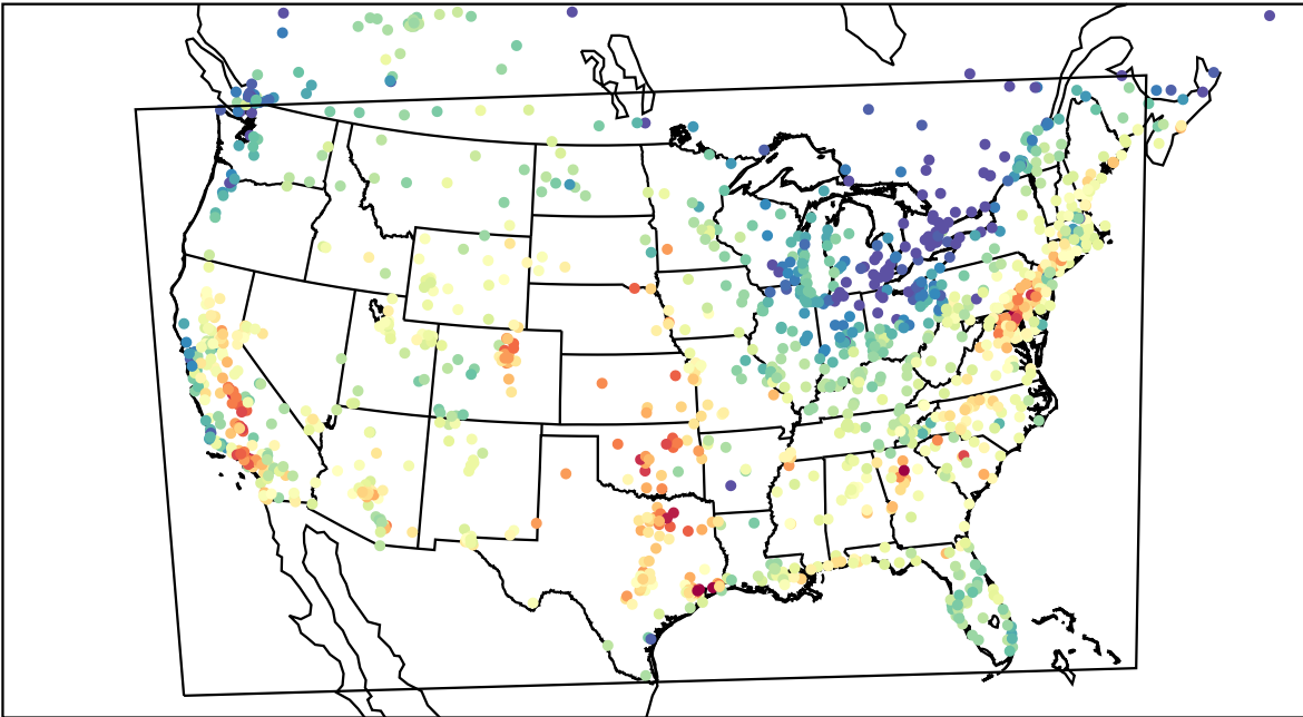
AirNOW (2023-09-08_19:00:00)
