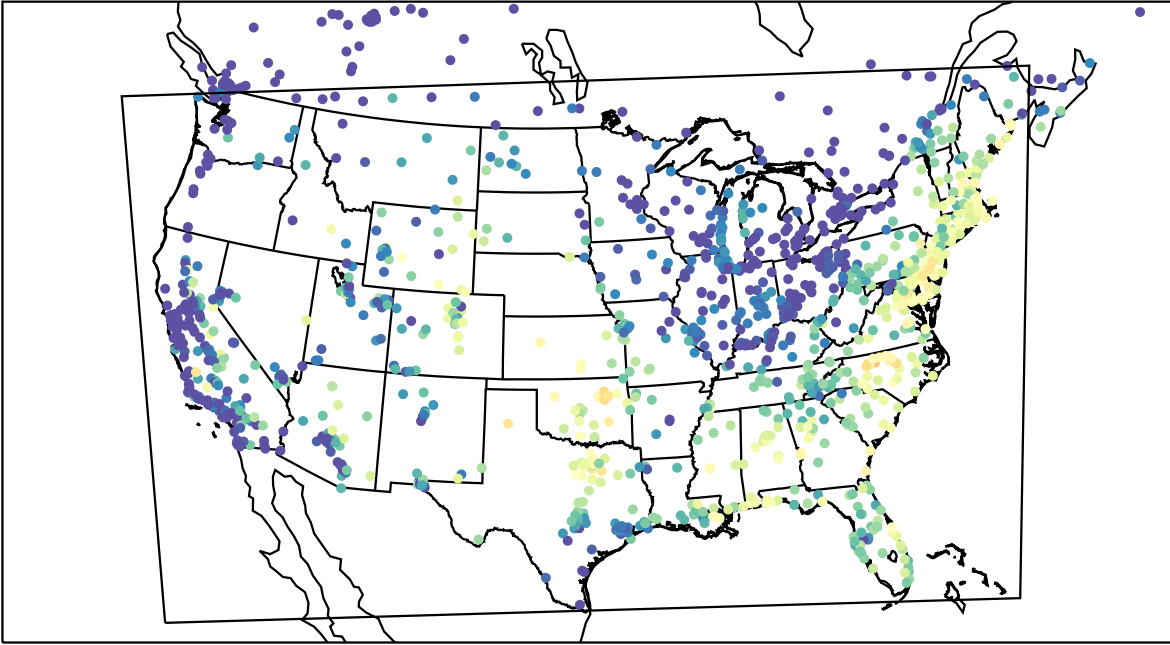
AirNOW (2023-09-08_15:00:00)
