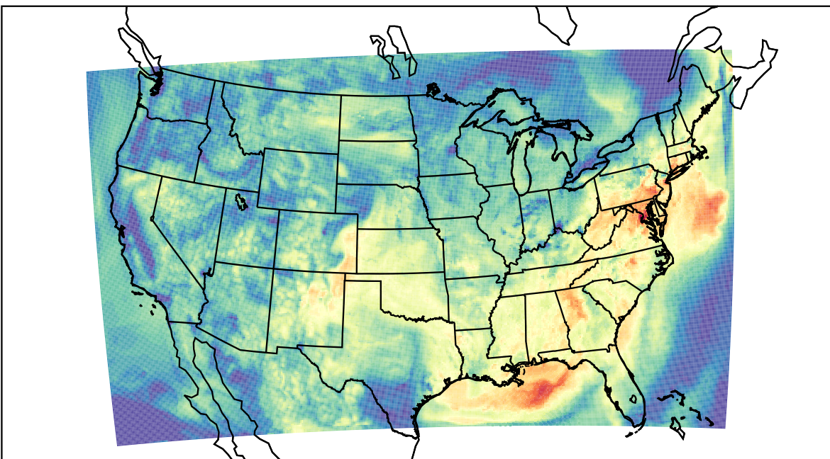
WRF (2023-09-09_15:00:00)
