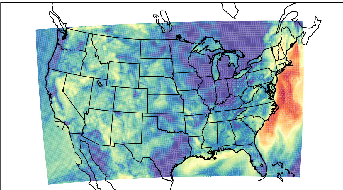
WRF (2023-09-08_12:00:00)
