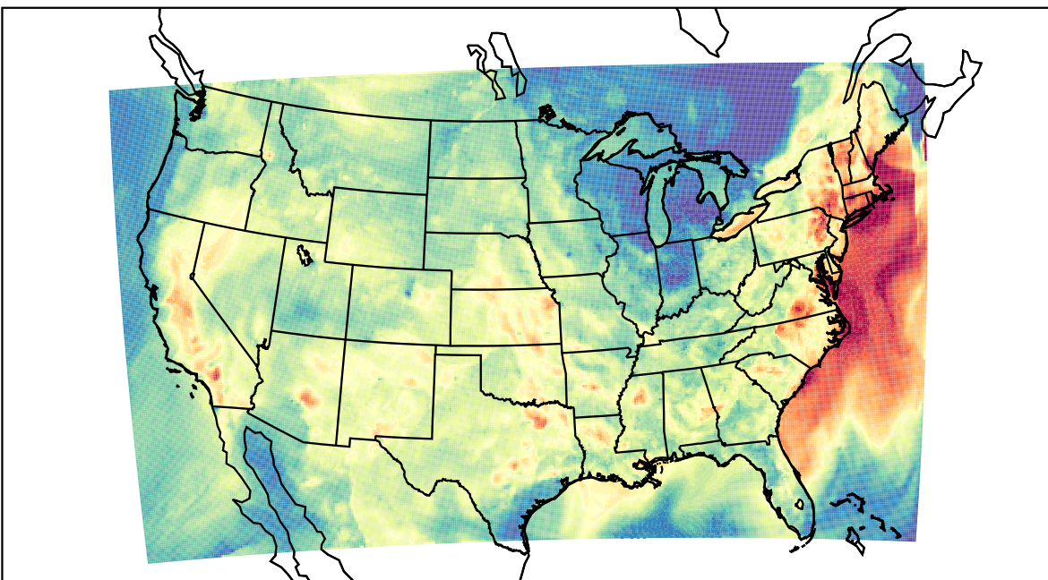
WRF (2023-09-08_01:00:00)
