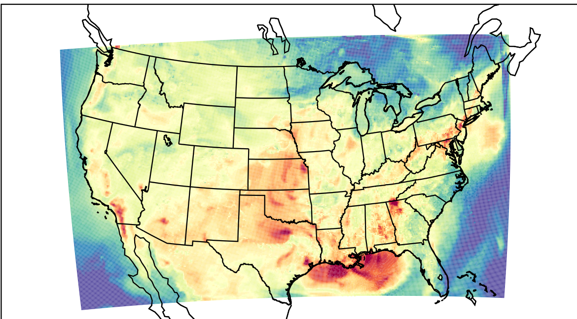
WRF (2023-09-09_23:00:00)
