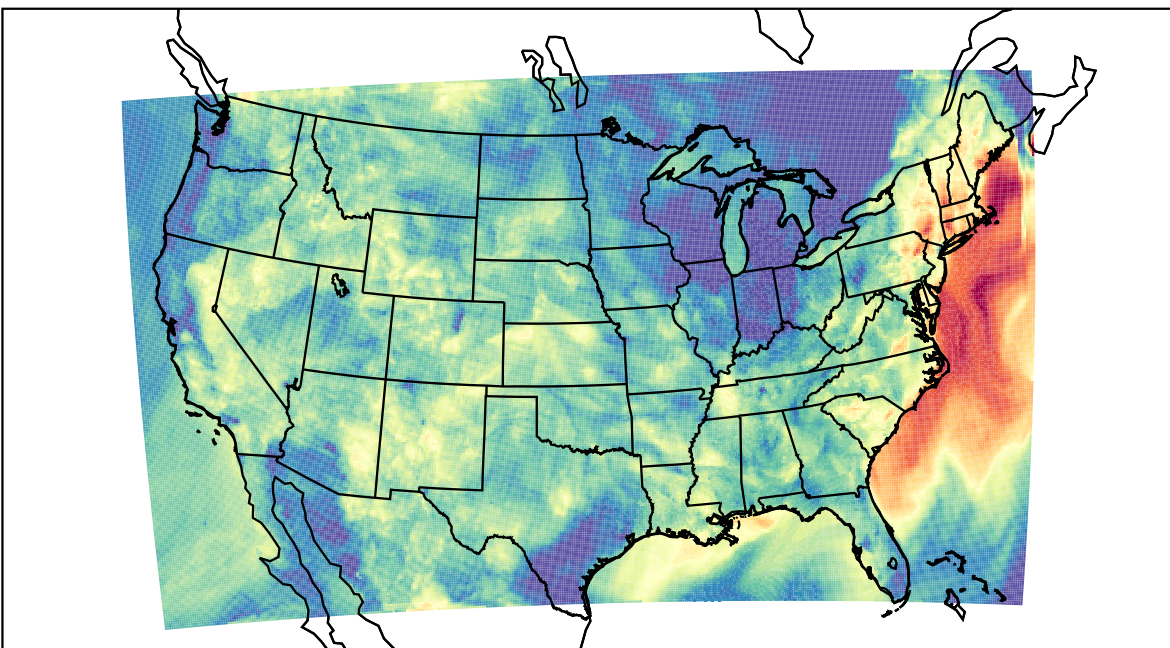
WRF (2023-09-08_06:00:00)
