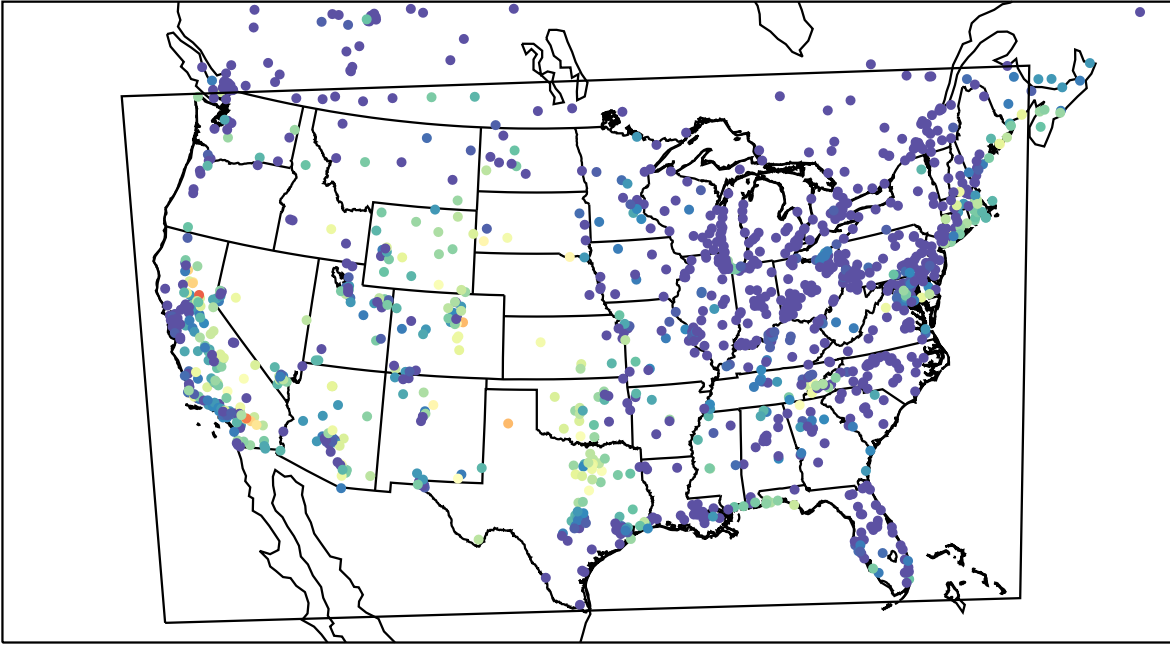
AirNOW (2023-09-09_07:00:00)
