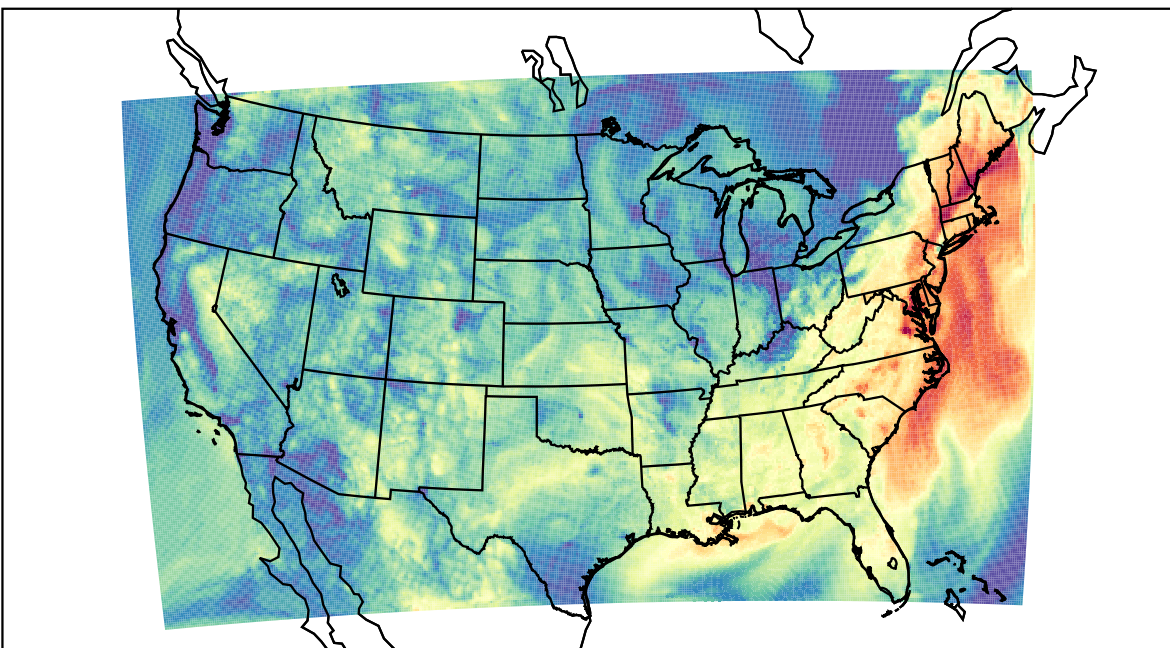
WRF (2023-09-08_15:00:00)
