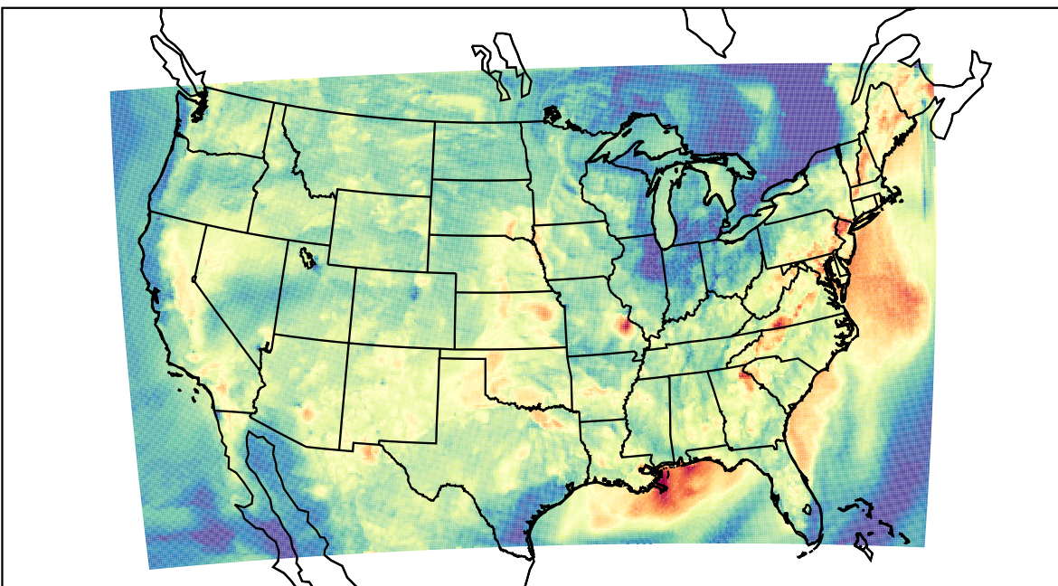
WRF (2023-09-09_02:00:00)
