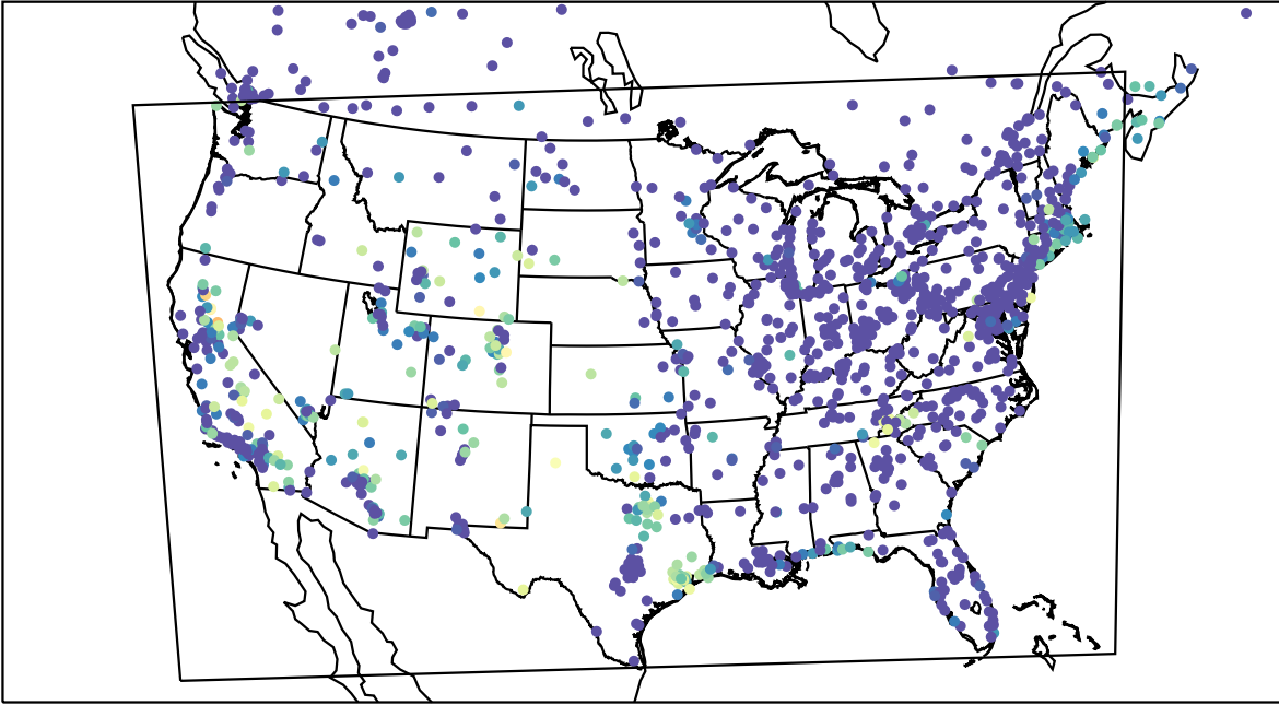
AirNOW (2023-09-09_11:00:00)
