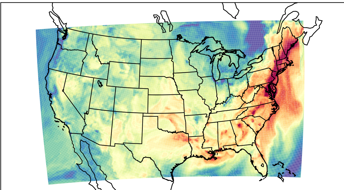
WRF (2023-09-08_17:00:00)
