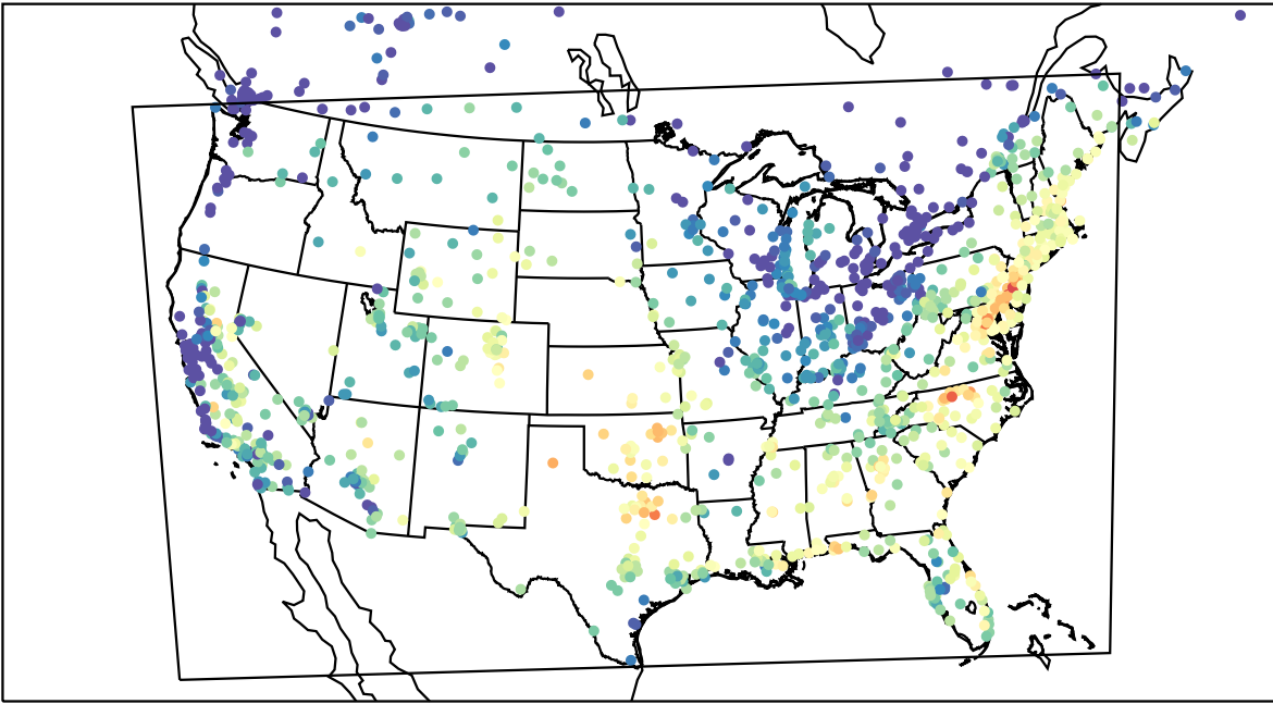
AirNOW (2023-09-08_16:00:00)
