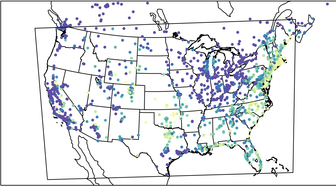
AirNOW (2023-09-08_14:00:00)
