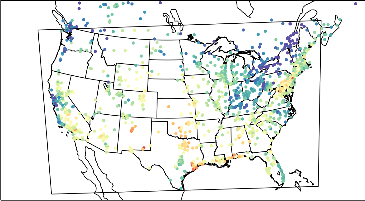
AirNOW (2023-09-09_17:00:00)
