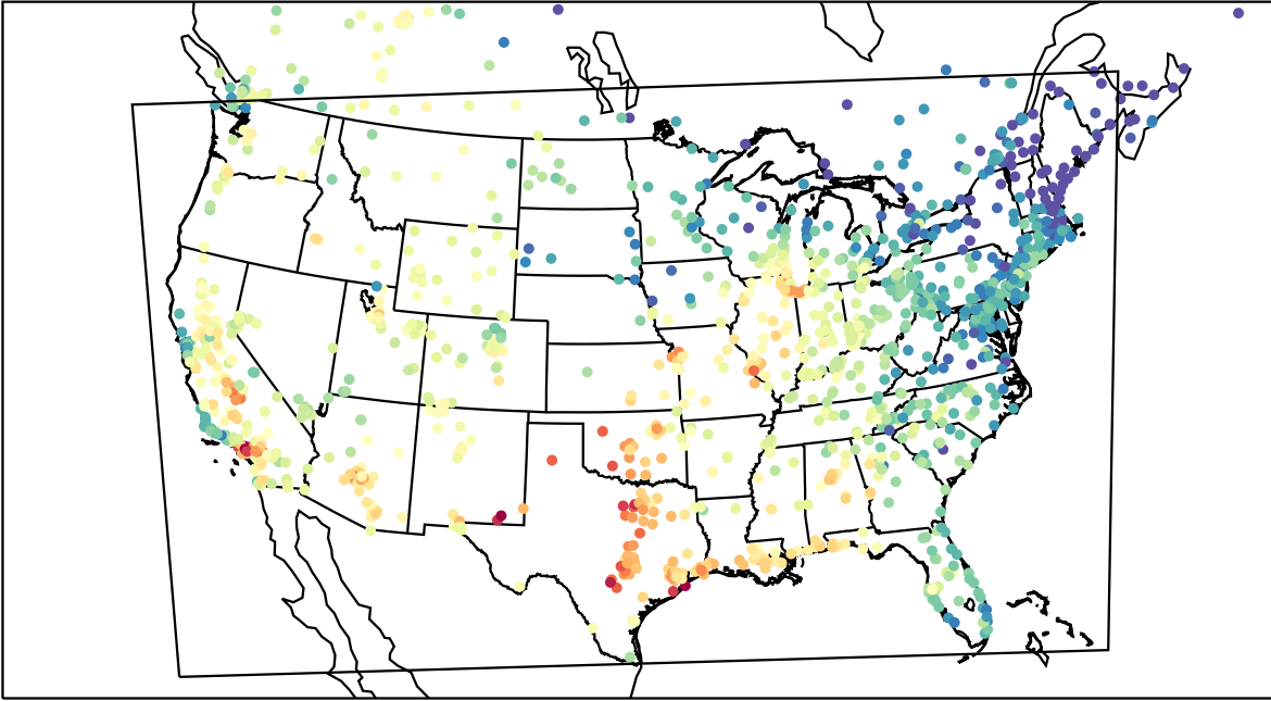
AirNOW (2023-09-10_21:00:00)
