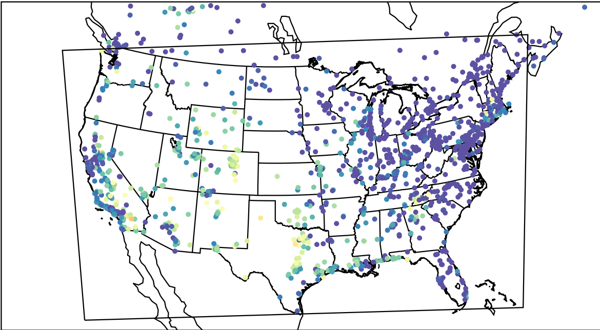
AirNOW (2023-09-10_07:00:00)
