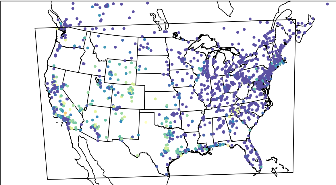
AirNOW (2023-09-10_11:00:00)
