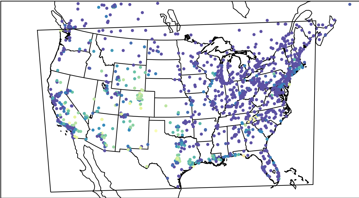
AirNOW (2023-09-10_12:00:00)
