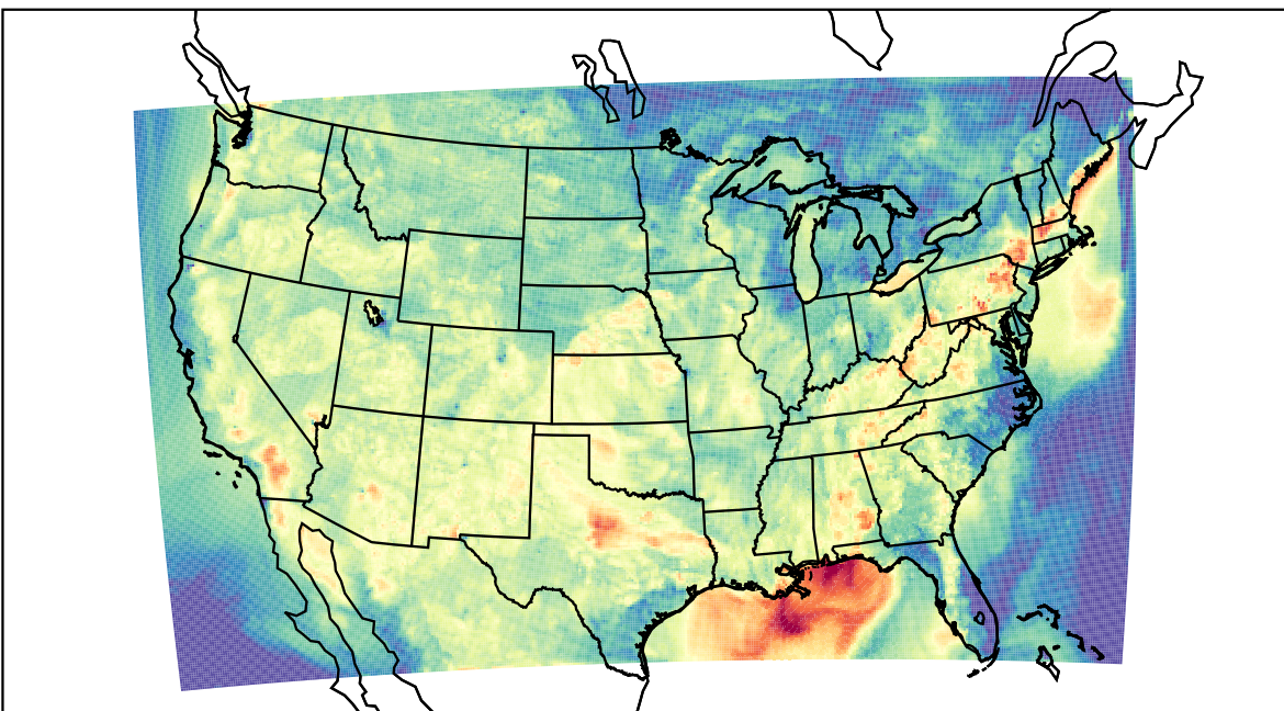
WRF (2023-09-10_02:00:00)
