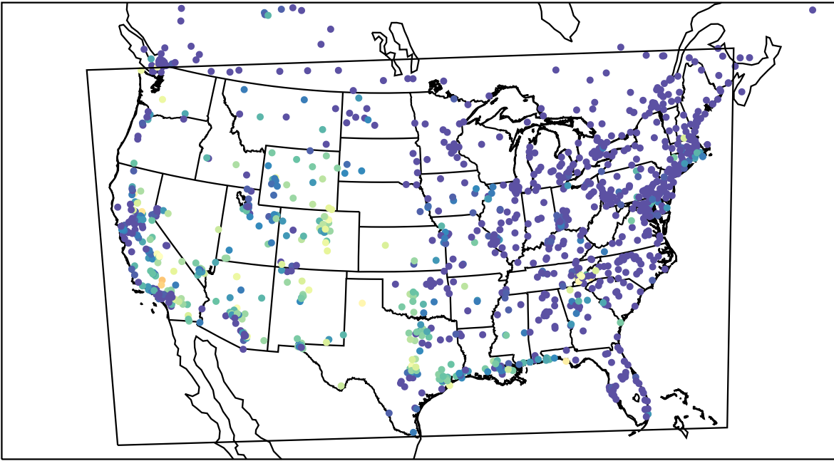
AirNOW (2023-09-10_10:00:00)
