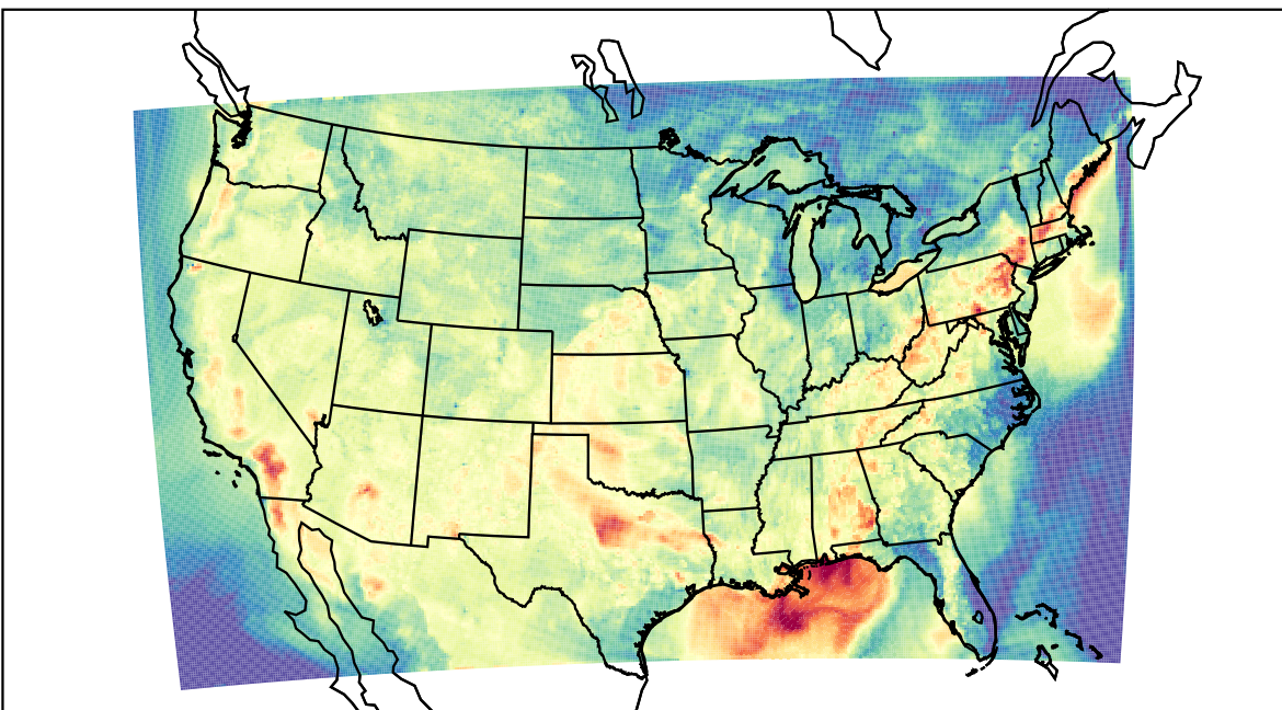
WRF (2023-09-10_01:00:00)
