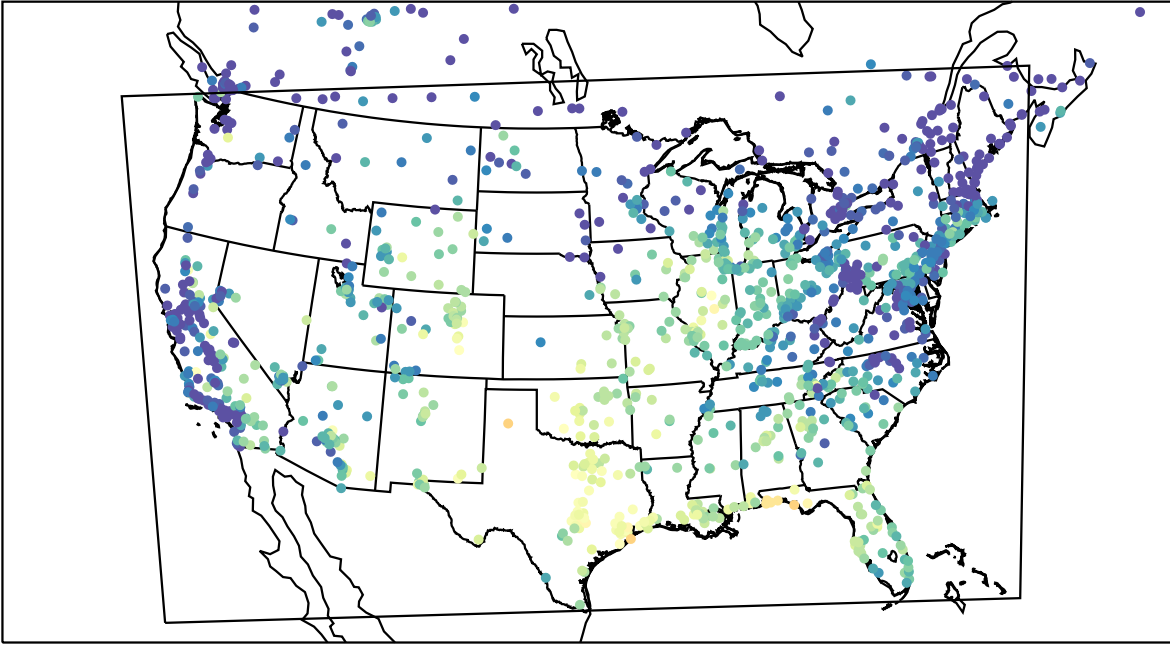
AirNOW (2023-09-10_15:00:00)
