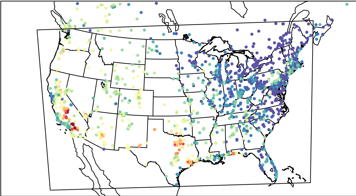
AirNOW (2023-09-10_01:00:00)
