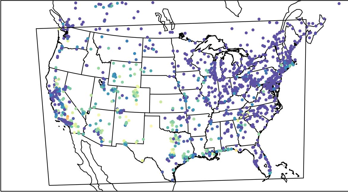
AirNOW (2023-09-10_09:00:00)
