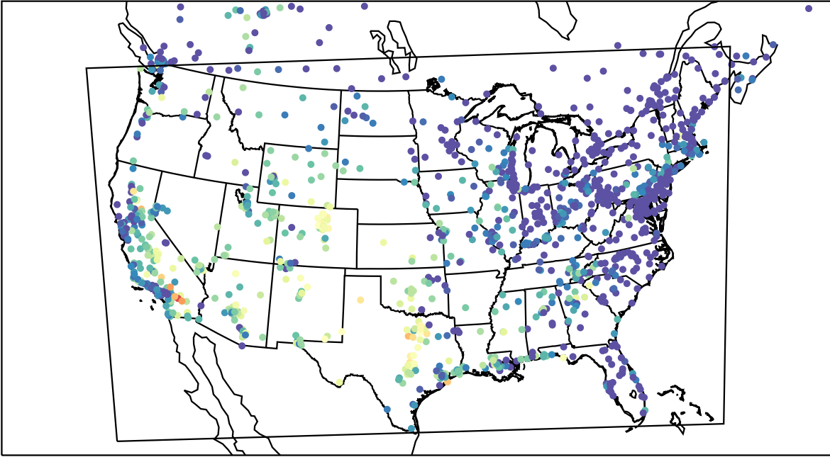
AirNOW (2023-09-10_05:00:00)
