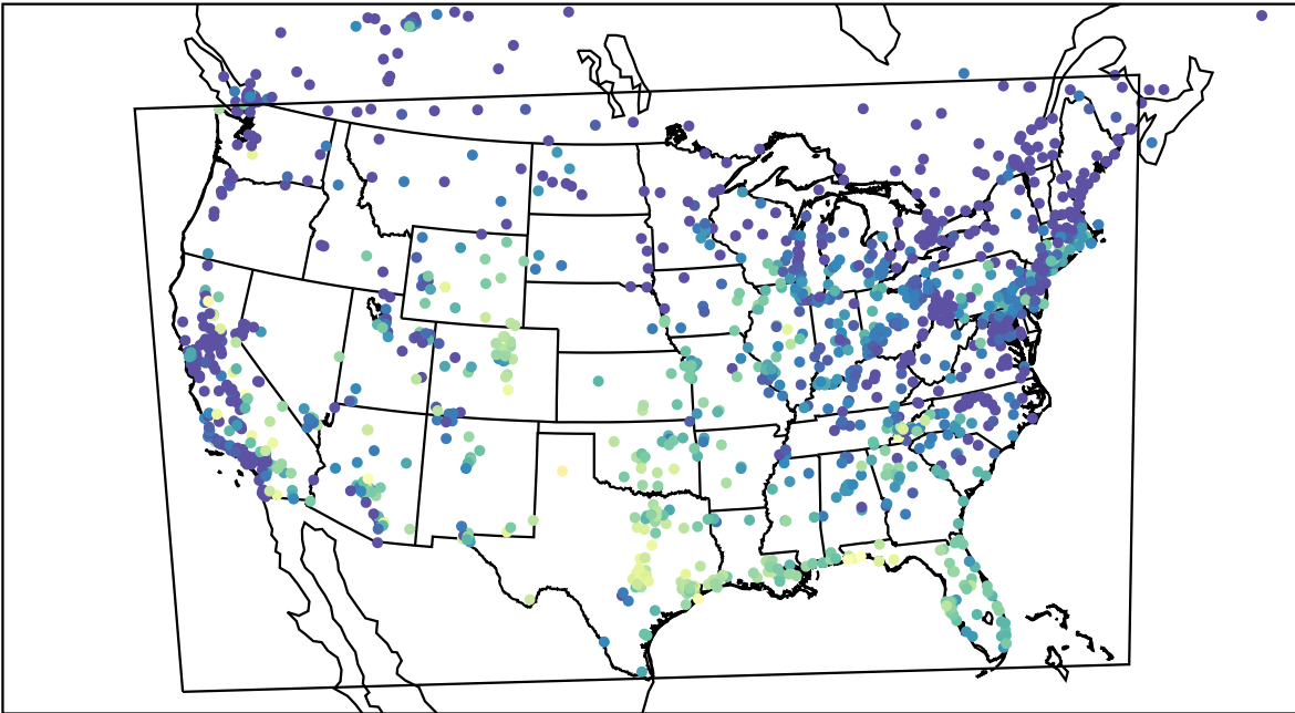
AirNOW (2023-09-10_14:00:00)
