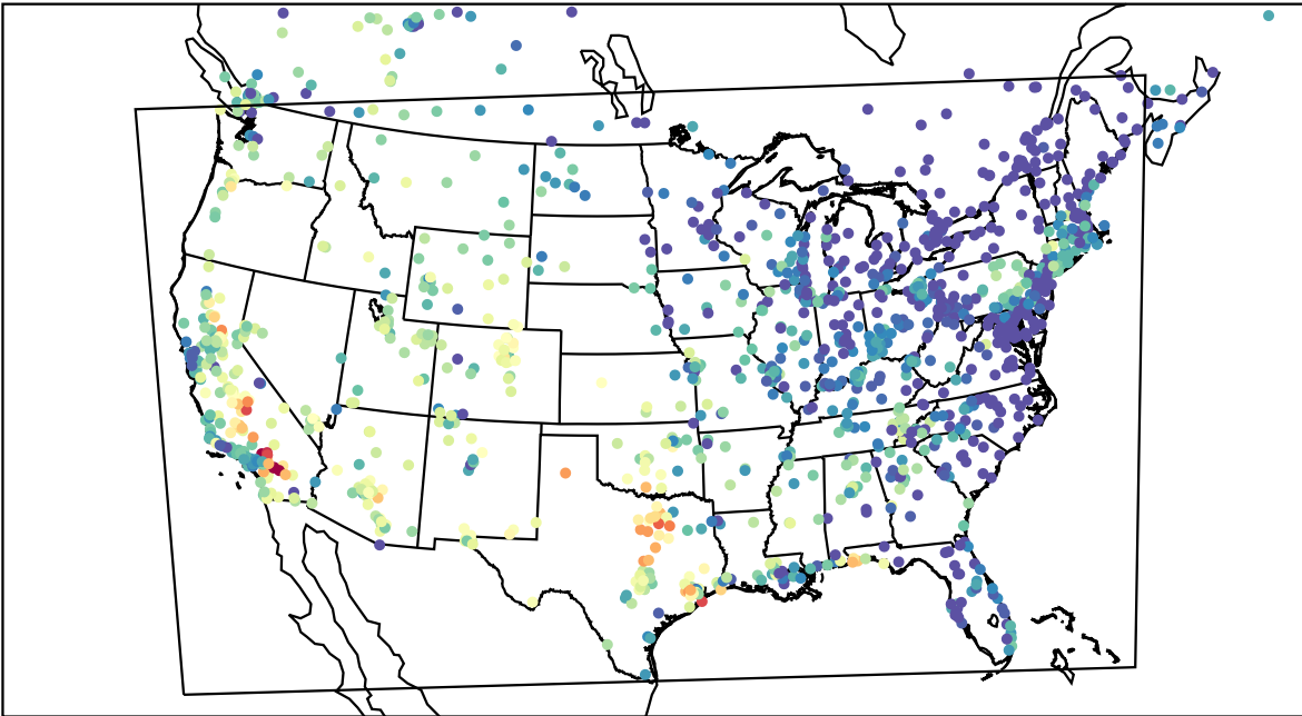
AirNOW (2023-09-10_02:00:00)
