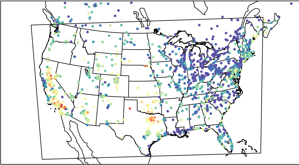
AirNOW (2023-09-09_02:00:00)
