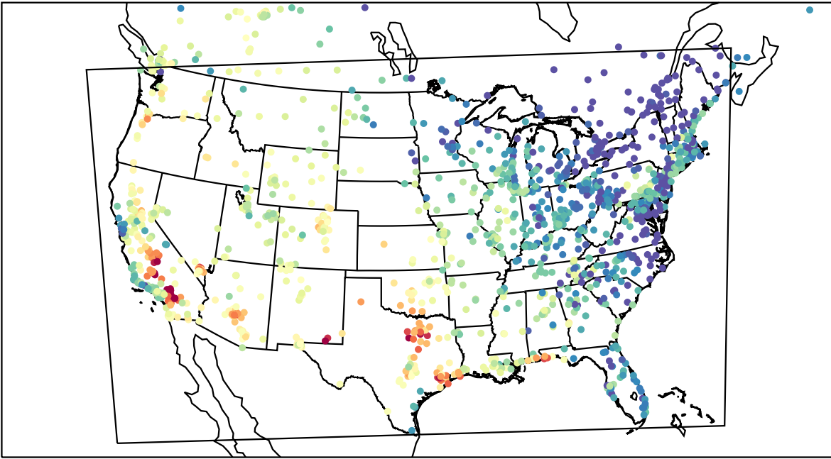
AirNOW (2023-09-10_00:00:00)
