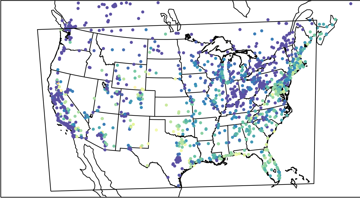
AirNOW (2023-09-09_14:00:00)
