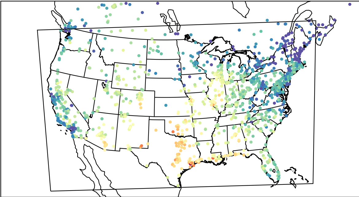
AirNOW (2023-09-10_17:00:00)
