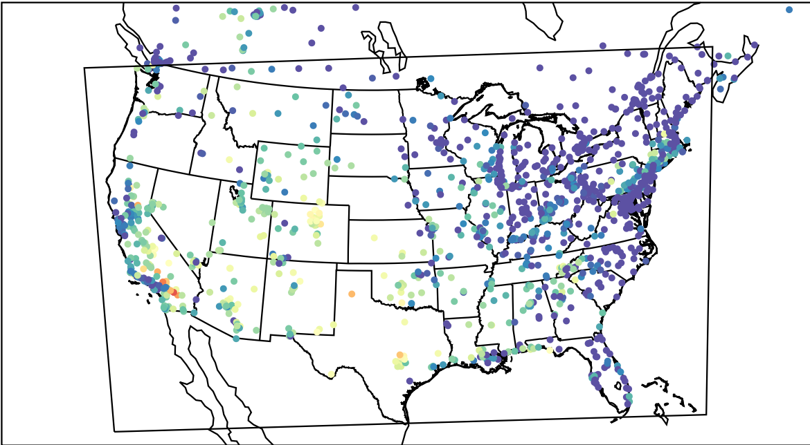
AirNOW (2023-09-10_04:00:00)
