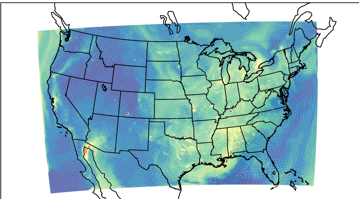
WRF 2023-09-11_21:00:00
