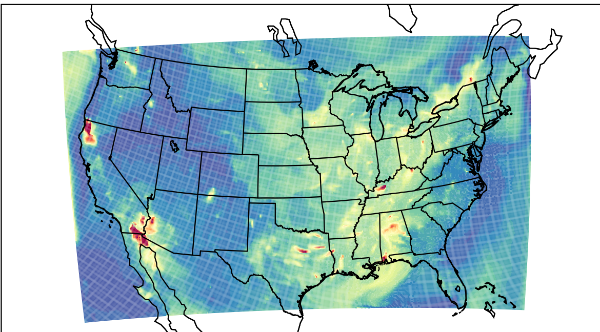
WRF 2023-09-11_05:00:00
