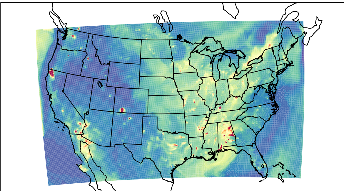
WRF 2023-09-11_02:00:00
