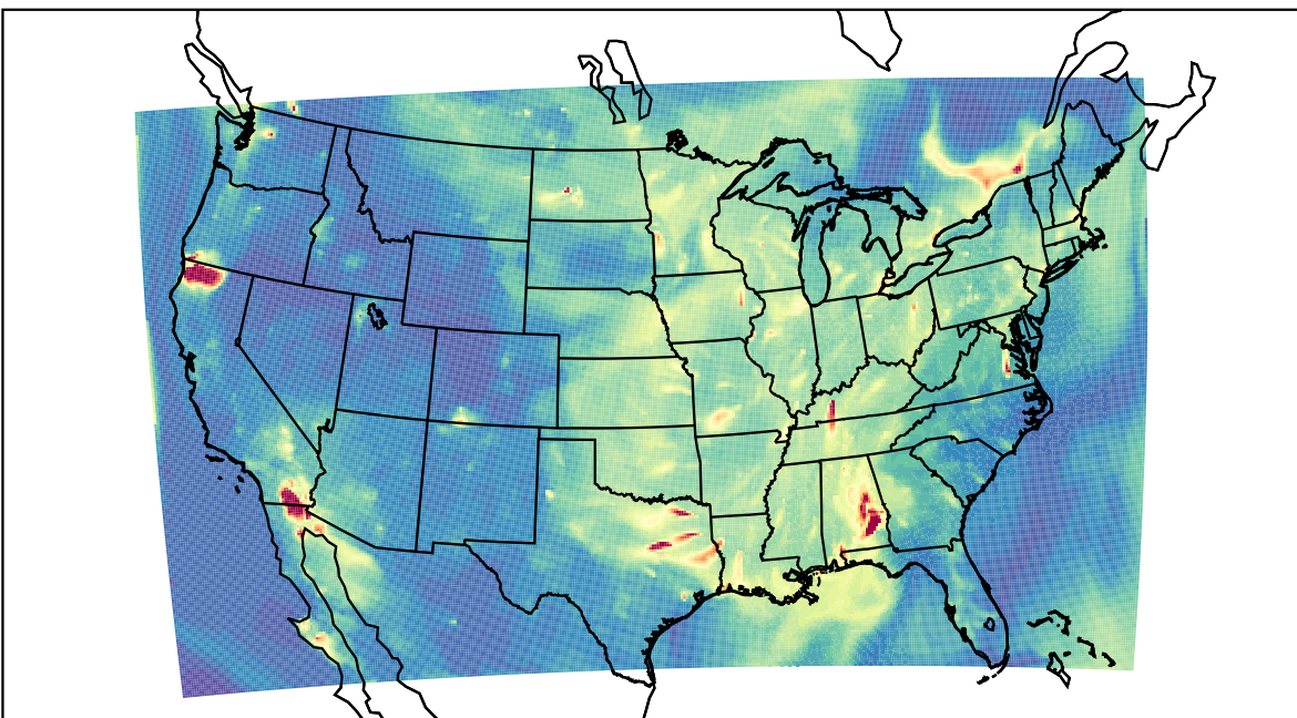
WRF 2023-09-10_05:00:00
