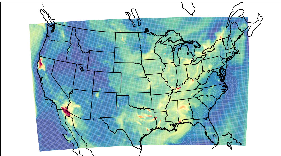
WRF 2023-09-11_07:00:00
