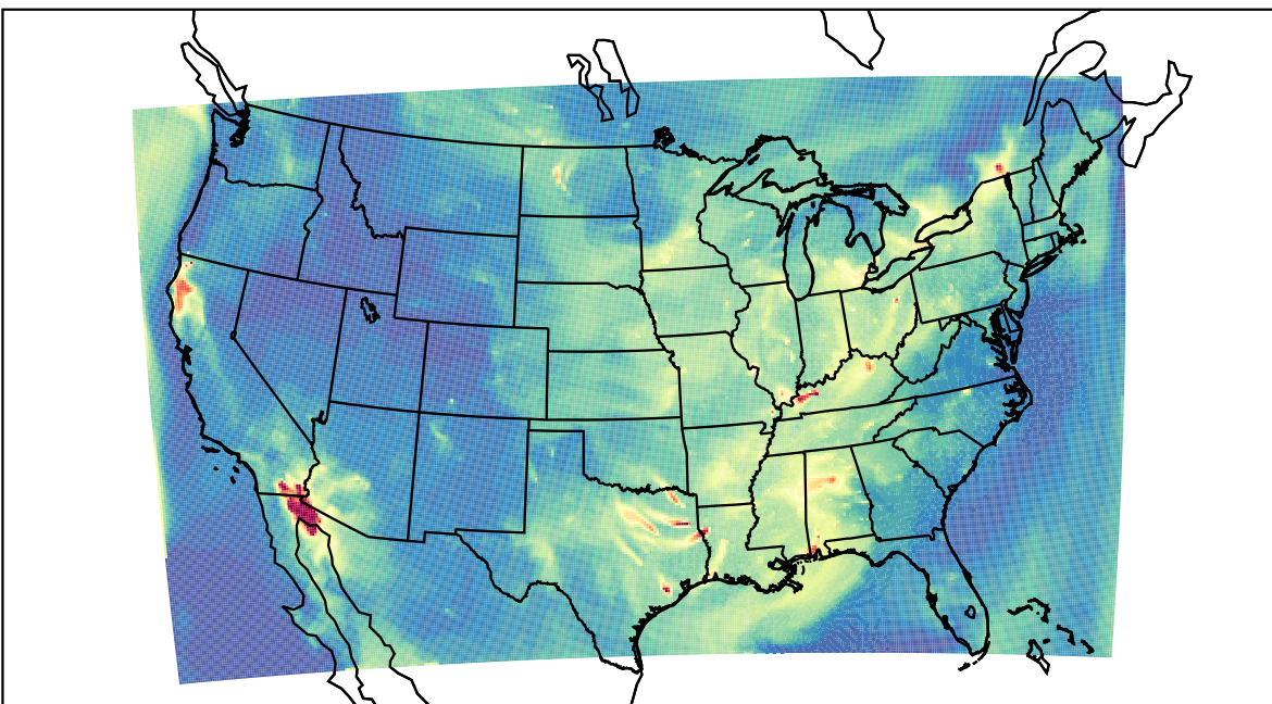
WRF 2023-09-11_09:00:00
