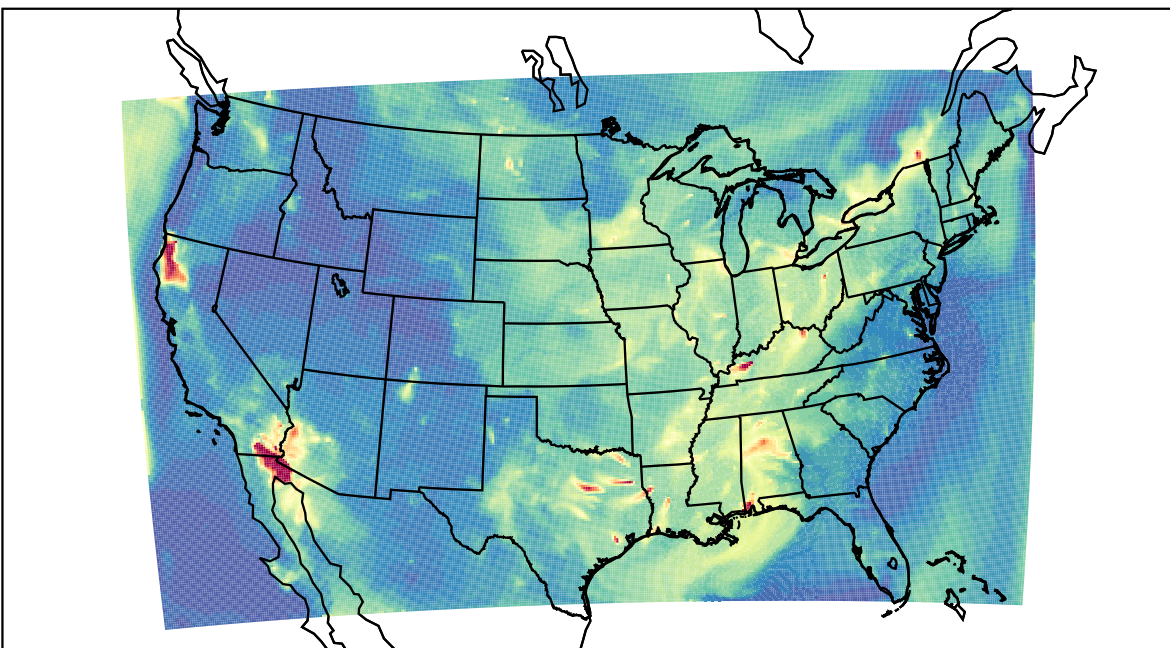
WRF 2023-09-11_06:00:00
