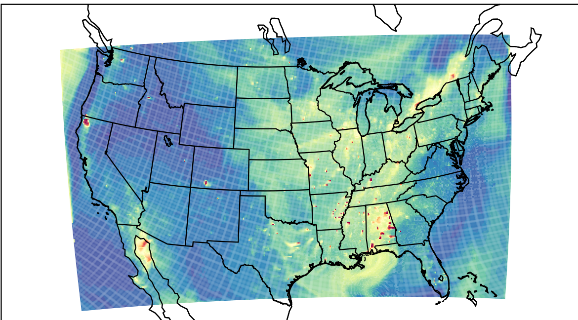
WRF 2023-09-11_00:00:00
