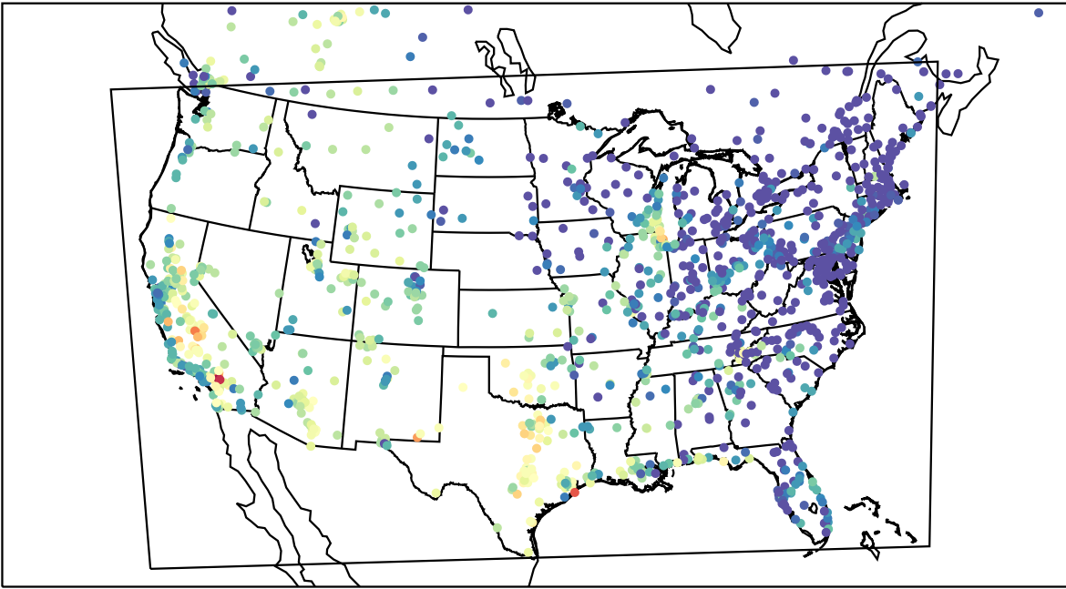
AirNOW (2023-09-11_02:00:00)
