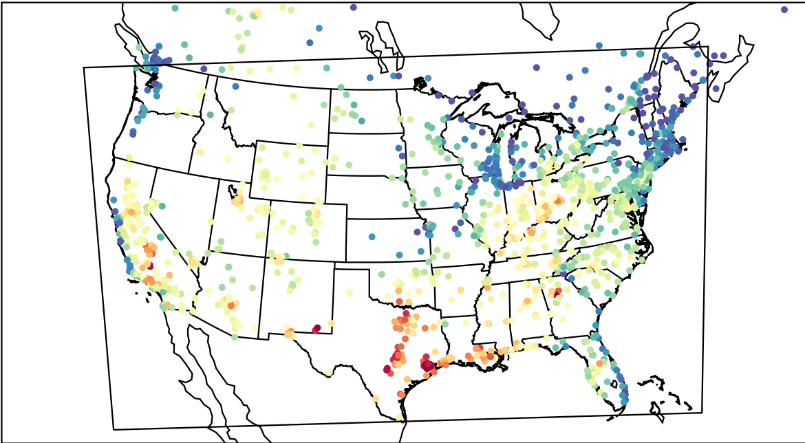
AirNOW (2023-09-11_20:00:00)
