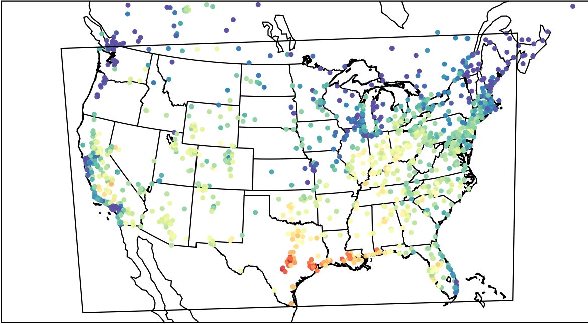
AirNOW (2023-09-11_17:00:00)
