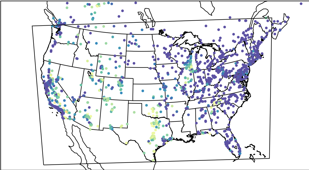
AirNOW (2023-09-11_07:00:00)
