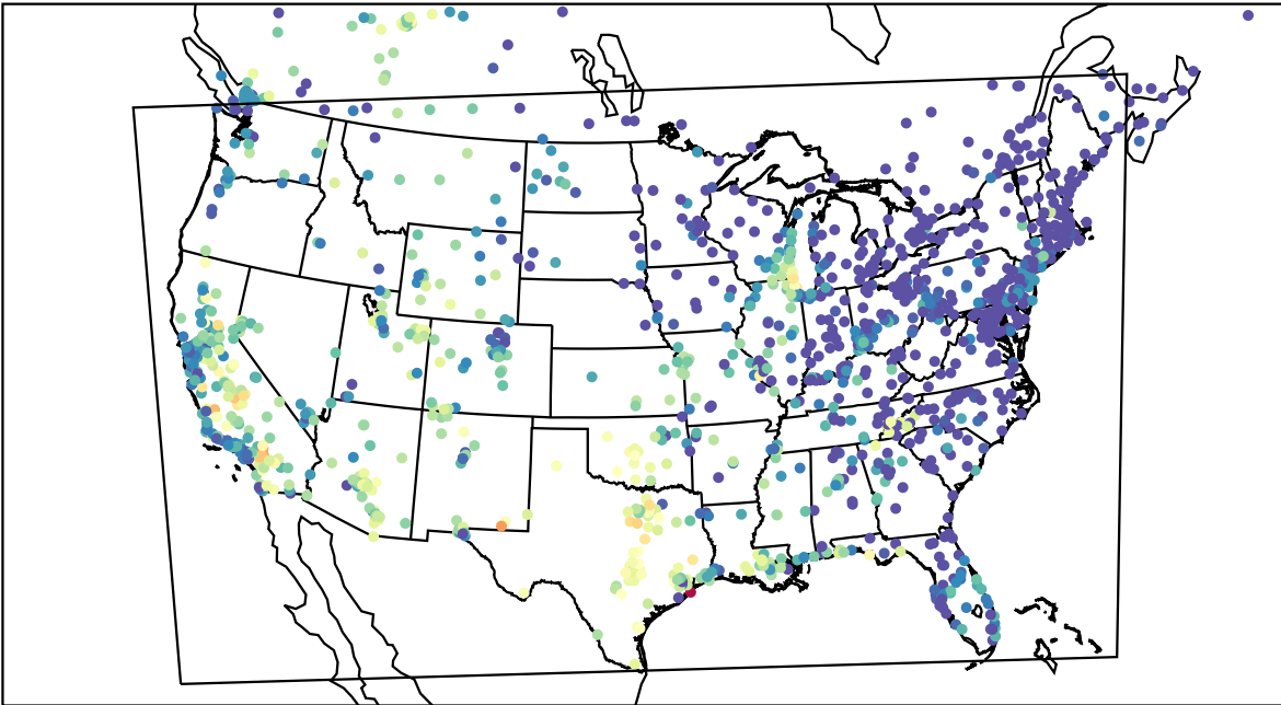
AirNOW (2023-09-11_03:00:00)
