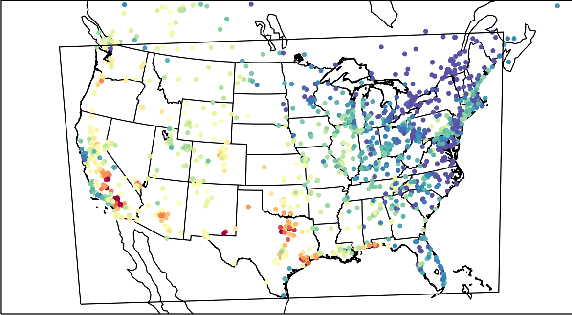
AirNOW (2023-09-10_00:00:00)
