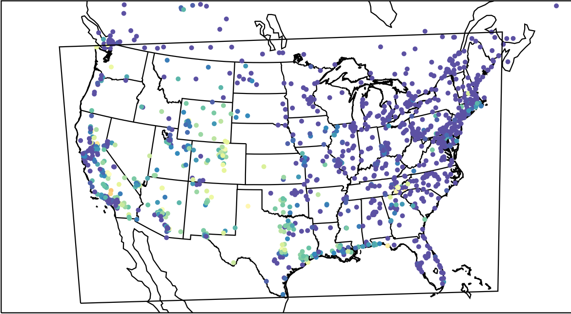
AirNOW (2023-09-10_10:00:00)
