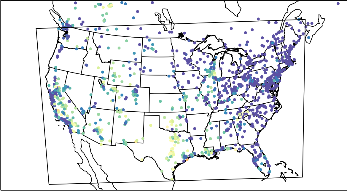
AirNOW (2023-09-11_05:00:00)
