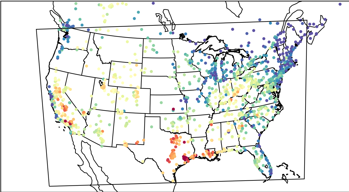
AirNOW (2023-09-11_22:00:00)
