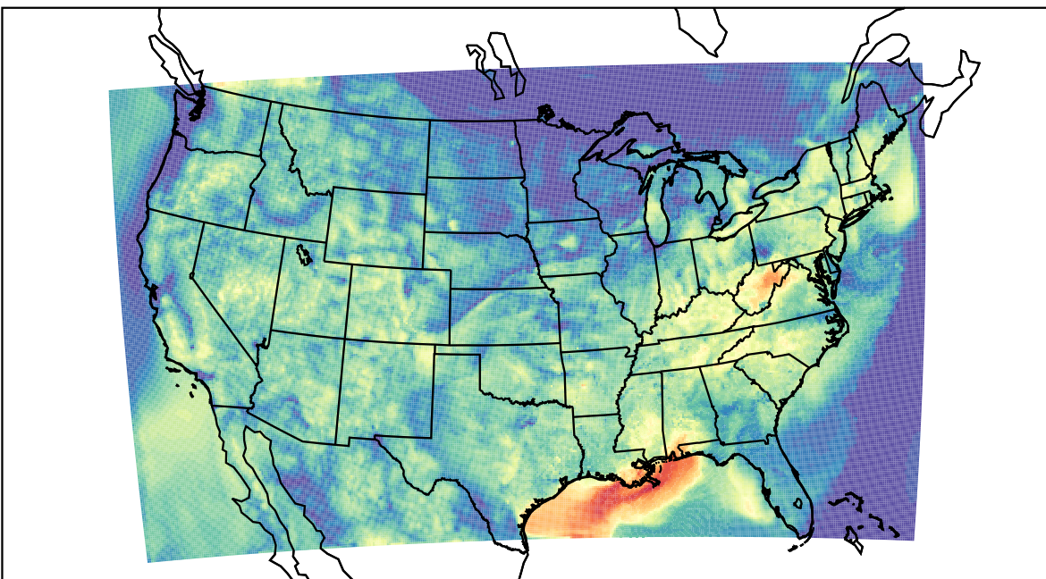
WRF (2023-09-11_14:00:00)
