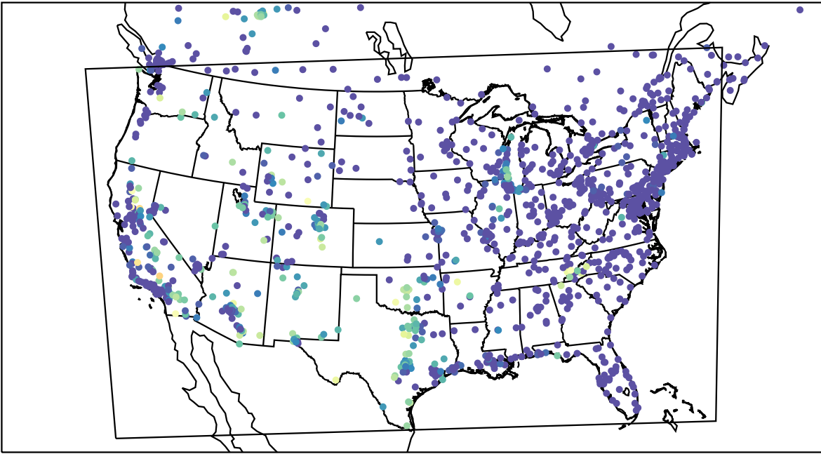
AirNOW (2023-09-11_11:00:00)
