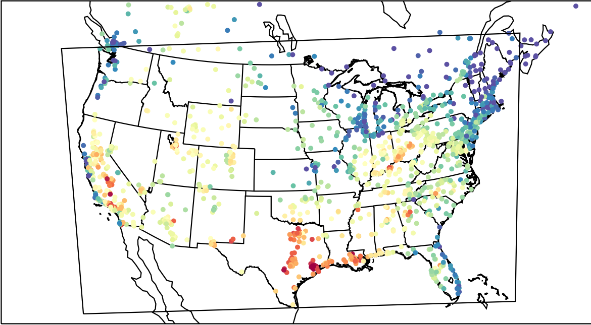
AirNOW (2023-09-11_21:00:00)
