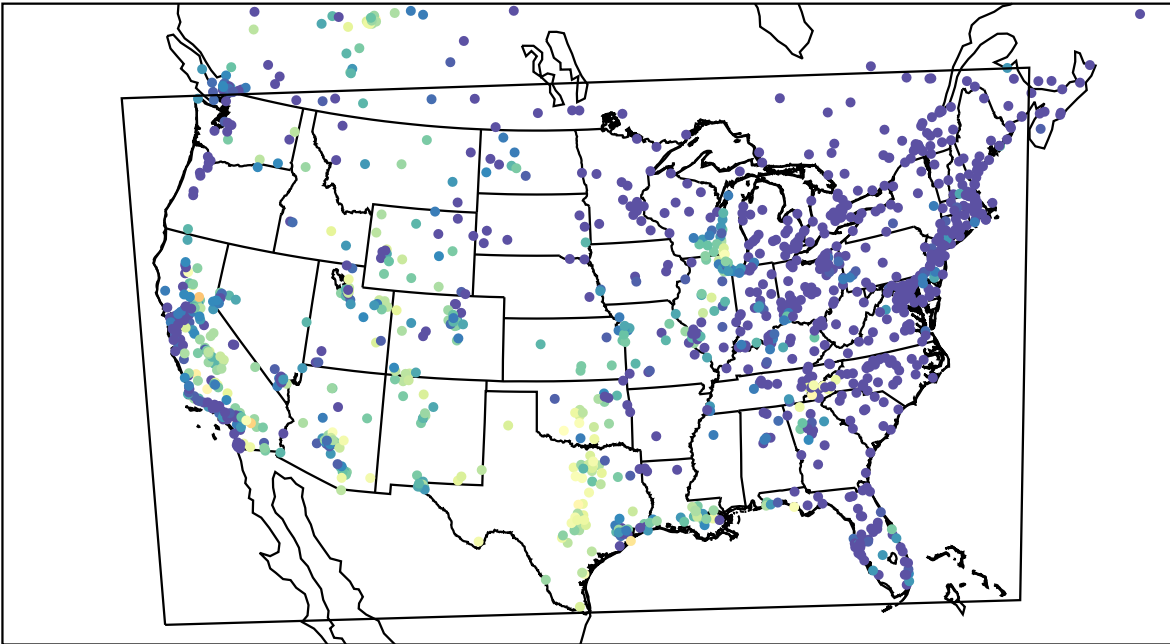
AirNOW (2023-09-11_06:00:00)
