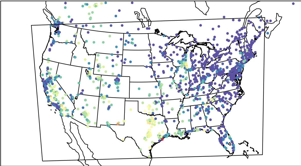
AirNOW (2023-09-11_04:00:00)
