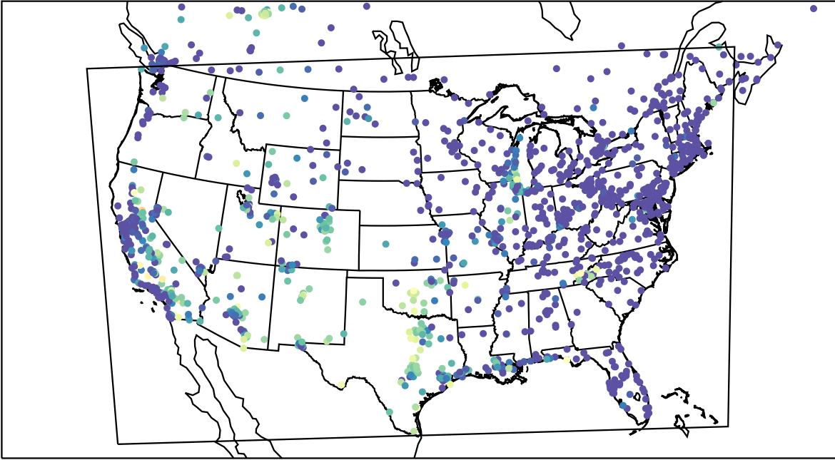
AirNOW (2023-09-11_09:00:00)
