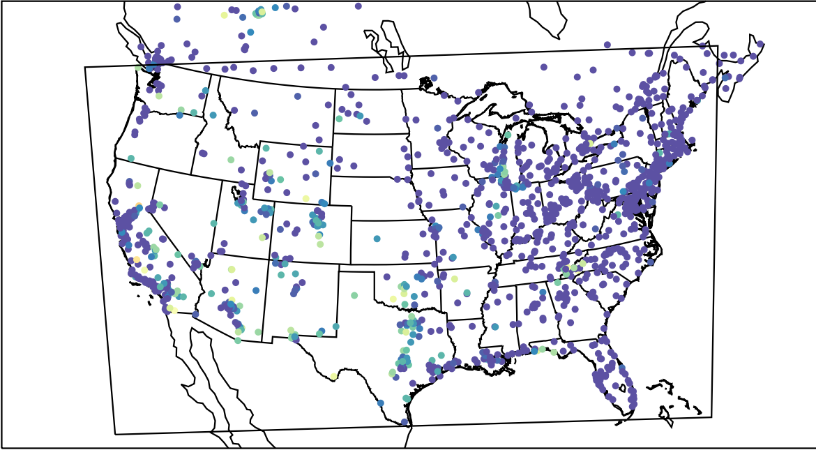
AirNOW (2023-09-11_12:00:00)
