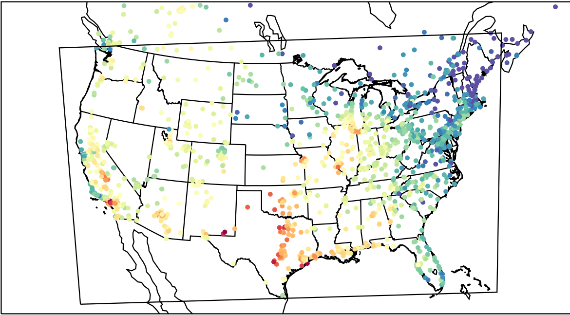
AirNOW (2023-09-10_21:00:00)
