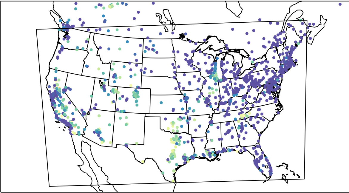
AirNOW (2023-09-11_08:00:00)
