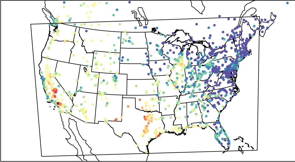
AirNOW (2023-09-11_00:00:00)
