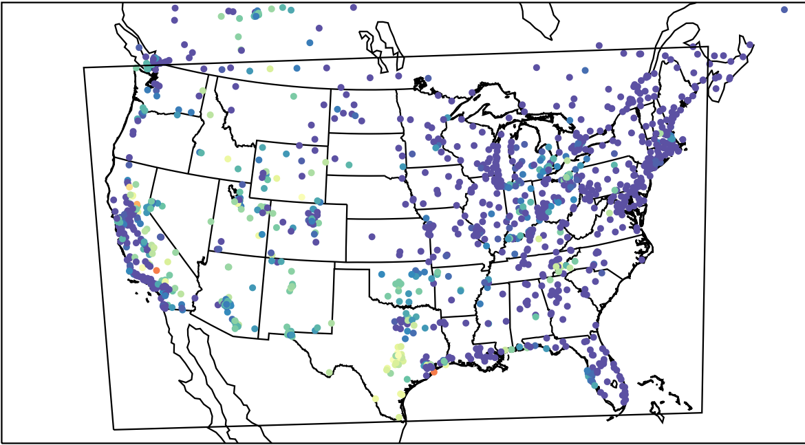
AirNOW (2023-09-12_08:00:00)
