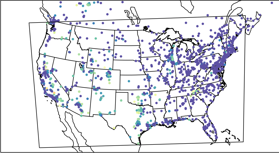
AirNOW (2023-09-11_11:00:00)
