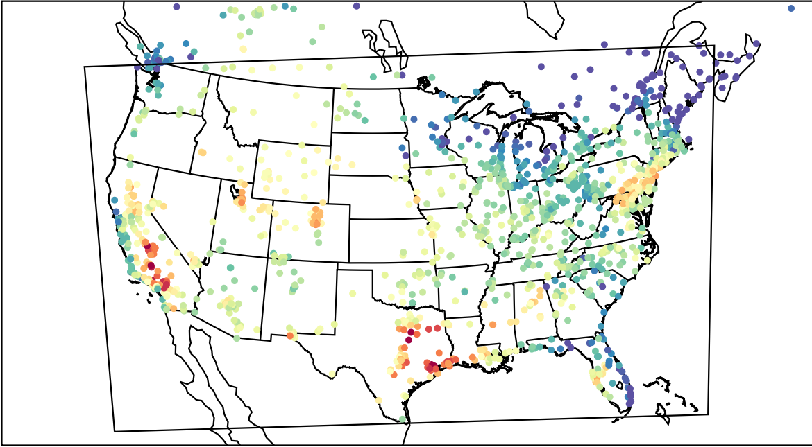
AirNOW (2023-09-12_21:00:00)
