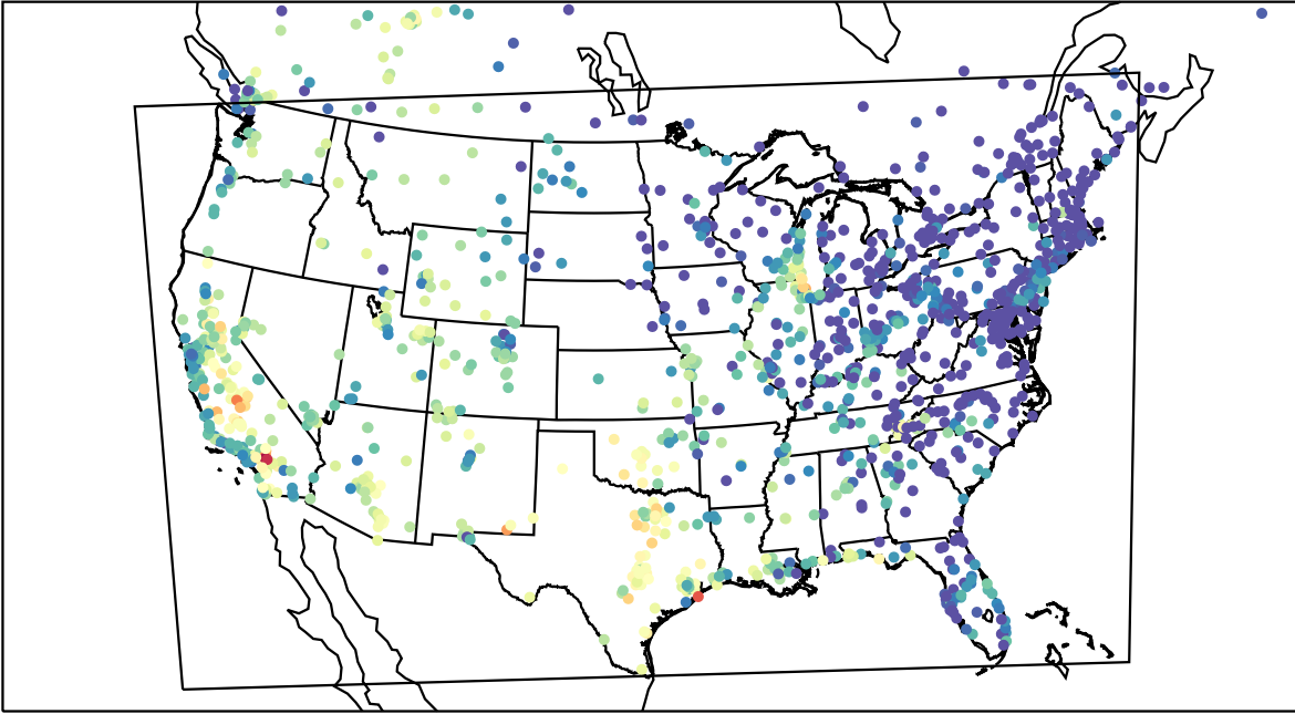
AirNOW (2023-09-11_02:00:00)
