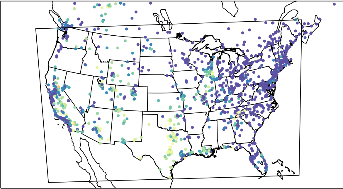
AirNOW (2023-09-11_06:00:00)
