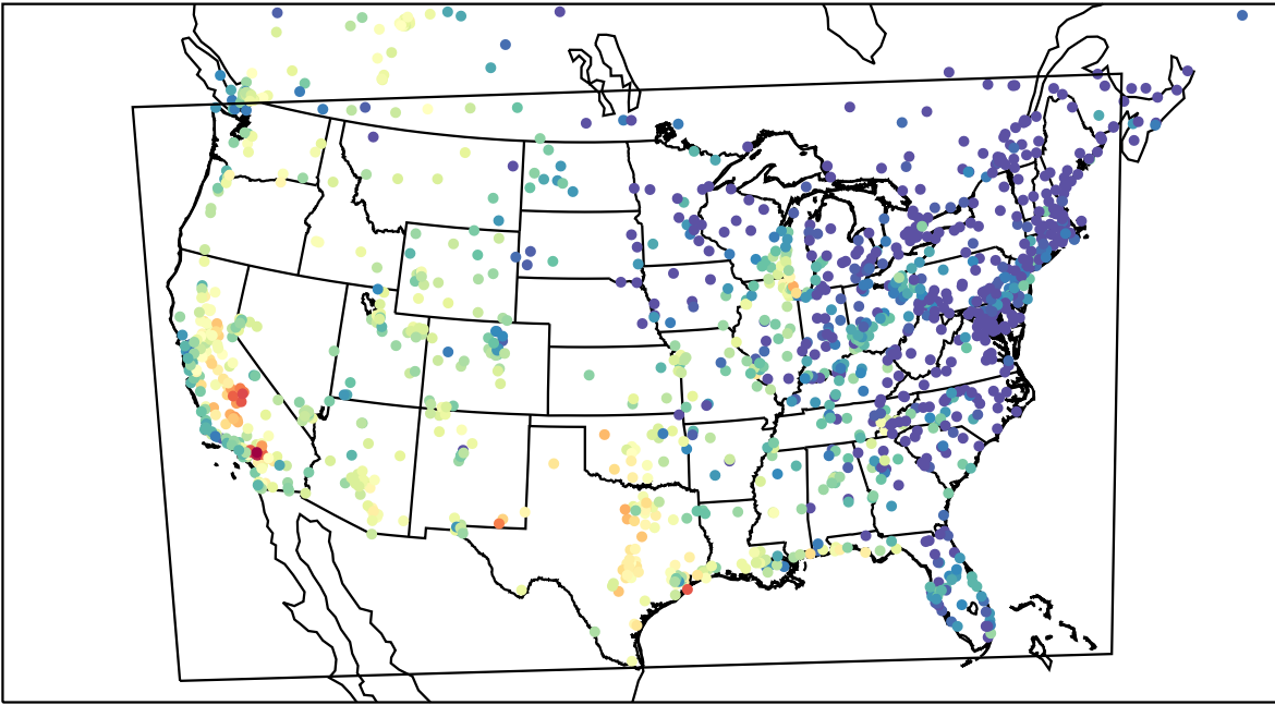
AirNOW (2023-09-11_01:00:00)
