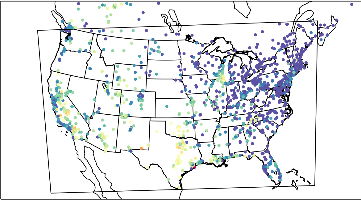
AirNOW (2023-09-11_03:00:00)
