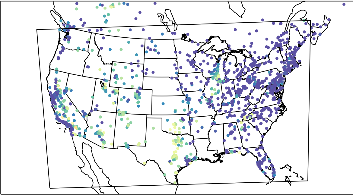
AirNOW (2023-09-11_07:00:00)
