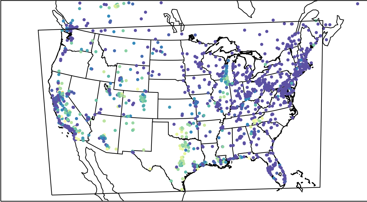
AirNOW (2023-09-11_08:00:00)
