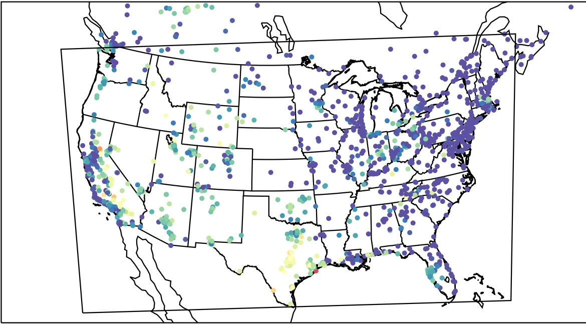
AirNOW (2023-09-12_05:00:00)
