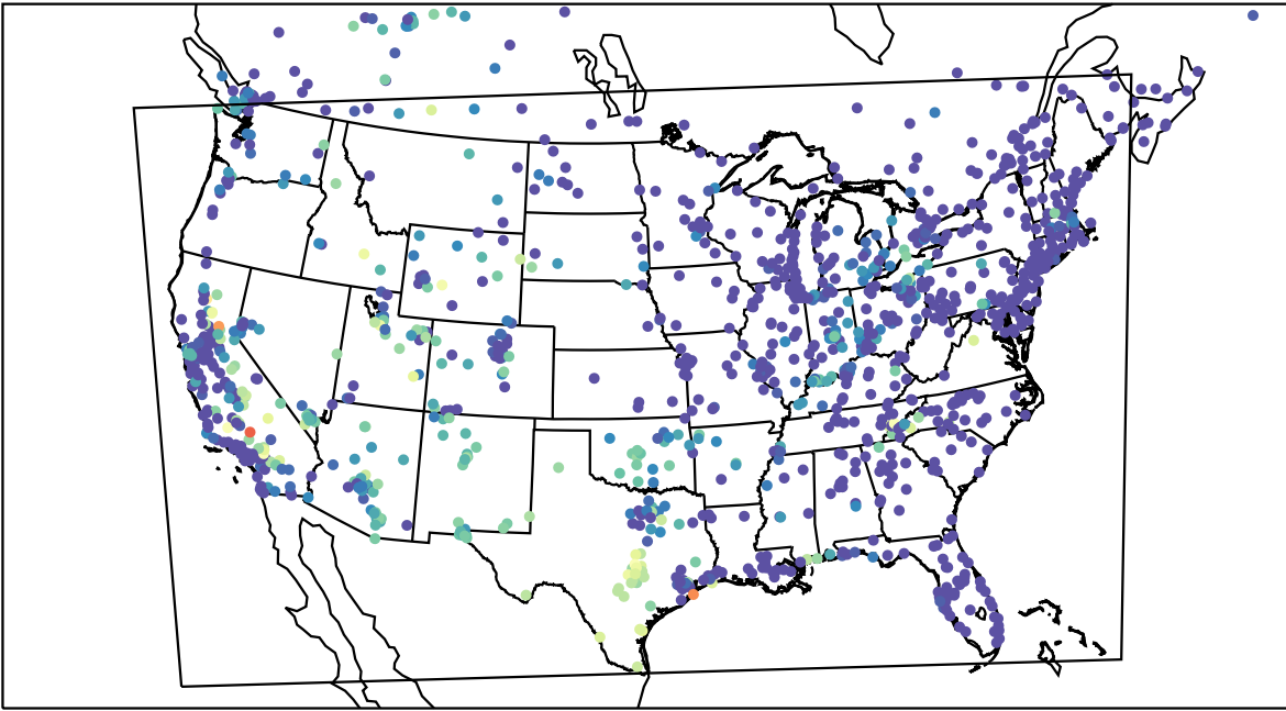
AirNOW (2023-09-12_09:00:00)
