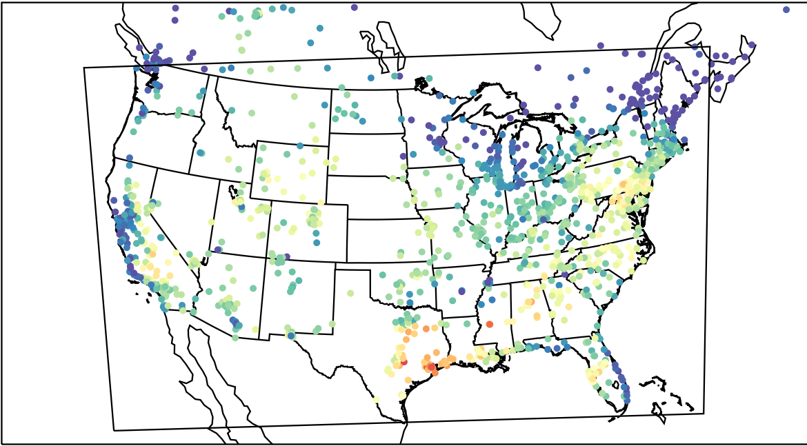
AirNOW (2023-09-12_17:00:00)
