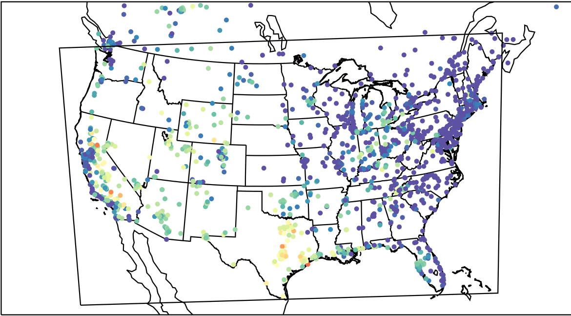
AirNOW (2023-09-12_03:00:00)
