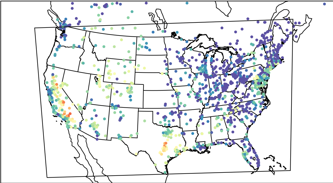
AirNOW (2023-09-13_02:00:00)
