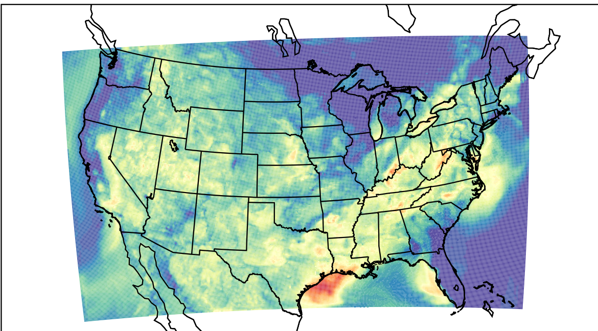
WRF (2023-09-12_06:00:00)
