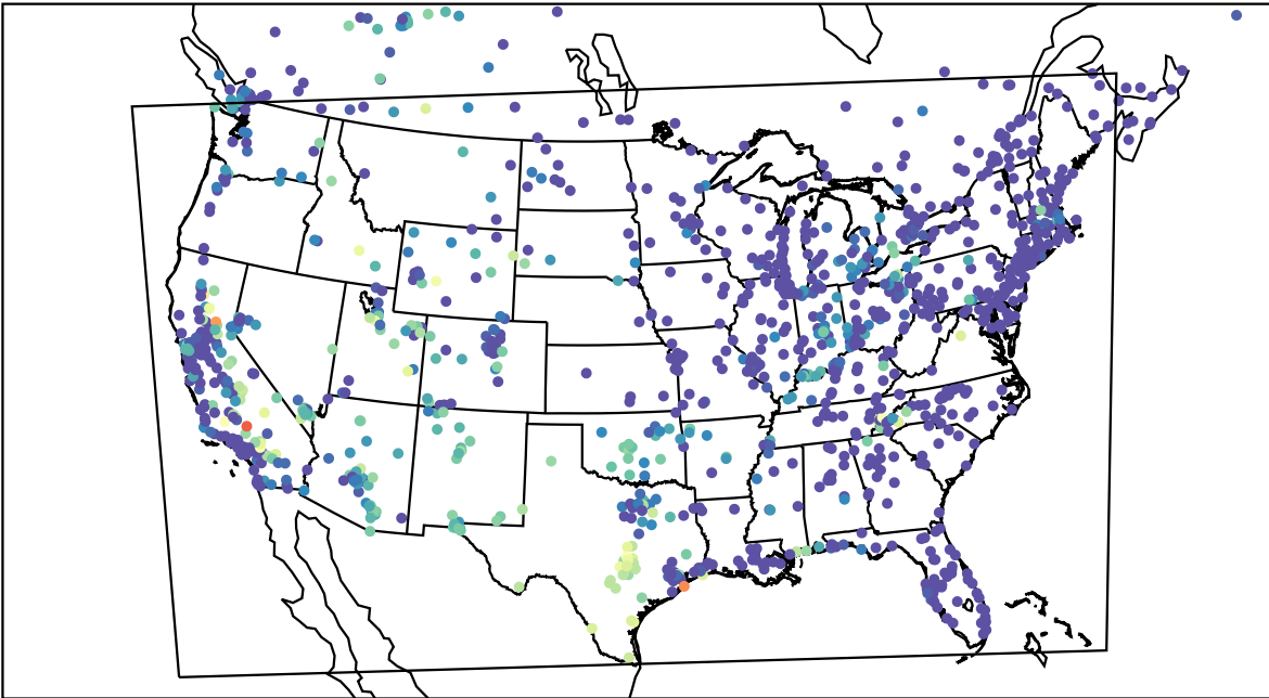
AirNOW (2023-09-12_09:00:00)
