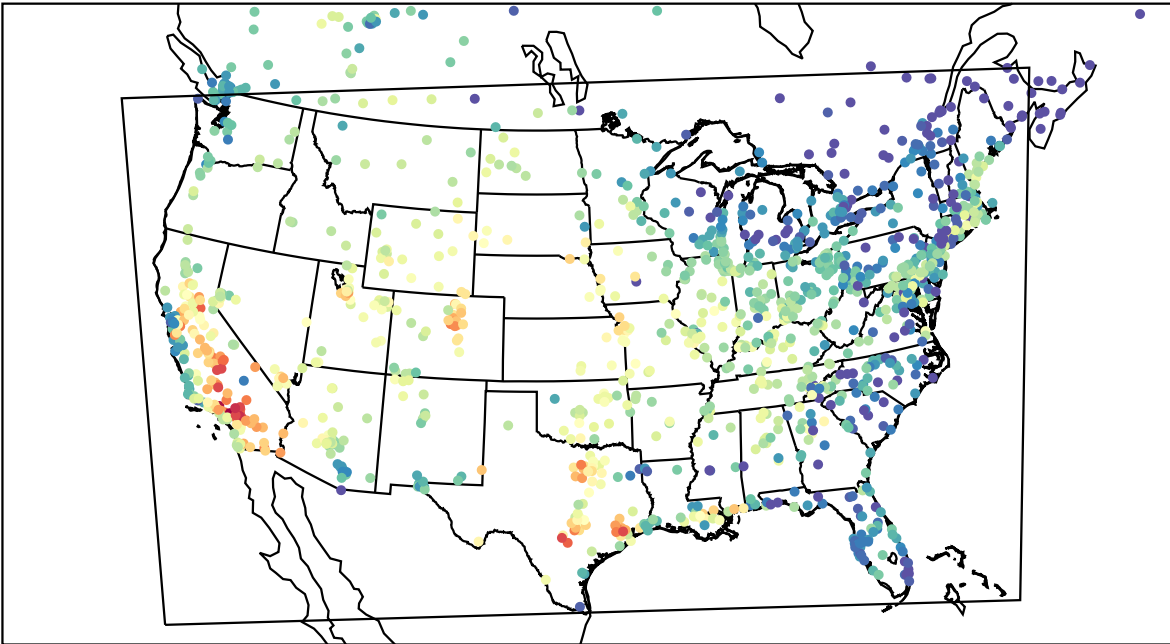
AirNOW (2023-09-13_23:00:00)
