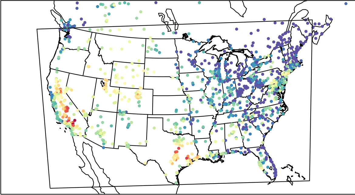
AirNOW (2023-09-13_00:00:00)
