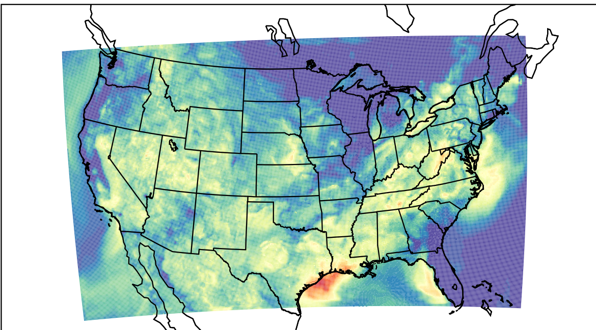
WRF (2023-09-12_08:00:00)
