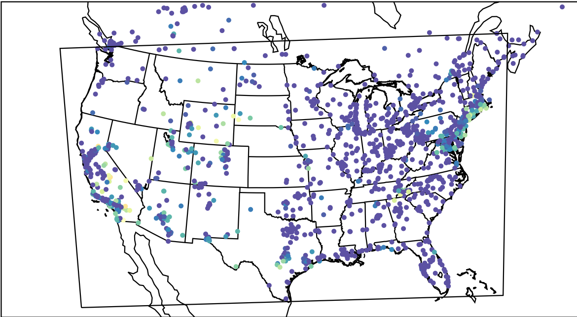
AirNOW (2023-09-13_12:00:00)
