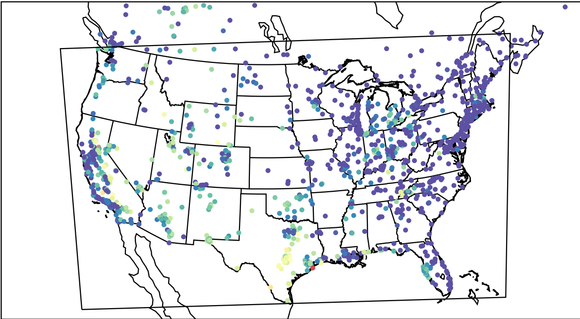
AirNOW (2023-09-12_06:00:00)
