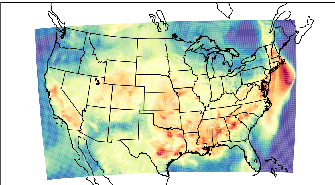
WRF (2023-09-13_22:00:00)
