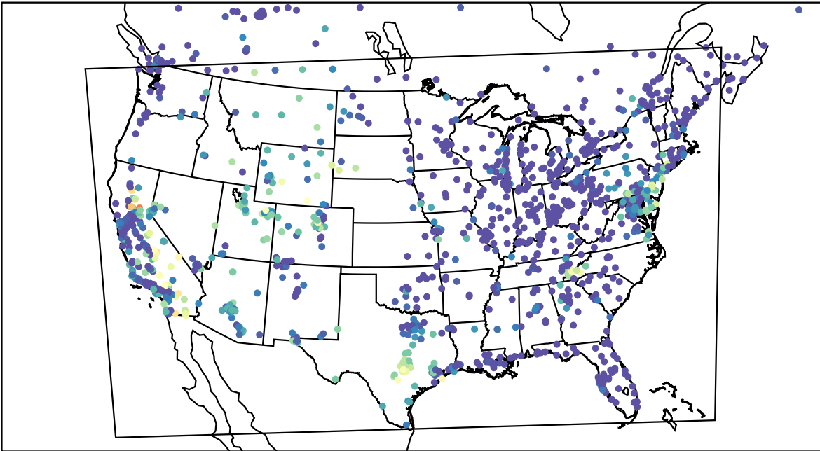
AirNOW (2023-09-13_08:00:00)
