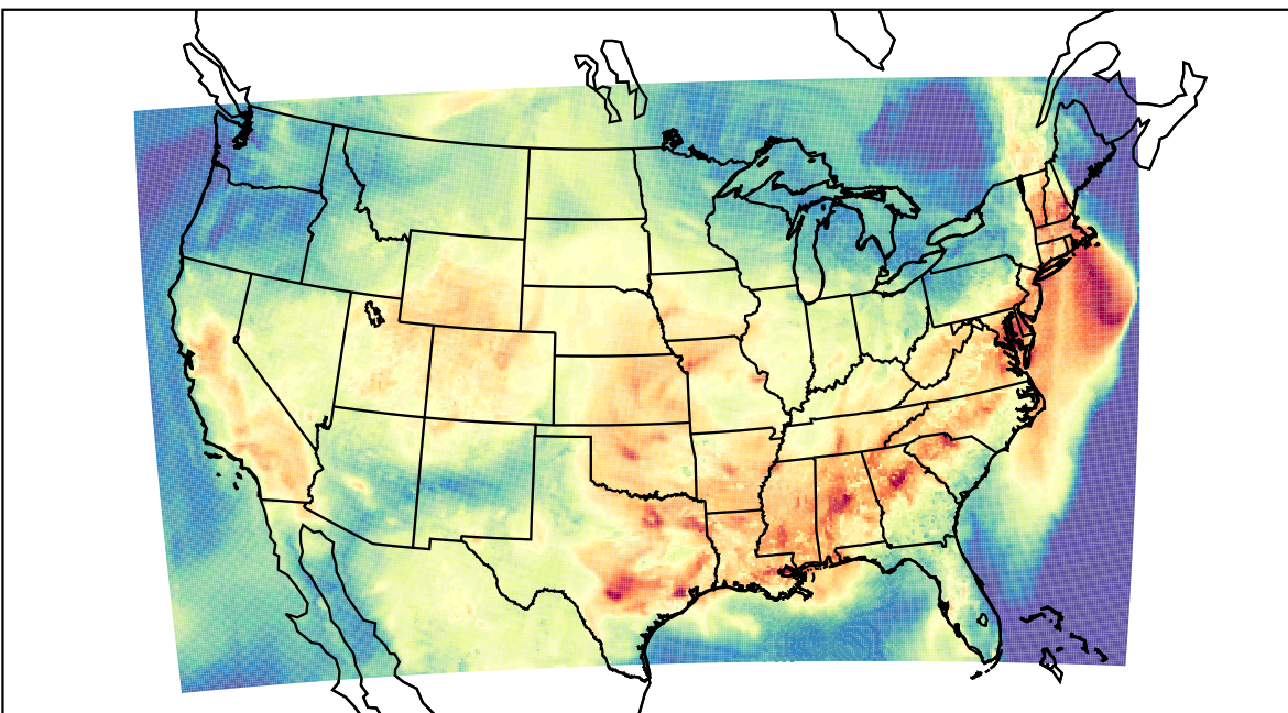
WRF (2023-09-13_21:00:00)
