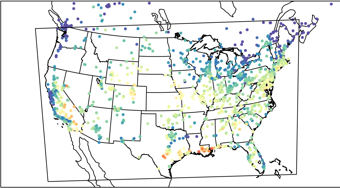
AirNOW (2023-09-13_17:00:00)
