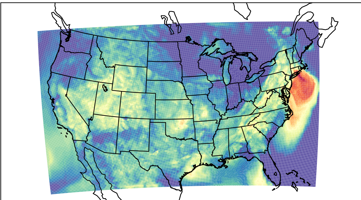
WRF (2023-09-13_09:00:00)
