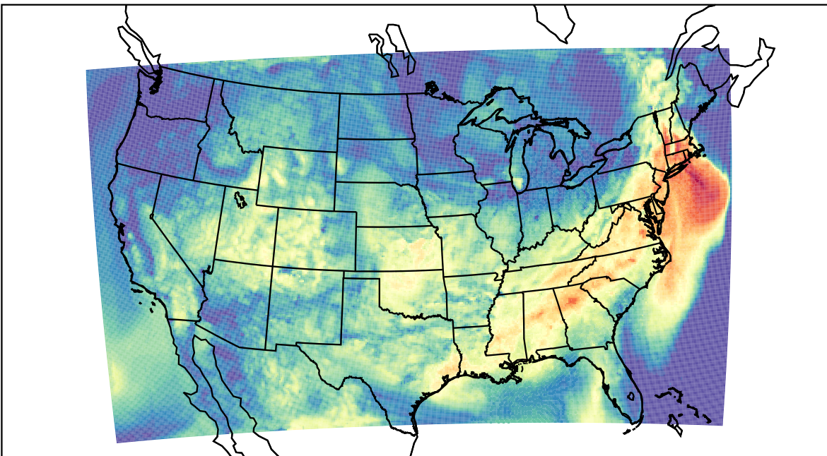
WRF (2023-09-13_15:00:00)
