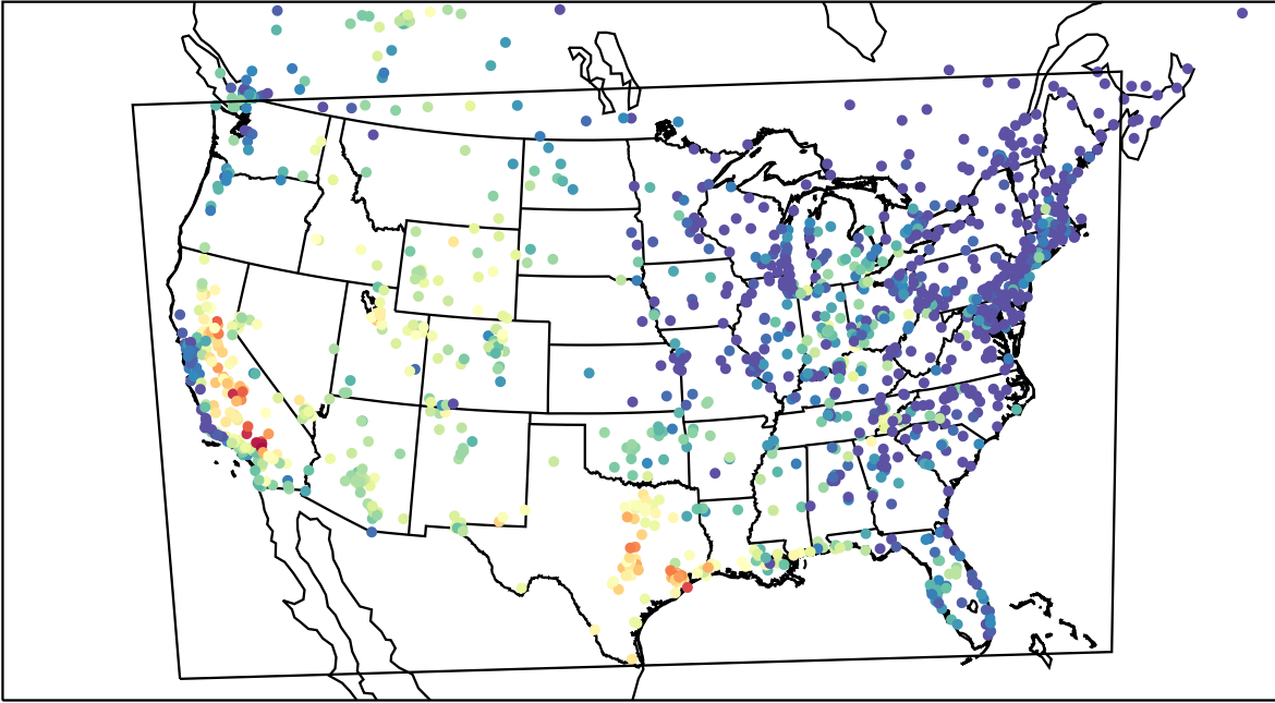
AirNOW (2023-09-12_01:00:00)
