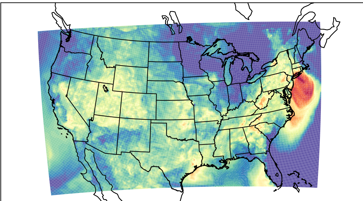
WRF (2023-09-13_05:00:00)
