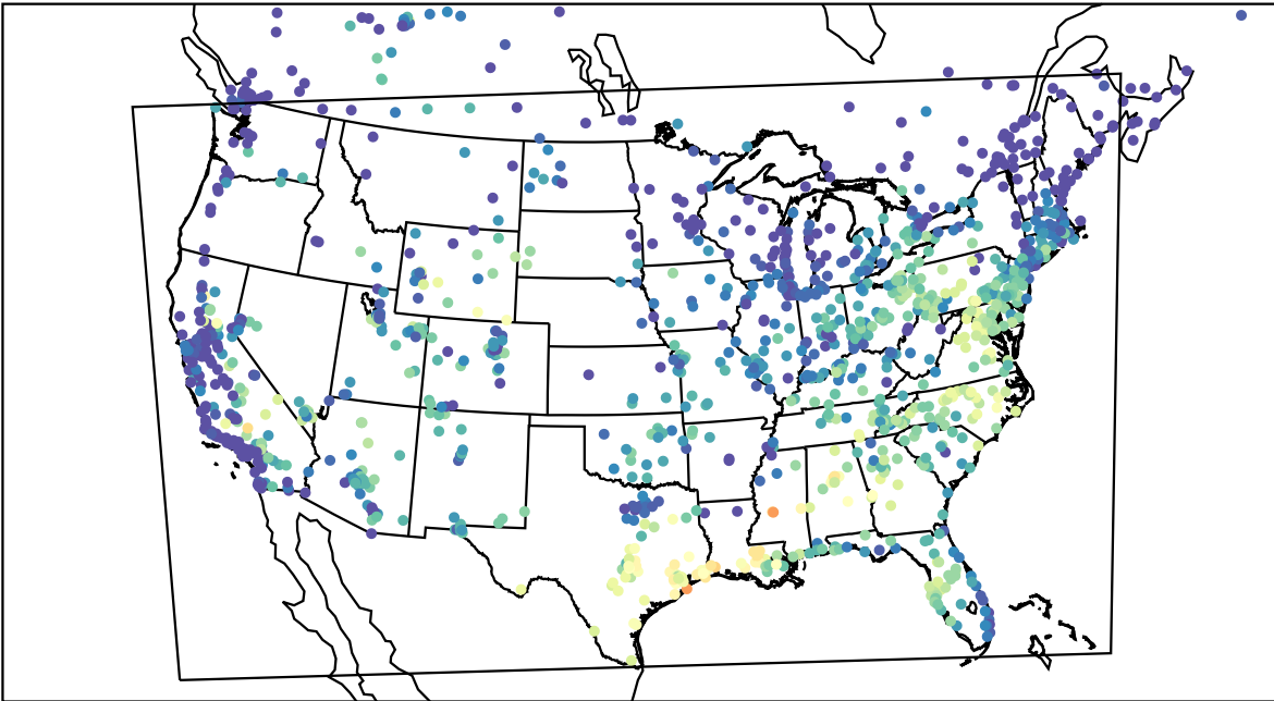
AirNOW (2023-09-12_15:00:00)
