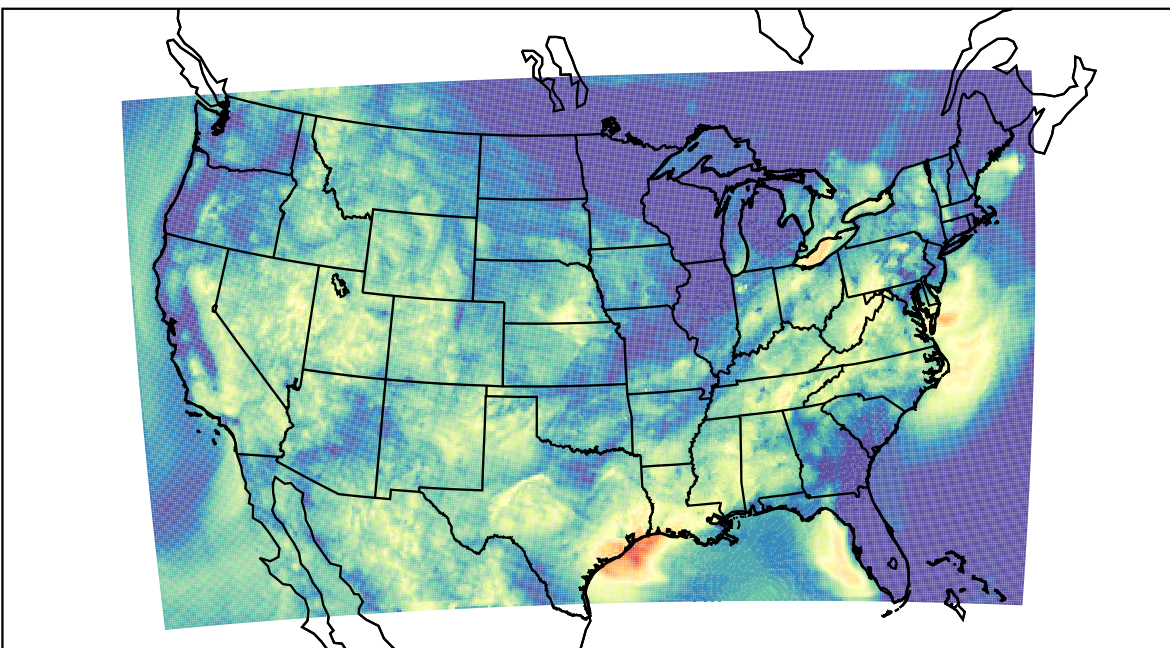
WRF (2023-09-12_11:00:00)
