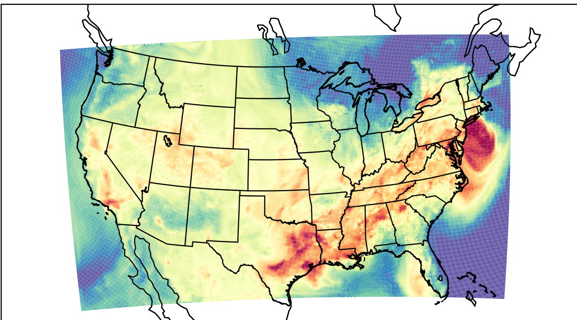
WRF (2023-09-12_22:00:00)
