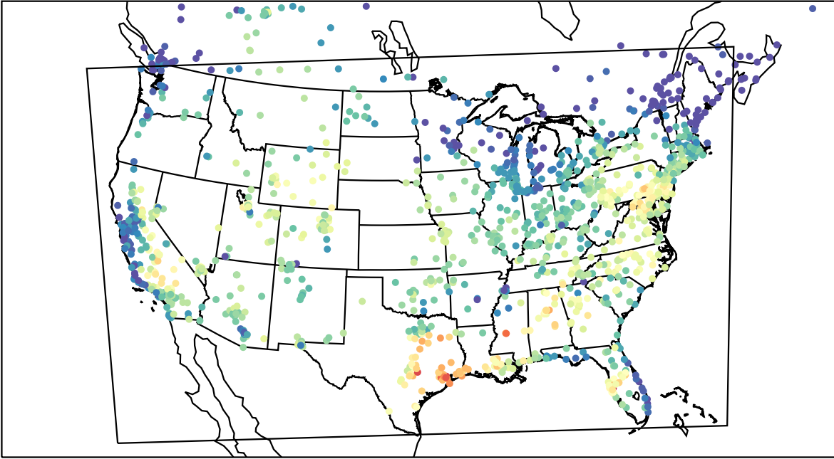
AirNOW (2023-09-12_17:00:00)
