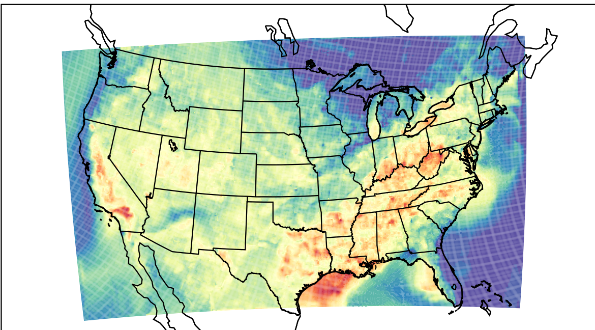
WRF (2023-09-12_01:00:00)
