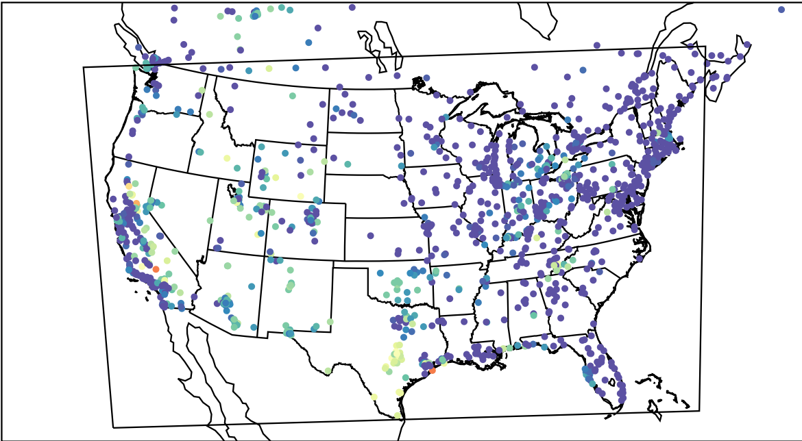
AirNOW (2023-09-12_08:00:00)
