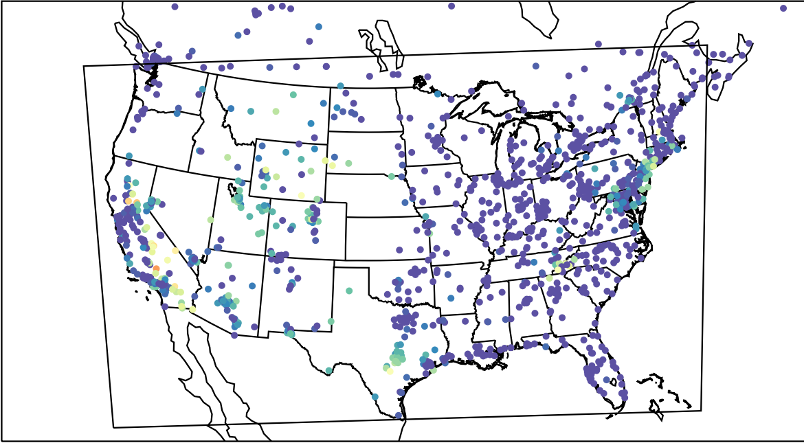
AirNOW (2023-09-13_10:00:00)
