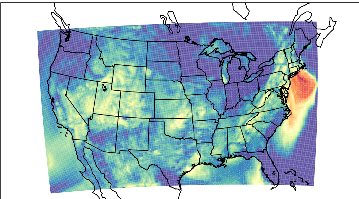
WRF (2023-09-13_12:00:00)
