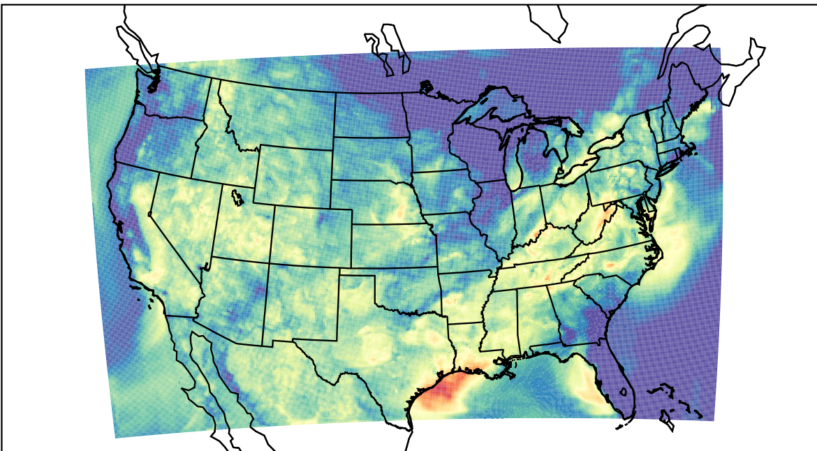
WRF (2023-09-12_07:00:00)
