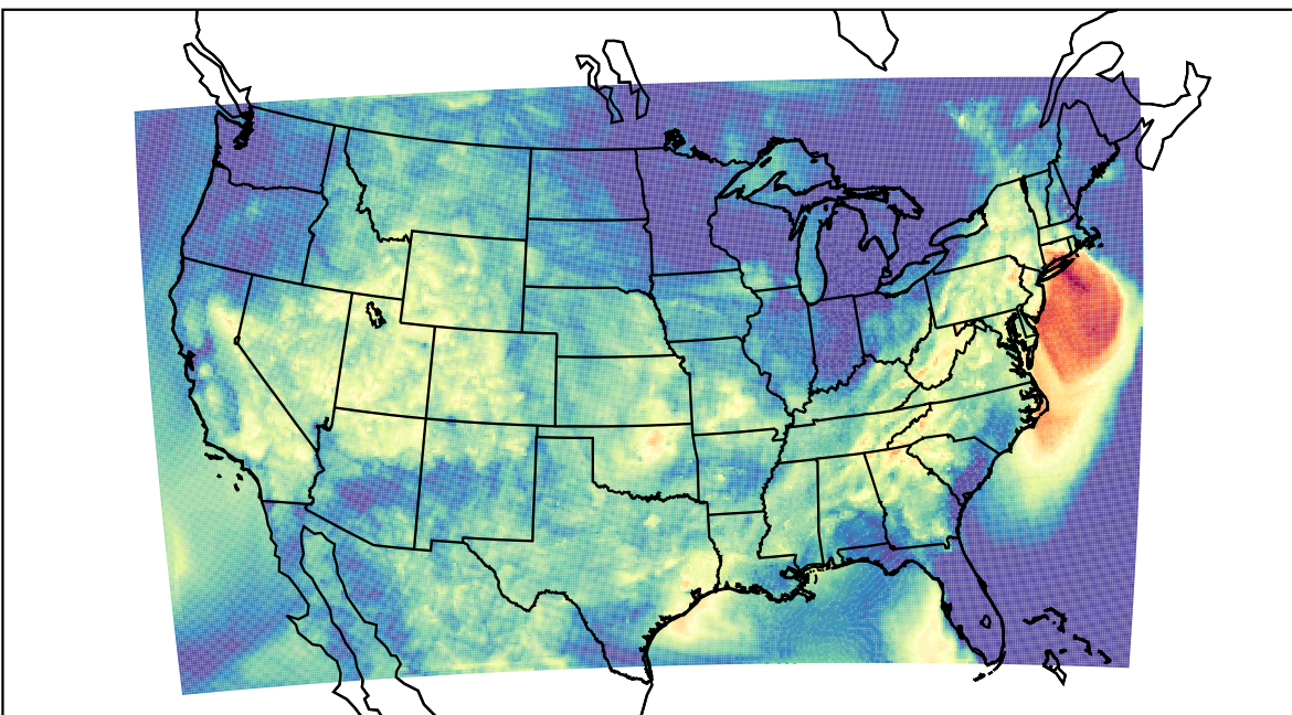
WRF (2023-09-13_07:00:00)
