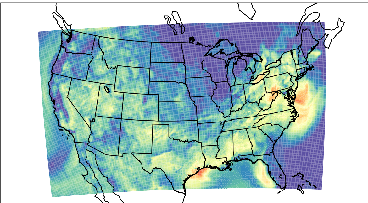
WRF (2023-09-12_14:00:00)
