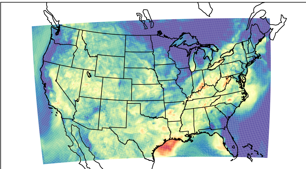
WRF (2023-09-12_05:00:00)
