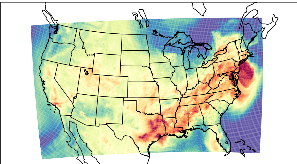
WRF (2023-09-12_21:00:00)
