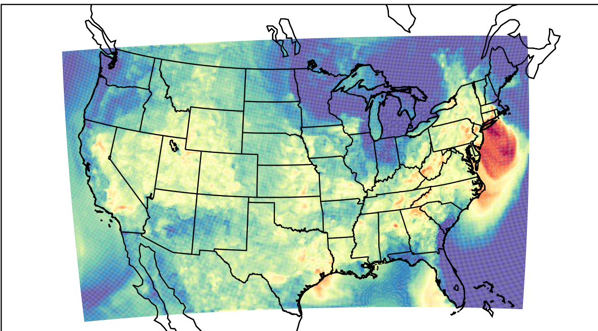
WRF (2023-09-13_03:00:00)
