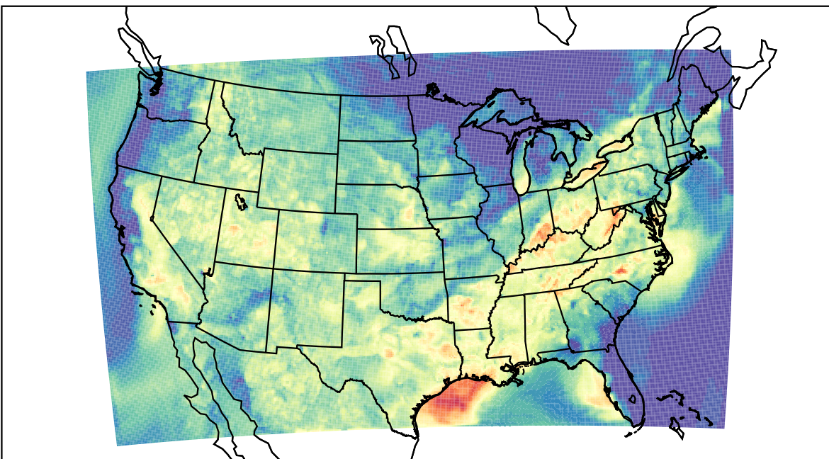
WRF (2023-09-12_04:00:00)
