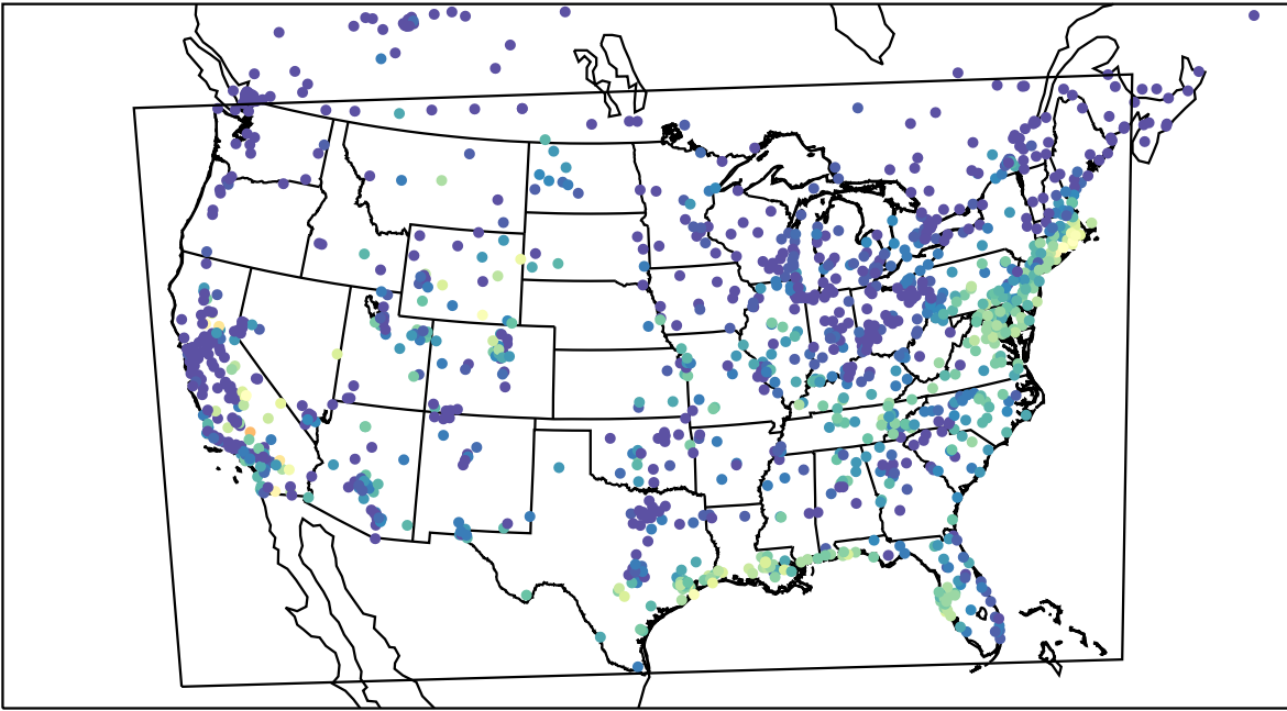
AirNOW (2023-09-13_14:00:00)
