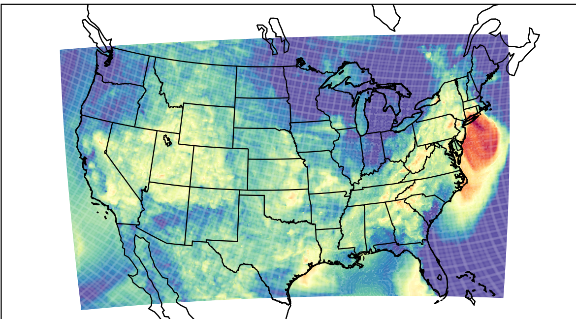
WRF (2023-09-13_06:00:00)
