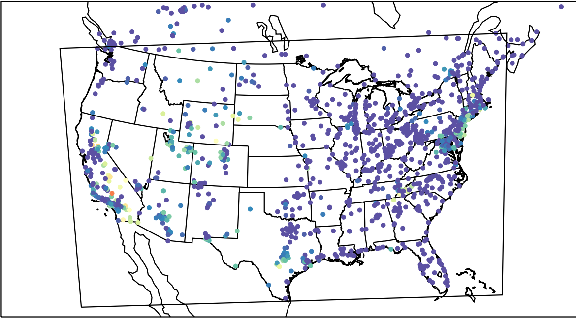
AirNOW (2023-09-13_11:00:00)
