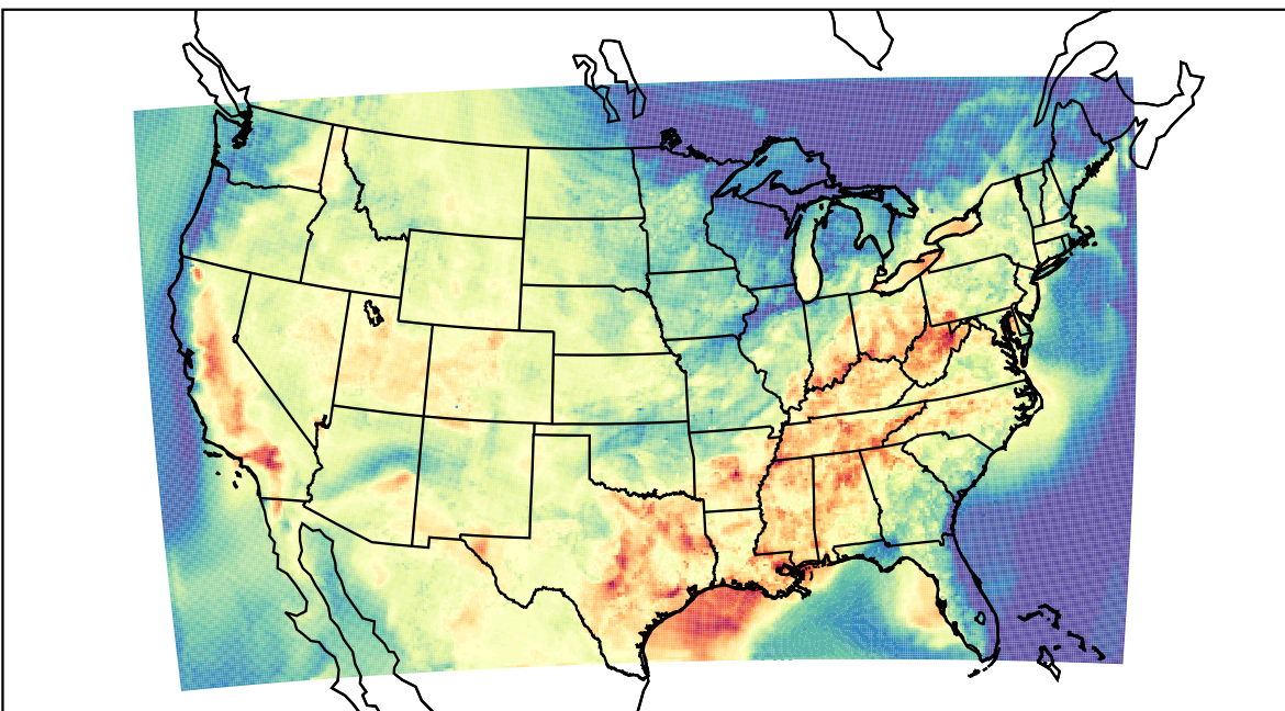
WRF (2023-09-12_00:00:00)
