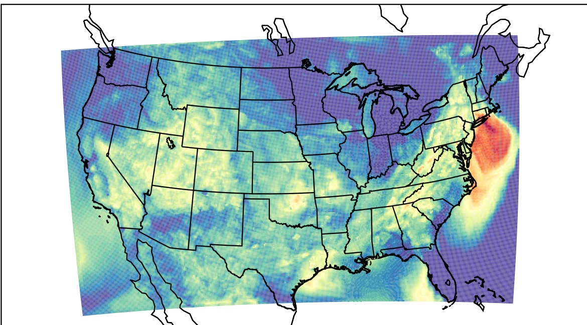
WRF (2023-09-13_08:00:00)
