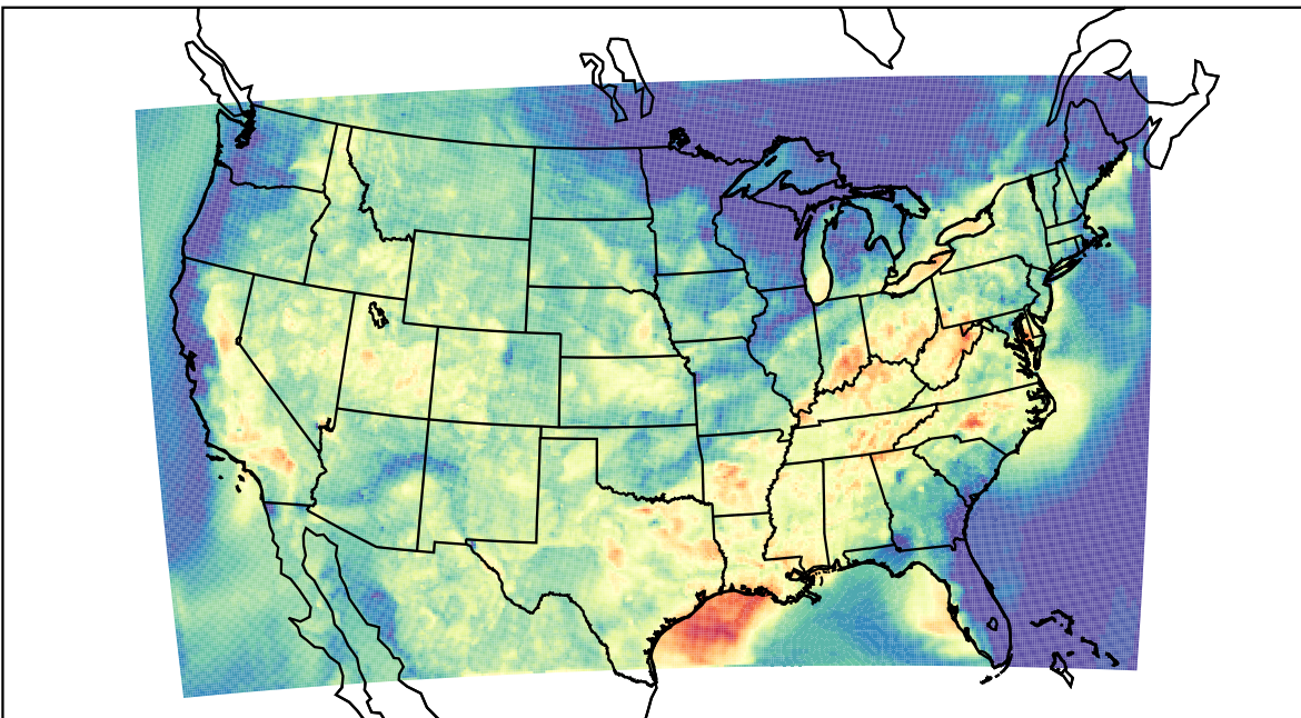
WRF (2023-09-12_03:00:00)
