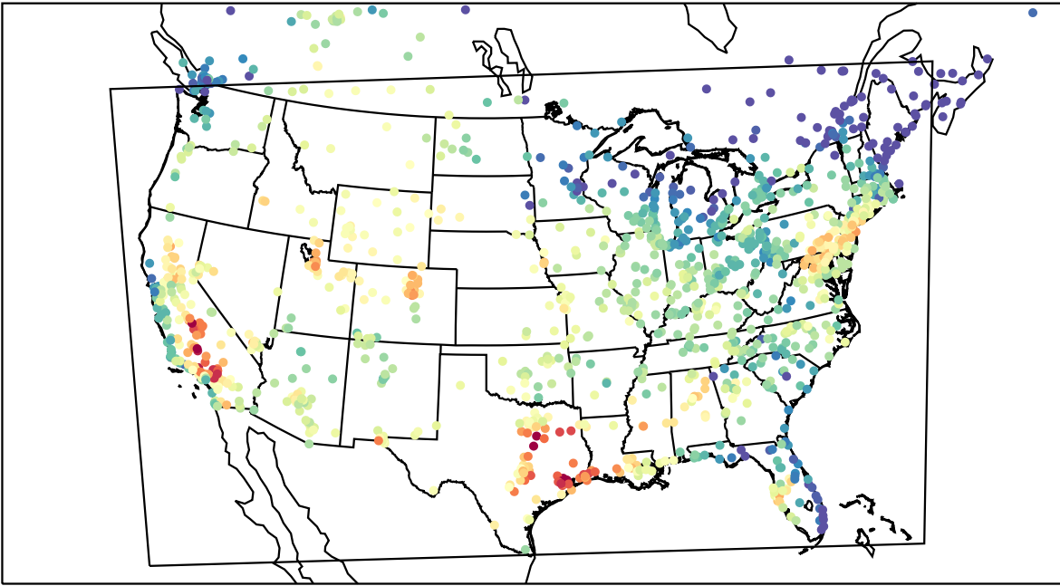
AirNOW (2023-09-12_21:00:00)
