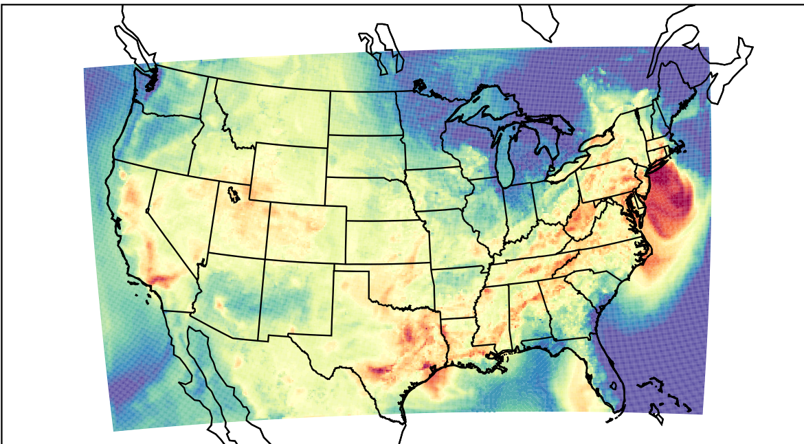
WRF (2023-09-13_00:00:00)
