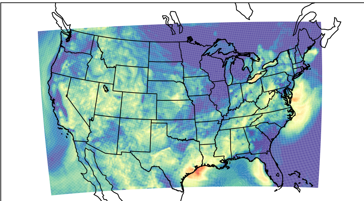
WRF (2023-09-12_12:00:00)
