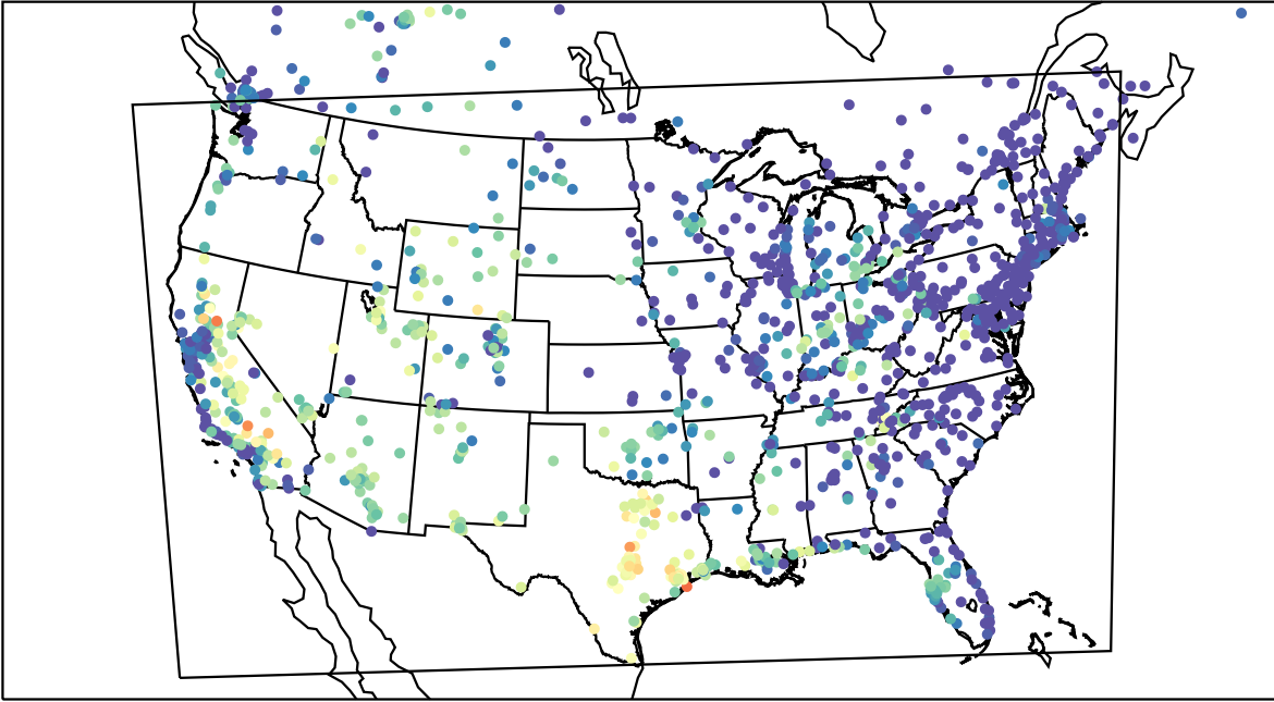
AirNOW (2023-09-12_03:00:00)
