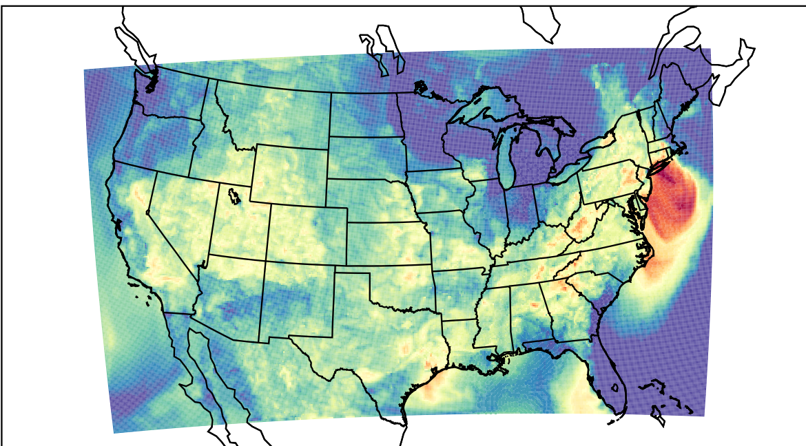
WRF (2023-09-13_04:00:00)
