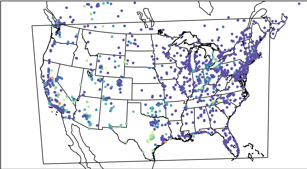
AirNOW (2023-09-12_11:00:00)
