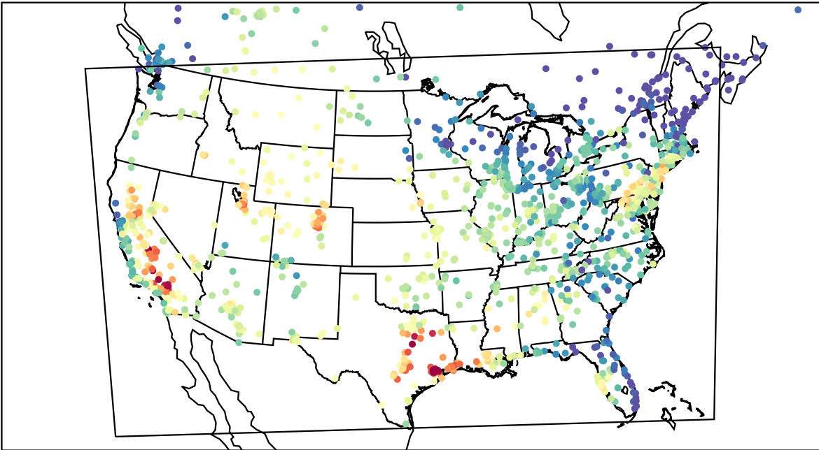
AirNOW (2023-09-12_22:00:00)
