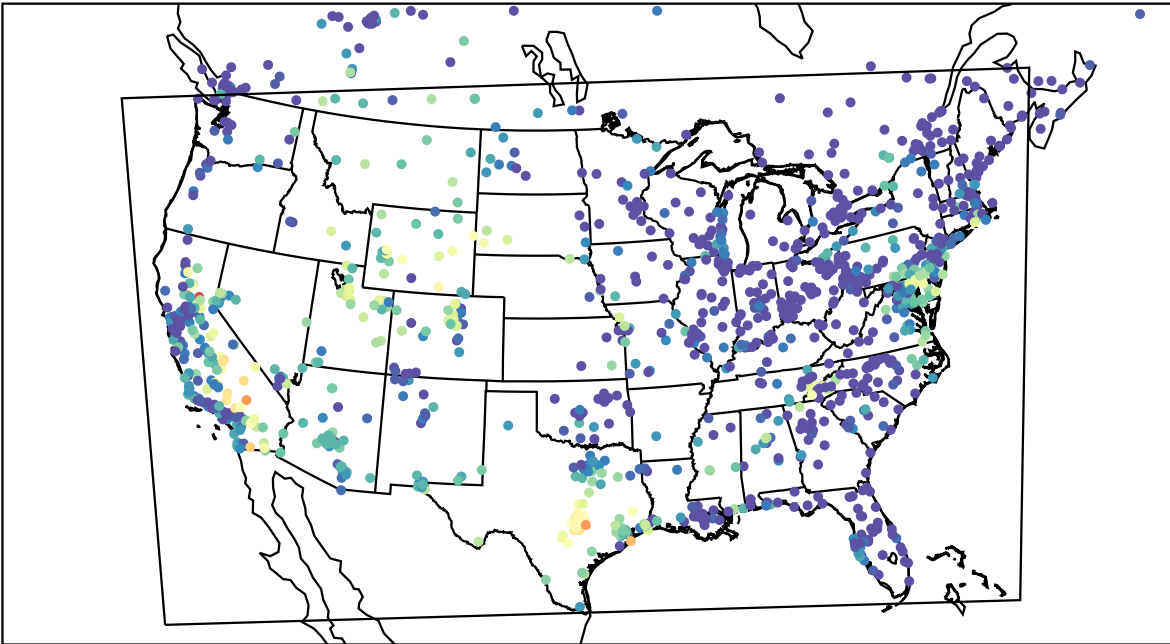
AirNOW (2023-09-13_05:00:00)
