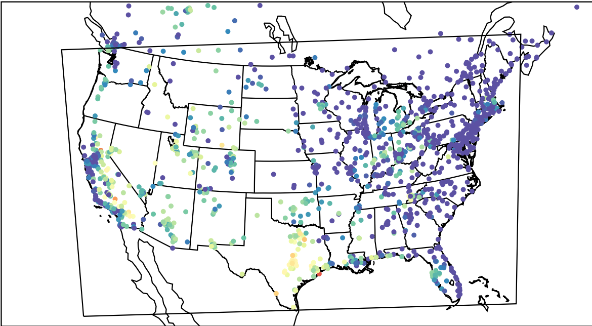
AirNOW (2023-09-12_04:00:00)
