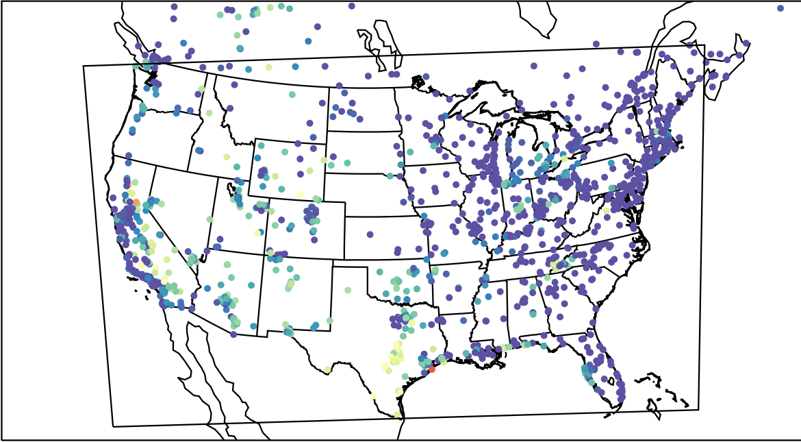
AirNOW (2023-09-12_07:00:00)
