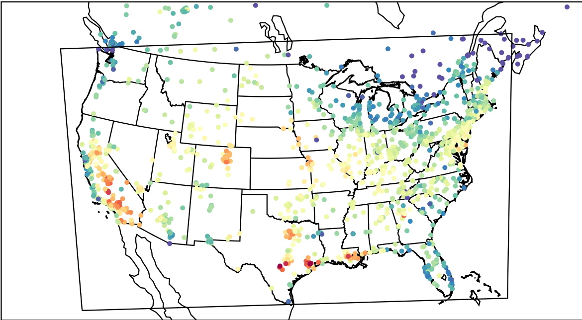
AirNOW (2023-09-13_21:00:00)
