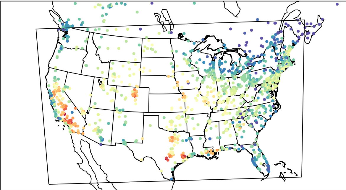
AirNOW (2023-09-13_22:00:00)
