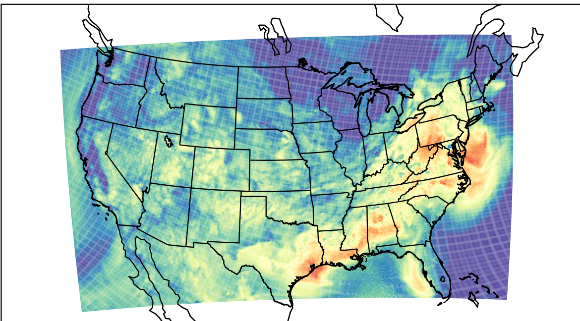
WRF (2023-09-12_15:00:00)
