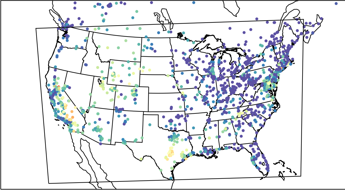
AirNOW (2023-09-13_04:00:00)
