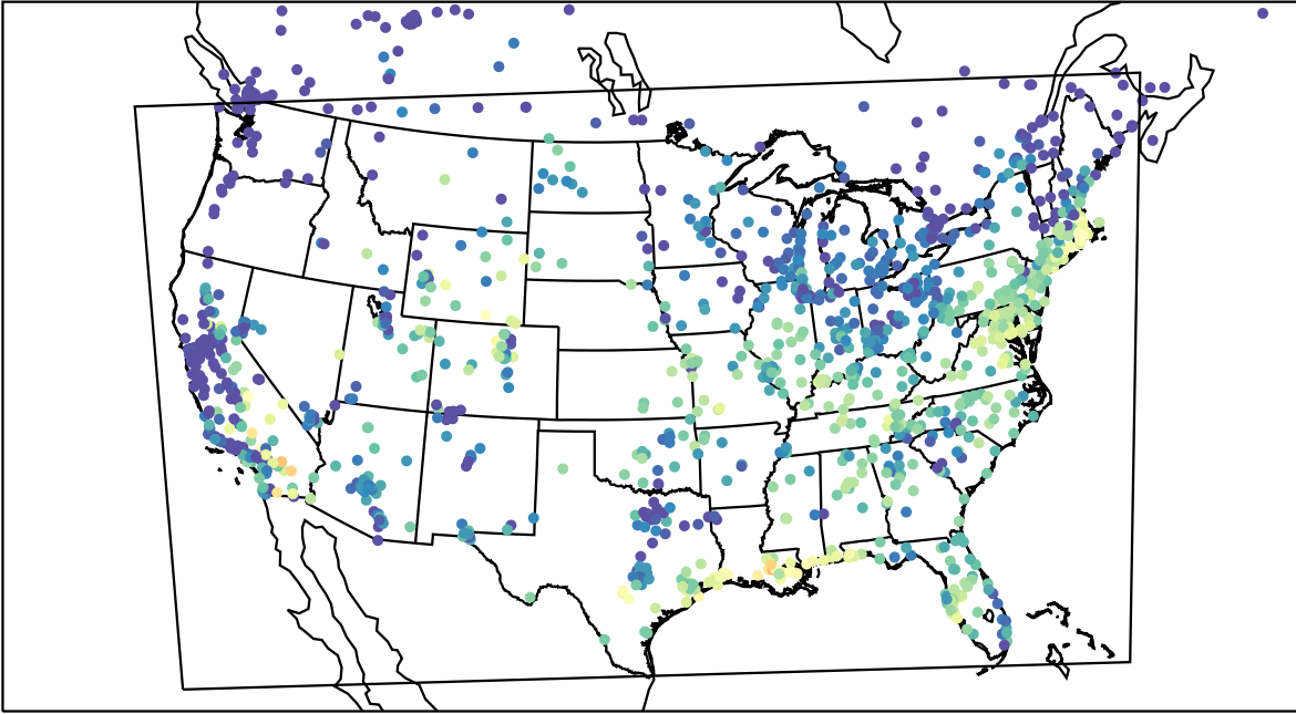
AirNOW (2023-09-13_15:00:00)
