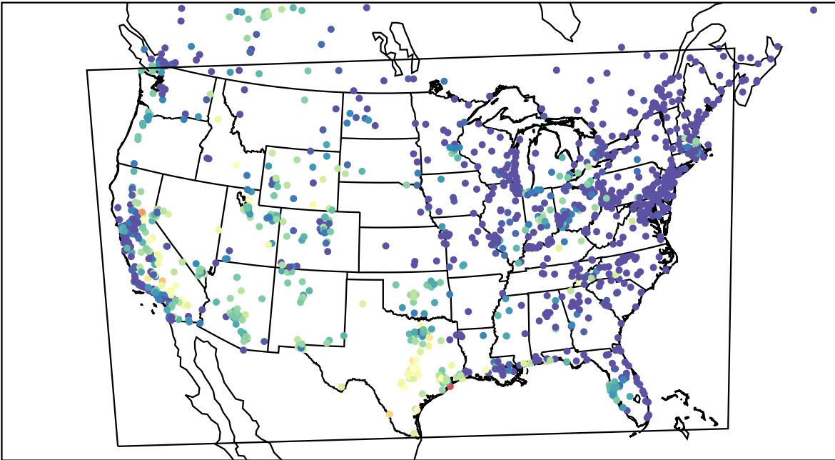
AirNOW (2023-09-12_05:00:00)
