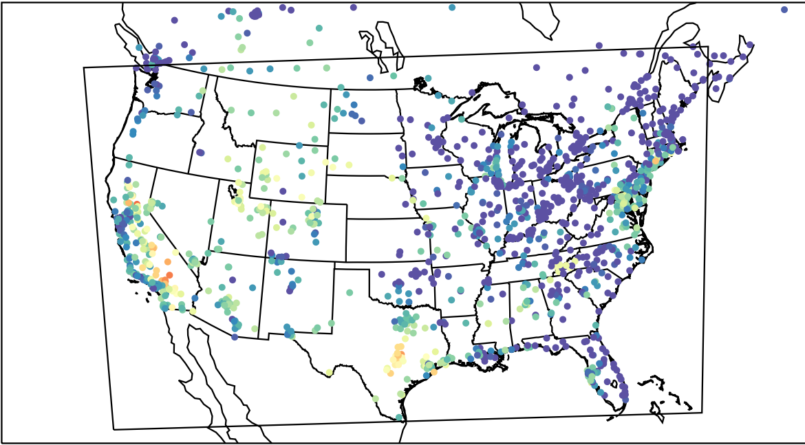
AirNOW (2023-09-13_03:00:00)
