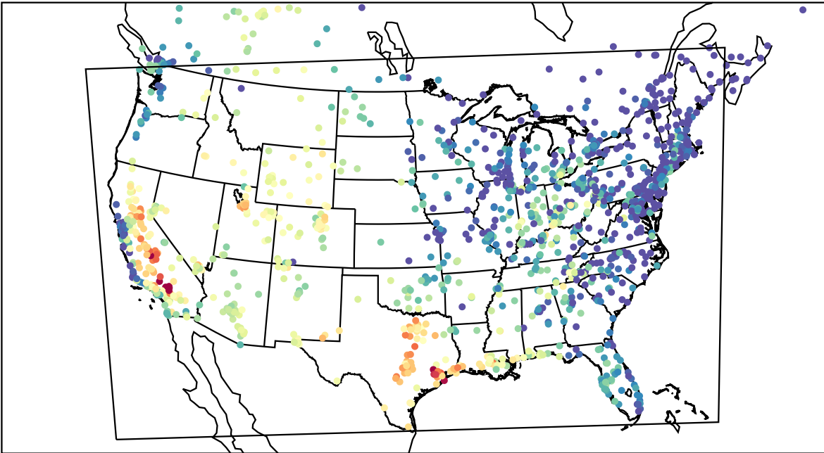
AirNOW (2023-09-12_00:00:00)
