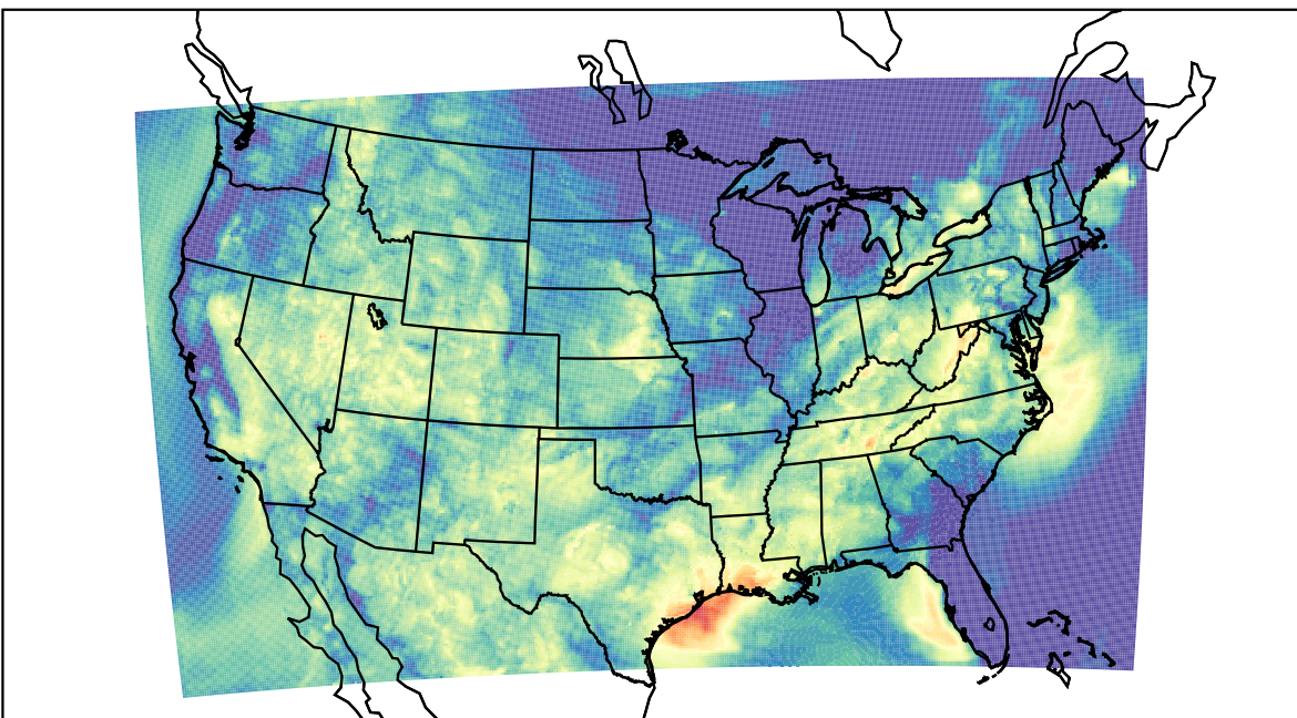
WRF (2023-09-12_09:00:00)
