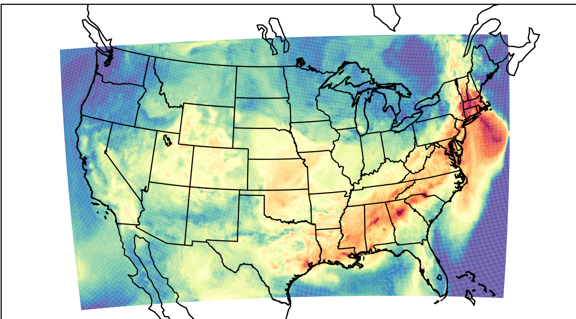
WRF (2023-09-13_17:00:00)
