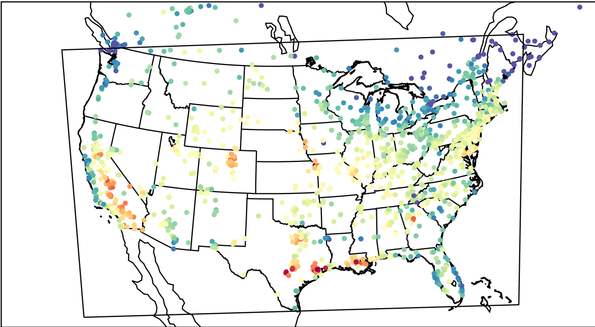
AirNOW (2023-09-13_20:00:00)
