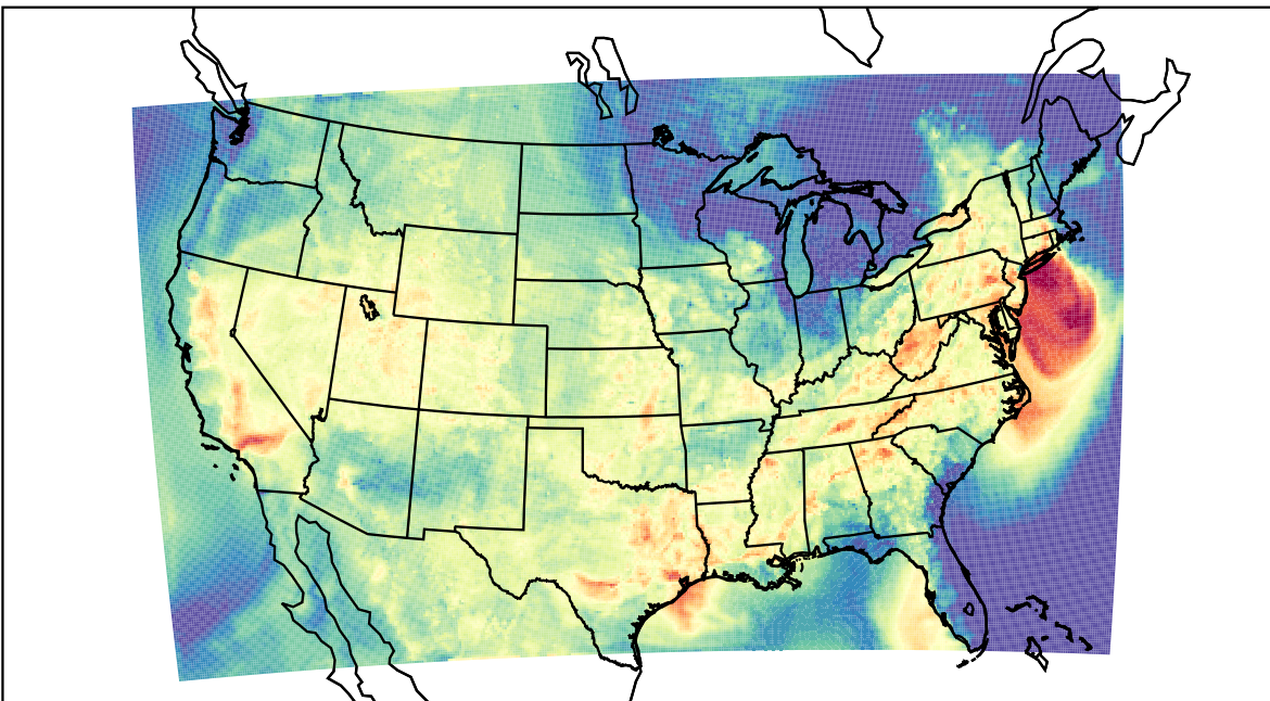
WRF (2023-09-13_01:00:00)
