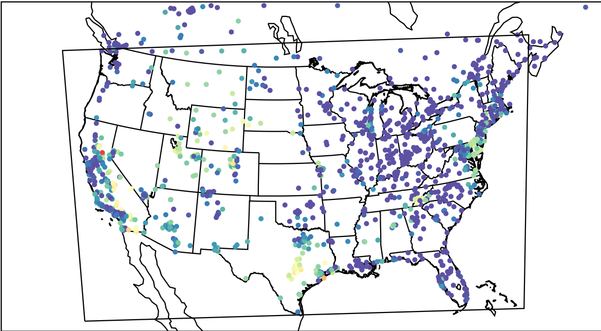
AirNOW (2023-09-13_06:00:00)
