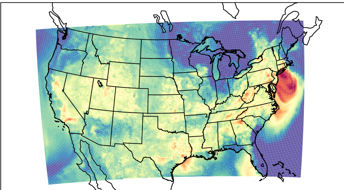
WRF (2023-09-13_02:00:00)
