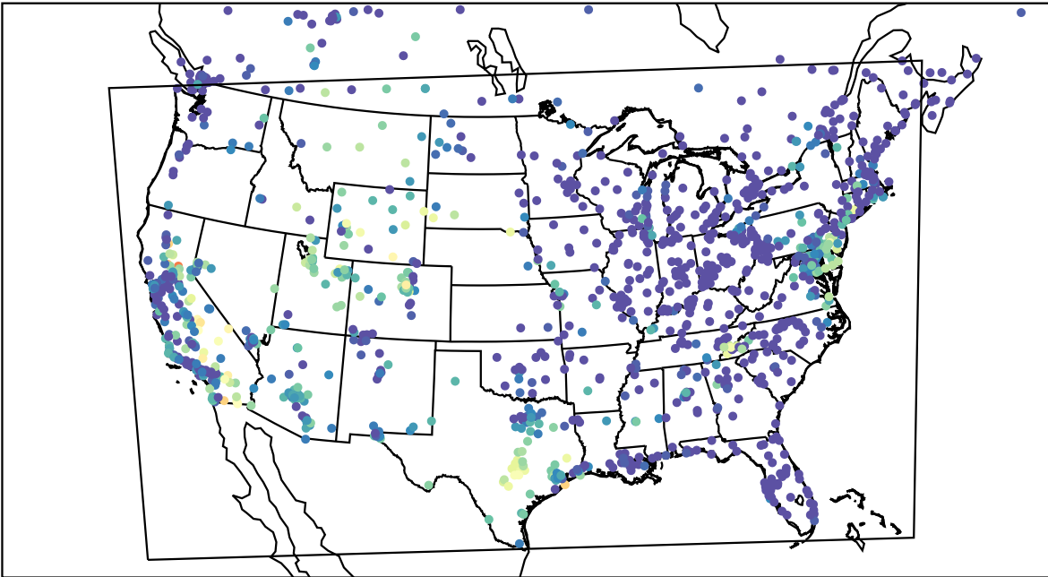
AirNOW (2023-09-13_07:00:00)
