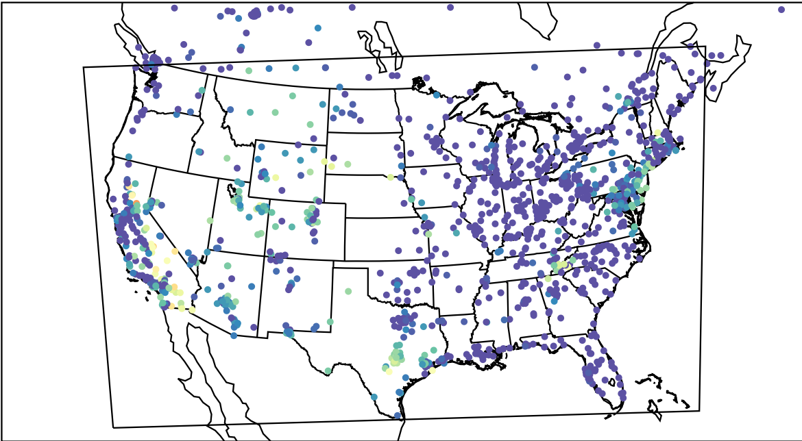
AirNOW (2023-09-13_09:00:00)
