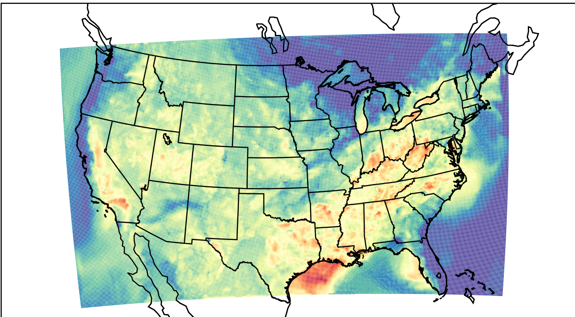
WRF (2023-09-12_02:00:00)
