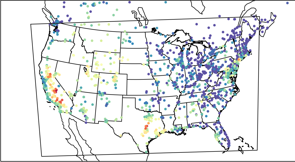
AirNOW (2023-09-13_01:00:00)
