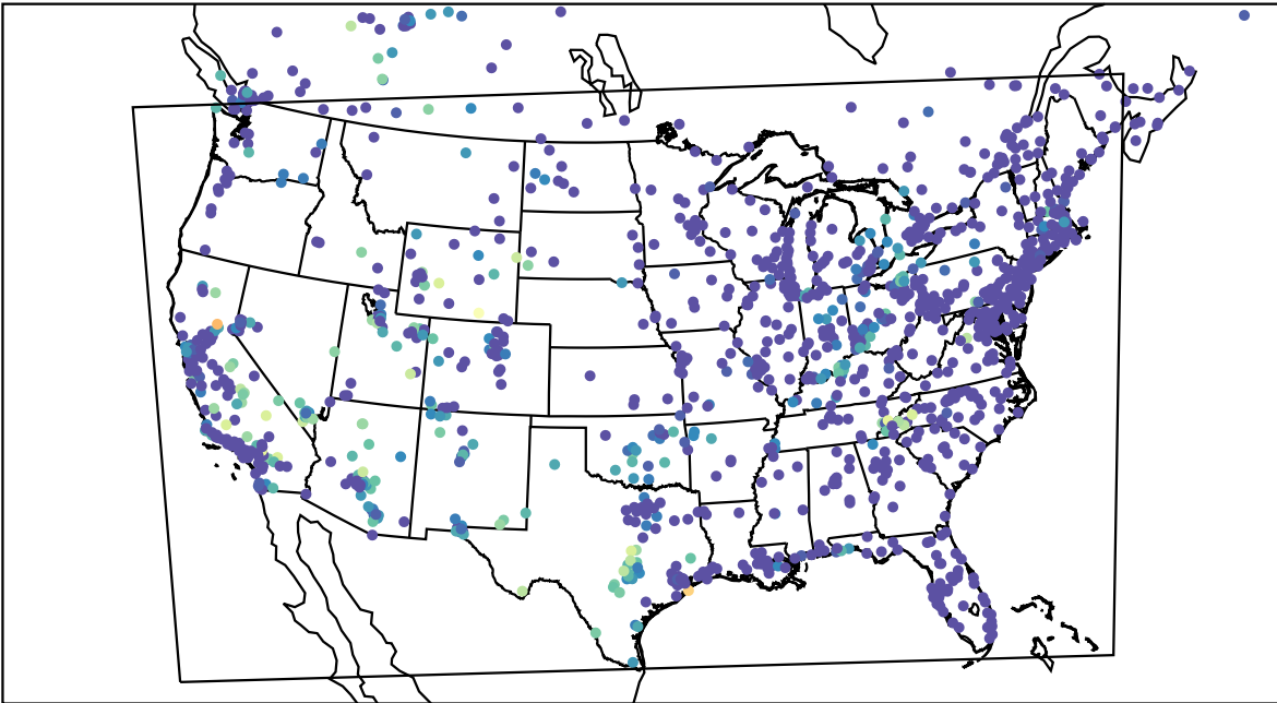
AirNOW (2023-09-12_12:00:00)
