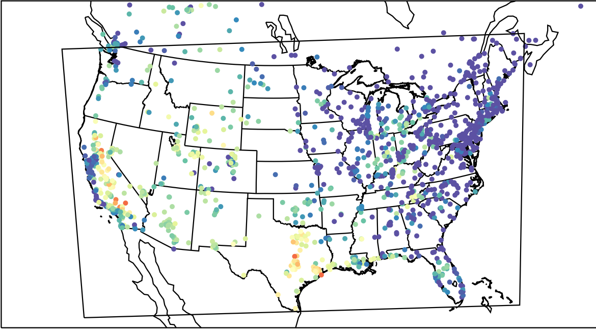
AirNOW (2023-09-12_02:00:00)
