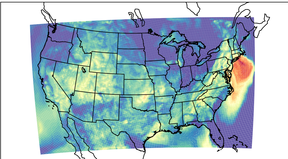
WRF (2023-09-13_11:00:00)
