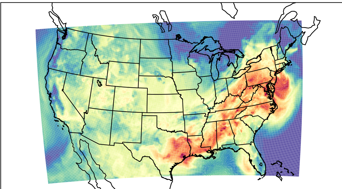
WRF (2023-09-12_17:00:00)
