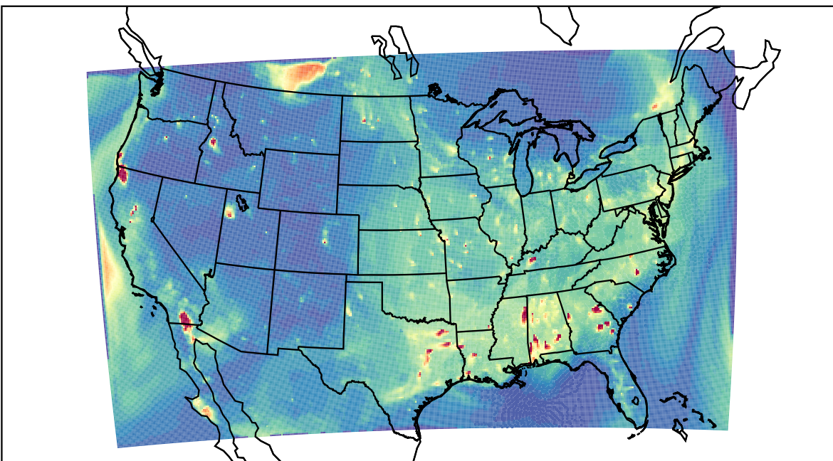
WRF 2023-09-14_02:00:00
