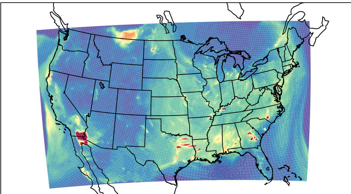
WRF 2023-09-14_06:00:00
