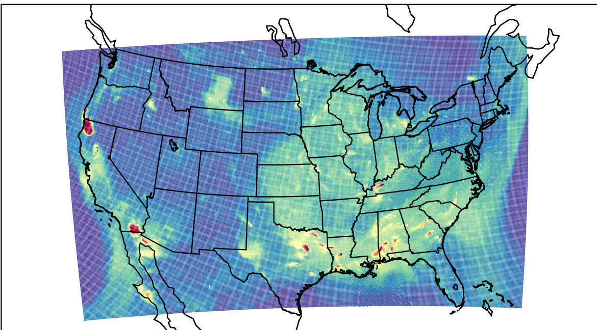
WRF 2023-09-15_04:00:00
