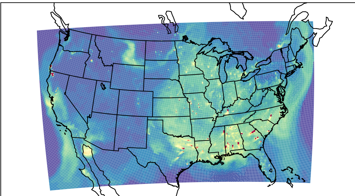
WRF 2023-09-15_00:00:00
