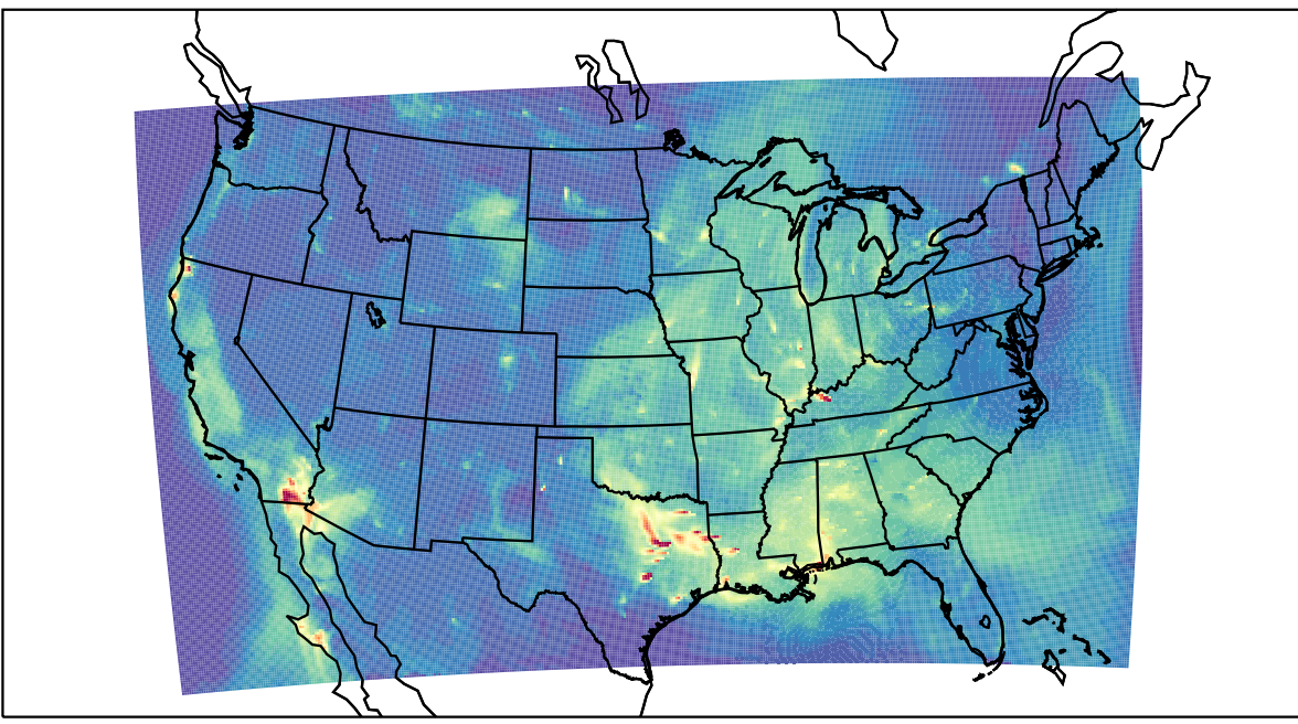
WRF 2023-09-15_14:00:00
