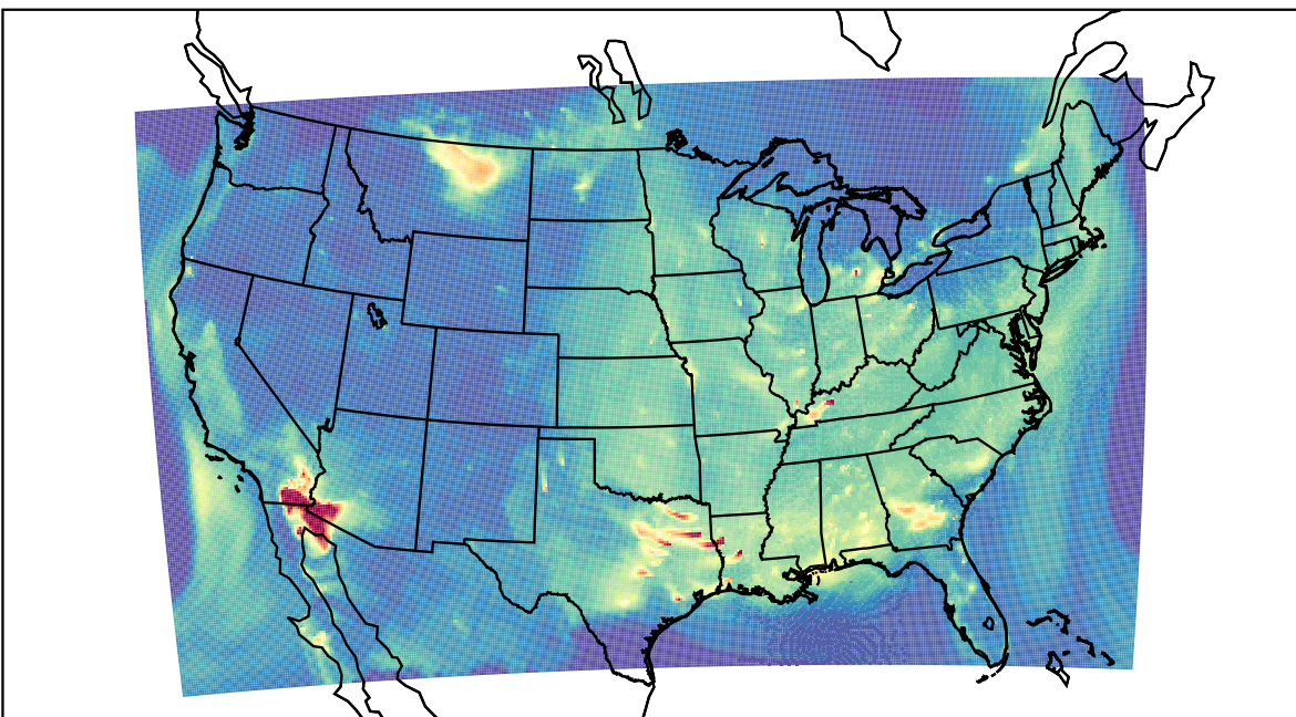
WRF 2023-09-14_12:00:00
