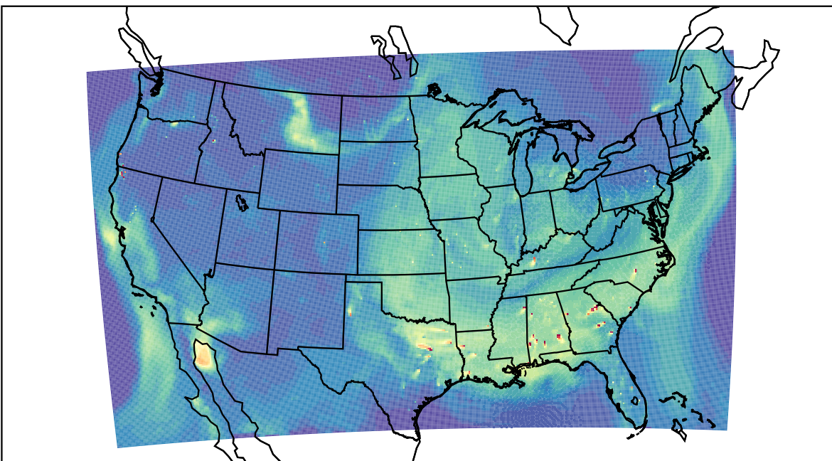
WRF 2023-09-14_21:00:00
