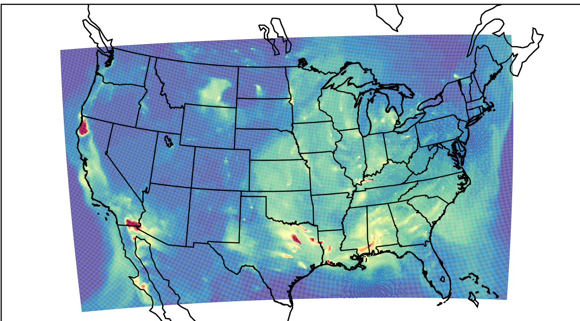
WRF 2023-09-15_07:00:00
