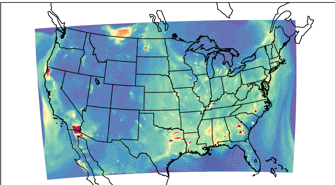
WRF 2023-09-14_05:00:00
