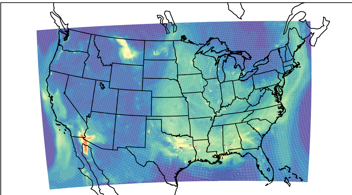
WRF 2023-09-14_17:00:00
