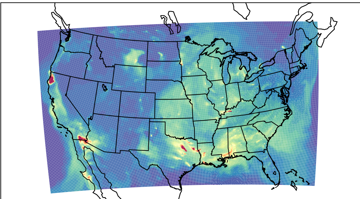
WRF 2023-09-15_08:00:00
