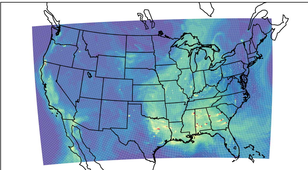
WRF 2023-09-15_21:00:00
