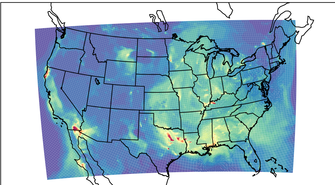
WRF 2023-09-15_11:00:00
