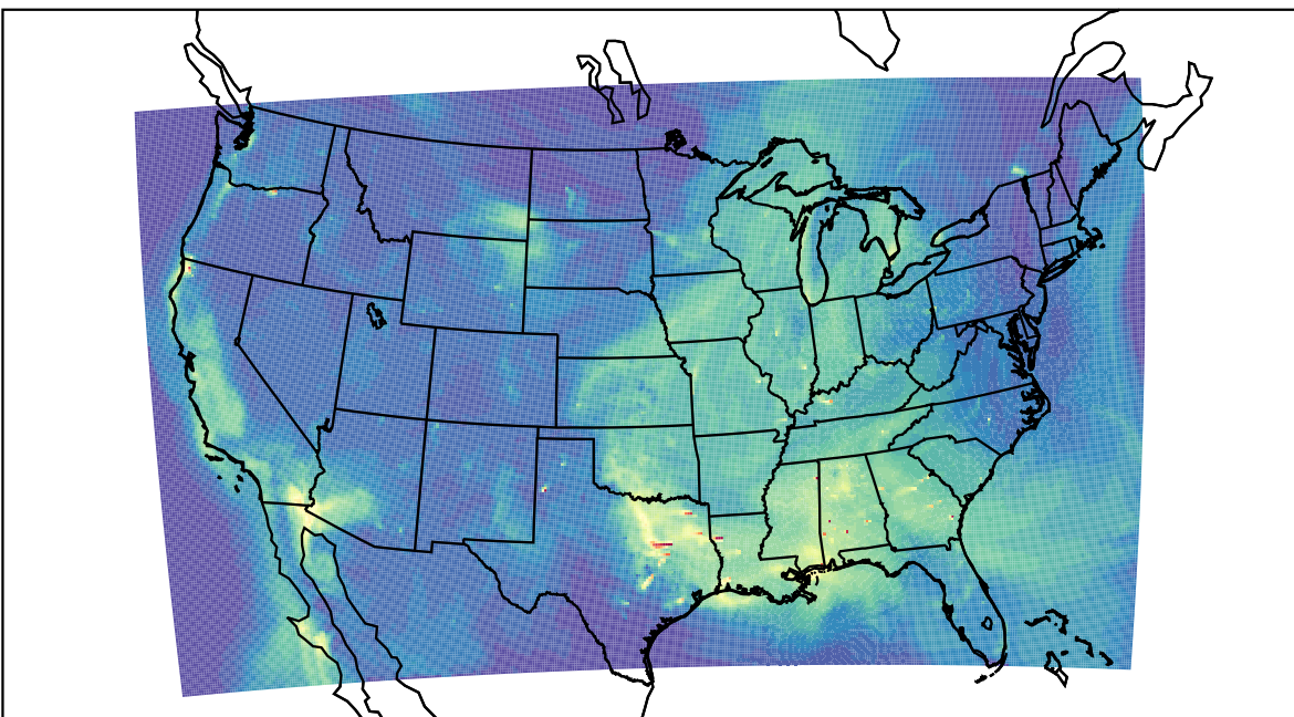
WRF 2023-09-15_17:00:00
