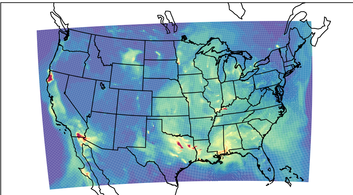
WRF 2023-09-15_09:00:00
