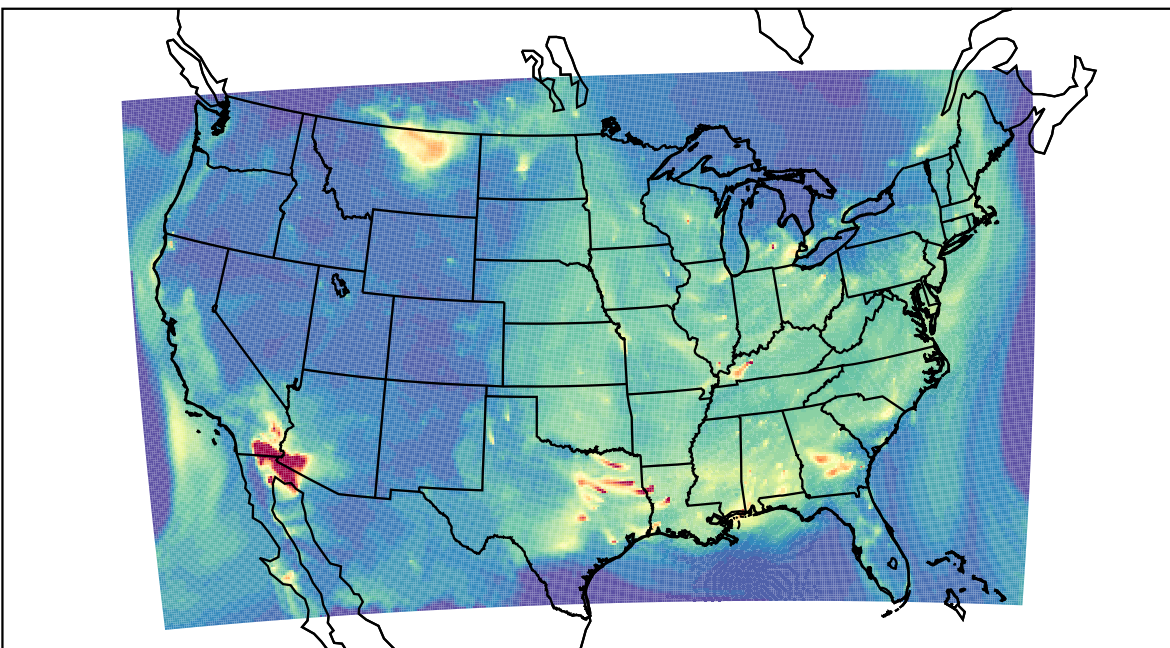
WRF 2023-09-14_11:00:00
