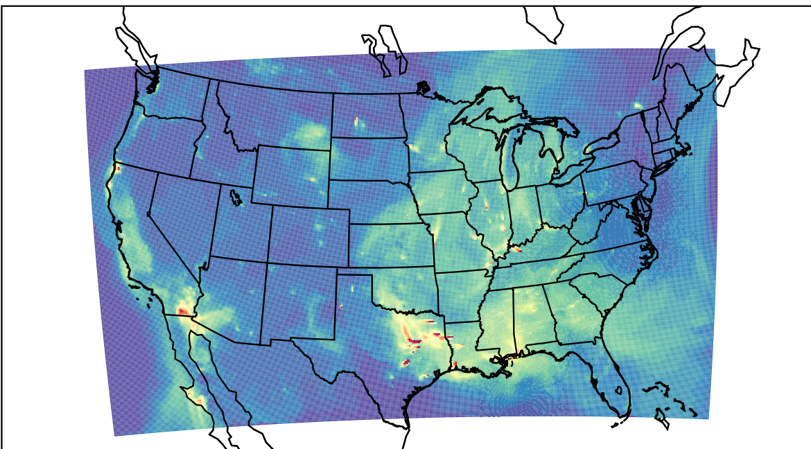
WRF 2023-09-15_15:00:00
