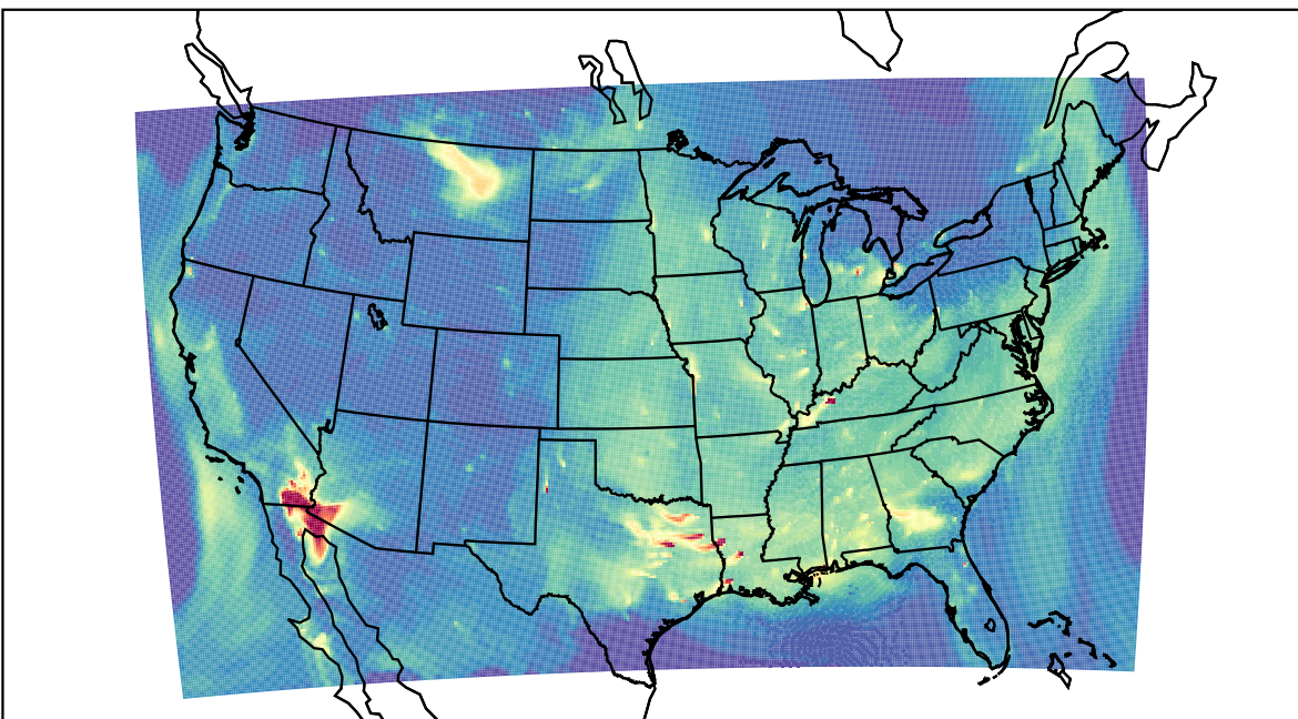
WRF 2023-09-14_14:00:00
