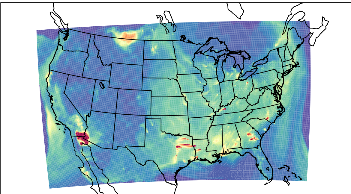
WRF 2023-09-14_07:00:00
