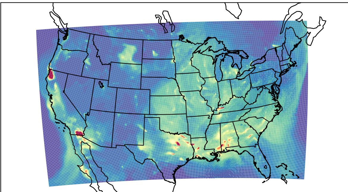
WRF 2023-09-15_05:00:00
