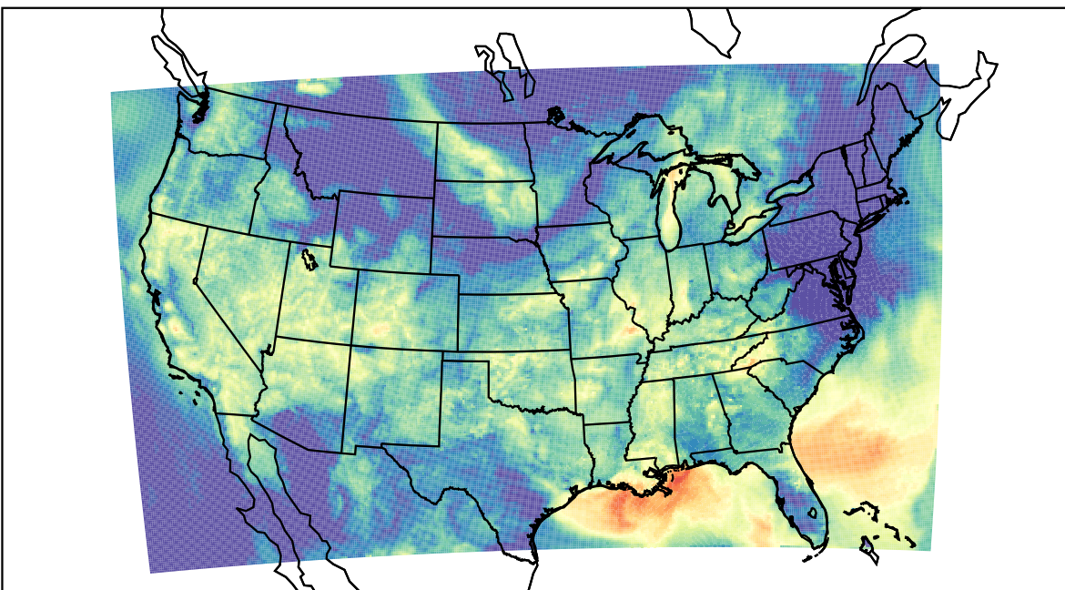
WRF (2023-09-16_09:00:00)
