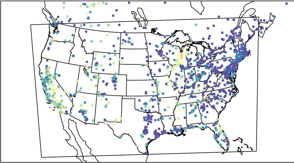
AirNOW (2023-09-16_04:00:00)
