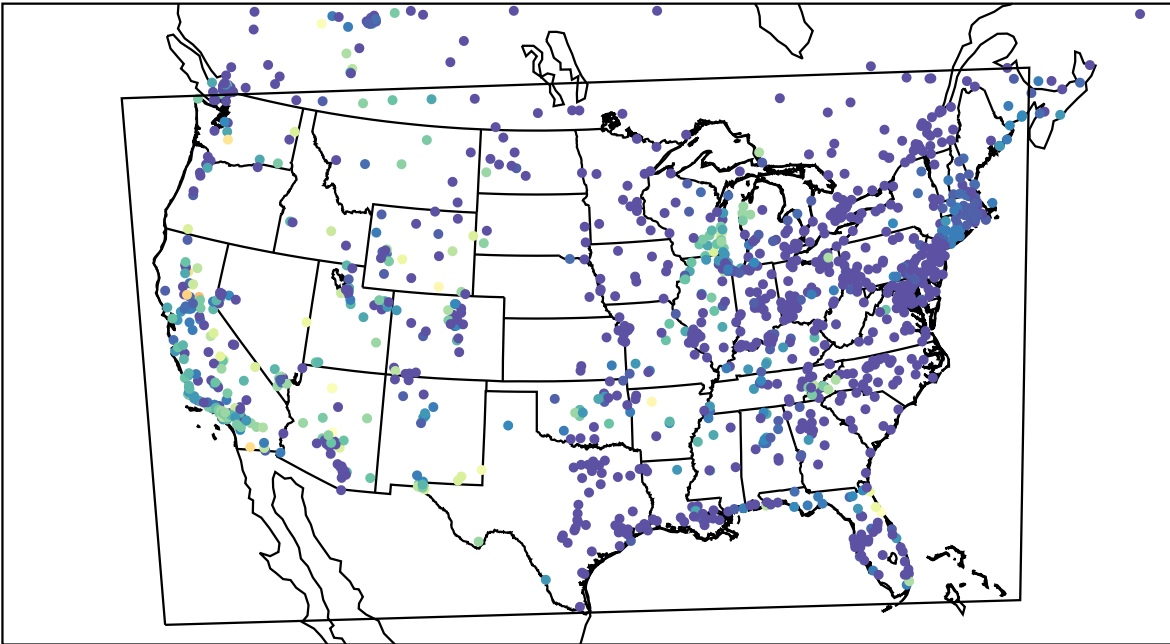
AirNOW (2023-09-16_11:00:00)
