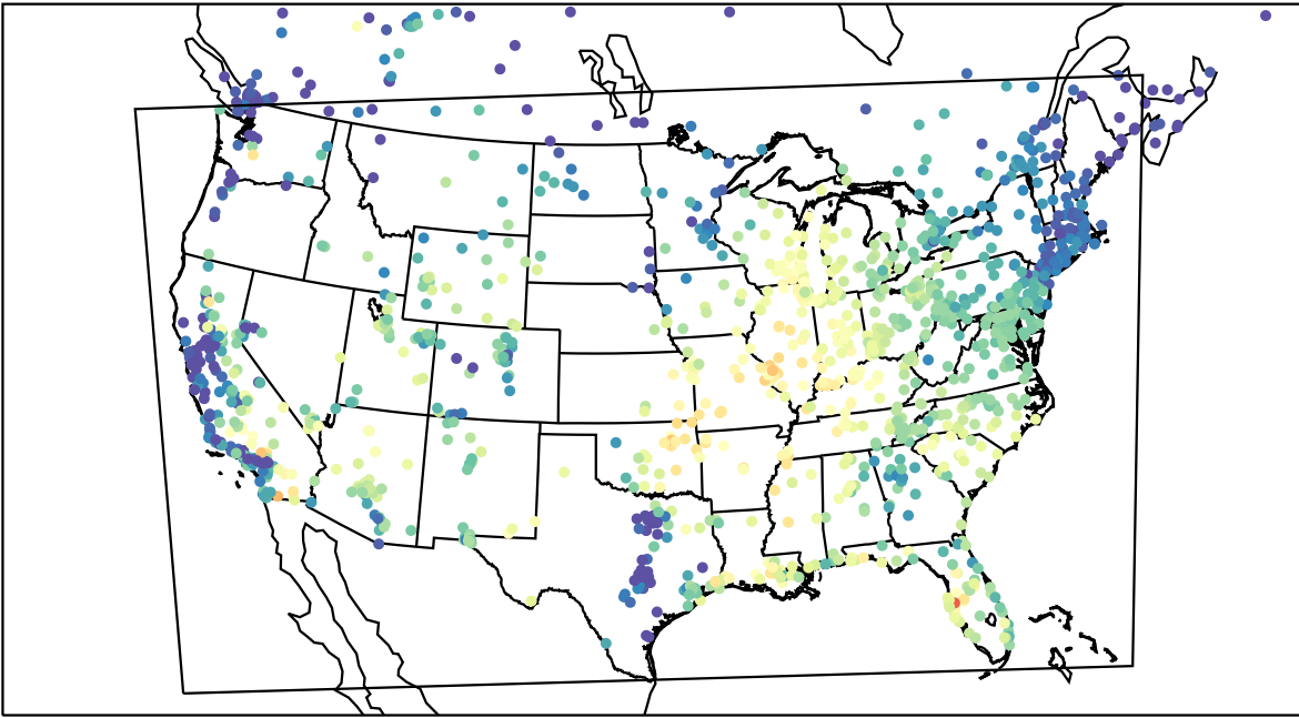
AirNOW (2023-09-15_16:00:00)
