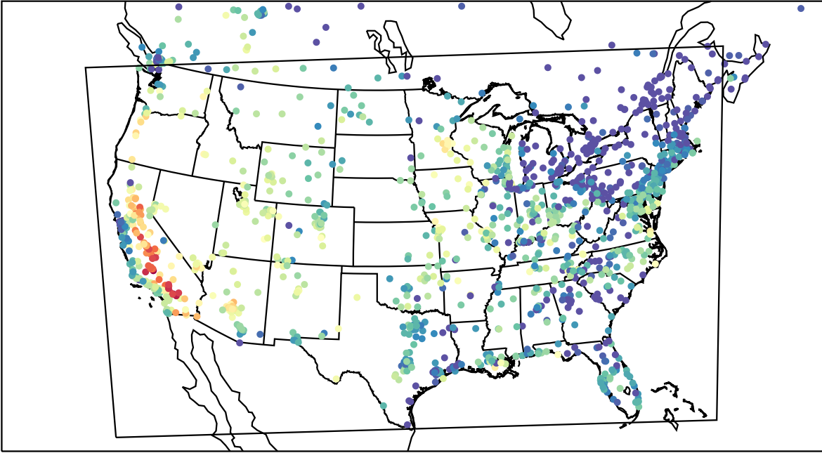
AirNOW (2023-09-15_01:00:00)
