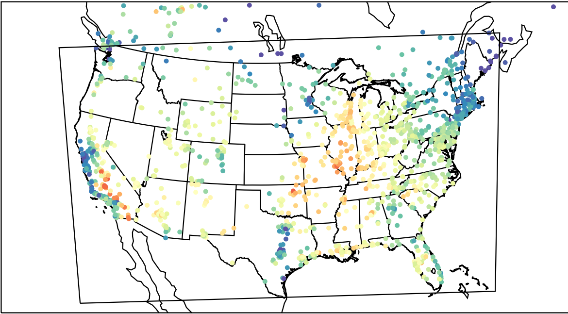
AirNOW (2023-09-15_18:00:00)
