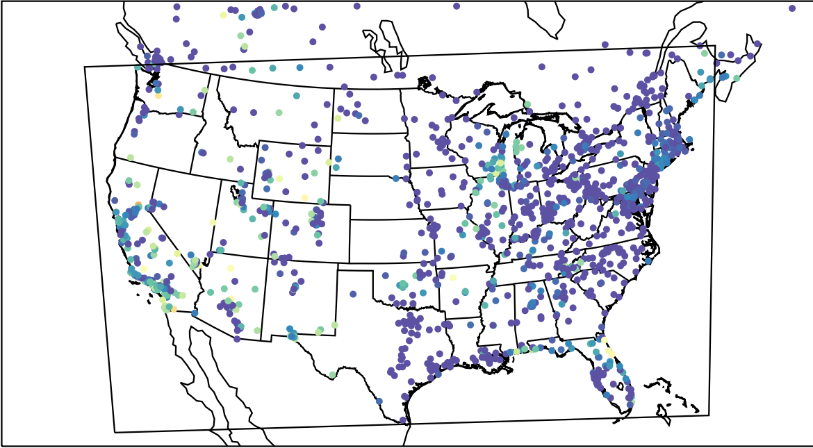
AirNOW (2023-09-16_12:00:00)
