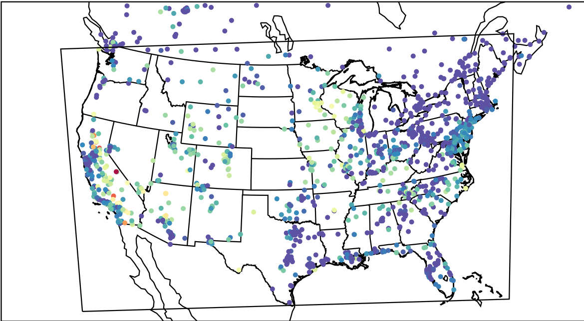
AirNOW (2023-09-15_05:00:00)
