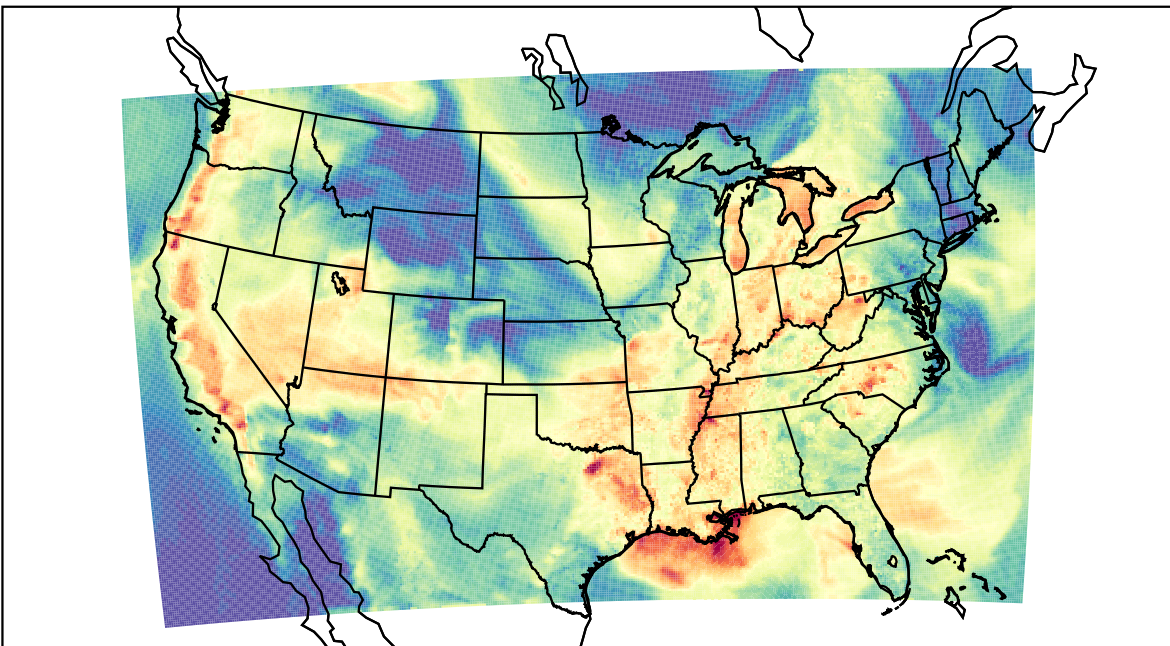
WRF (2023-09-16_23:00:00)
