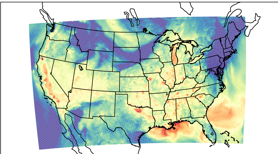
WRF (2023-09-16_01:00:00)
