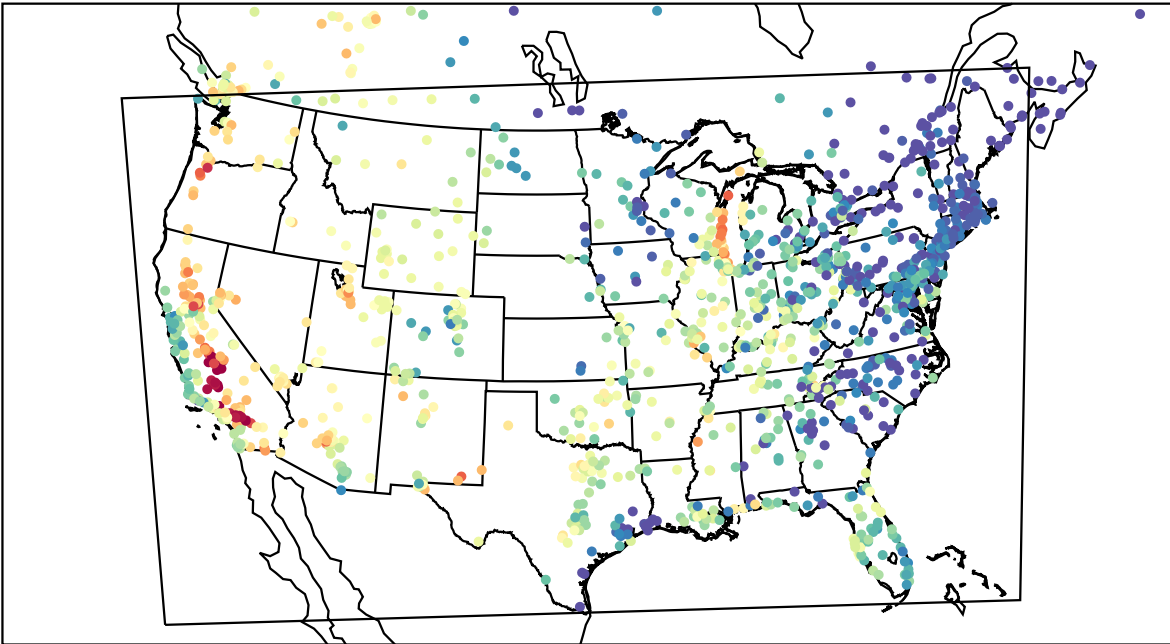
AirNOW (2023-09-16_00:00:00)
