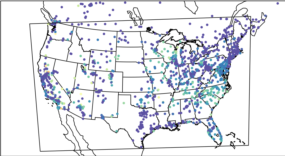
AirNOW (2023-09-15_13:00:00)
