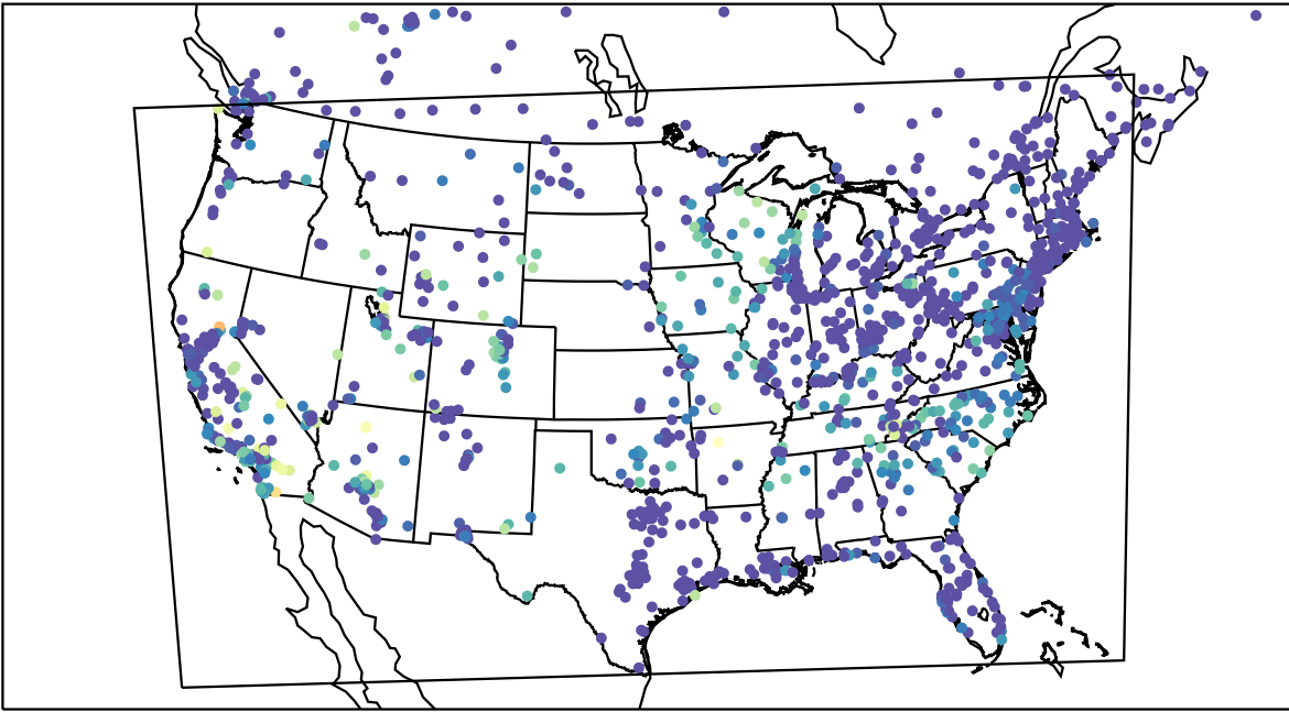
AirNOW (2023-09-15_12:00:00)
