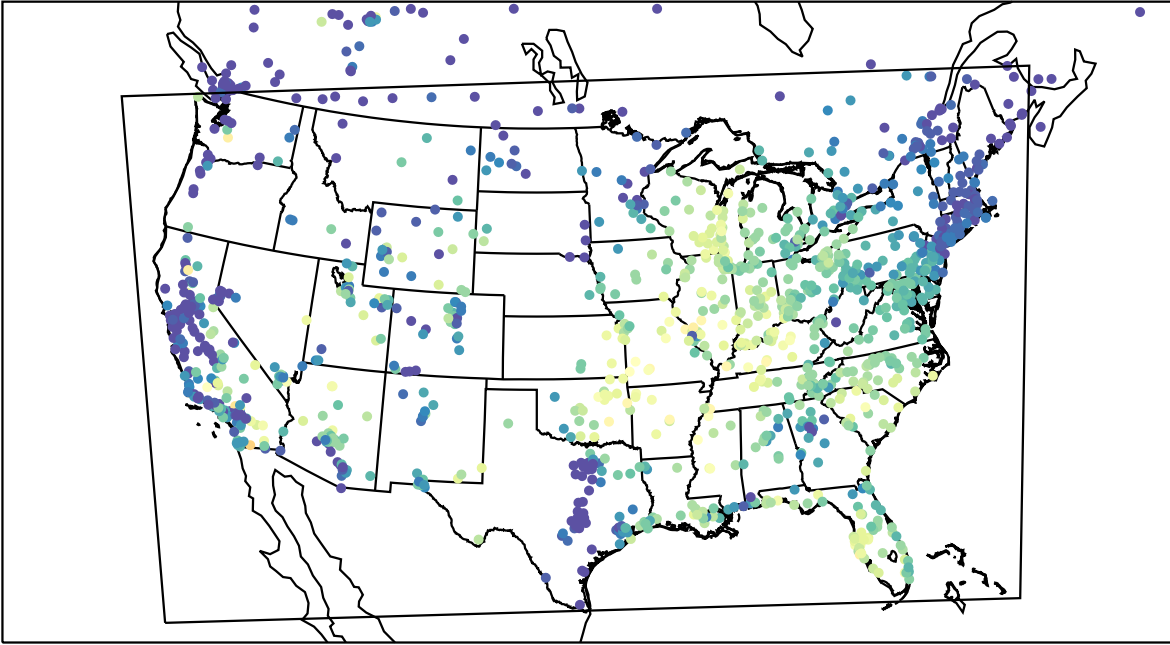
AirNOW (2023-09-15_15:00:00)
