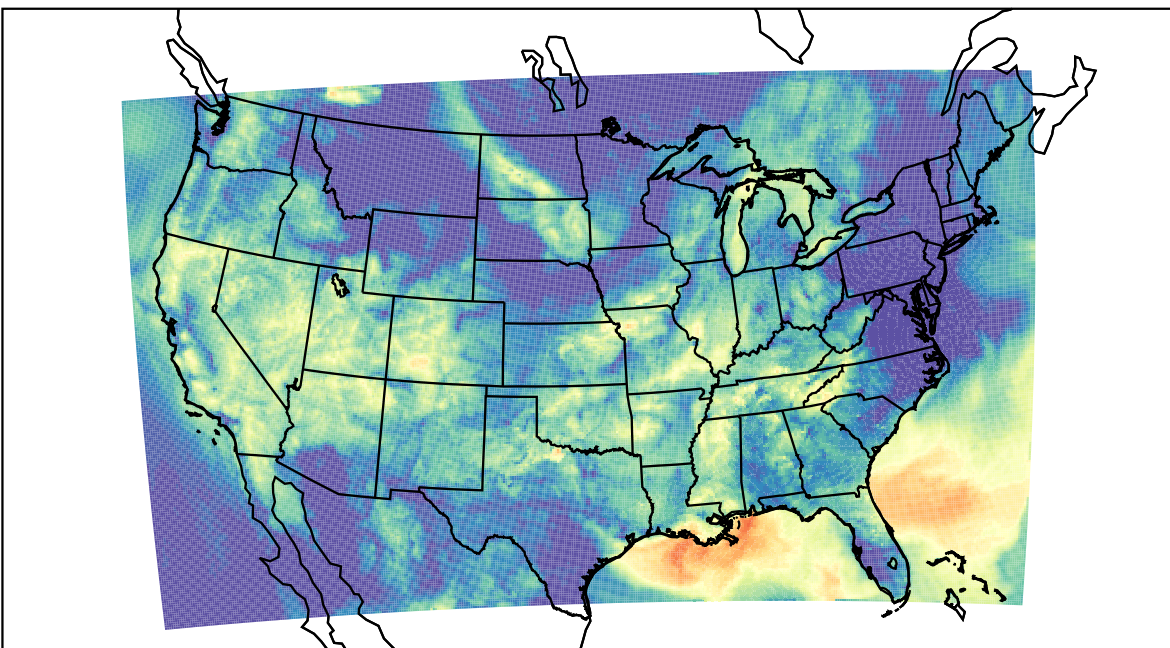
WRF (2023-09-16_12:00:00)
