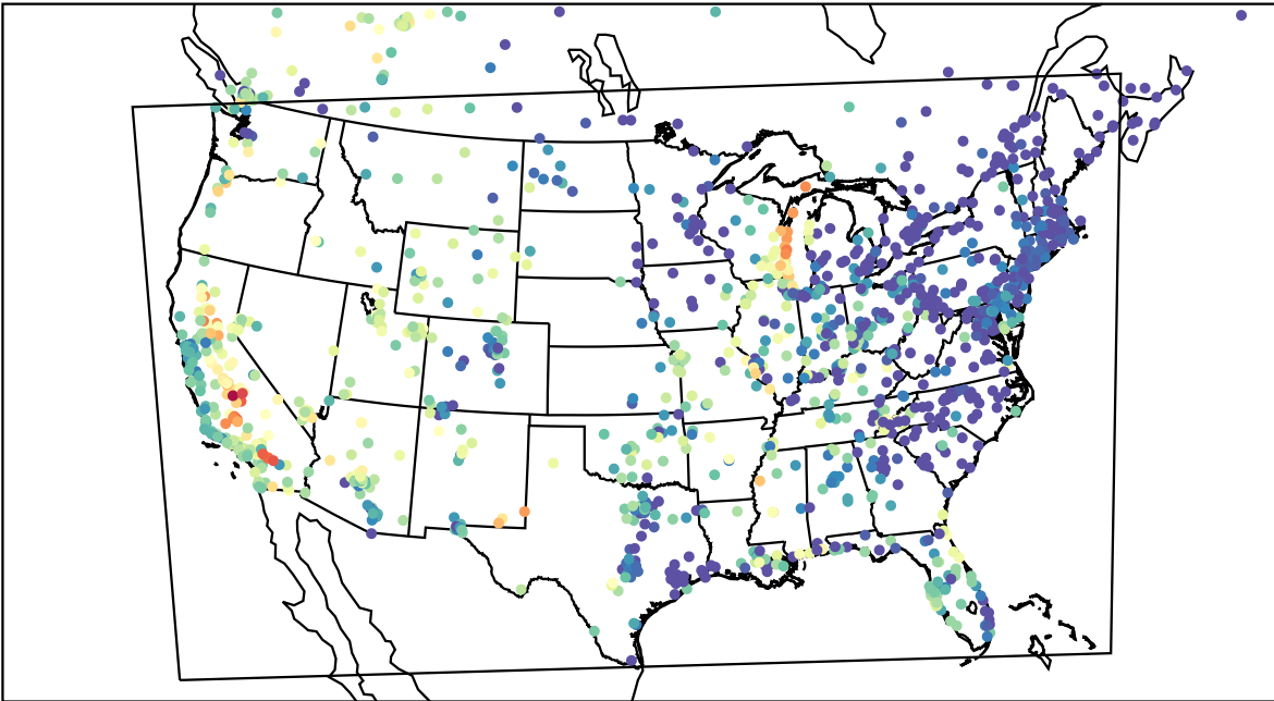
AirNOW (2023-09-16_02:00:00)
