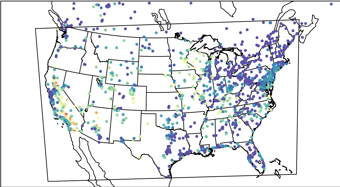
AirNOW (2023-09-15_04:00:00)
