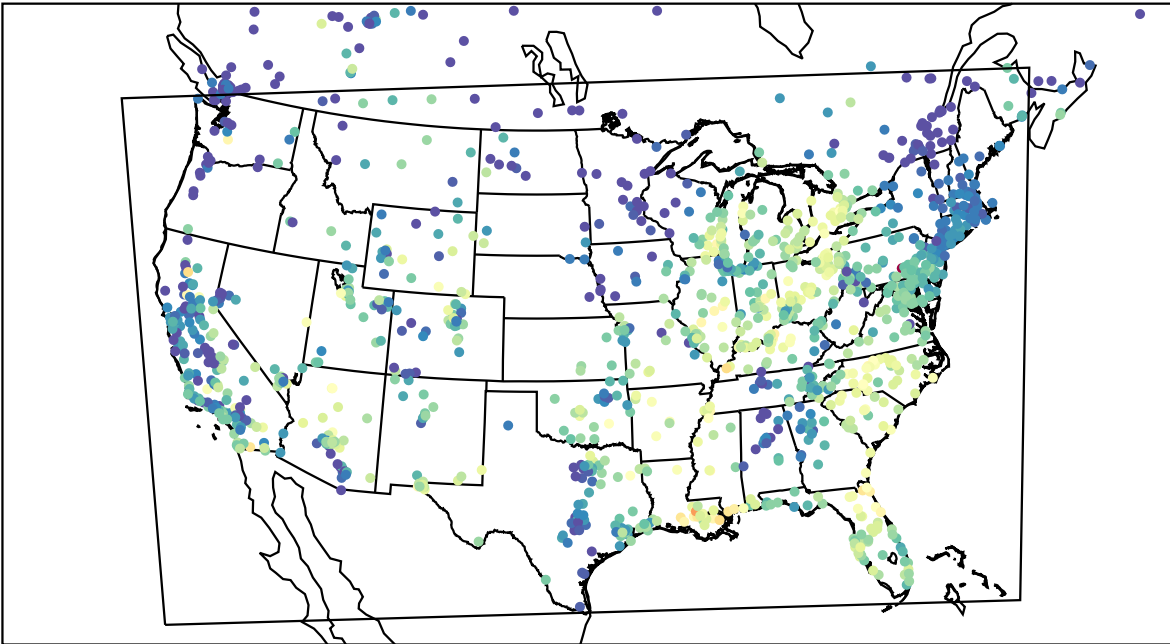
AirNOW (2023-09-16_15:00:00)
