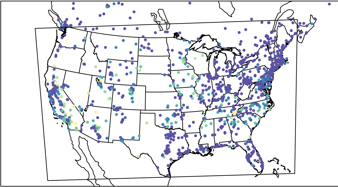
AirNOW (2023-09-15_10:00:00)
