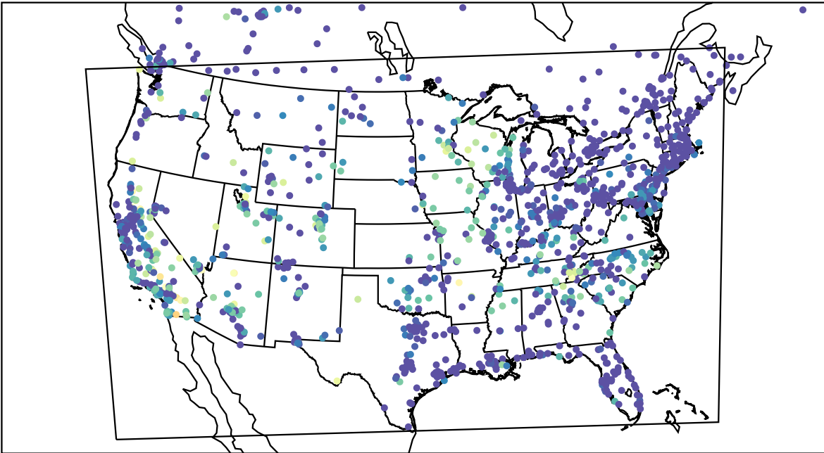
AirNOW (2023-09-15_09:00:00)
