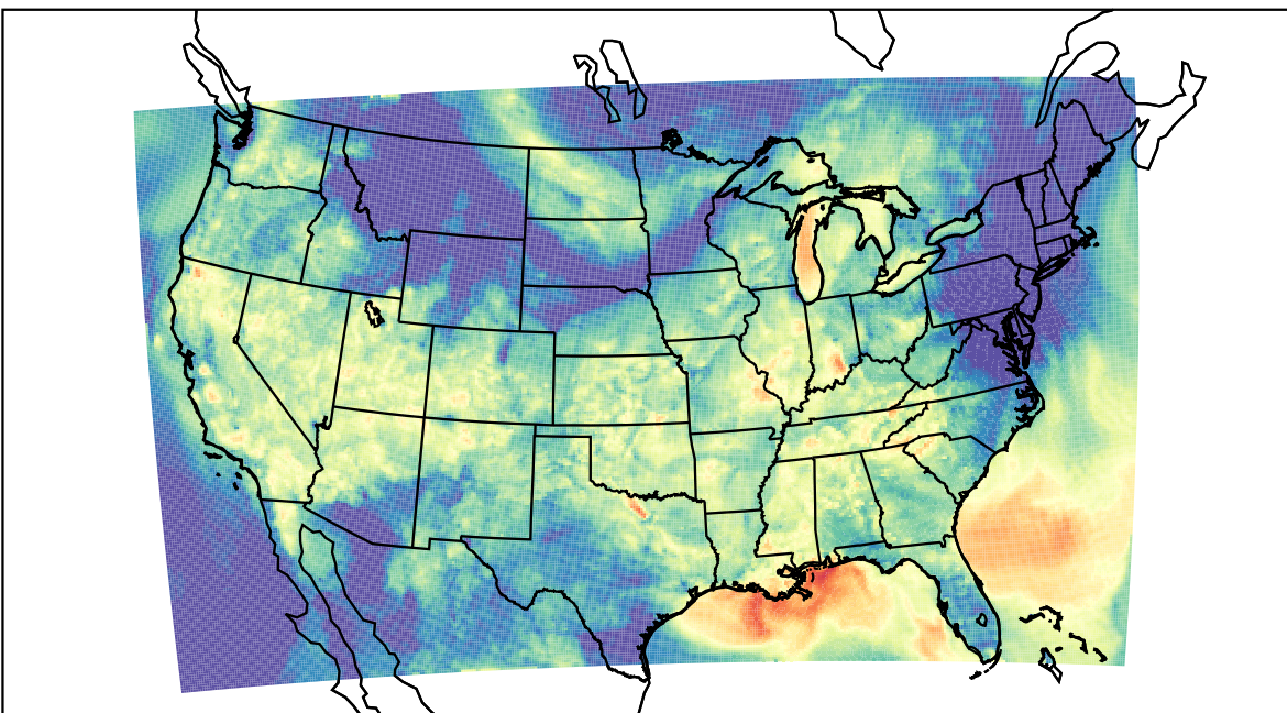
WRF (2023-09-16_05:00:00)
