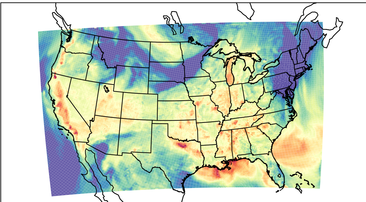
WRF (2023-09-16_00:00:00)
