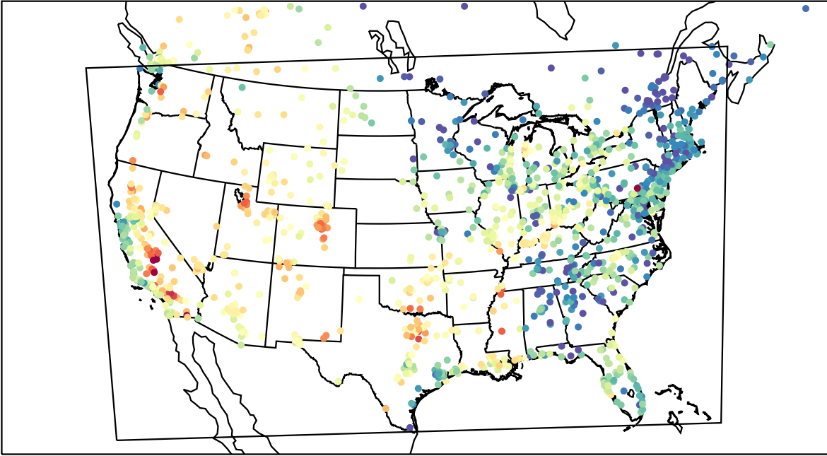
AirNOW (2023-09-16_23:00:00)
