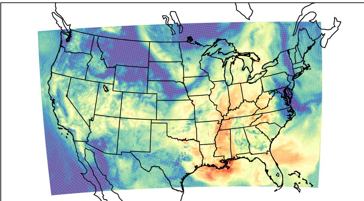
WRF (2023-09-16_16:00:00)
