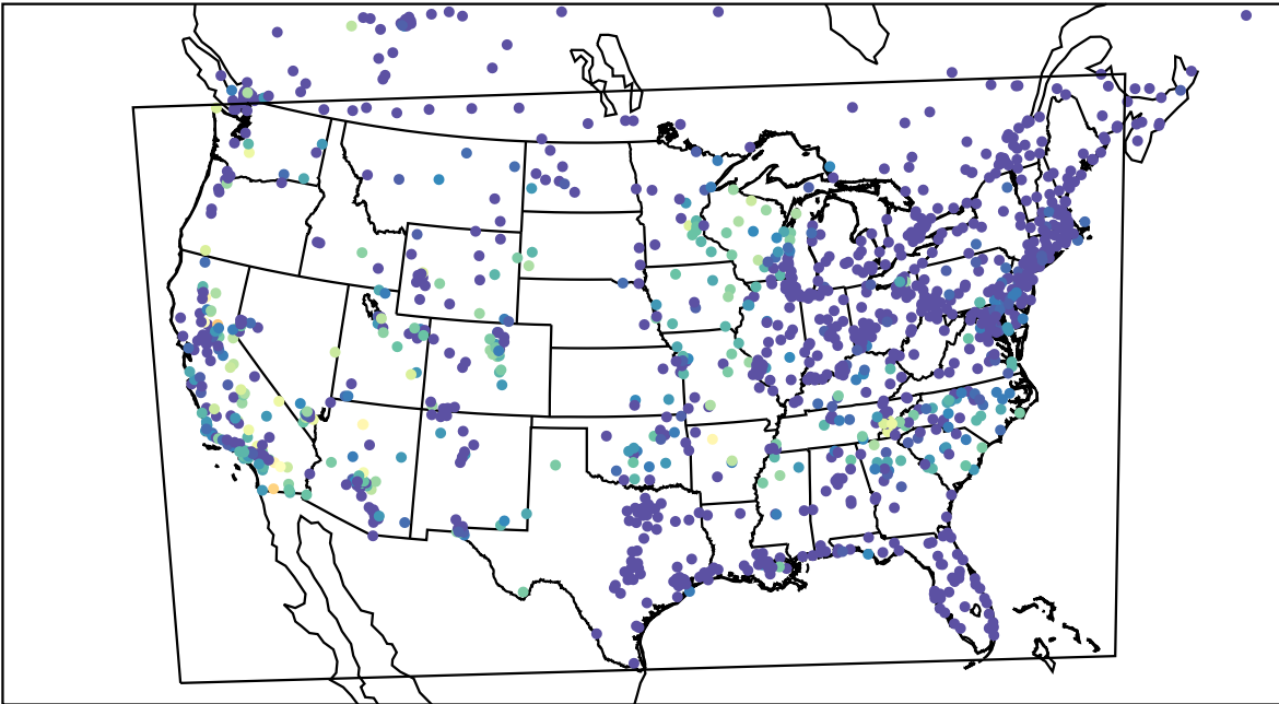
AirNOW (2023-09-15_11:00:00)
