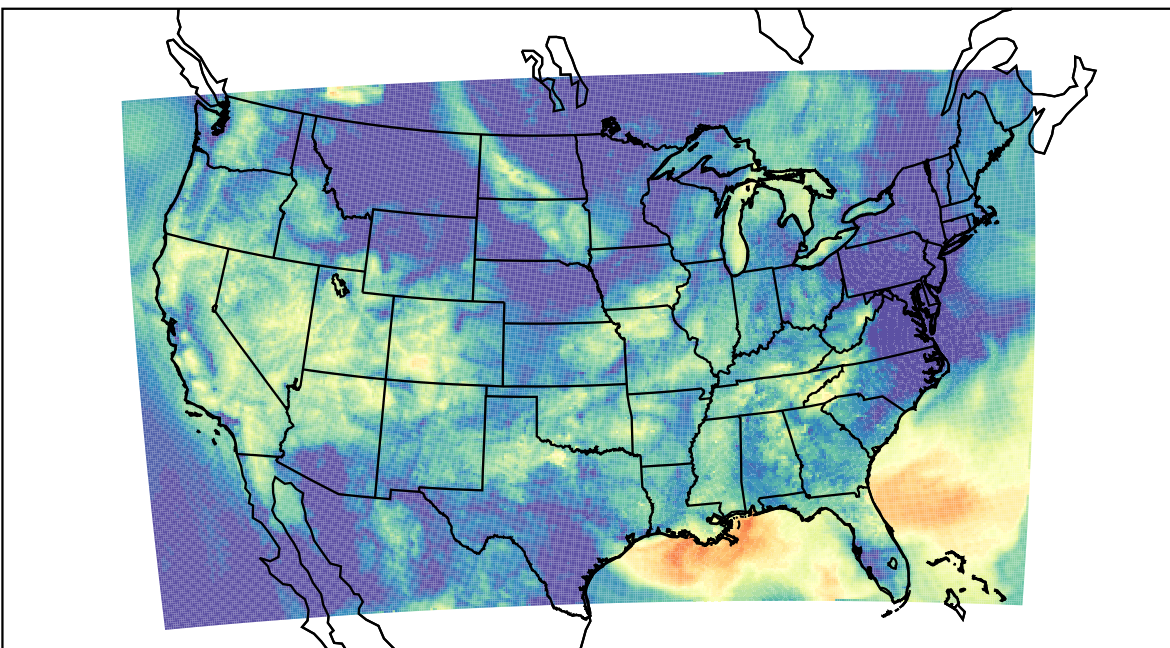
WRF (2023-09-16_13:00:00)
