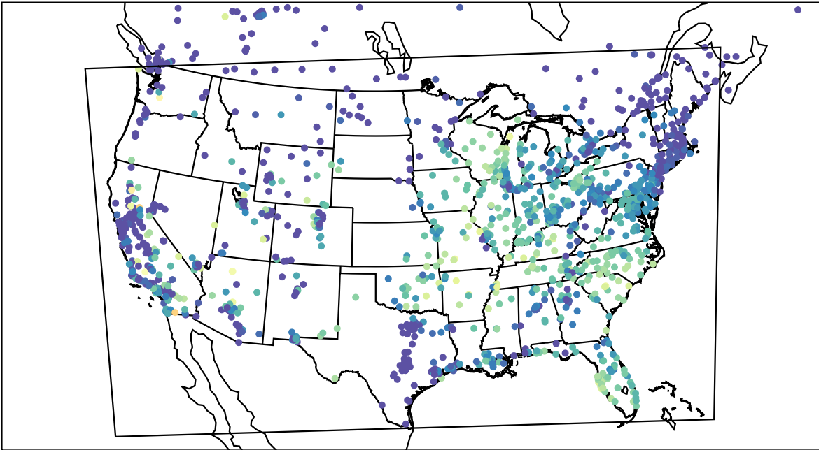
AirNOW (2023-09-15_14:00:00)
