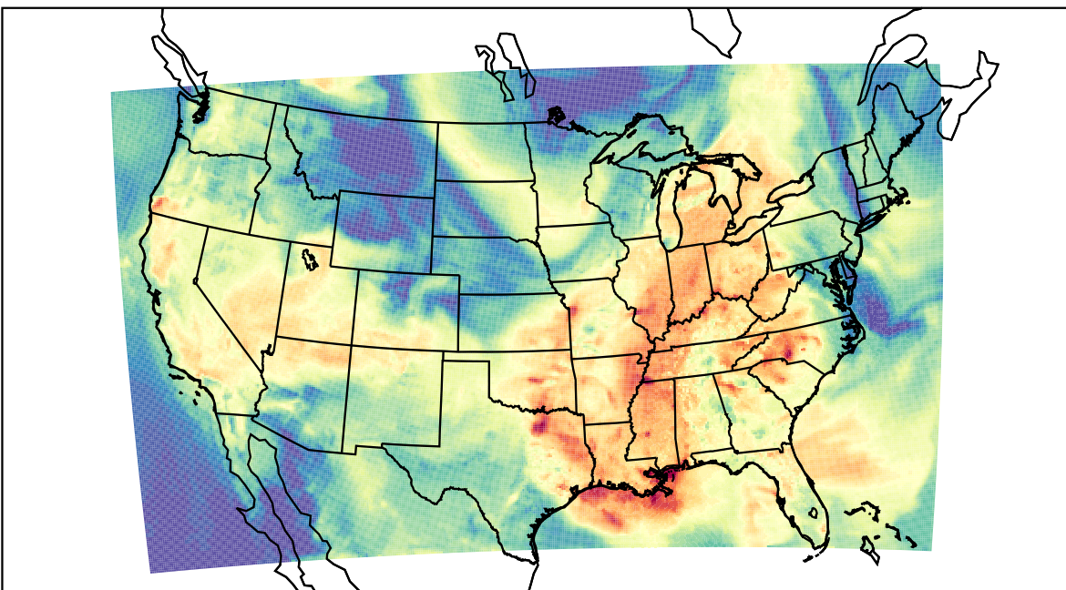
WRF (2023-09-16_19:00:00)
