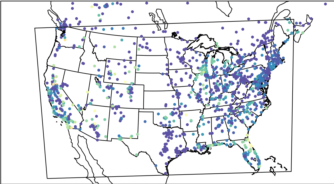
AirNOW (2023-09-16_13:00:00)
