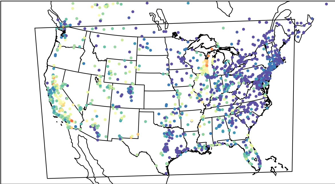
AirNOW (2023-09-16_03:00:00)
