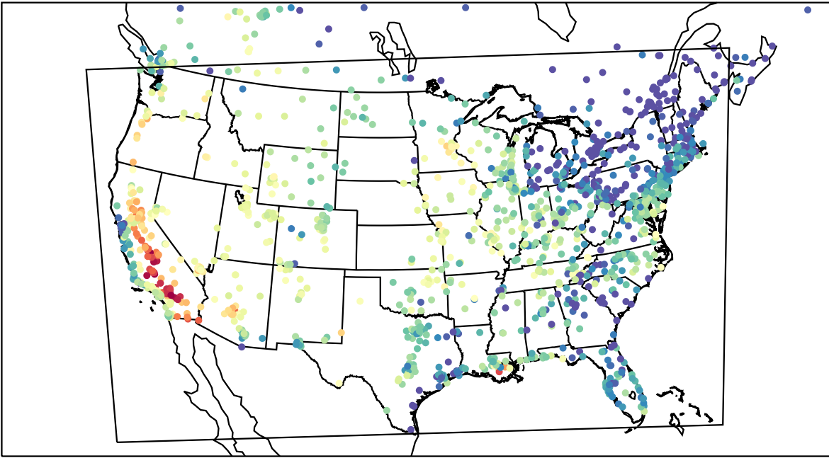
AirNOW (2023-09-15_00:00:00)
