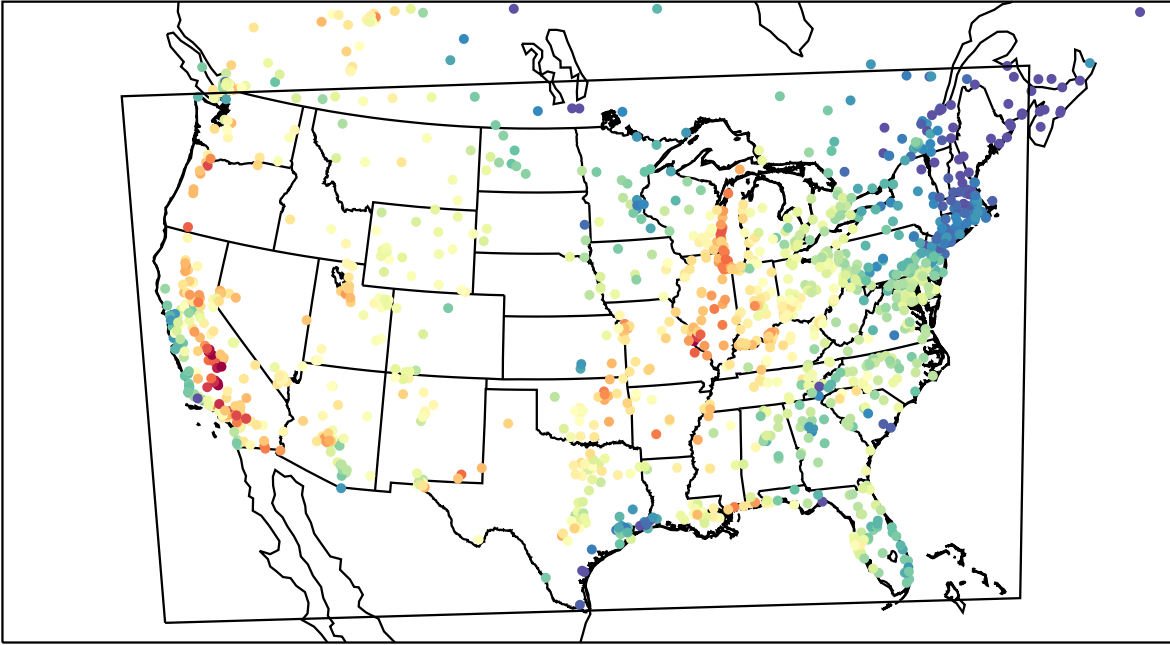
AirNOW (2023-09-15_22:00:00)
