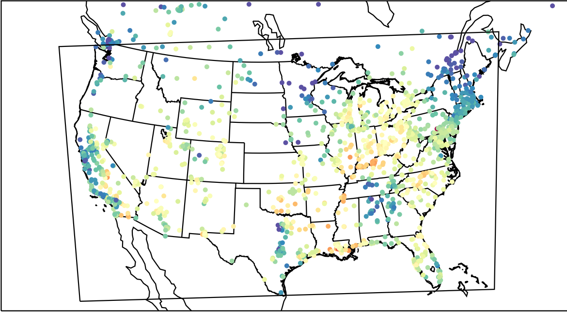
AirNOW (2023-09-16_17:00:00)
