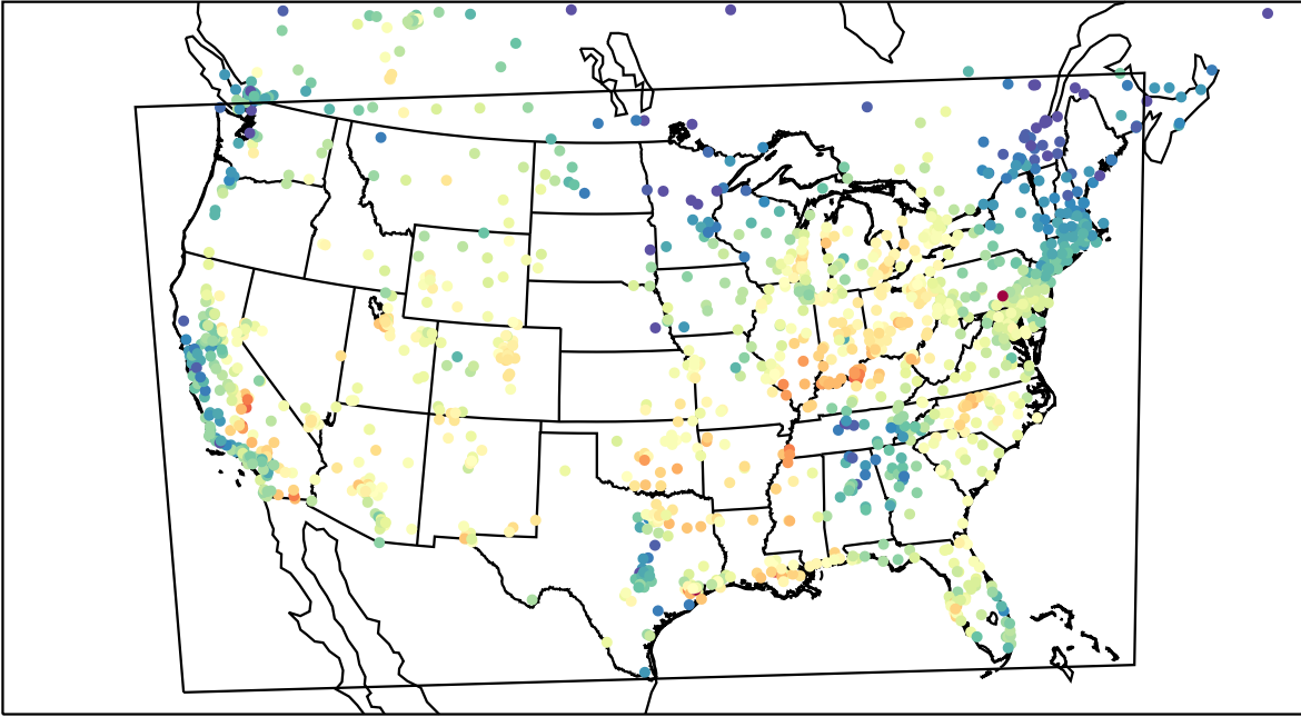
AirNOW (2023-09-16_18:00:00)
