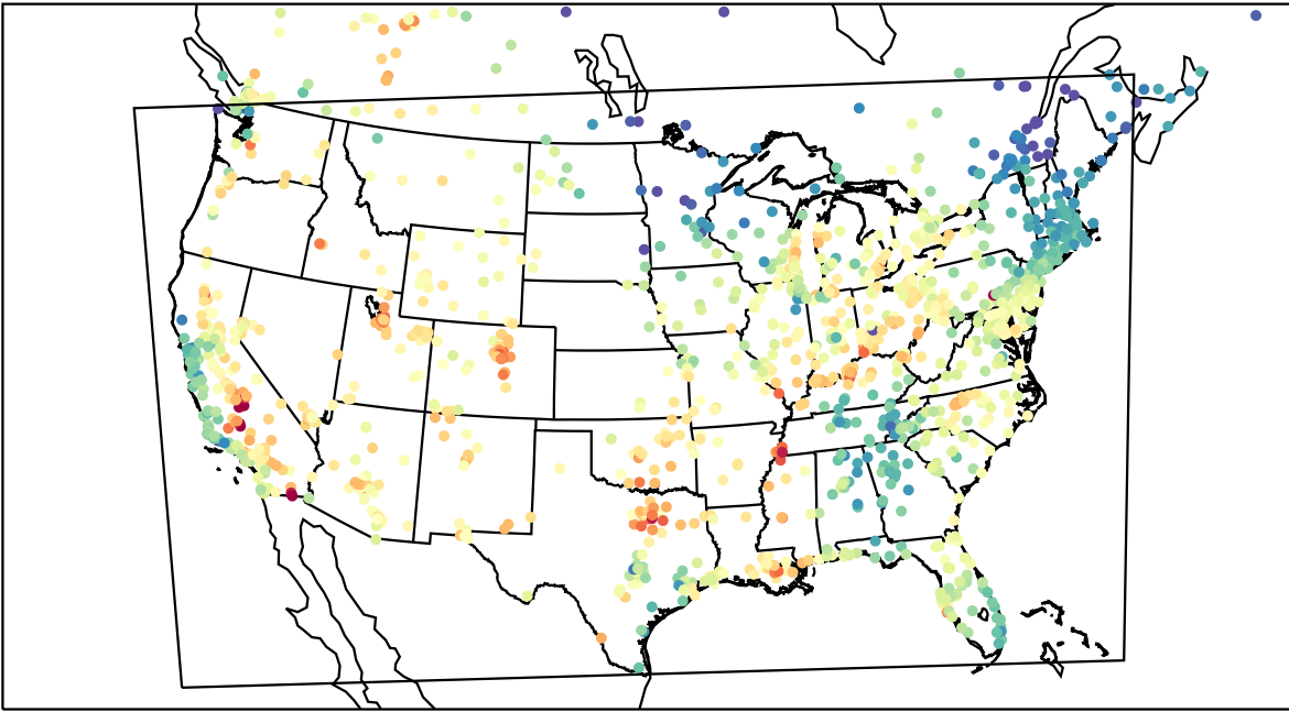
AirNOW (2023-09-16_21:00:00)
