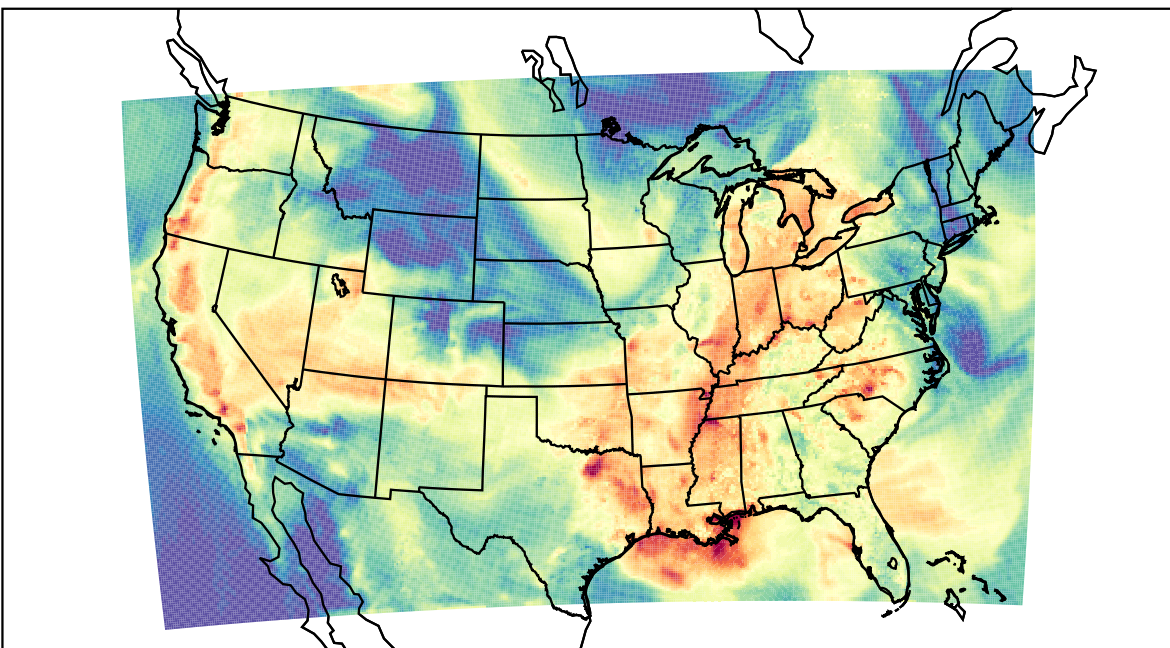
WRF (2023-09-16_22:00:00)
