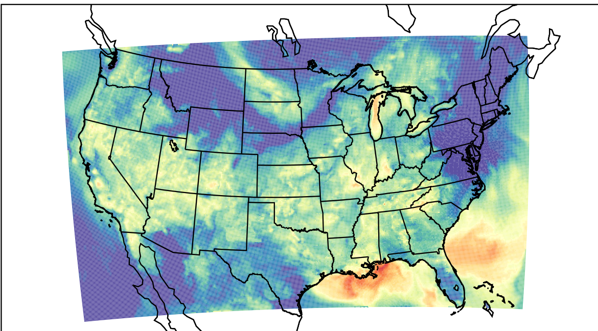
WRF (2023-09-16_07:00:00)
