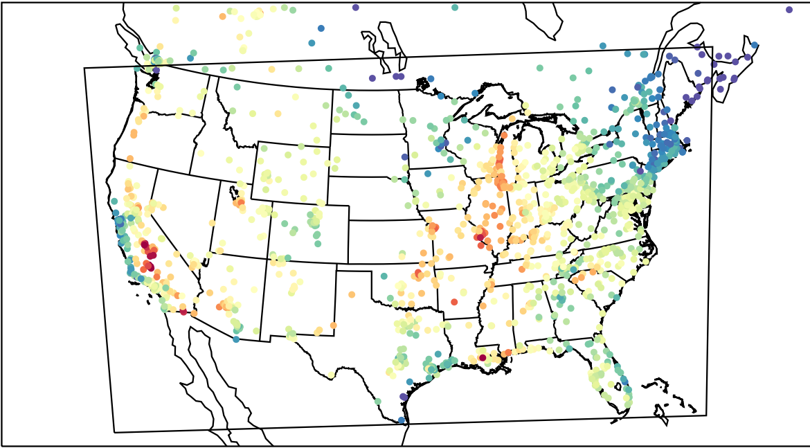
AirNOW (2023-09-15_20:00:00)
