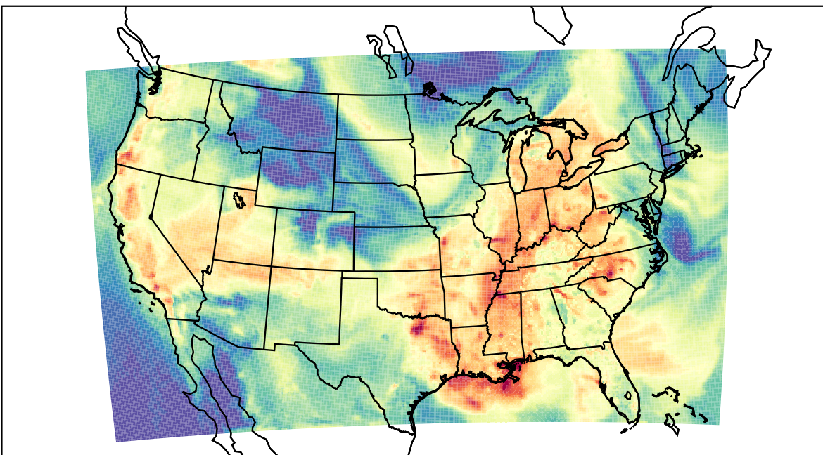
WRF (2023-09-16_21:00:00)
