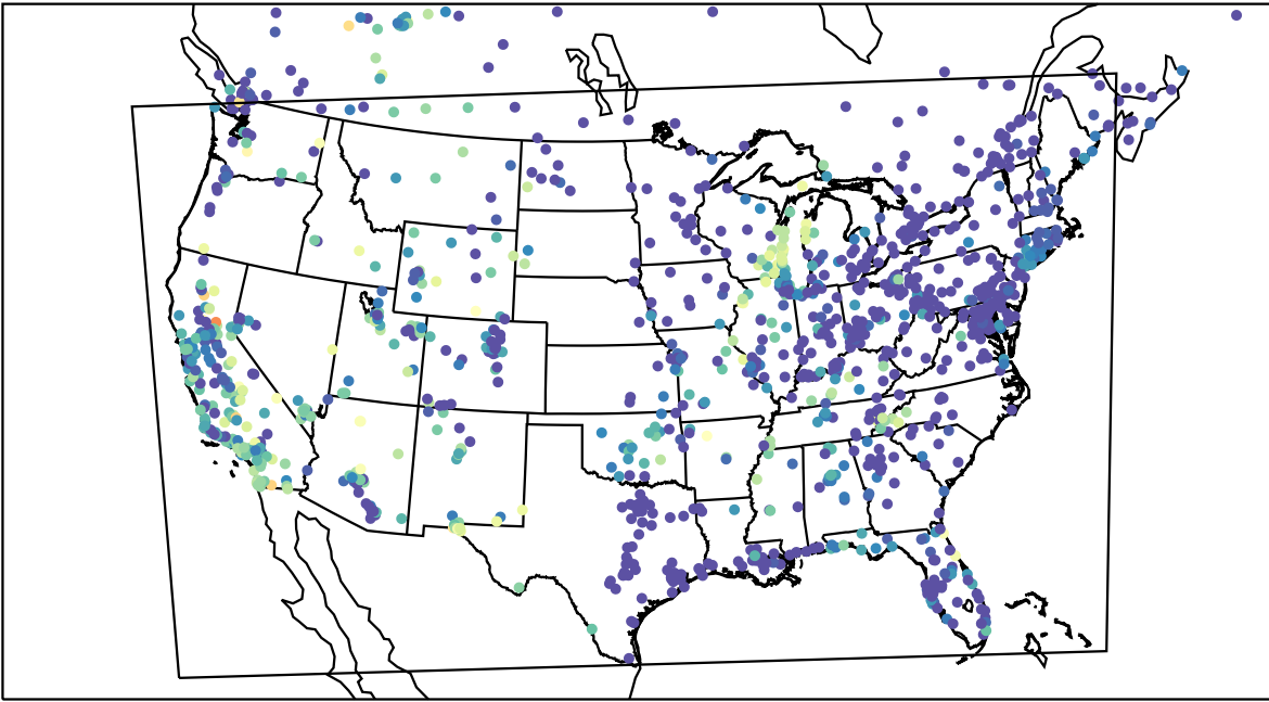
AirNOW (2023-09-16_08:00:00)
