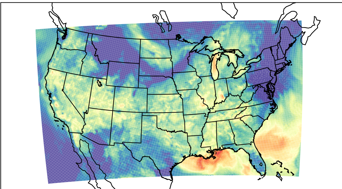
WRF (2023-09-16_06:00:00)
