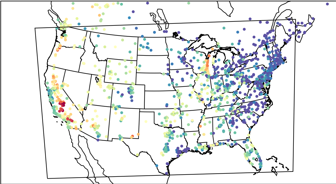
AirNOW (2023-09-16_01:00:00)
