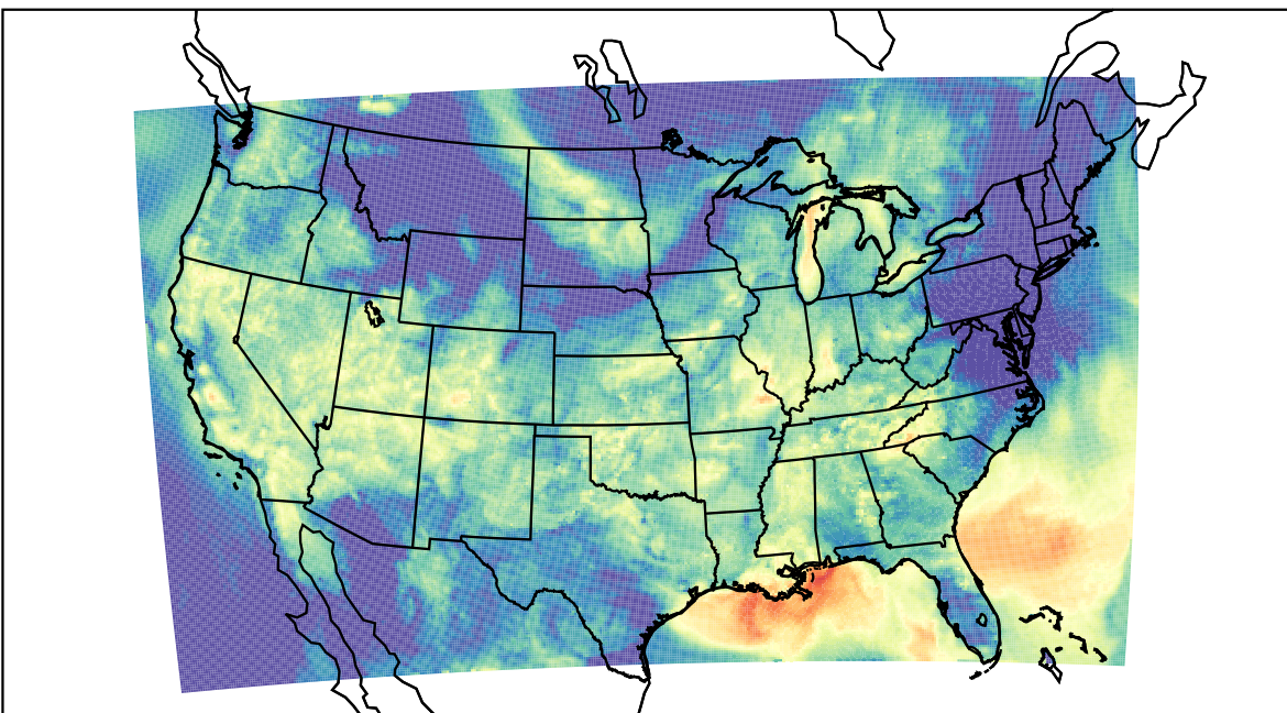
WRF (2023-09-16_08:00:00)
