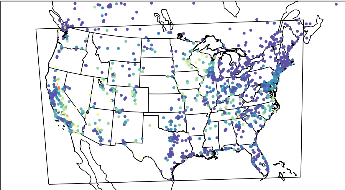
AirNOW (2023-09-15_06:00:00)
