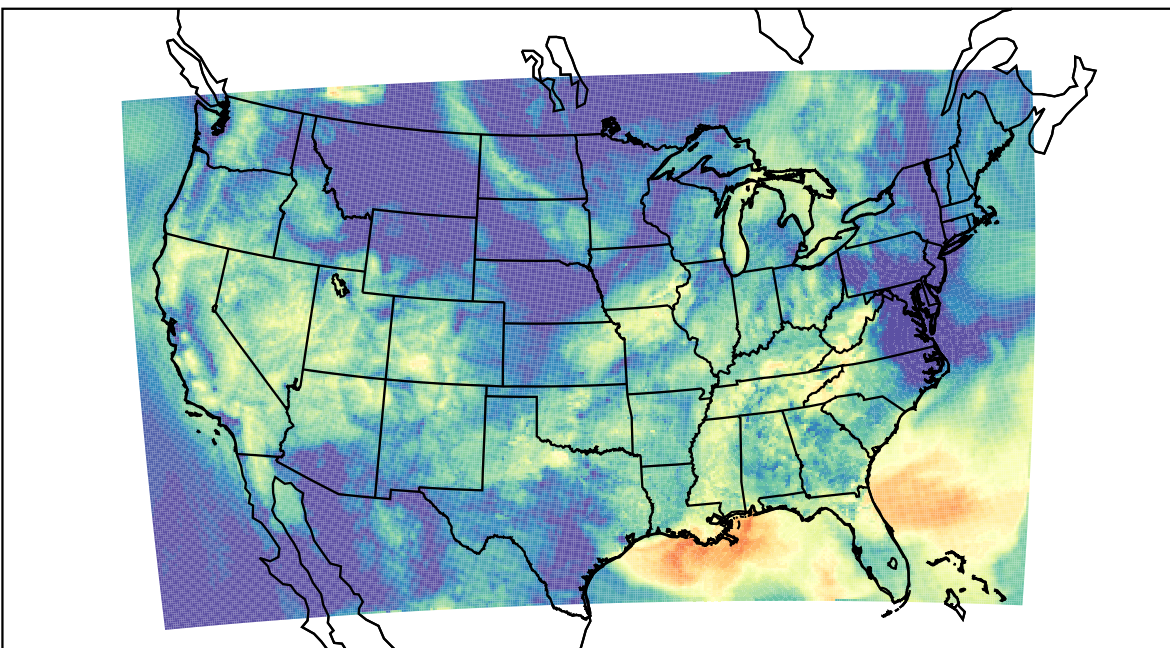
WRF (2023-09-16_14:00:00)
