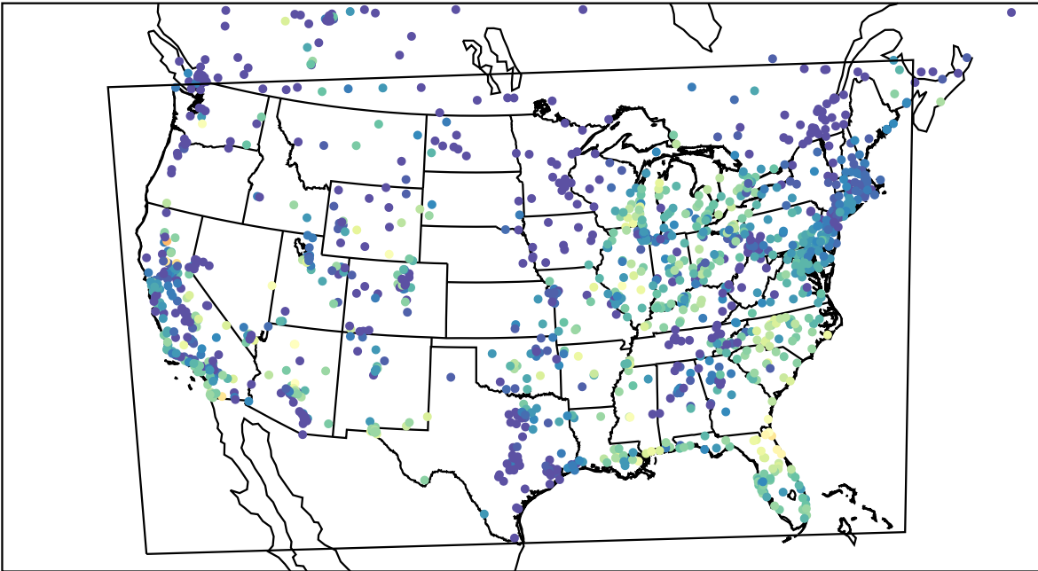
AirNOW (2023-09-16_14:00:00)
