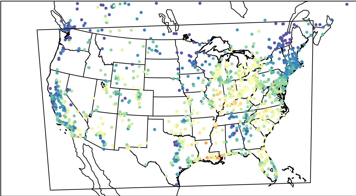
AirNOW (2023-09-16_16:00:00)
