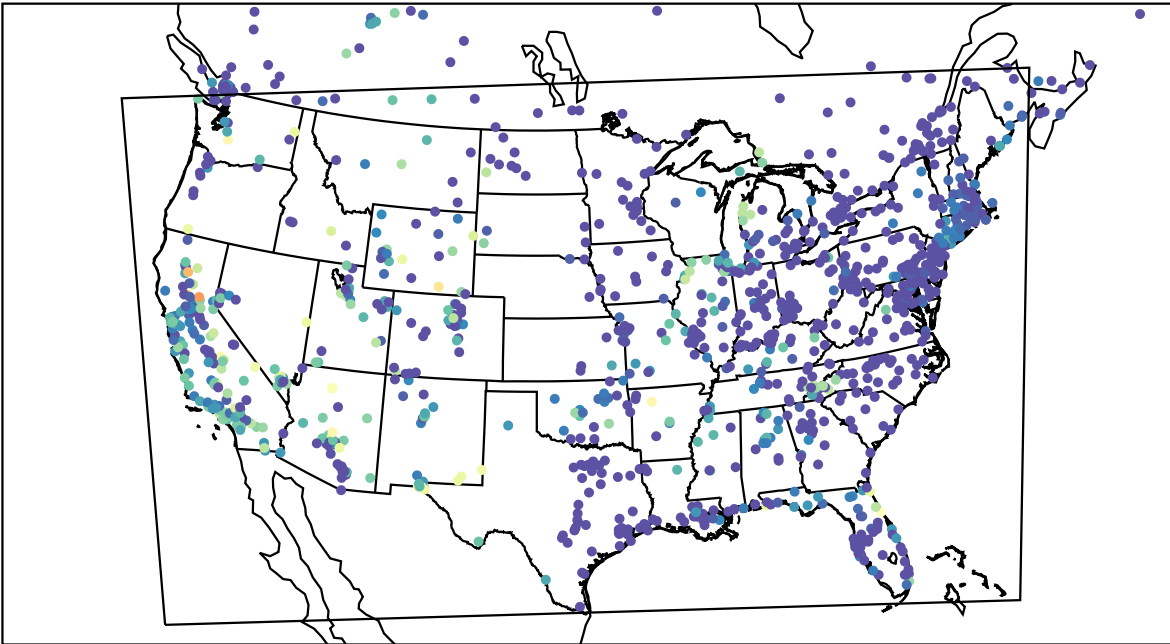
AirNOW (2023-09-16_10:00:00)
