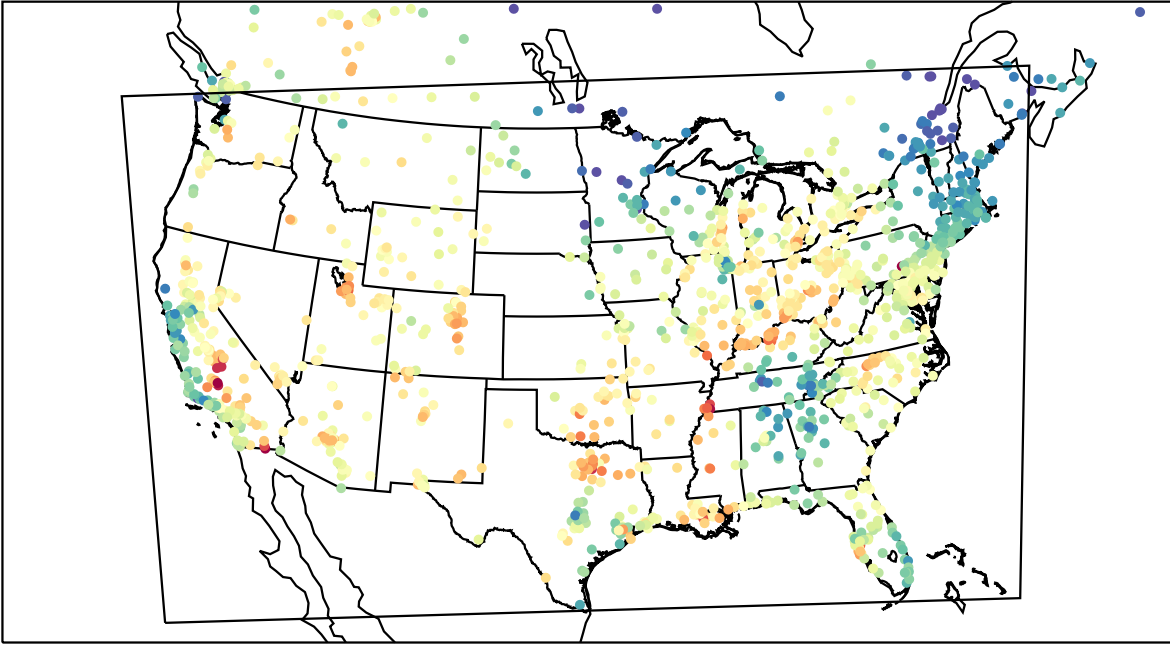
AirNOW (2023-09-16_20:00:00)
