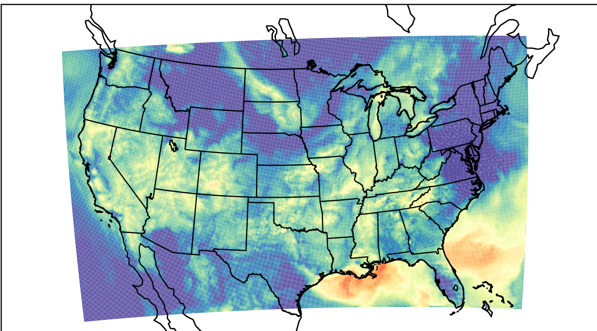
WRF (2023-09-16_11:00:00)
