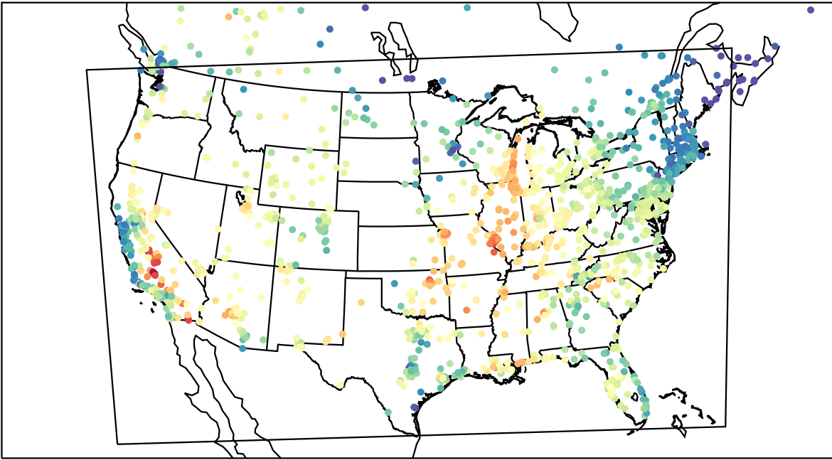
AirNOW (2023-09-15_19:00:00)
