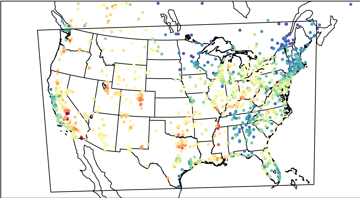
AirNOW (2023-09-16_22:00:00)
