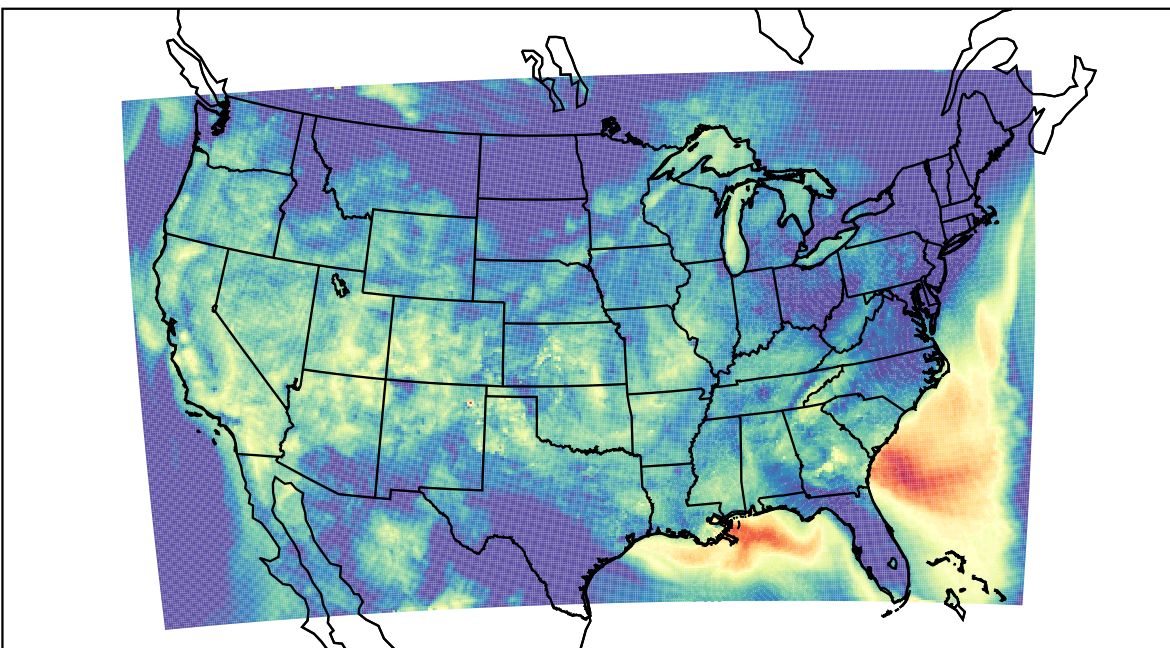
WRF (2023-09-15_12:00:00)
