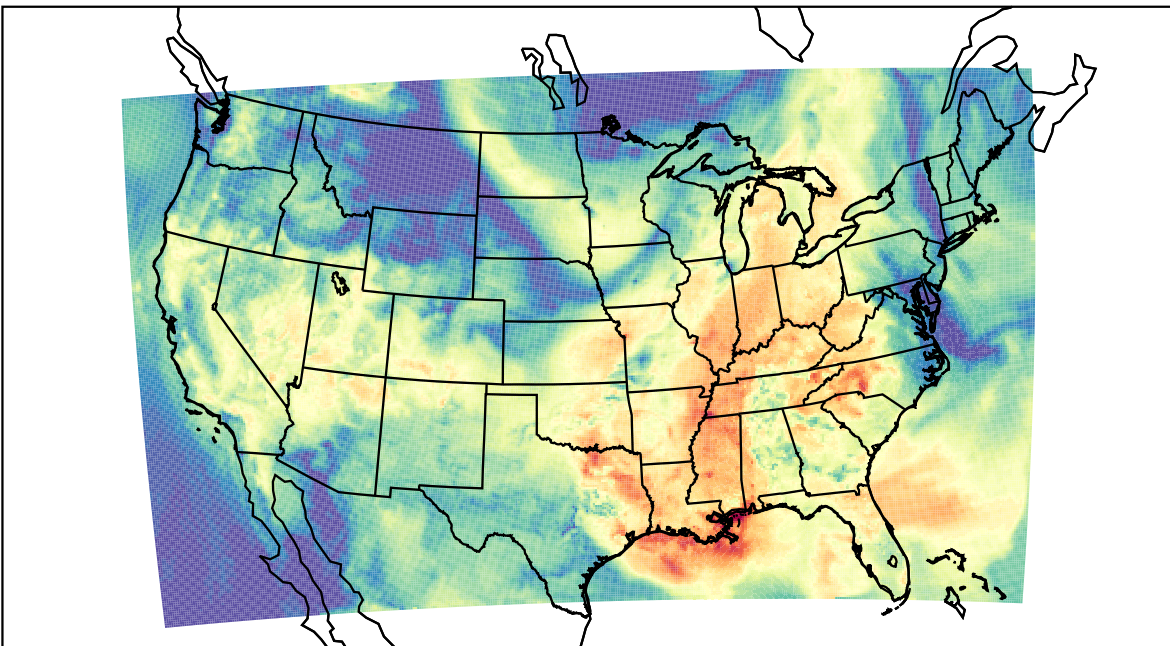
WRF (2023-09-16_17:00:00)
