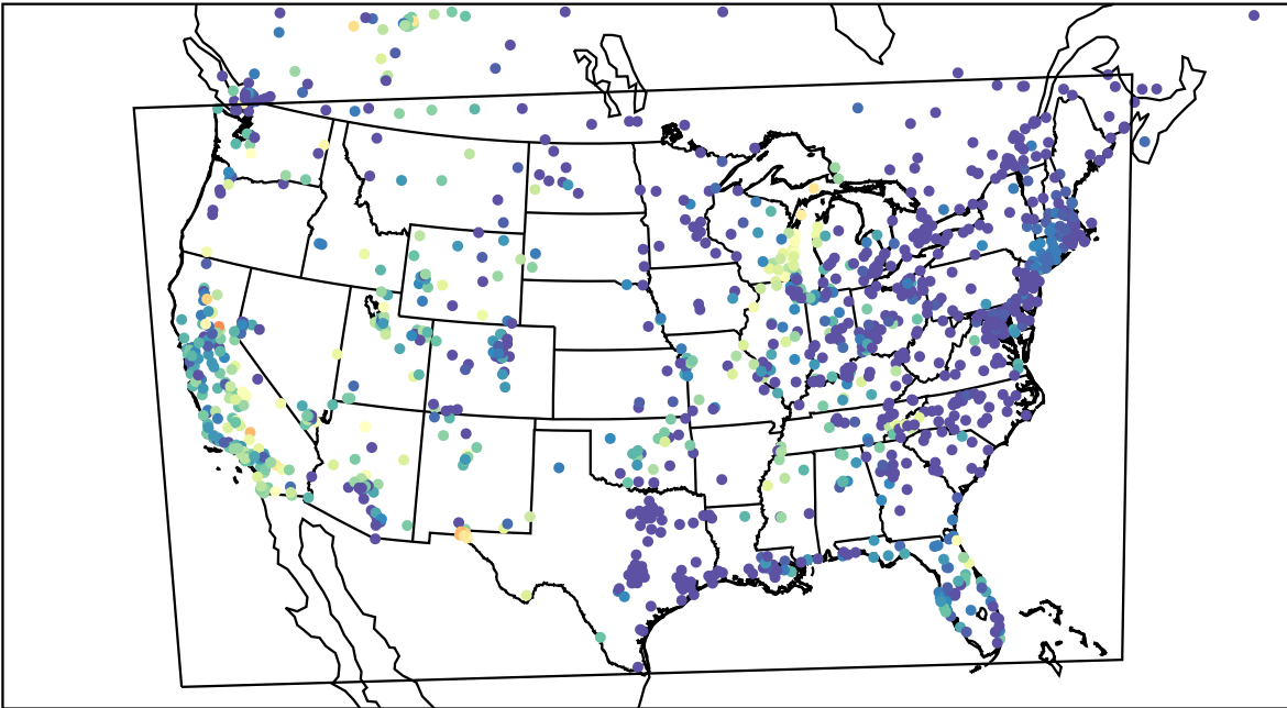
AirNOW (2023-09-16_06:00:00)
