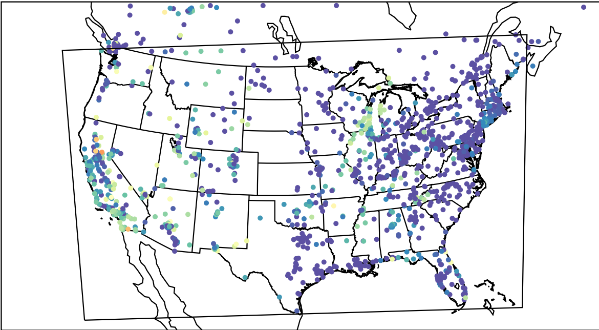
AirNOW (2023-09-16_09:00:00)
