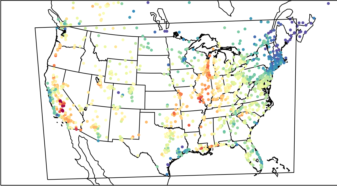
AirNOW (2023-09-15_21:00:00)
