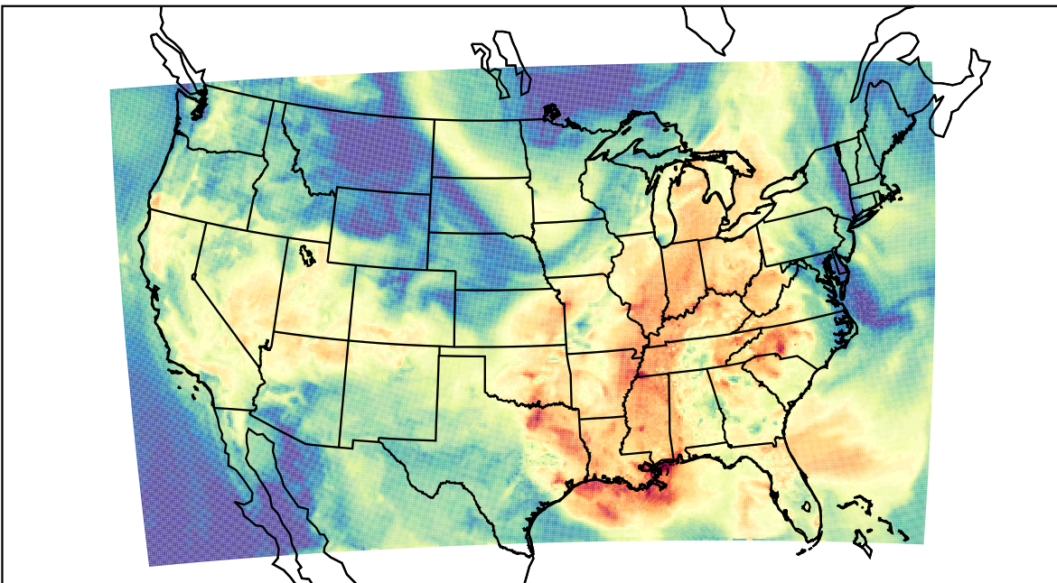
WRF (2023-09-16_18:00:00)
