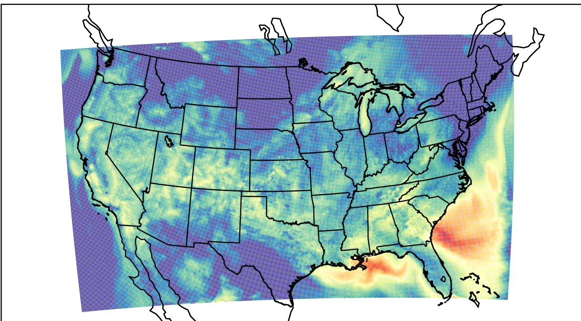
WRF (2023-09-15_14:00:00)
