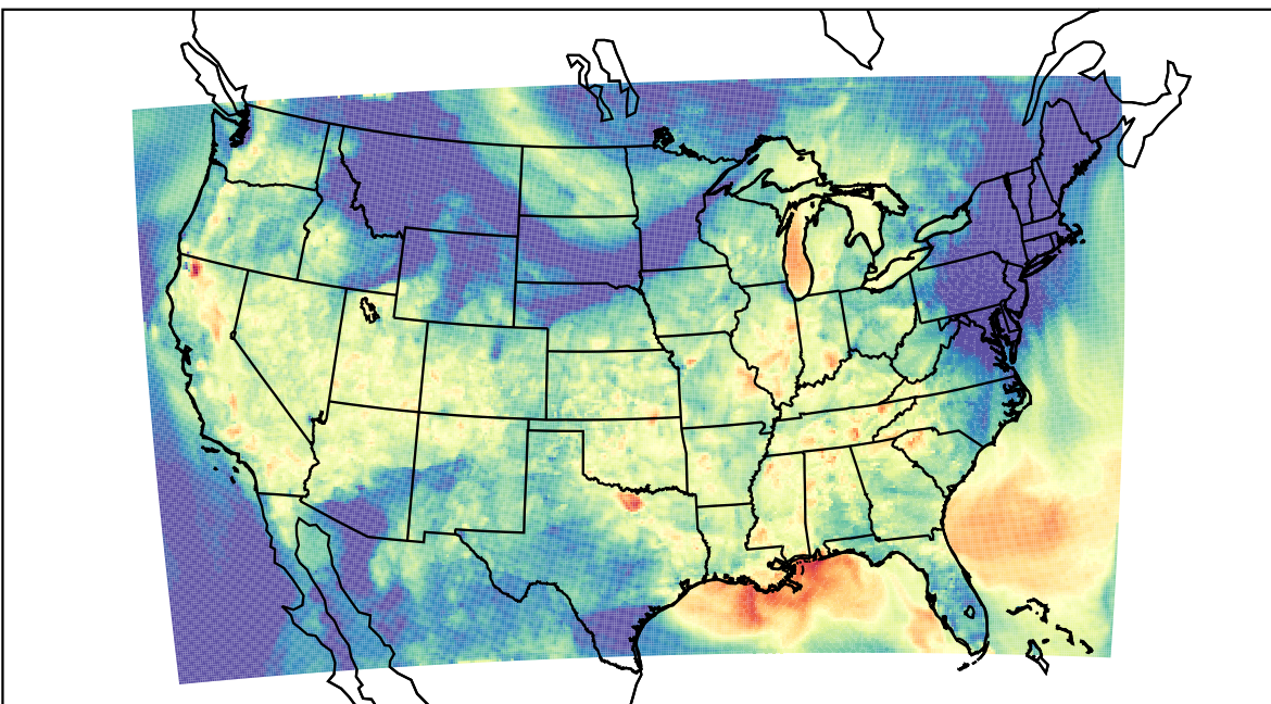
WRF (2023-09-16_03:00:00)
