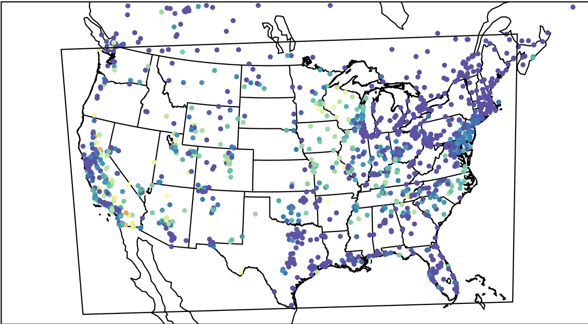
AirNOW (2023-09-15_07:00:00)
