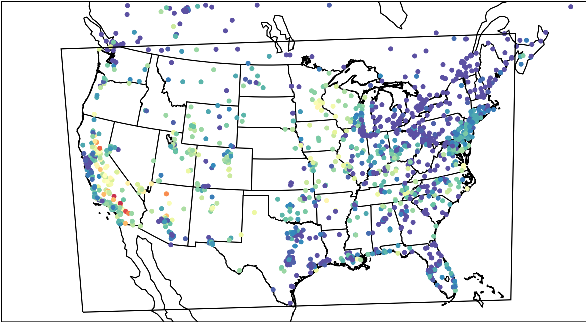
AirNOW (2023-09-15_03:00:00)
