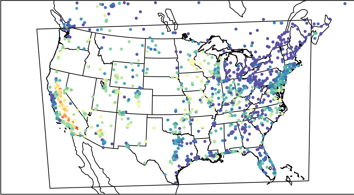
AirNOW (2023-09-15_02:00:00)
