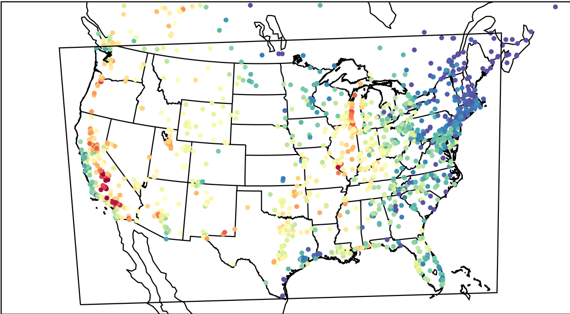
AirNOW (2023-09-15_23:00:00)
