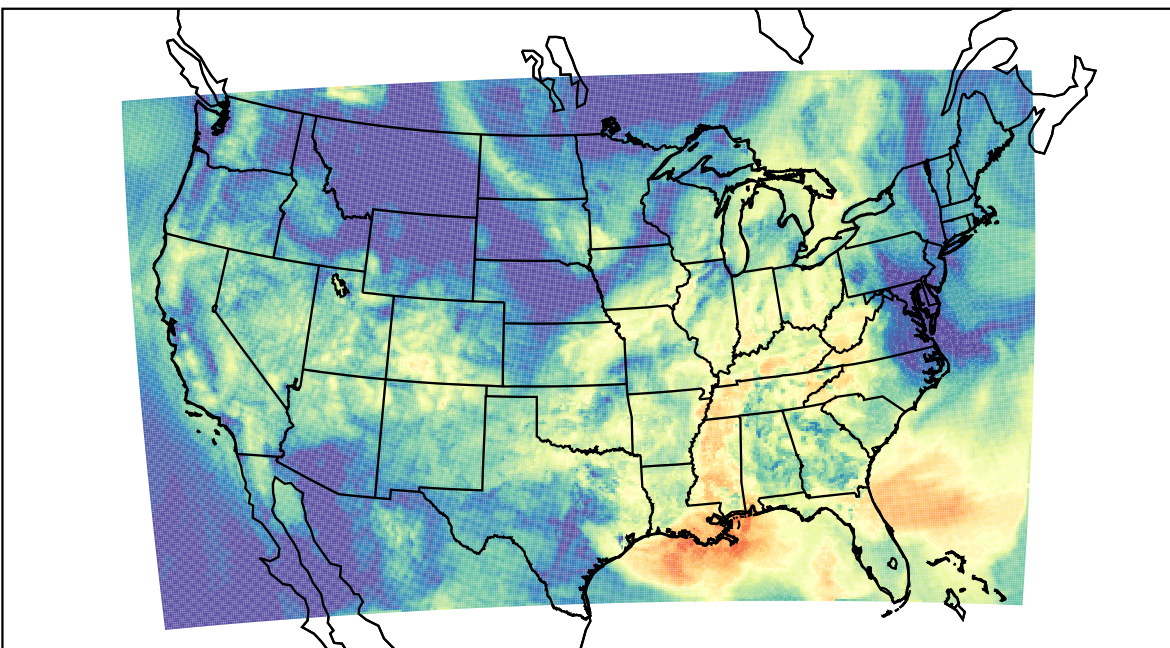
WRF (2023-09-16_15:00:00)
