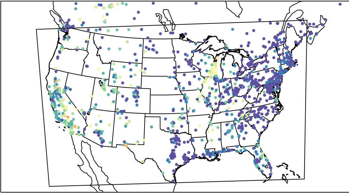
AirNOW (2023-09-16_05:00:00)
