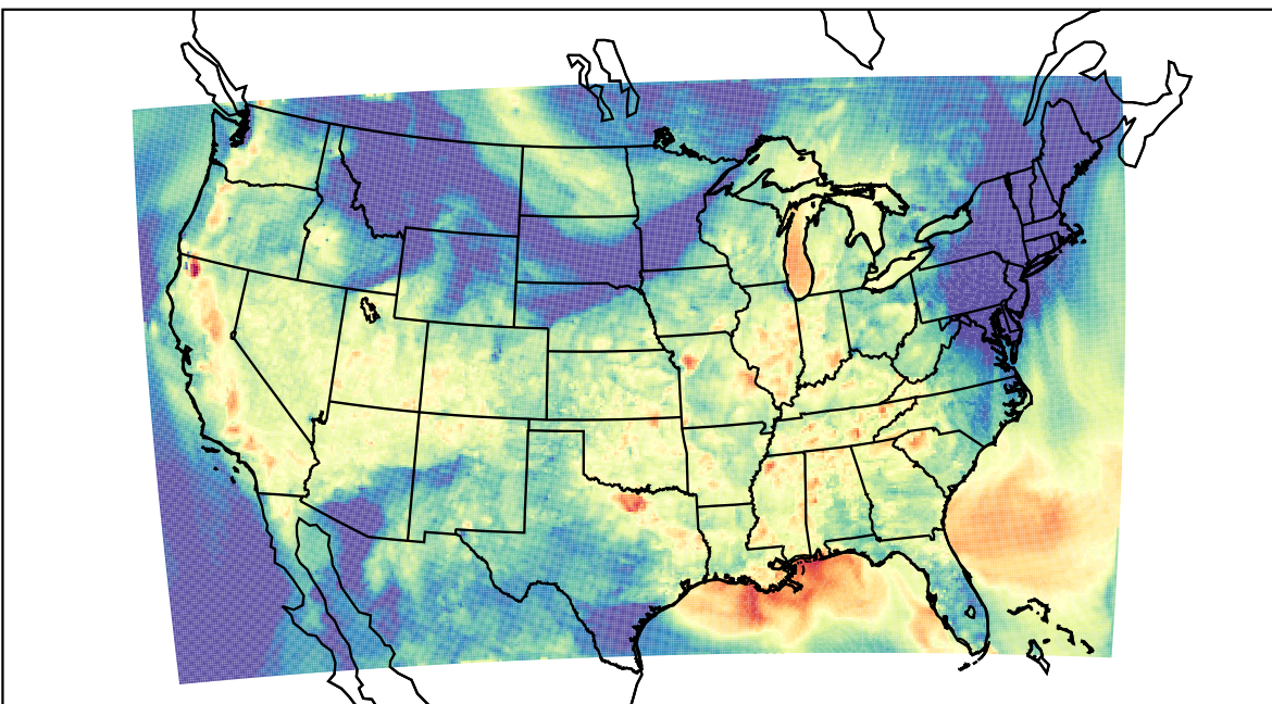
WRF (2023-09-16_02:00:00)
