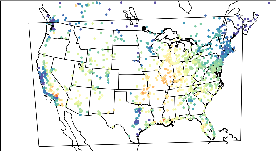
AirNOW (2023-09-15_17:00:00)
