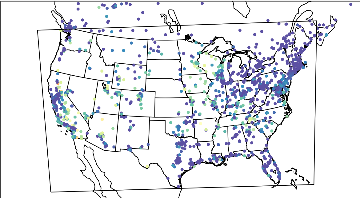
AirNOW (2023-09-15_08:00:00)
