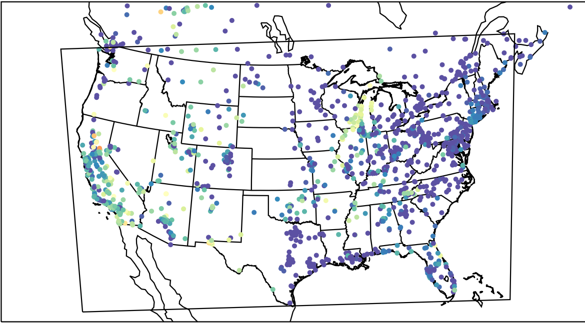
AirNOW (2023-09-16_07:00:00)
