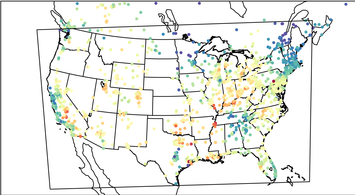
AirNOW (2023-09-16_19:00:00)
