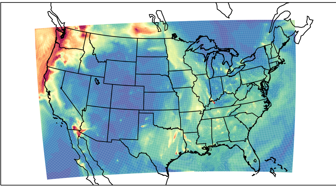
WRF 2023-09-19_13:00:00
