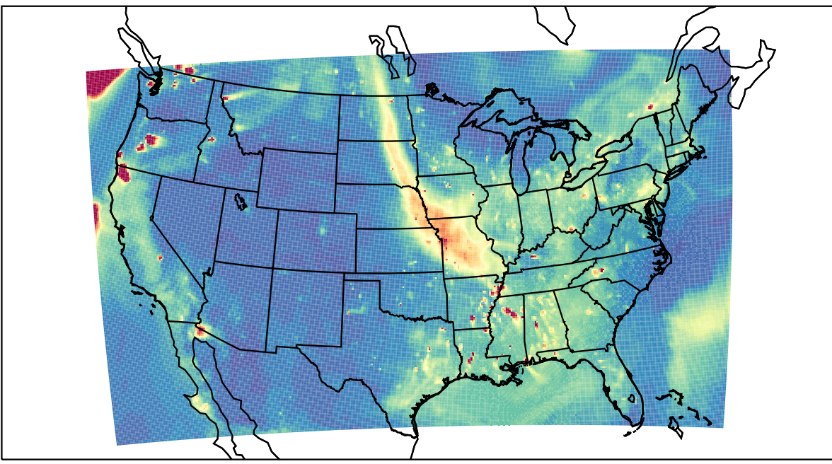
WRF 2023-09-18_01:00:00
