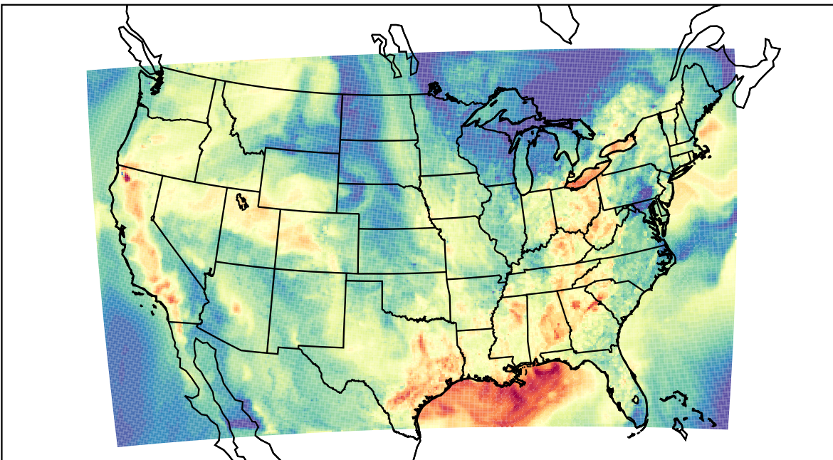
WRF (2023-09-18_00:00:00)
