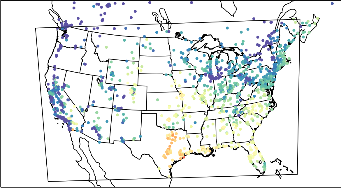
AirNOW (2023-09-19_15:00:00)
