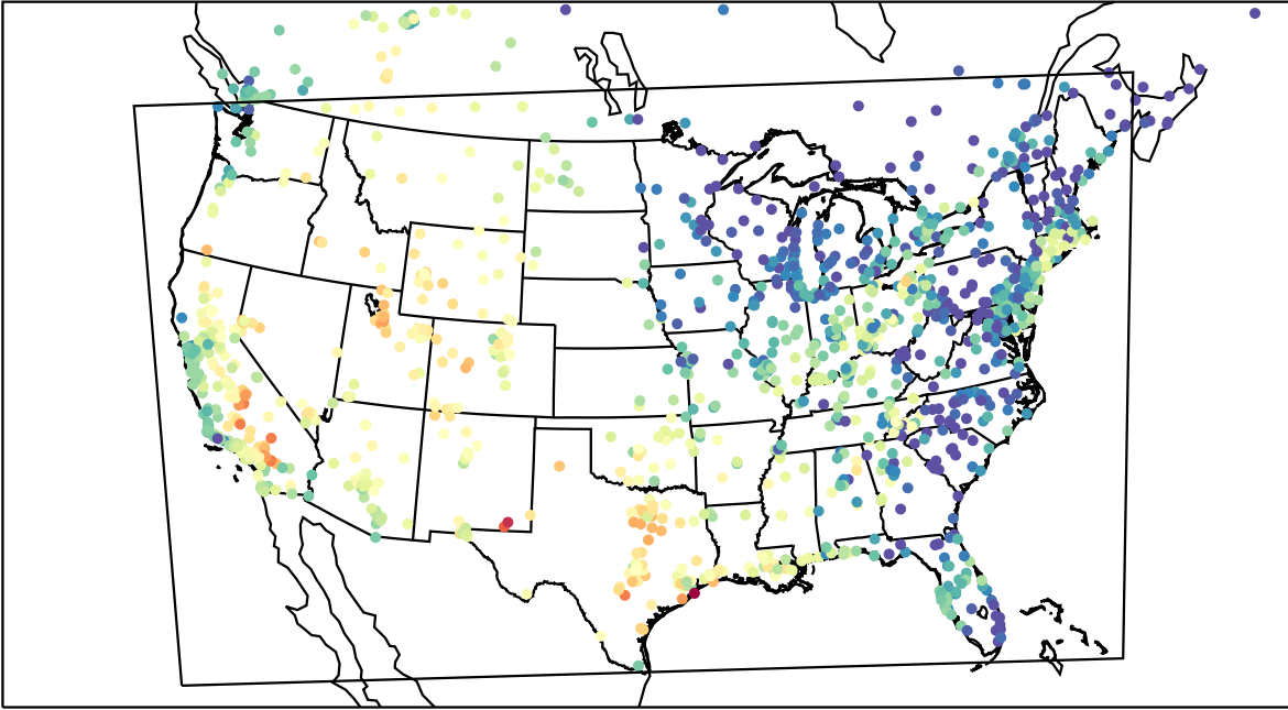
AirNOW (2023-09-18_00:00:00)
