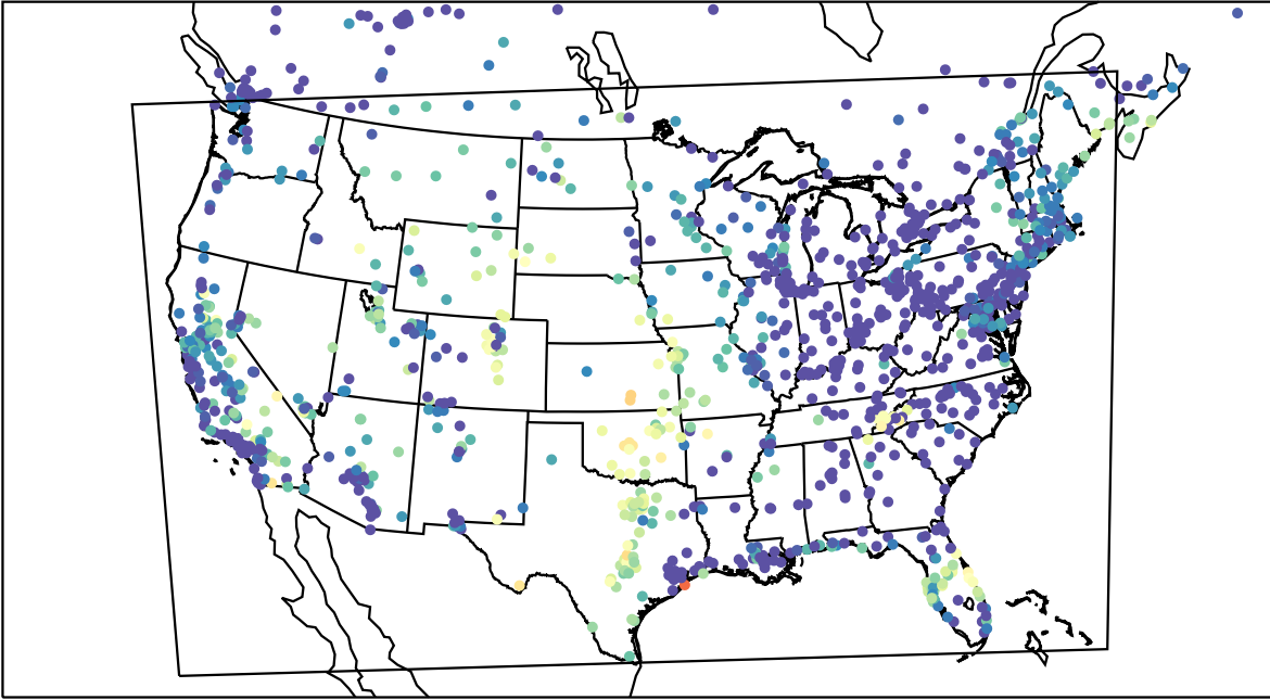
AirNOW (2023-09-19_09:00:00)
