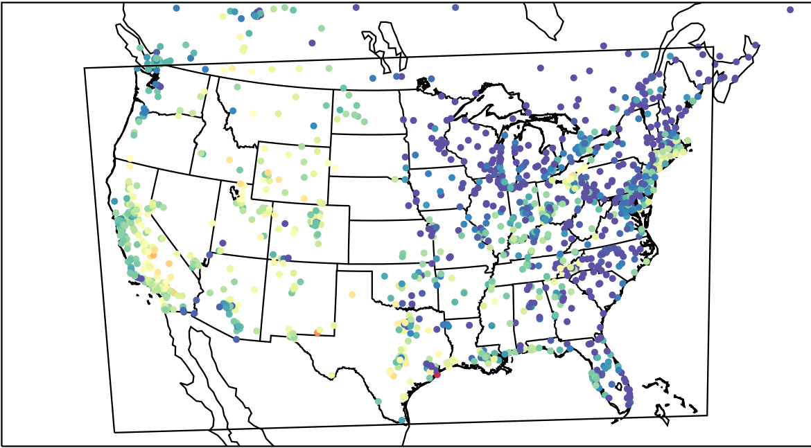
AirNOW (2023-09-18_02:00:00)
