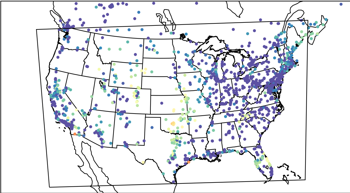
AirNOW (2023-09-19_11:00:00)
