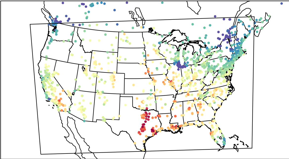
AirNOW (2023-09-19_19:00:00)
