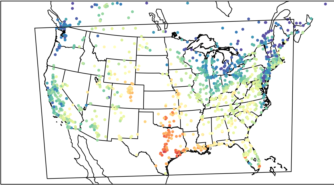
AirNOW (2023-09-18_17:00:00)
