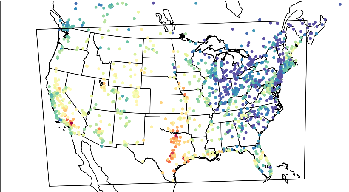
AirNOW (2023-09-19_00:00:00)
