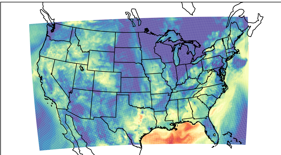
WRF (2023-09-18_12:00:00)
