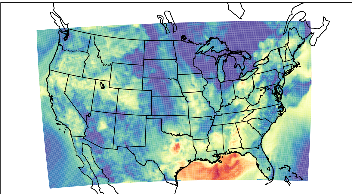
WRF (2023-09-18_07:00:00)
