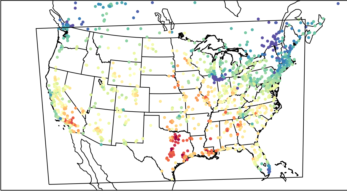
AirNOW (2023-09-19_21:00:00)
