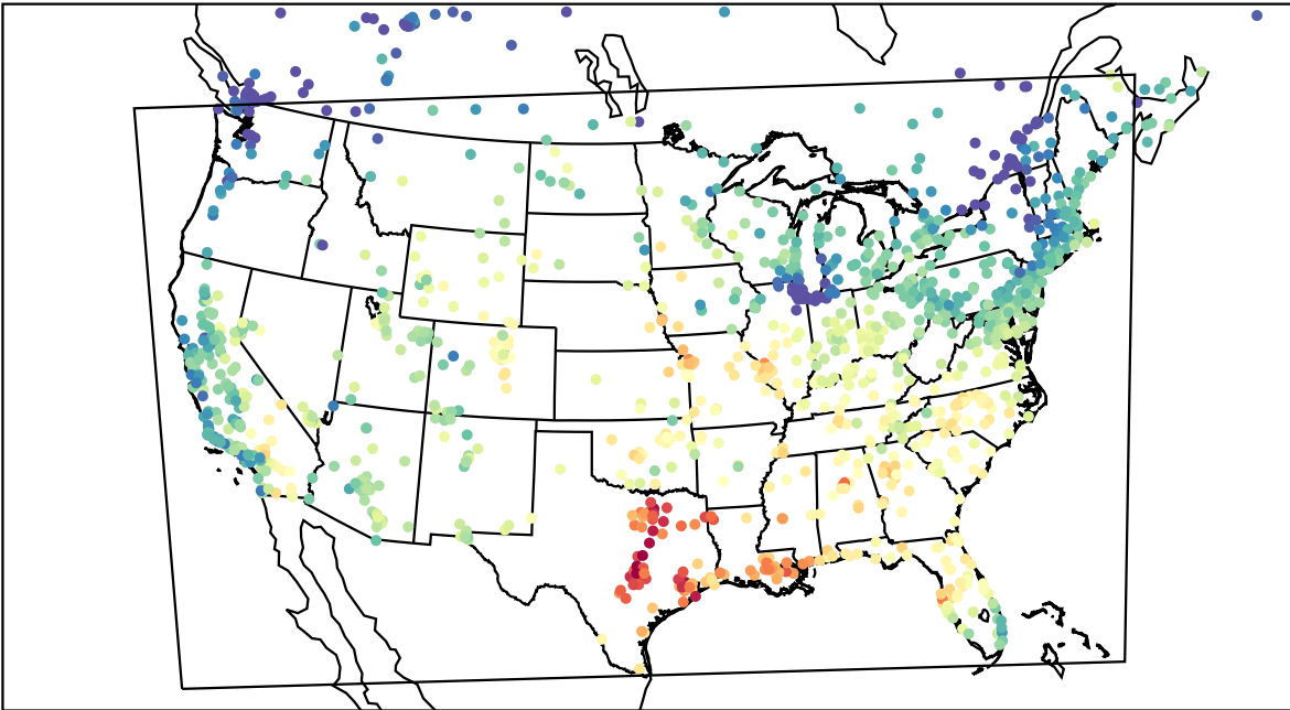
AirNOW (2023-09-19_17:00:00)
