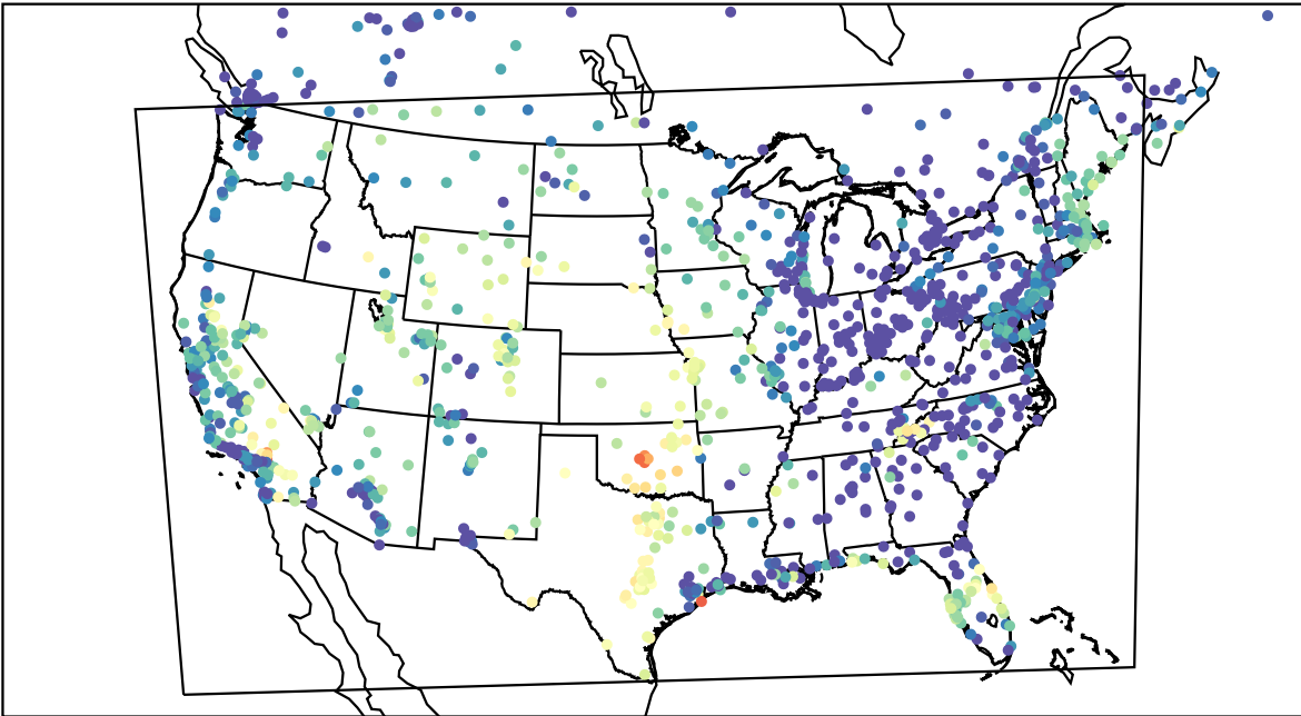
AirNOW (2023-09-19_05:00:00)
