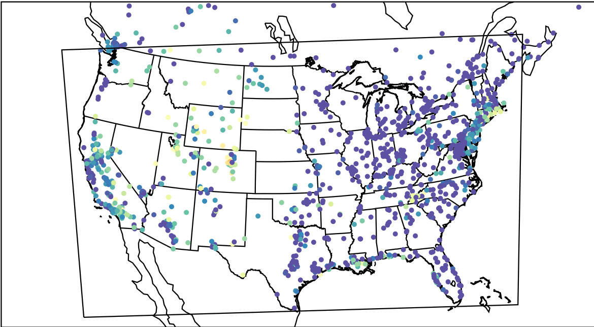
AirNOW (2023-09-18_10:00:00)
