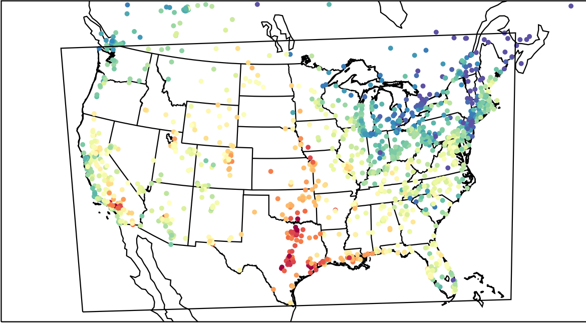
AirNOW (2023-09-18_22:00:00)
