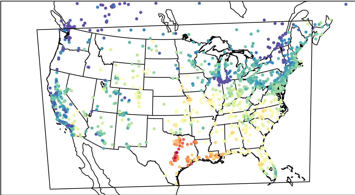
AirNOW (2023-09-19_16:00:00)
