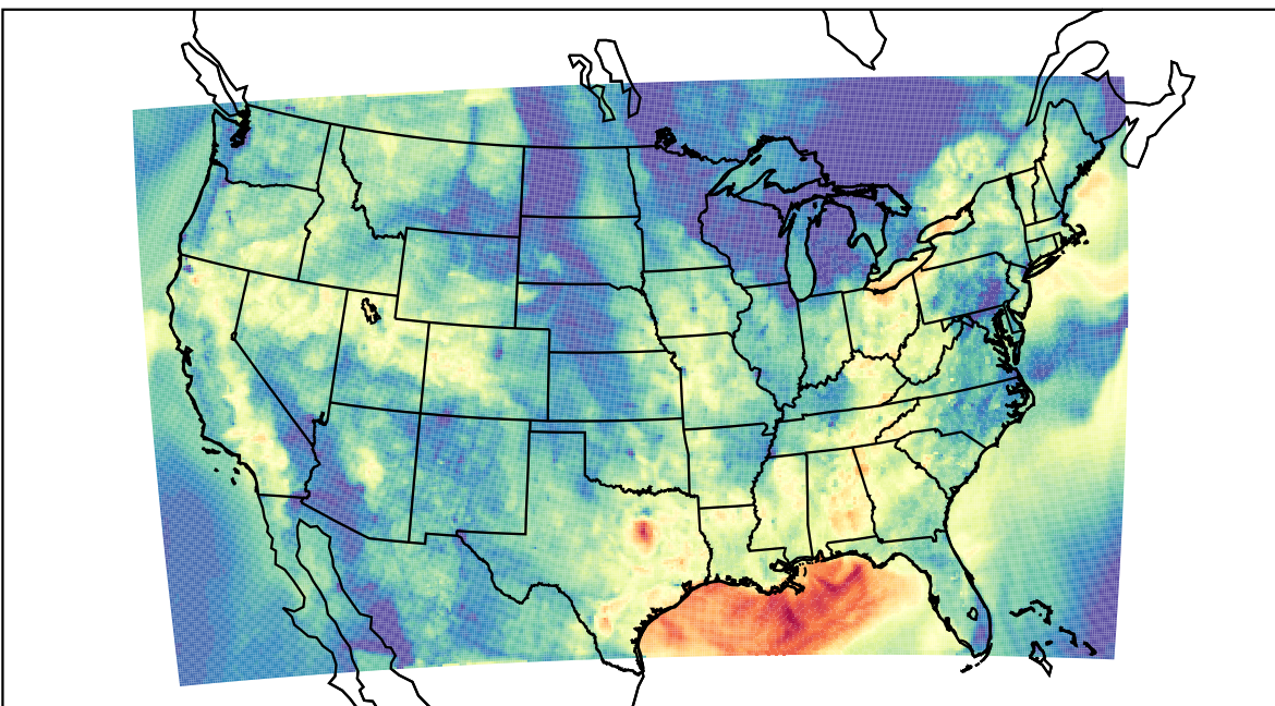
WRF (2023-09-18_03:00:00)
