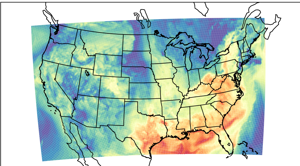
WRF (2023-09-18_16:00:00)
