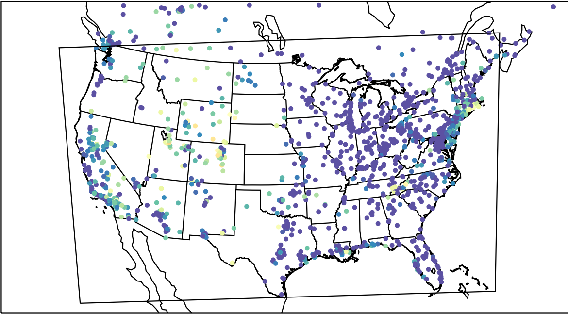
AirNOW (2023-09-18_11:00:00)
