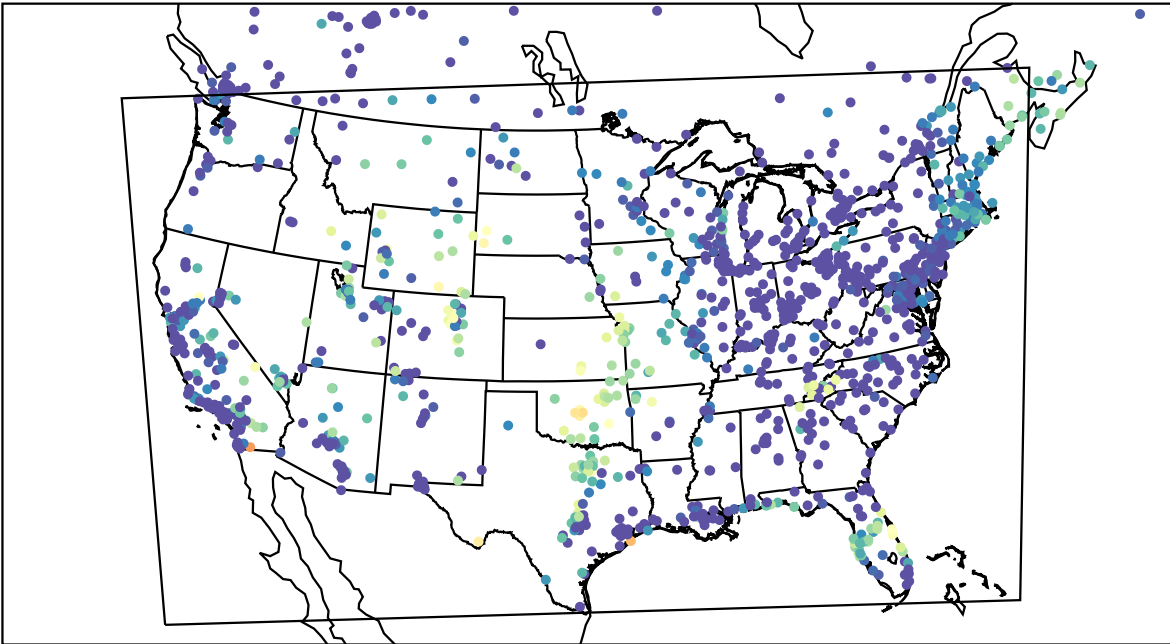
AirNOW (2023-09-19_12:00:00)
