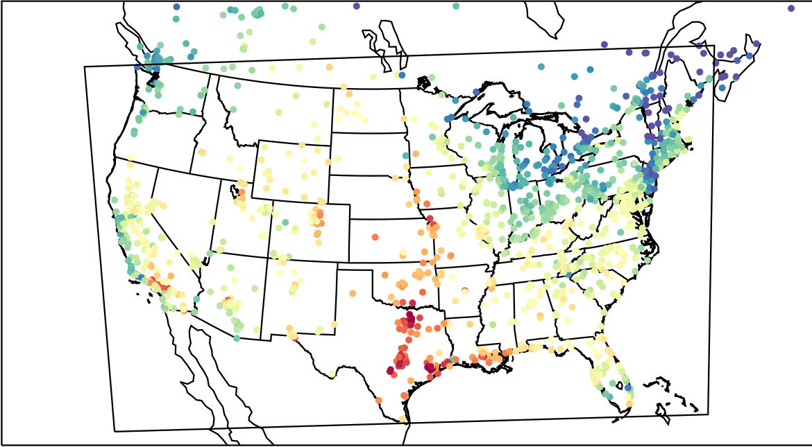
AirNOW (2023-09-18_21:00:00)
