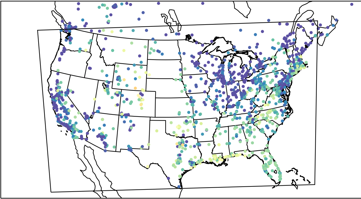
AirNOW (2023-09-18_14:00:00)
