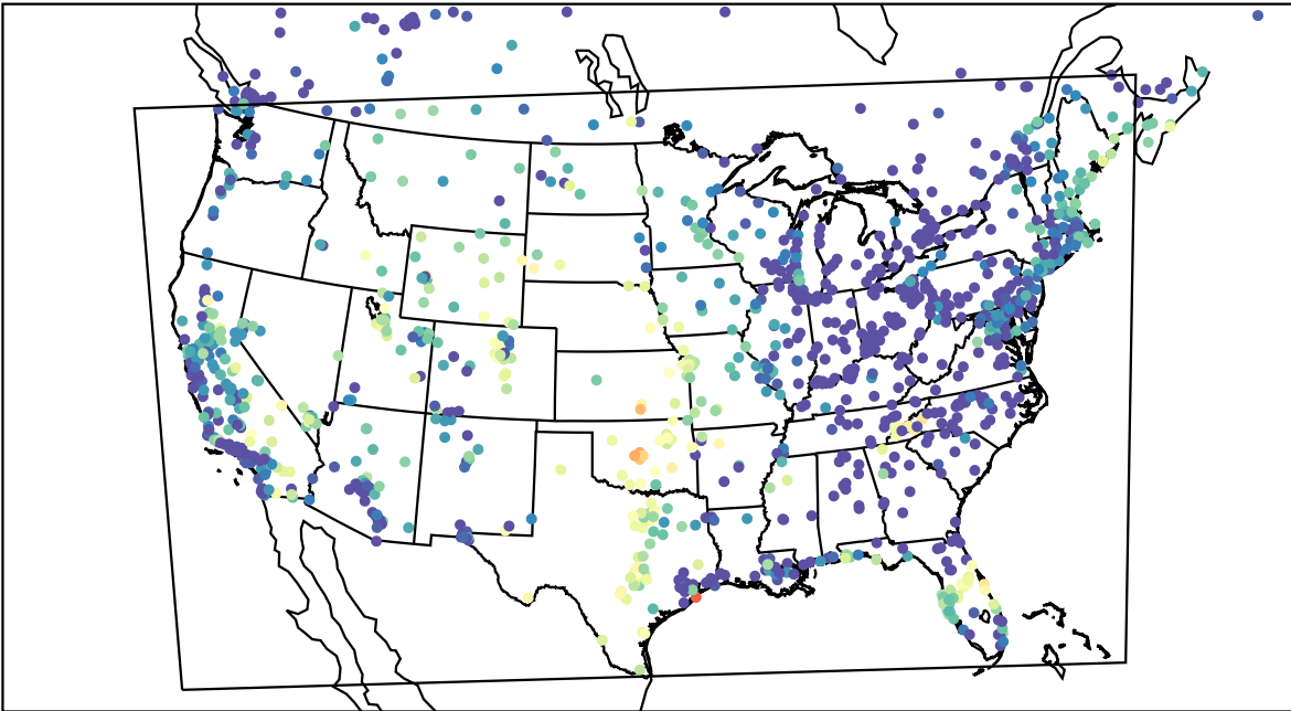
AirNOW (2023-09-19_07:00:00)
