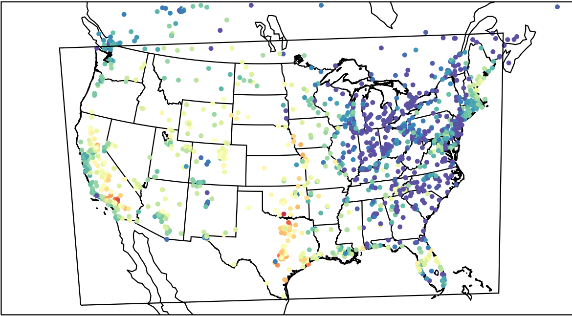
AirNOW (2023-09-19_01:00:00)
