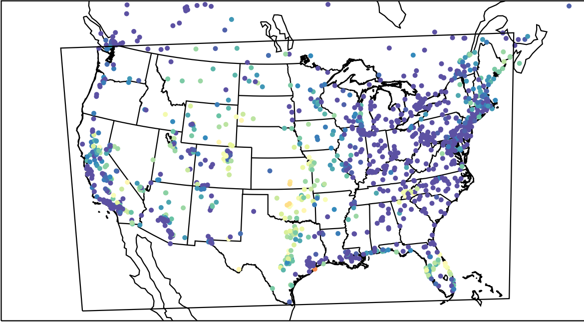
AirNOW (2023-09-19_10:00:00)
