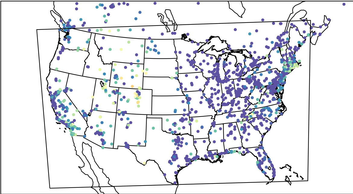
AirNOW (2023-09-18_12:00:00)
