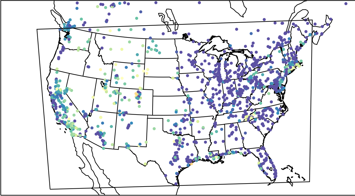
AirNOW (2023-09-18_09:00:00)
