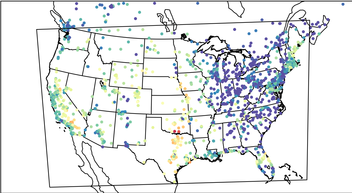
AirNOW (2023-09-19_02:00:00)
