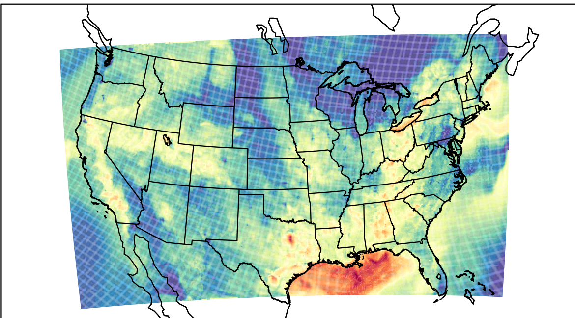
WRF (2023-09-18_02:00:00)
