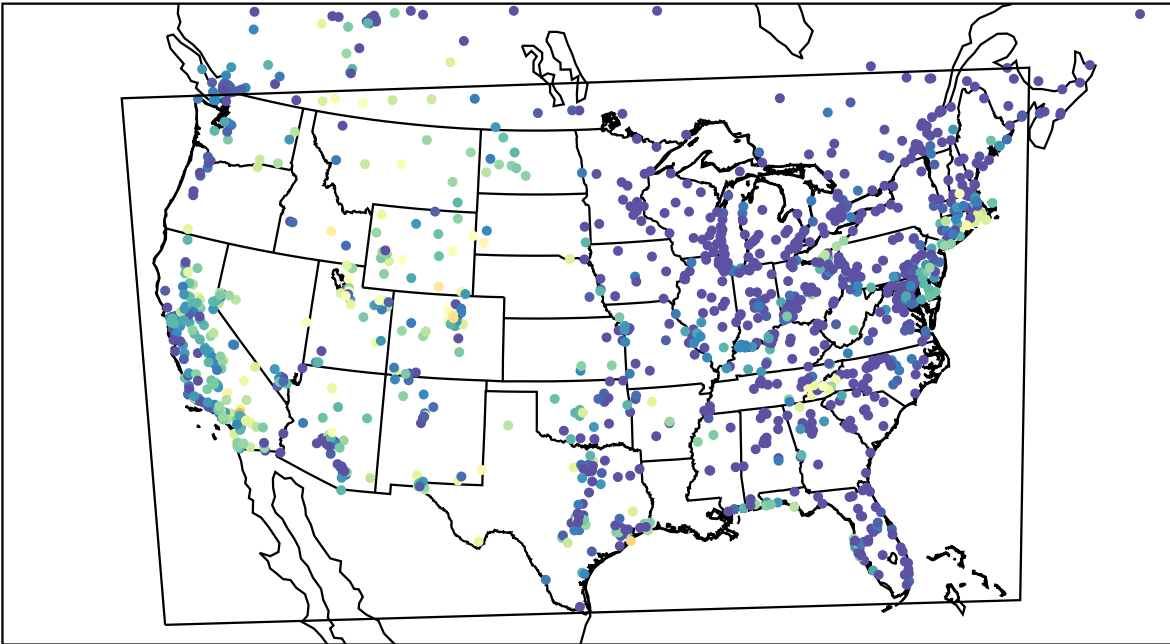
AirNOW (2023-09-18_07:00:00)
