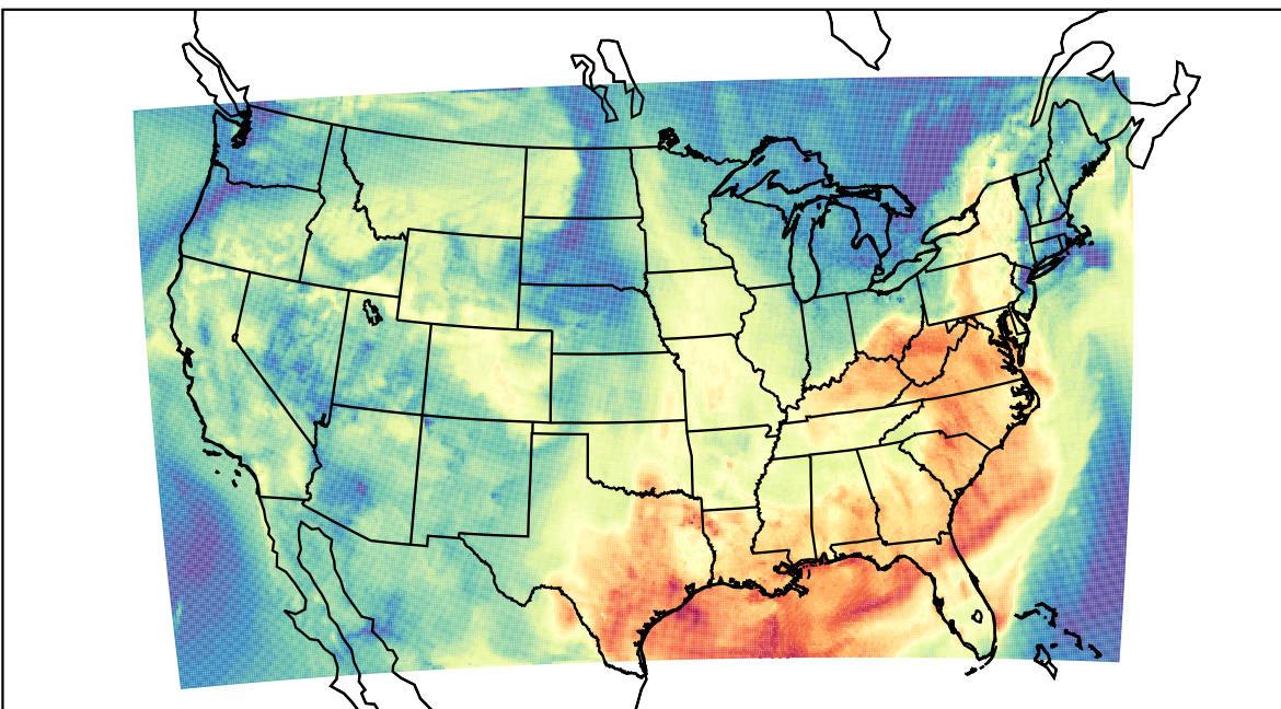
WRF (2023-09-18_17:00:00)
