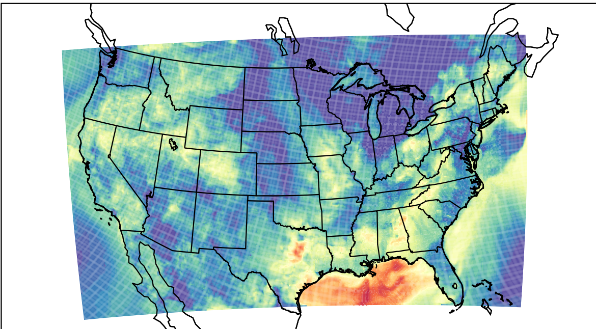
WRF (2023-09-18_09:00:00)
