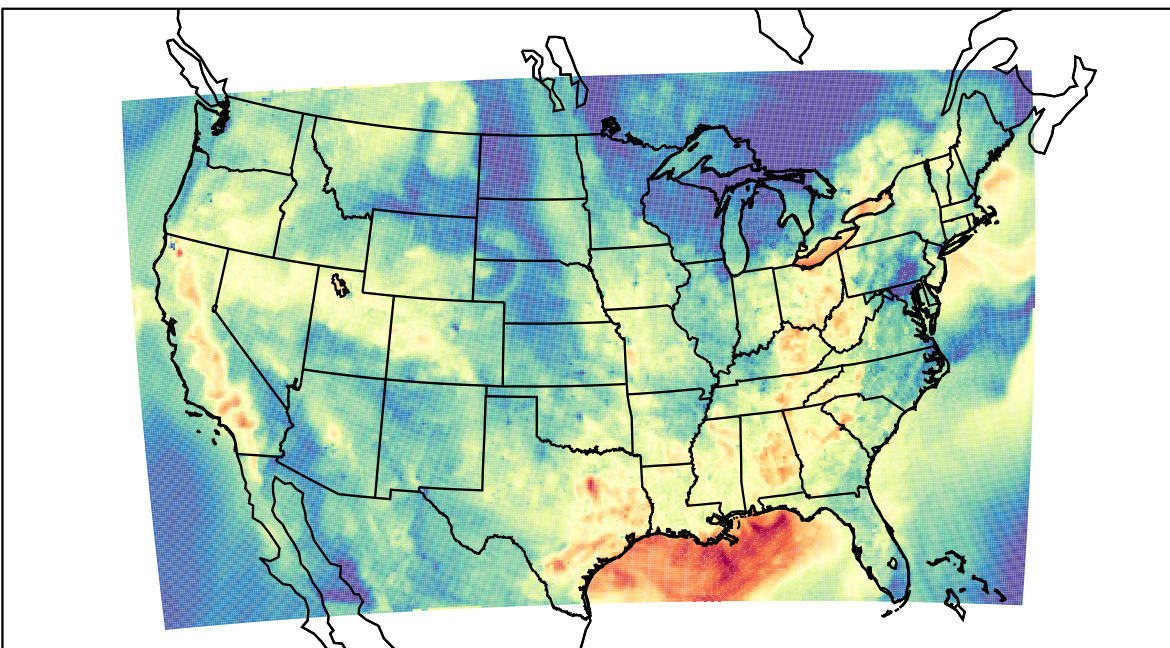
WRF (2023-09-18_01:00:00)
