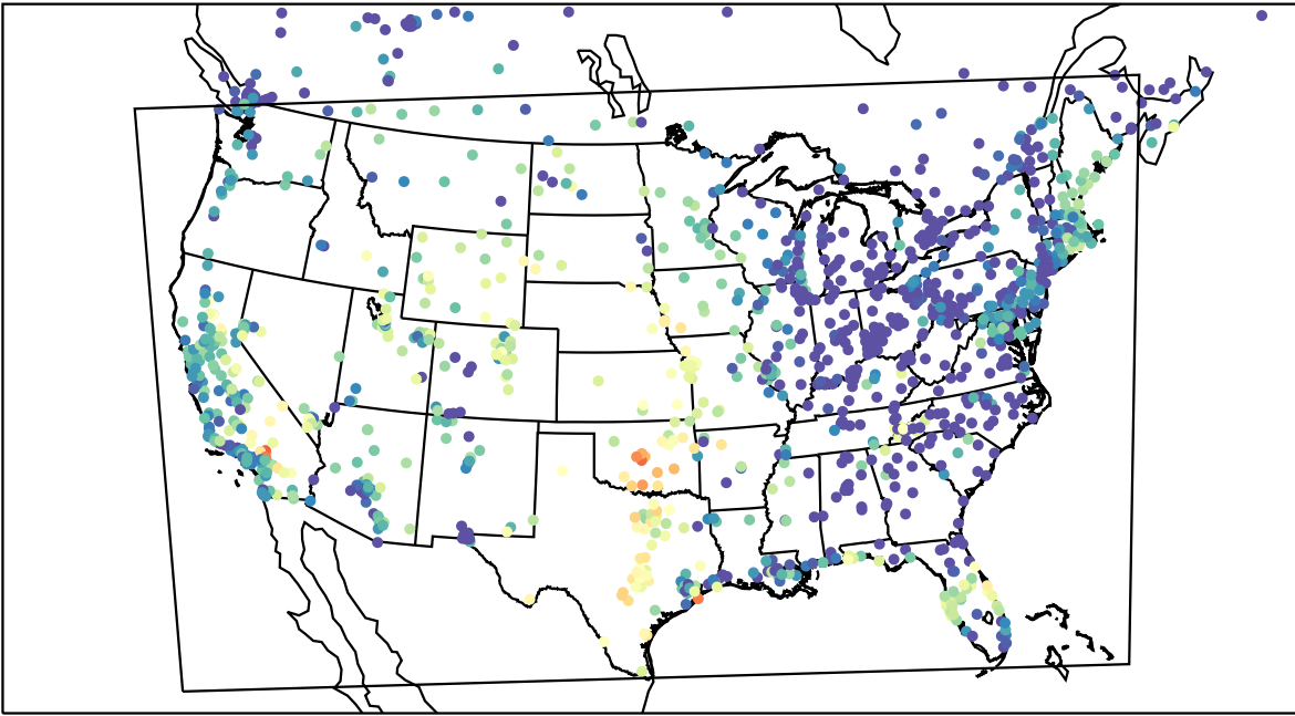
AirNOW (2023-09-19_04:00:00)
