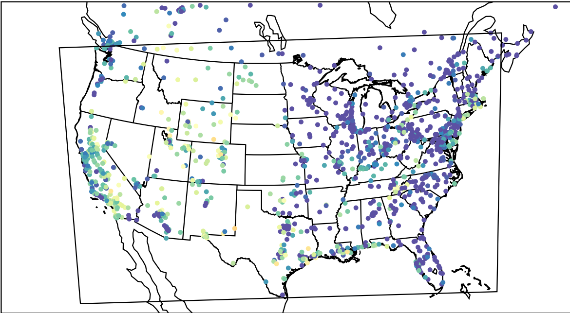
AirNOW (2023-09-18_05:00:00)
