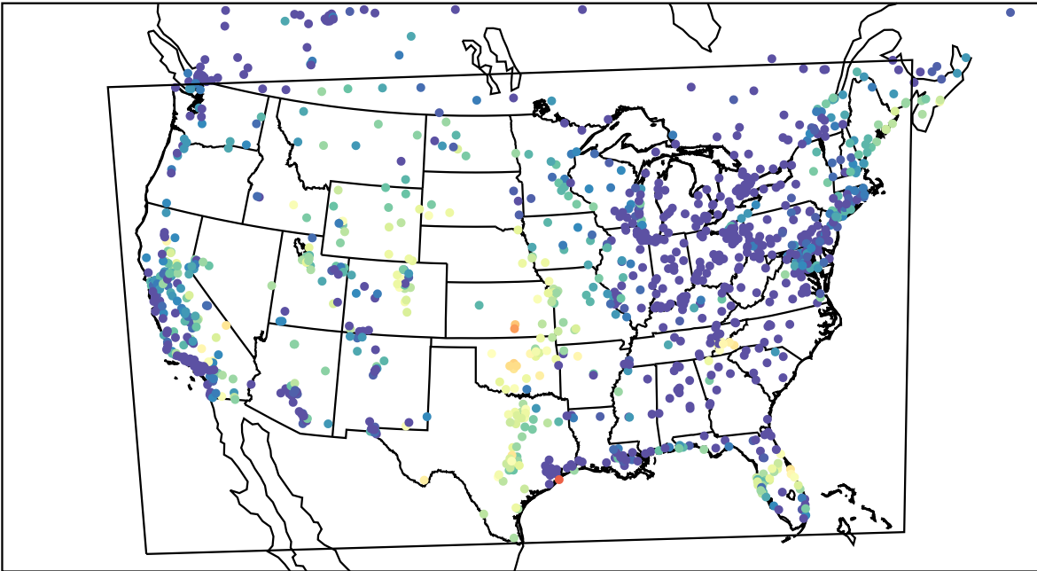
AirNOW (2023-09-19_08:00:00)
