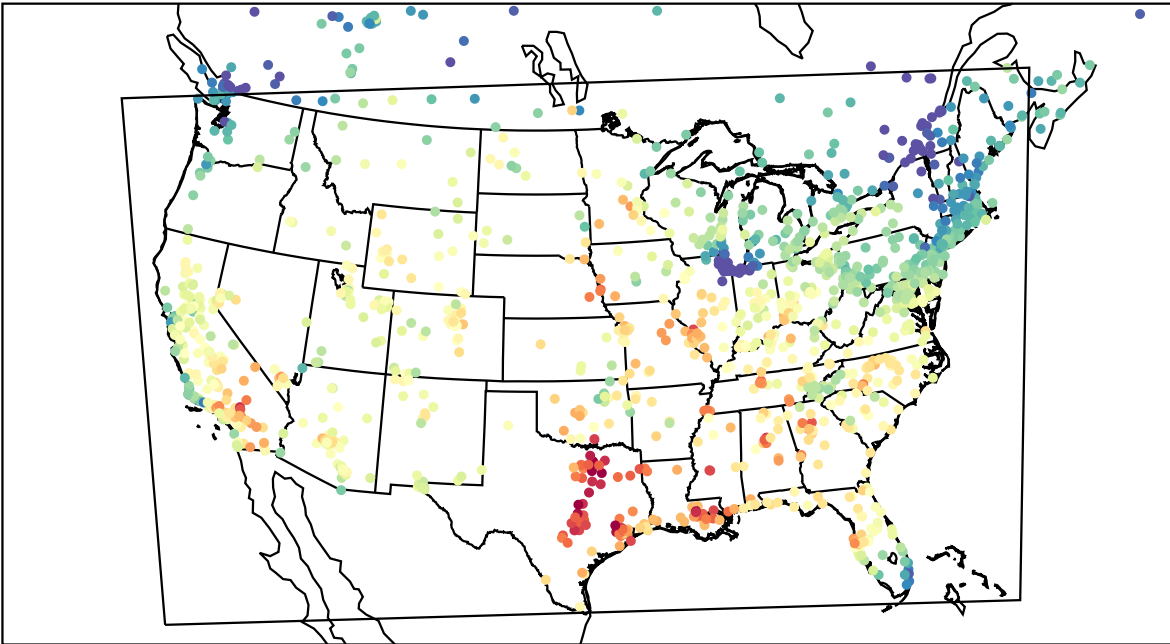
AirNOW (2023-09-19_20:00:00)
