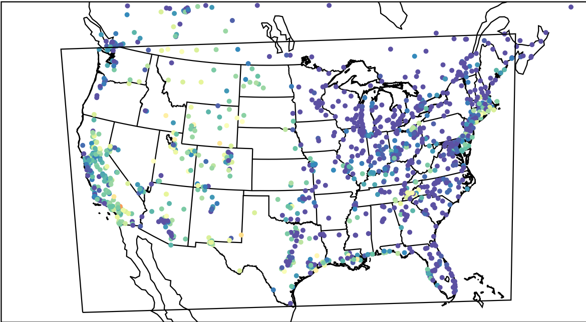
AirNOW (2023-09-18_06:00:00)
