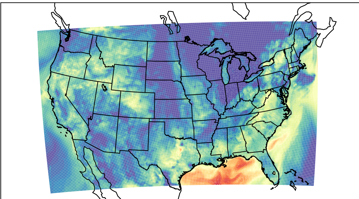
WRF (2023-09-18_13:00:00)
