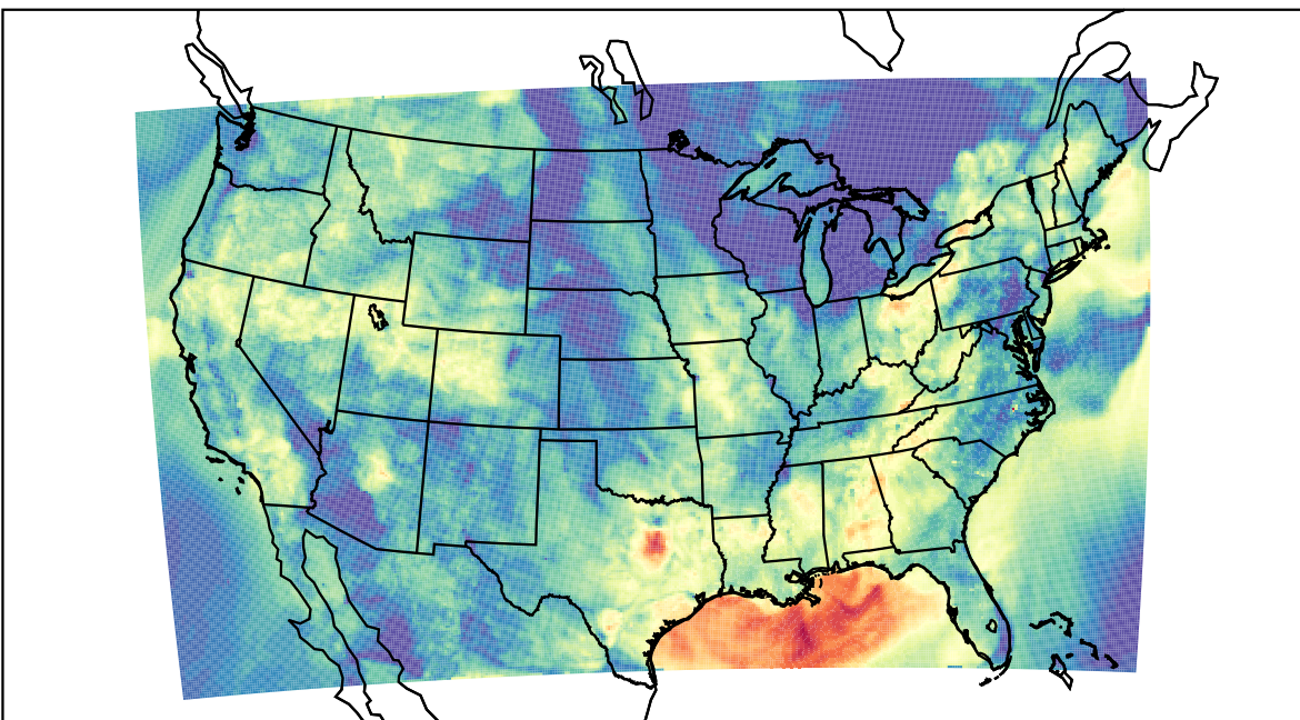
WRF (2023-09-18_05:00:00)
