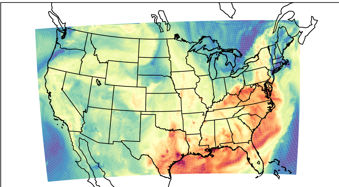
WRF (2023-09-18_19:00:00)
