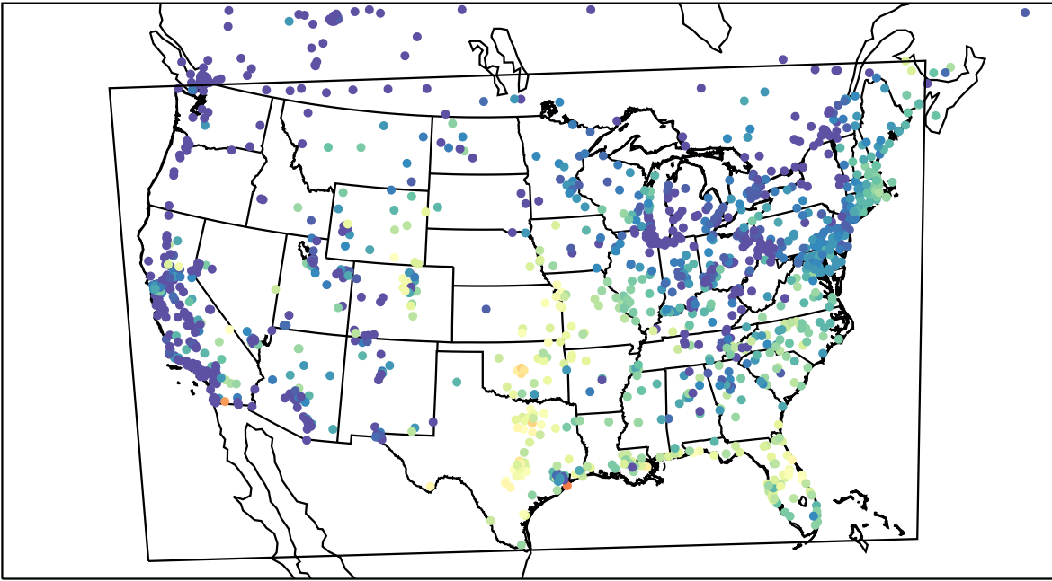
AirNOW (2023-09-19_14:00:00)
