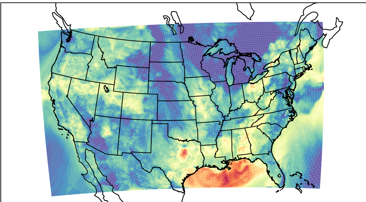
WRF (2023-09-18_06:00:00)
