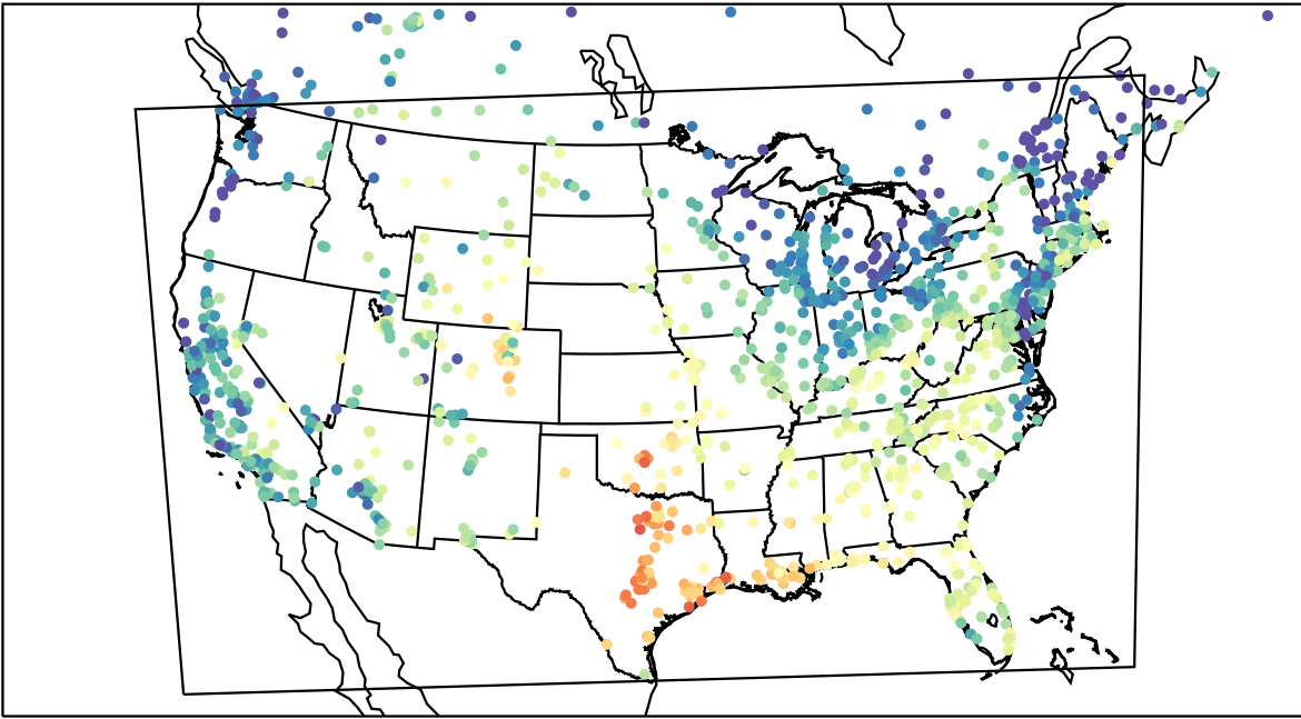
AirNOW (2023-09-18_16:00:00)
