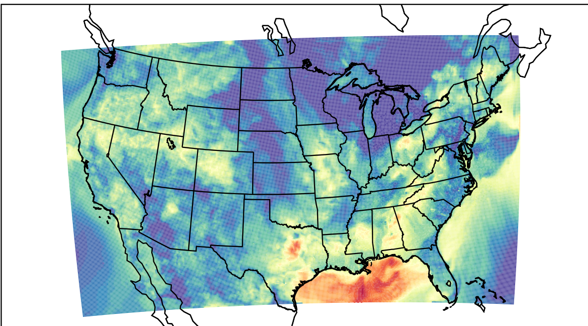
WRF (2023-09-18_08:00:00)
