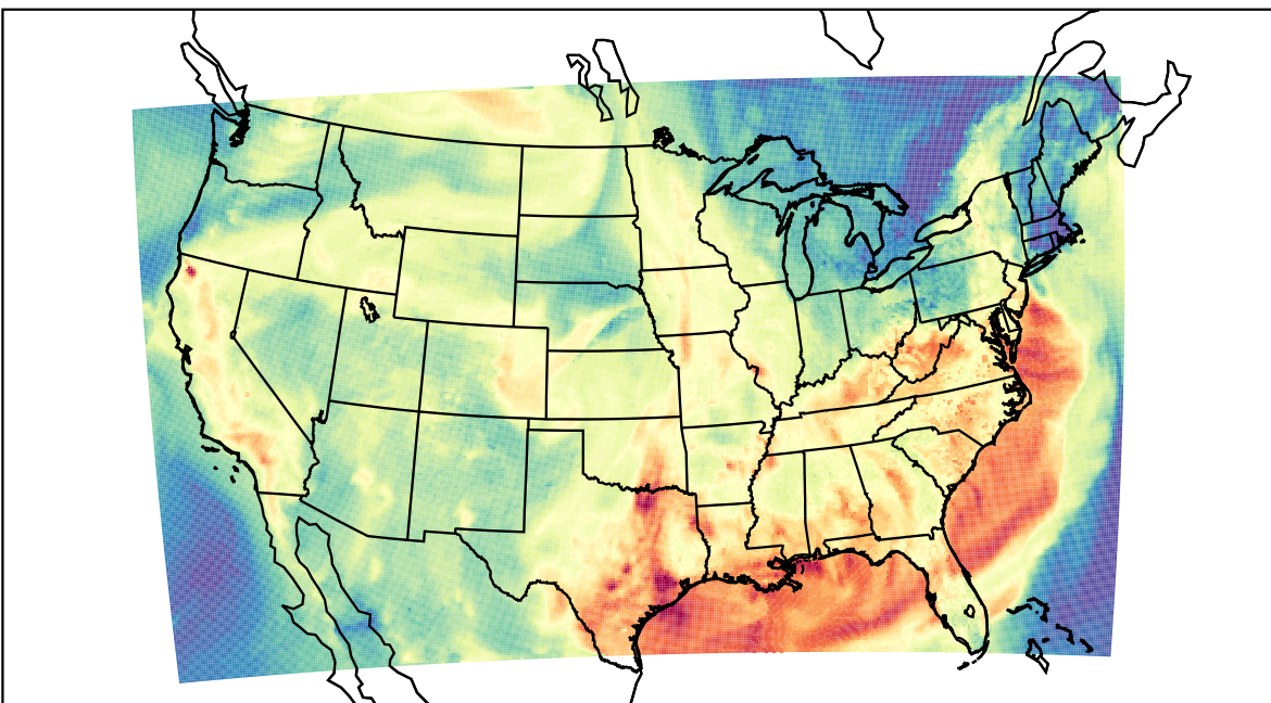
WRF (2023-09-18_22:00:00)
