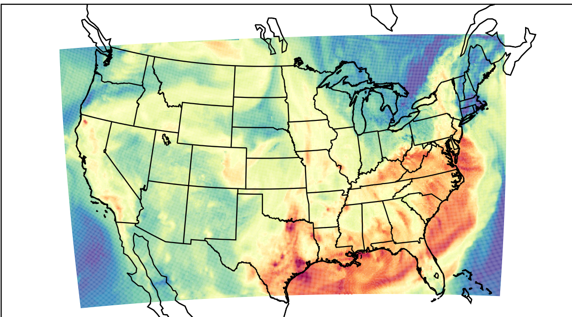
WRF (2023-09-18_21:00:00)
