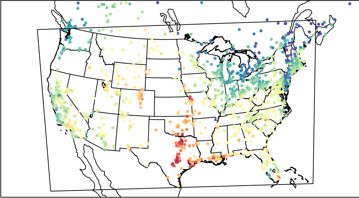
AirNOW (2023-09-18_19:00:00)
