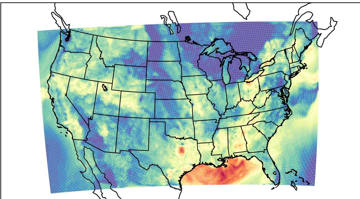
WRF (2023-09-18_04:00:00)
