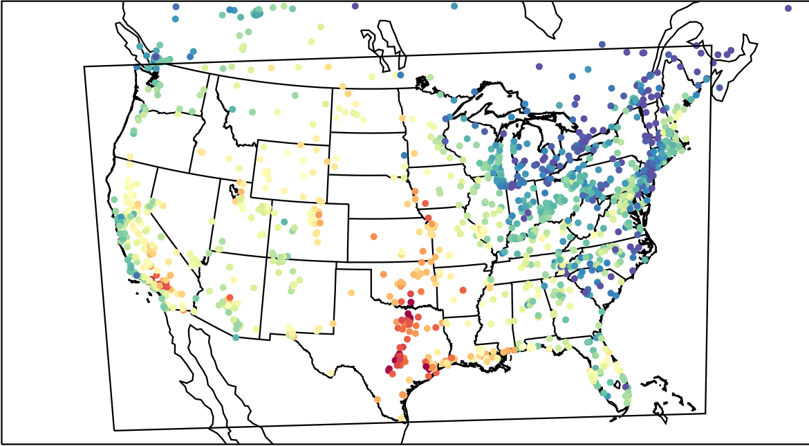
AirNOW (2023-09-18_23:00:00)
