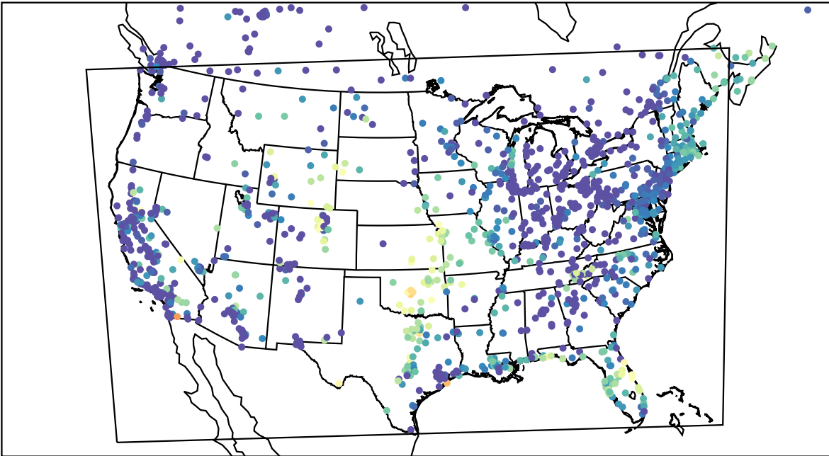
AirNOW (2023-09-19_13:00:00)
