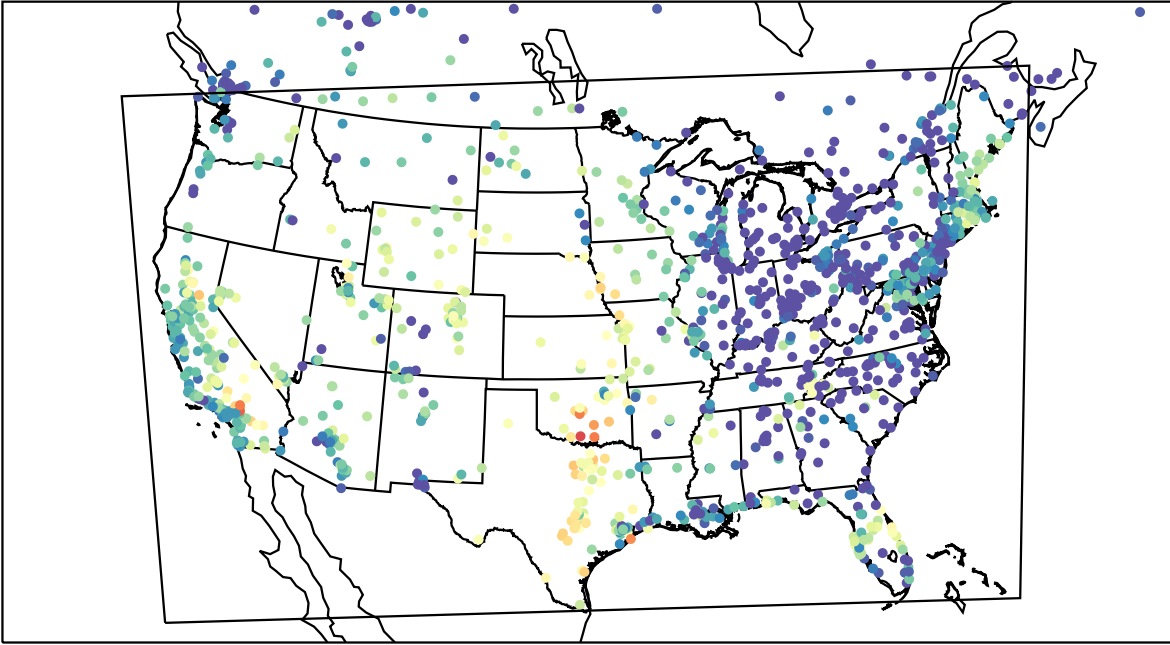
AirNOW (2023-09-19_03:00:00)
