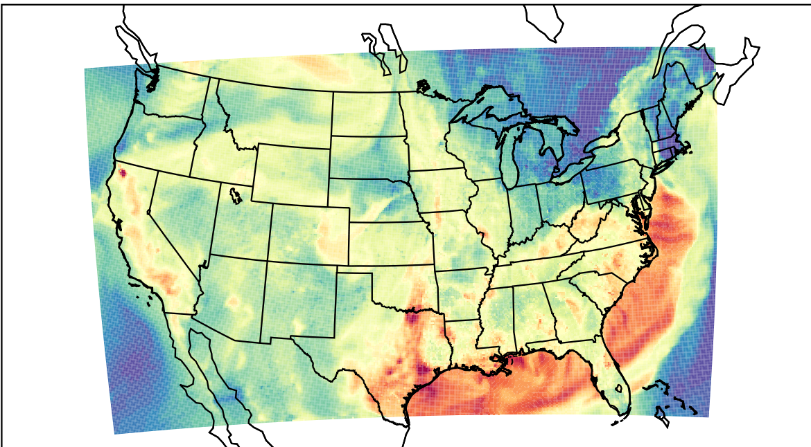
WRF (2023-09-18_23:00:00)
