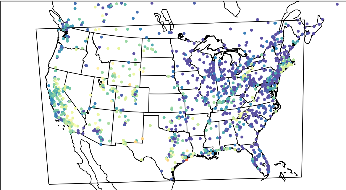
AirNOW (2023-09-18_04:00:00)
