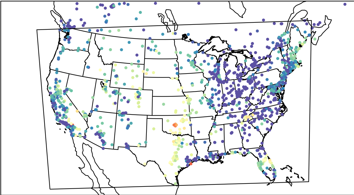
AirNOW (2023-09-19_06:00:00)
