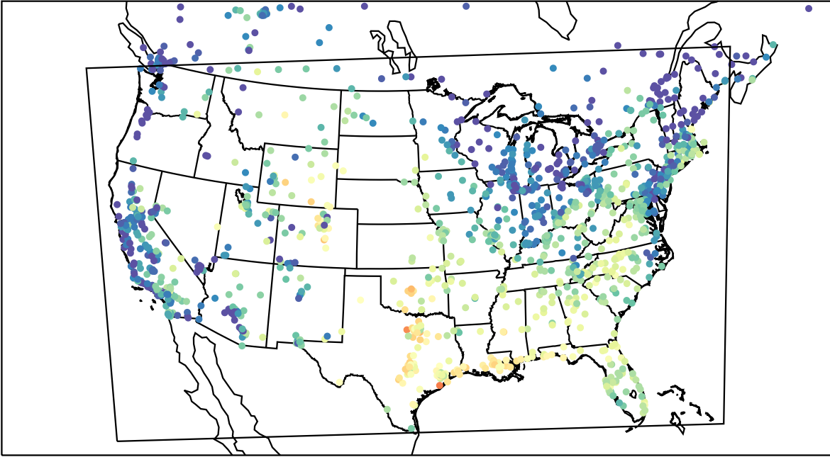
AirNOW (2023-09-18_15:00:00)
