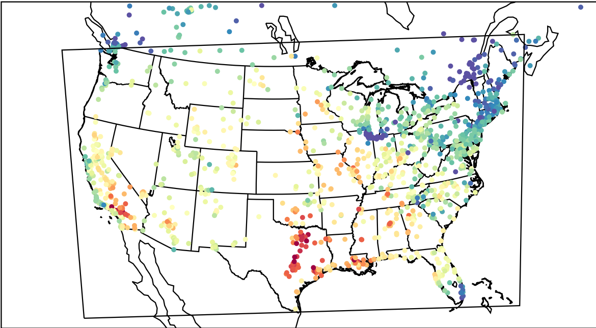
AirNOW (2023-09-19_22:00:00)
