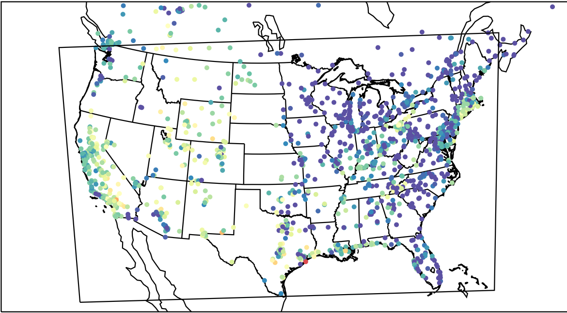
AirNOW (2023-09-18_03:00:00)
