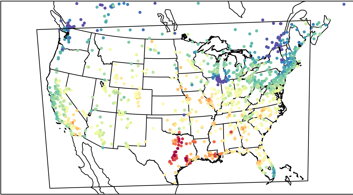
AirNOW (2023-09-19_18:00:00)
