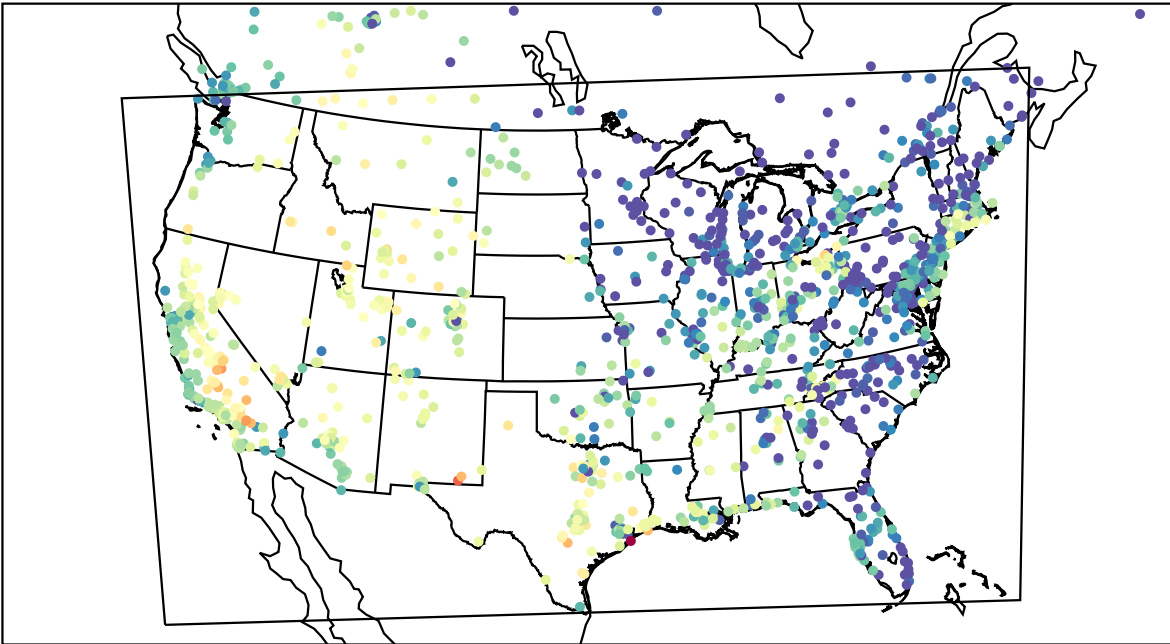
AirNOW (2023-09-18_01:00:00)
