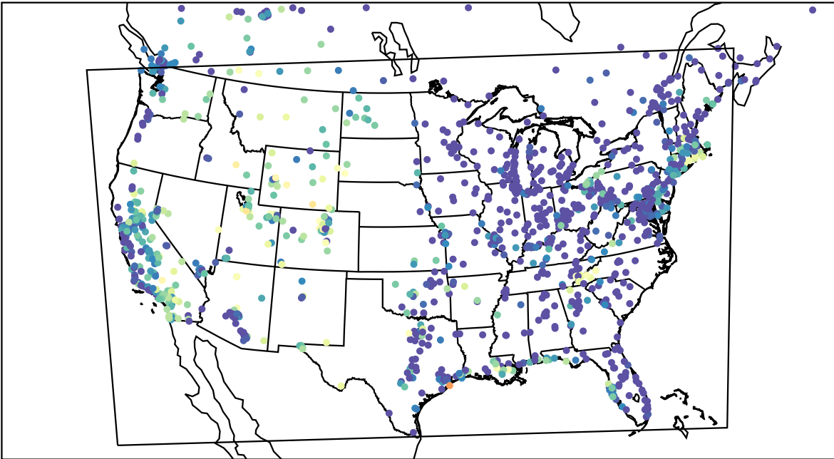
AirNOW (2023-09-18_08:00:00)
