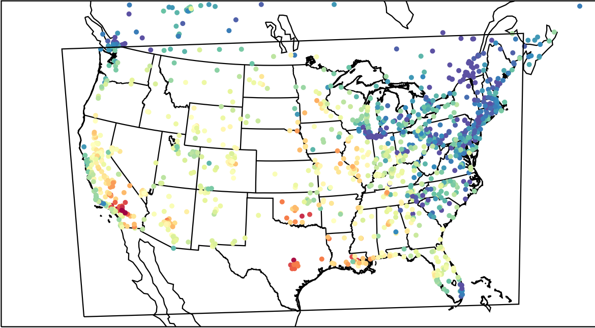
AirNOW (2023-09-19_23:00:00)
