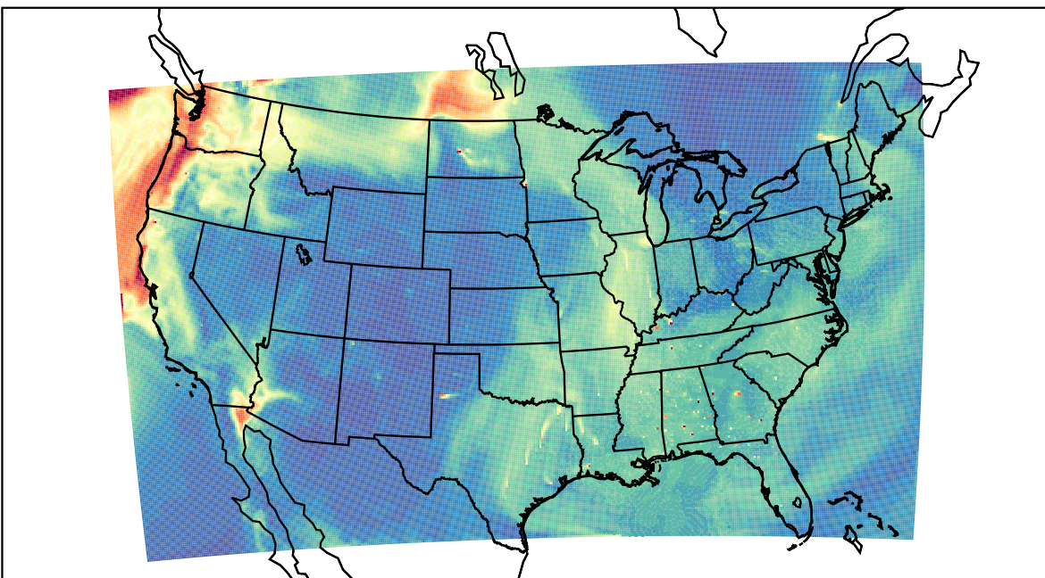
WRF 2023-09-19_17:00:00
