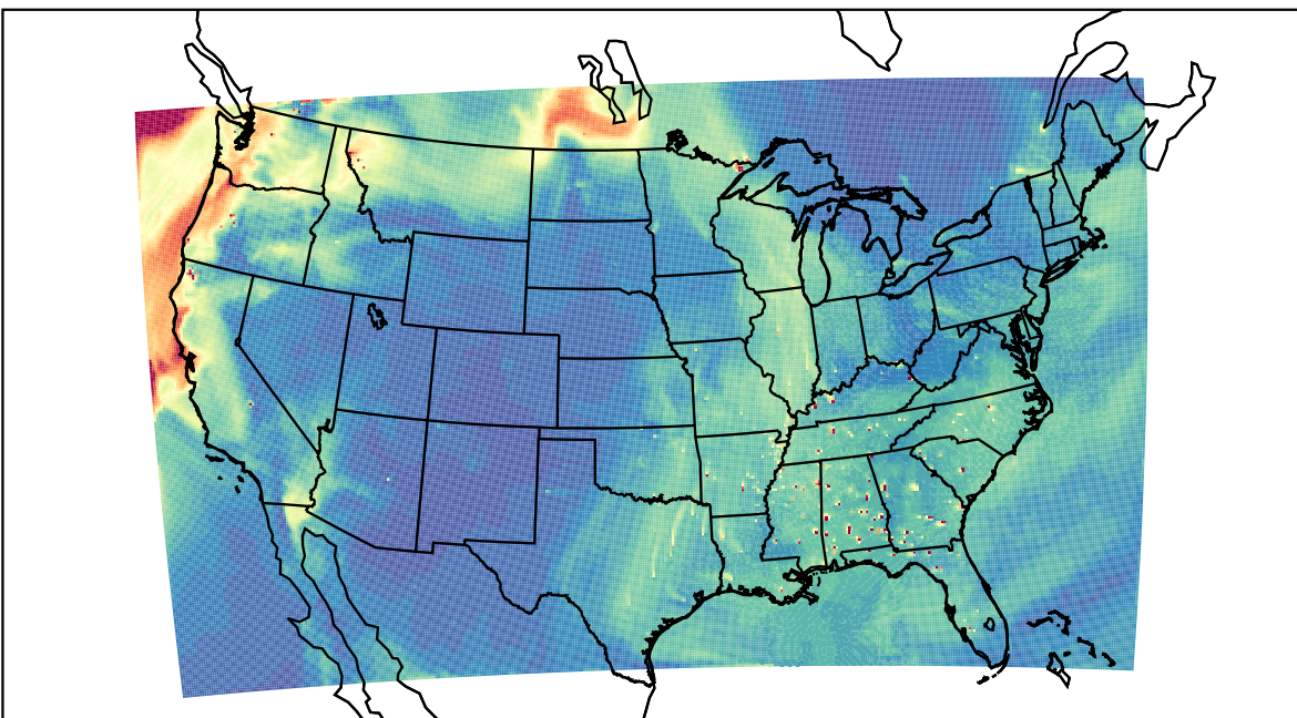
WRF 2023-09-19_20:00:00
