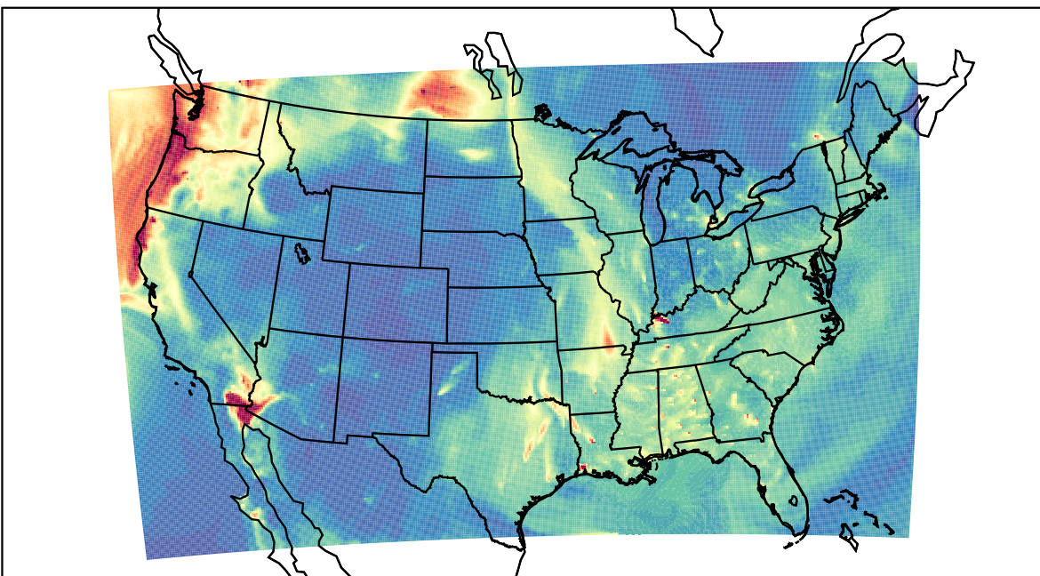
WRF 2023-09-19_12:00:00
