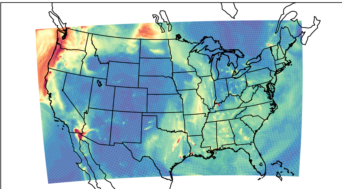
WRF 2023-09-19_14:00:00
