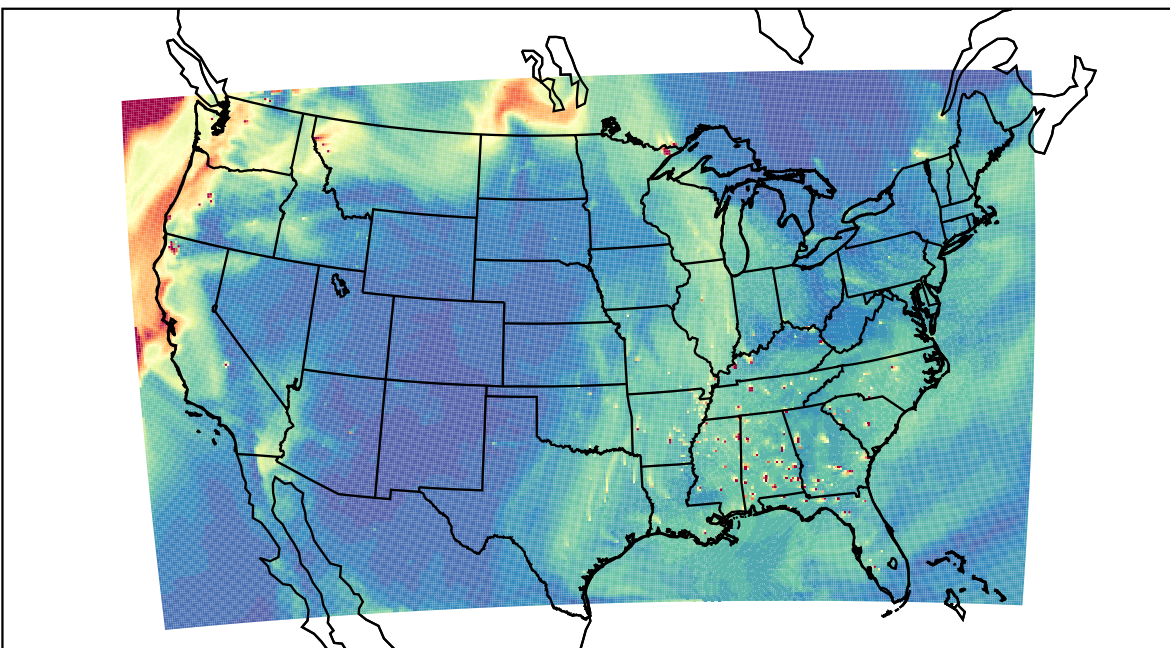
WRF 2023-09-19_21:00:00
