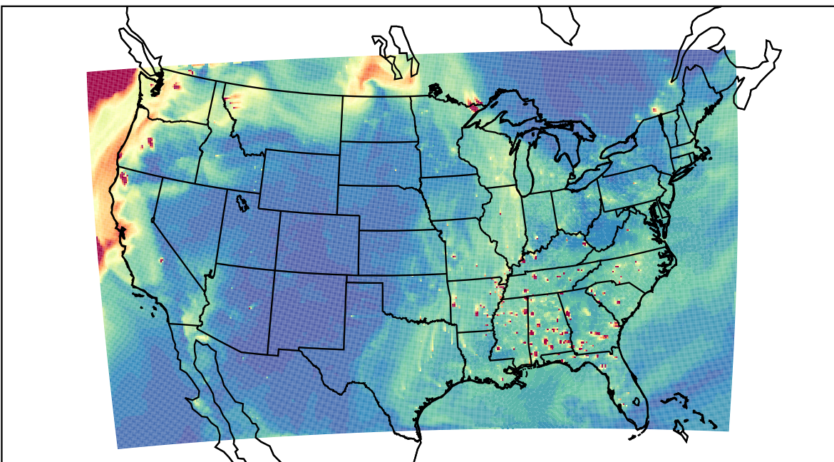
WRF 2023-09-19_23:00:00
