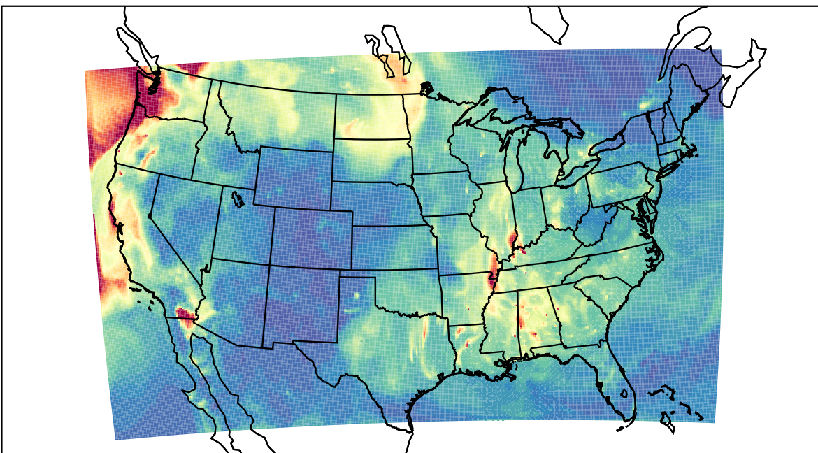
WRF 2023-09-20_12:00:00
