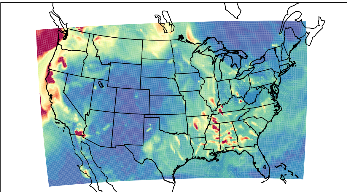
WRF 2023-09-20_05:00:00
