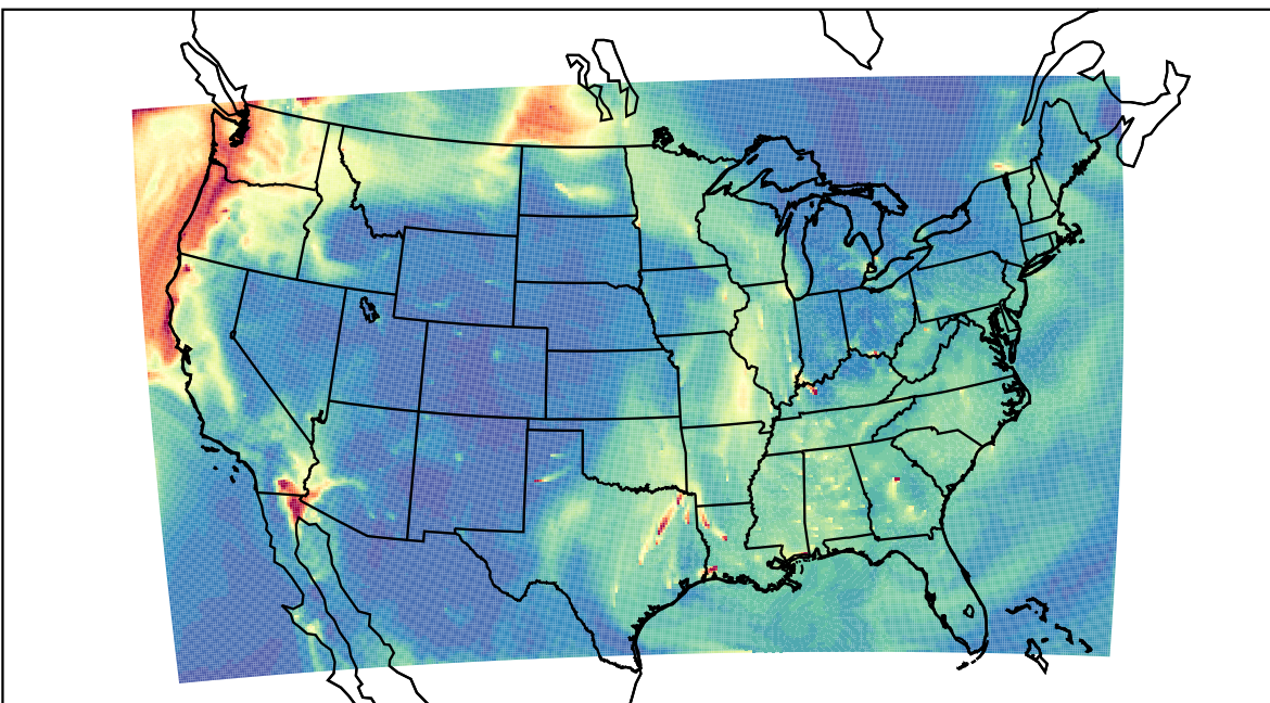
WRF 2023-09-19_15:00:00
