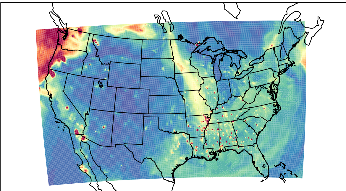
WRF 2023-09-19_02:00:00
