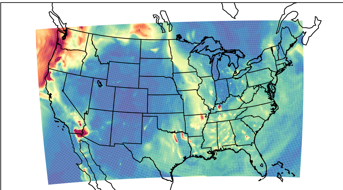
WRF 2023-09-19_08:00:00
