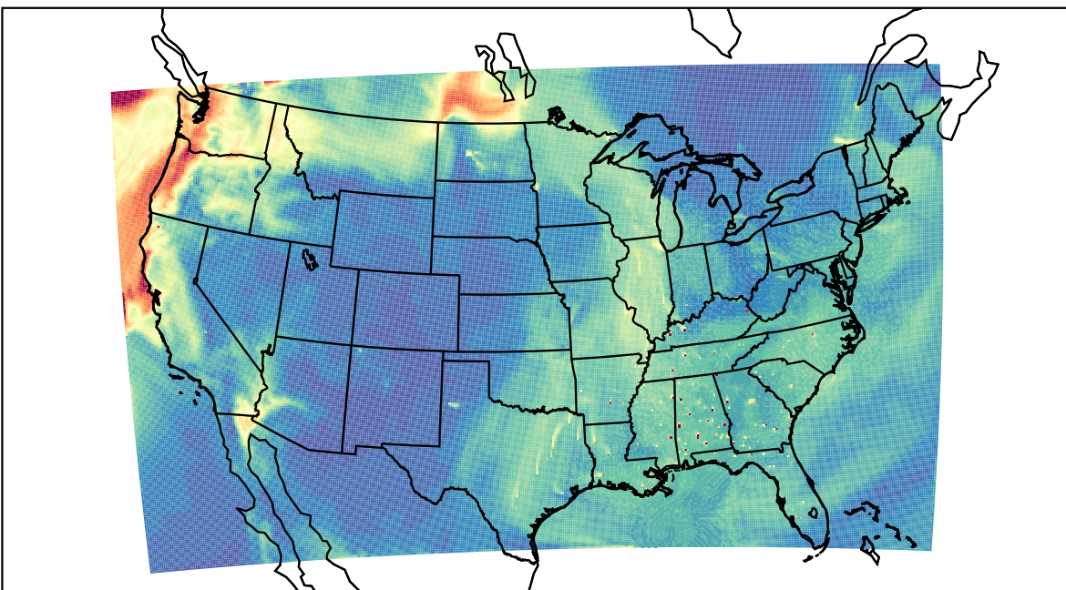
WRF 2023-09-19_18:00:00
