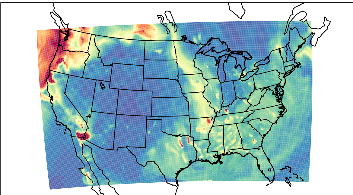
WRF 2023-09-19_07:00:00
