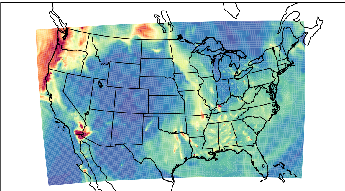
WRF 2023-09-19_10:00:00
