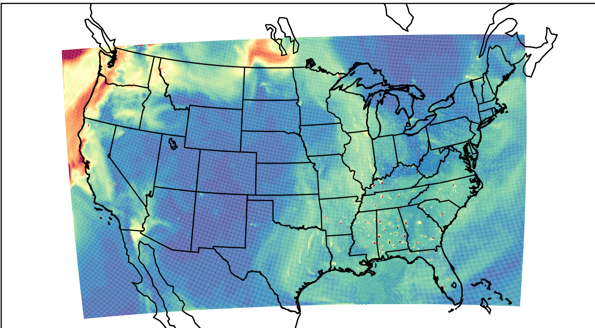
WRF 2023-09-19_19:00:00
