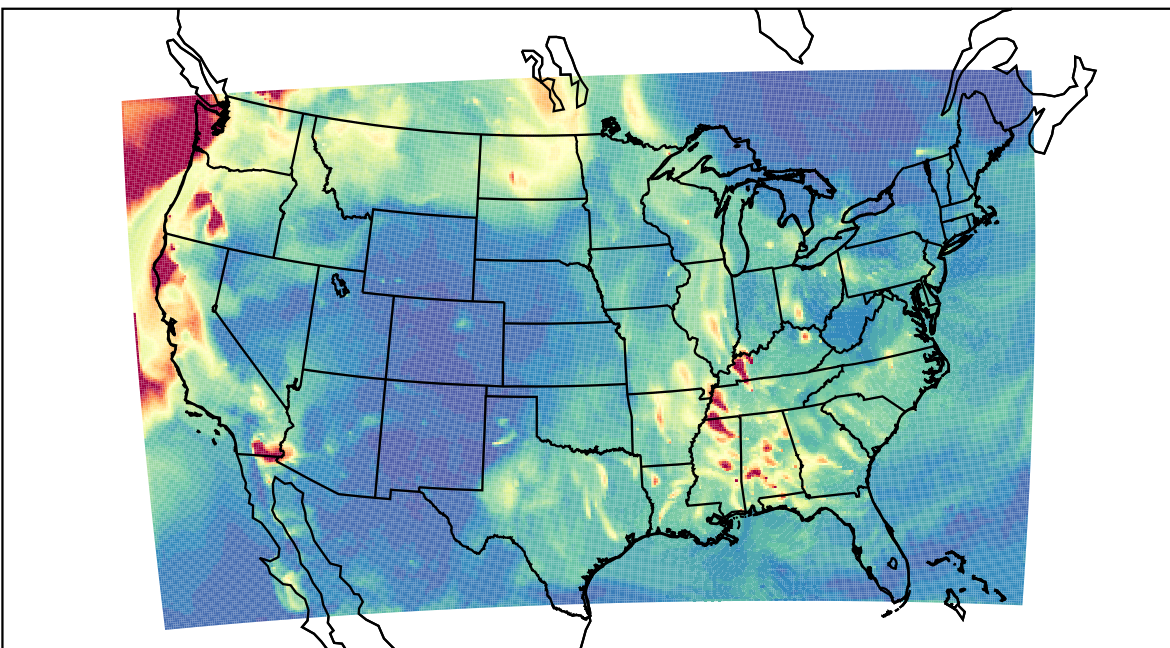
WRF 2023-09-20_07:00:00
