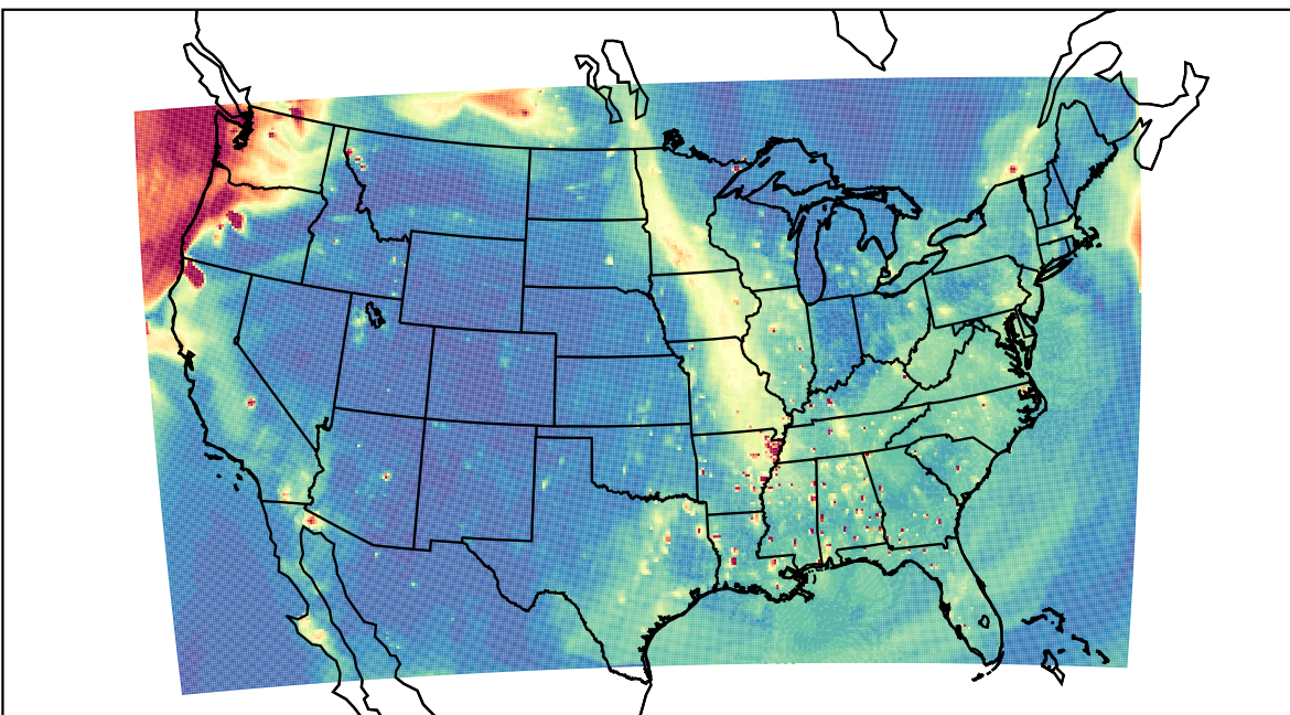
WRF 2023-09-19_01:00:00
