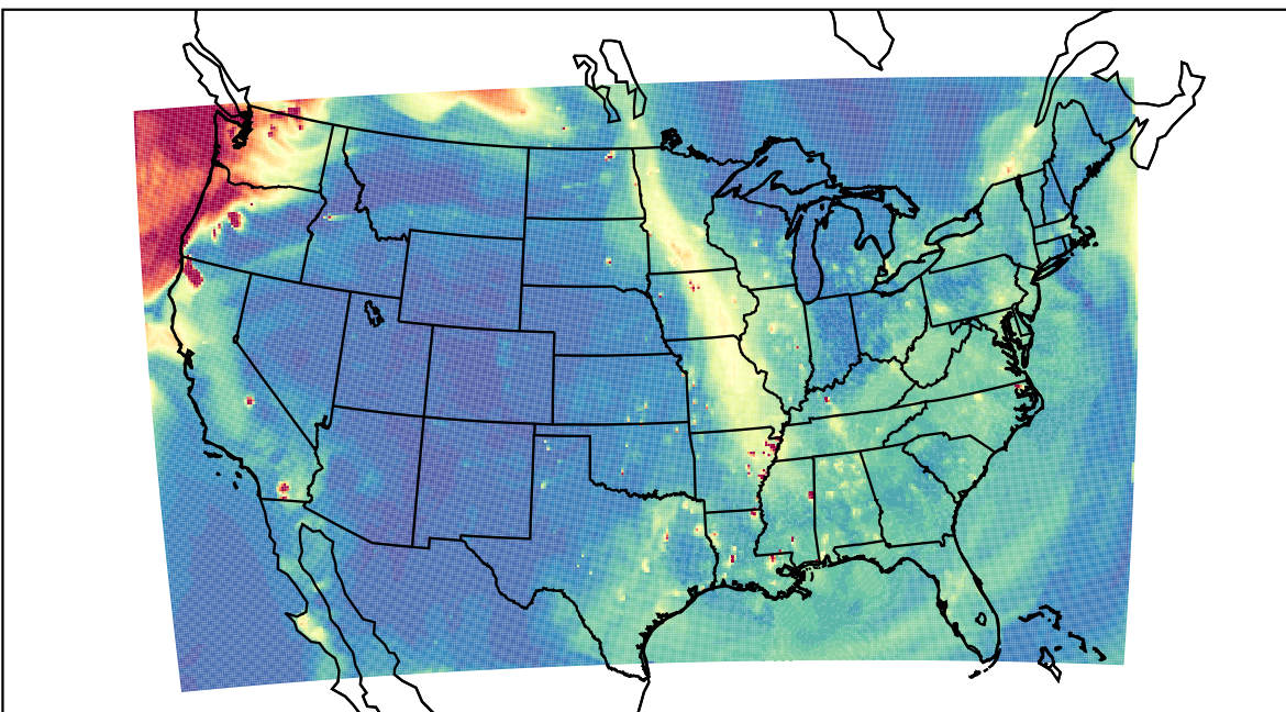
WRF 2023-09-19_00:00:00
