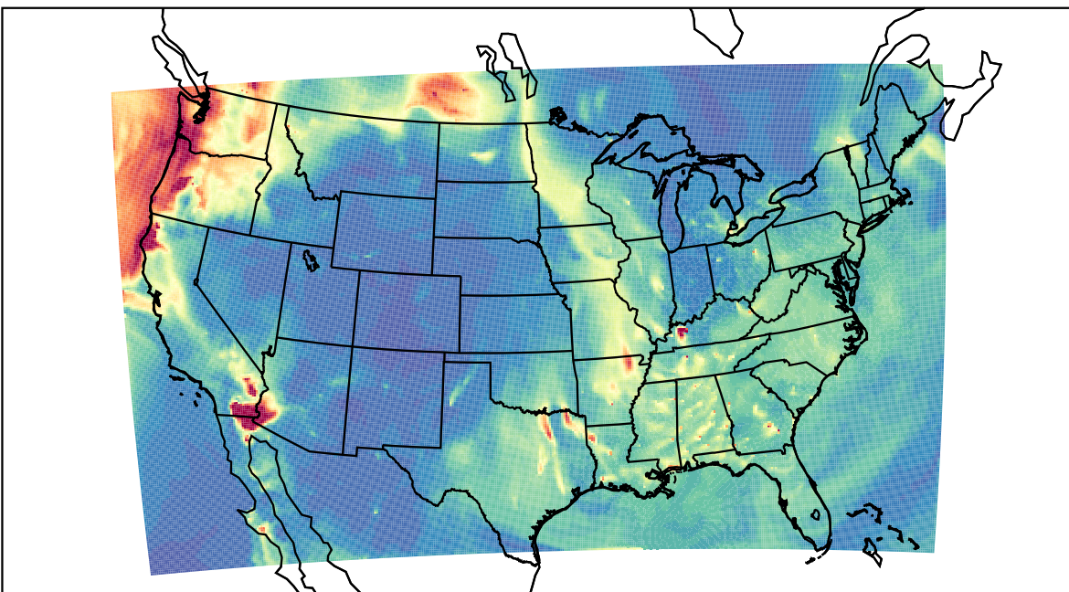
WRF 2023-09-19_09:00:00
