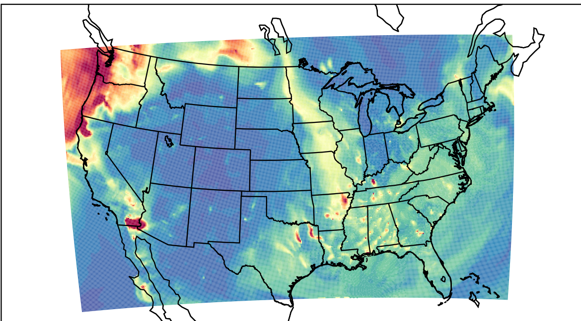
WRF 2023-09-19_06:00:00
