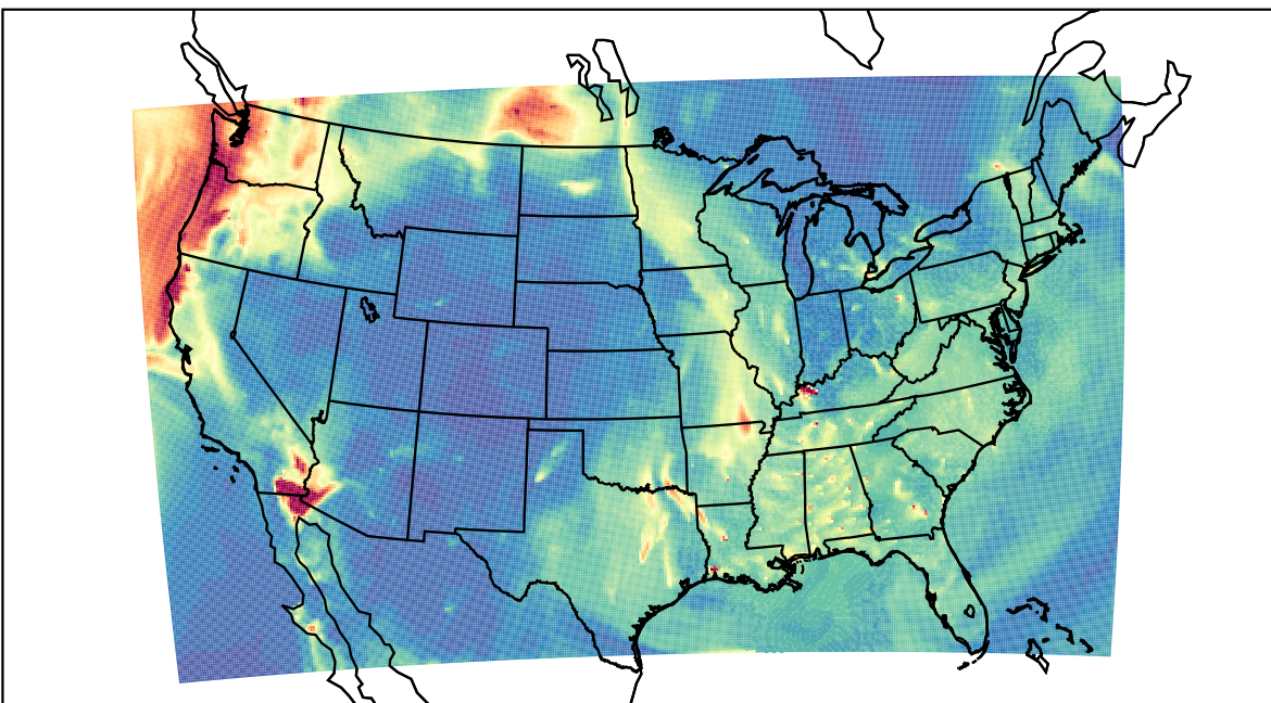
WRF 2023-09-19_11:00:00
