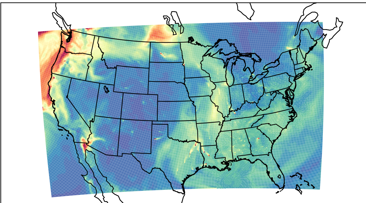
WRF 2023-09-19_16:00:00
