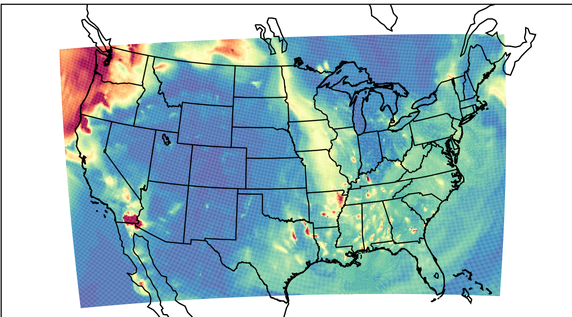
WRF 2023-09-19_05:00:00
