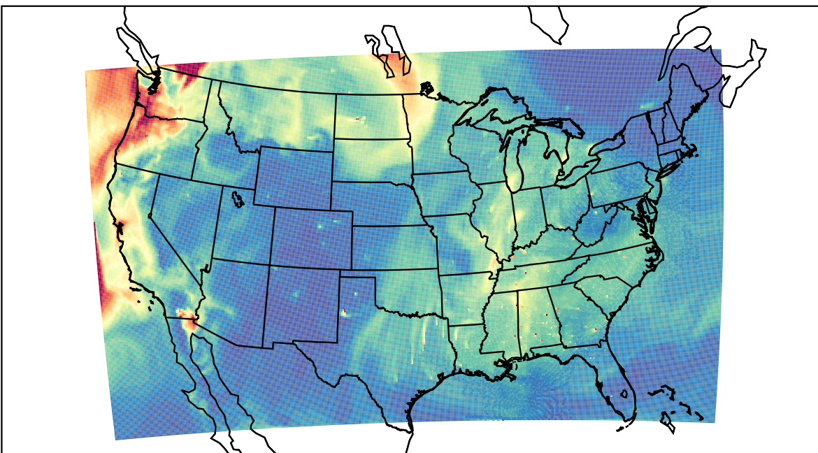
WRF 2023-09-20_17:00:00
