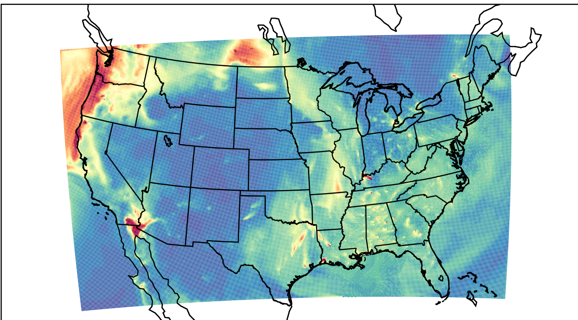
WRF 2023-09-19_13:00:00
