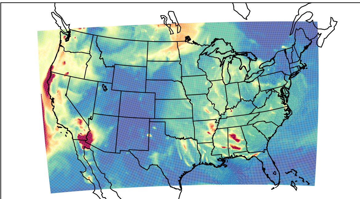
WRF 2023-09-21_05:00:00
