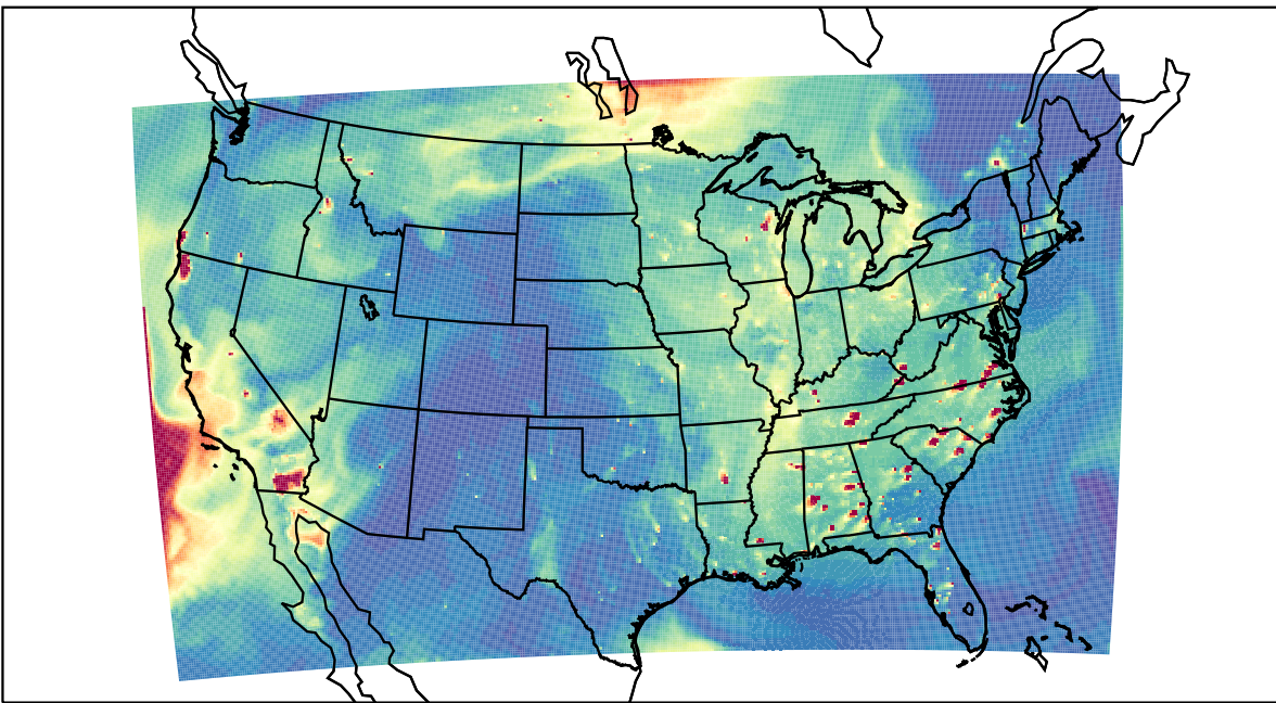
WRF 2023-09-22_00:00:00
