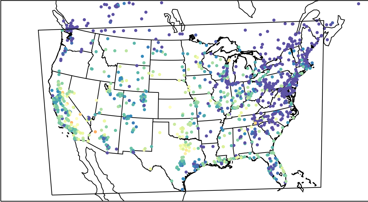
AirNOW (2023-09-21_05:00:00)
