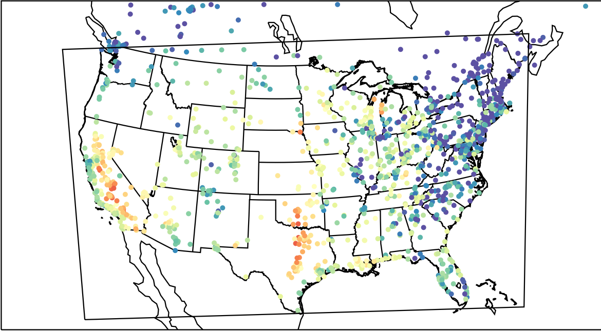
AirNOW (2023-09-21_00:00:00)
