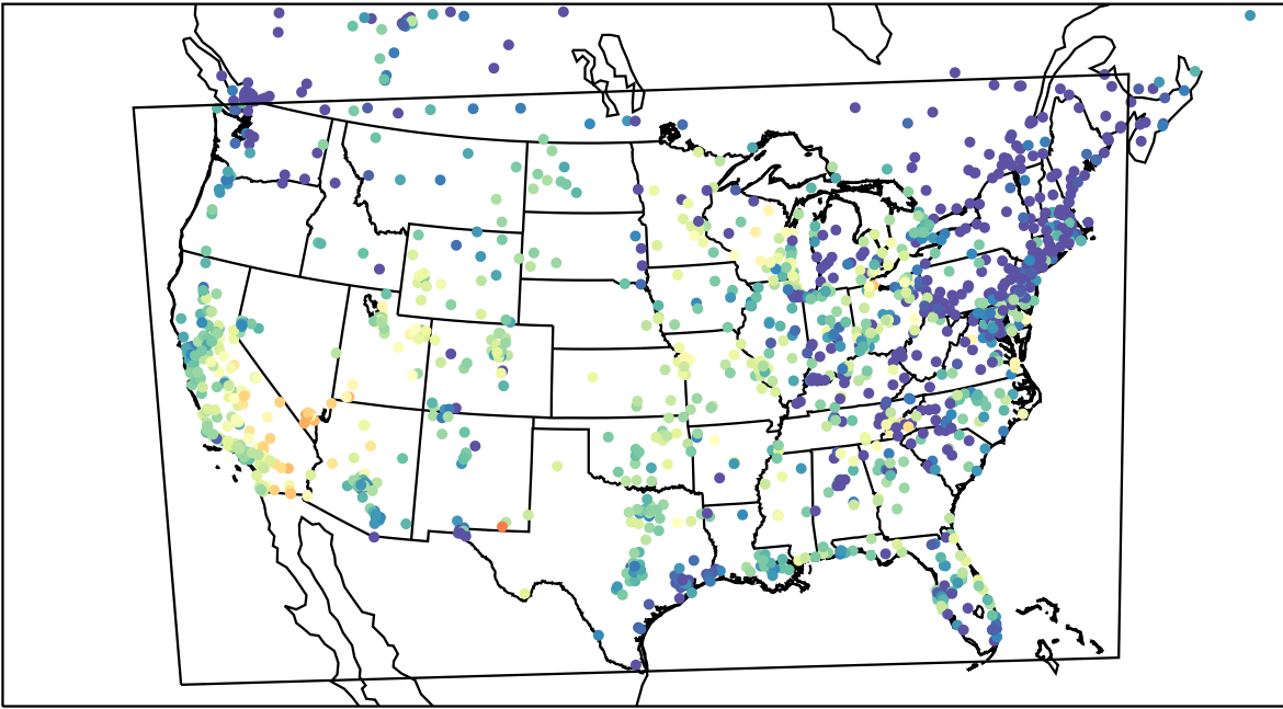
AirNOW (2023-09-22_02:00:00)
