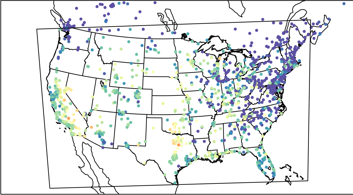
AirNOW (2023-09-21_03:00:00)
