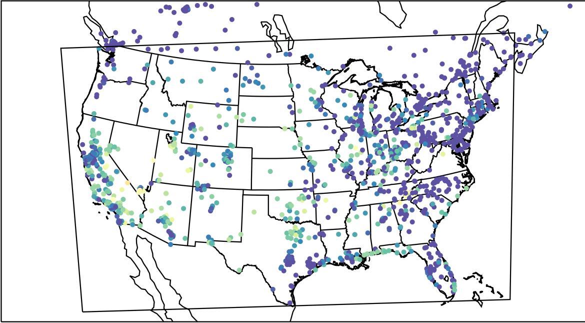
AirNOW (2023-09-21_09:00:00)
