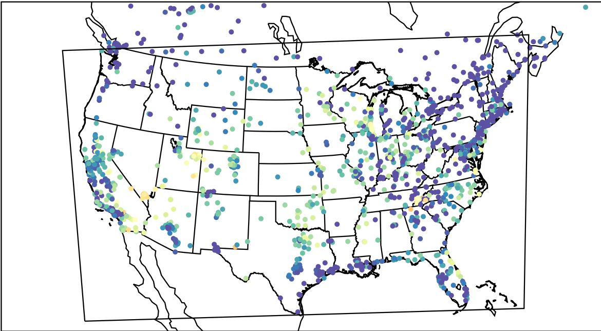
AirNOW (2023-09-22_06:00:00)
