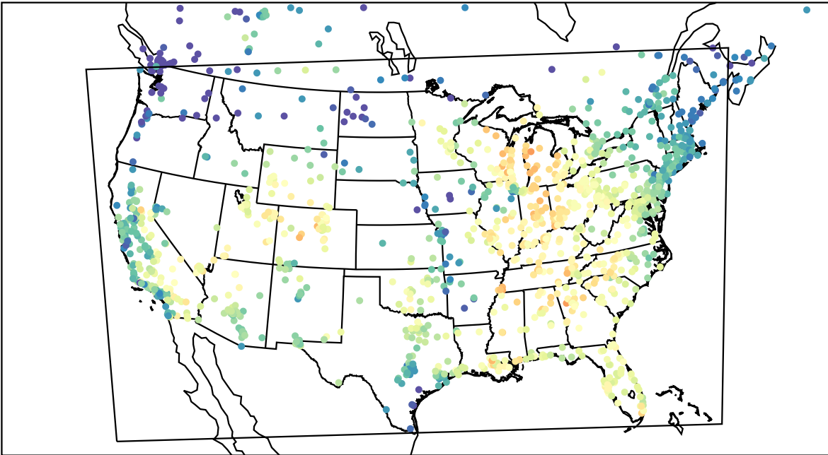
AirNOW (2023-09-22_17:00:00)
