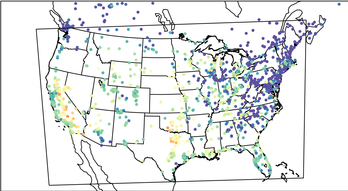
AirNOW (2023-09-21_02:00:00)
