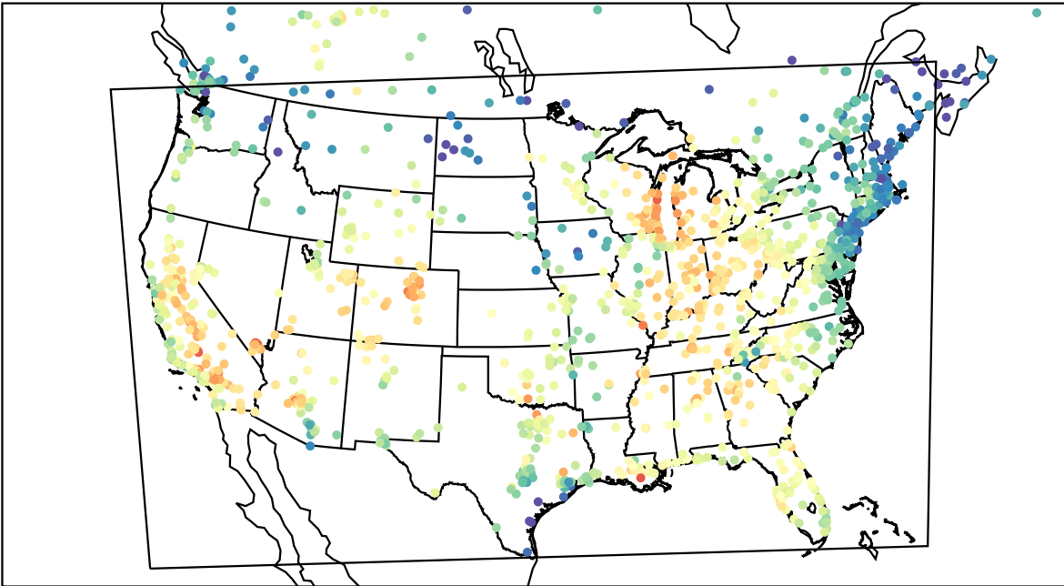
AirNOW (2023-09-22_21:00:00)
