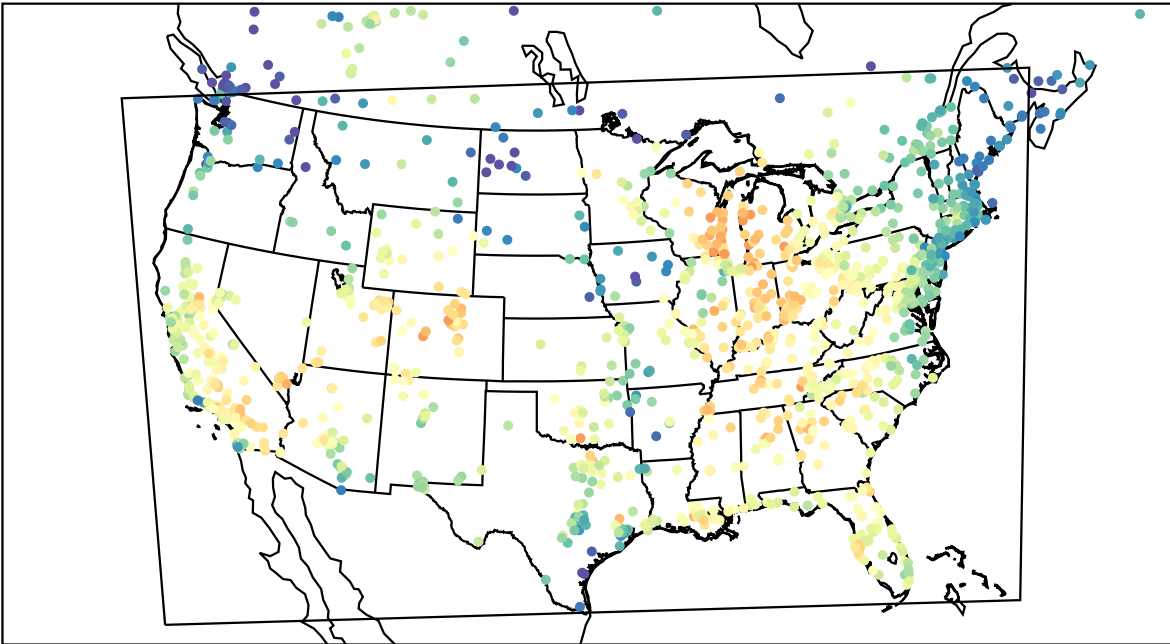
AirNOW (2023-09-22_19:00:00)
