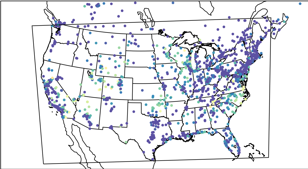
AirNOW (2023-09-22_12:00:00)
