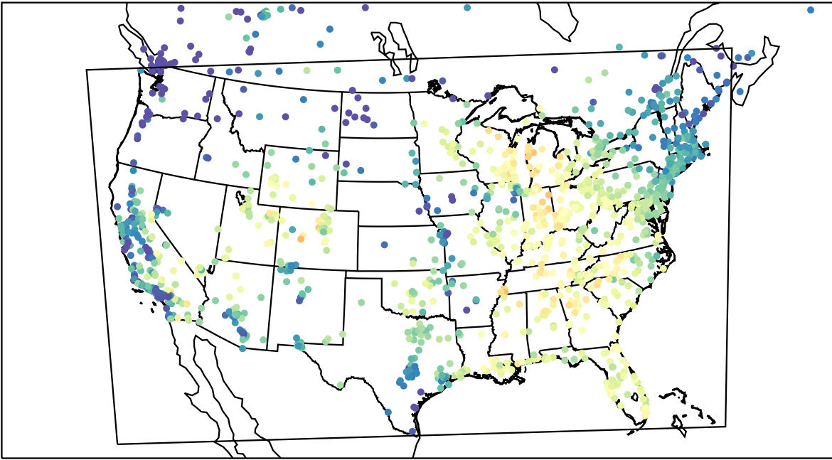
AirNOW (2023-09-22_16:00:00)
