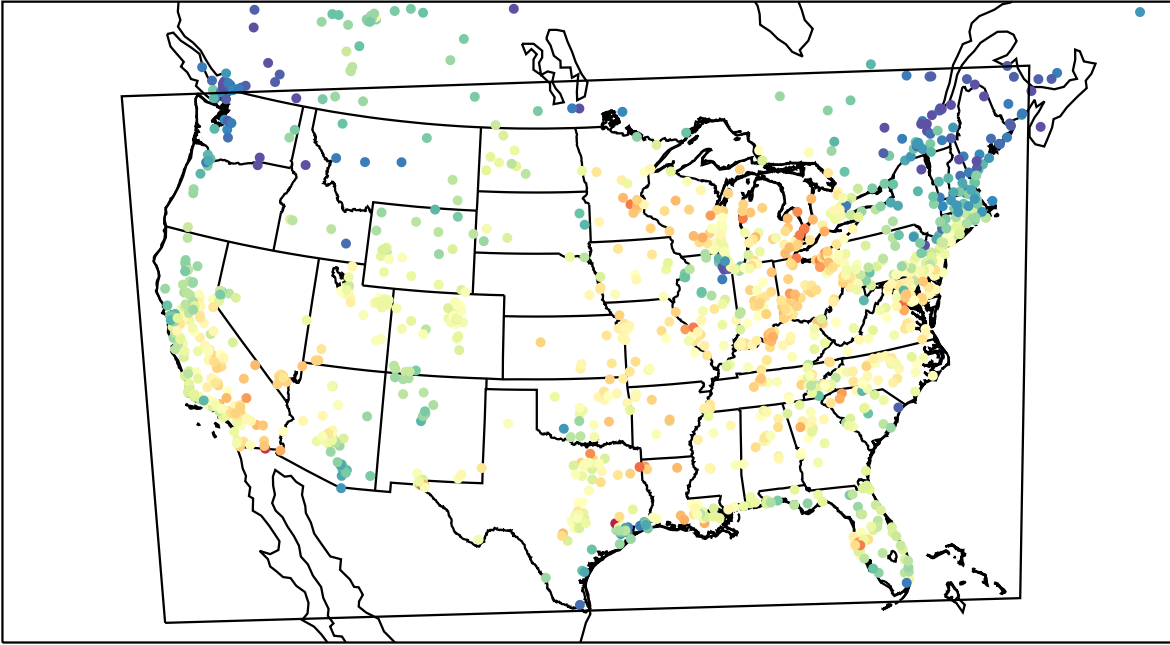
AirNOW (2023-09-21_21:00:00)
