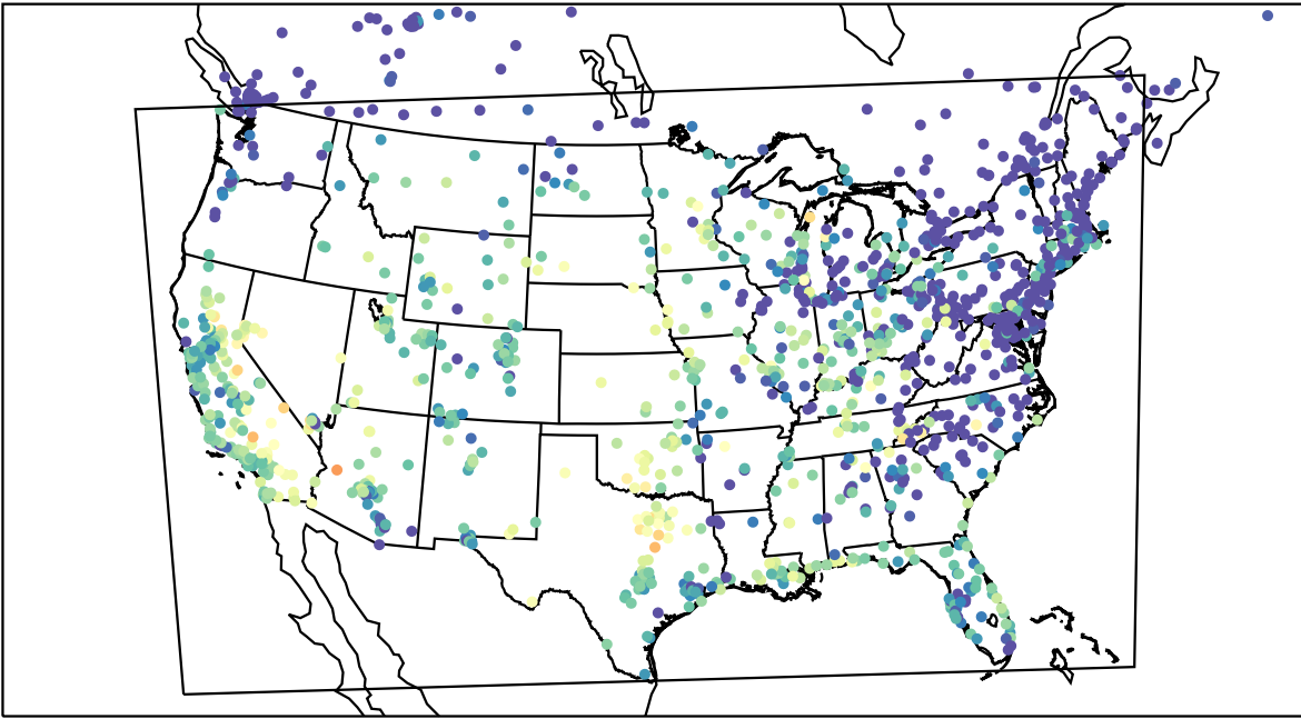
AirNOW (2023-09-21_04:00:00)
