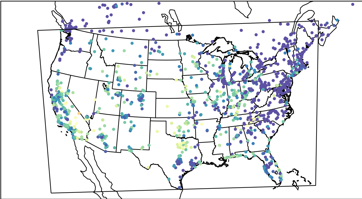
AirNOW (2023-09-21_07:00:00)
