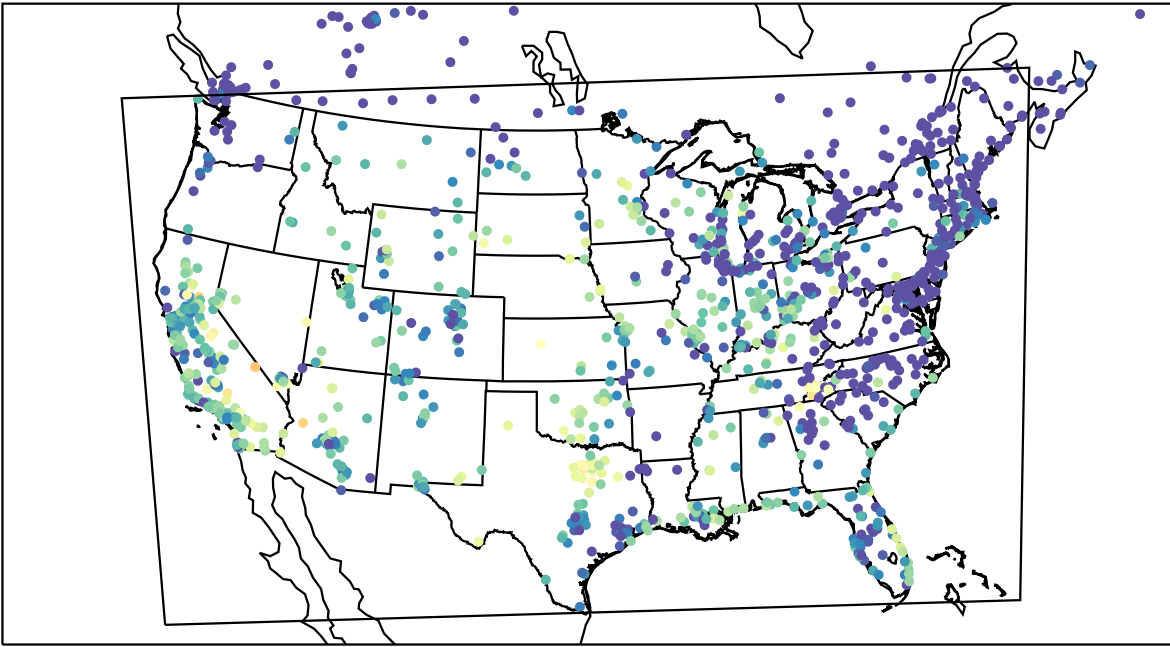
AirNOW (2023-09-21_06:00:00)
