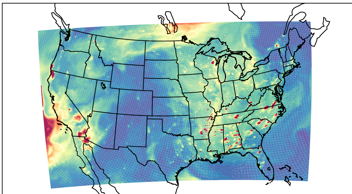
WRF 2023-09-22_01:00:00
