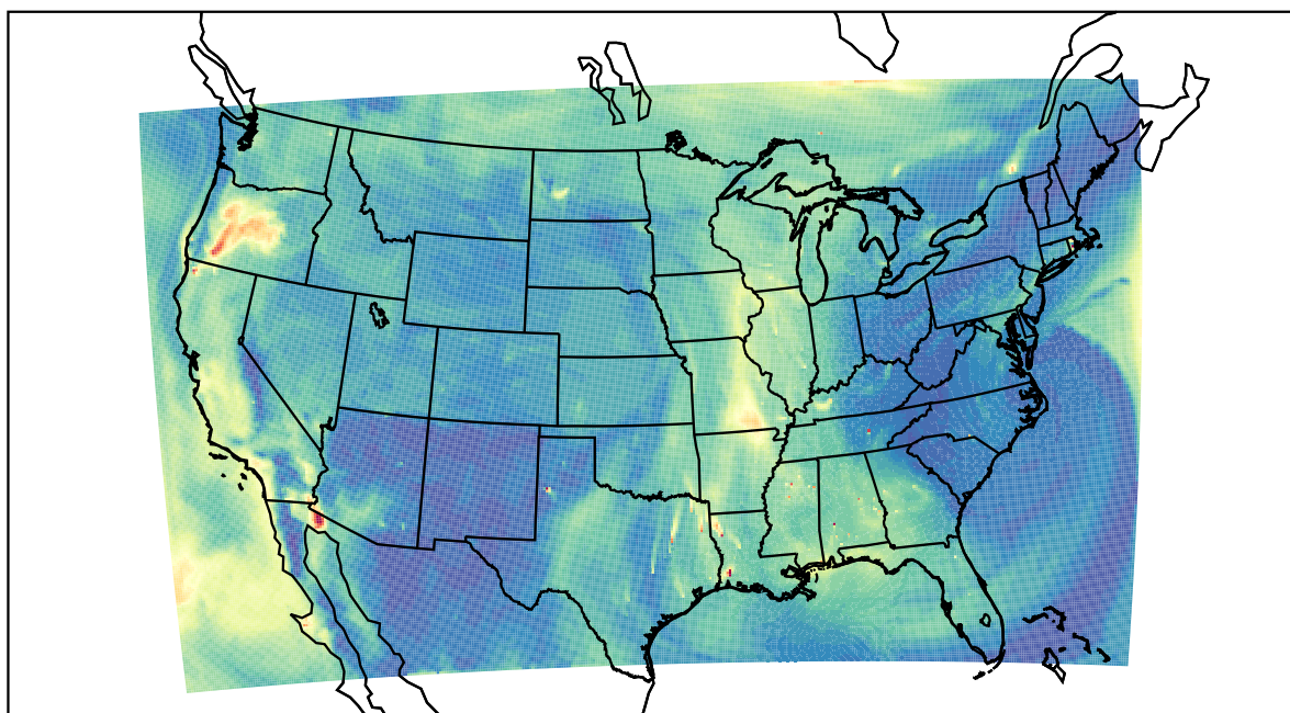
WRF 2023-09-23_17:00:00
