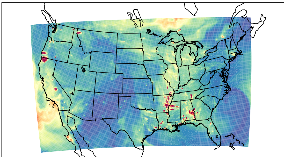
WRF 2023-09-23_02:00:00
