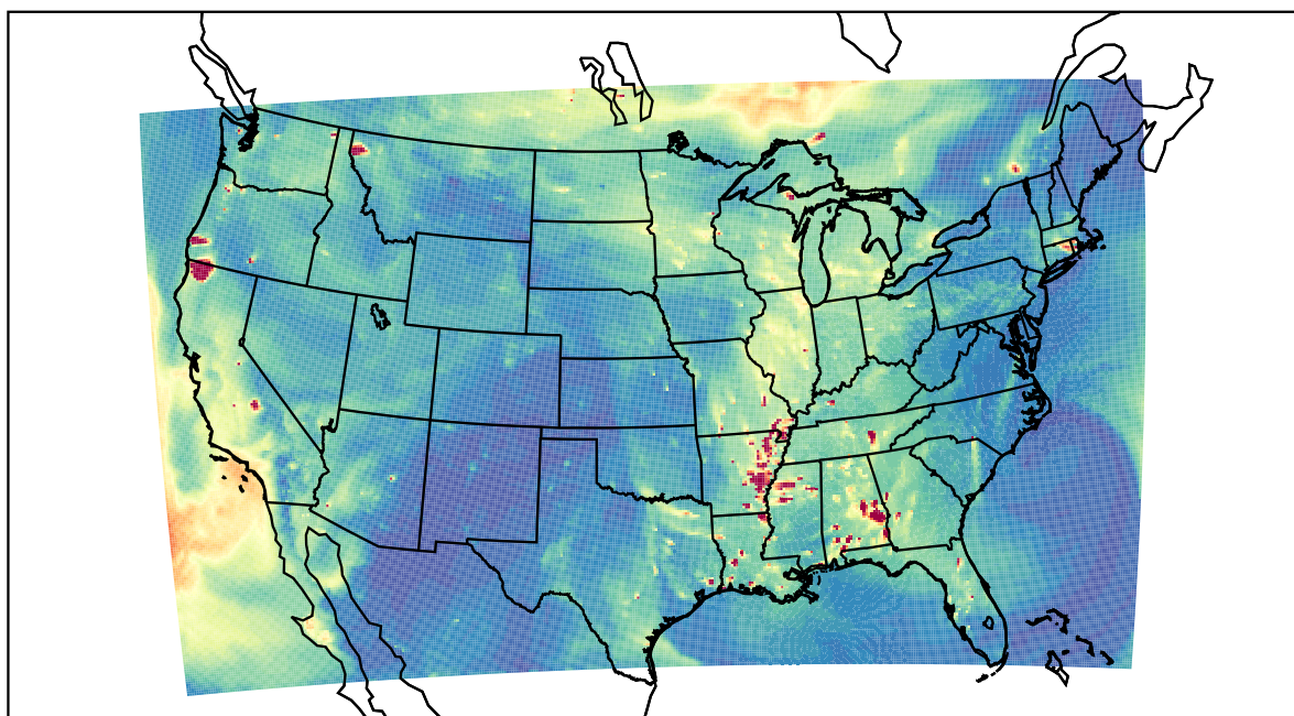
WRF 2023-09-23_01:00:00
