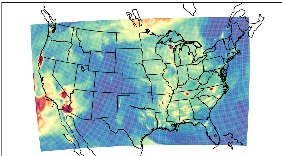
WRF 2023-09-22_05:00:00
