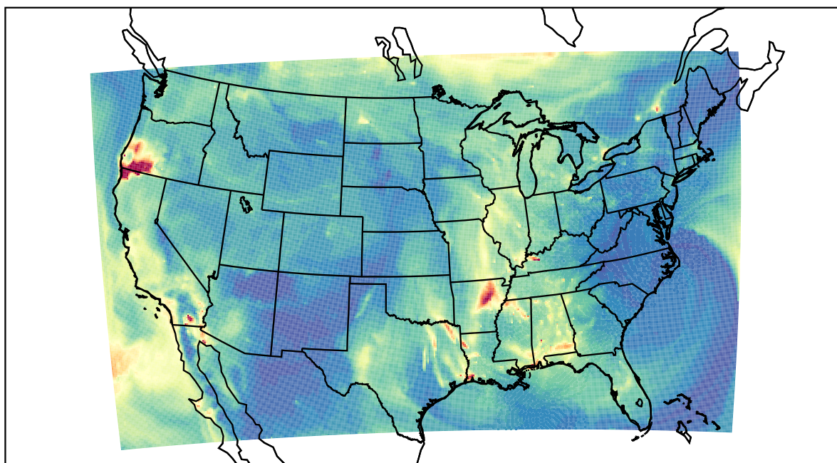
WRF 2023-09-23_11:00:00
