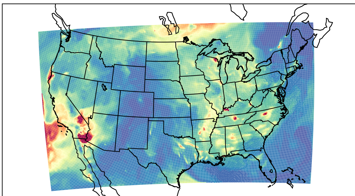
WRF 2023-09-22_06:00:00
