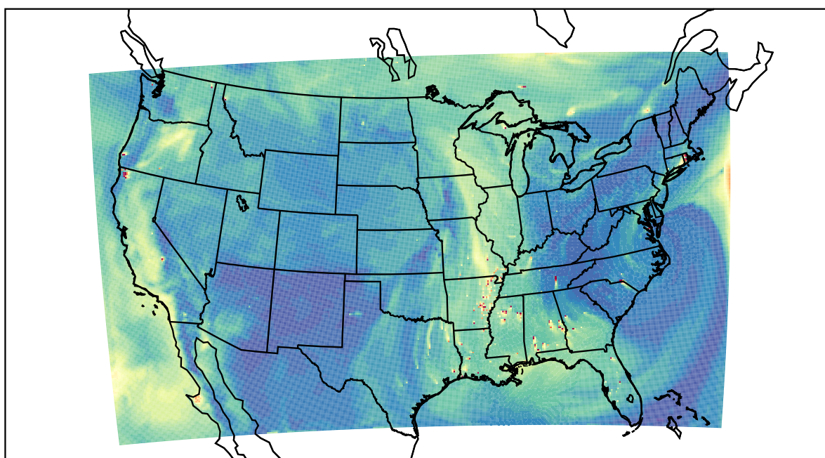
WRF 2023-09-23_21:00:00
