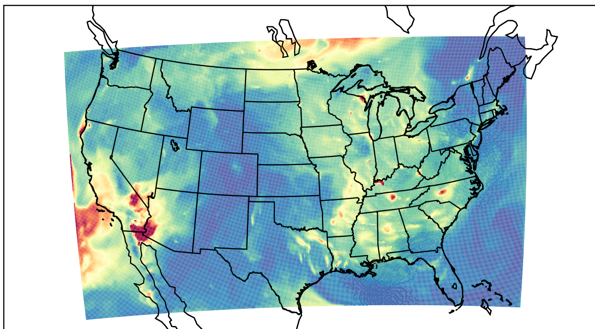
WRF 2023-09-22_07:00:00
