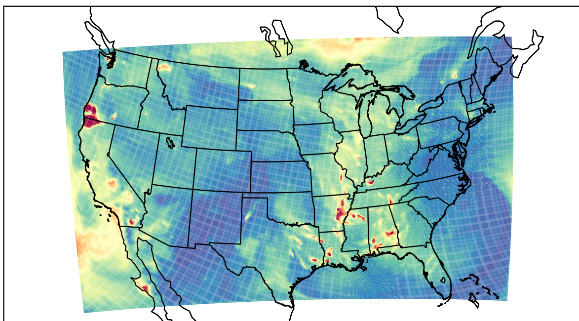
WRF 2023-09-23_05:00:00
