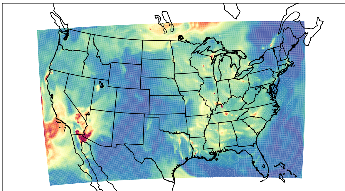
WRF 2023-09-22_09:00:00
