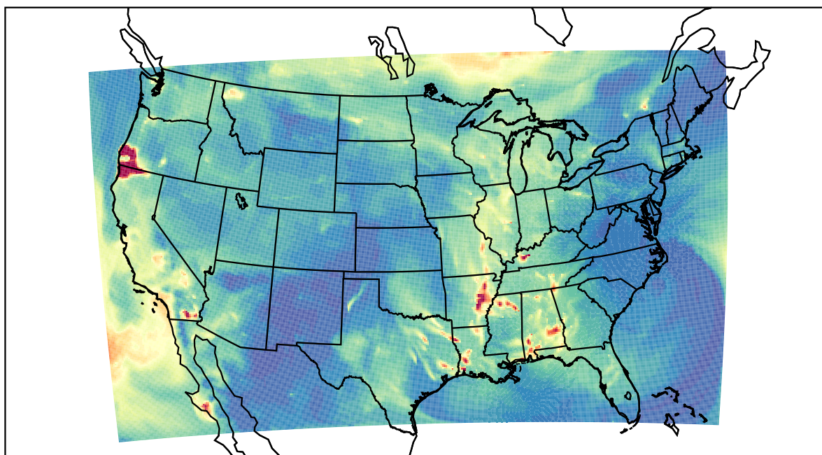
WRF 2023-09-23_06:00:00
