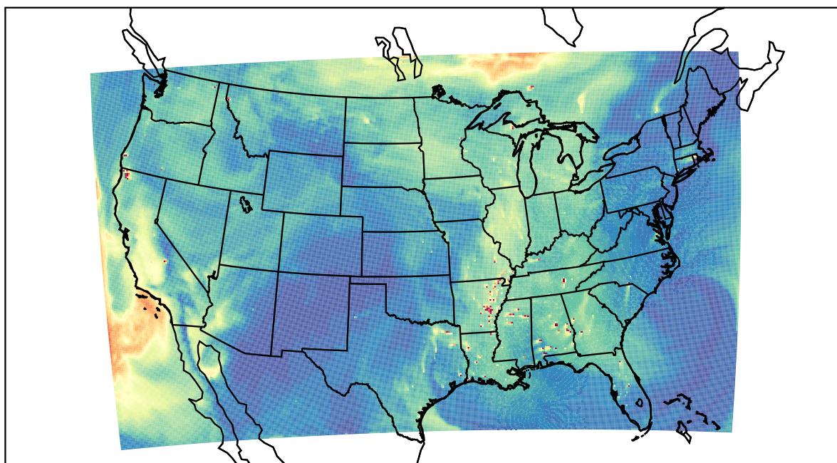
WRF 2023-09-22_21:00:00
