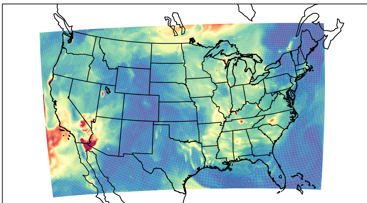
WRF 2023-09-22_08:00:00
