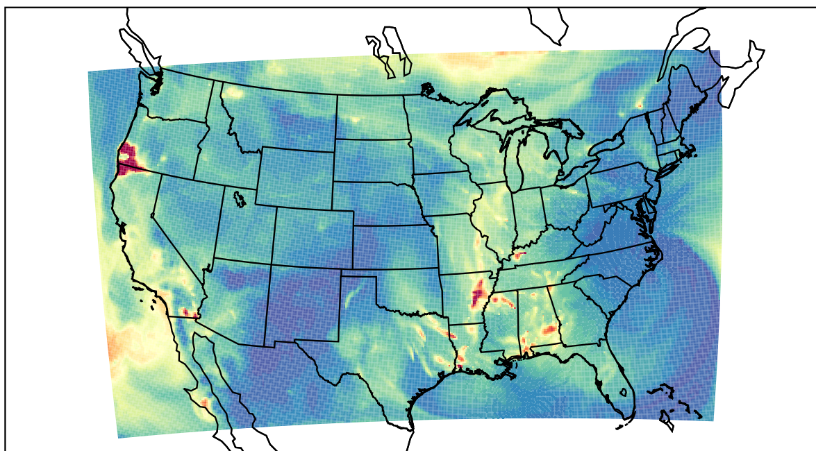
WRF 2023-09-23_07:00:00
