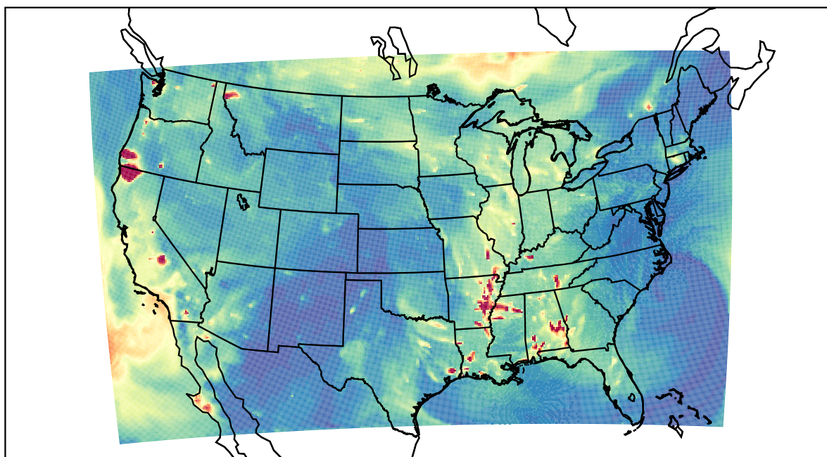
WRF 2023-09-23_03:00:00
