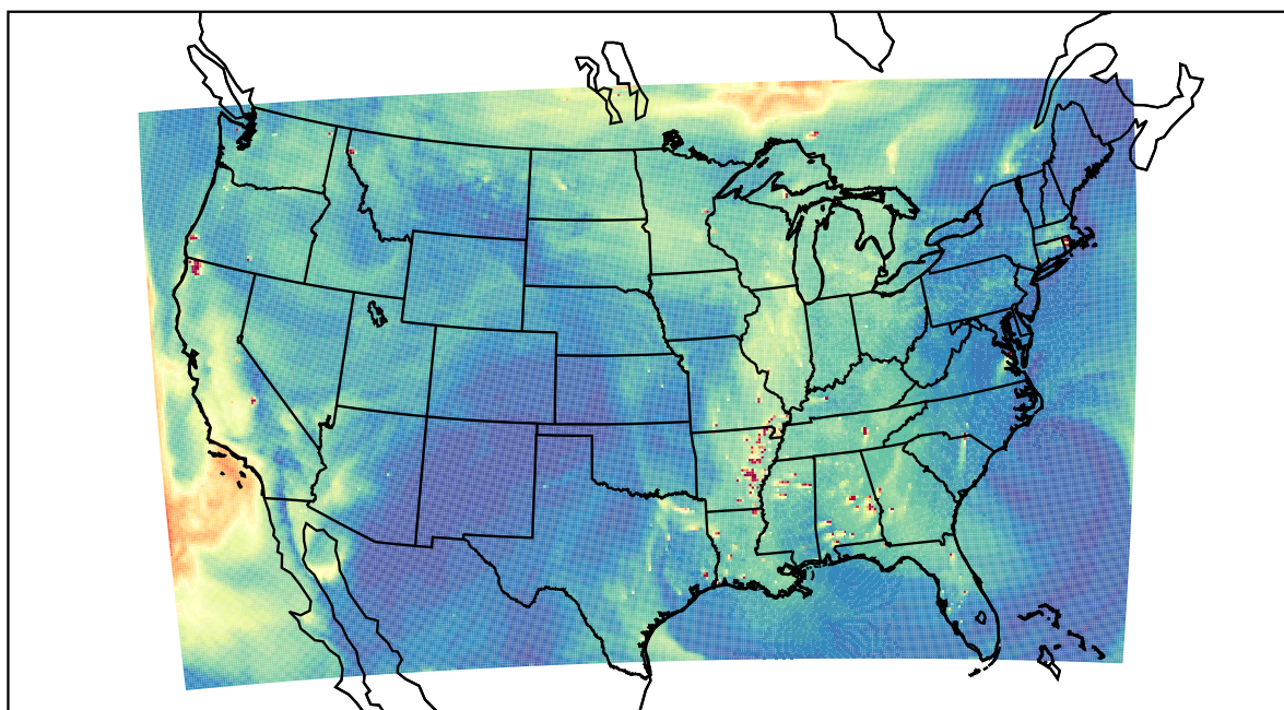
WRF 2023-09-22_22:00:00
