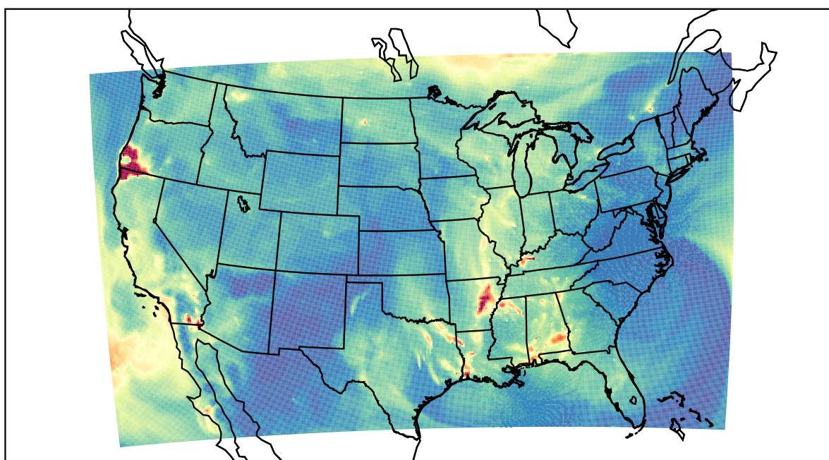
WRF 2023-09-23_08:00:00
