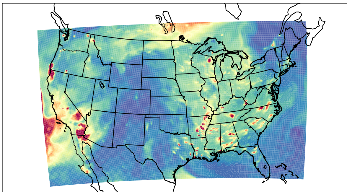
WRF 2023-09-22_03:00:00
