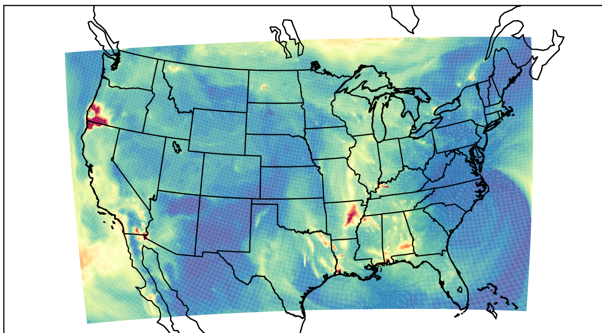
WRF 2023-09-23_09:00:00
