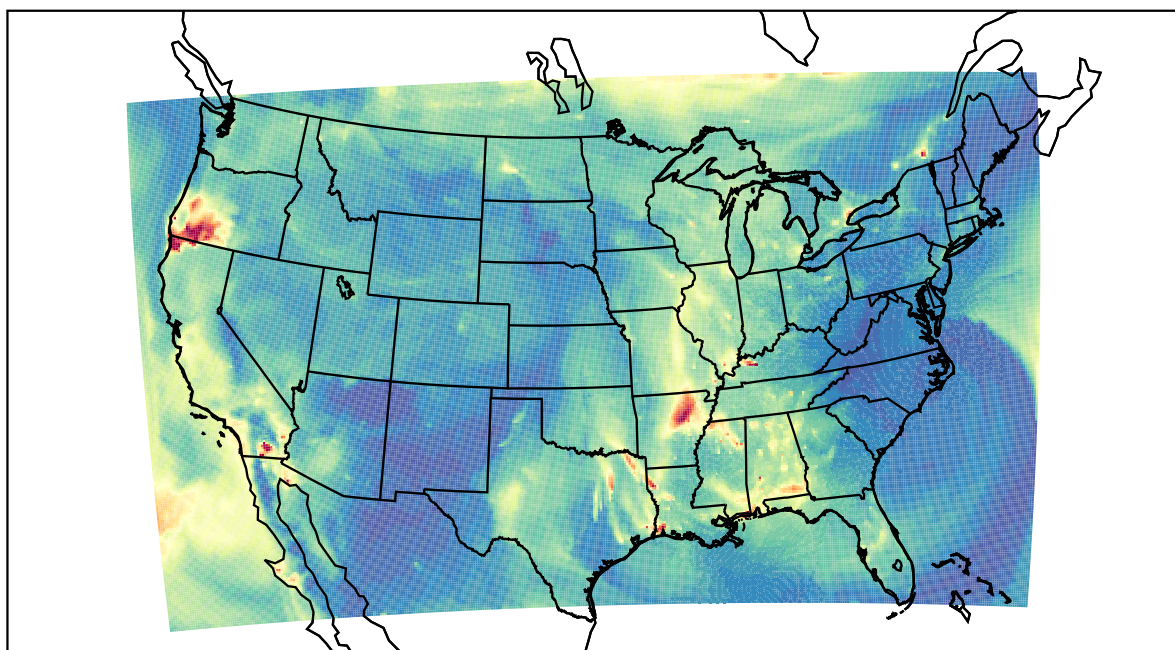
WRF 2023-09-23_12:00:00
