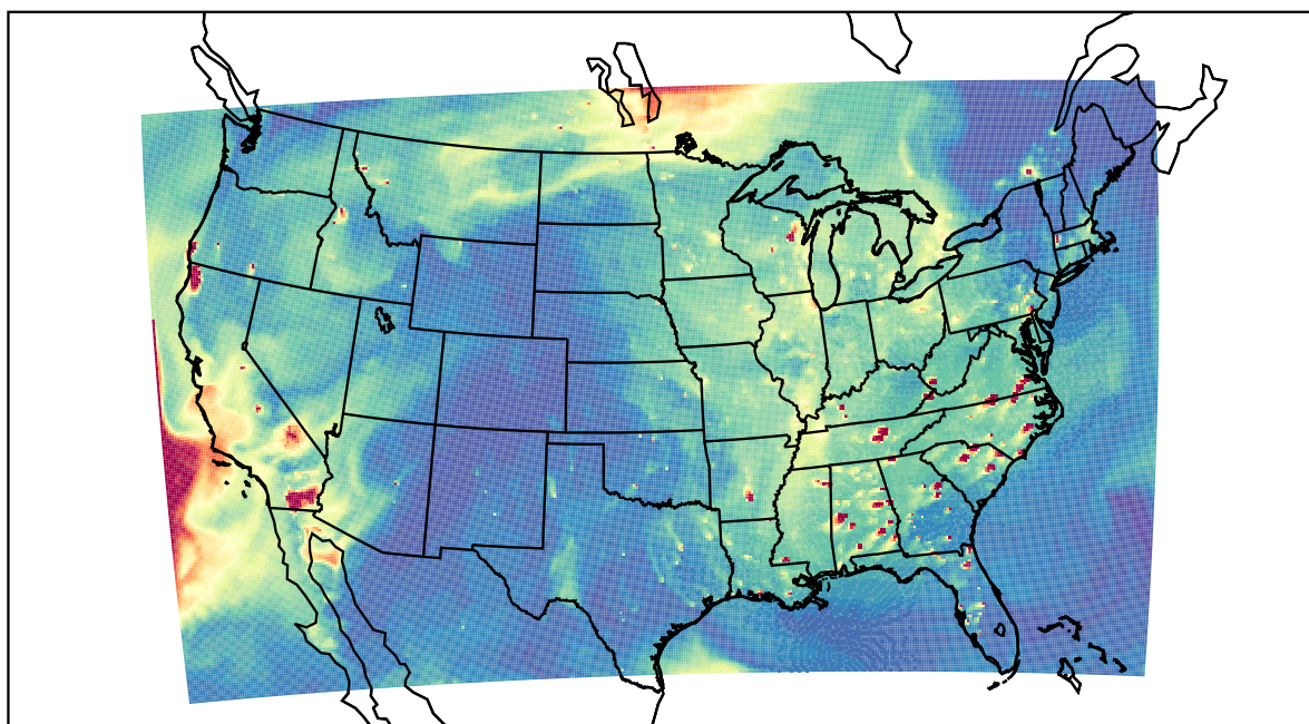
WRF 2023-09-22_00:00:00
