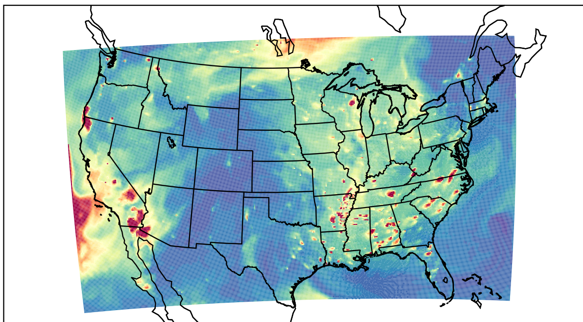
WRF 2023-09-22_02:00:00
