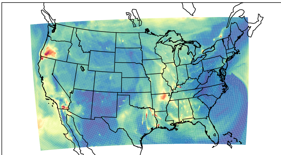
WRF 2023-09-23_14:00:00
