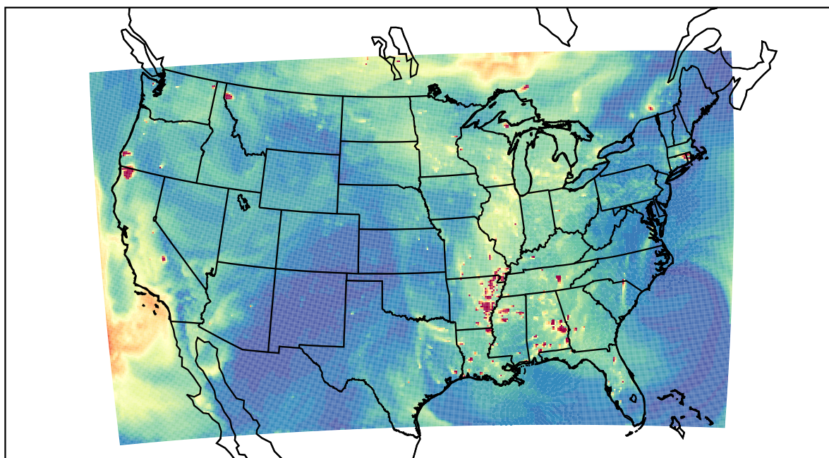
WRF 2023-09-23_00:00:00
