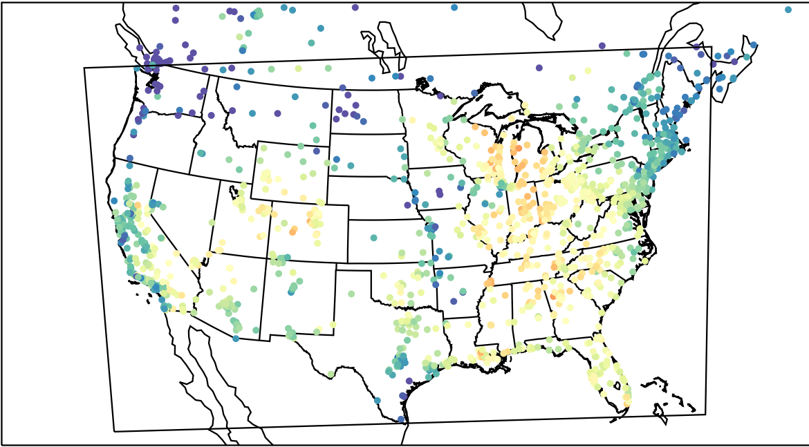
AirNOW (2023-09-22_17:00:00)
