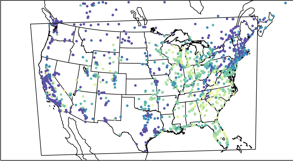
AirNOW (2023-09-22_14:00:00)
