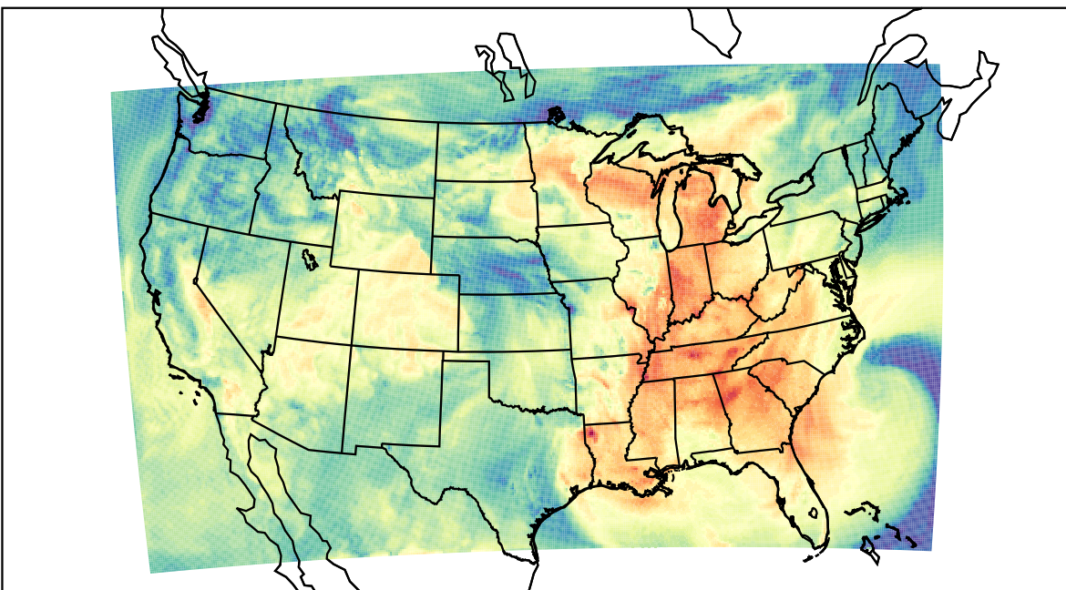
WRF (2023-09-22_17:00:00)
