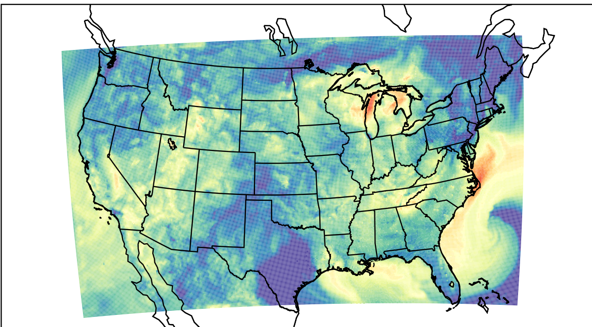
WRF (2023-09-22_08:00:00)
