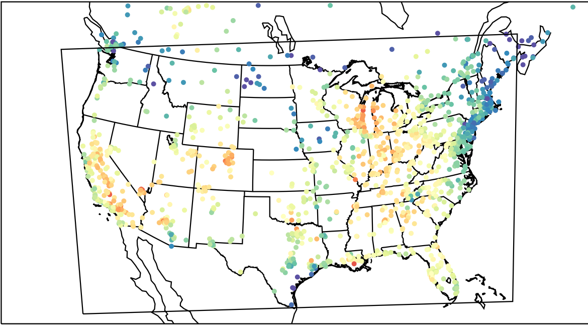
AirNOW (2023-09-22_21:00:00)
