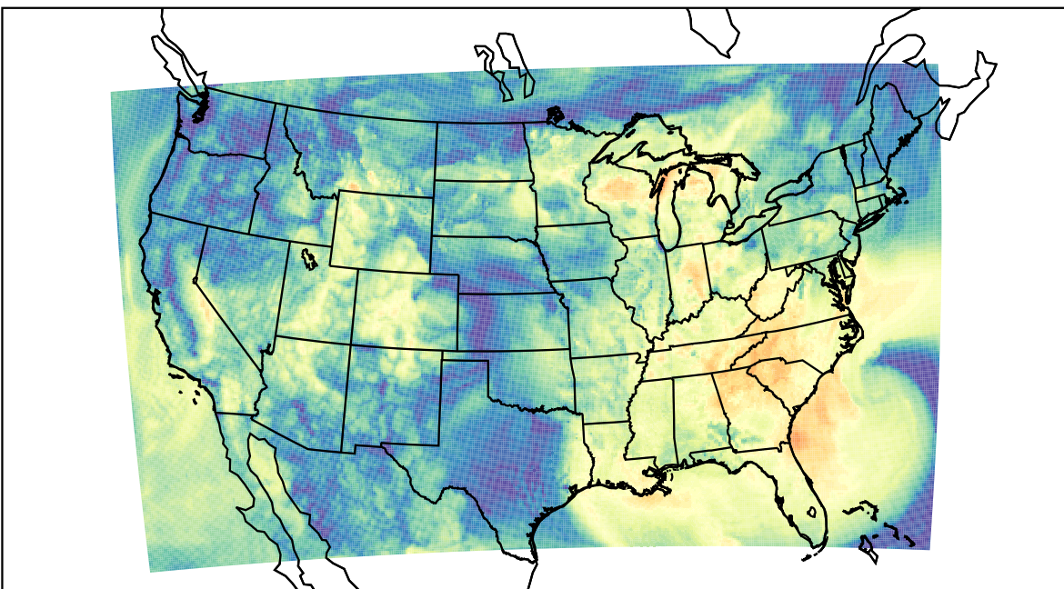
WRF (2023-09-22_15:00:00)
