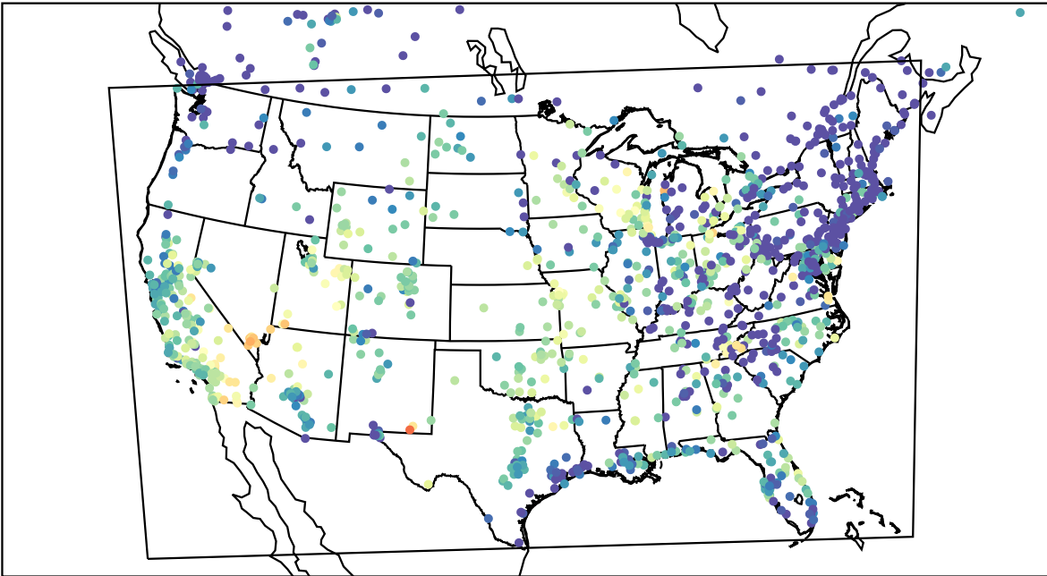
AirNOW (2023-09-22_03:00:00)
