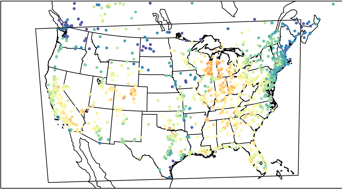
AirNOW (2023-09-22_19:00:00)
