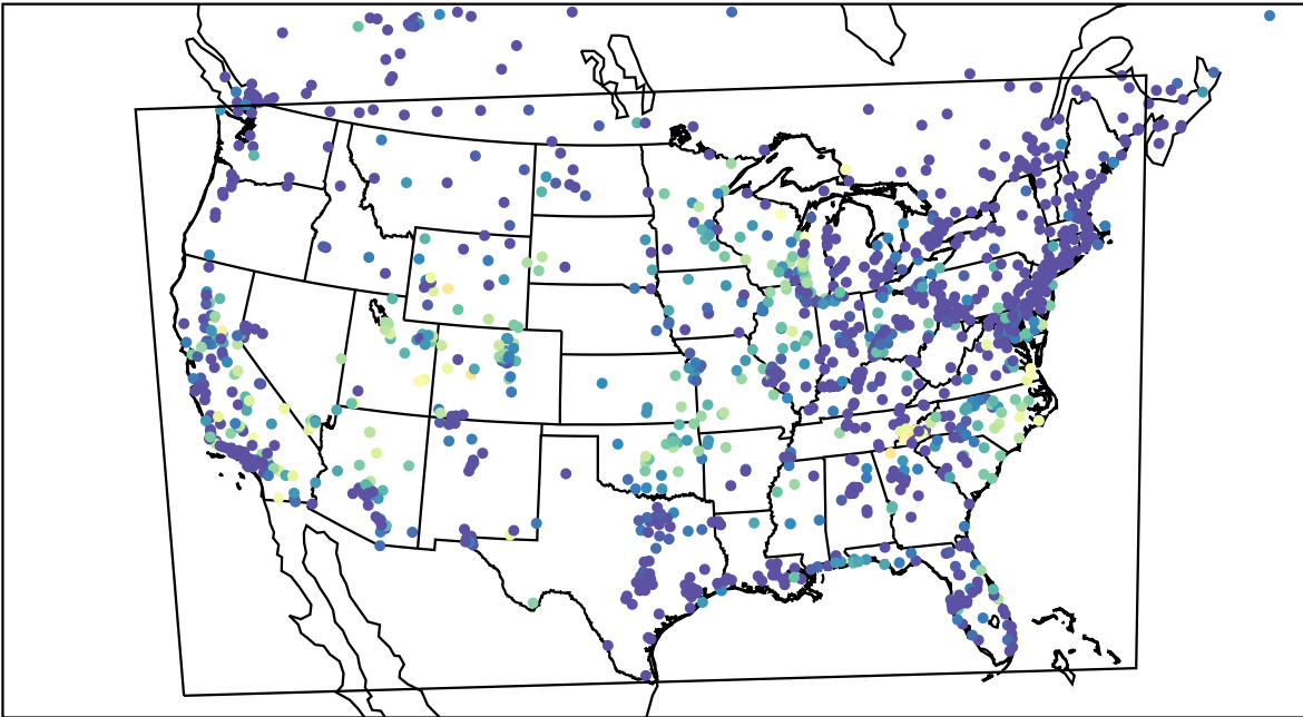
AirNOW (2023-09-22_11:00:00)
