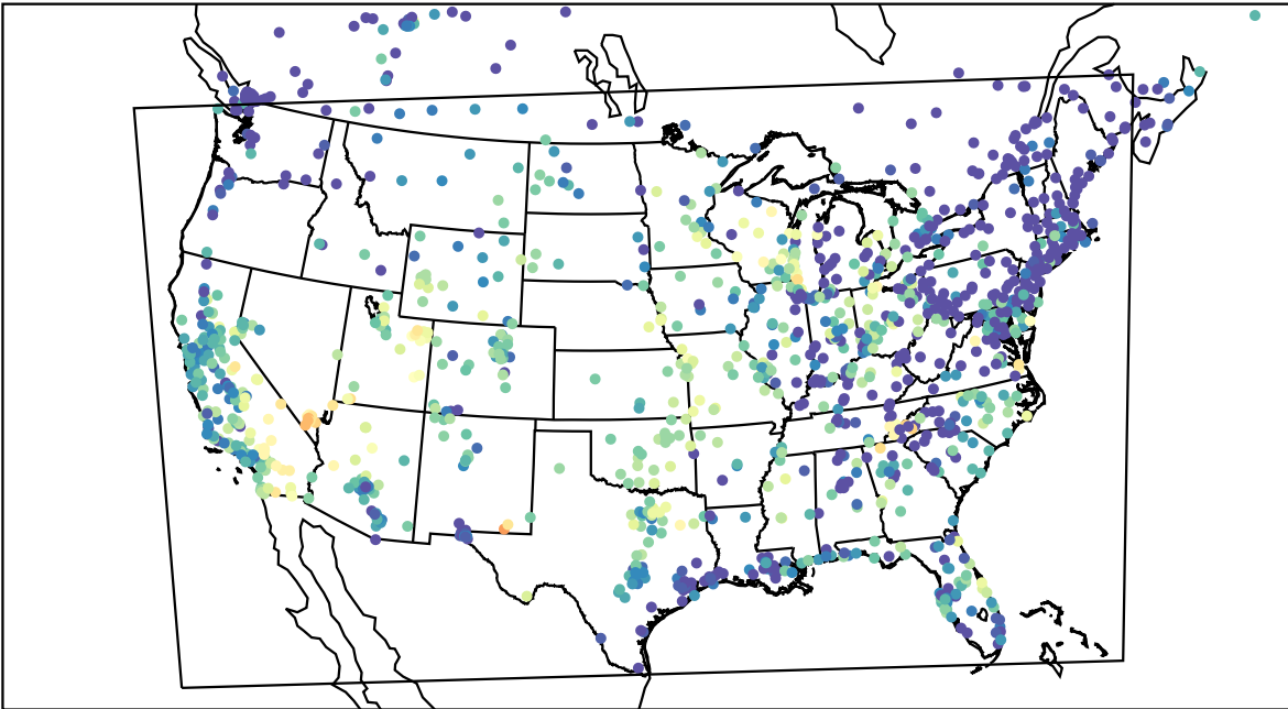
AirNOW (2023-09-22_04:00:00)
