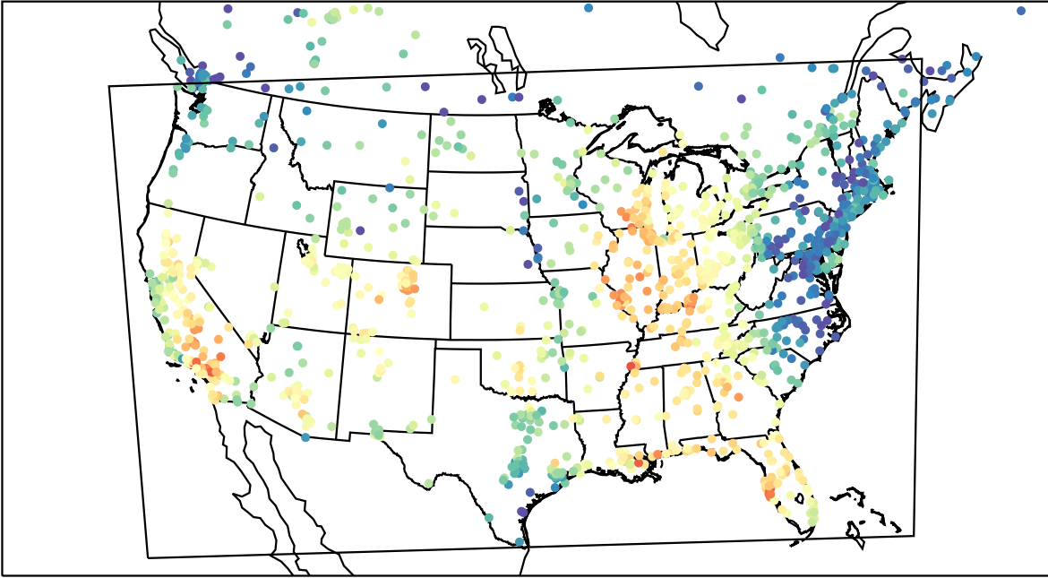
AirNOW (2023-09-23_19:00:00)
