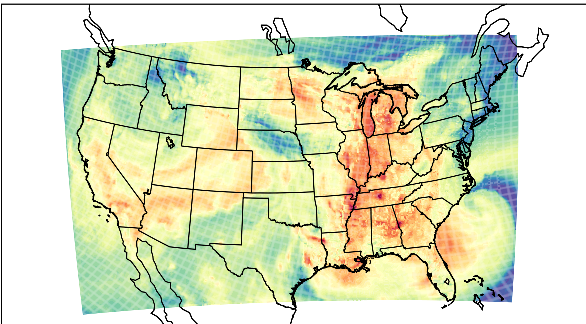
WRF (2023-09-22_22:00:00)
