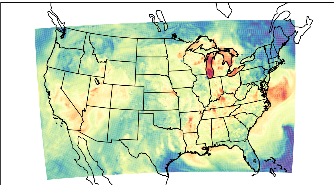
WRF (2023-09-22_00:00:00)
