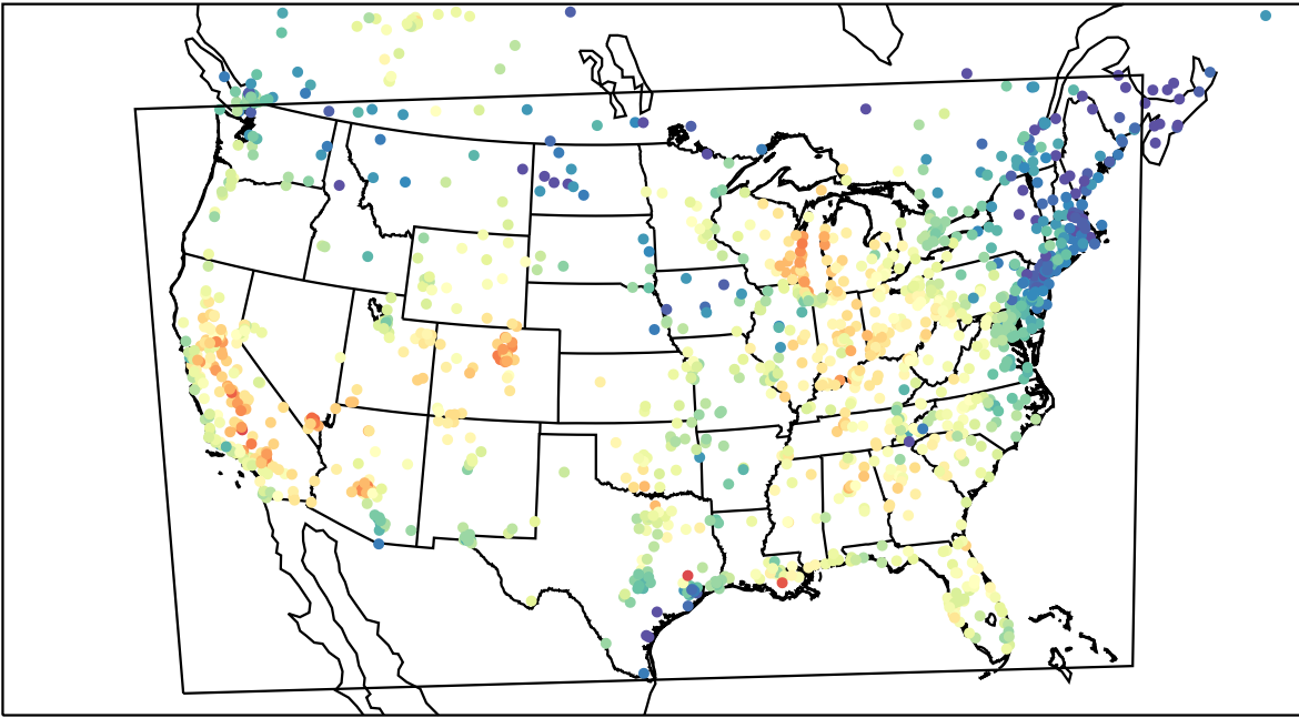
AirNOW (2023-09-22_22:00:00)
