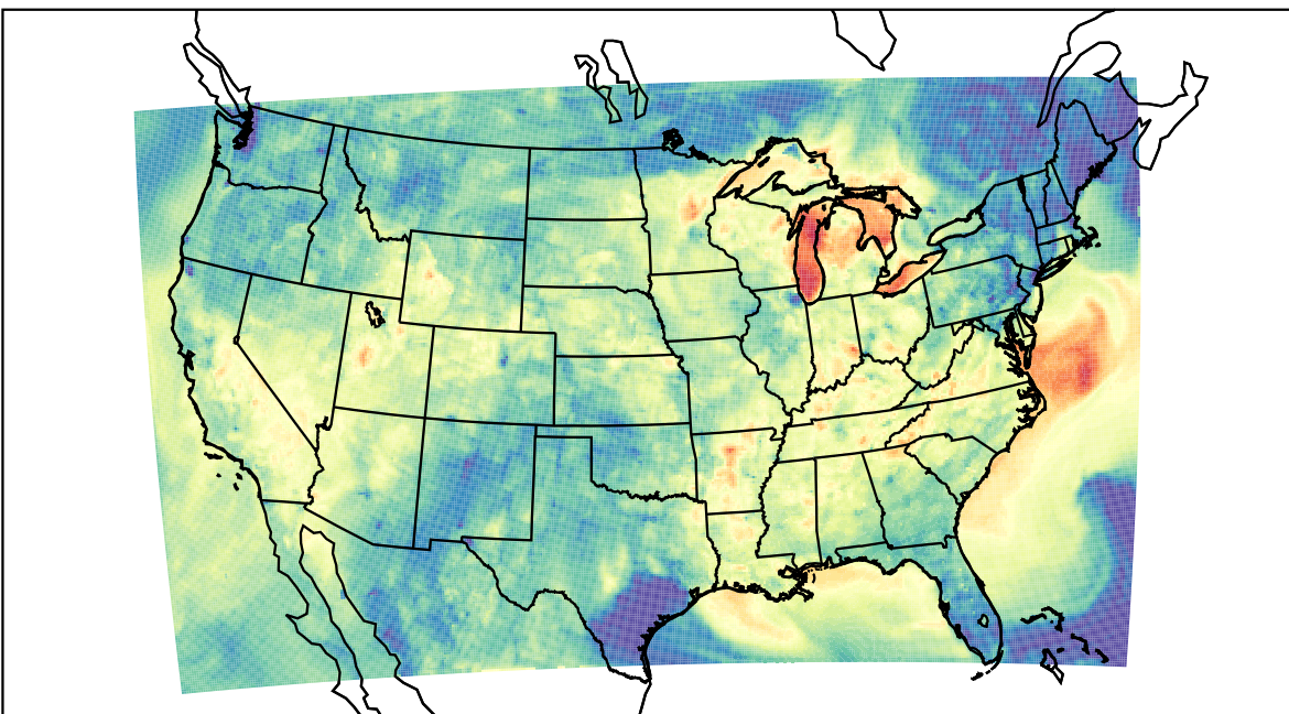
WRF (2023-09-22_02:00:00)
