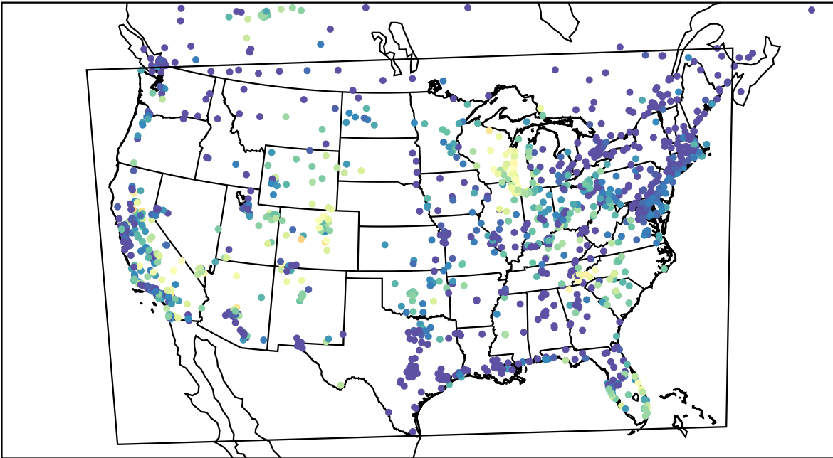
AirNOW (2023-09-23_08:00:00)
