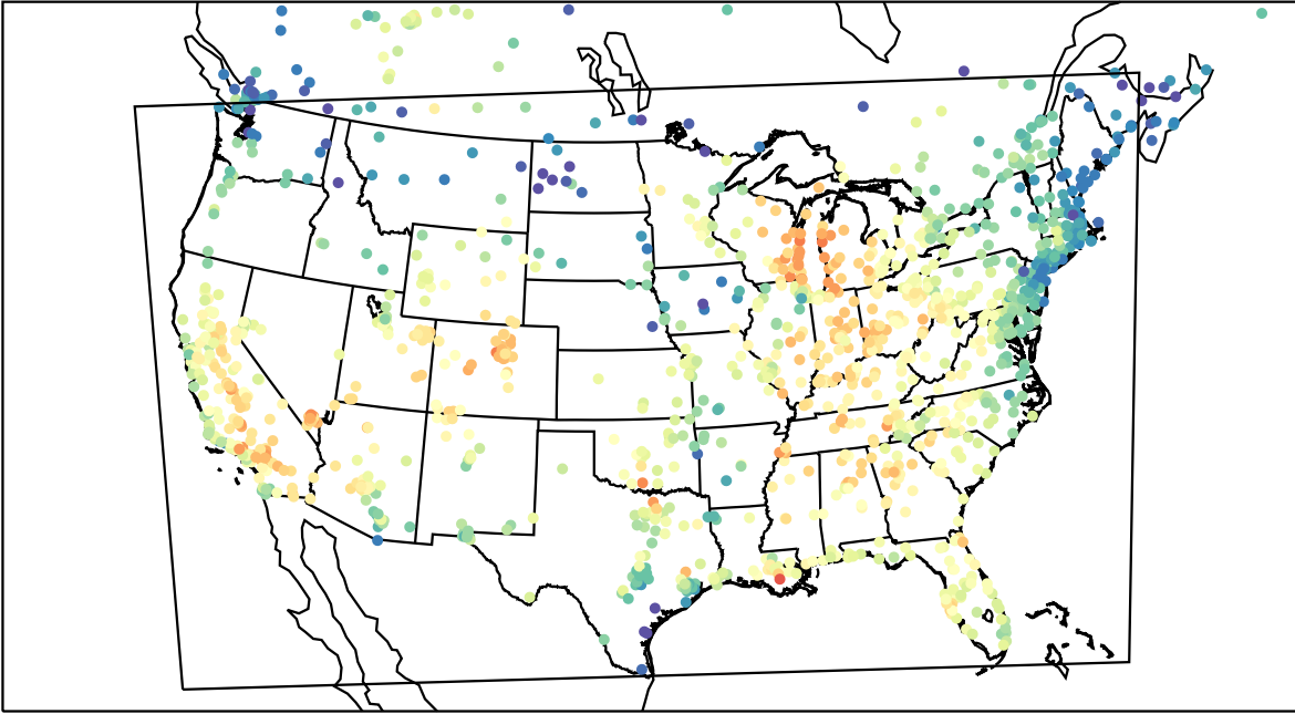
AirNOW (2023-09-22_20:00:00)
