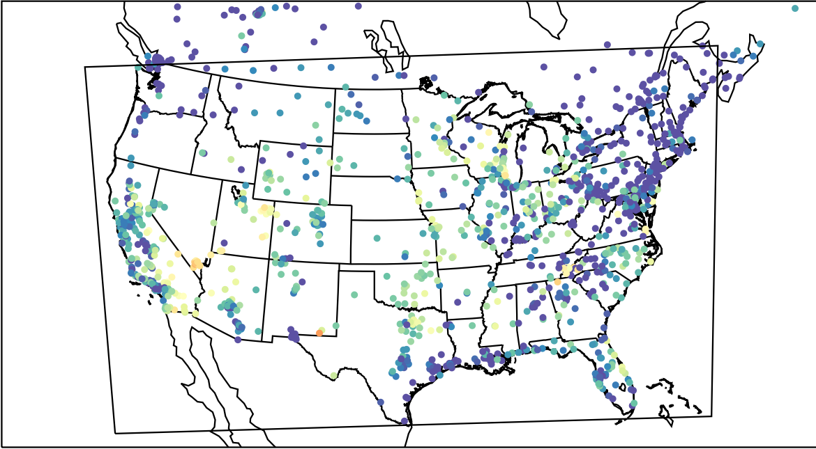
AirNOW (2023-09-22_05:00:00)
