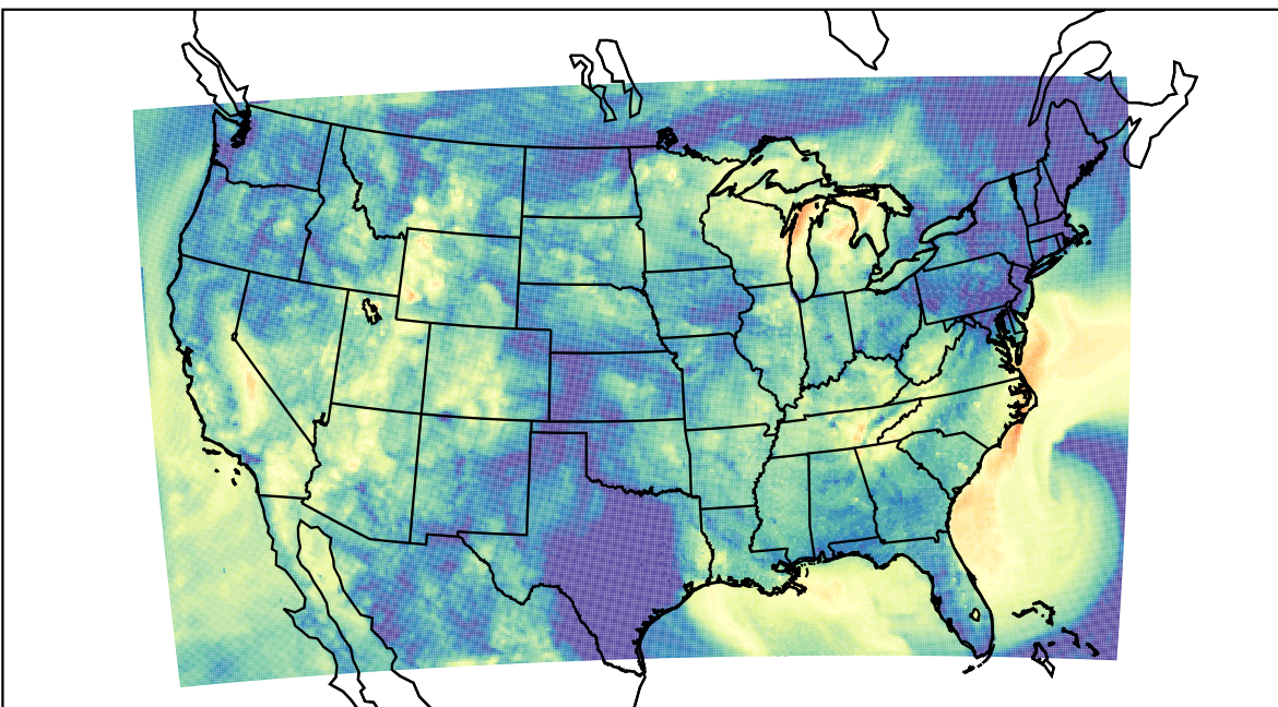
WRF (2023-09-22_11:00:00)
