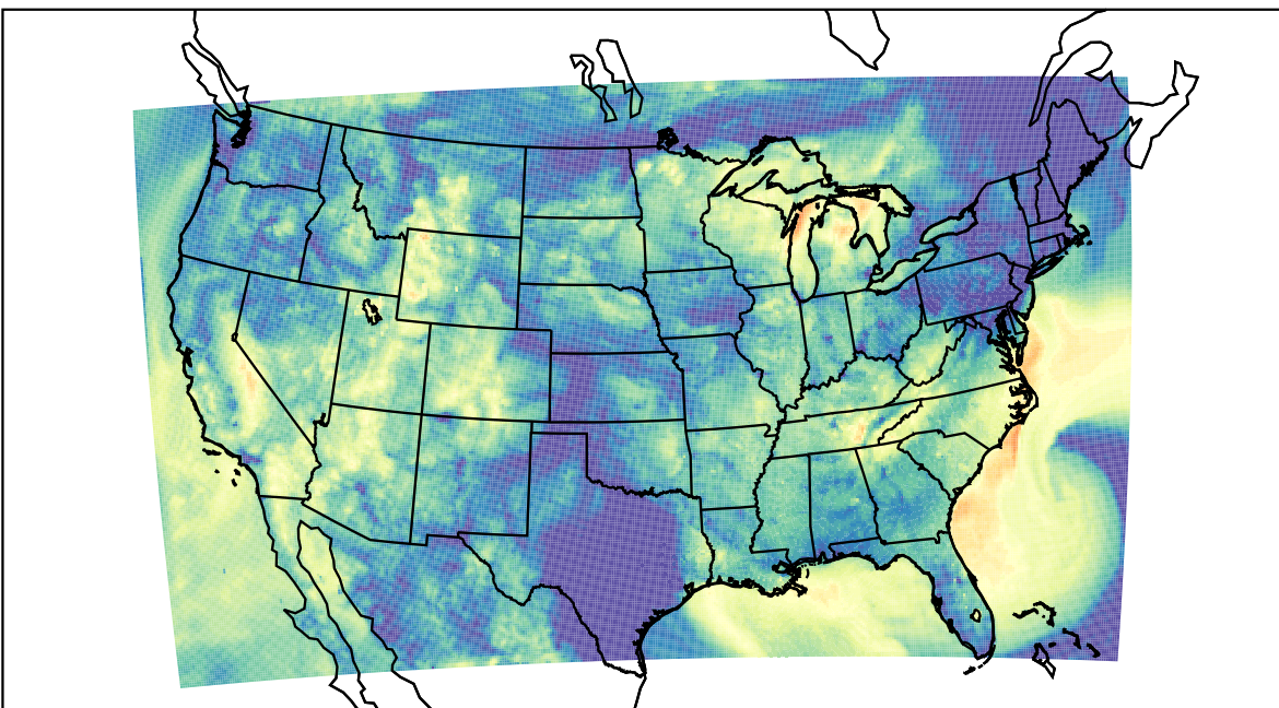
WRF (2023-09-22_12:00:00)
