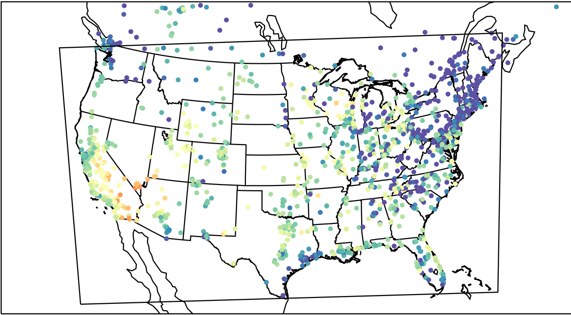
AirNOW (2023-09-22_01:00:00)
