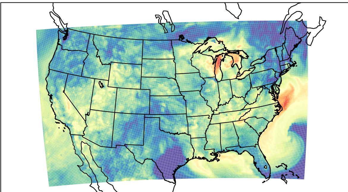
WRF (2023-09-22_06:00:00)
