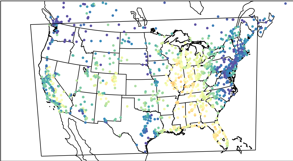
AirNOW (2023-09-23_16:00:00)
