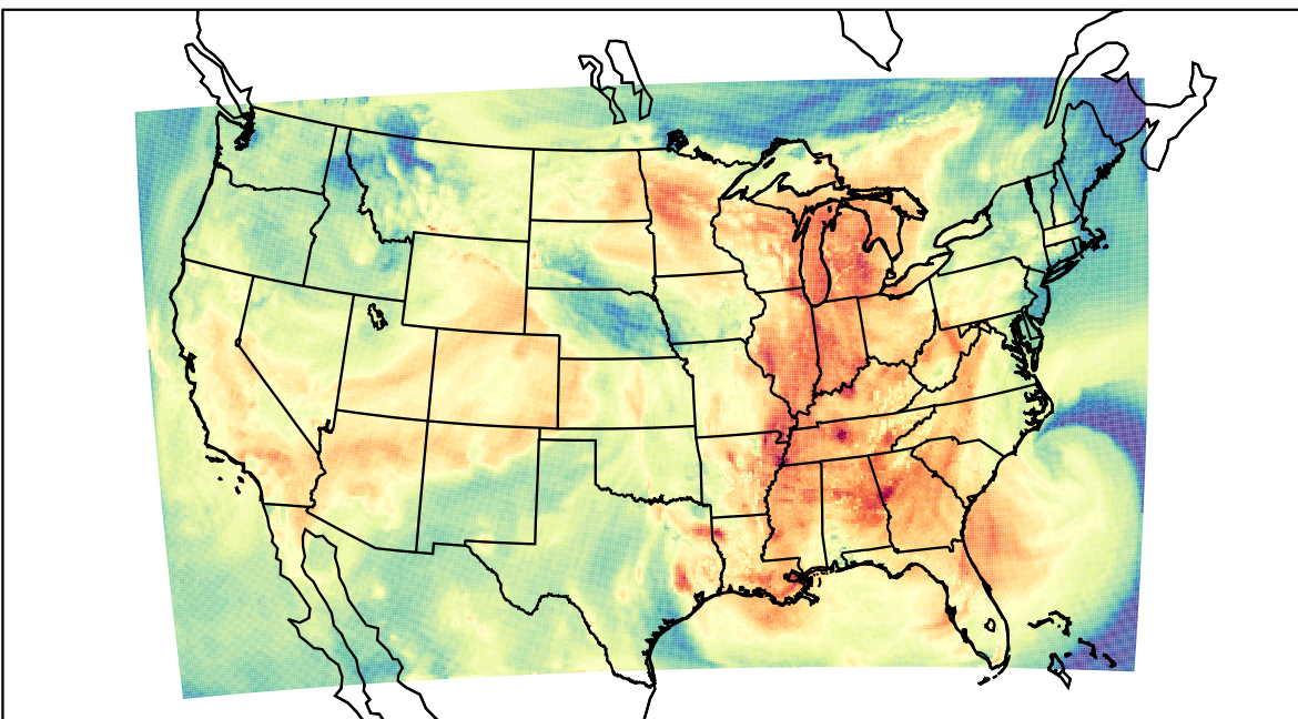
WRF (2023-09-22_21:00:00)
