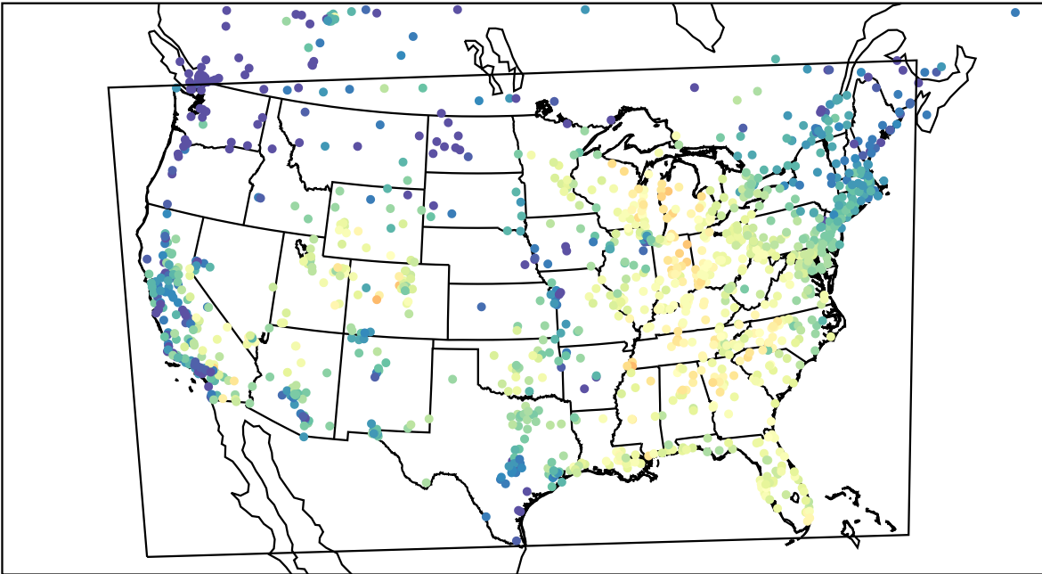
AirNOW (2023-09-22_16:00:00)
