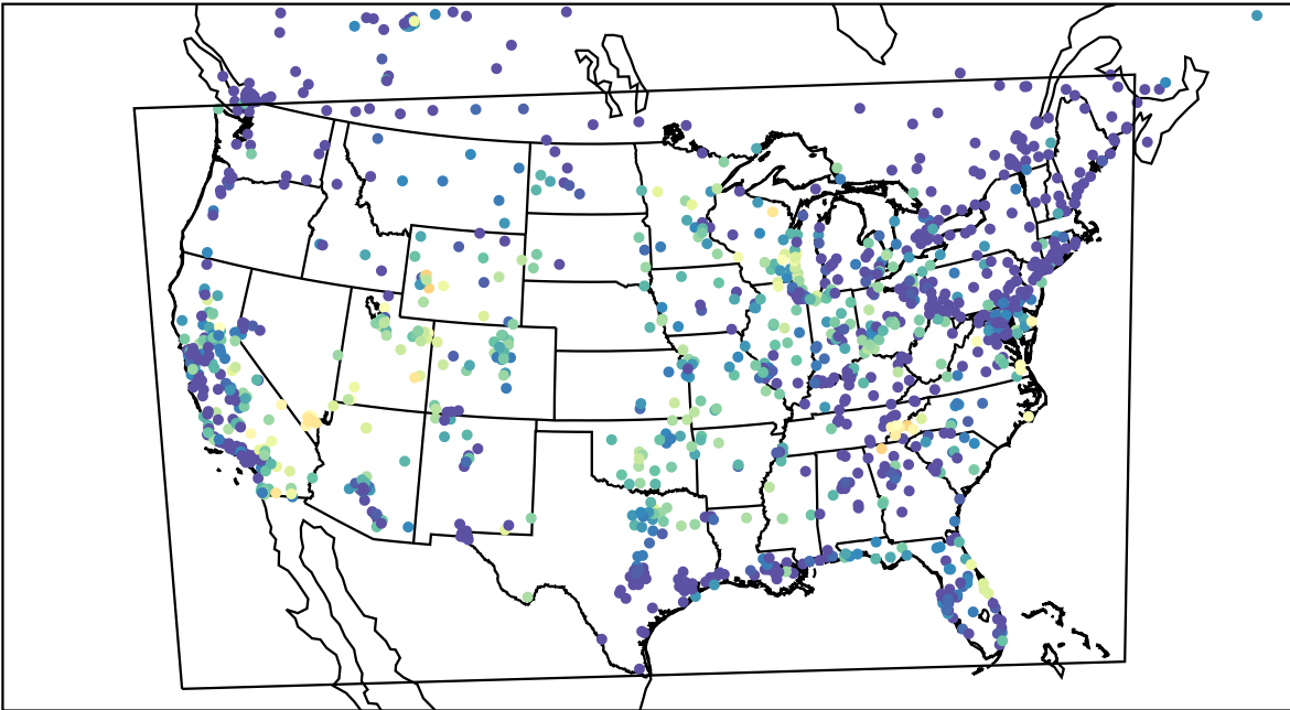
AirNOW (2023-09-22_08:00:00)
