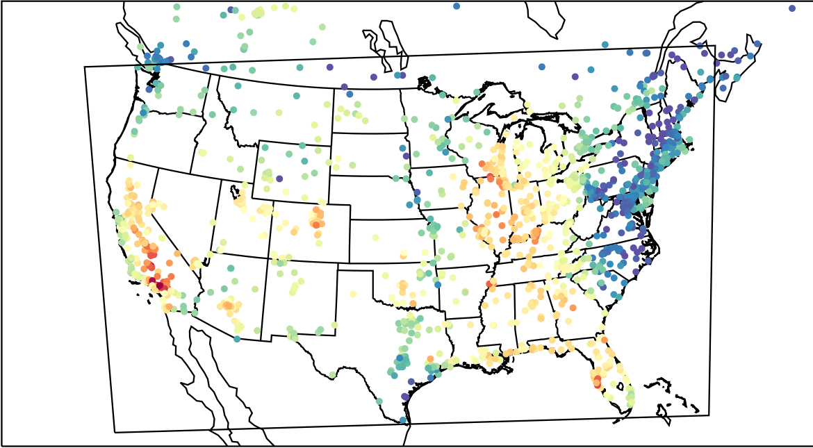
AirNOW (2023-09-23_21:00:00)
